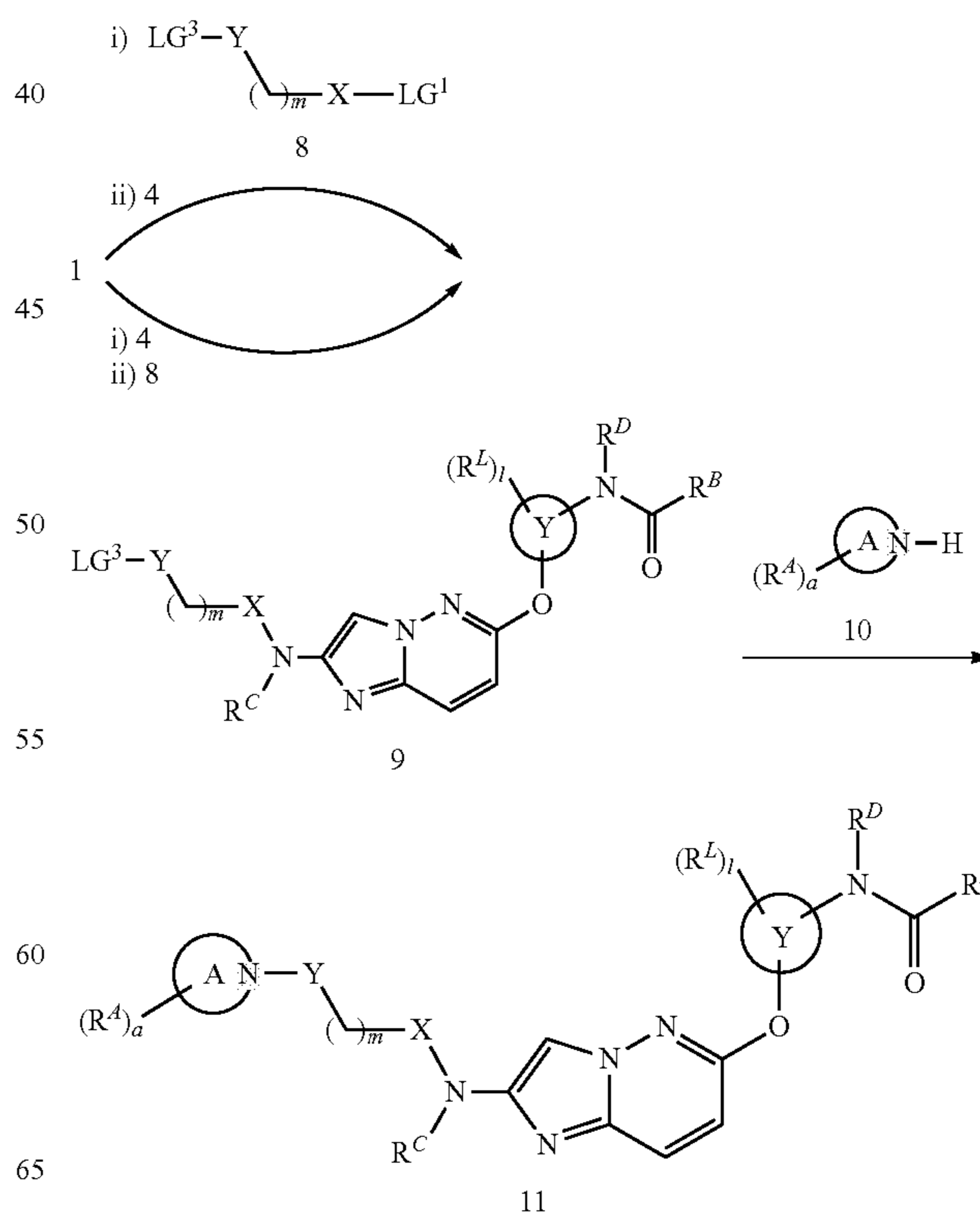
Scheme 2. Exemplary synthesis of certain compounds of Formula (I).
