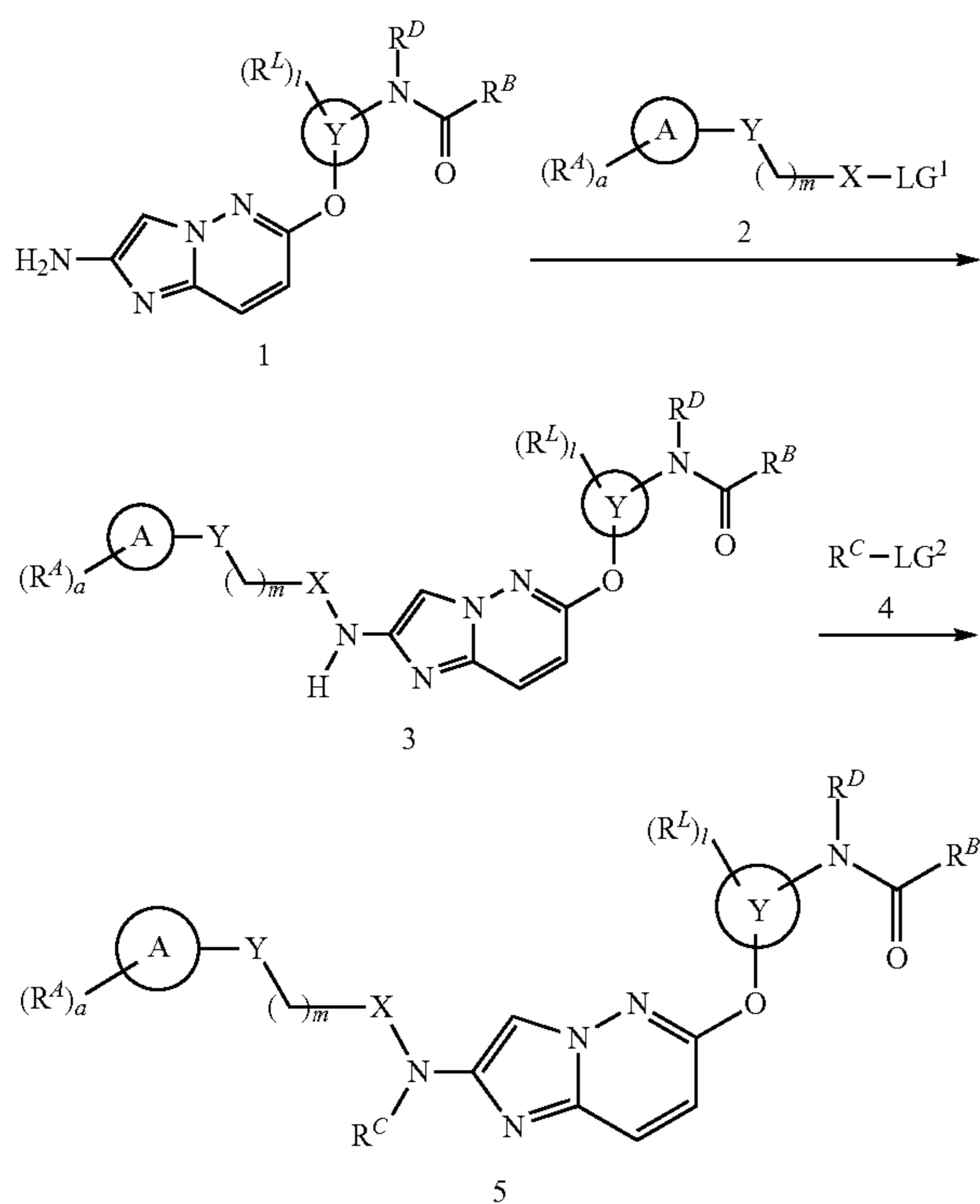
Scheme 1. Exemplary synthesis of compounds of Formula (I).
