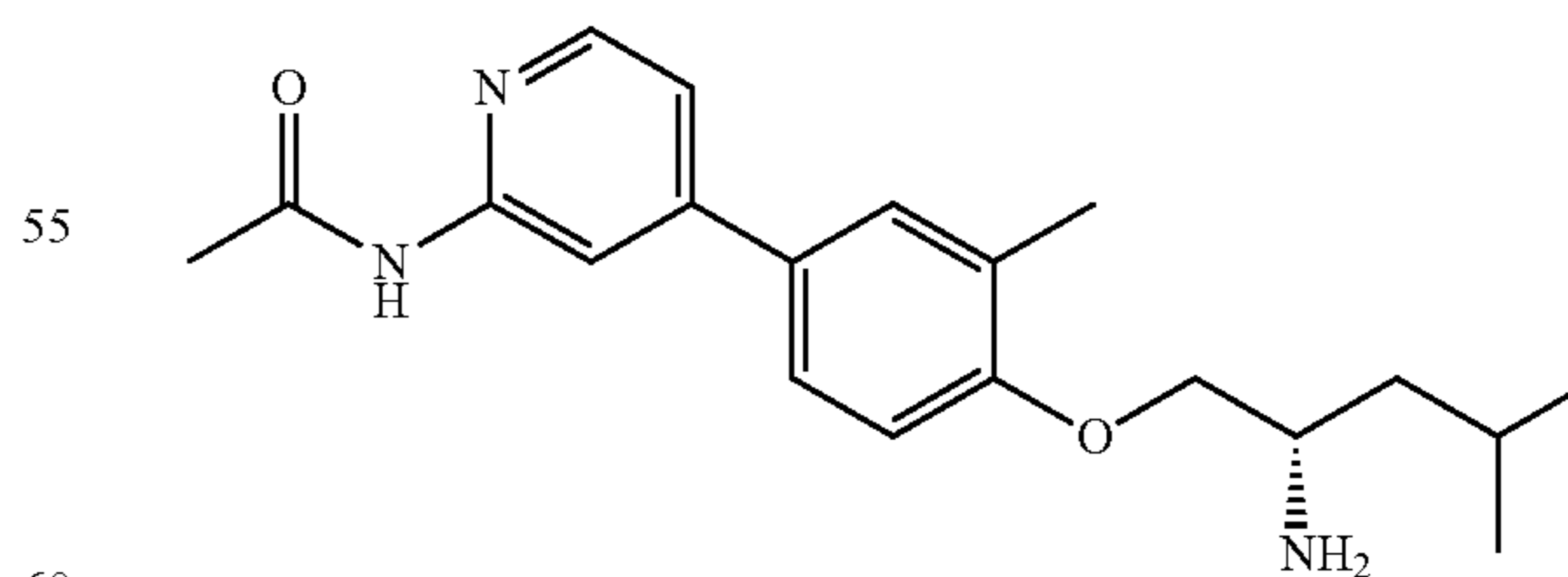
Part C: (S)-N-(4-(4-((2-amino-4-methylpentyl)oxy)-3-methylphenyl)pyridin-2-yl)acetamide
