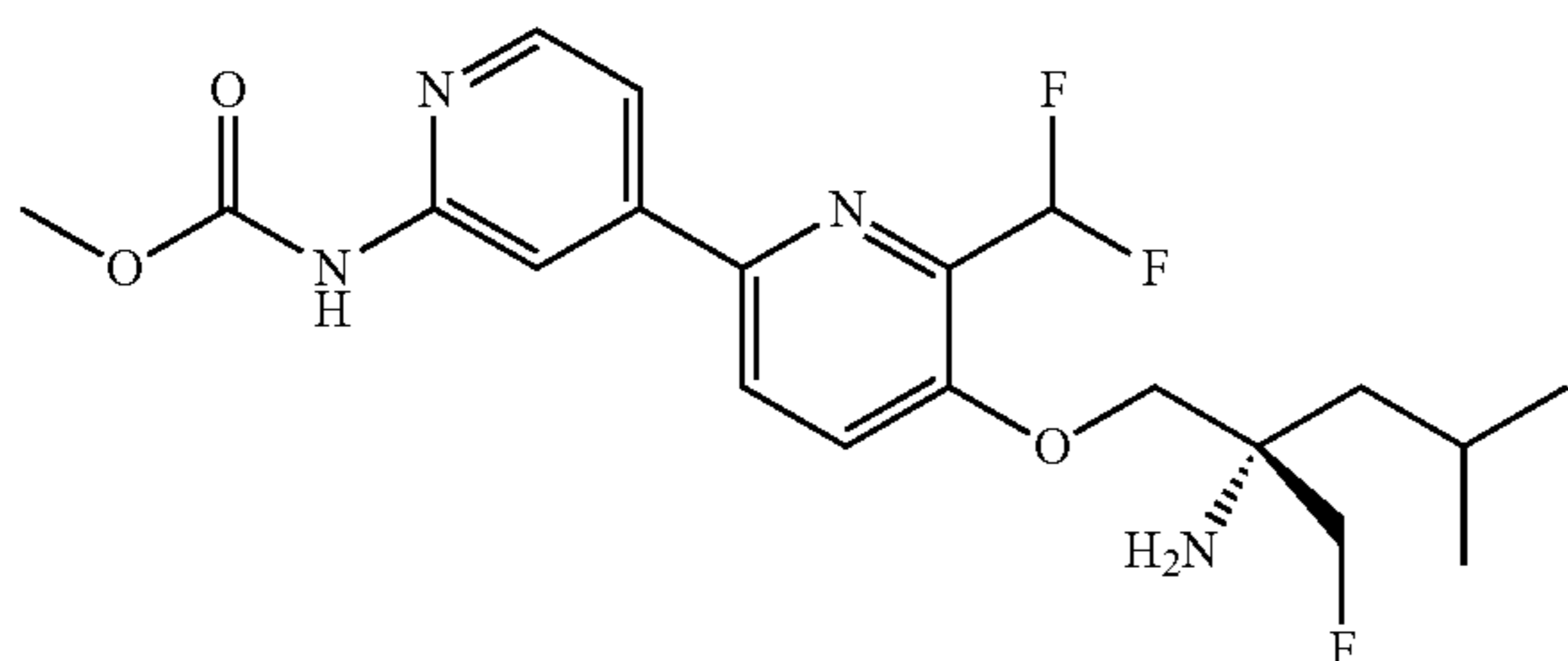
Part F: (S)-methyl (5-((2-amino-2-(fluoromethyl)-4-methylpentyl)oxy)-6-(difluoromethyl)-[2,4'-bipyridin]-2'-yl)carbamate
