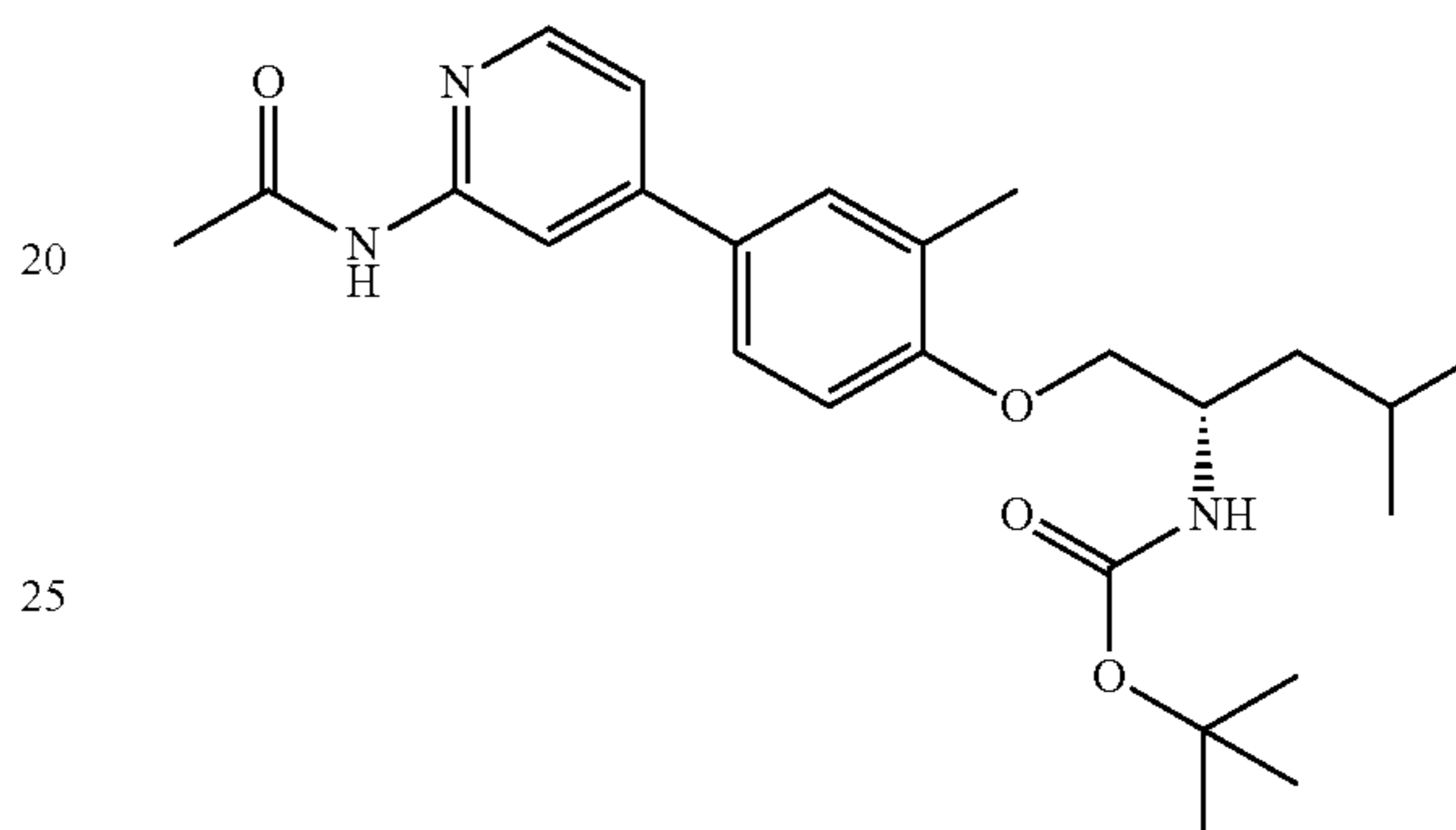
Part B: (S)-tert-butyl (1-(4-(2-acetamidopyridin-4-yl)-2-methylphenoxy)-4-methylpentan-2-yl)carbamate
