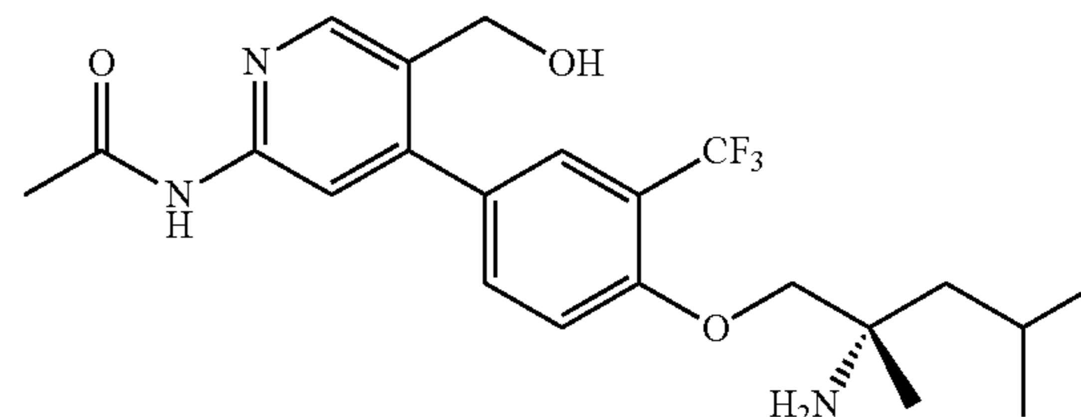
Part C: (S)-N-(4-(4-((2-amino-2,4-dimethylpentyl)oxy)-3-(trifluoromethyl)phenyl)-5-(hydroxymethyl)pyridin-2-yl)acetamide
