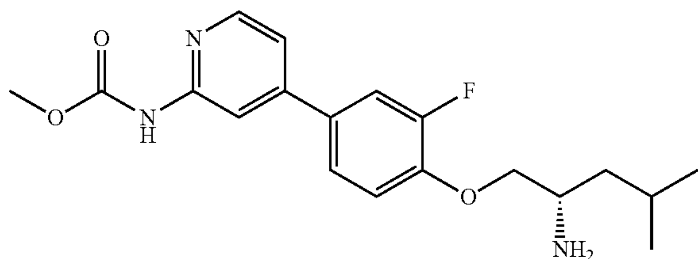
Part C: (S)-methyl (4-(4-((2-amino-4-methylpentyl)oxy)-3-fluorophenyl)pyridin-2-yl)carbamate
