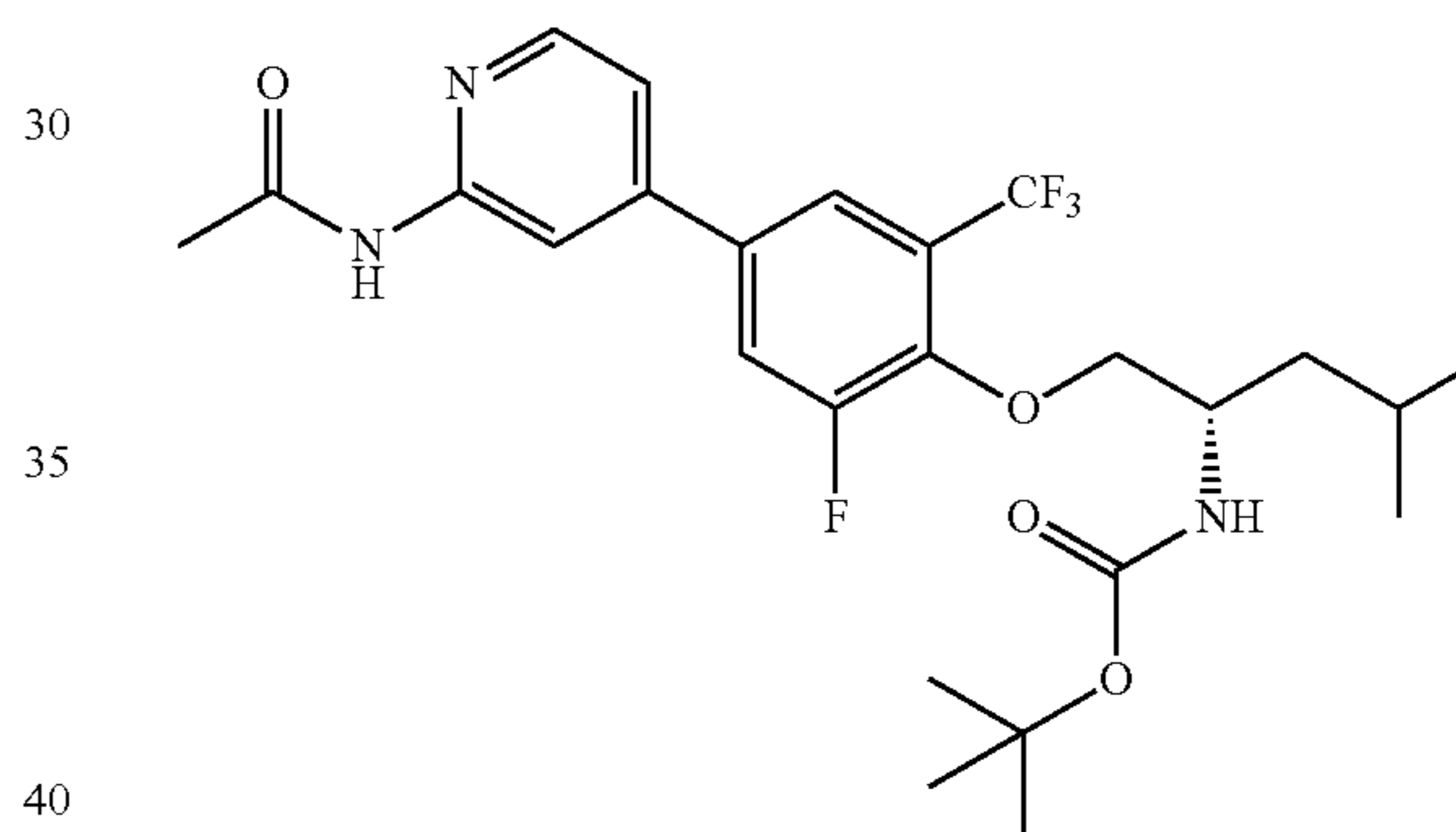
Part B: (S)-tert-butyl (1-(4-(2-acetamidopyridin-4-yl)-2-fluoro-6-(trifluoromethyl)phenoxy)-4-methylpentan-2-yl) carbamate
