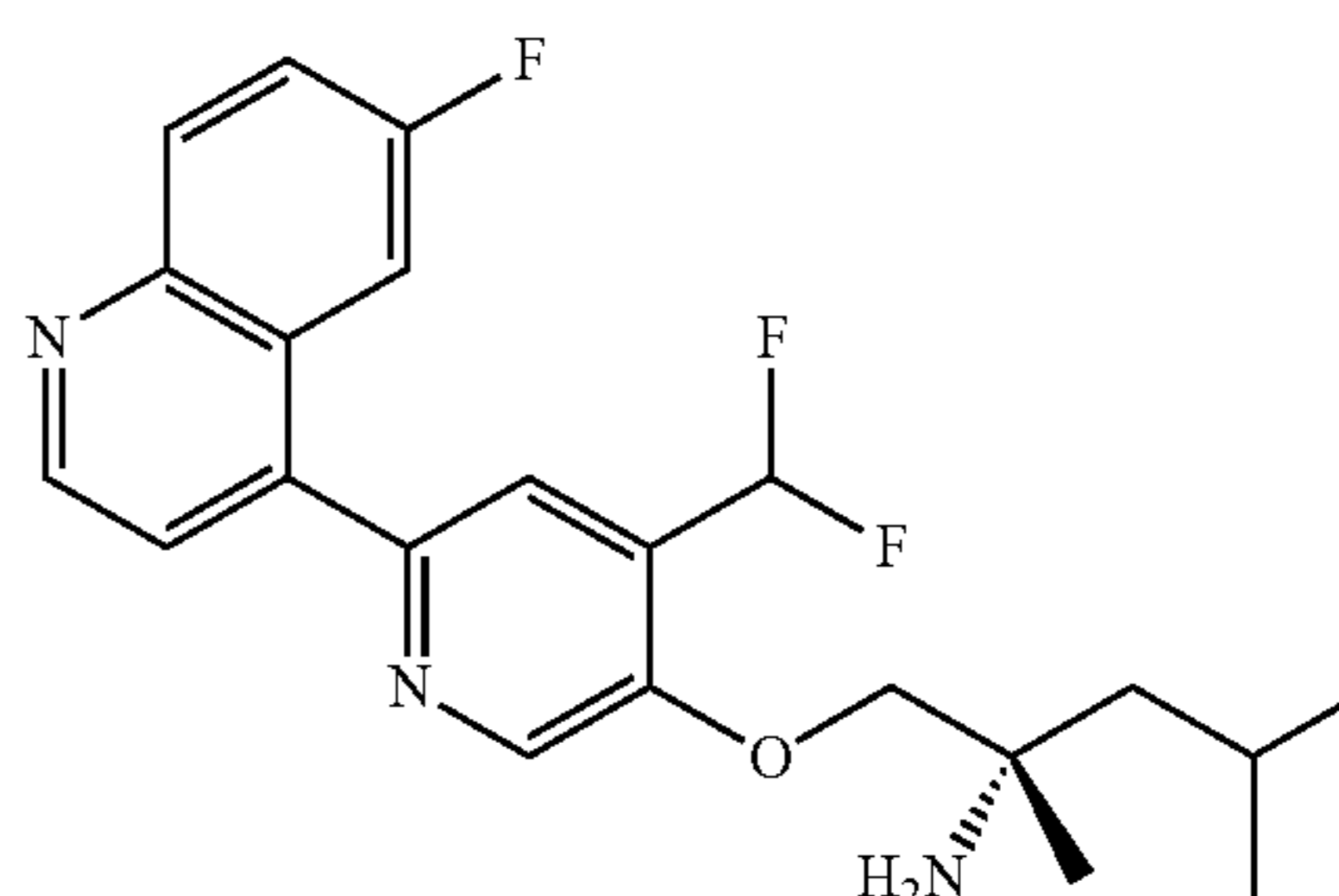
Part B: (S)-1-((4-(difluoromethyl)-6-(6-fluoroquinolin-4-yl)pyridin-3-yl)oxy)-2,4-dimethylpentan-2-amine
