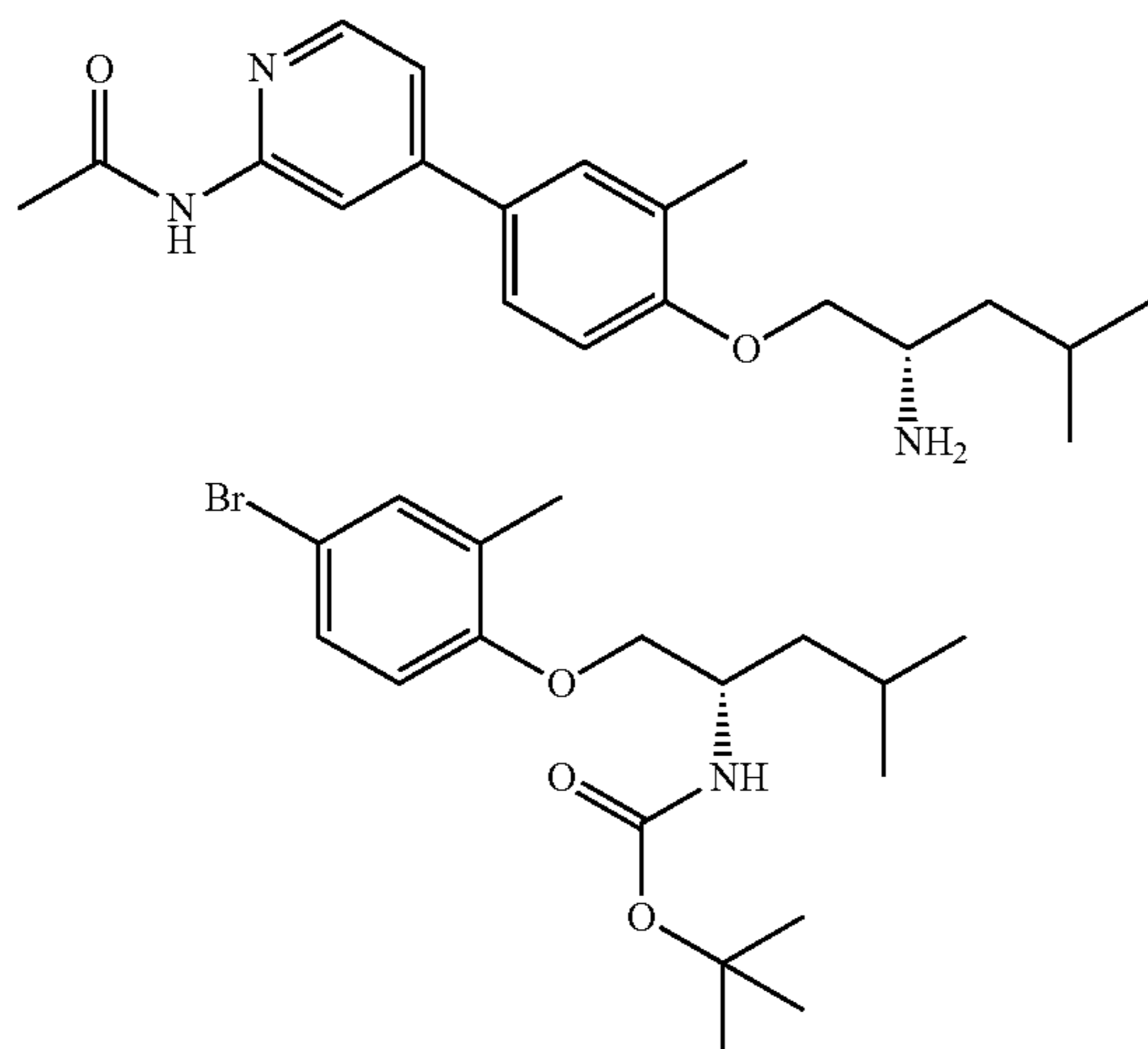
Part A: (S)-tert-butyl (1-(4-(2-acetamidopyridin-4-yl)-2-methylphenoxy)-4-methylpentan-2-yl)carbamate
