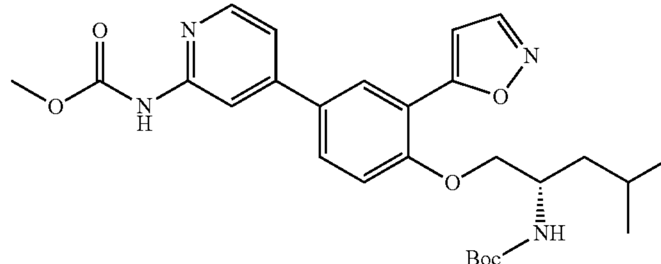
Part B: (S)-methyl (4-(4-((2-Boc-amino-4-methylpentyl)oxy)-3-(isoxazol-5-yl)phenyl)pyridin-2-yl)carbamate
