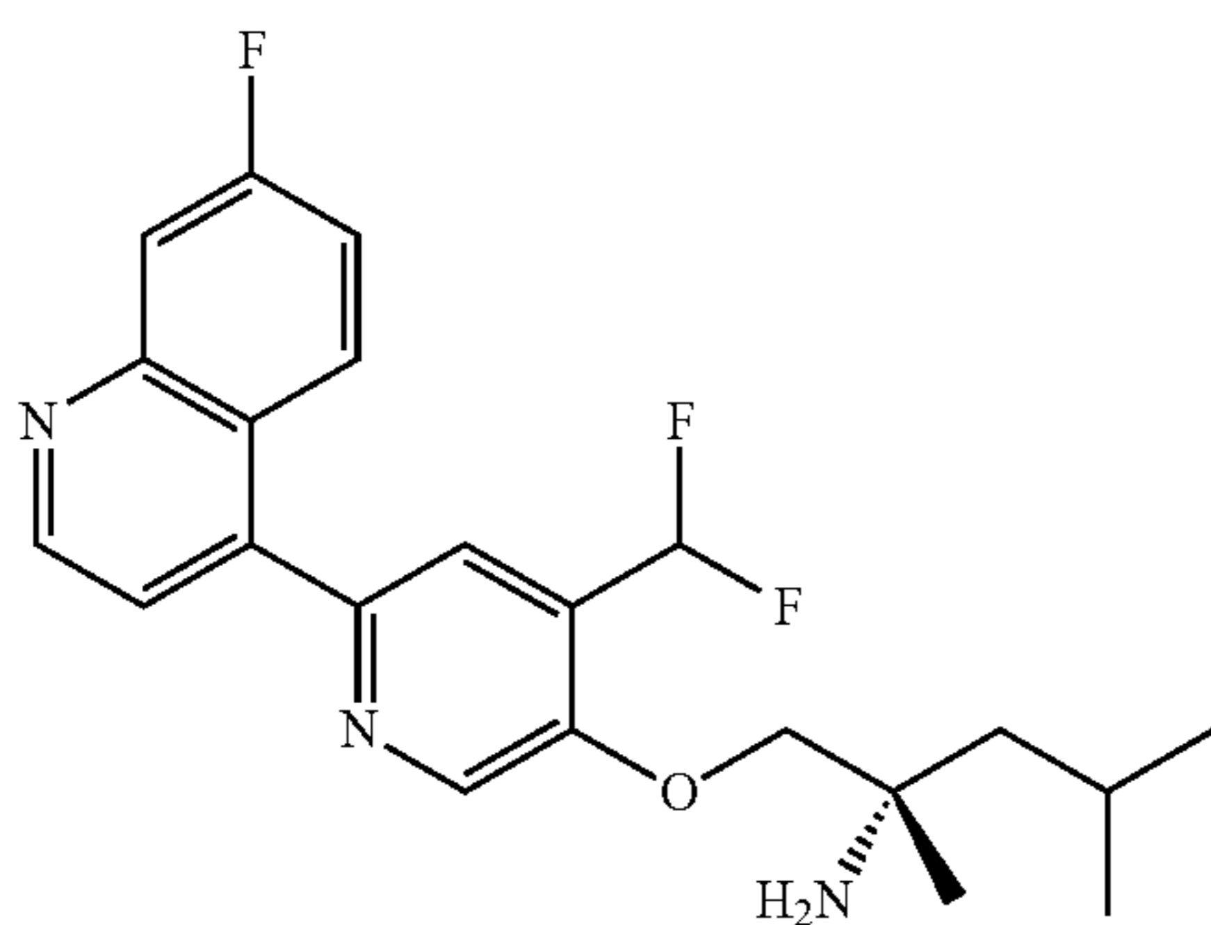
Part B: (S)-1-((4-(difluoromethyl)-6-(7-fluoroquinolin-4-yl)pyridin-3-yl)oxy)-2,4-dimethylpentan-2-amine
