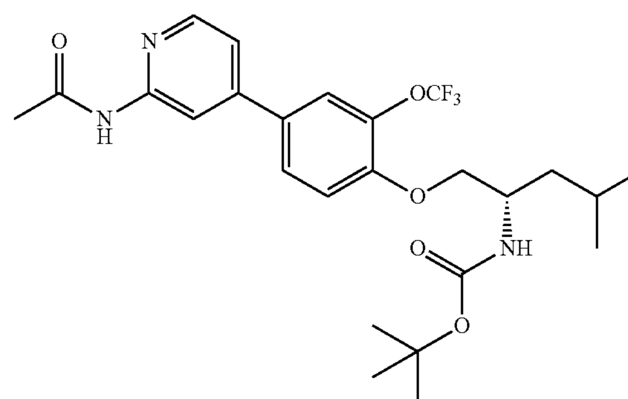
Part B: (S)-tert-butyl (1-(4-(2-acetamidopyridin-4-yl)-2-(trifluoromethoxy)phenoxy)-4-methylpentan-2-yl)carbamate
