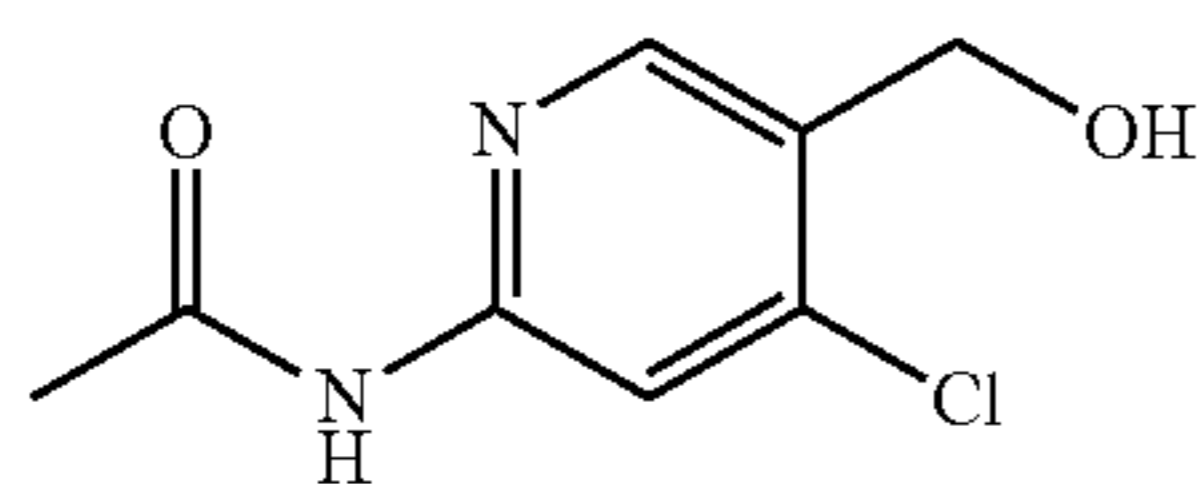
Part A: N-(4-chloro-5-(hydroxymethyl)pyridin-2-yl)acetamide
