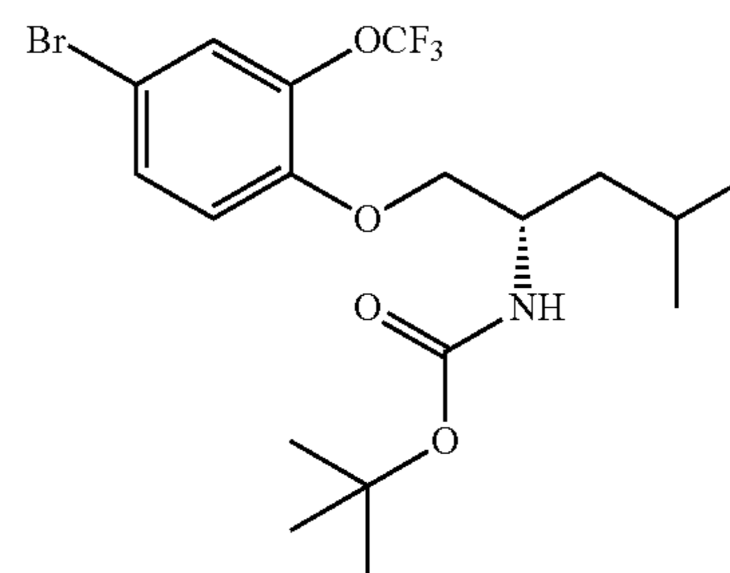
Part A: (S)-tert-butyl (1-(4-bromo-2-(trifluoromethoxy)phenoxy)-4-methylpentan-2-yl)carbamate
