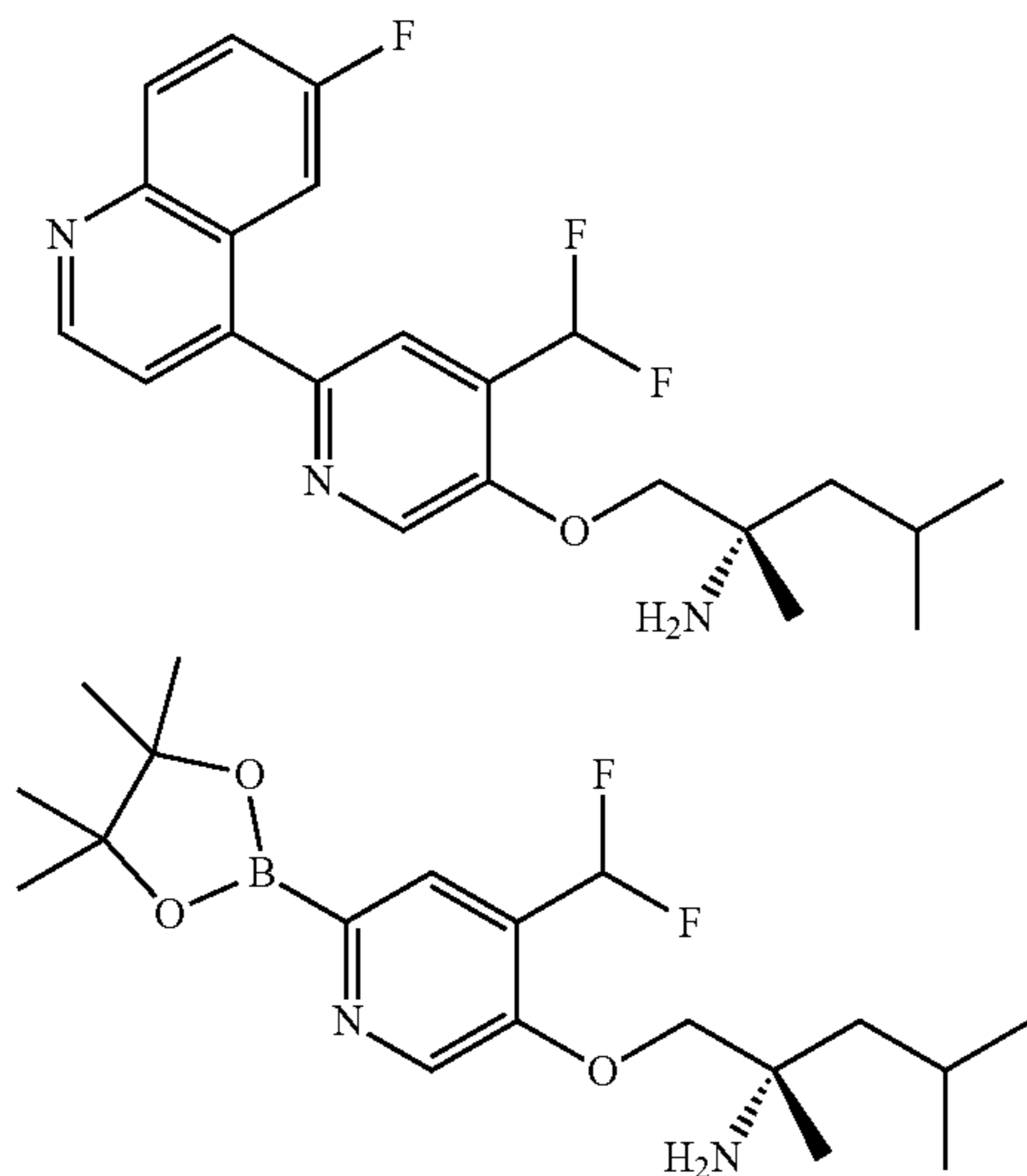
Part A: (S)-1-((4-(difluoromethyl)-6-(4,4,5,5-tetramethyl-1,3,2-dioxaborolan-2-yl)pyridin-3-yl)oxy)-2,4-dimethylpentan-2-amine
