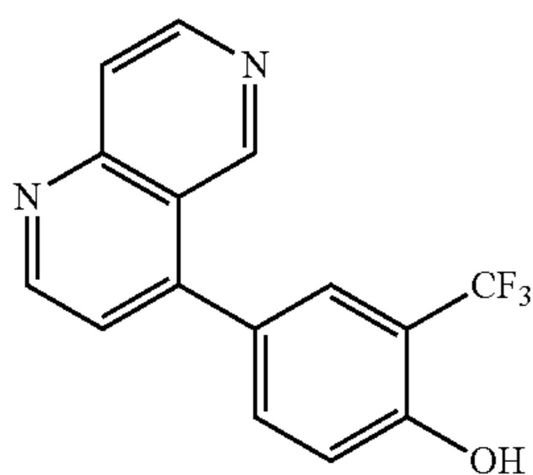
Part B: 4-(1,6-naphthyridin-4-yl)-2-(trifluoromethyl)phenol
