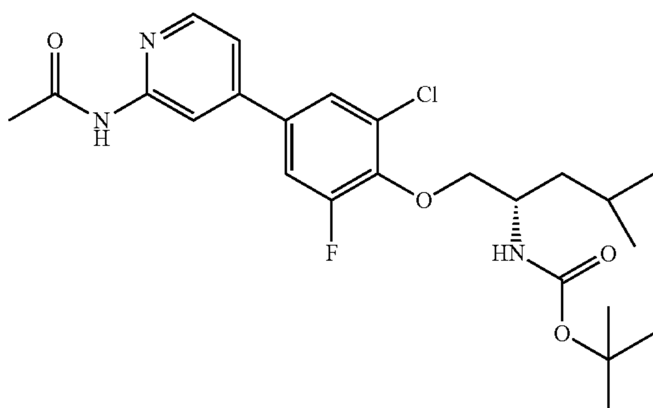
Part B: (S)-tert-butyl (1-(4-(2-acetamidopyridin-4-yl)-2-chloro-6-fluorophenoxy)-4-methylpentan-2-yl) carbamate
