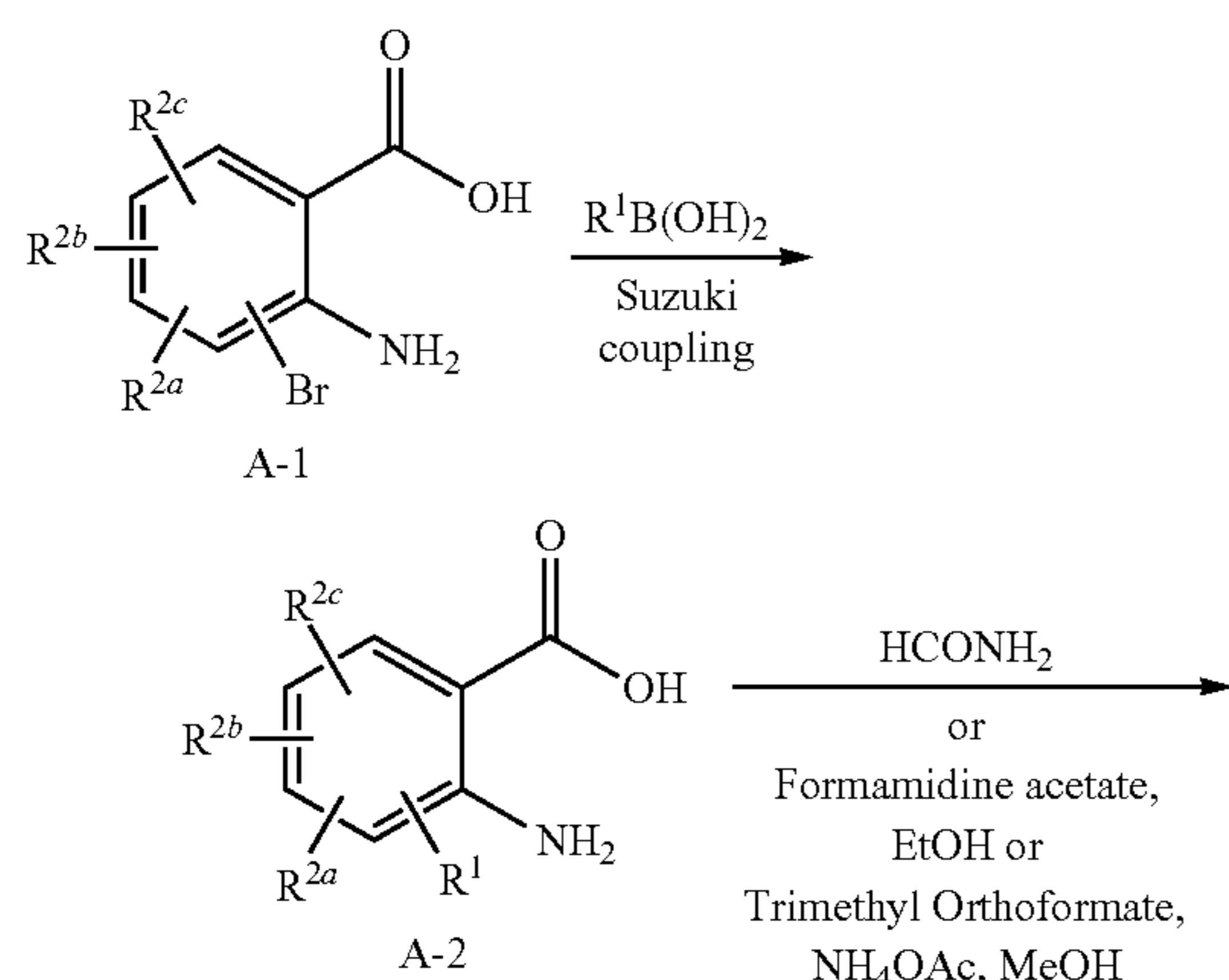
General Reaction Scheme 1
