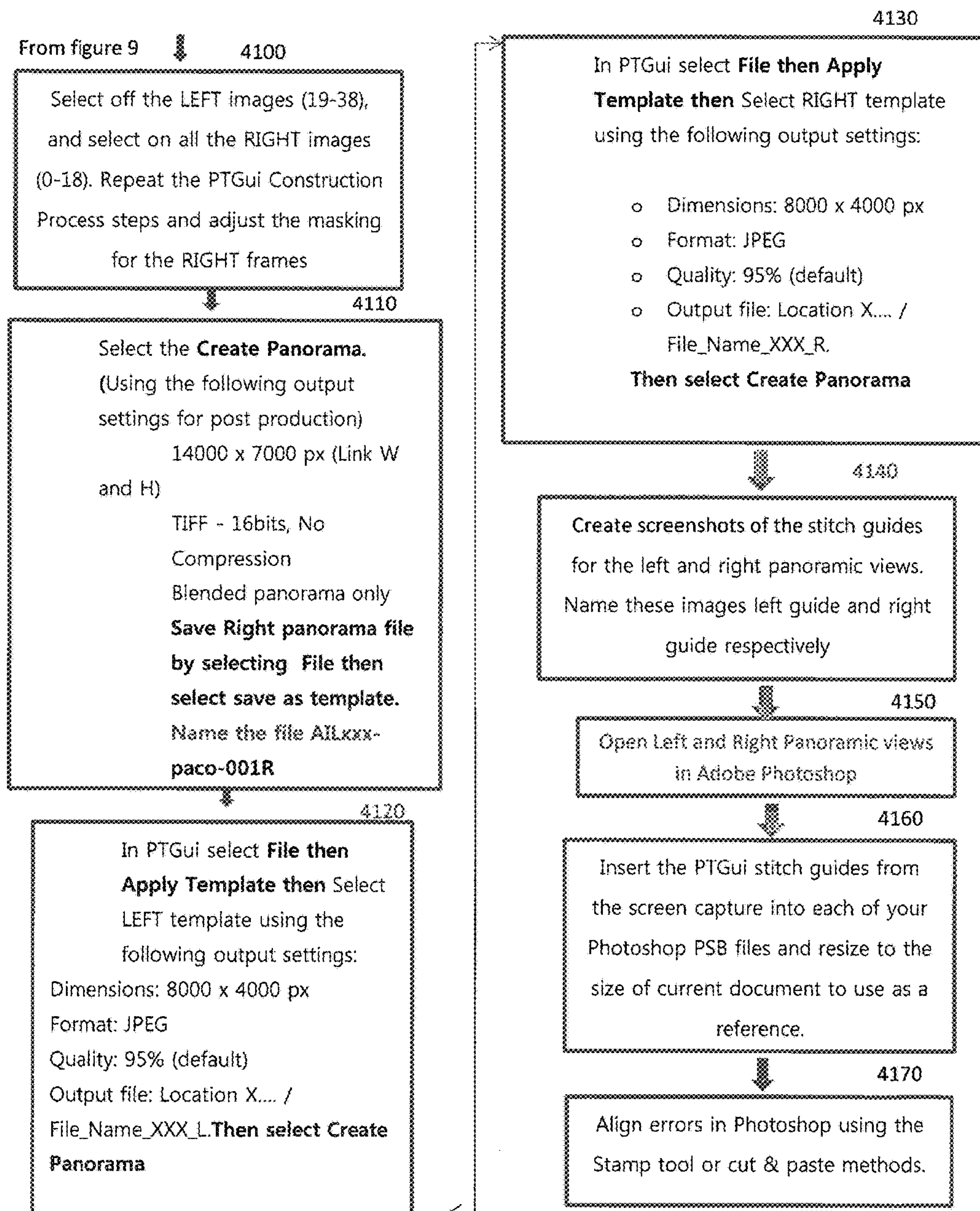
Flowchart for creation of Panoramic Virtual Tour from Camera Images
