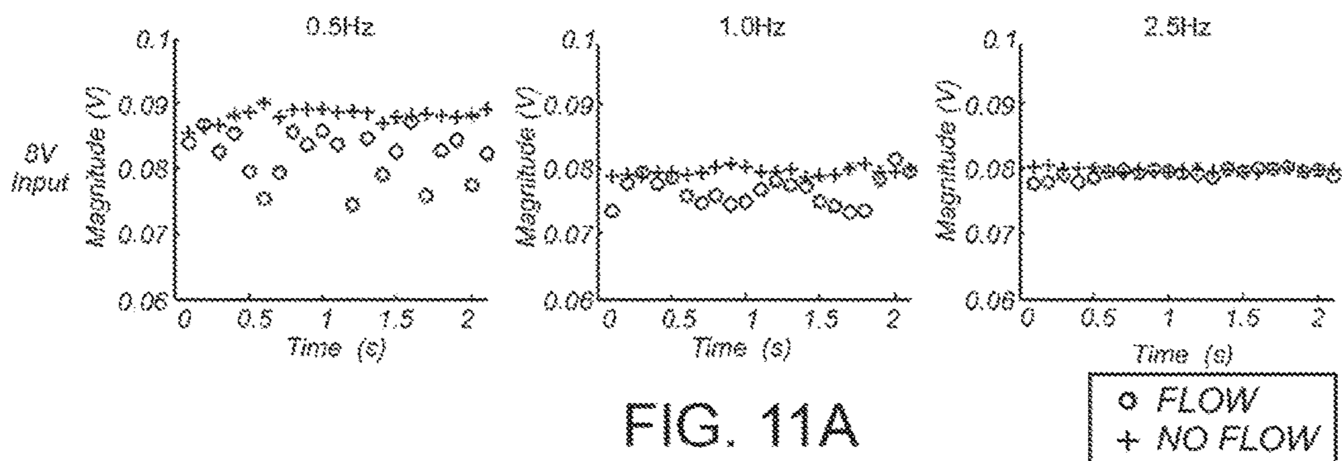
Elongate Member #2 Resistive Member #3: Magnitude Plot
