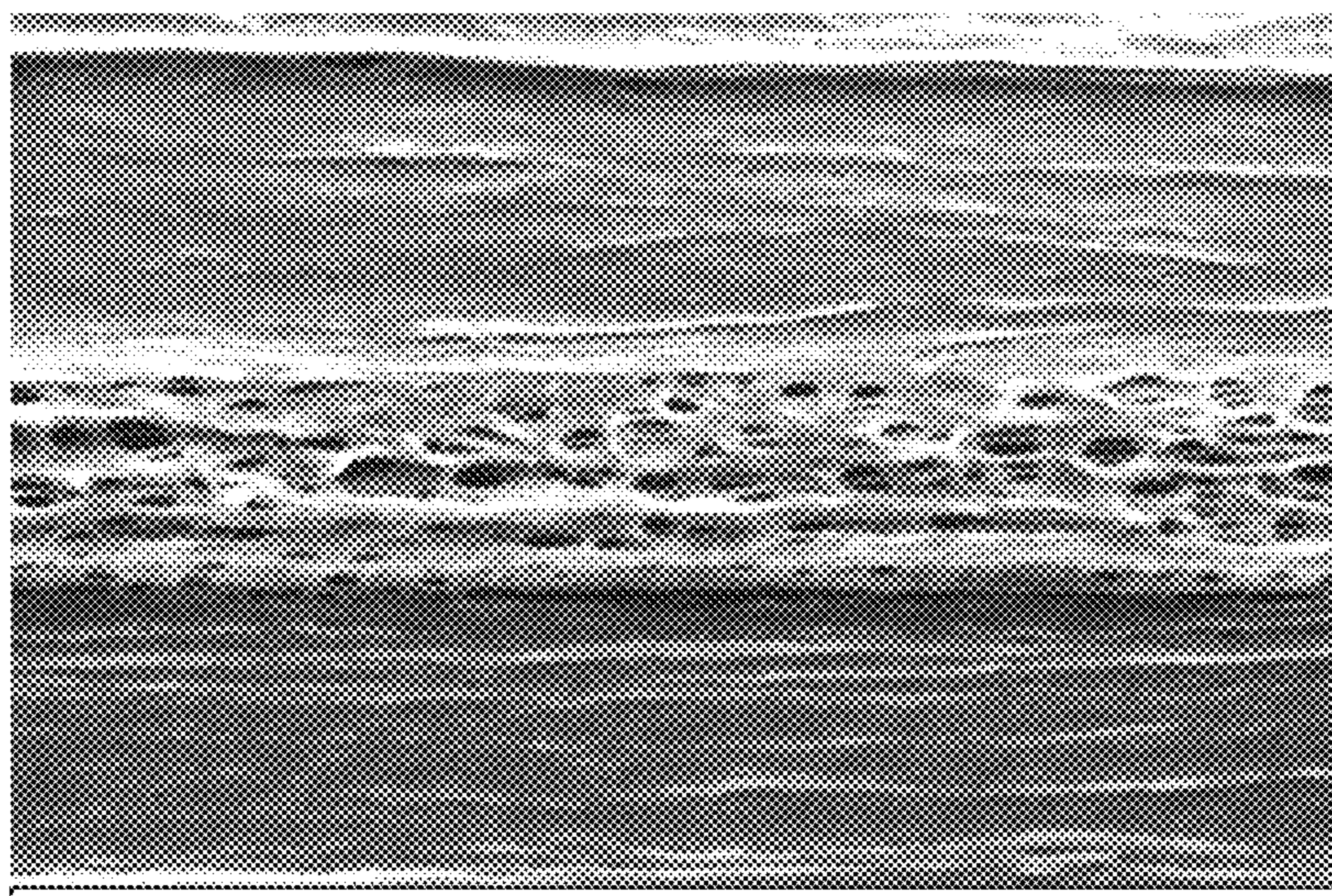
SEM Cross Sectional Micrograph of PP/PE/PP Trilayer Membrane With Larger Pores in Inner PE Layer.
