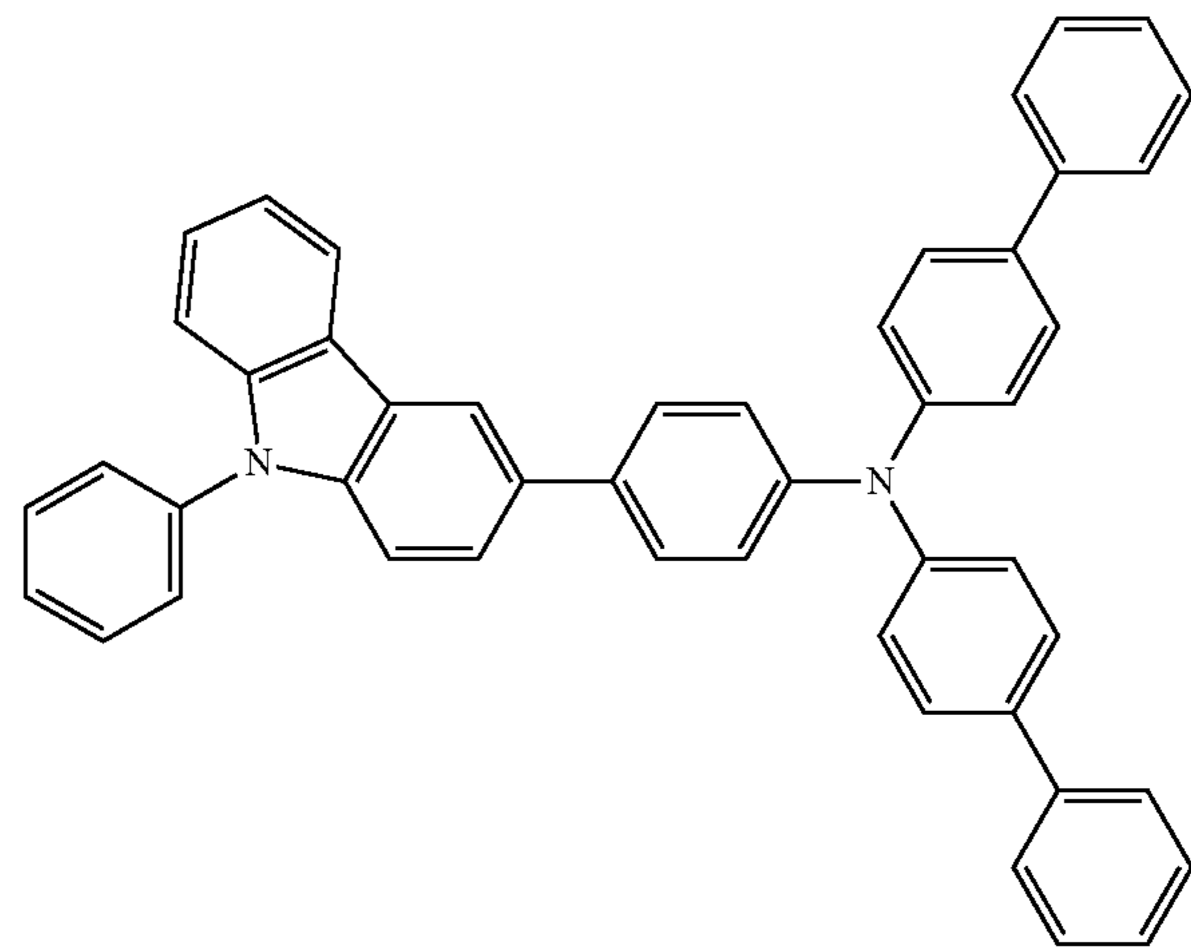
(4-phenyl-N-(4-phenylphenyl)-N-[4-[4-(4-phenyl-N-(4-phenylphenyl)anilino)phenyl]phenyl]aniline),
