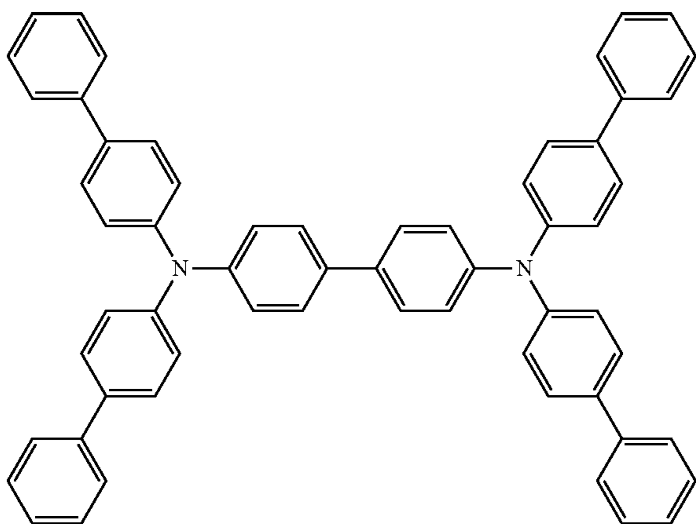
(4-phenyl-N-(4-phenylphenyl)-N-[4-[4-(N-(4-phenylphenyl)phenyl]anilino)phenyl]phenyl)aniline),
