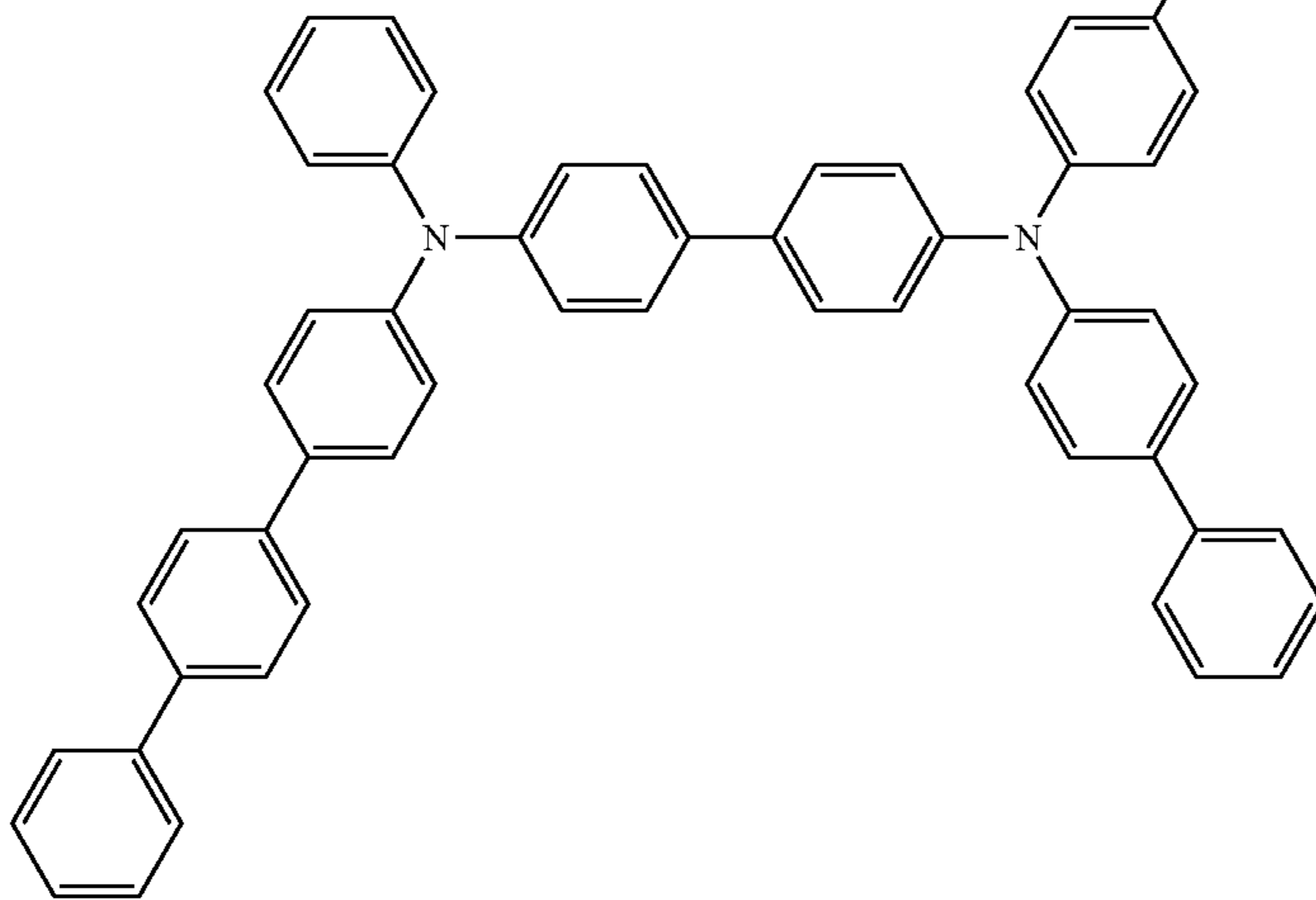
(4-phenyl-N-(4-phenylphenyl)-N-[4-[4-(N-(4-phenylphenyl)phenyl]anilino)phenyl]phenyl)aniline),
