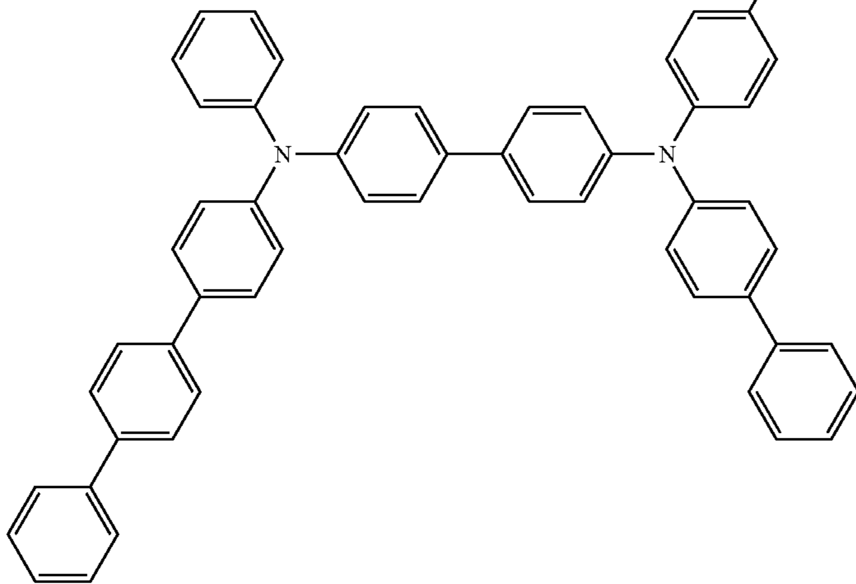
(4-phenyl-N-(4-phenylphenyl)-N-[4-[4-(N-[4-(4-phenyl-phenyl)phenyl]anilino)phenyl]phenyl]aniline),
