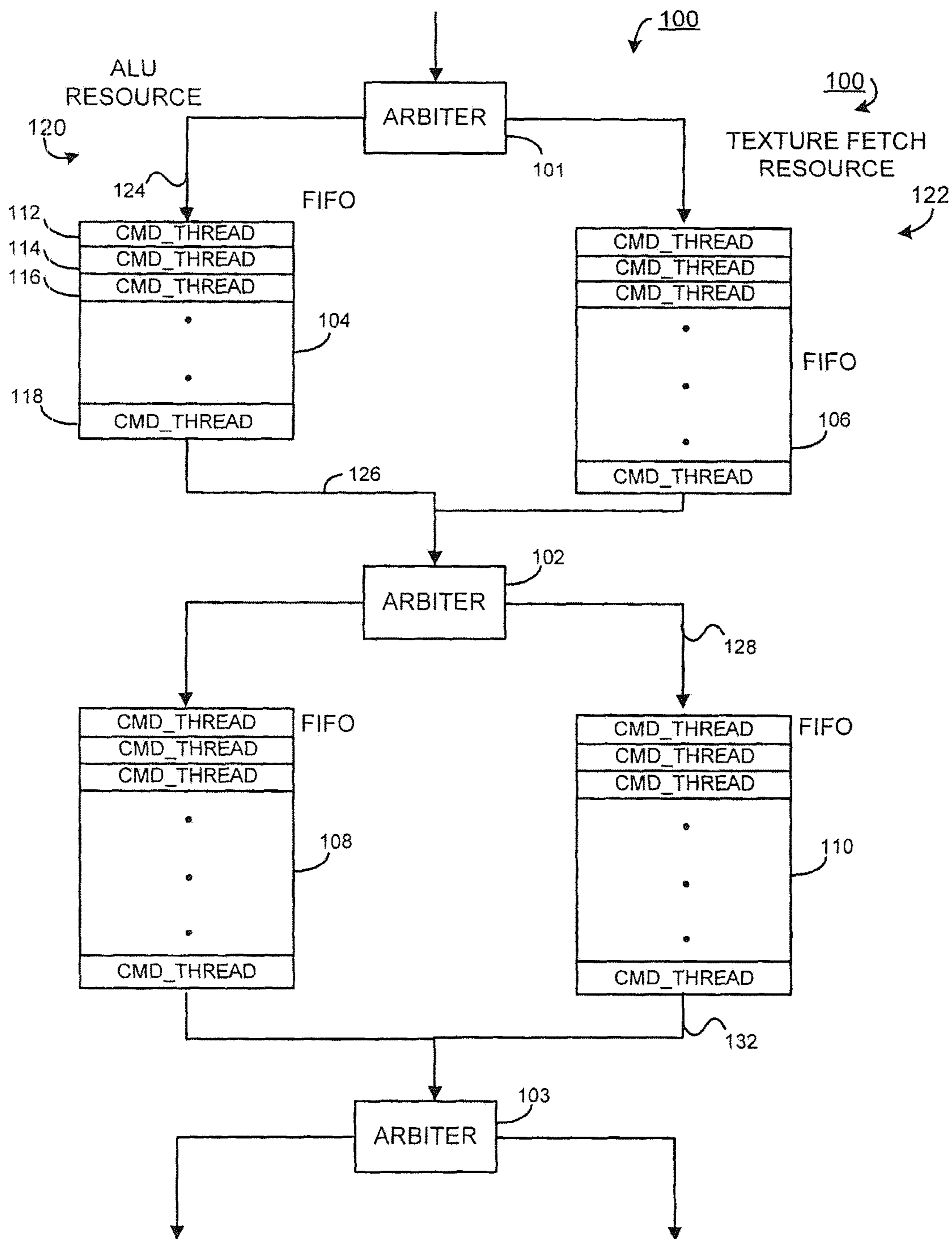
FIG. 1 (PRIOR ART)
