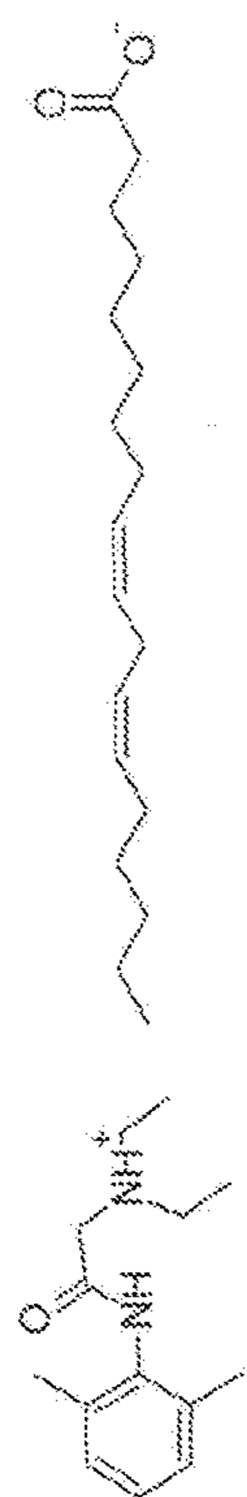
CLX-SYN-G177C-B-1, CDCl 3
