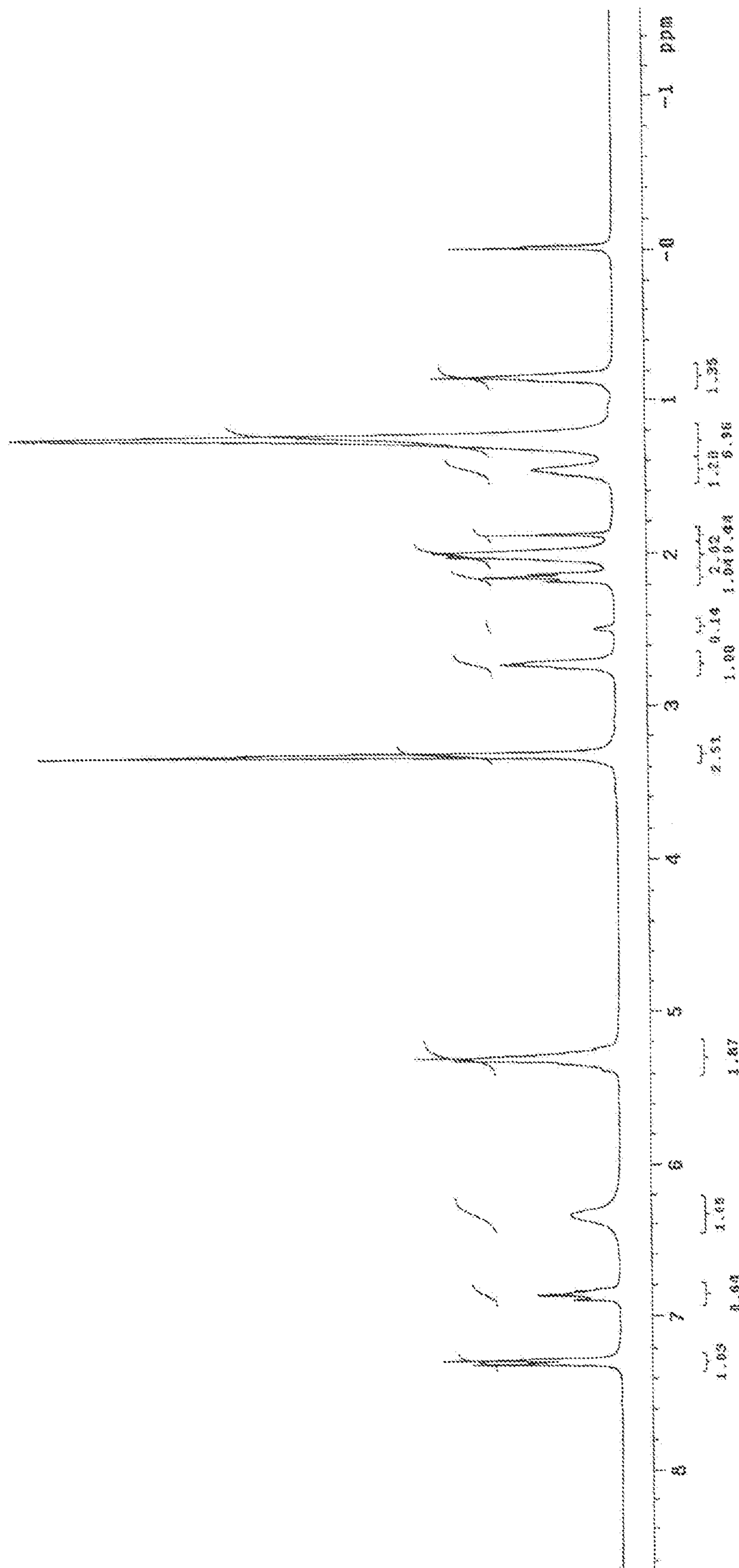
CLX-SYN-G177C-5-1A, DMSO-d6
