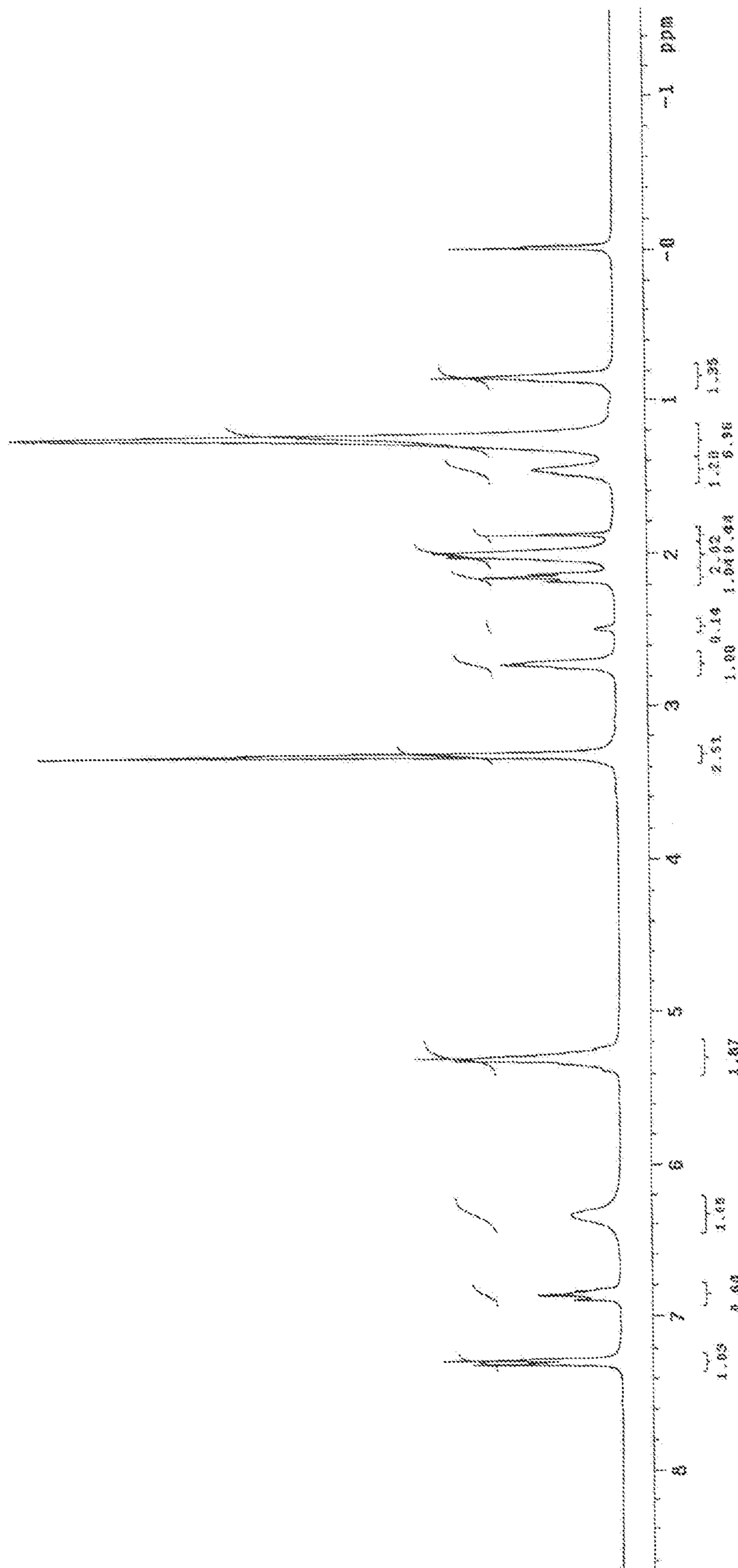
CLX-SYN-G177C-5-1A, DMSO-d6
