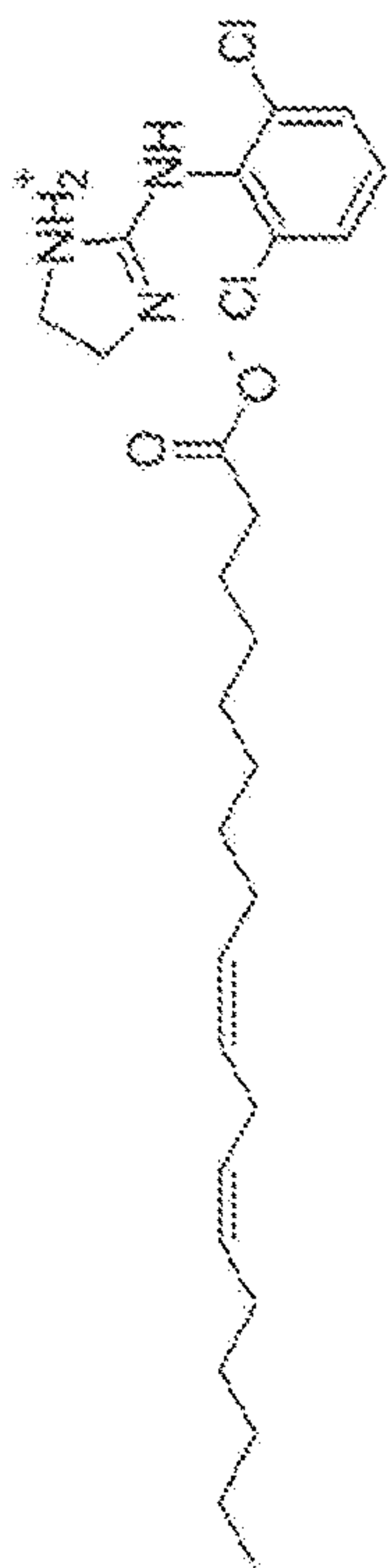
CLX-SYN-G177C-5-1A, DMSO-d6
