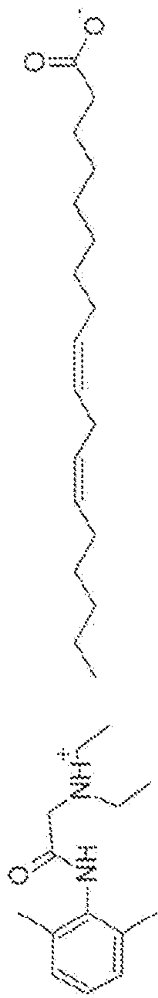
CLX-SYN-G177C-B-1, CDCl 3
