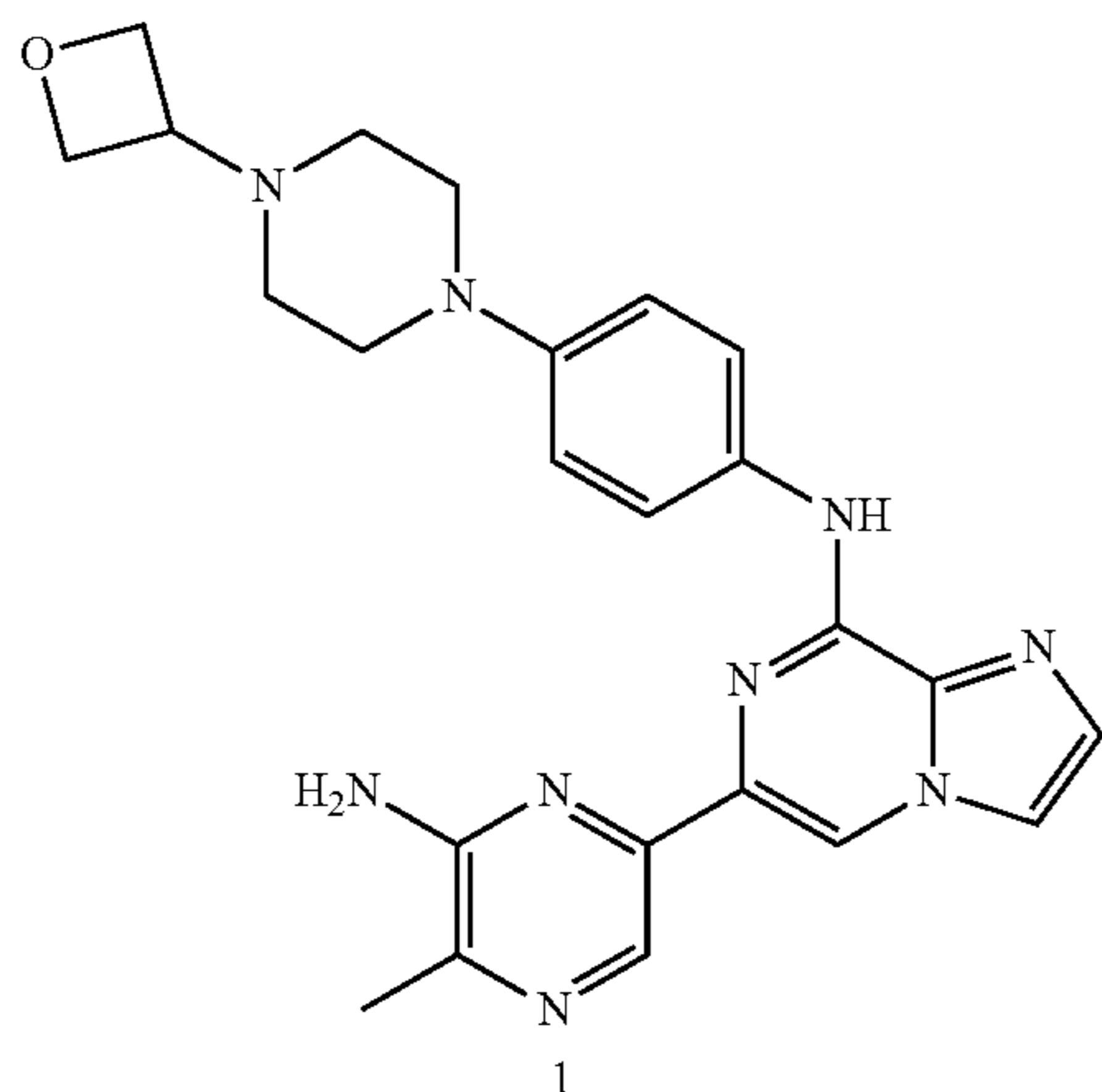
2-Bis(tert-butoxycarbonyl)amino-6-bromo-3-chloropyrazine XI
