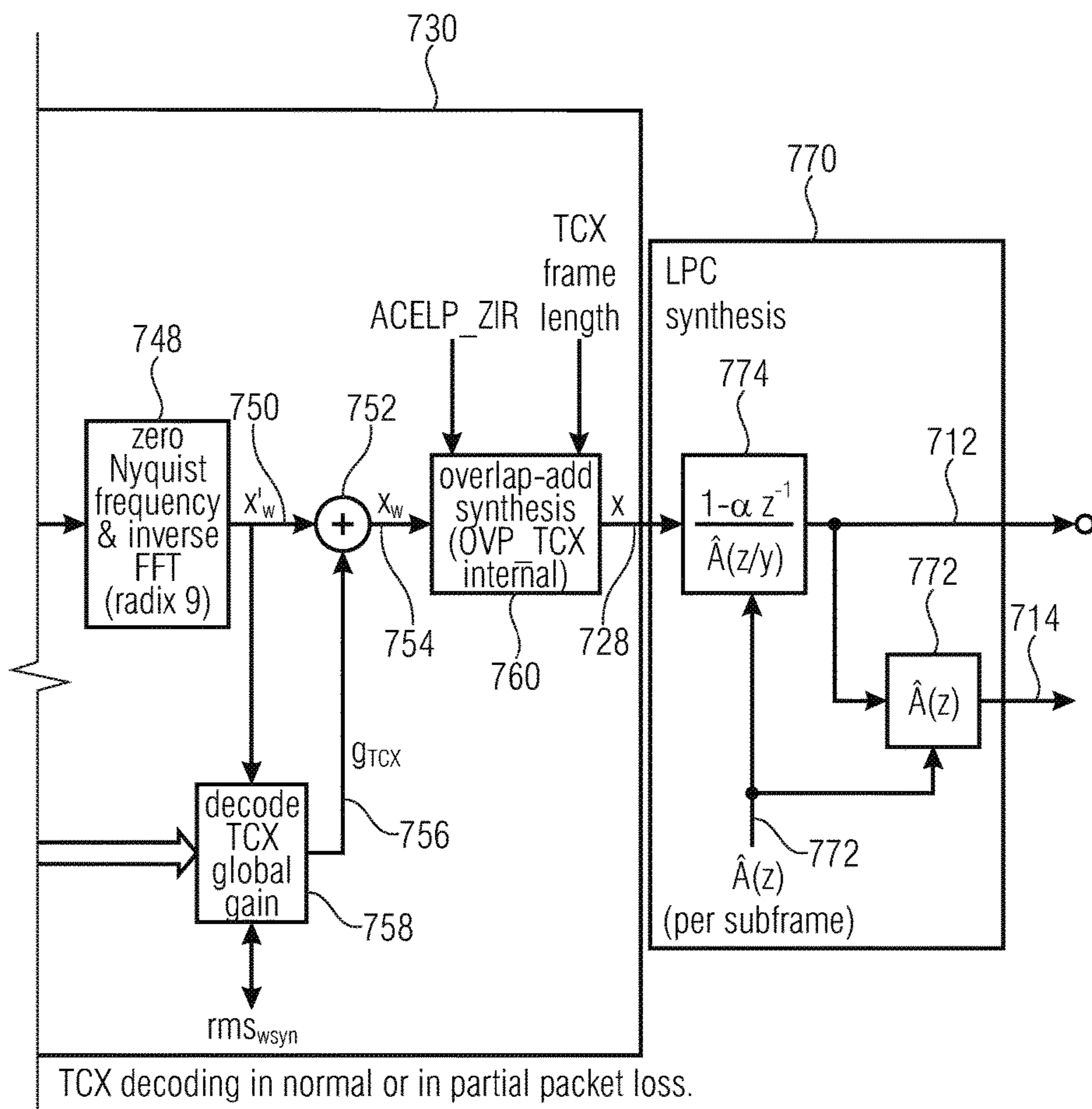
Block diagram of the TCX decoder
