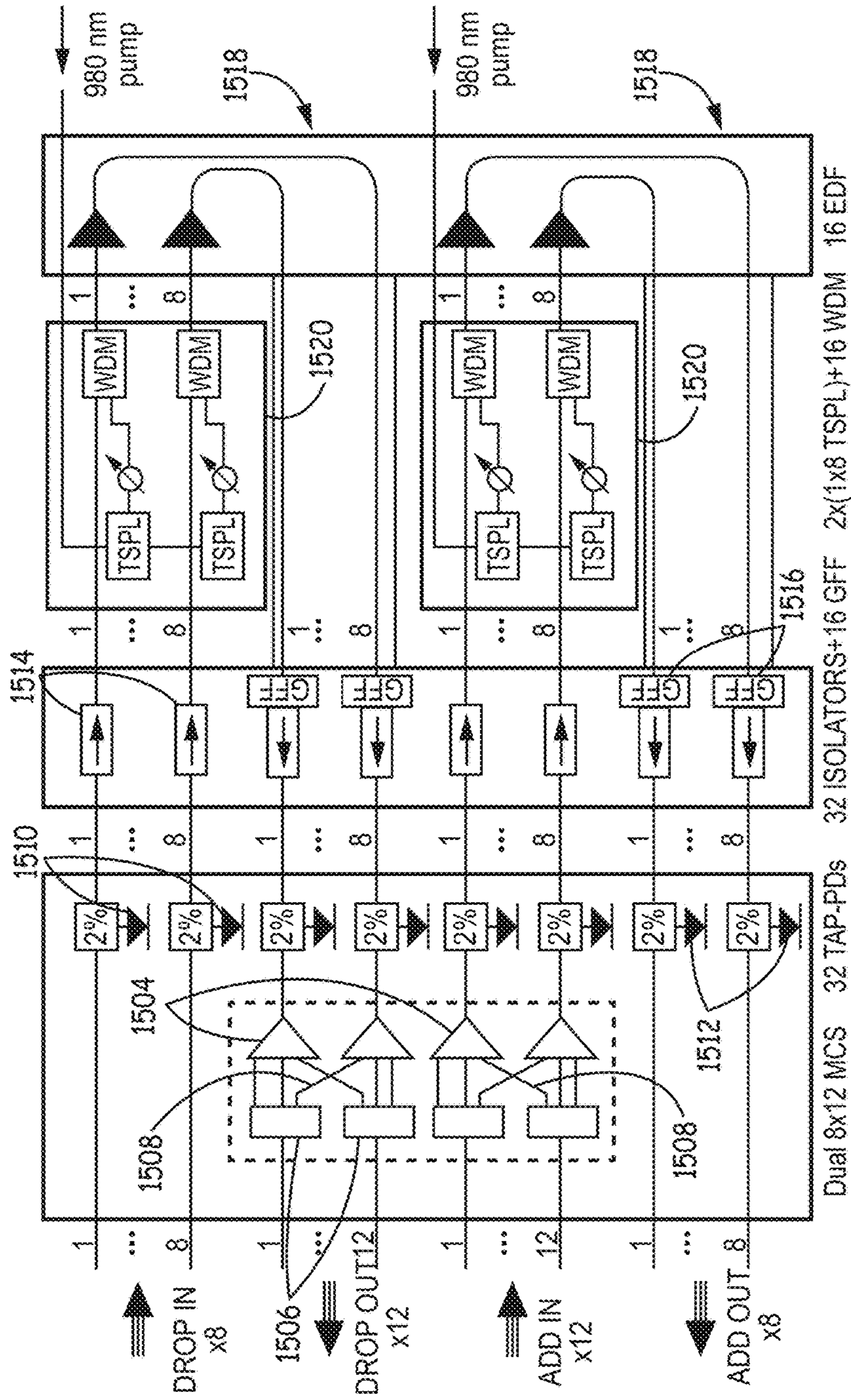
Functional diagram optics modules
