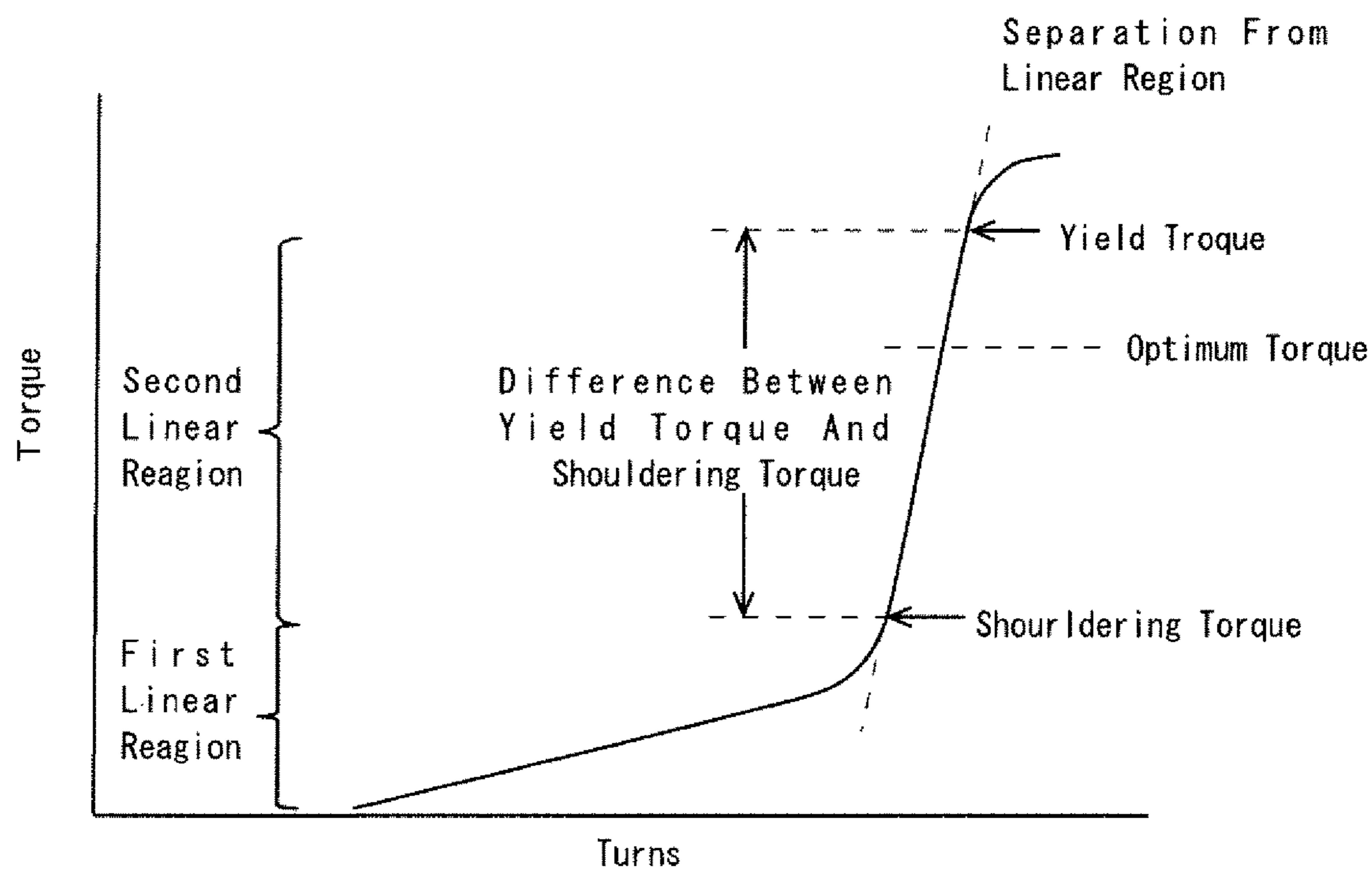
Torque Chart At Time Of Tightening
