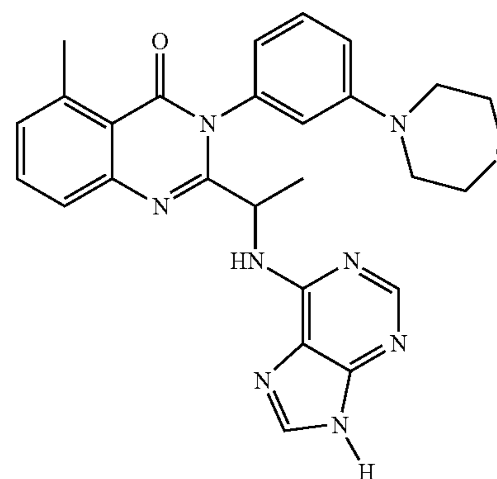
5-Methyl-3-(3-morpholin-4-yl-phenyl)-2-[1-(9H-purin-6-ylamino)-ethyl]-3H-quinazolin-4-one
