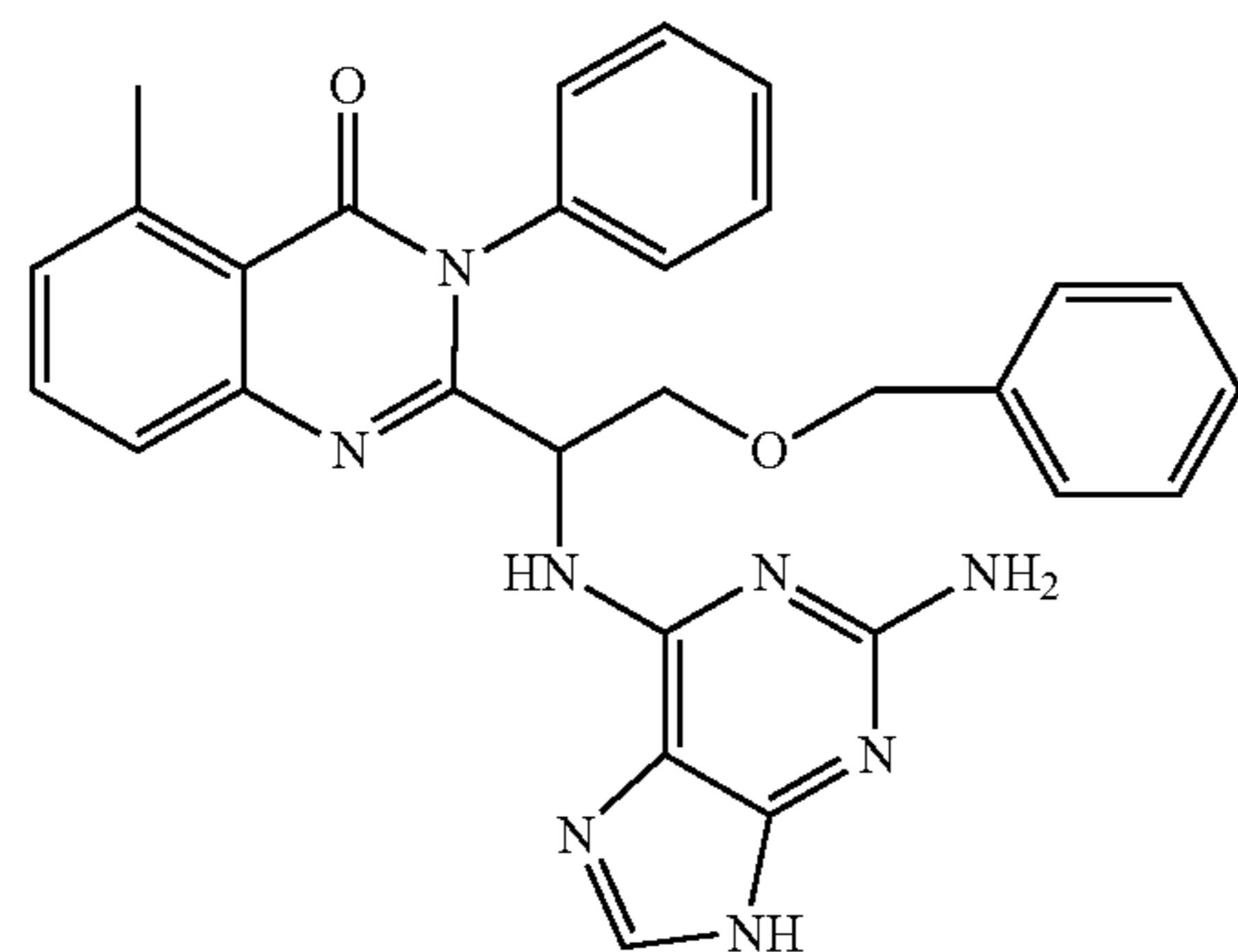
2-[2-benzyloxy-1-(7H-pyrrolo[2,3-d]pyrimidin-4-ylamino)-ethyl]-5-methyl-3-phenyl-3H-quinazolin-4-one (30)
