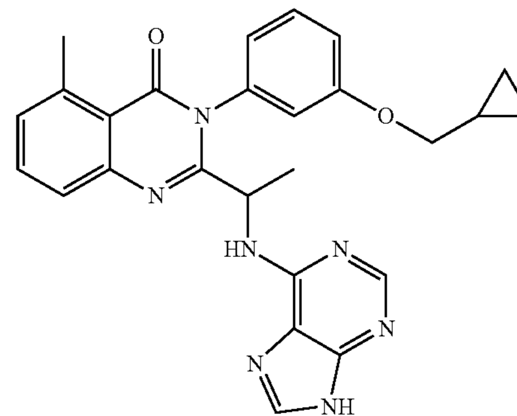
3-(3-Cyclopropylmethoxy-phenyl)-5-methyl-2-[1-(9H-purin-6-ylamino)-ethyl]-3H-quinazolin-4-one (130)
