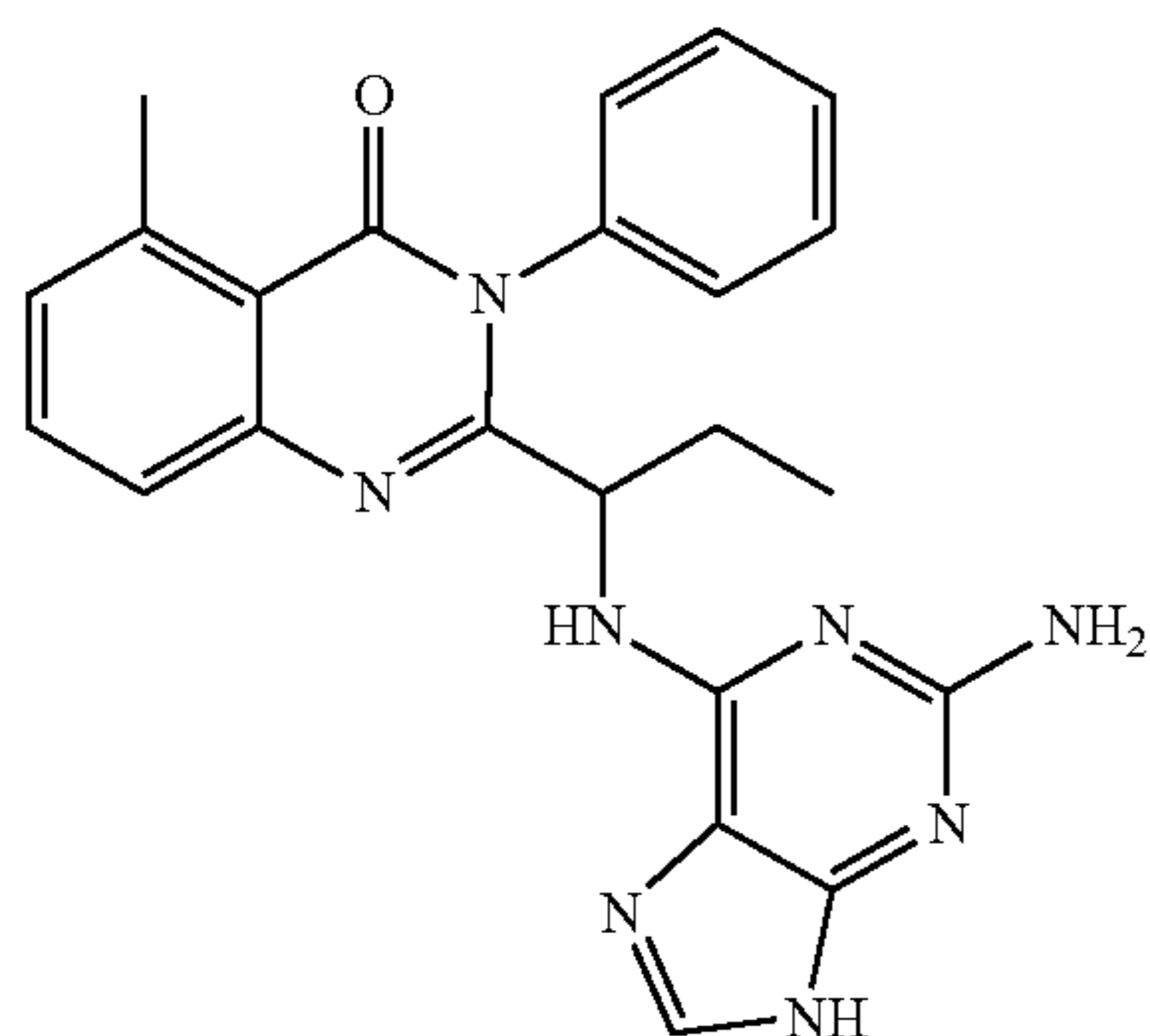
5-methyl-3-phenyl-2-[1-(7H-pyrrolo[2,3-d]pyrimidin-4-ylamino)-propyl]-3H-quinazolin-4-one (24)
