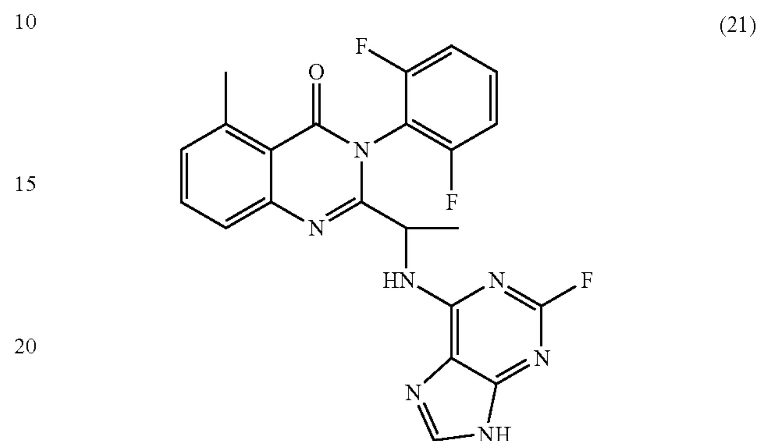
2-[1-(2-amino-9H-purin-6-ylamino)-ethyl]-3-(2,6-difluoro-phenyl)-5-methyl-3H-quinazolin-4-one (20)
