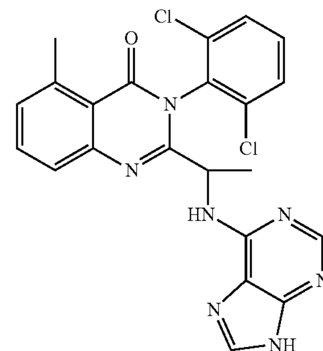
2-[1-(2-amino-9H-purin-6-ylamino)-ethyl]-3-(2,6-dichloro-phenyl)-5-methyl-3H-quinazolin-4-one (81)
