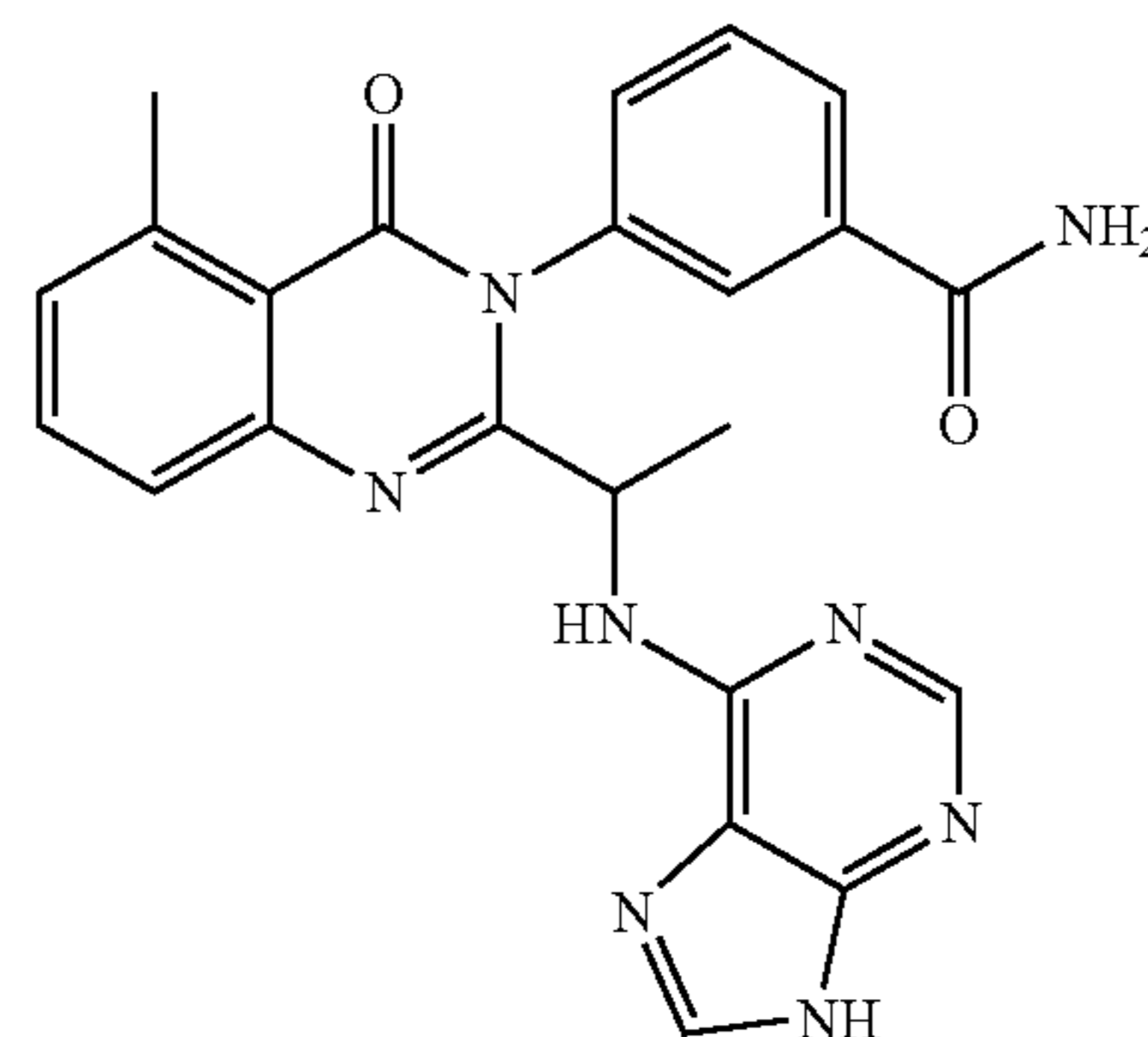
3-(5-Methyl-4-oxo-2-[1-(9H-purin-6-ylamino)-ethyl]-4H-quinazolin-3-yl)-benzamide
