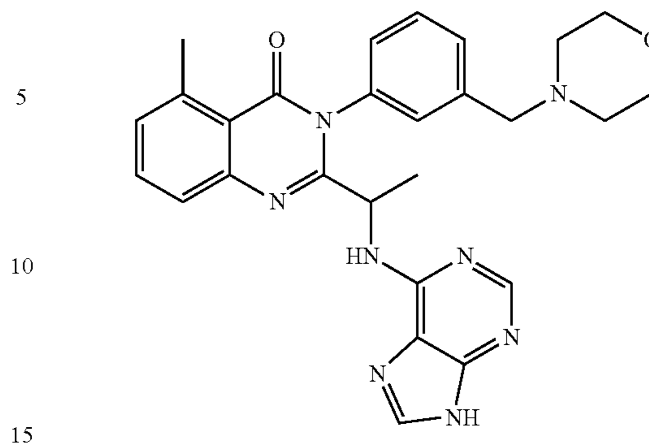
2-[1-(2-amino-9H-purin-6-ylamino)-ethyl]-5-methyl-3-(3-morpholin-4-ylmethyl-phenyl)-3H-quinazolin-4-one (88)
