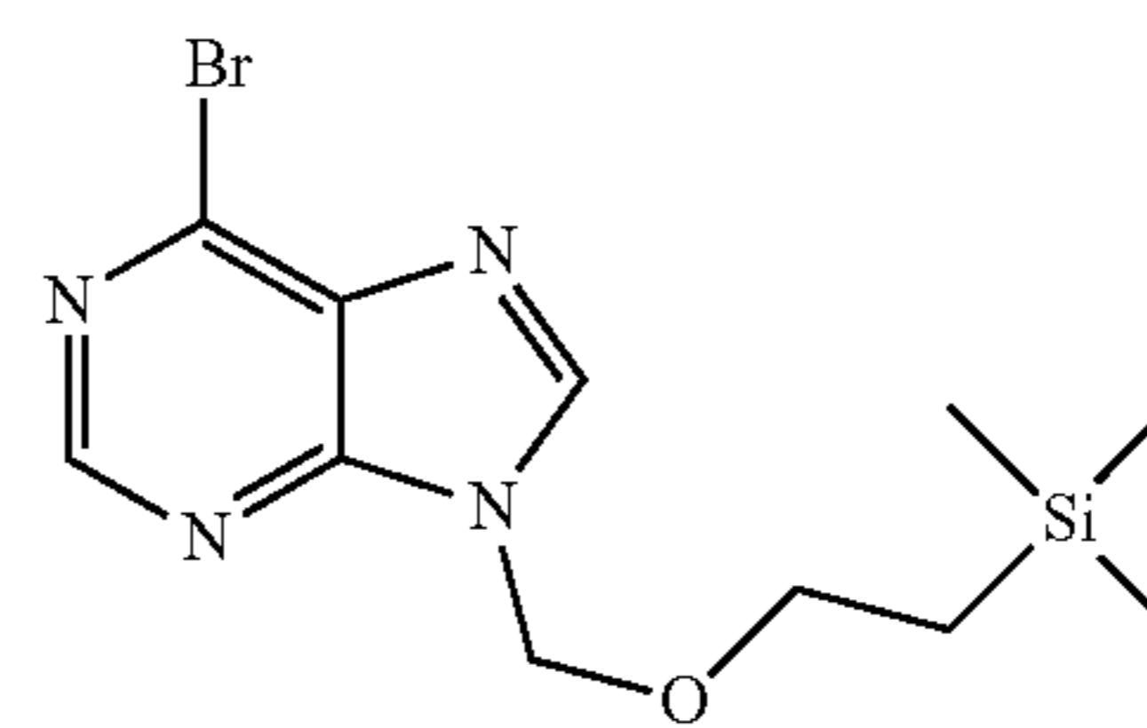
2-amino-6-bromo-9-(2-trimethylsilyl-ethoxymethyl)-9H-purine (11)
