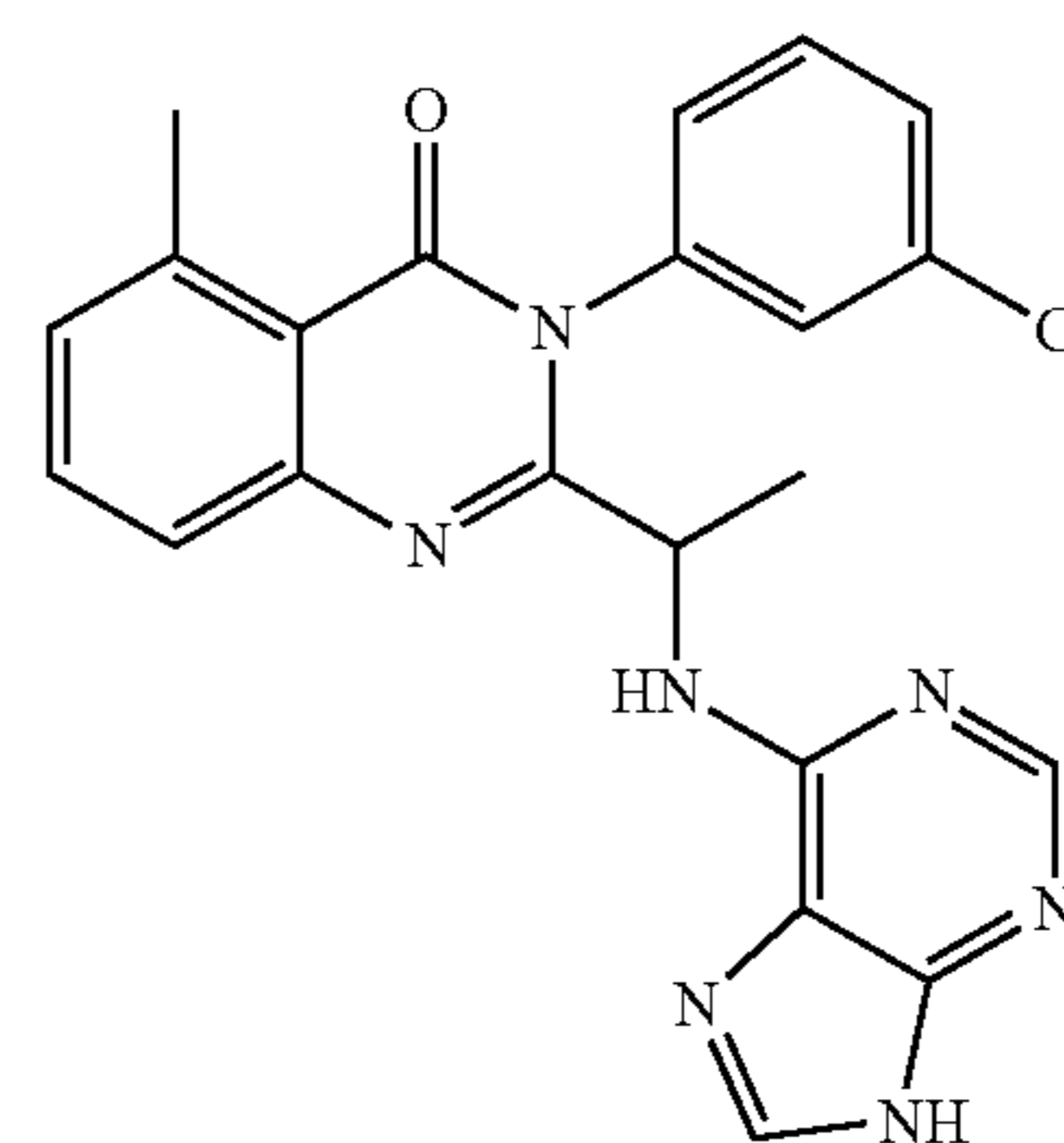
2-[1-(2-amino-9H-purin-6-ylamino)-ethyl]-3-(3-chloro-phenyl)-5-methyl-3H-quinazolin-4-one (67)
