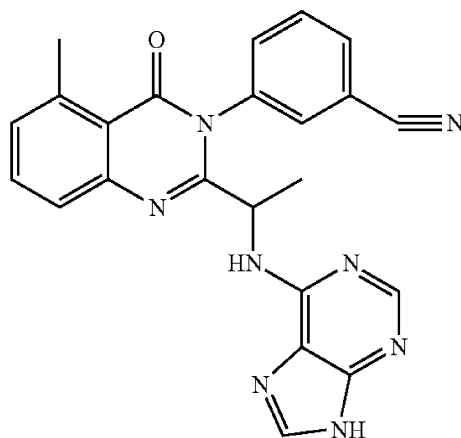
3-(5-Methyl-4-oxo-2-[1-(9H-purin-6-ylamino)-ethyl]-4H-quinazolin-3-yl)-benzonitrile
