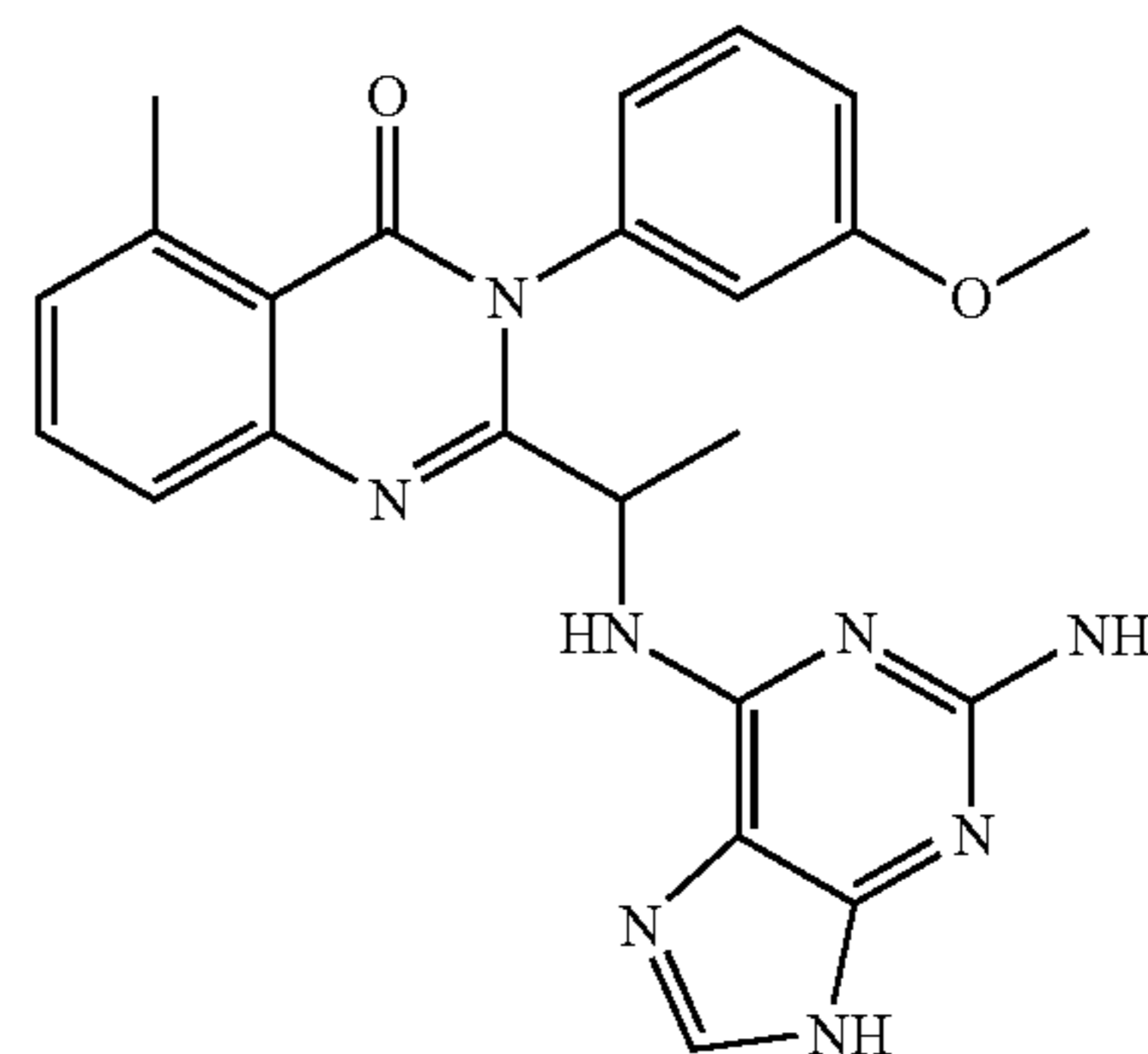
2-[1-(2-Amino-9H-purin-6-ylamino)-ethyl]-3-(3-methoxy-phenyl)-5-methyl-3H-quinazolin-4-one
