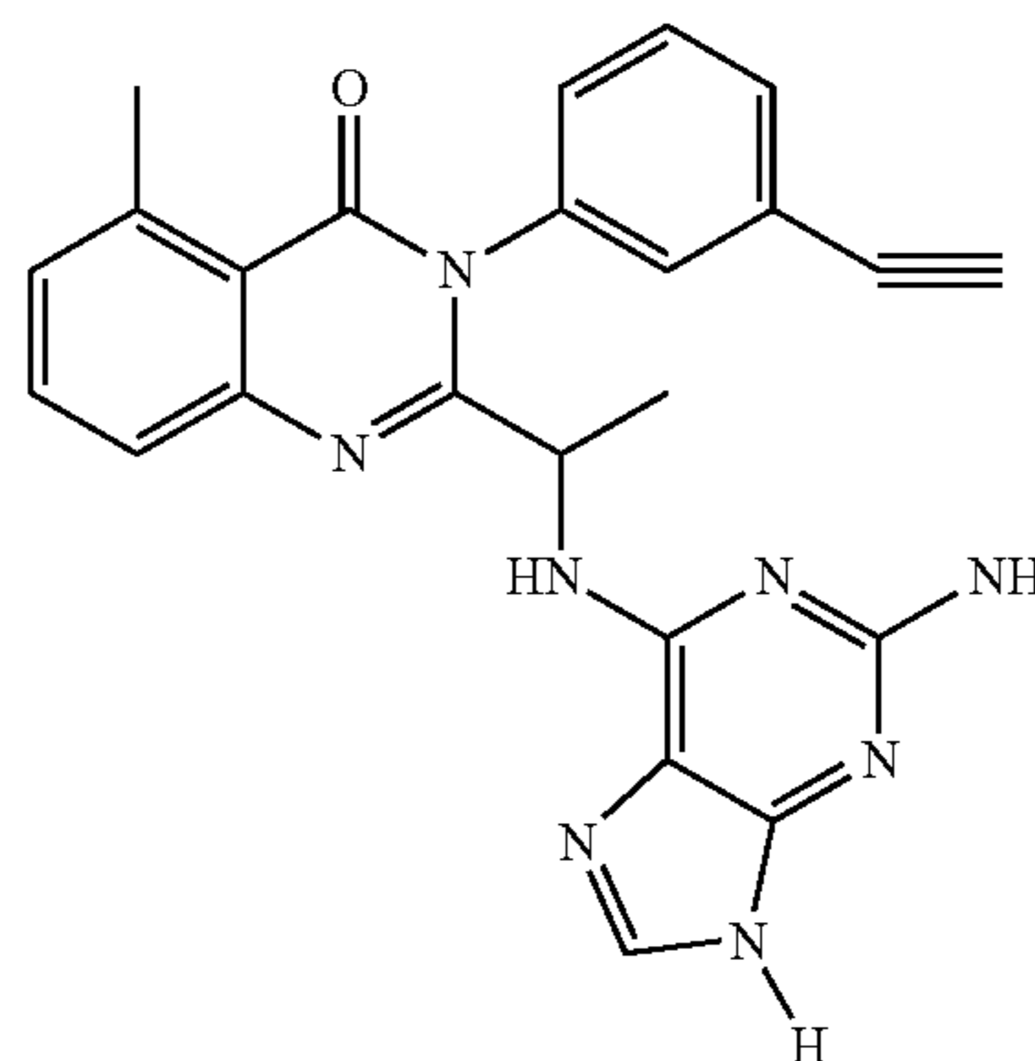
2-[1-(2-Amino-9H-purin-6-ylamino)-ethyl]-3-(3-ethynyl-phenyl)-5-methyl-3H-quinazolin-4-one
