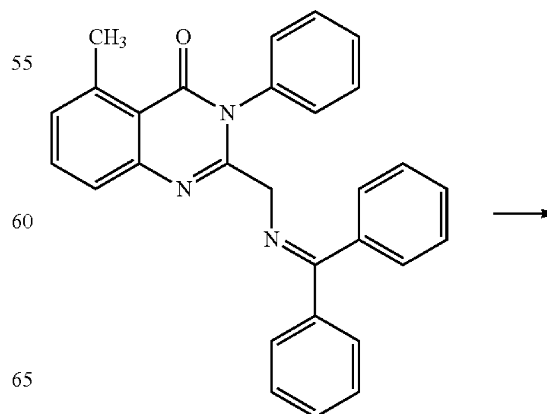
2-[(Benzhydrylidene-amino)-methyl]-5-methyl-3-phenyl-3H-quinazolin-4-one (162)
