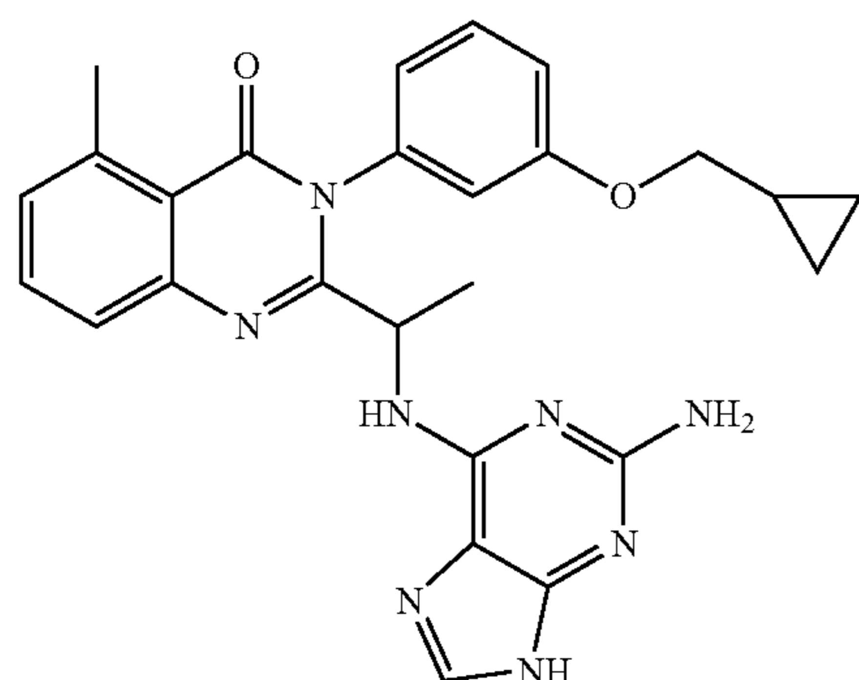
2-[1-(2-Amino-9H-purin-6-ylamino)-ethyl]-3-(3-cyclopropylmethoxy-phenyl)-5-methyl-3H-quinazolin-4-one
