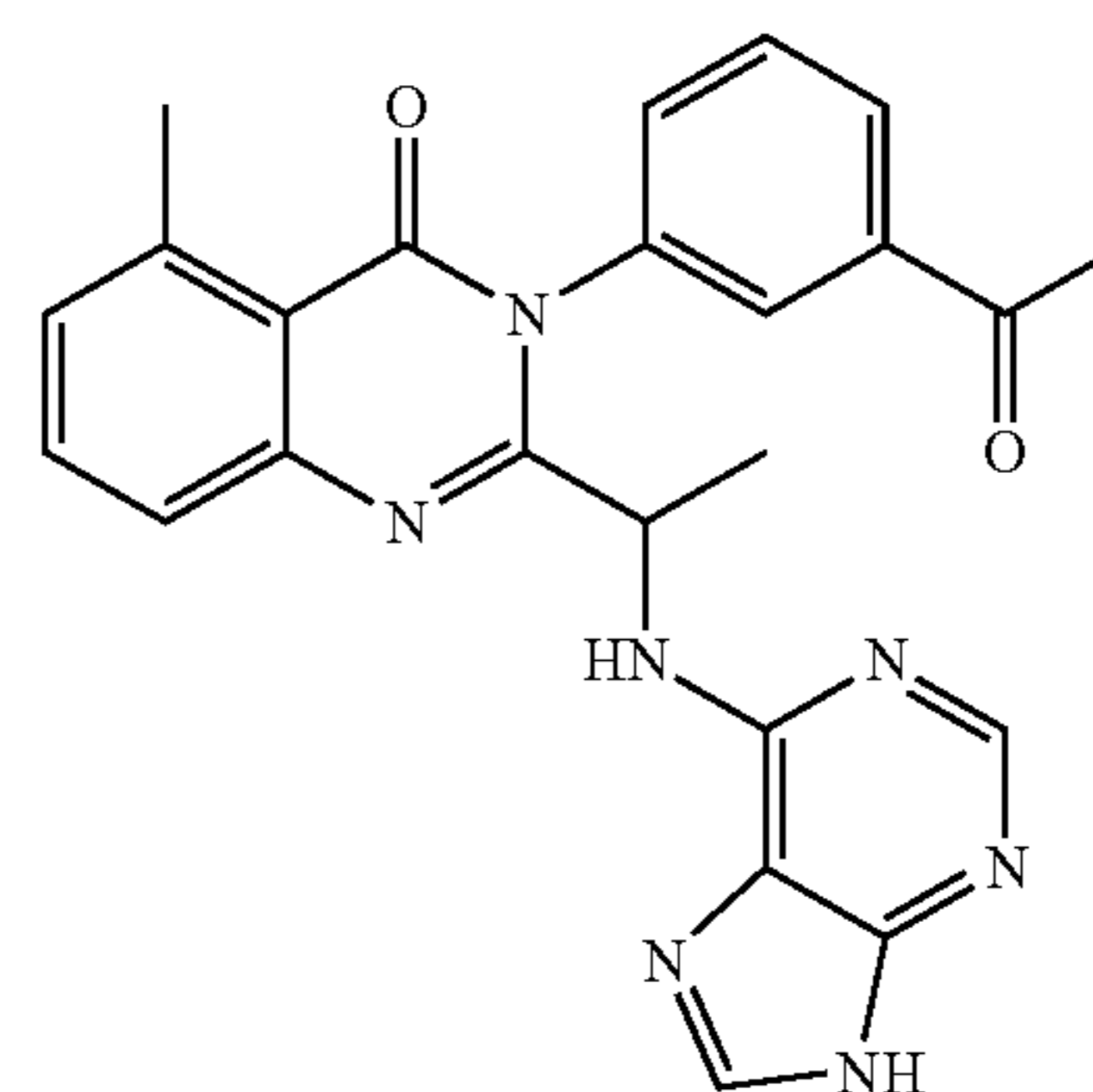
3-(3-Acetyl-phenyl)-5-methyl-2-[1-(9H-purin-6-ylamino)-ethyl]-3H-quinazolin-4-one
