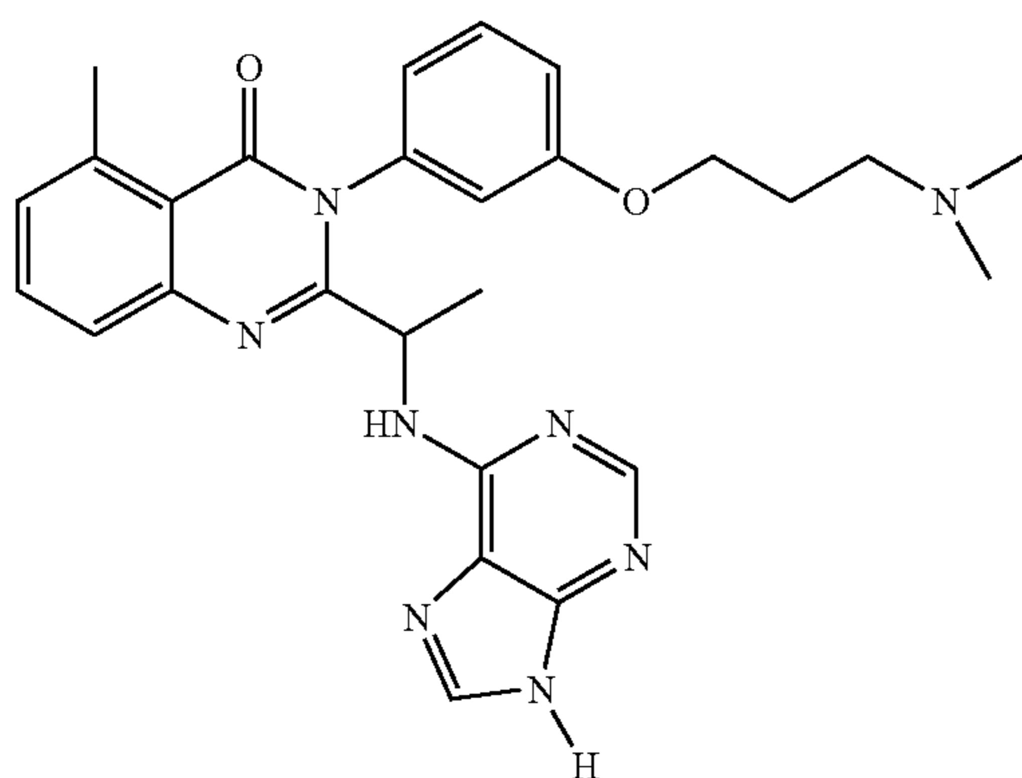
3-[3-(3-Dimethylamino-propoxy)-phenyl]-5-methyl-2-[1-(9H-purin-6-ylamino)-ethyl]-3H-quinazolin-4-one
