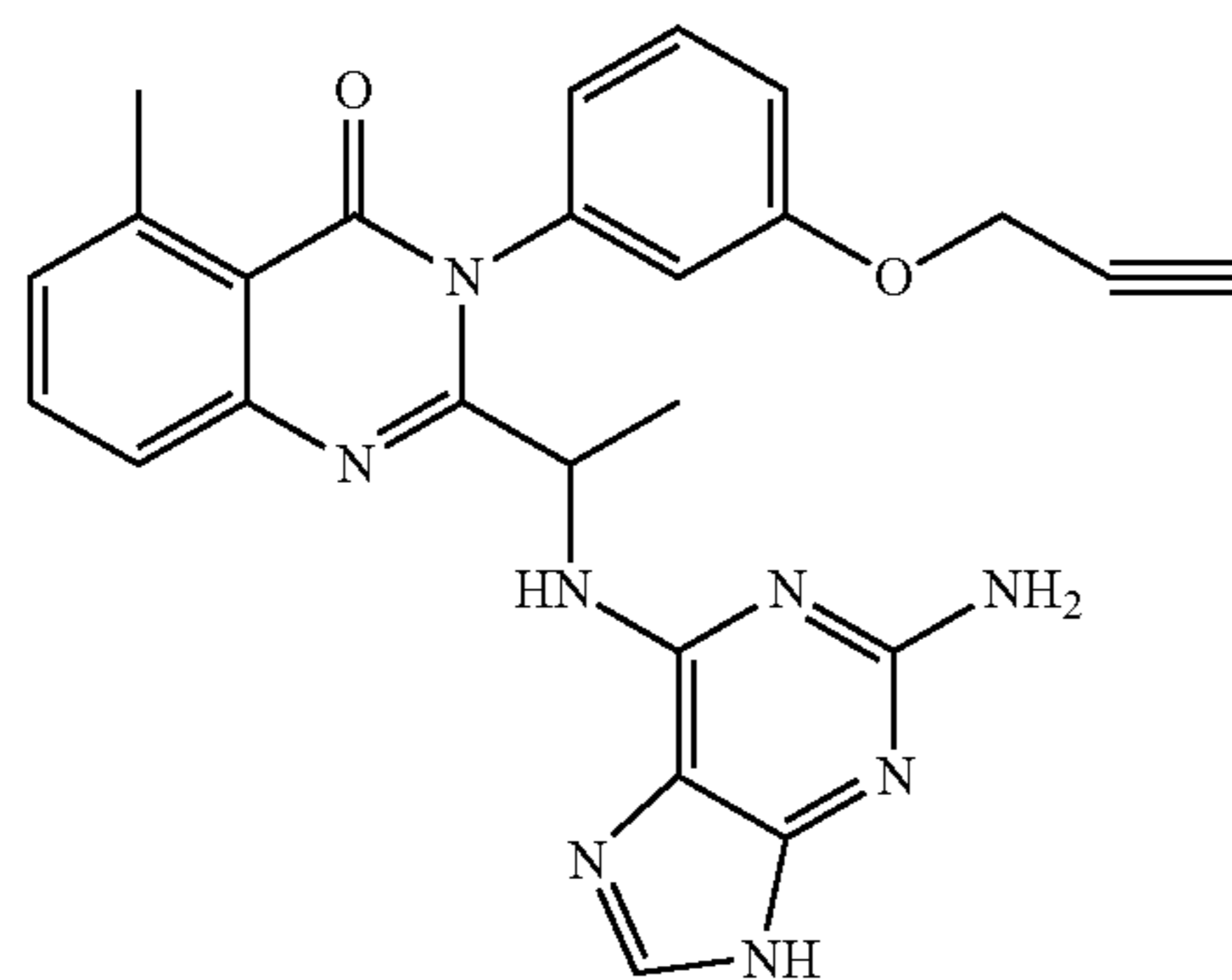
2-[1-(2-Amino-9H-purin-6-ylamino)-ethyl]-5-methyl-3-(3-prop-2-ynyloxy-phenyl)-3H-quinazolin-4-one
