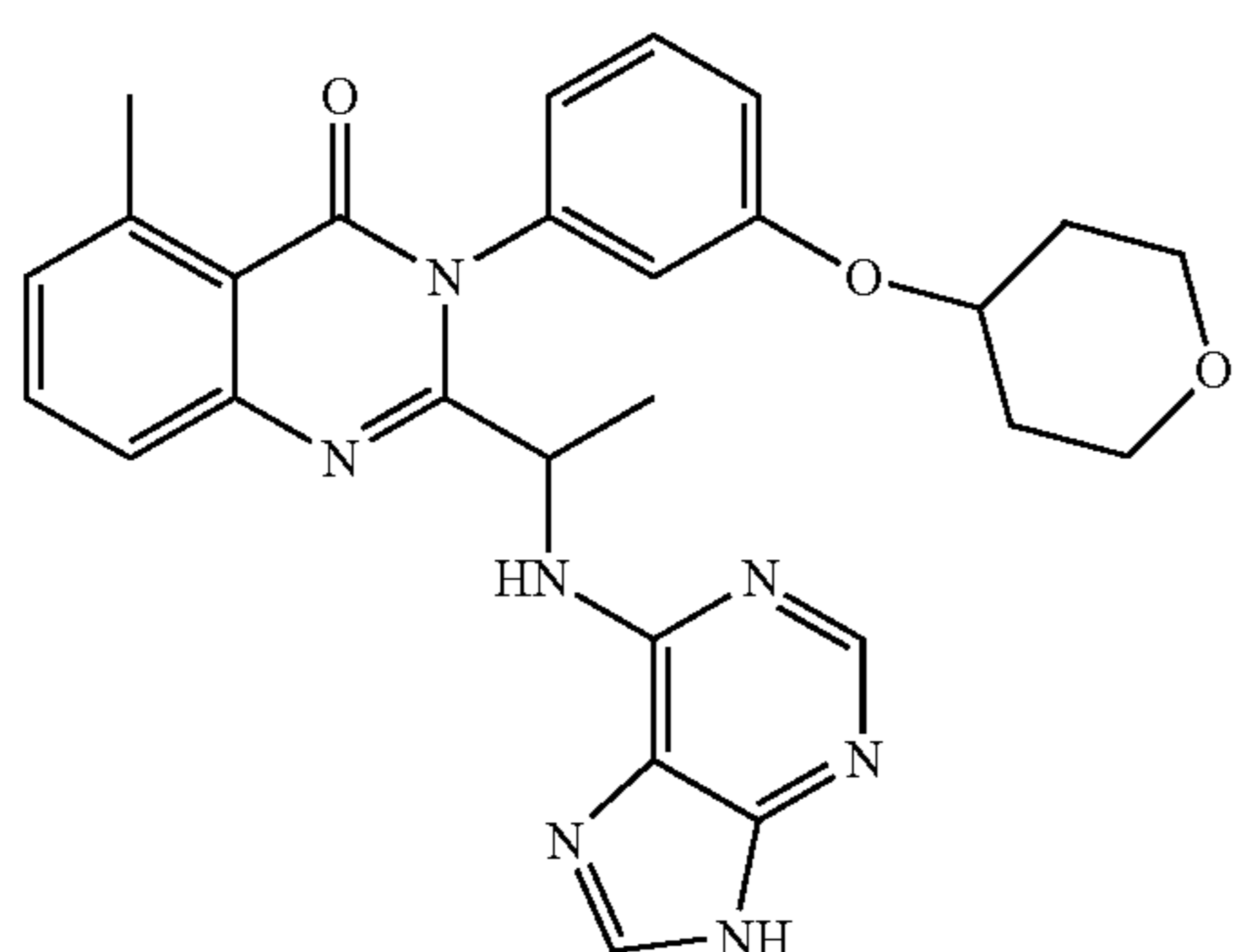
5-Methyl-2-[1-(9H-purin-6-ylamino)-ethyl]-3-[3-(tetrahydro-pyran-4-yloxy)-phenyl]-3H-quinazolin-4-one
