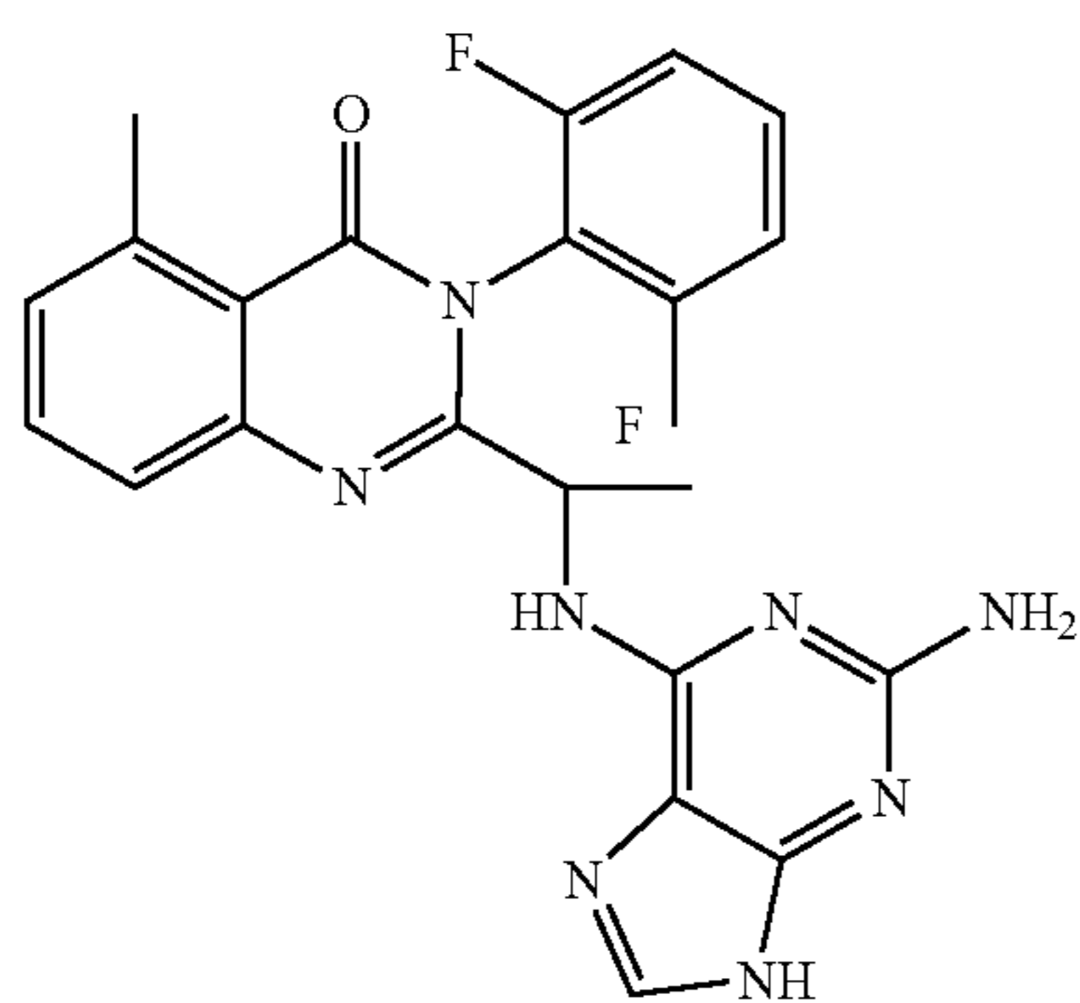
3-(2,6-difluoro-phenyl)-2-[1-(2-fluoro-9H-purin-6-ylamino)-ethyl]-5-methyl-3H-quinazolin-4-one (21)
