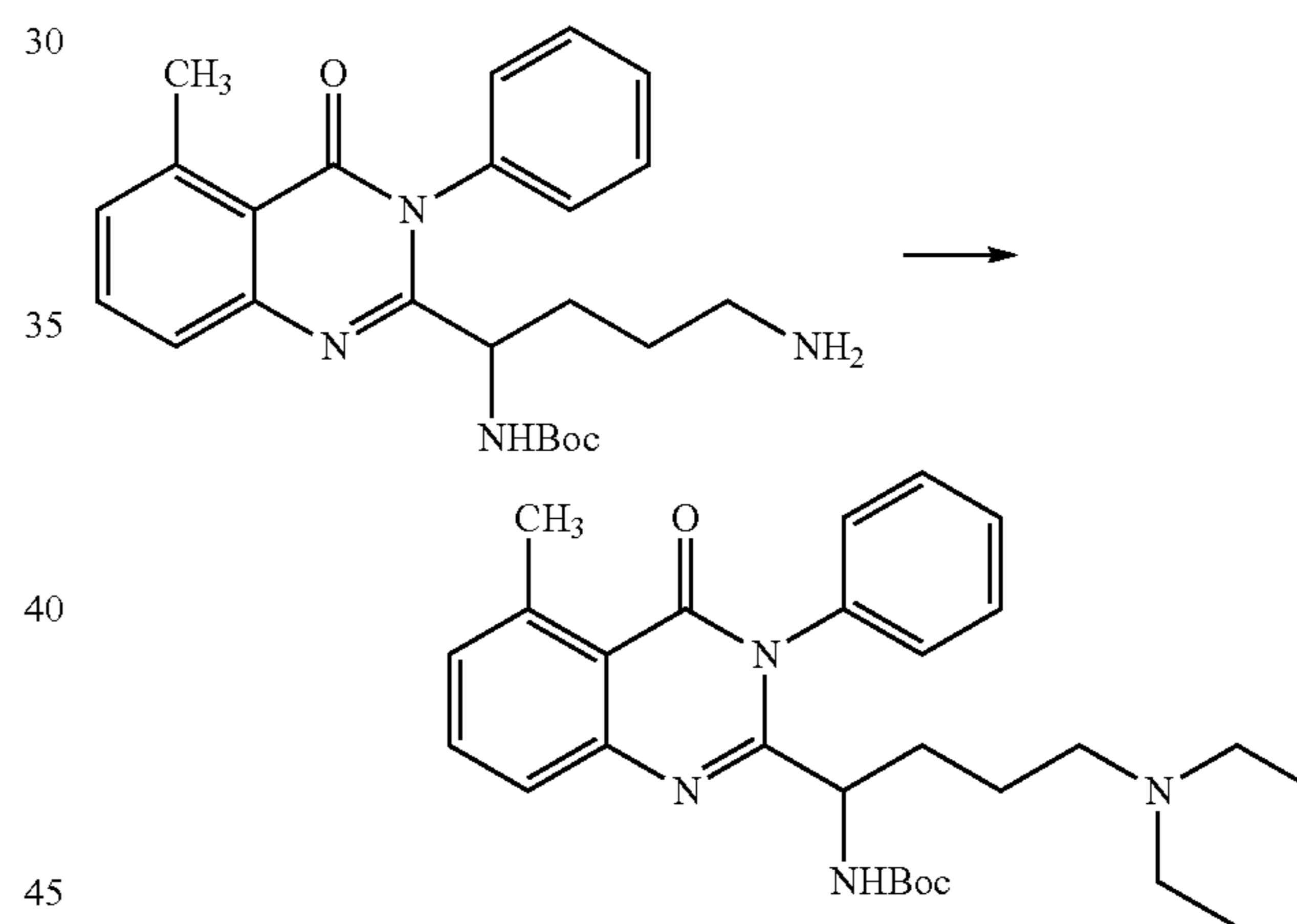
2-(1-amino-4-diethylamino-butyl)-5-methyl-3-phenyl-3H-quinazolin-4-one (106)
