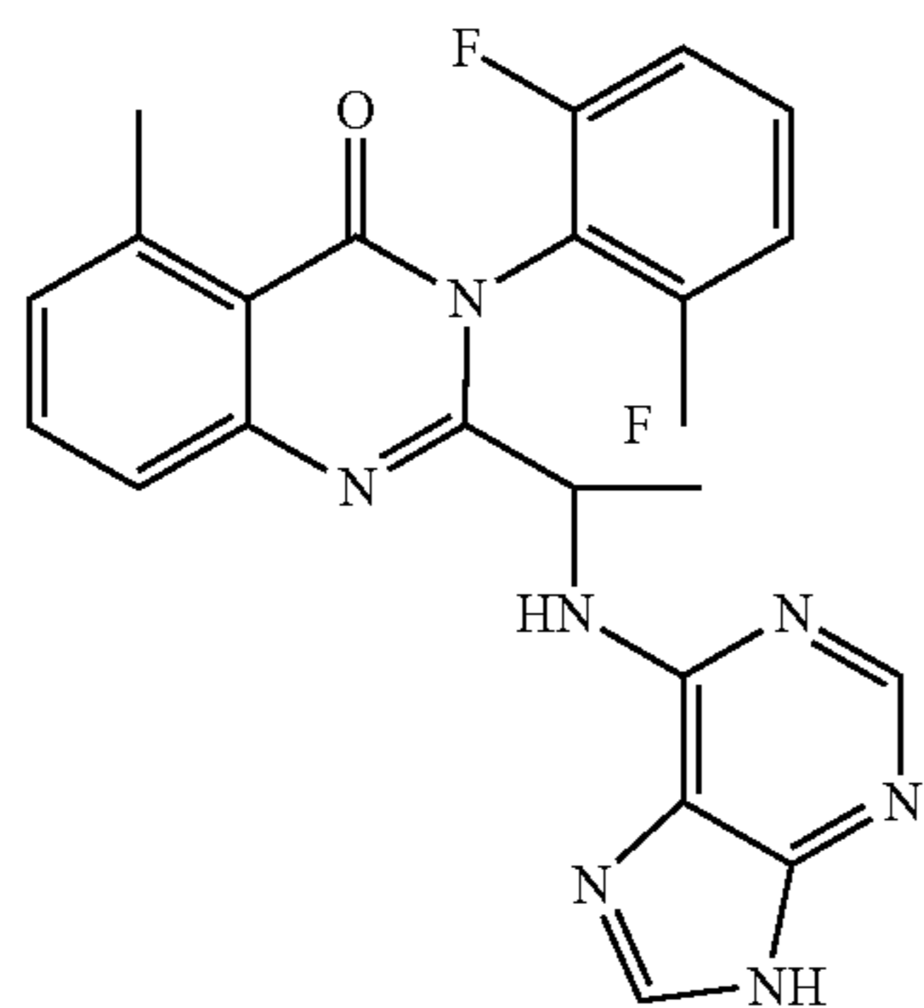
2-[1-(2-amino-9H-purin-6-ylamino)-ethyl]-3-(2,6-difluoro-phenyl)-5-methyl-3H-quinazolin-4-one (20)
