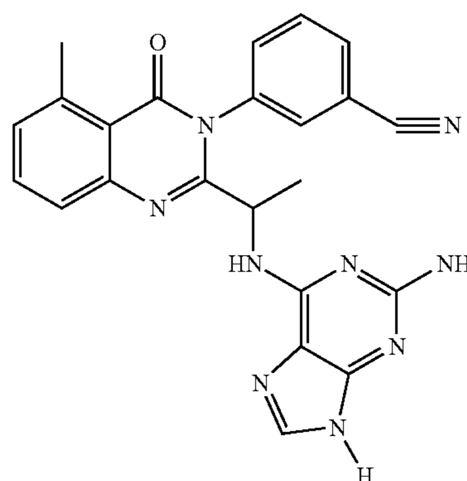
3-{2-[1-(2-Amino-9H-purin-6-ylamino)-ethyl]-5-methyl-4-oxo-4H-quinazolin-3-yl}-benzonitrile
