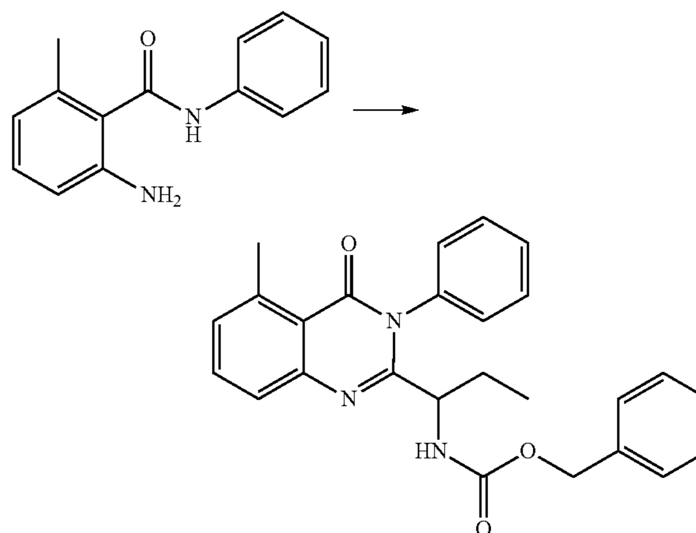
2-(1-amino-propyl)-5-methyl-3-phenyl-3H-quinazolin-4-one (17)
