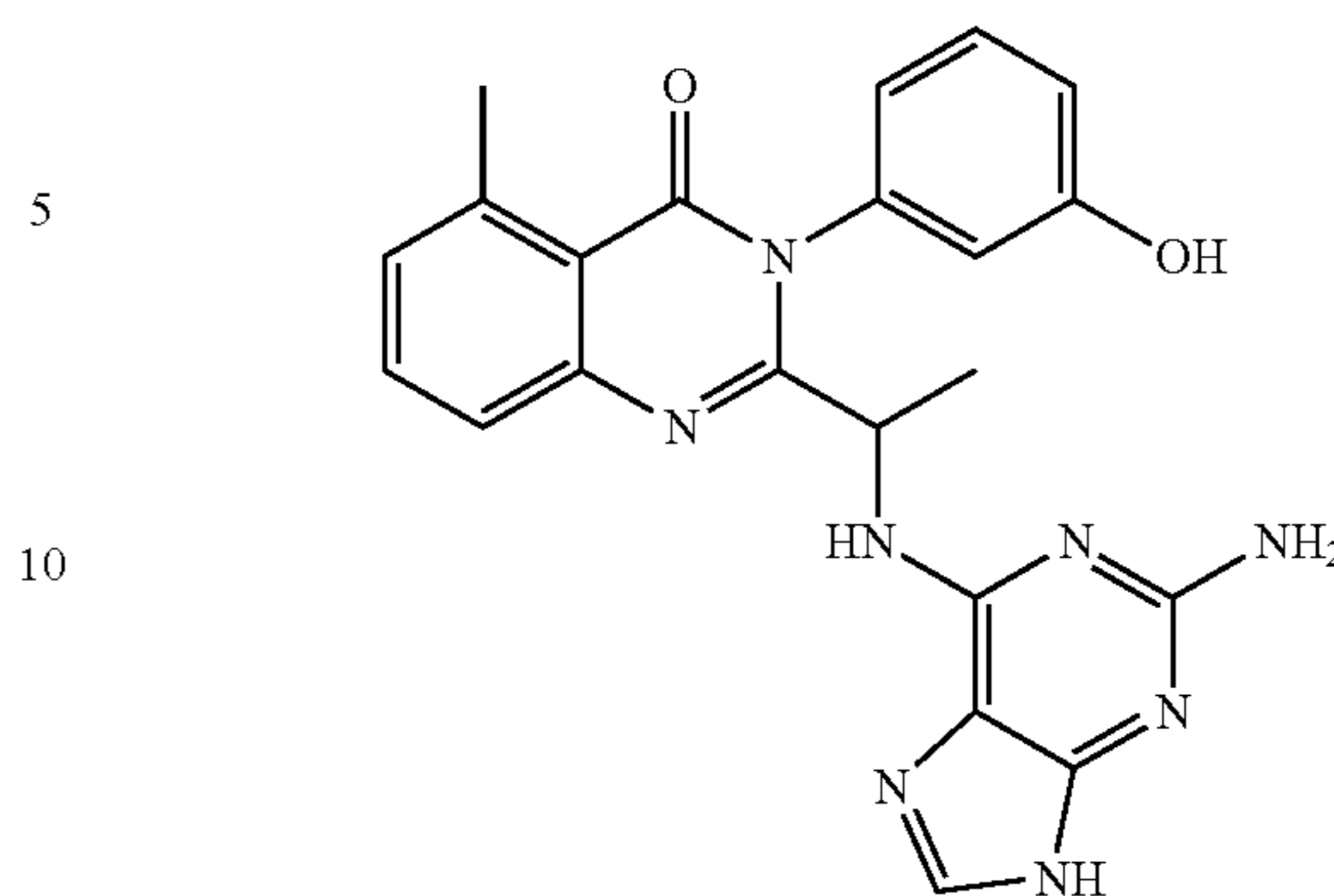
2-[1-(2-Amino-9H-purin-6-ylamino)-ethyl]-3-(3-hydroxy-phenyl)-5-methyl-3H-quinazolin-4-one
