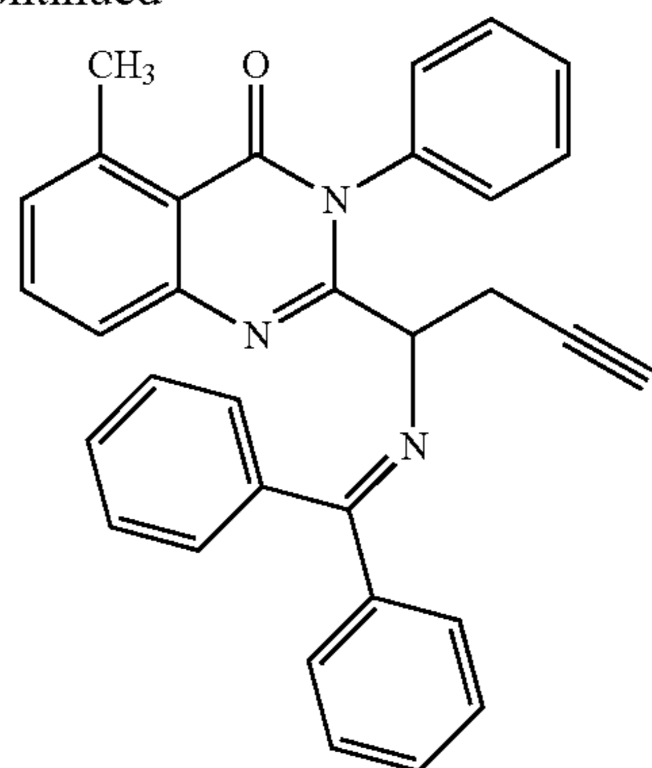
2-(1-amino-but-3-ynyl)-5-methyl-3-phenyl-3H-quinazolin-4-one (164)
