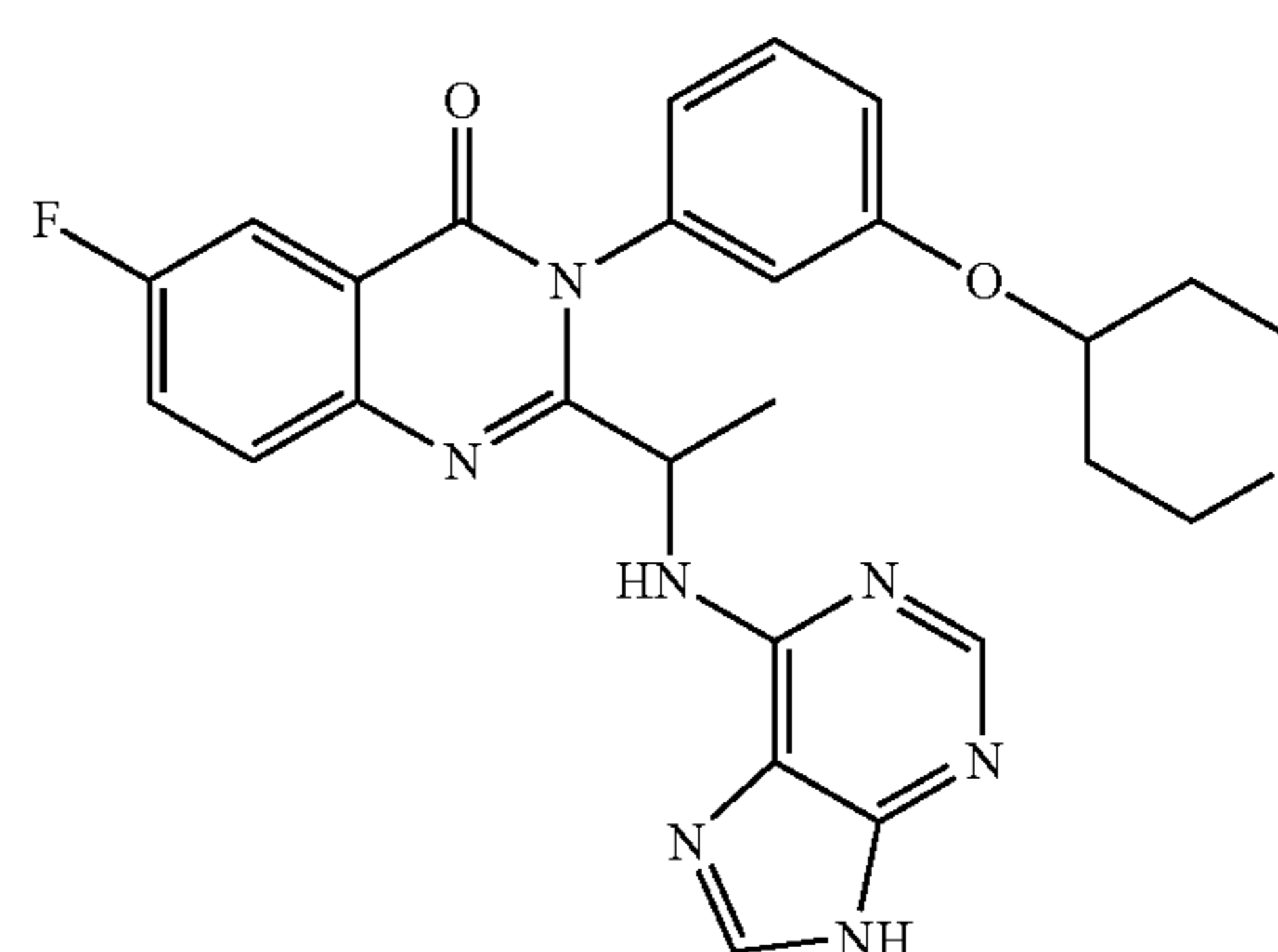
6-Fluoro-2-[1-(9H-purin-6-ylamino)-ethyl]-3-[3-(tetrahydro-pyran-4-yloxy)-phenyl]-3H-quinazolin-4-one
