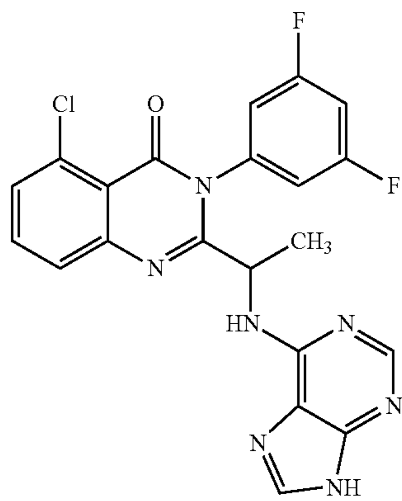
2-[1-(2-amino-9H-purin-6-ylamino)-propyl]-5-chloro-3-(3,5-difluoro-phenyl)-3H-quinazolin-4-one (171)
