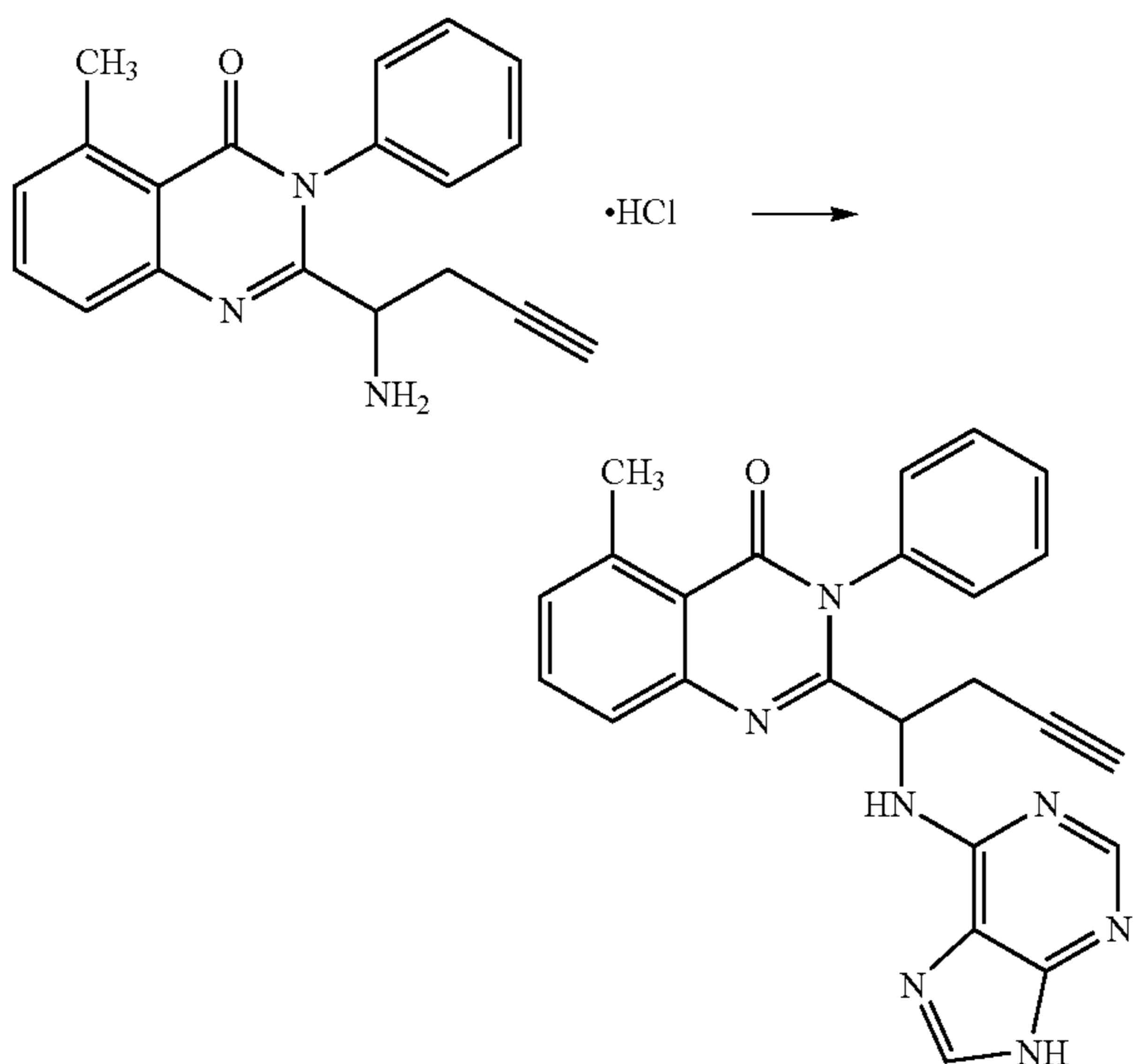
2-[1-(2-amino-9H-purin-6-ylamino)-but-3-ynyl]-5-methyl-3-phenyl-3H-quinazolin-4-one (161)
