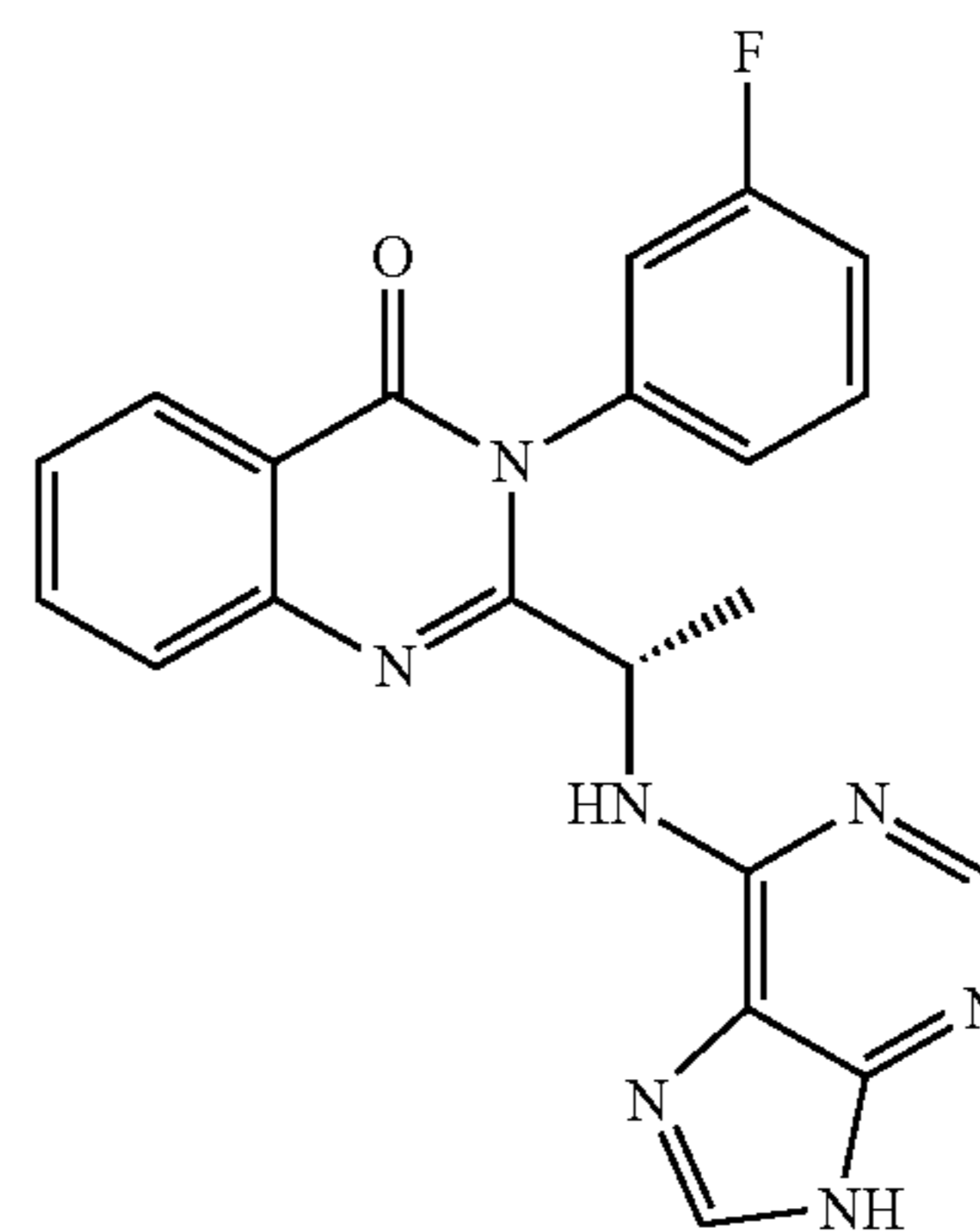
(S)-5-chloro-3-(3,5-difluoro-phenyl)-2-[1-(9H-purin-6-ylamino)-propyl]-3H-quinazolin-4-one (117)
