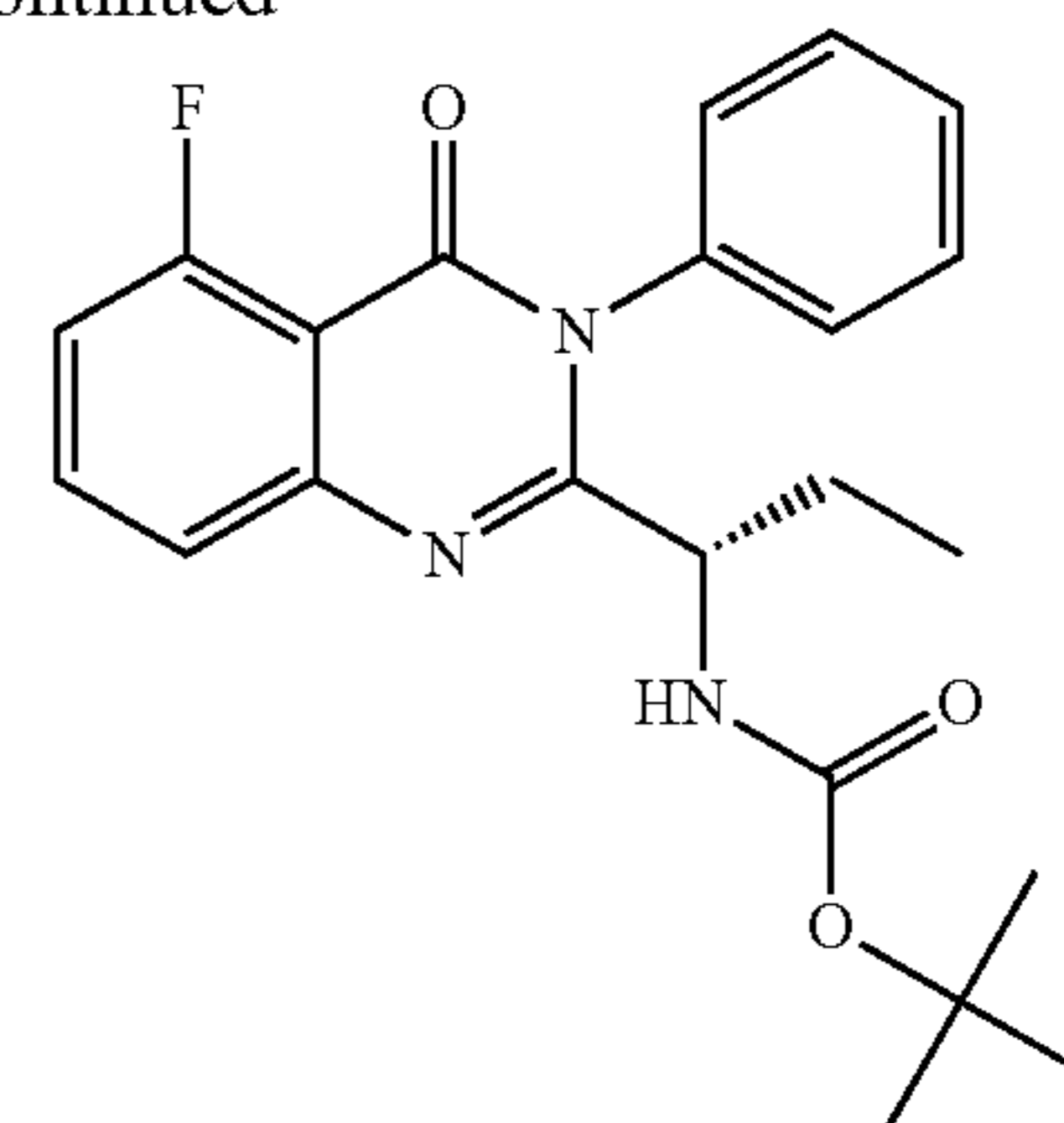
(S)-2-(1-amino-propyl)-5-fluoro-3-phenyl-3H-quinazolin-4-one (111)
