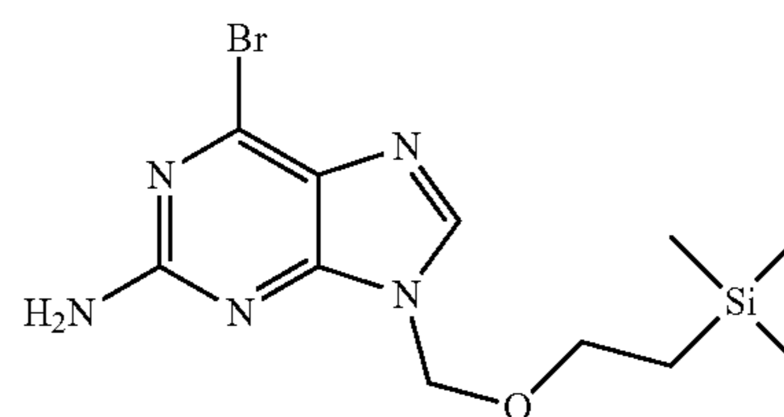
2-di-tert-butylloxycarbonylamino-6-bromo-9-(2-trimethylsilyl-ethoxymethyl)-9H-purine (12)
