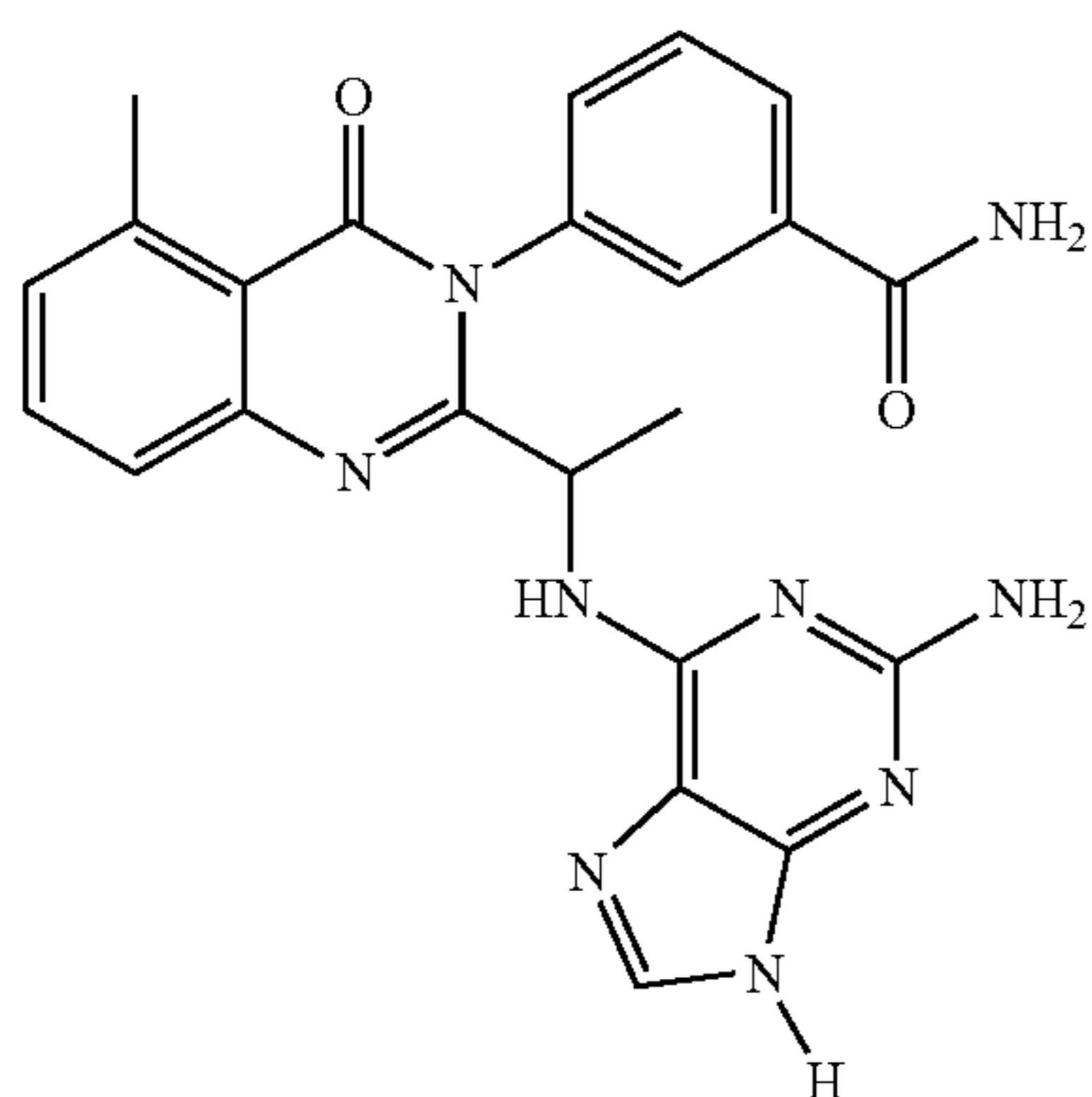
3-{2-[1-(2-Amino-9H-purin-6-ylamino)-ethyl]-5-methyl-4-oxo-4H-quinazolin-3-yl}-benzamide
