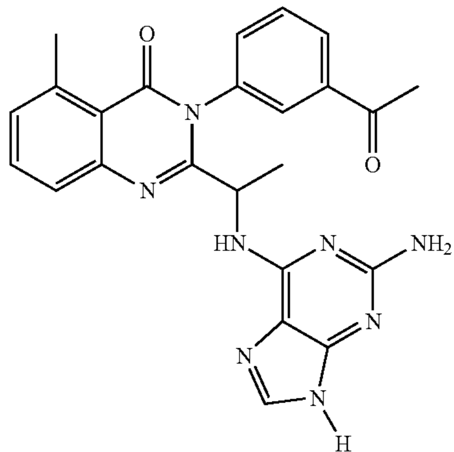
3-(3-Acetyl-phenyl)-2-[1-(2-amino-9H-purin-6-ylamino)-ethyl]-5-methyl-3H-quinazolin-4-one
