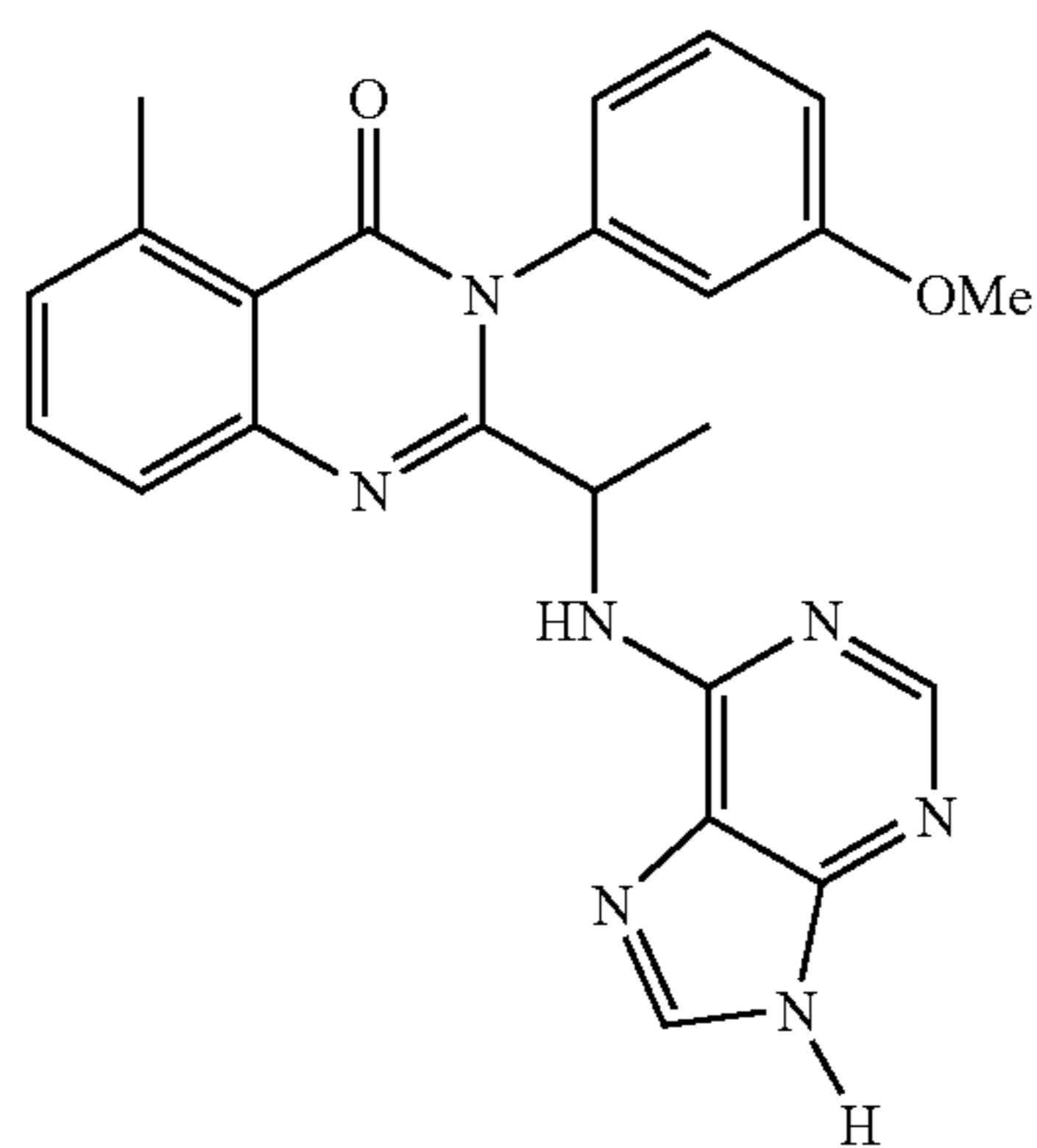
3-(3-Methoxy-phenyl)-5-methyl-2-[1-(9H-purin-6-ylamino)-ethyl]-3H-quinazolin-4-one
