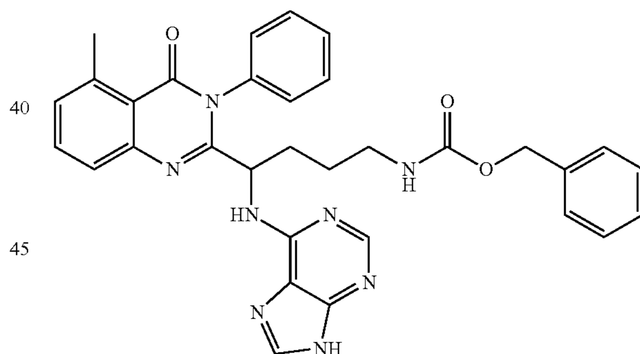
[4-(2-amino-9H-purin-6-ylamino)-4-(5-methyl-4-oxo-3-phenyl-3,4-dihydro-quinazolin-2-yl)-butyl]-carbamic acid benzyl ester (52)
