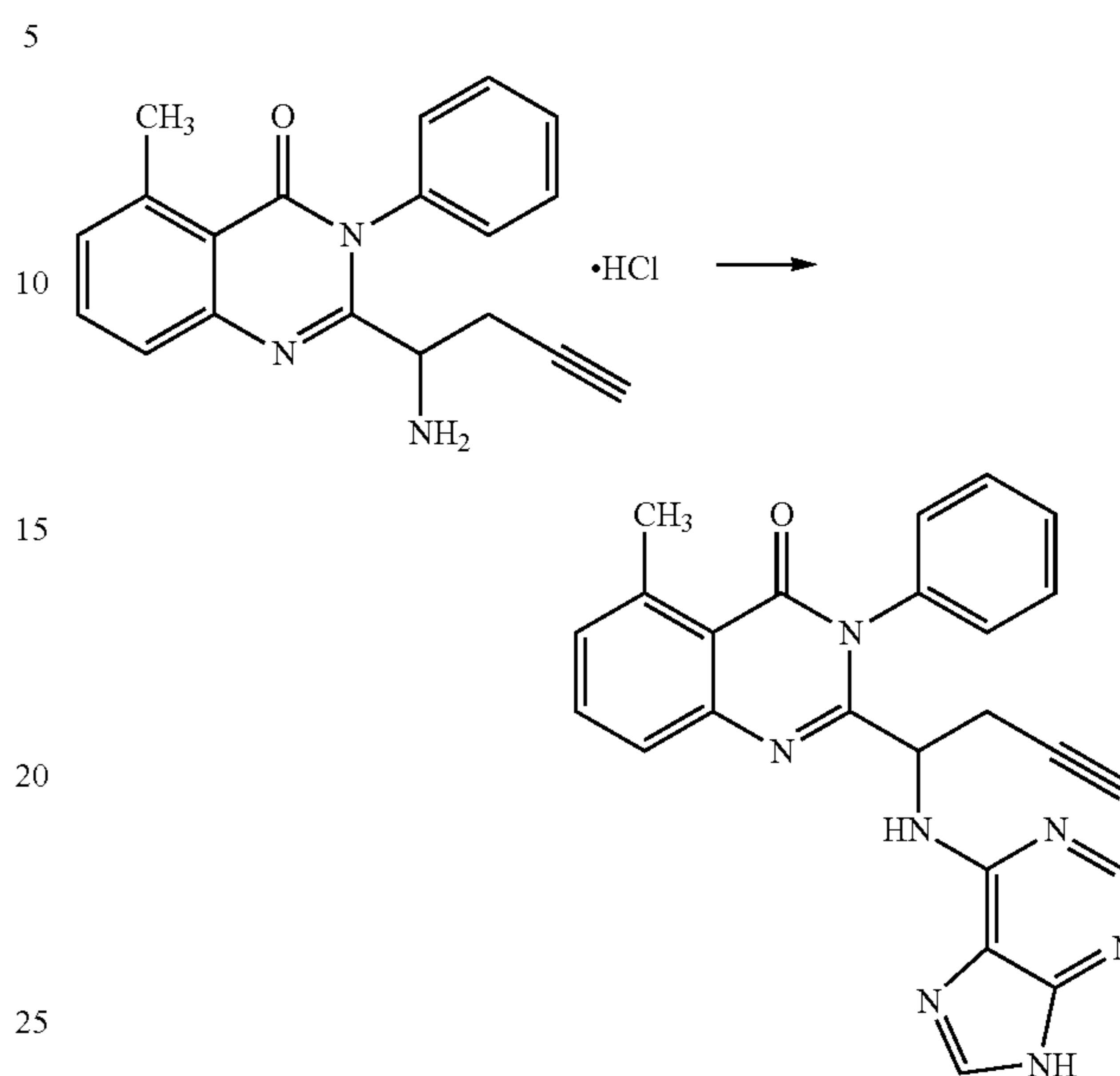
2-(1-amino-but-3-ynyl)-5-methyl-3-phenyl-3H-quinazolin-4-one (164)
