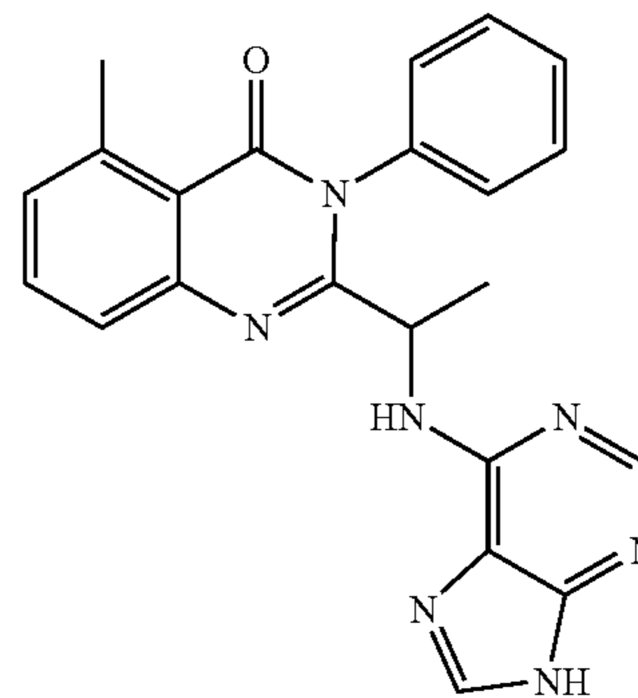
2-[1-(2-amino-9H-purin-6-ylamino)-ethyl]-5-methyl-3-phenyl-3H-quinazolin-4-one (27)
