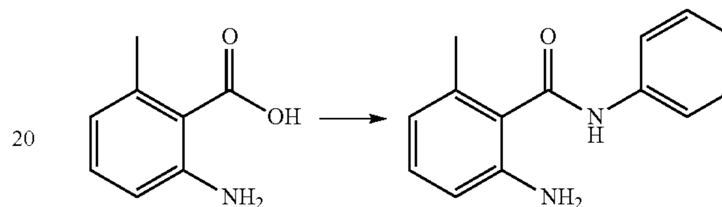
[1-(5-methyl-4-oxo-3-phenyl-3,4-dihydroquinazolin-2-yl)propyl]-carbamic acid benzyl ester (16)
