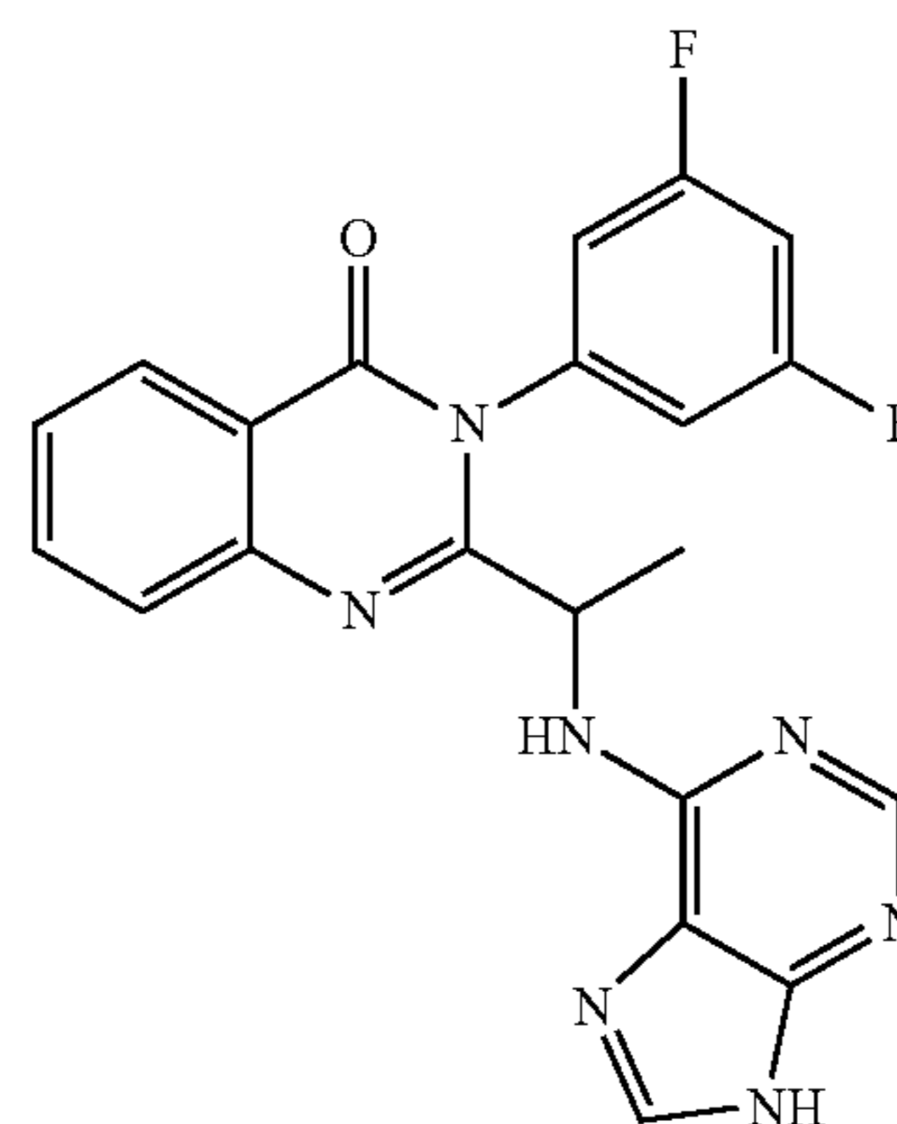
2-[1-(5-bromo-7H-pyrrolo[2,3-d]pyrimidin-4-ylamino)-ethyl]-3-(3-fluoro-phenyl)-5-methyl-3H-quinazolin-4-one (96)
