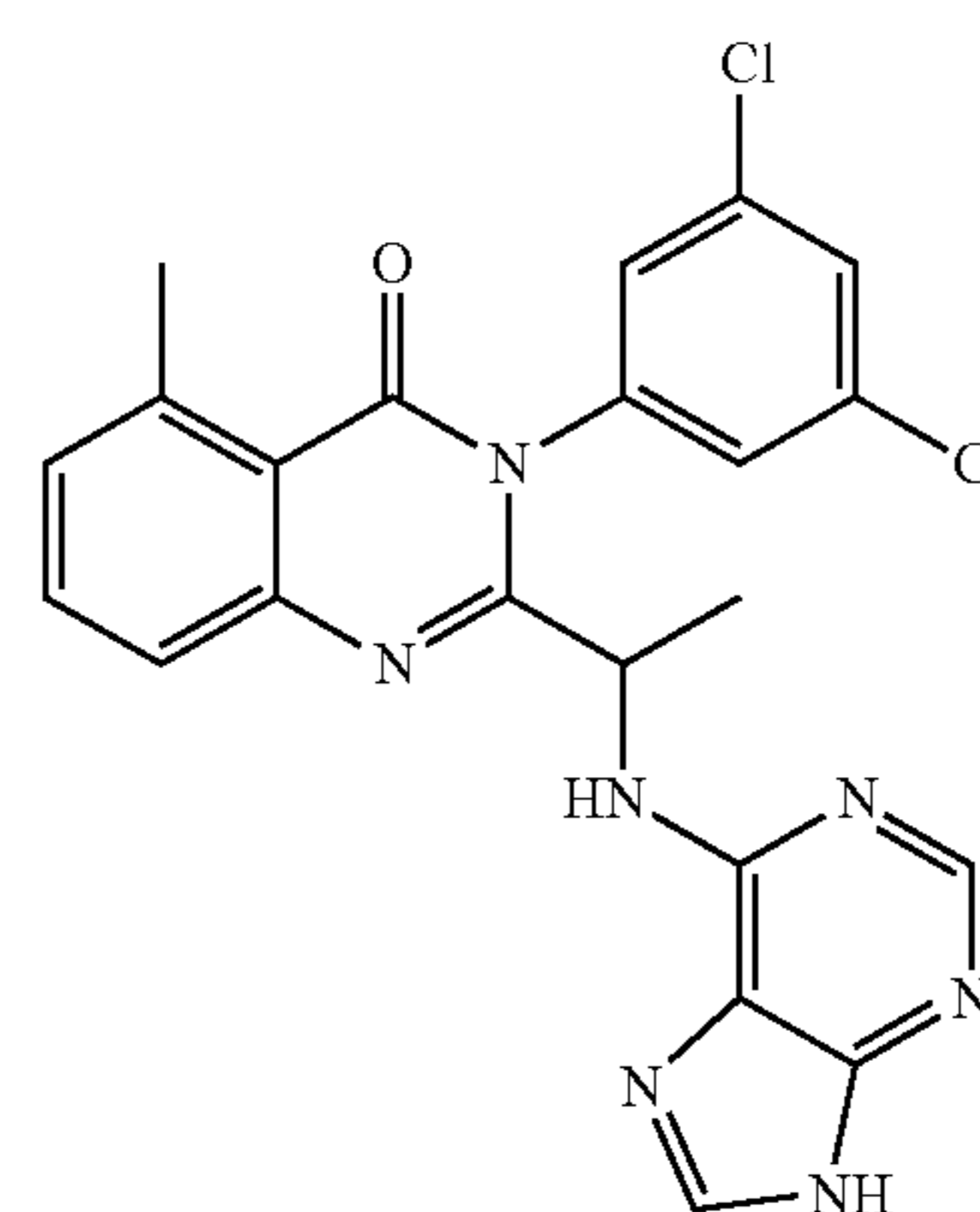
3-(2,6-dichloro-phenyl)-5-methyl-2-[1-(9H-purin-6-ylamino)-ethyl]-3H-quinazolin-4-one (80)
