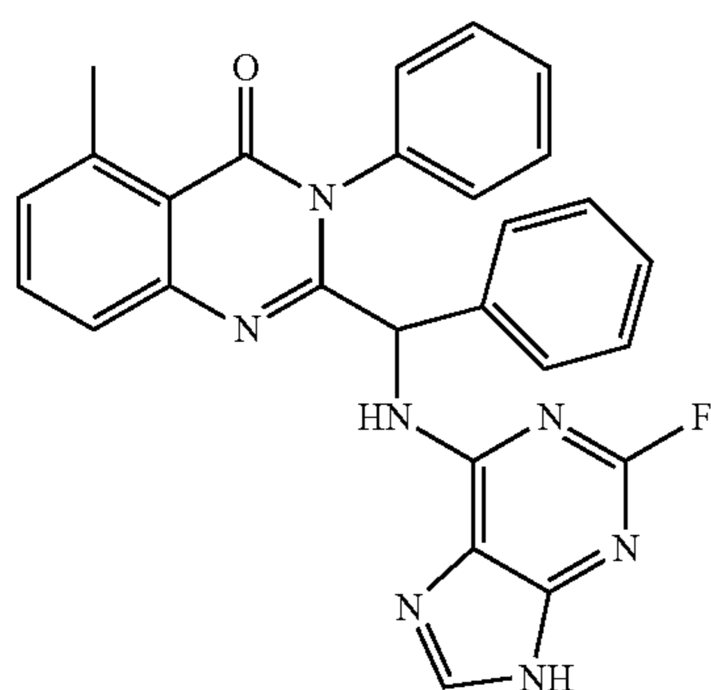
5-methyl-3-phenyl-2-[phenyl-(7H-pyrrolo[2,3-d]pyrimidin-4-ylamino)-methyl]-3H-quinazolin-4-one (45)
