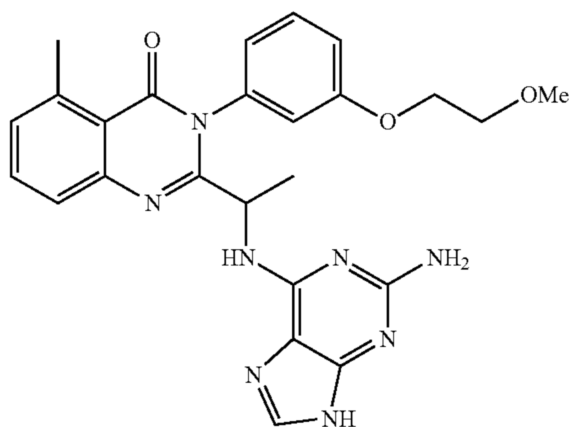
2-[1-(2-Amino-9H-purin-6-ylamino)-ethyl]-3-[3-(2-methoxy-ethoxy)-phenyl]-5-methyl-3H-quinazolin-4-one
