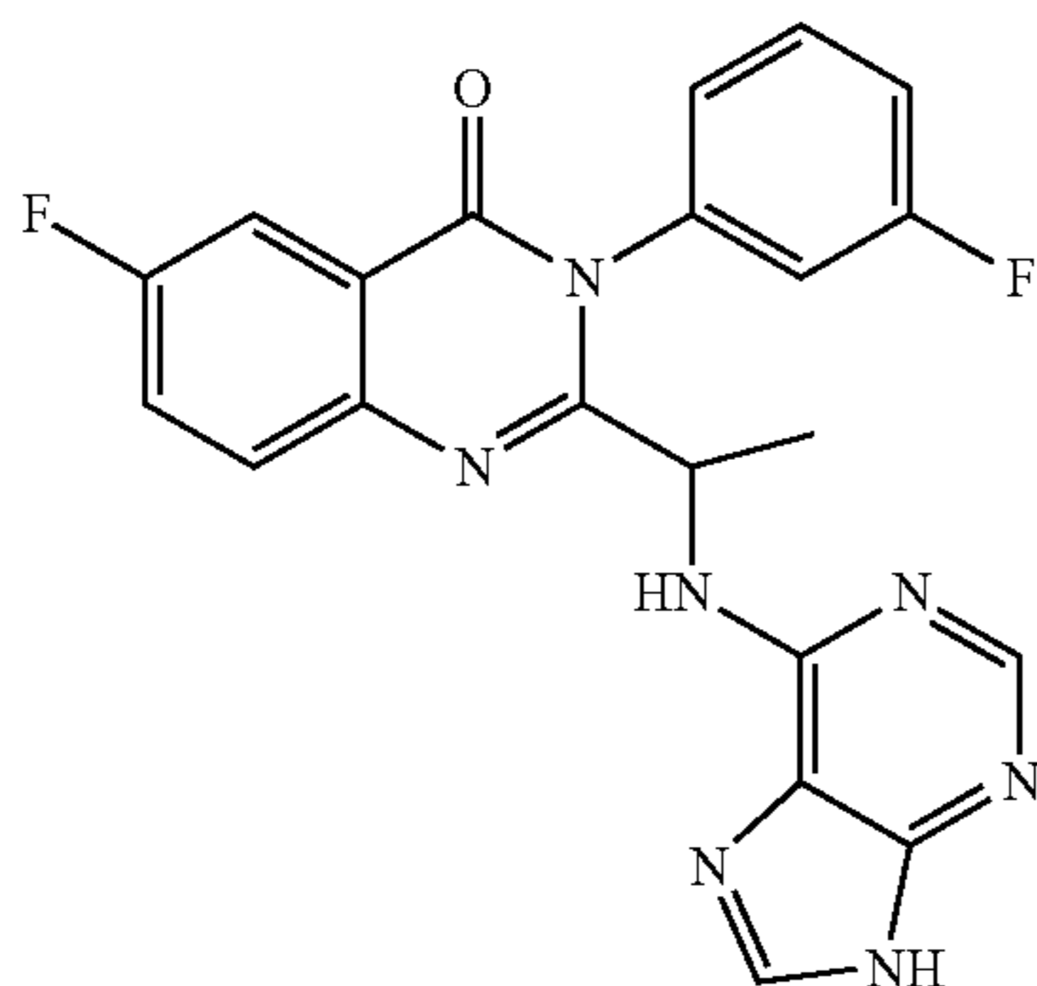
2-[4-diethylamino-1-(9H-purin-6-ylamino)-butyl]-5-methyl-3-phenyl-3H-quinazolin-4-one (103)
