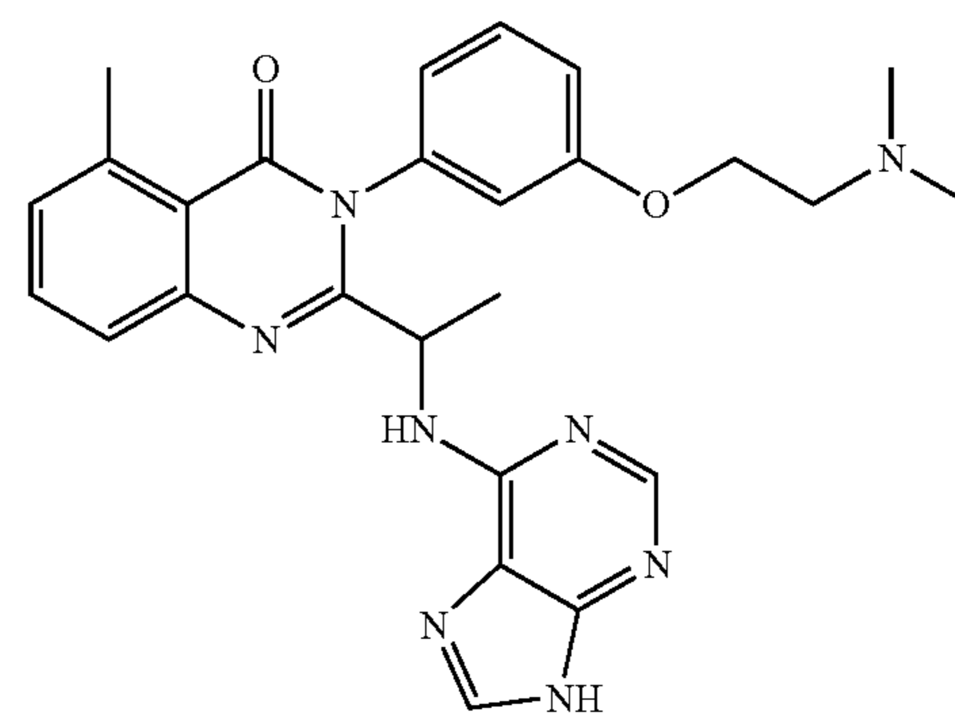
3-[3-(2-Dimethylamino-ethoxy)-phenyl]-5-methyl-2-[1-(9H-purin-6-ylamino)-ethyl]-3H-quinazolin-4-one (129)
