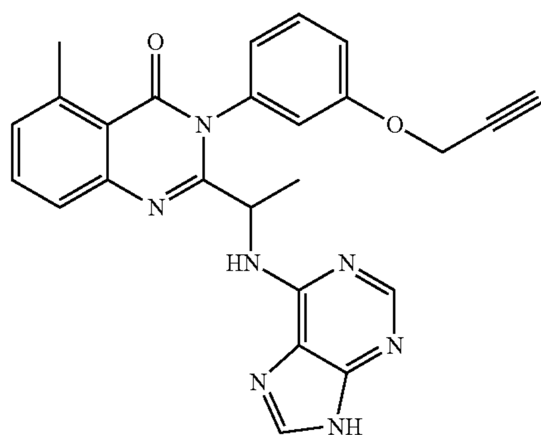
5-Methyl-3-(3-prop-2-ynoxy-phenyl)-2-[1-(9H-purin-6-ylamino)-ethyl]-3H-quinazolin-4-one
