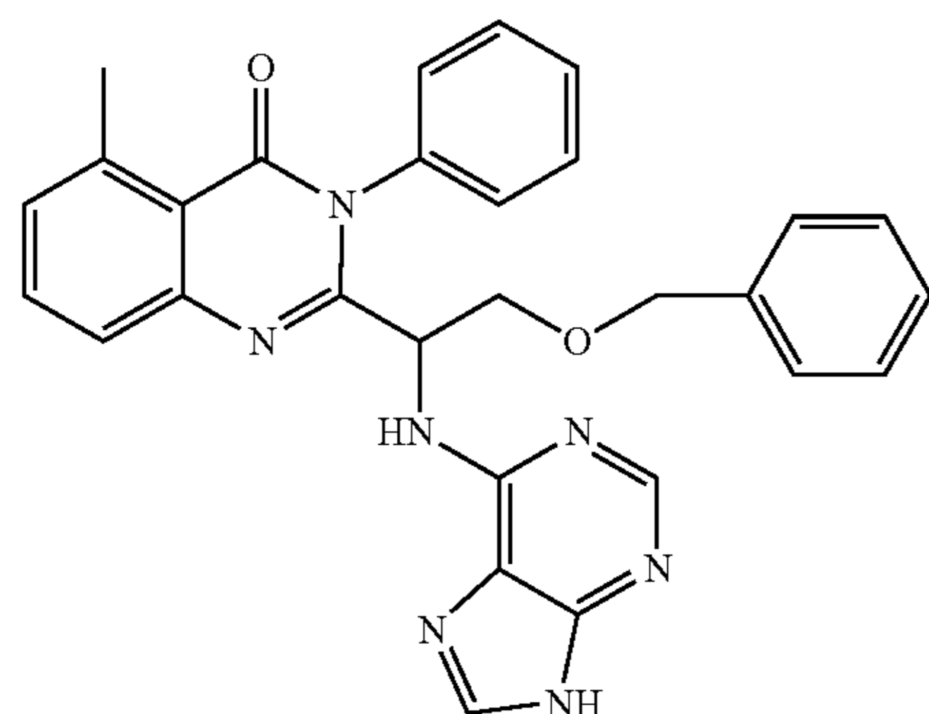
2-[1-(2-amino-9H-purin-6-ylamino)-2-benzyloxy-ethyl]-5-methyl-3-phenyl-3H-quinazolin-4-one (29)
