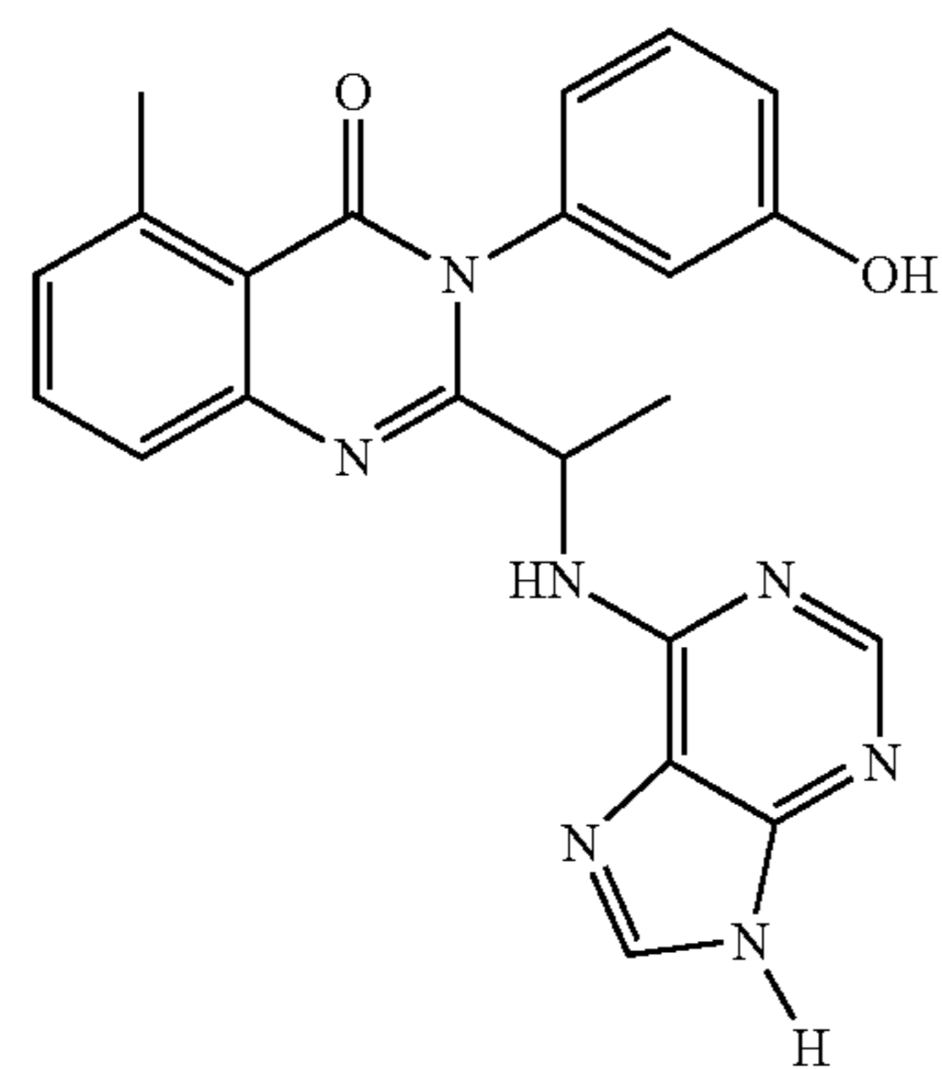
3-(3-Hydroxy-phenyl)-5-methyl-2-[1-(9H-purin-6-ylamino)-ethyl]-3H-quinazolin-4-one
