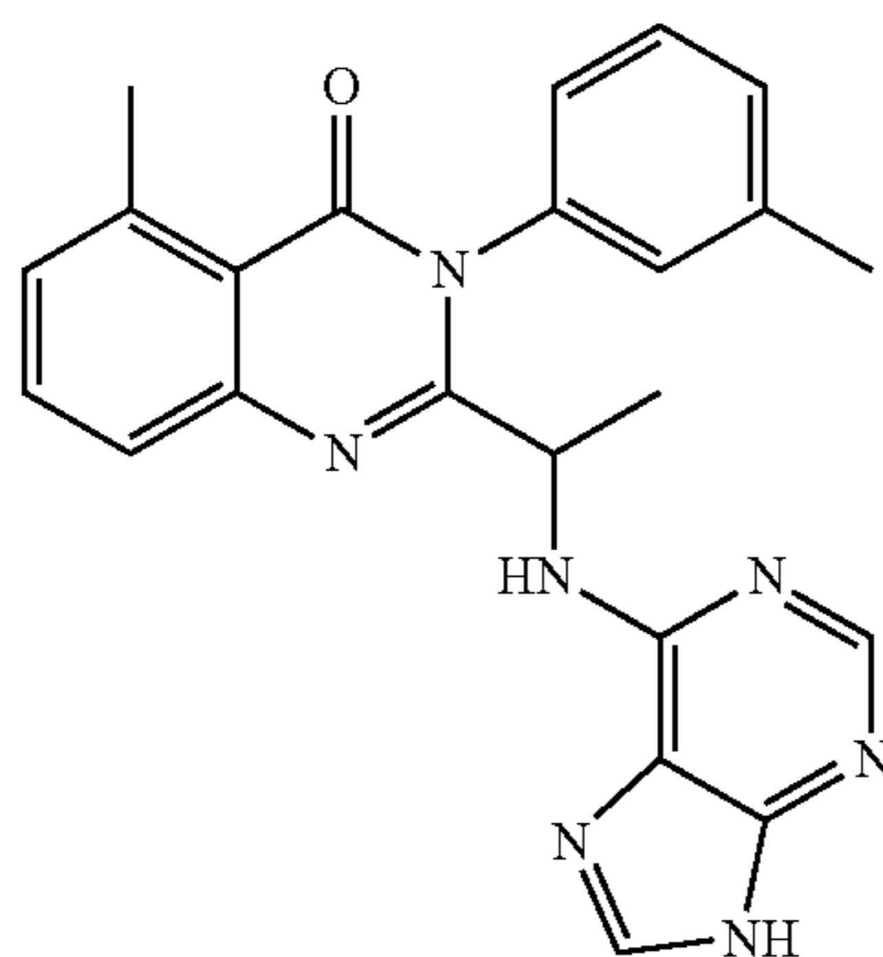
2-[1-(2-amino-9H-purin-6-ylamino)-ethyl]-3-(3-methyl-phenyl)-5-methyl-3H-quinazolin-4-one (65)
