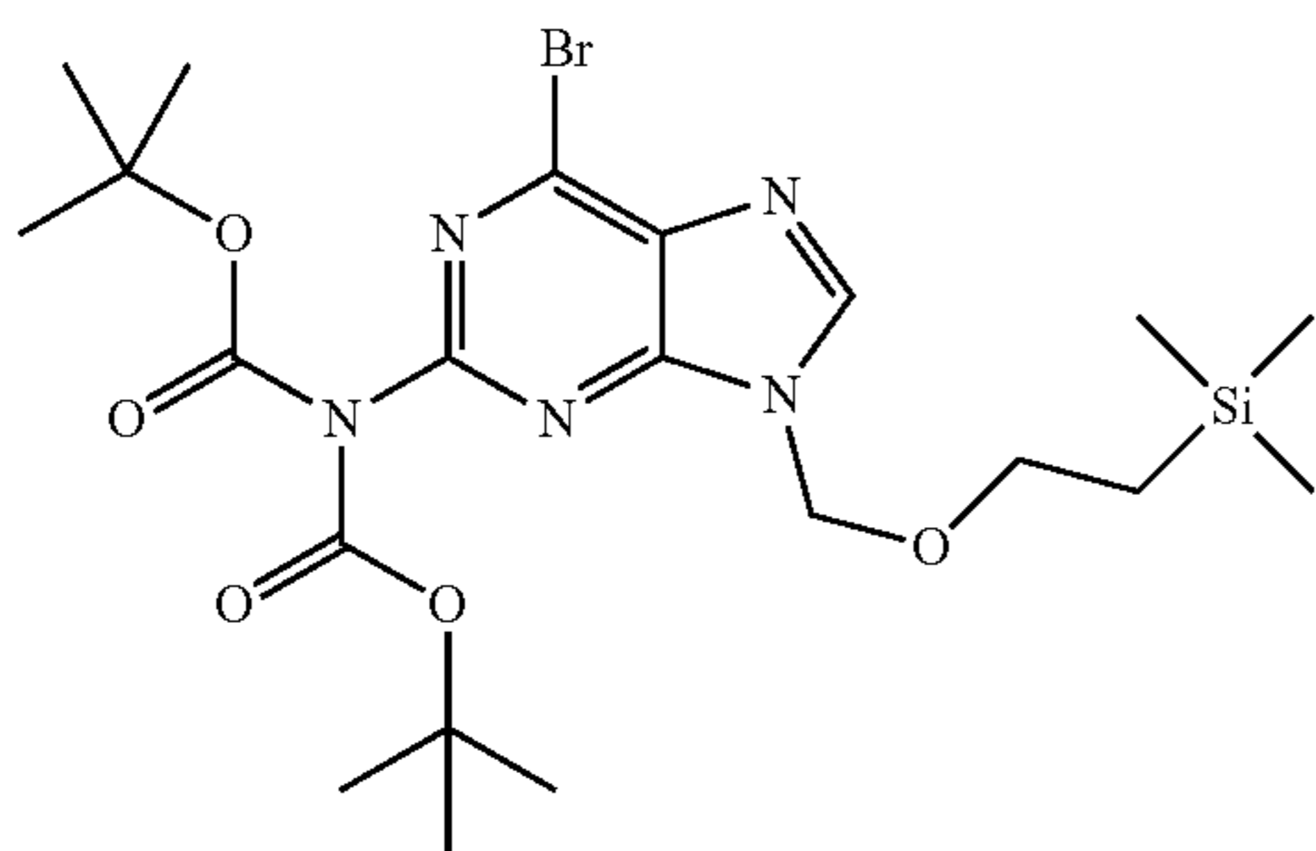
6-chloro-9-(2-trimethylsilyl-ethoxymethyl)-9H-purine (13)
