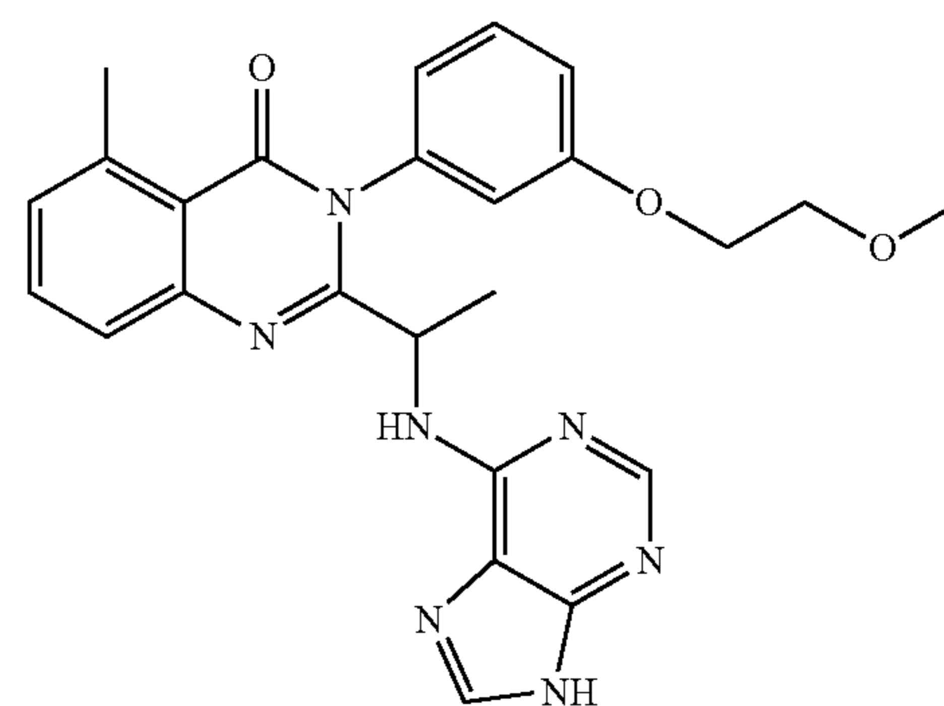
3-[3-(2-Methoxy-ethoxy)-phenyl]-5-methyl-2-[1-(9H-purin-6-ylamino)-ethyl]-3H-quinazolin-4-one
