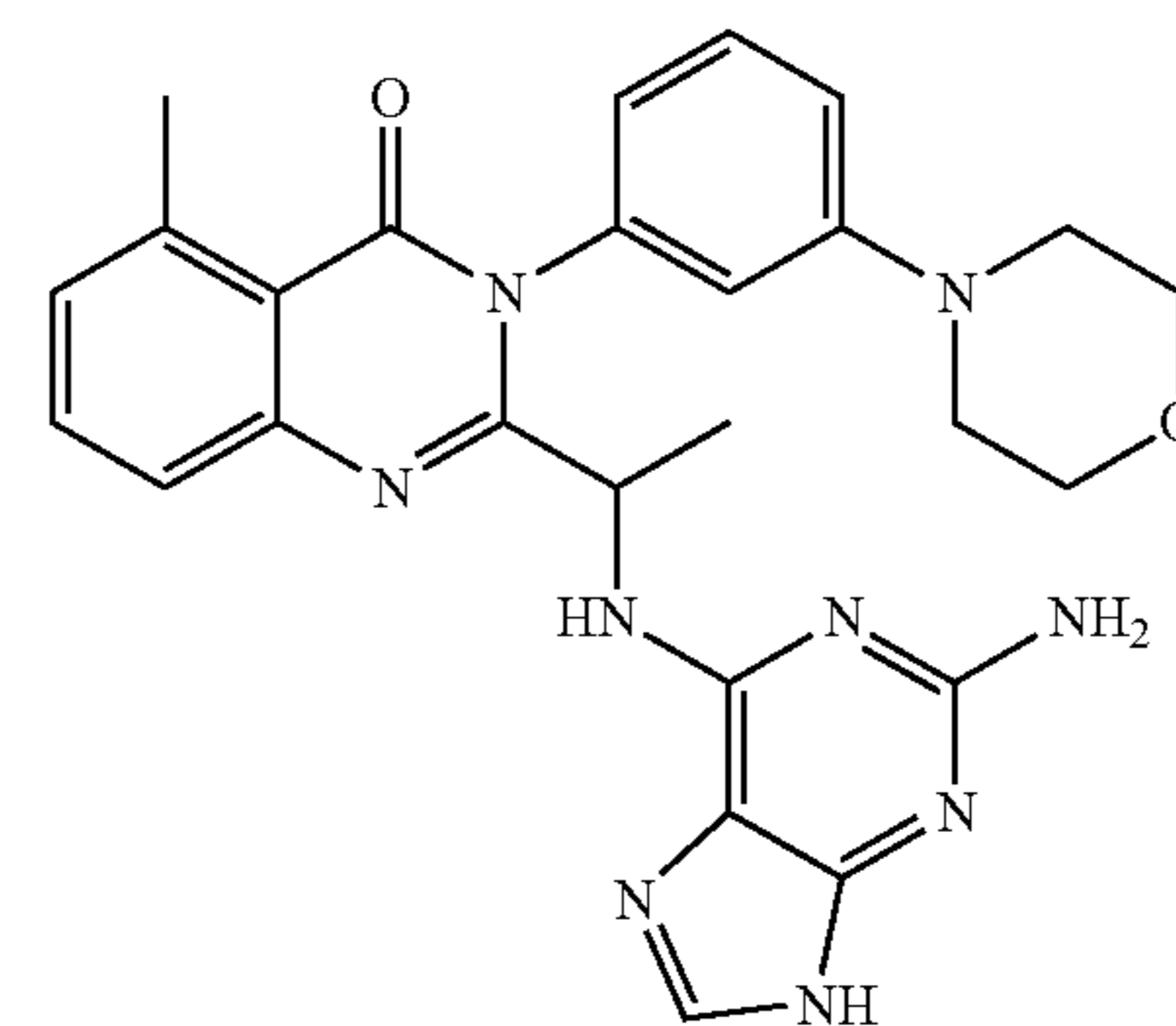
2-[1-(2-Amino-9H-purin-6-ylamino)-ethyl]-5-methyl-3-(3-morpholin-4-yl-phenyl)-3H-quinazolin-4-one
