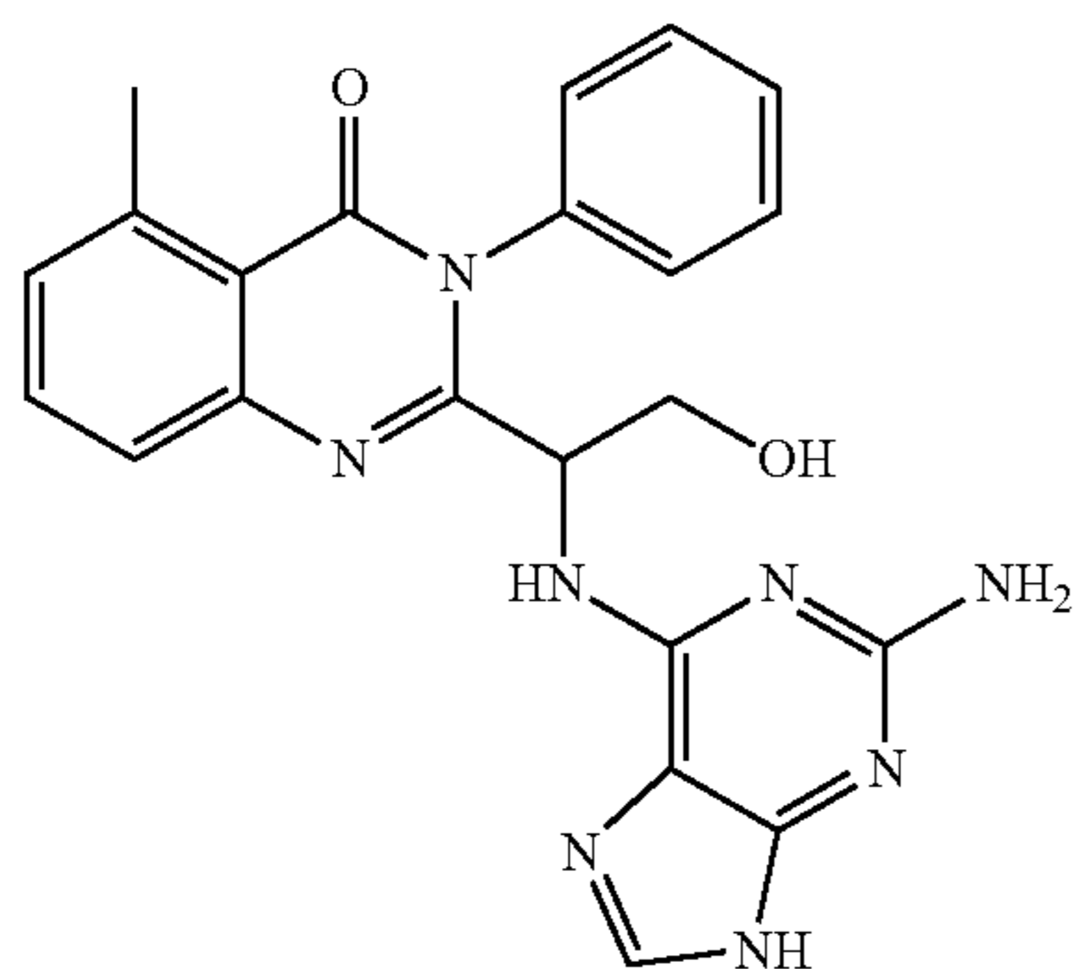
2-[1-(2-amino-9H-purin-6-ylamino)-ethyl]-3-(3-fluoro-phenyl)-3H-quinazolin-4-one (69)
