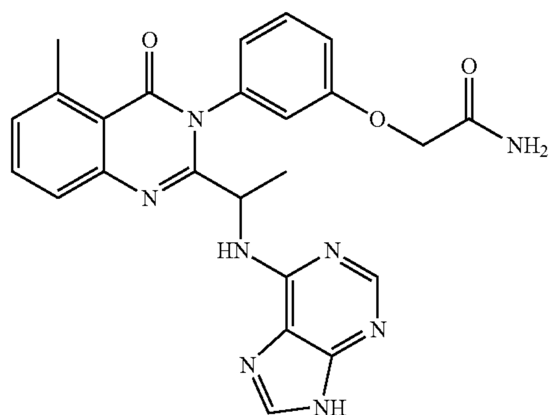
2-(3-(5-Methyl-4-oxo-2-[1-(9H-purin-6-ylamino)-ethyl]-4H-quinazolin-3-yl)-phenoxy)-acetamide
