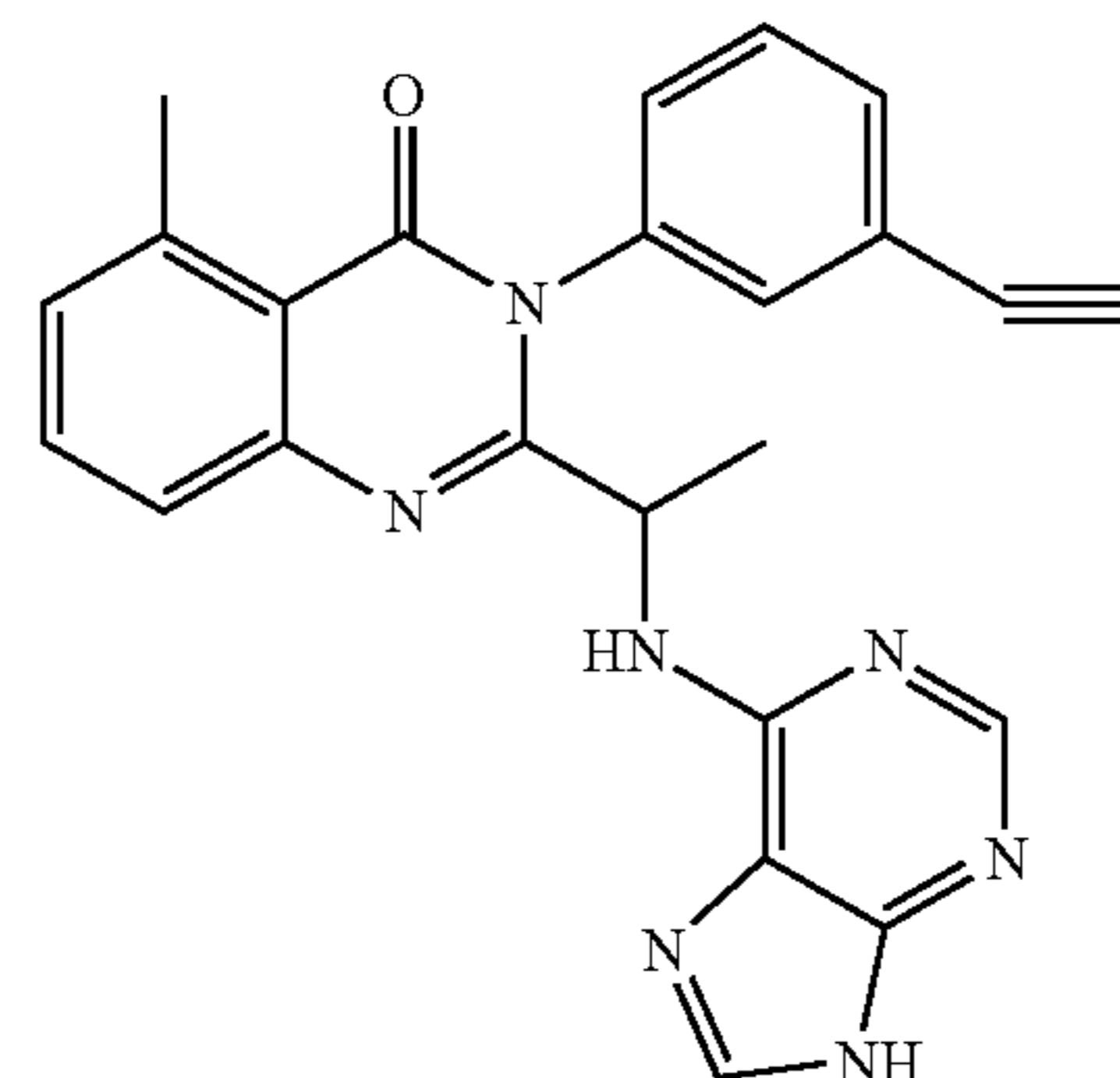
3-(3-Ethynyl-phenyl)-5-methyl-2-[1-(9H-purin-6-ylamino)-ethyl]-3H-quinazolin-4-one
