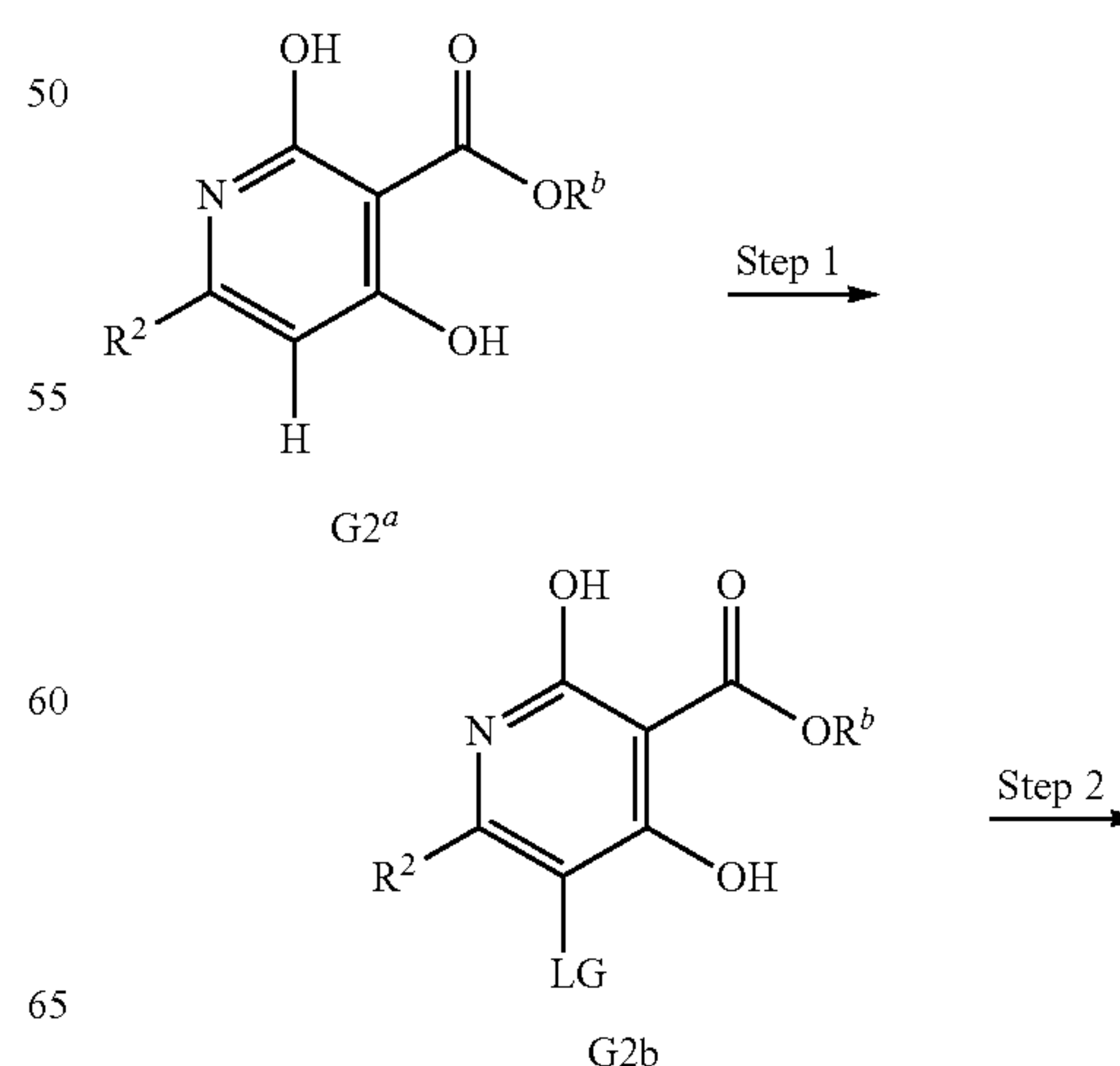
Scheme 2
