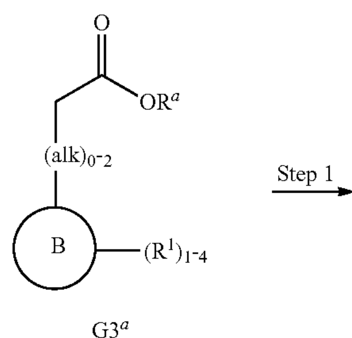
Scheme 3
