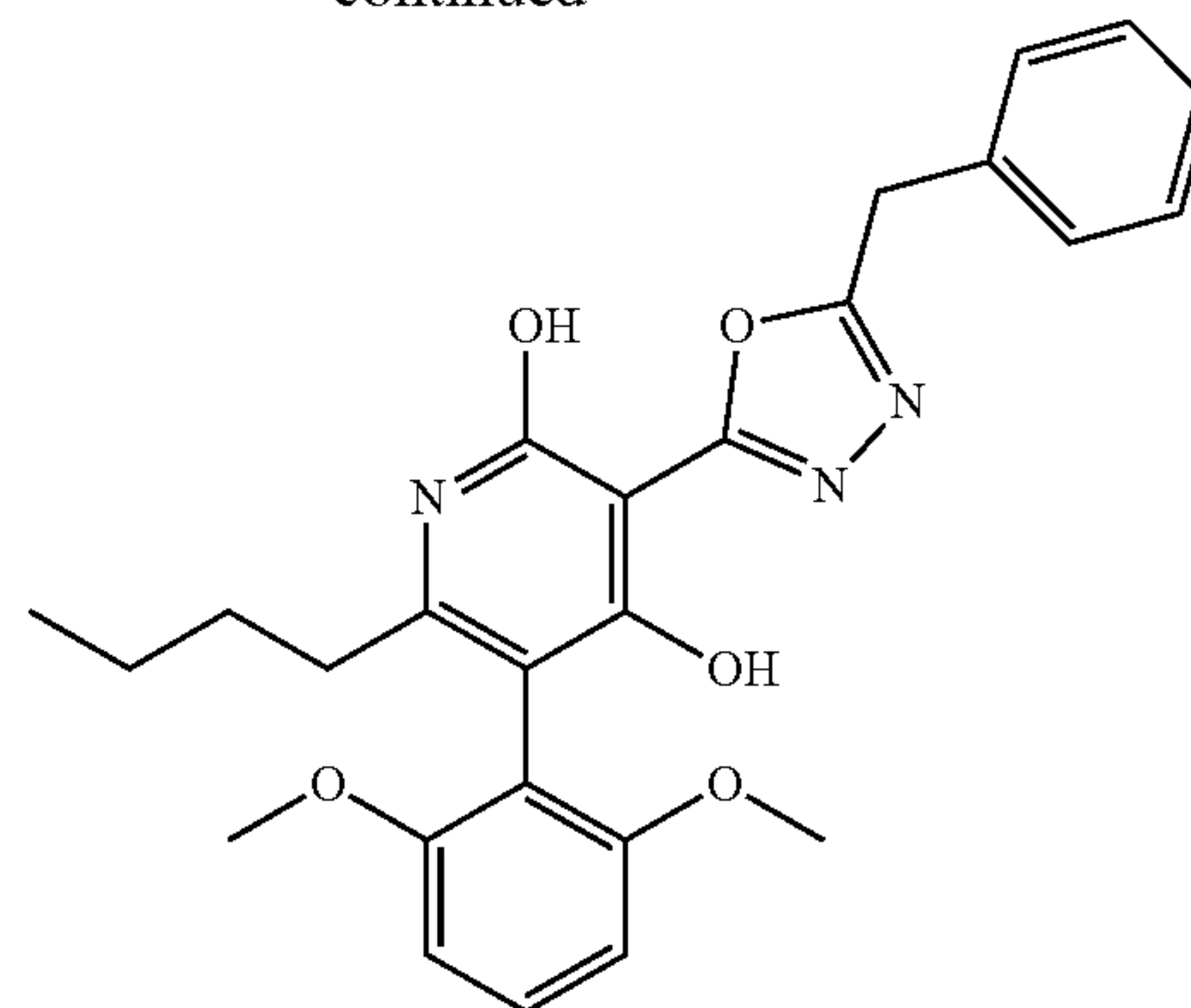
Example 1
