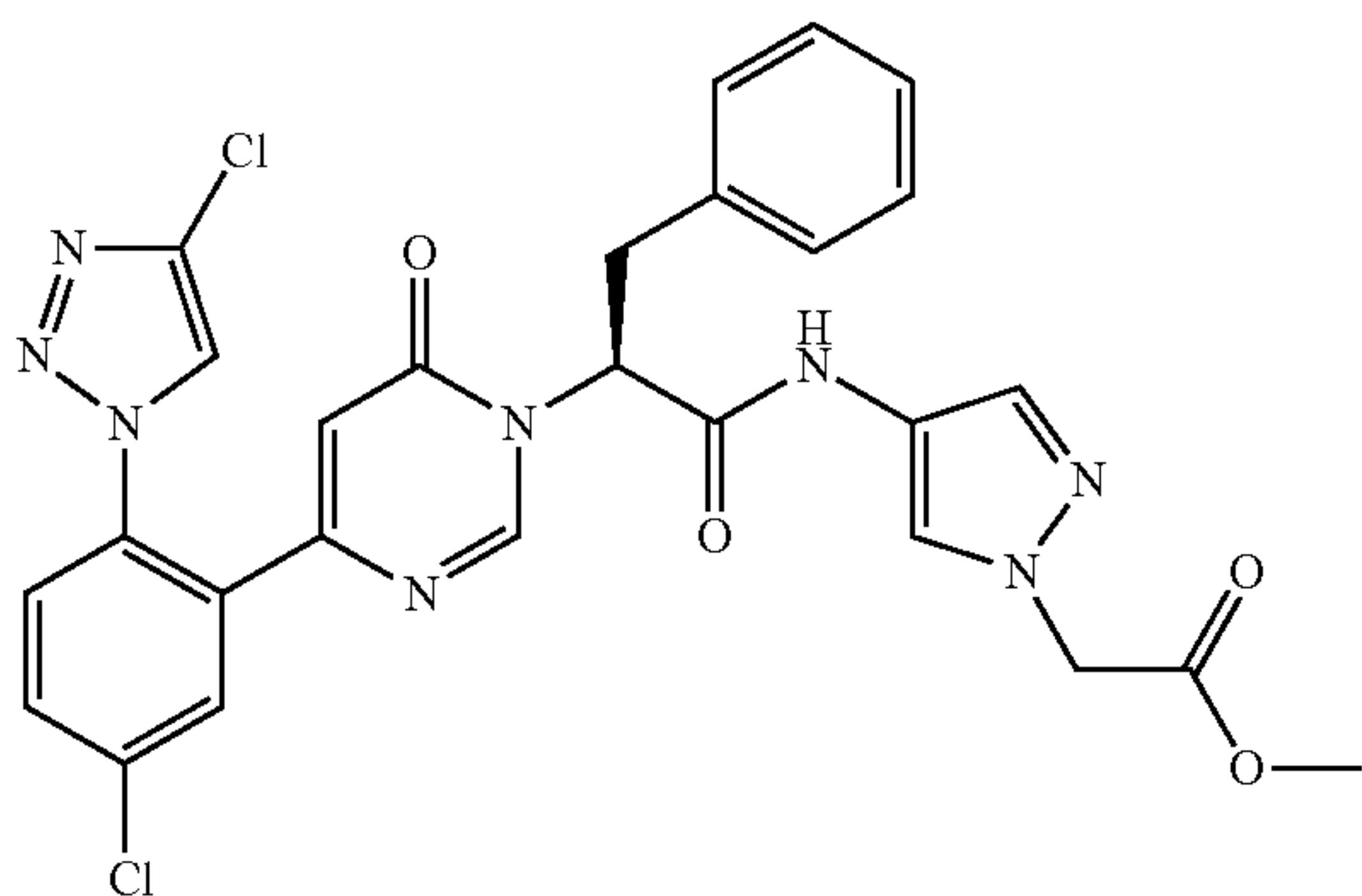
10A. Preparation of Methyl 2-(4-amino-1H-pyrazol-1-yl)acetate
