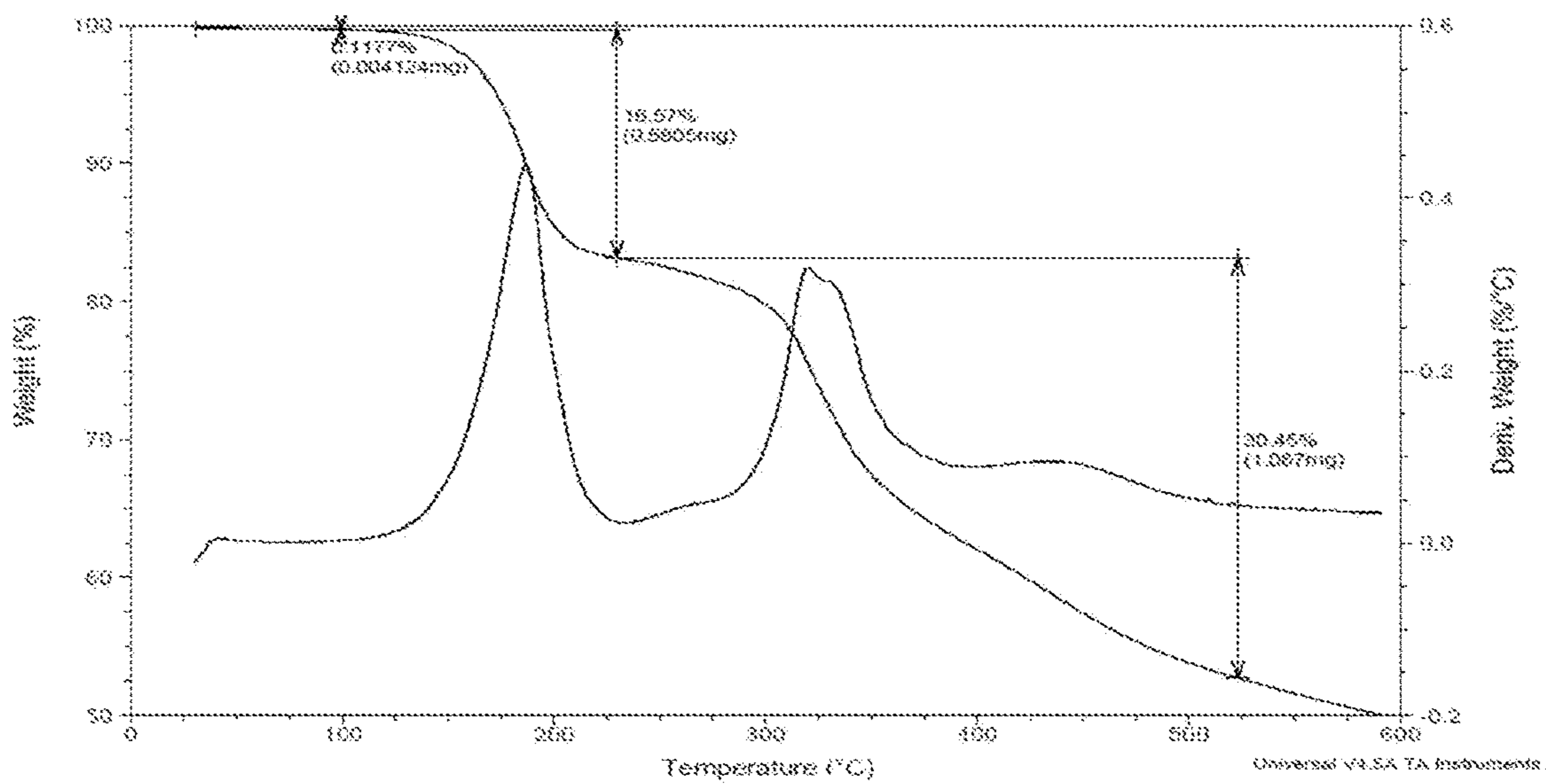
Figure 6. TGA Dihydrochloric Acid Salt
