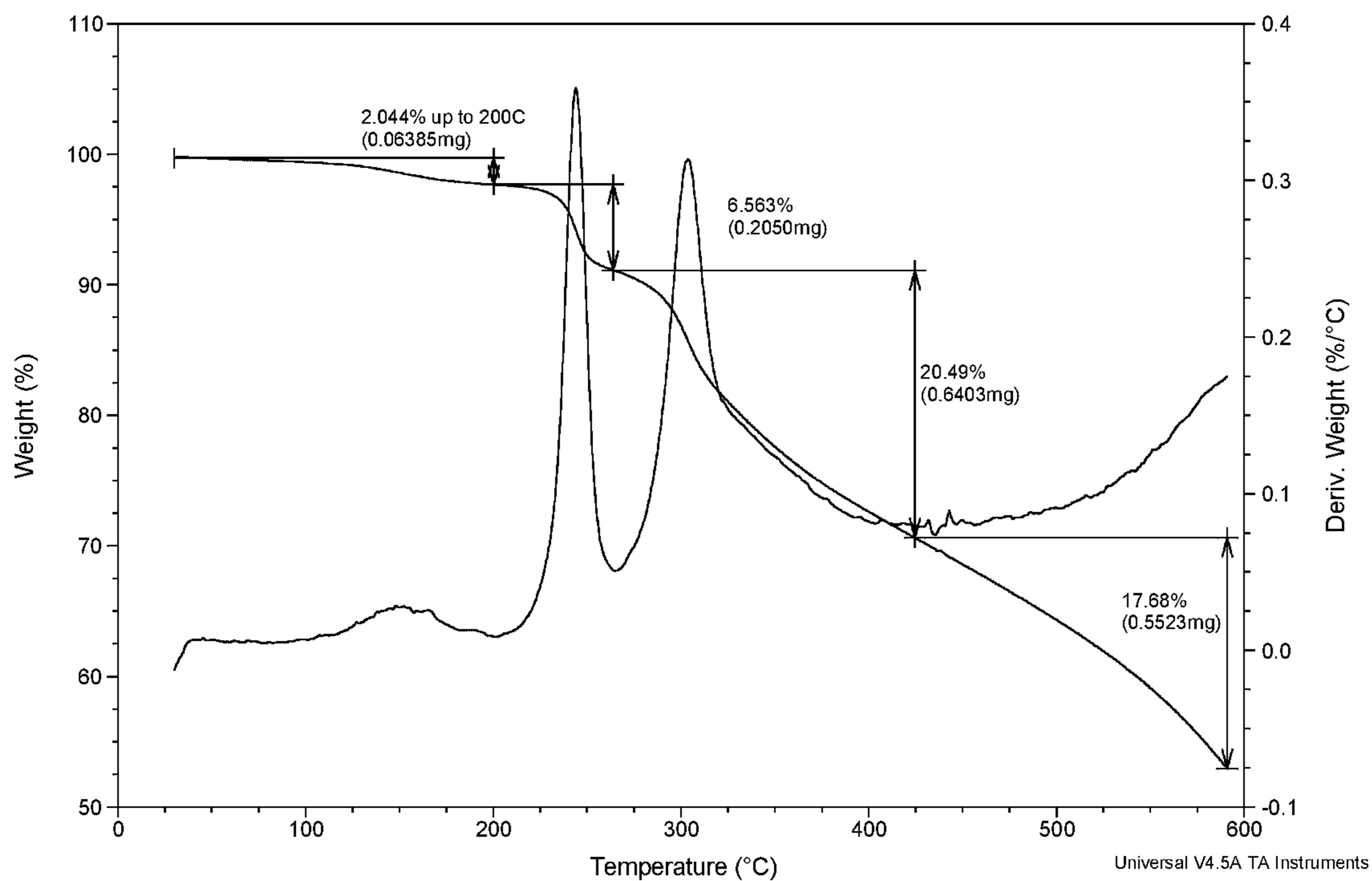
Figure 3. TGA Phosphoric Acid Salt (Form I)
