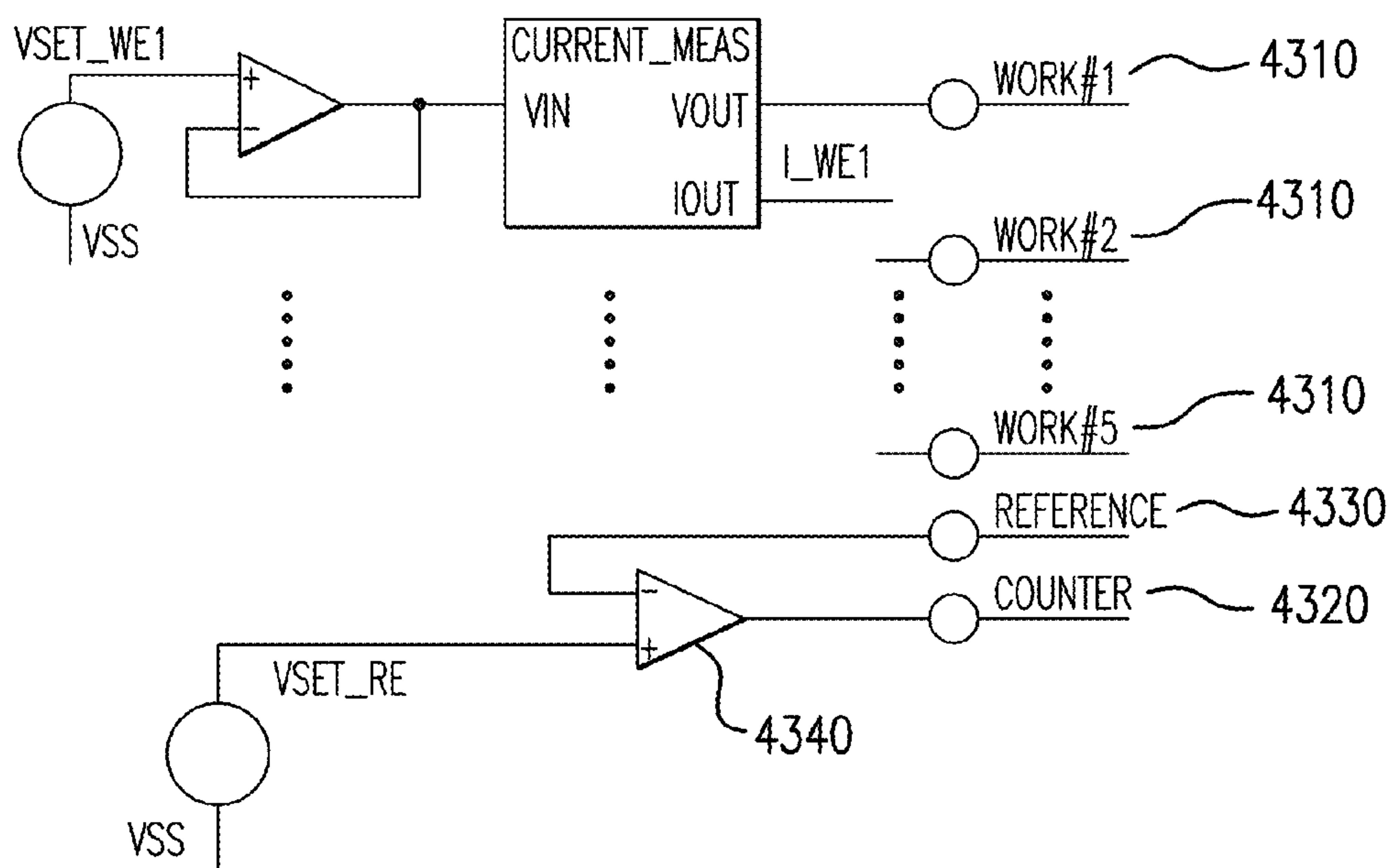
POTENTIOSTAT CONFIGURATION
