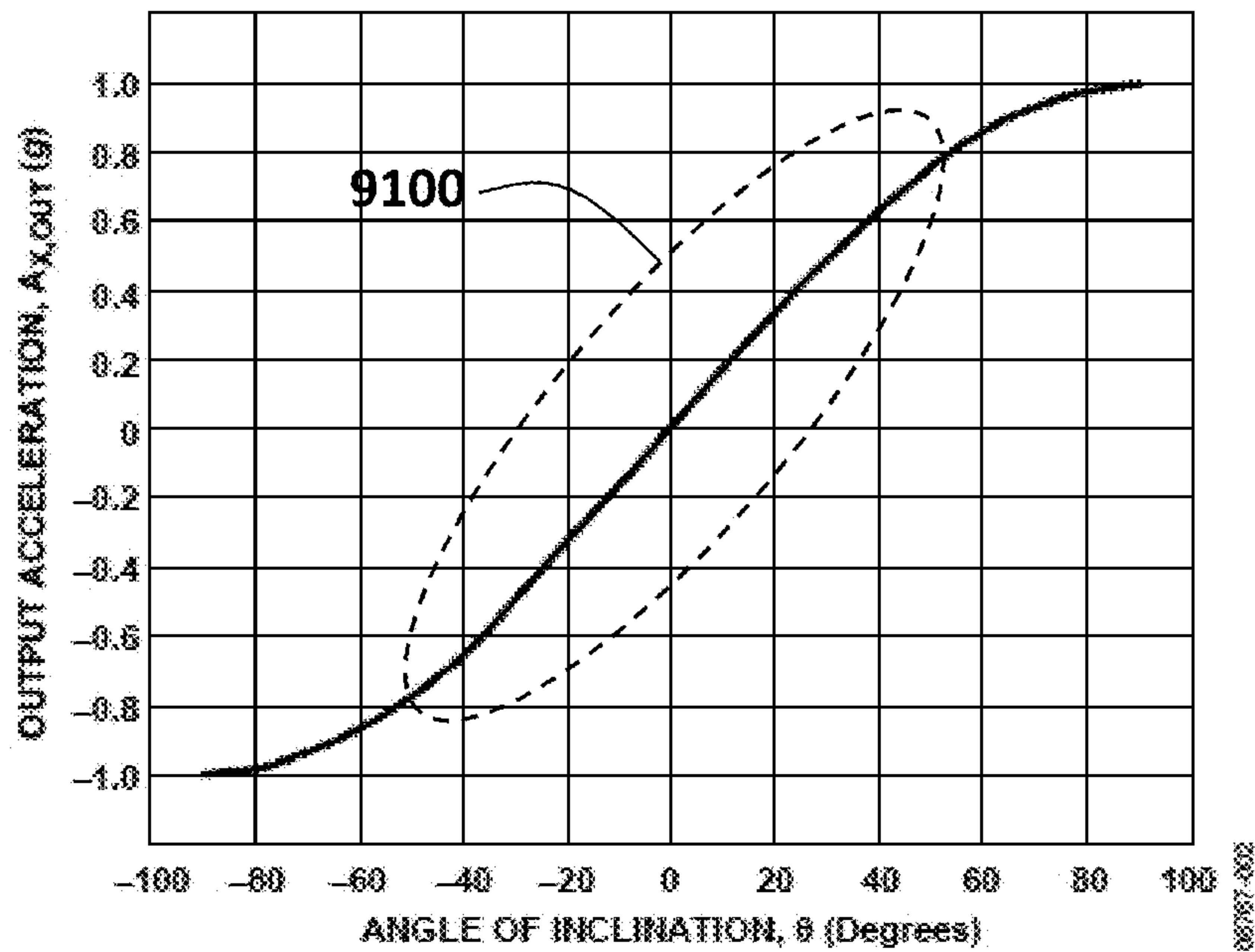
Output Acceleration vs. Angle of Inclination for Single-Axis Inclination Sensing
