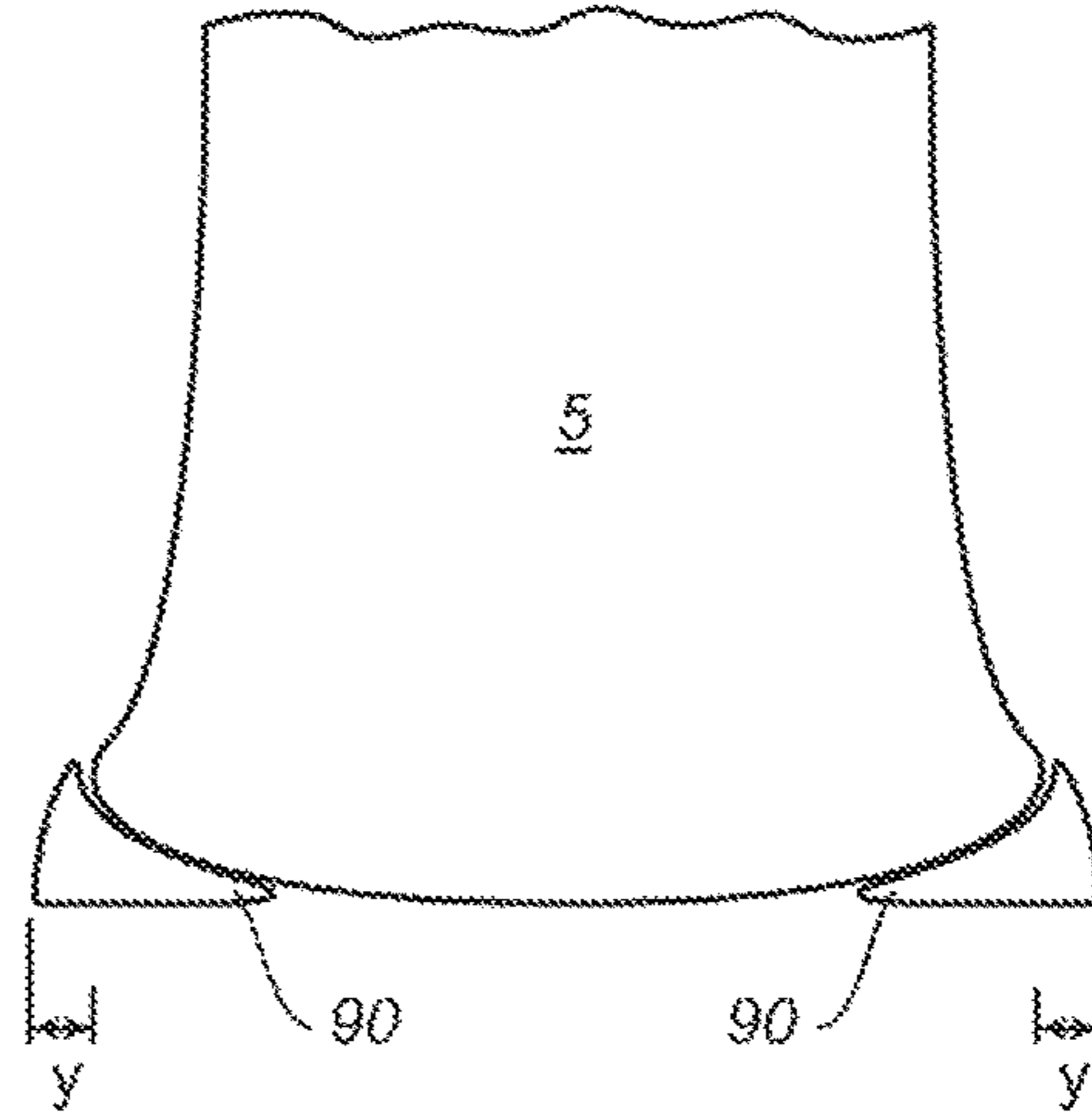
FIG. 11 (PRIOR ART)
