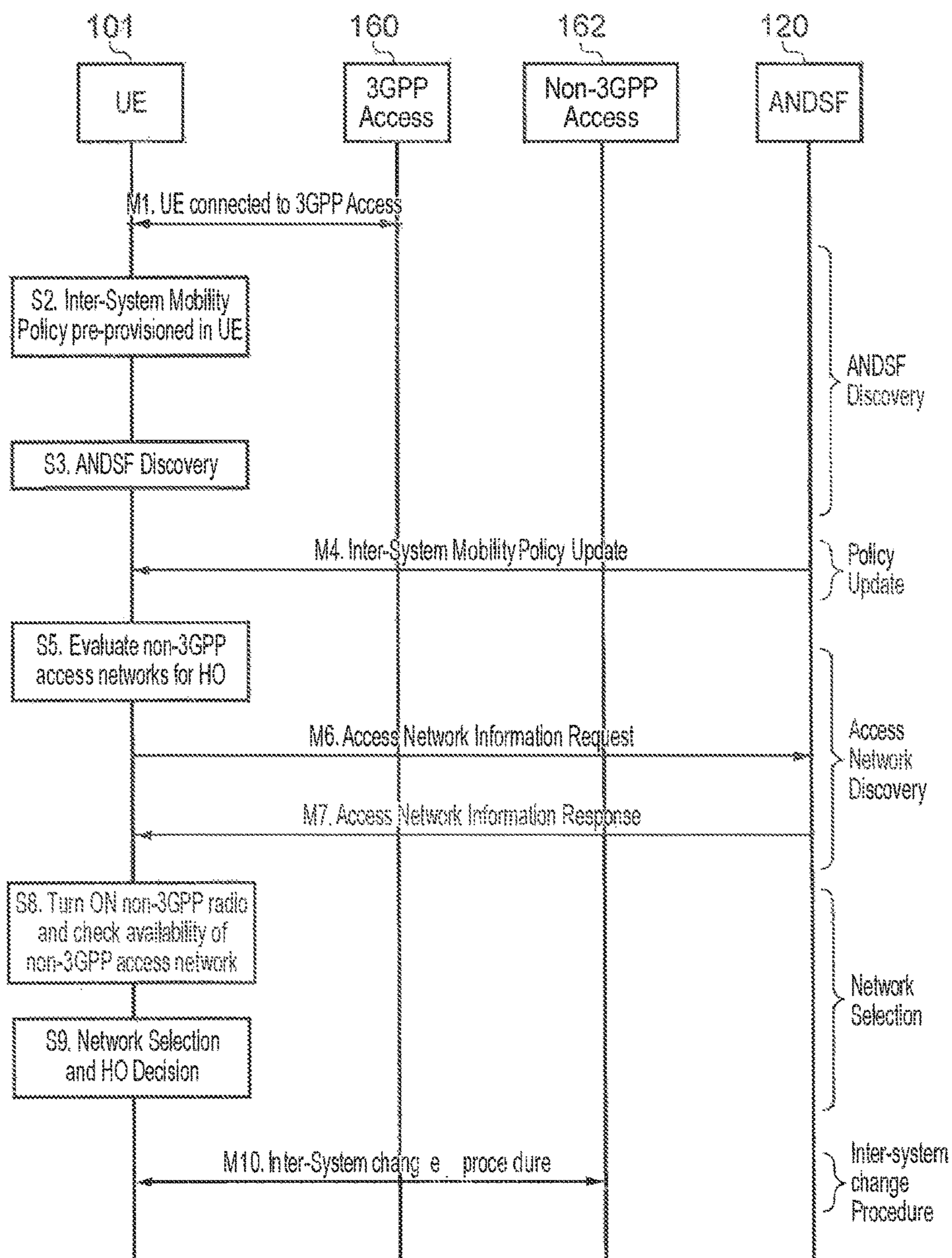
Procedure for Inter-system change between 3GPP access and non-3GPP using ANDSF
