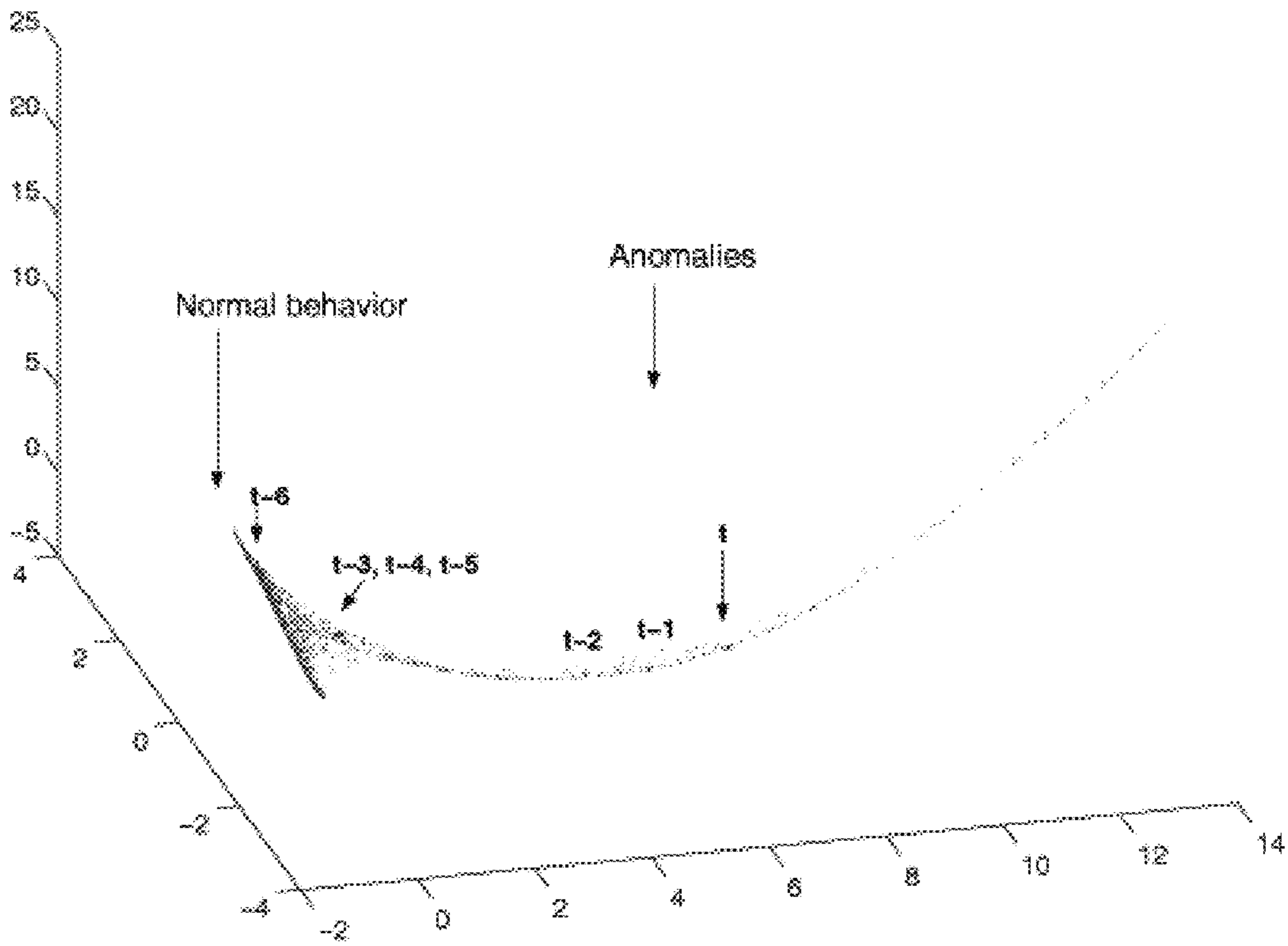
Embedding Of The Path Graph - Build Up Of An Anomaly At Time 't'
