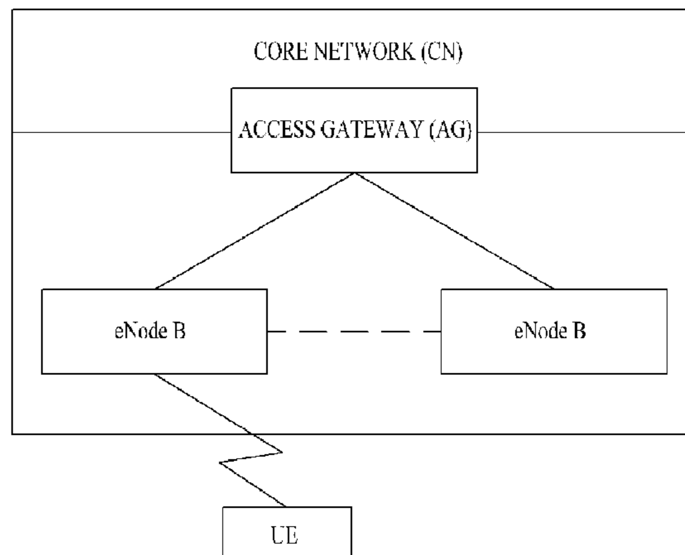
E-UMTS
