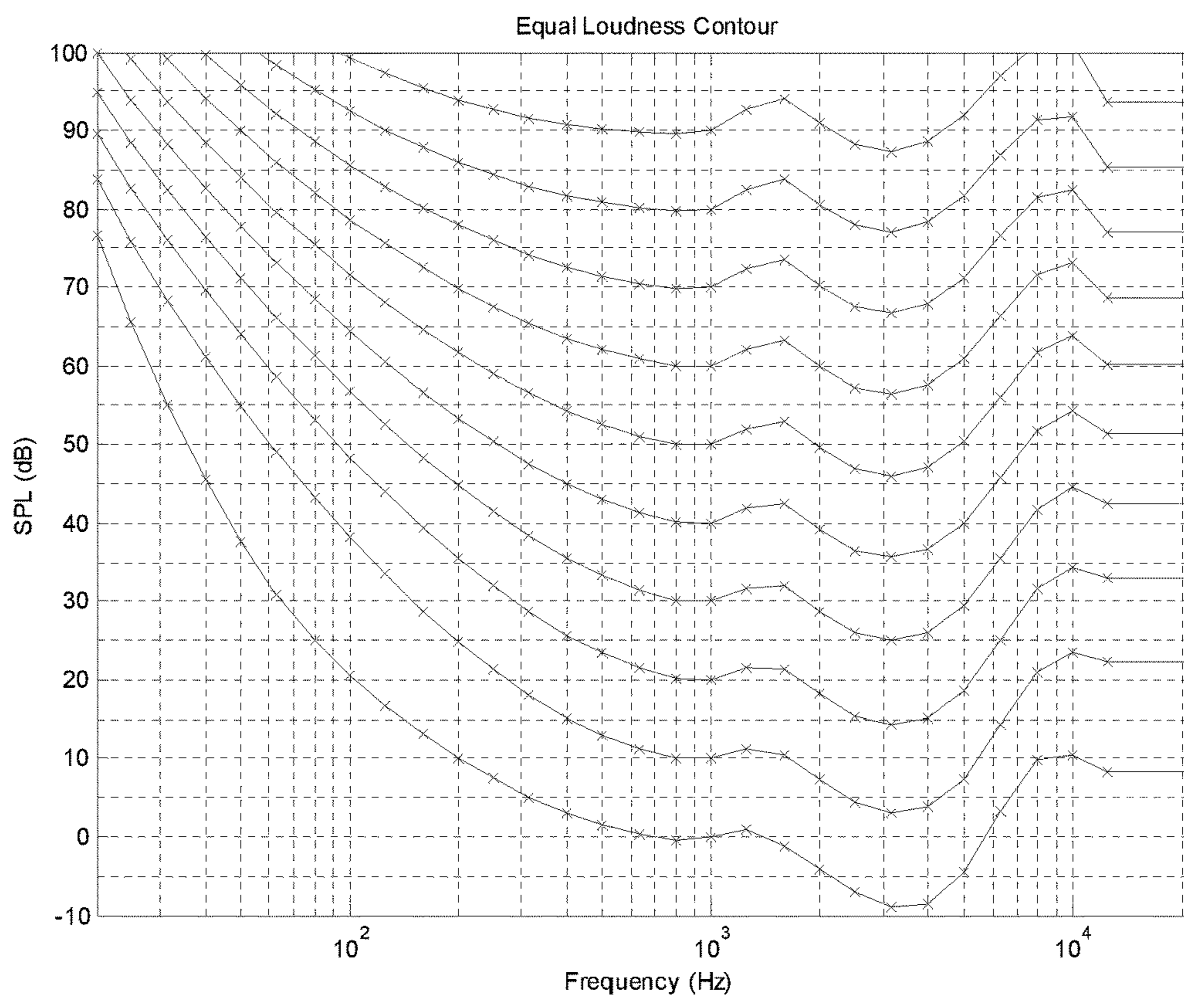
FIG. 2 (Prior Art)
