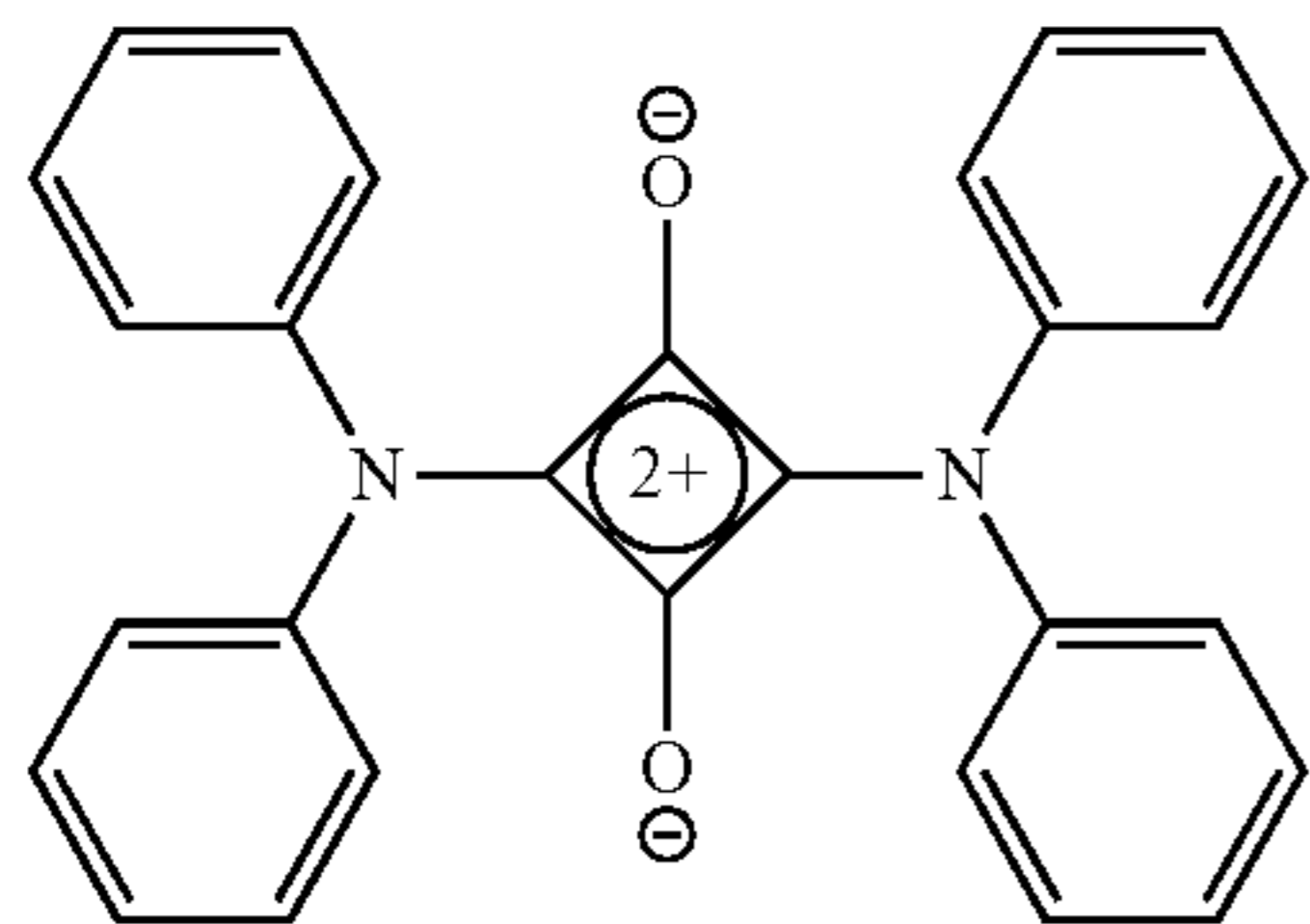
diphenylamino-squarate (YSQ)
