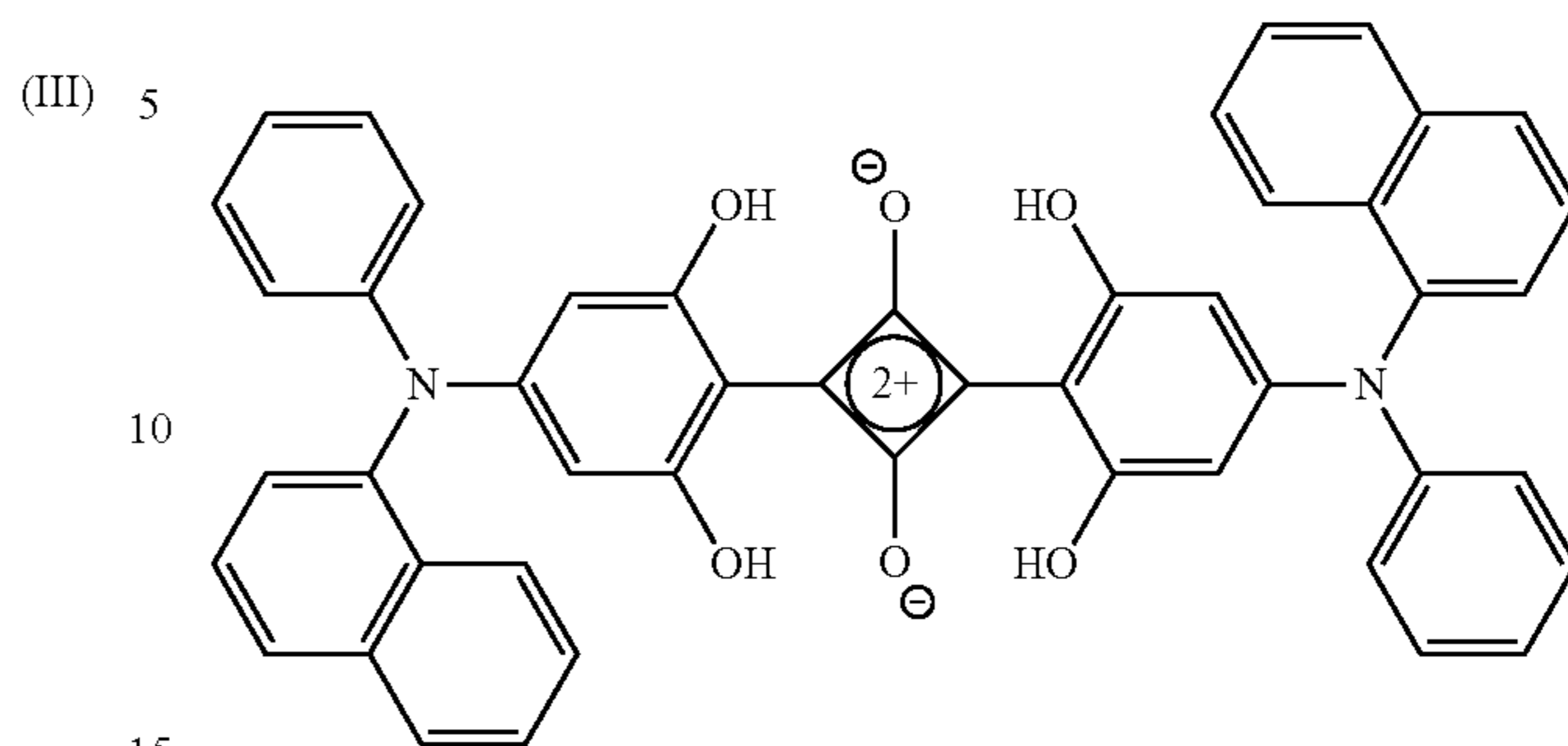
2,4-bis[4-(N-Phenyl-1-naphthylamino)-2,6-dihydroxyphenyl]squaraine (1NPSQ)
