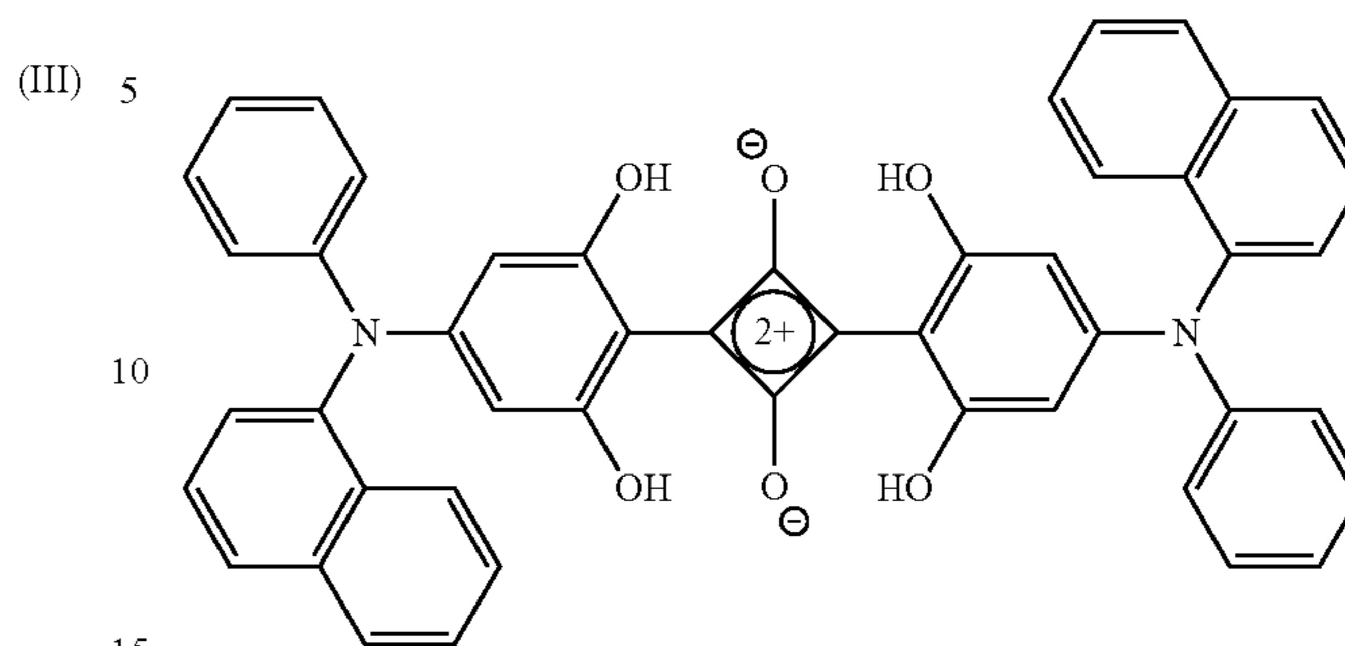
2,4-bis[4-(N-Phenyl-1-naphthylamino)-2,6-dihydroxyphenyl]squaraine (1NPSQ)
