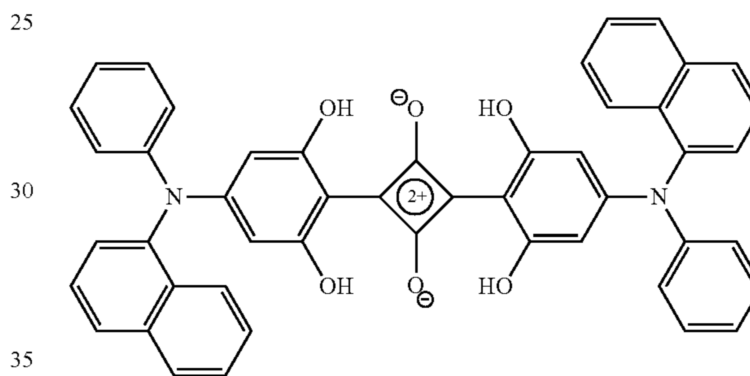
1NPSQ
