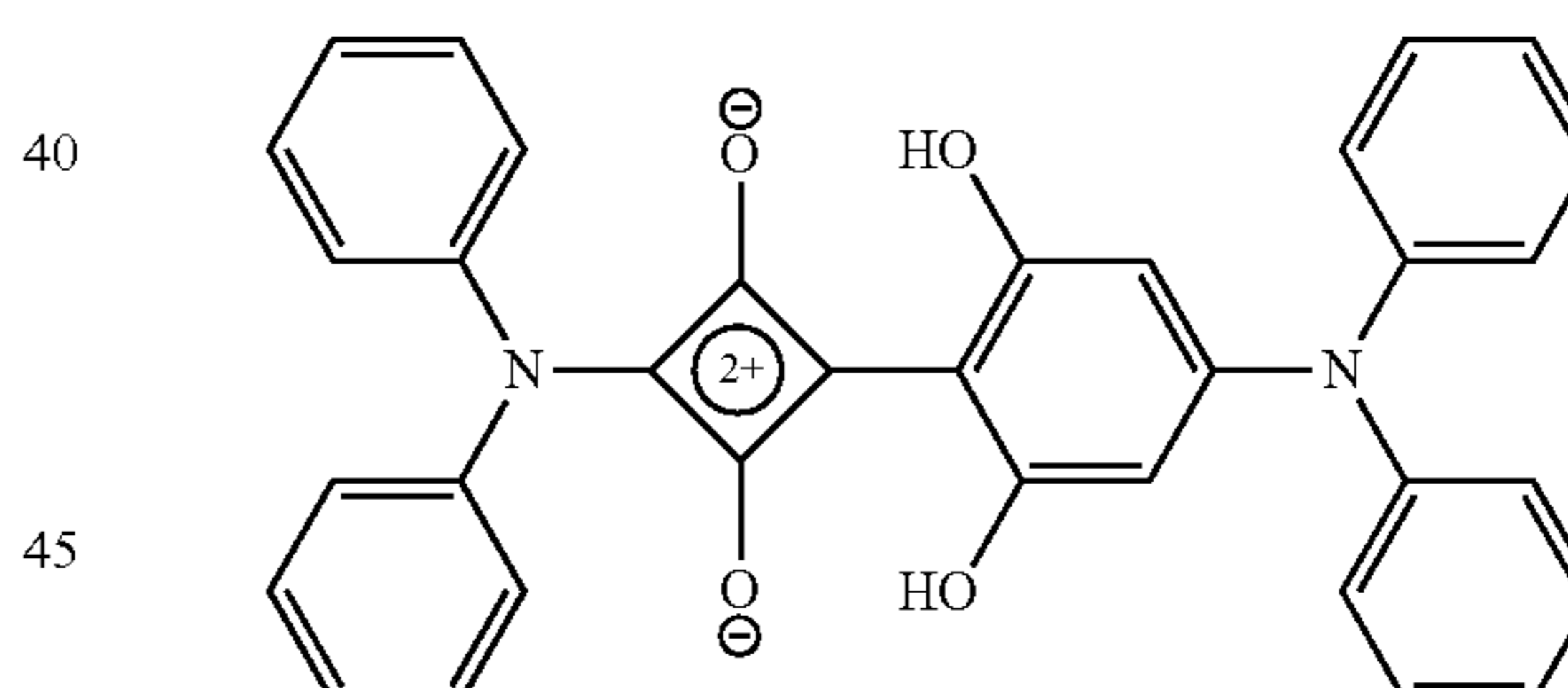
DPUSQ
