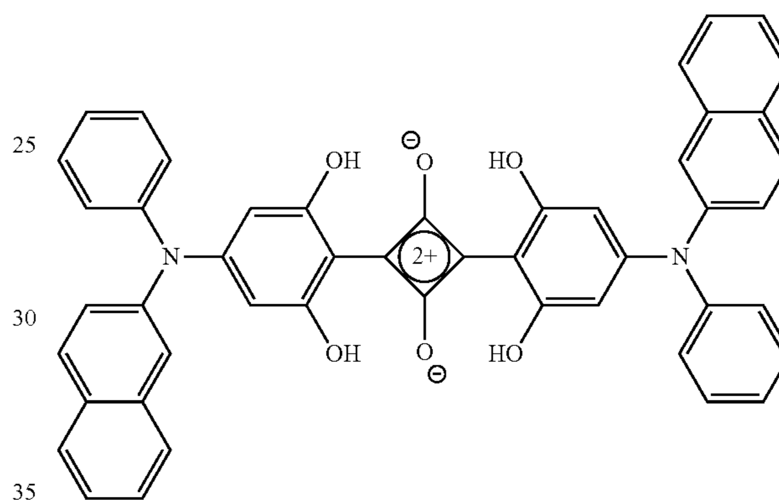
2,4-bis[4-(N-Phenyl-2-naphthylamino)-2,6-dihydroxyphenyl]squaraine (2NPSQ)
