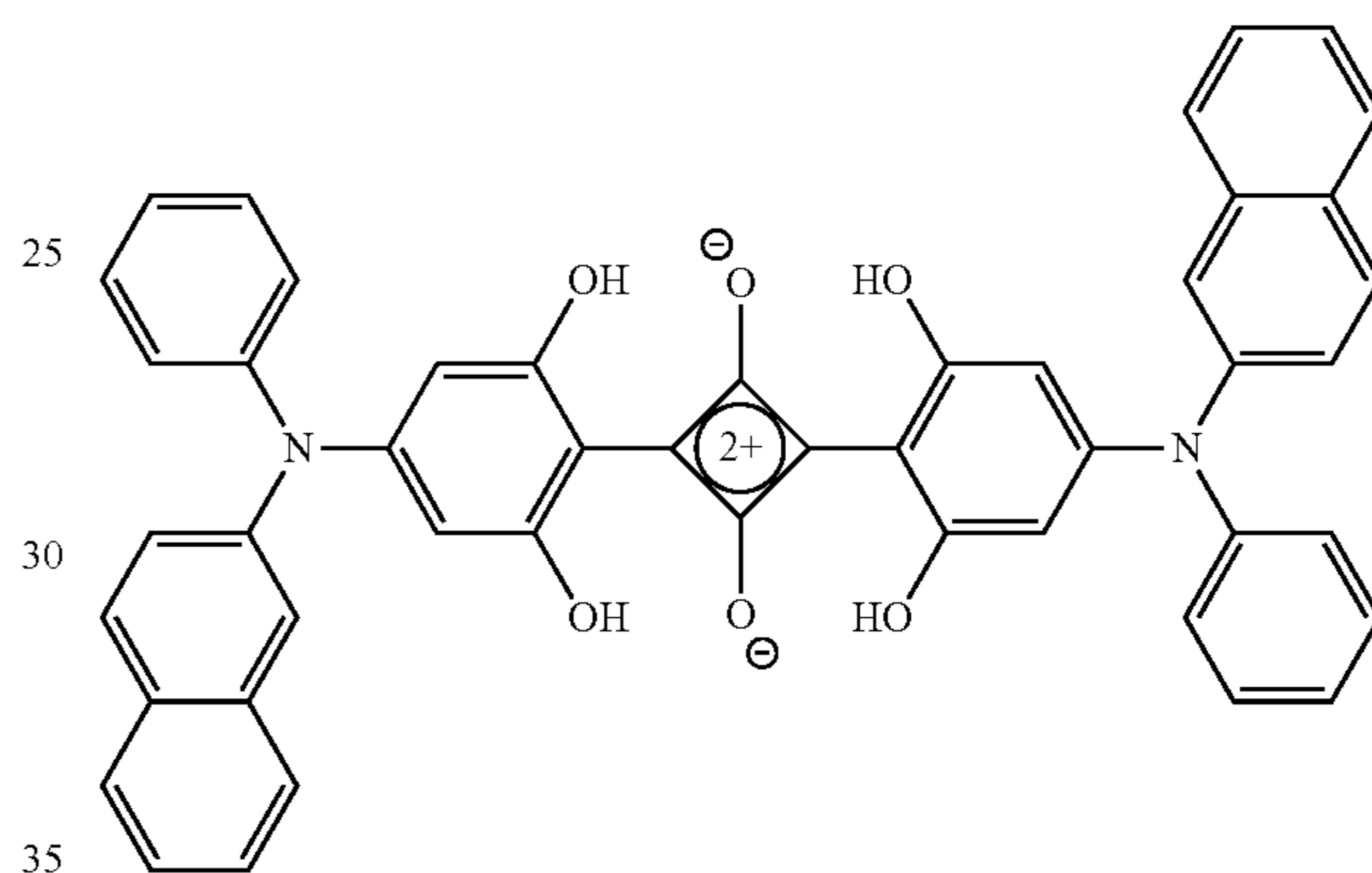
2,4-bis[4-(N-Phenyl-2-naphthylamino)-2,6-dihydroxyphenyl]squaraine (2NPSQ)
