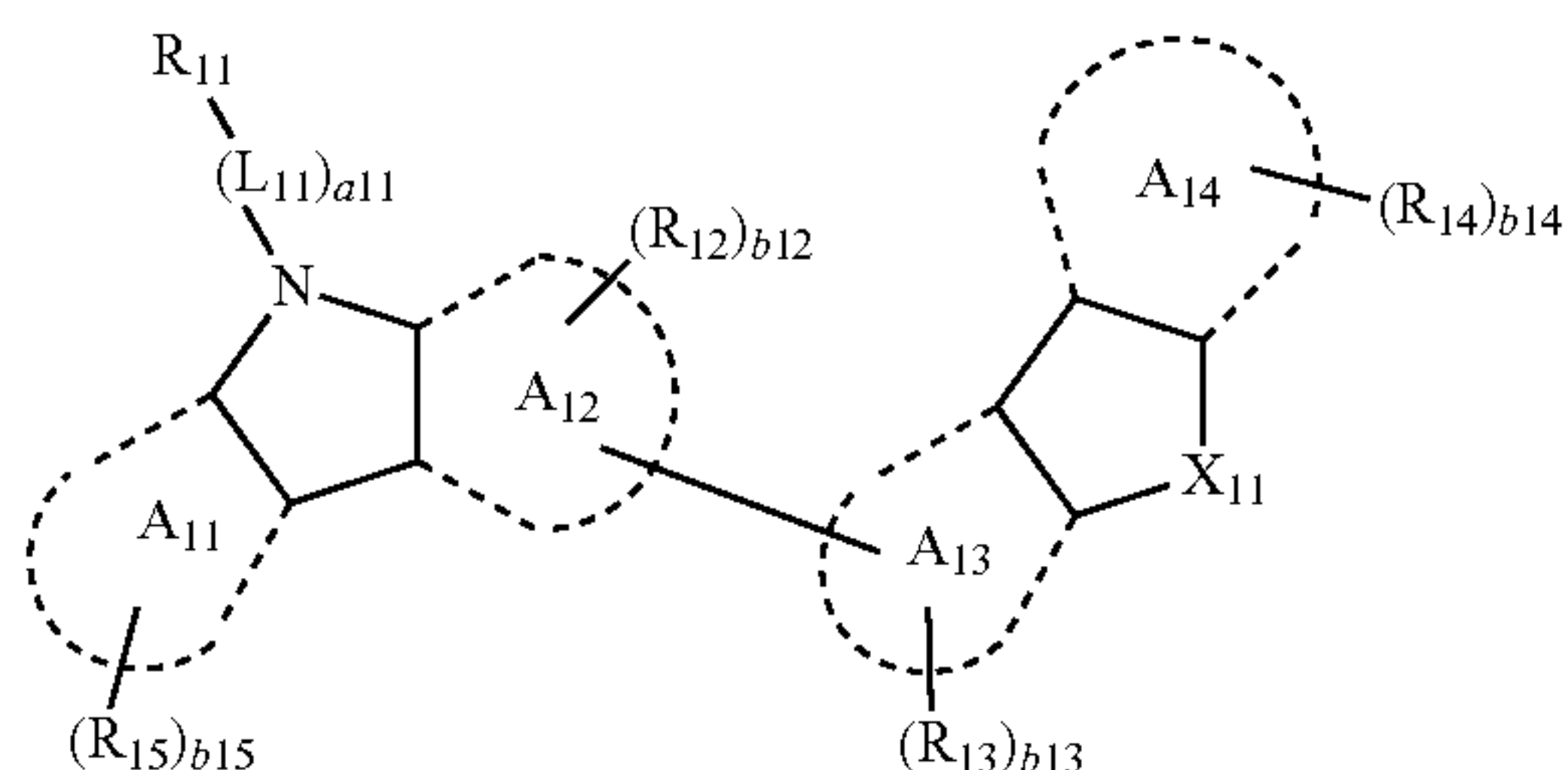
Formula 10A
