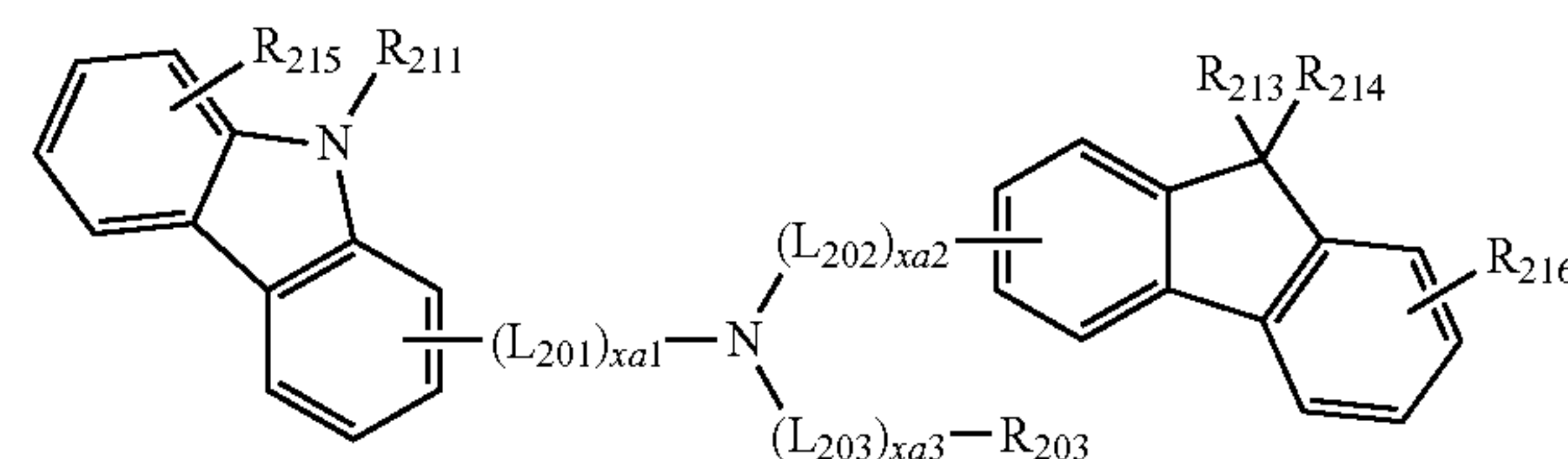
Formula 201A
