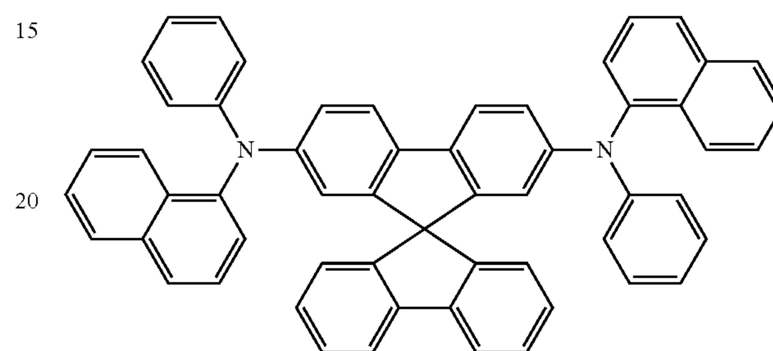
Spiro-NPB
