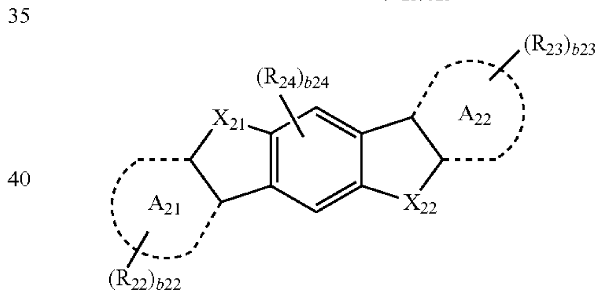
Formula 10D
