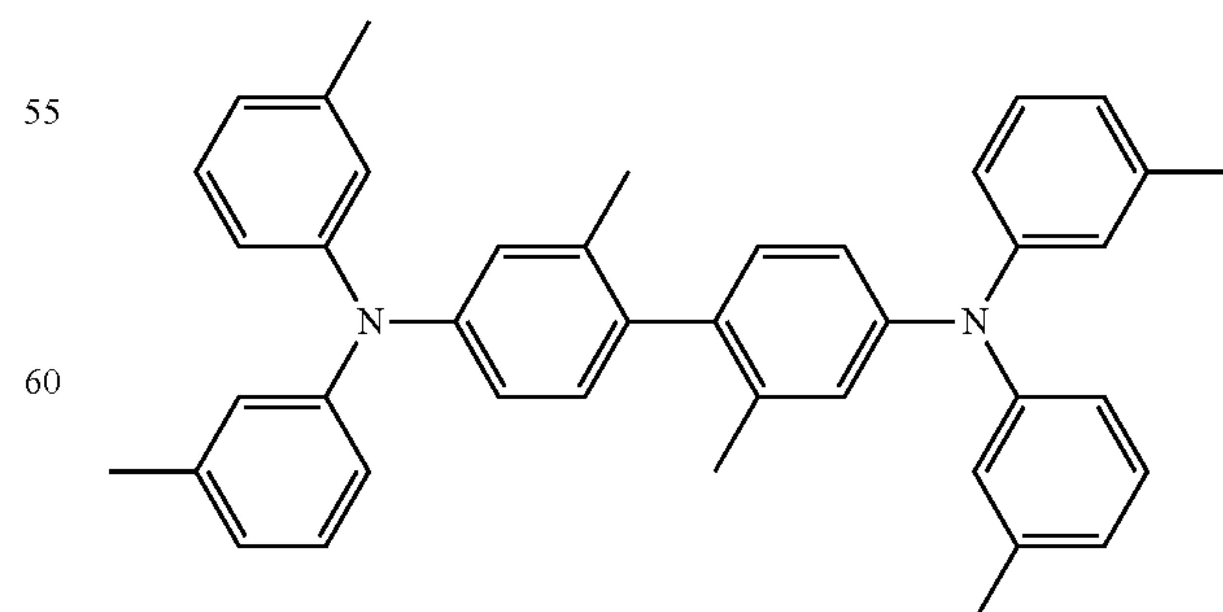
HMTDP
