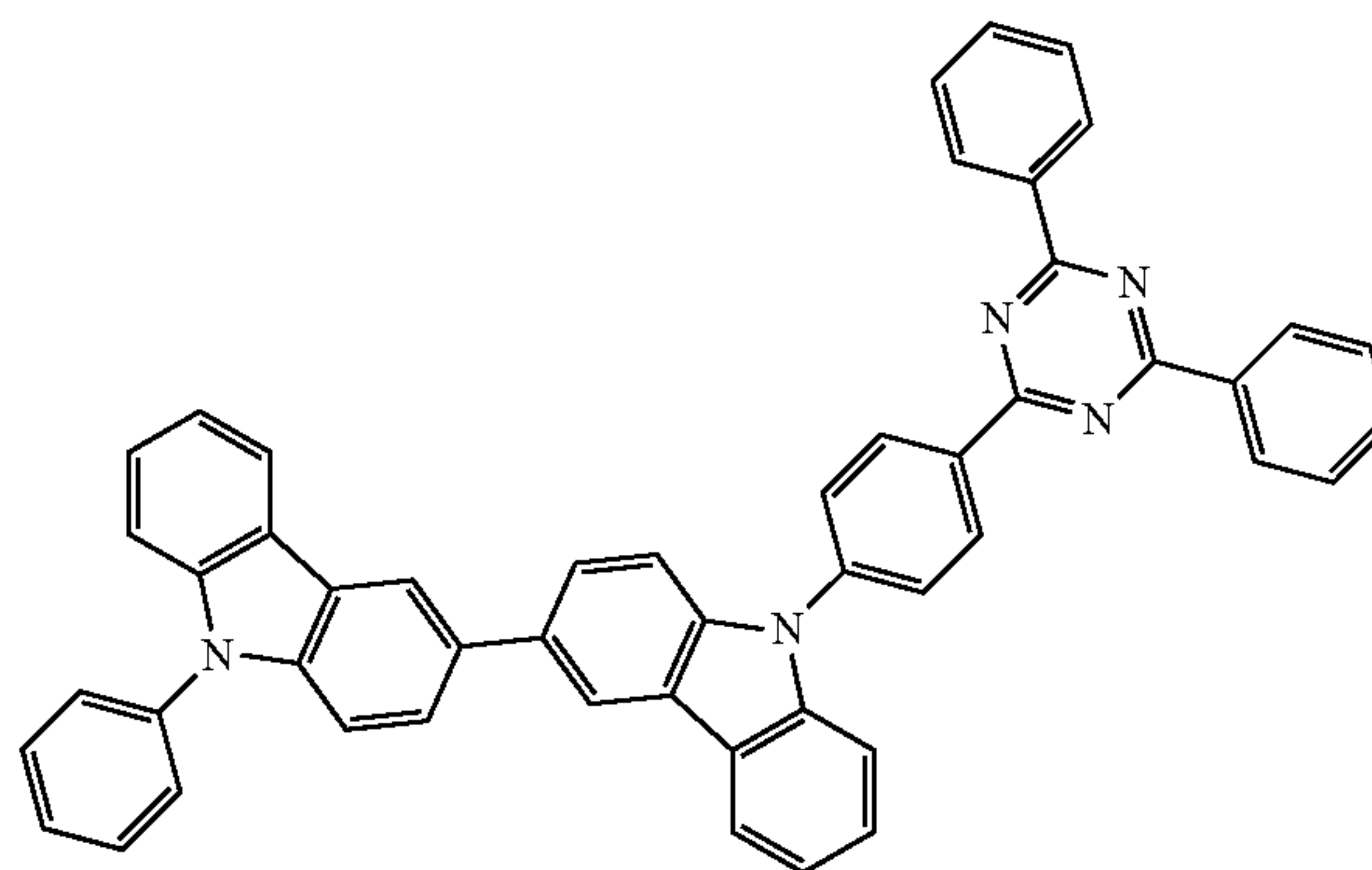
Host B
