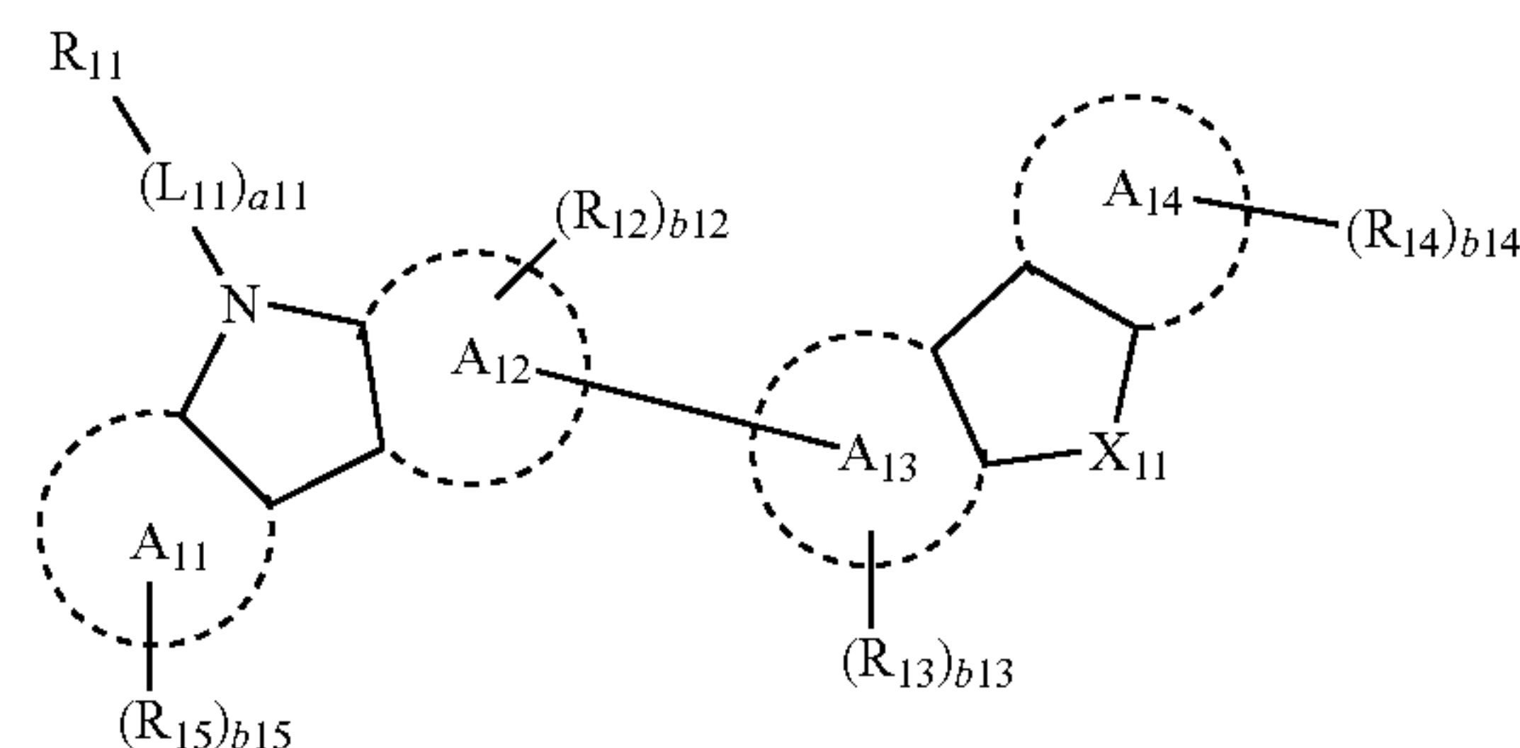
Formula 10A
