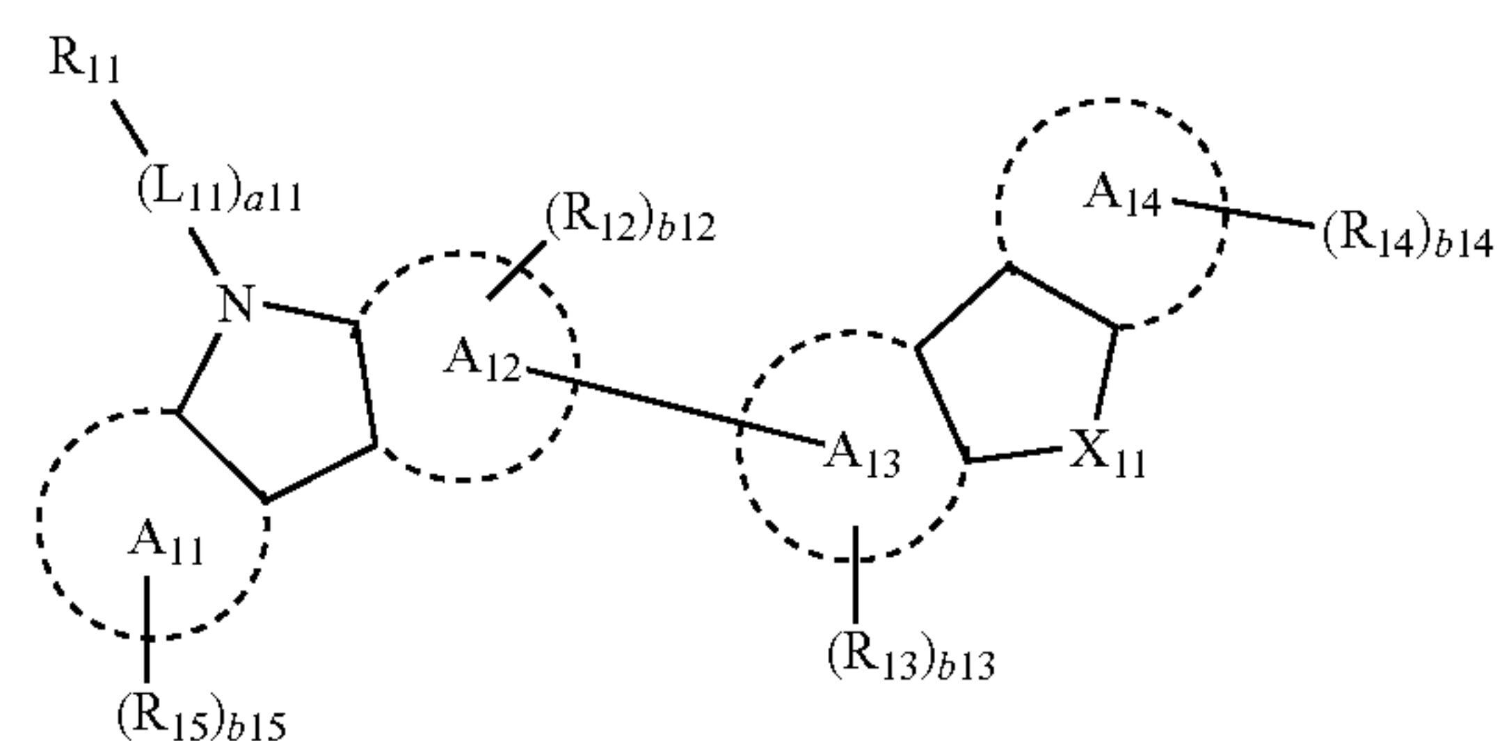
Formula 1
