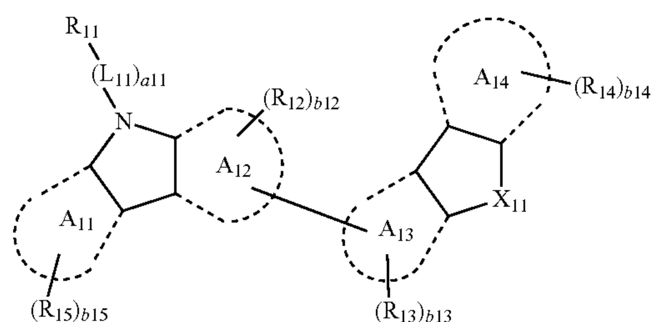
Formula 1
