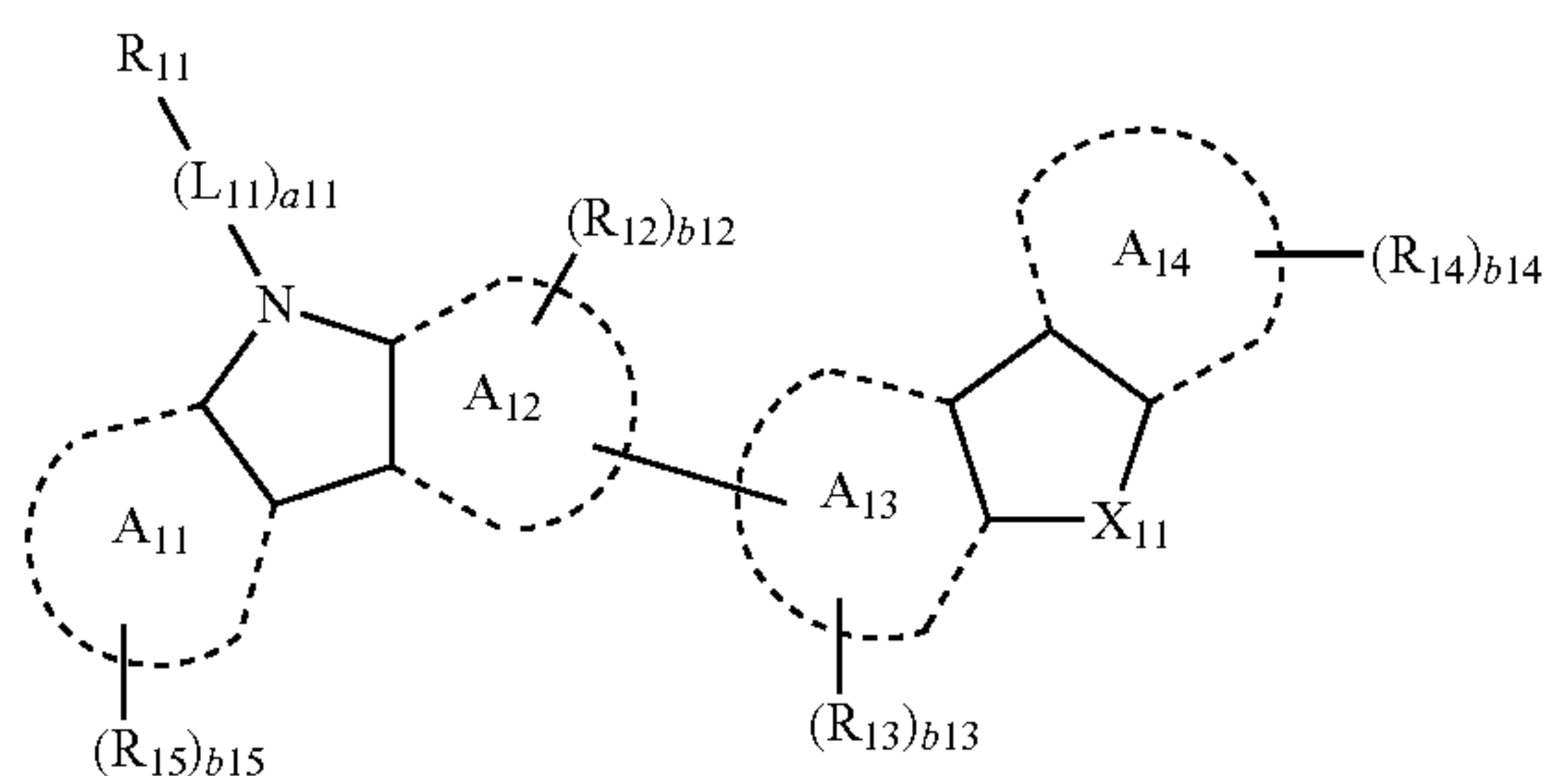
Formula 10A
