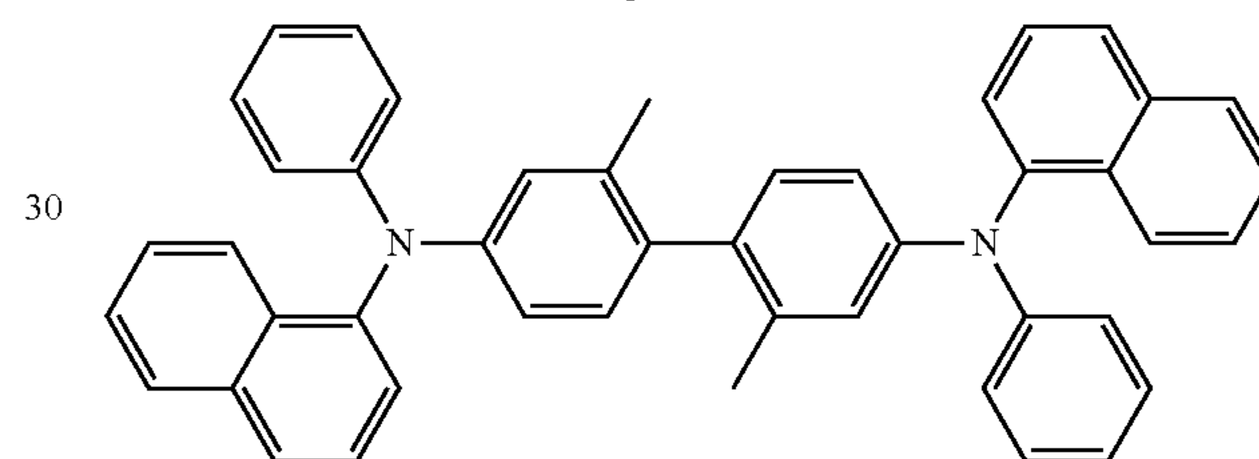
\alpha -NPB
