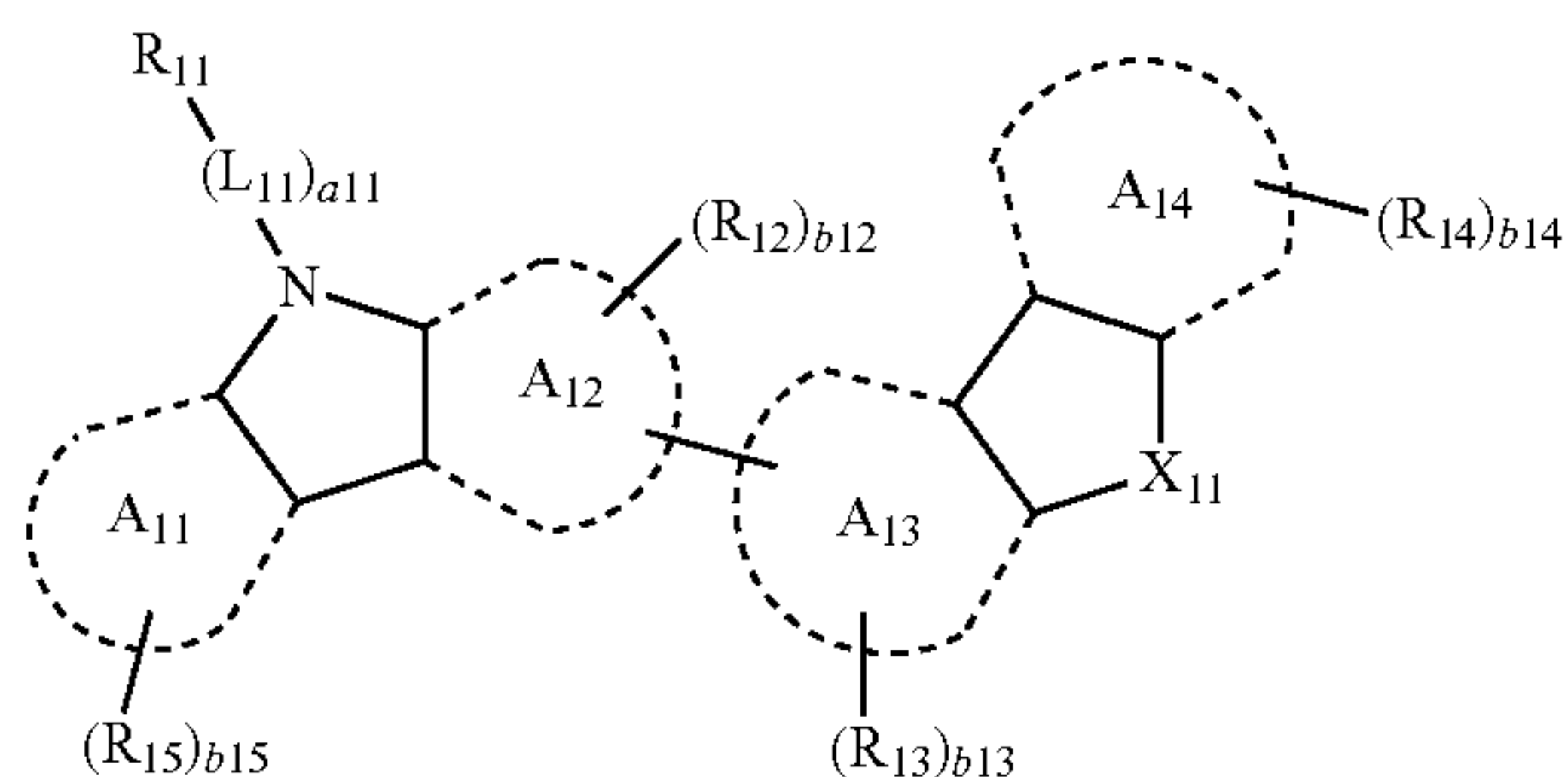
Formula 1
