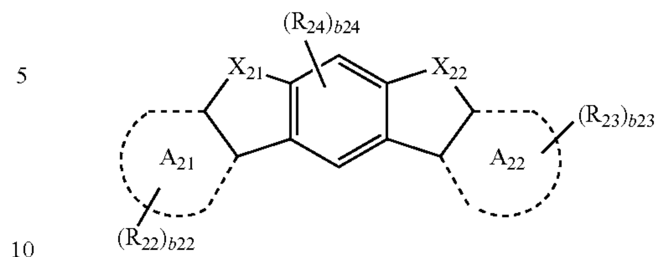
Formula 1
