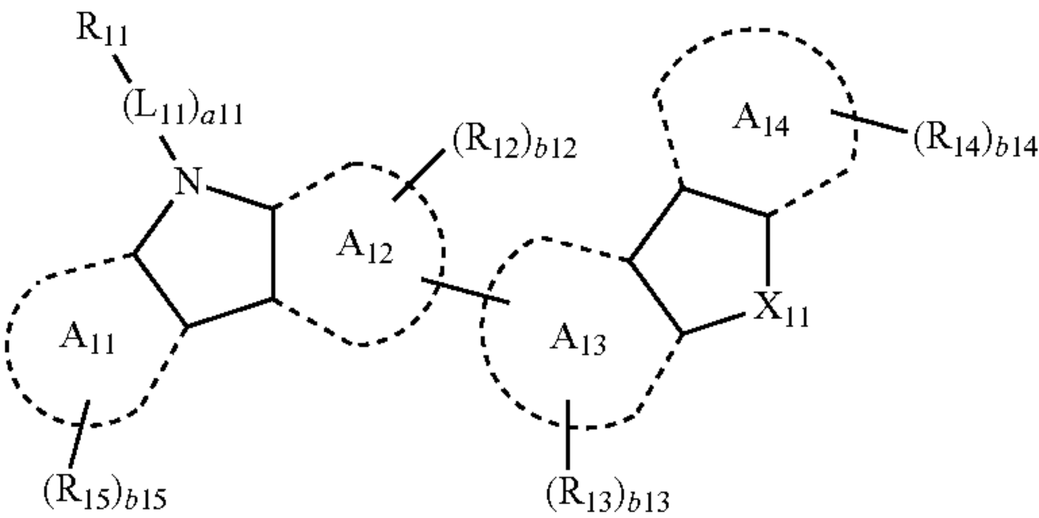
Formula 1
