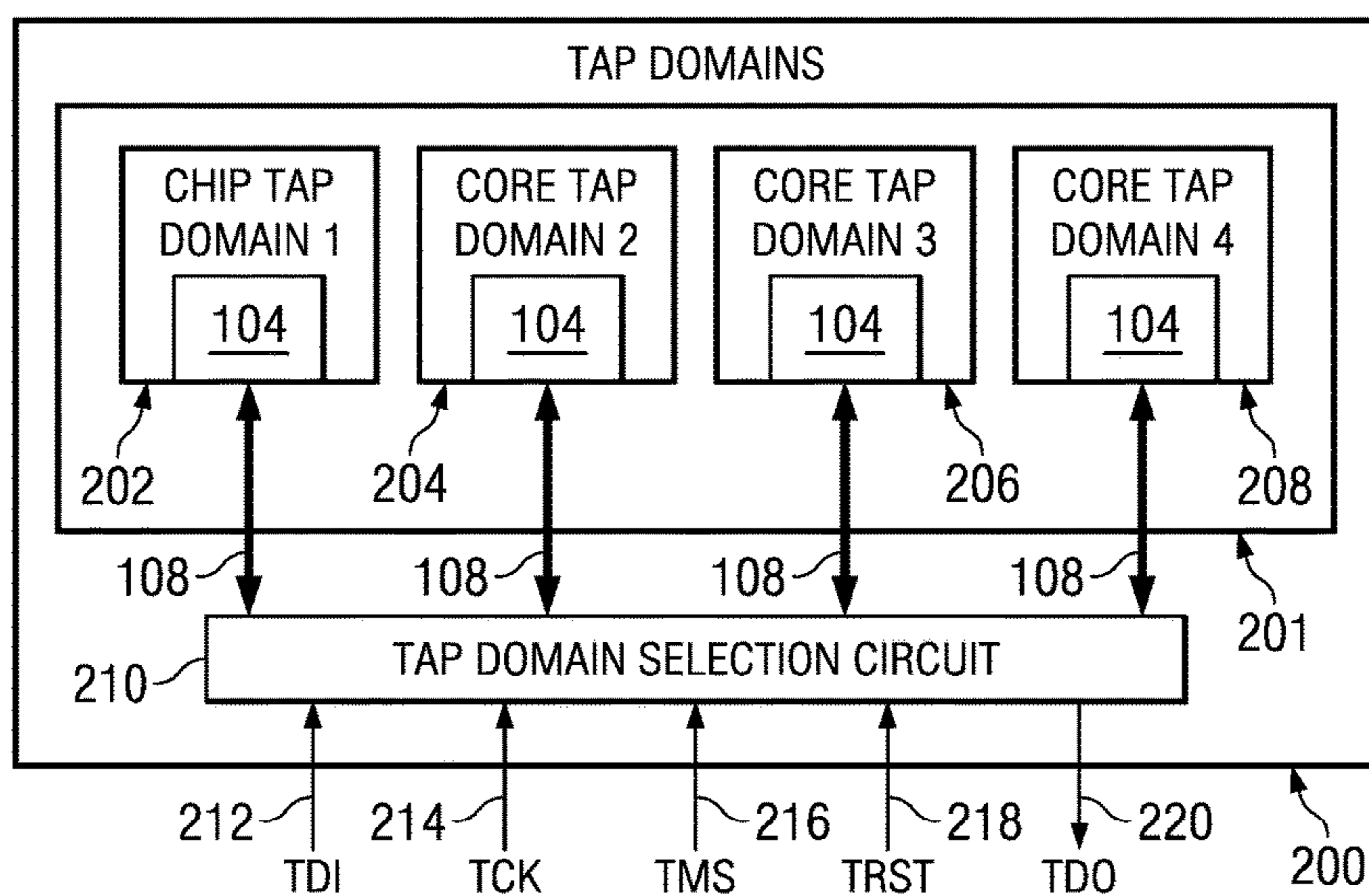
FIG. 2 (PRIOR ART)
