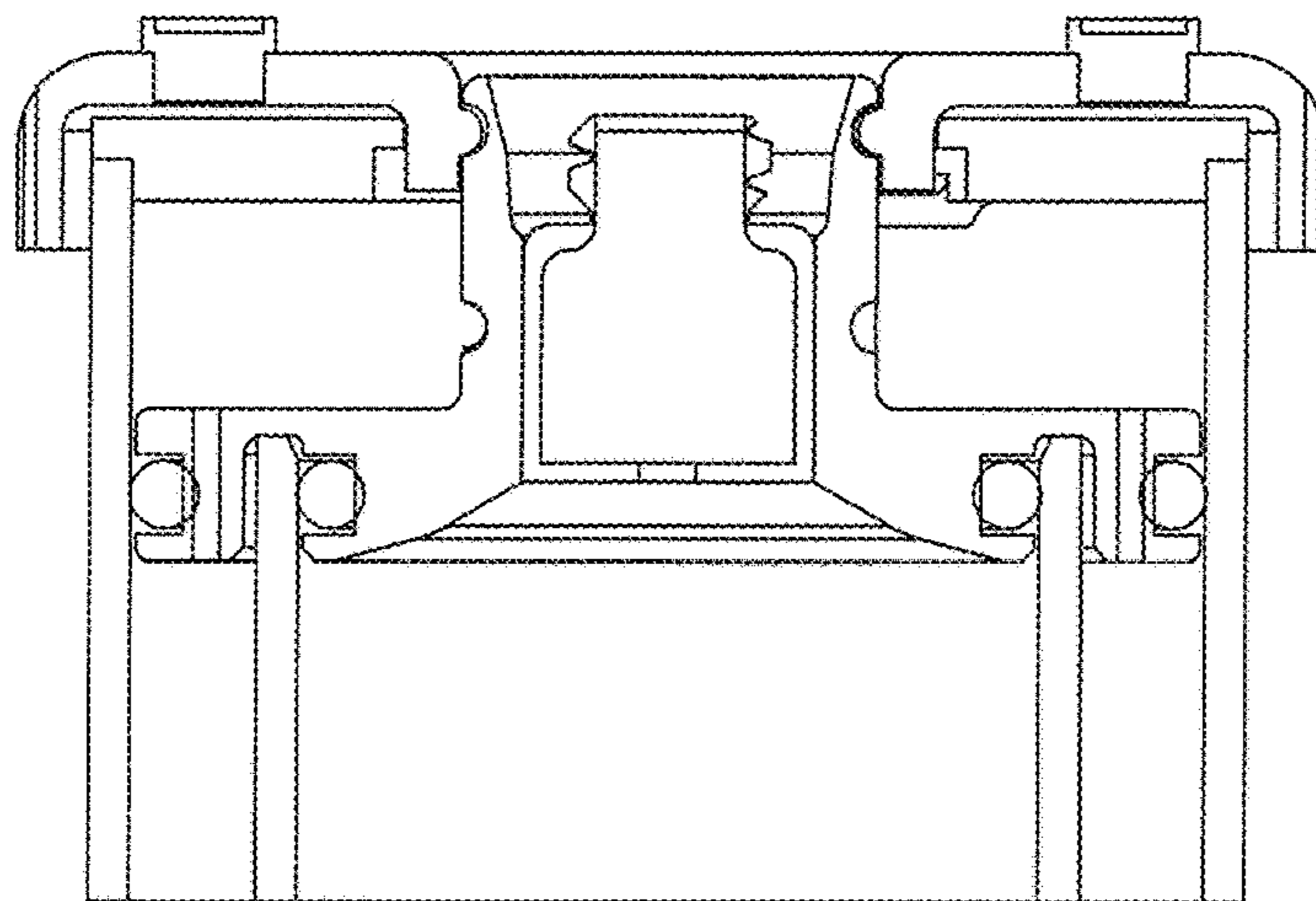
CLOSED FIG. 7A
