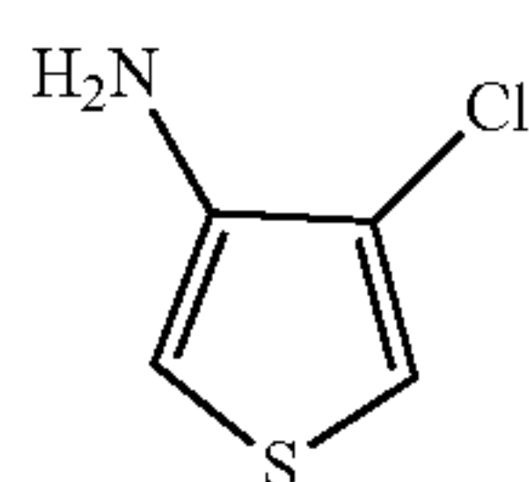
4-Chlorothiophen-3-amine
