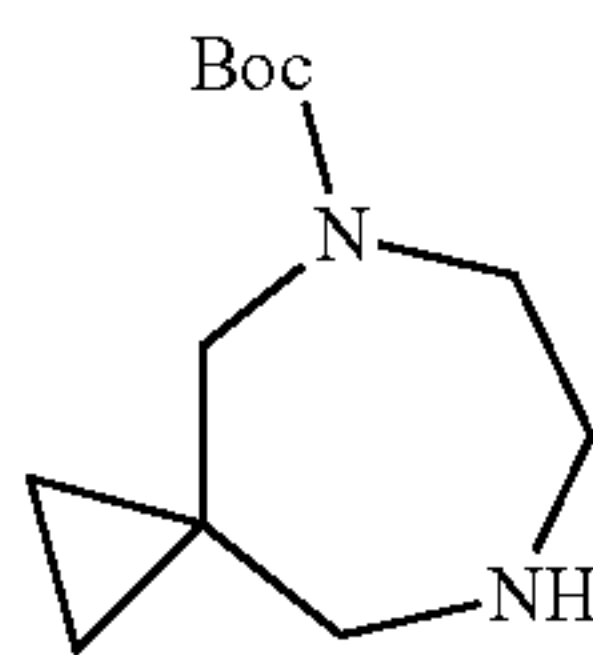
tert-Butyl 5,8-diazaspiro[2.6]nonane-5-carboxylate
