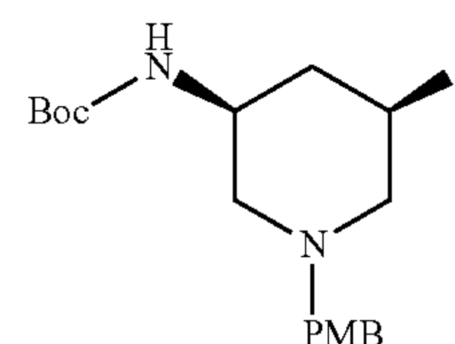
tert-Butyl ((3S,5R)-5-fluoro-1-(4-methoxybenzyl)piperidin-3-yl)carbamate
