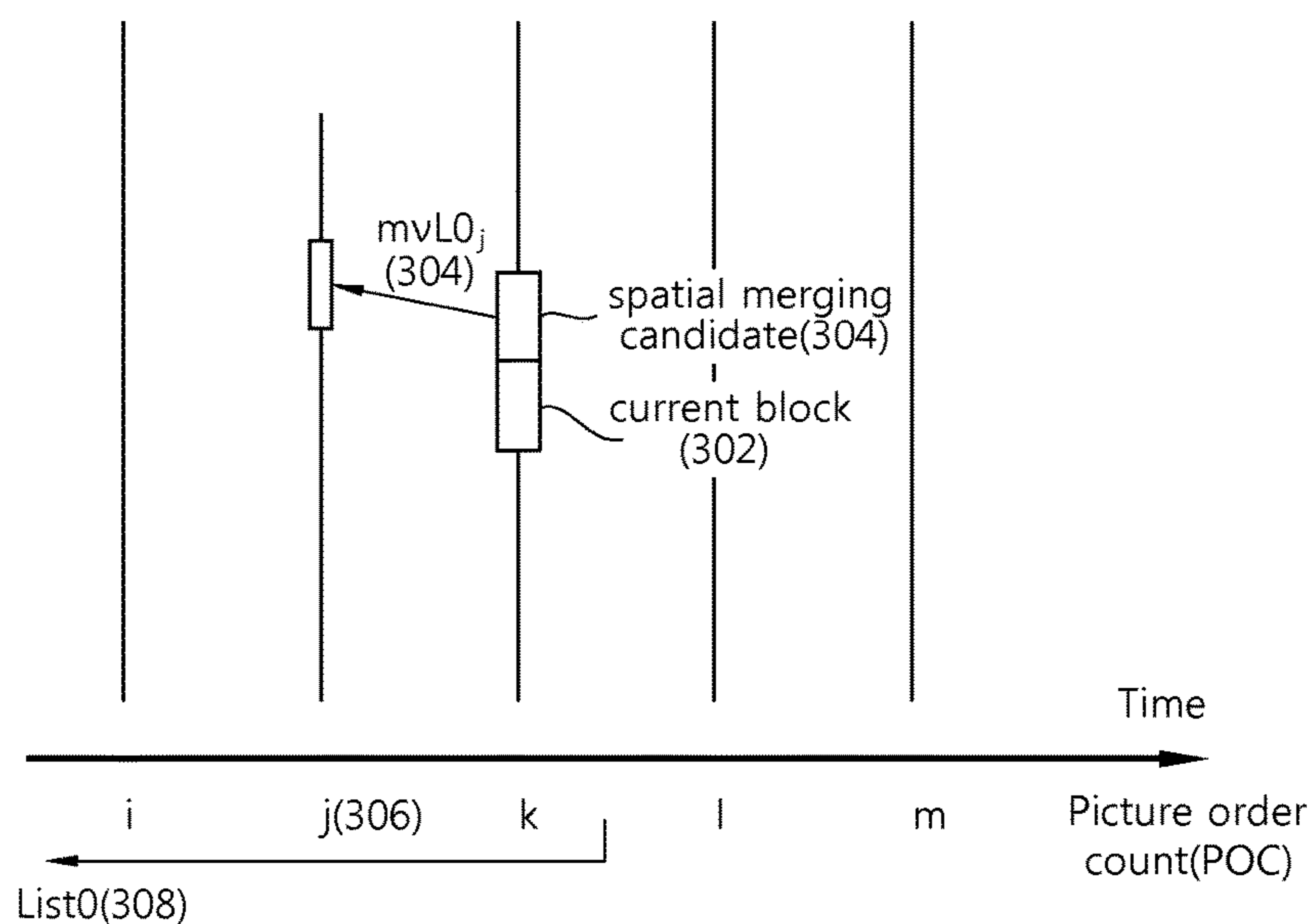
(A)
