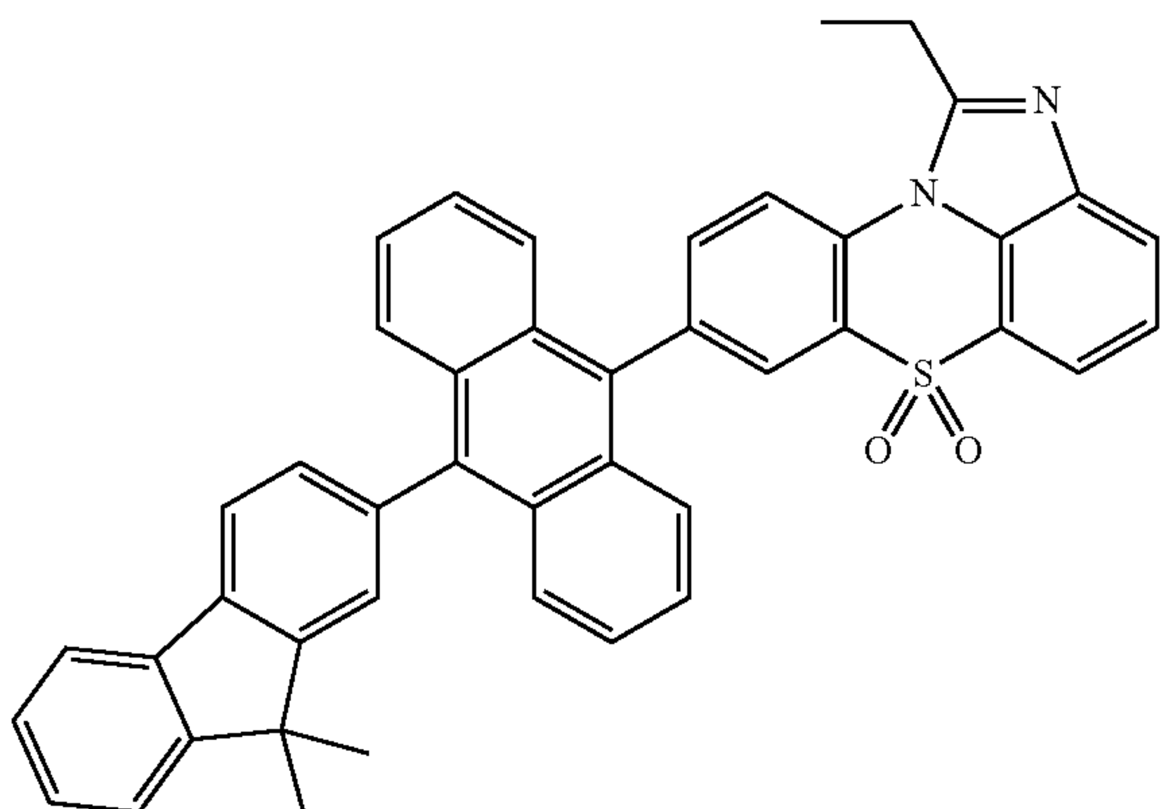
[Chemical Formula 1-3-5]
