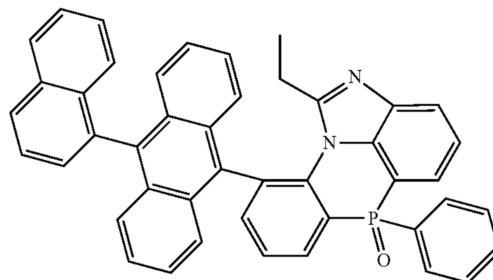
[Chemical Formula 2-8-3]
