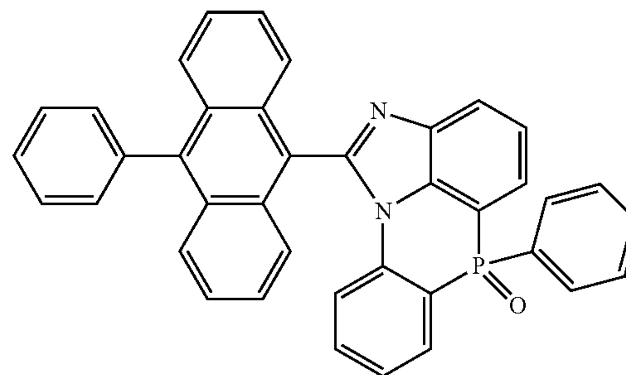
[Chemical Formula 2-5-1]
