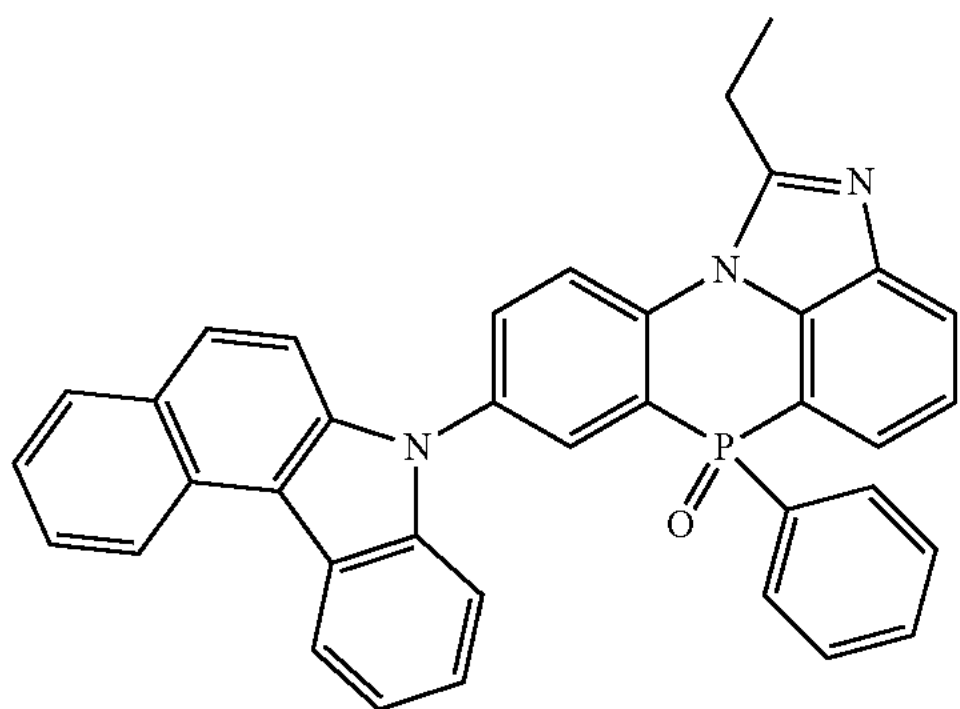
[Chemical Formula 2-3-51]
