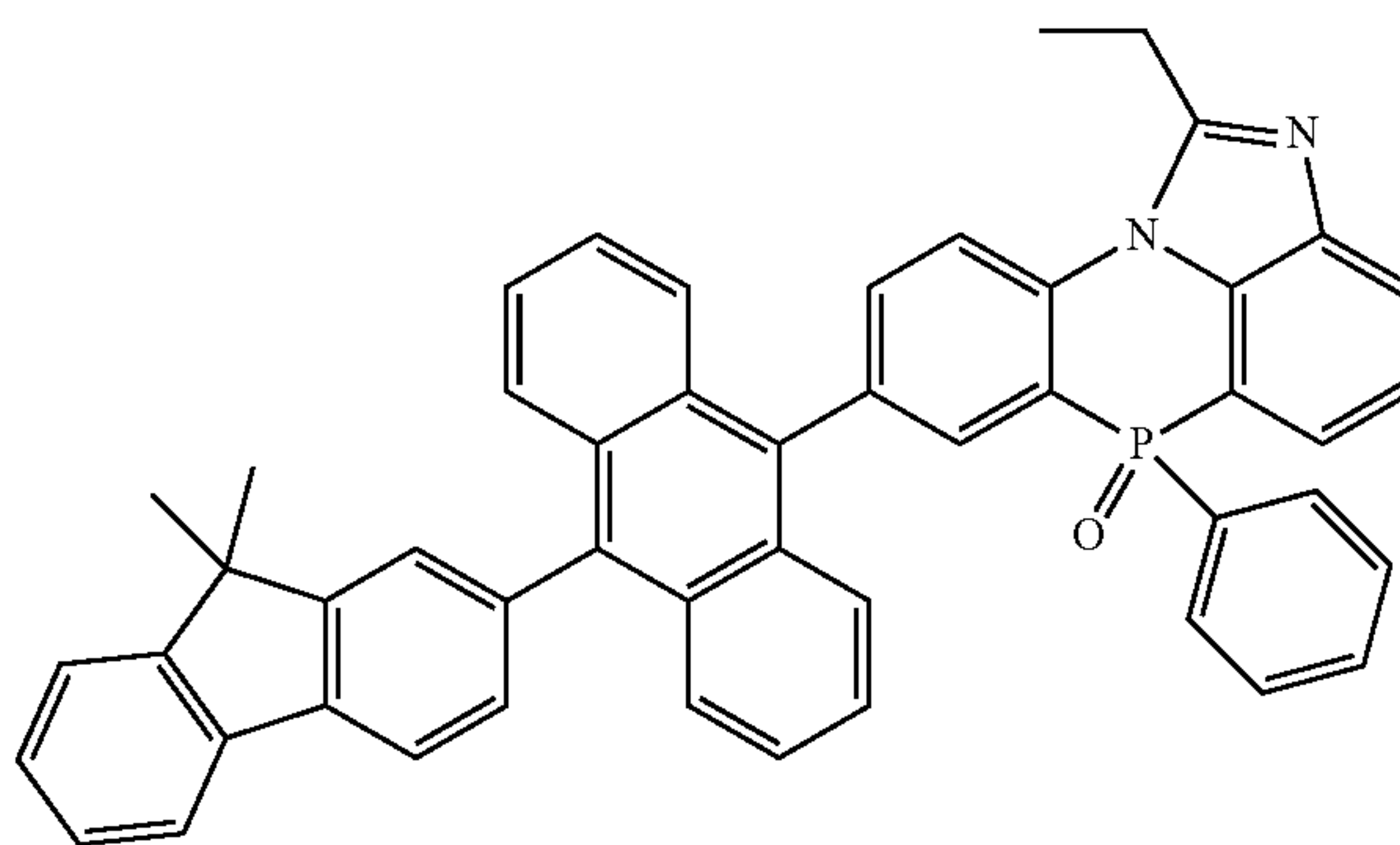
[Chemical Formula 2-3-6]
