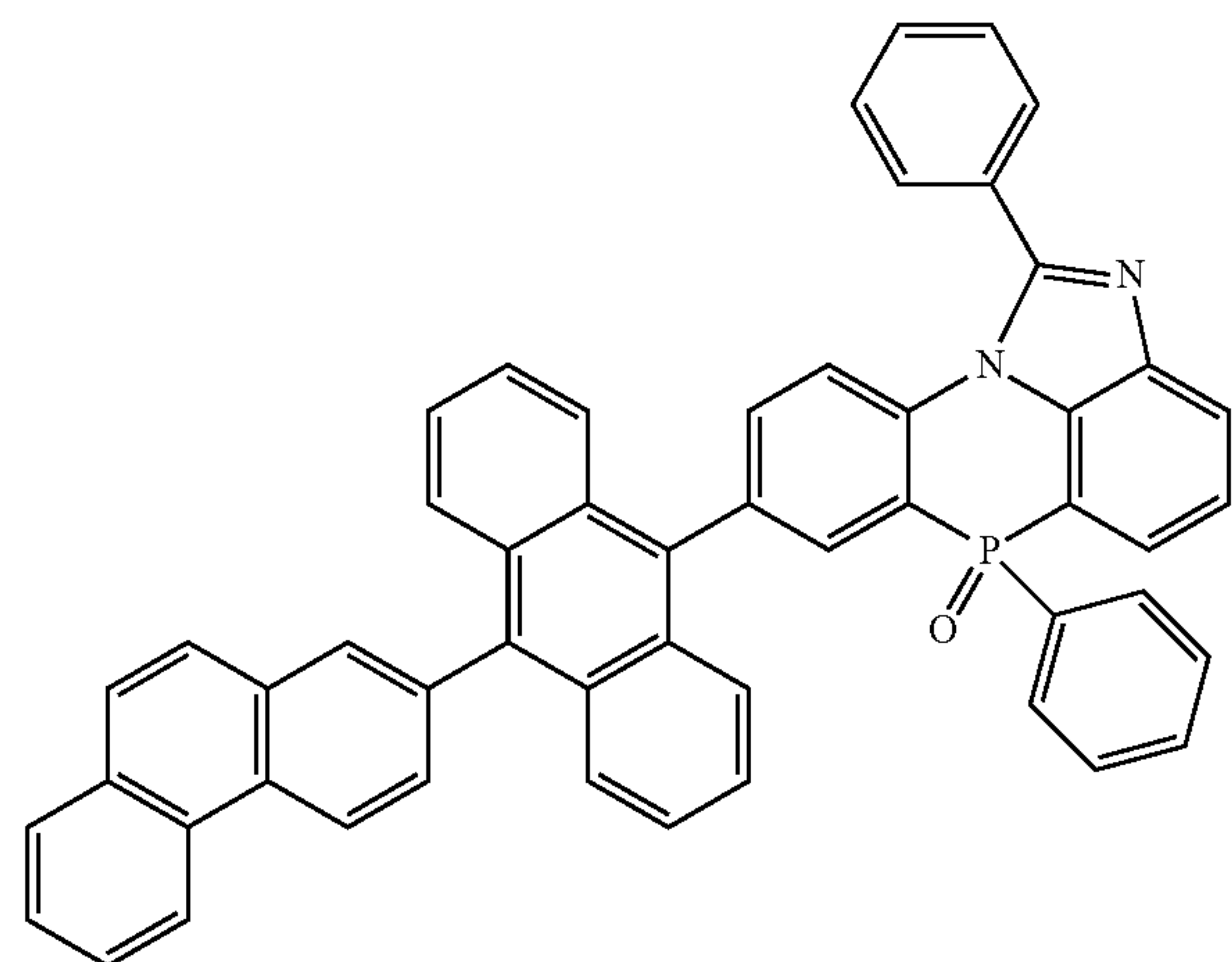
[Chemical Formula 2-4-9]
