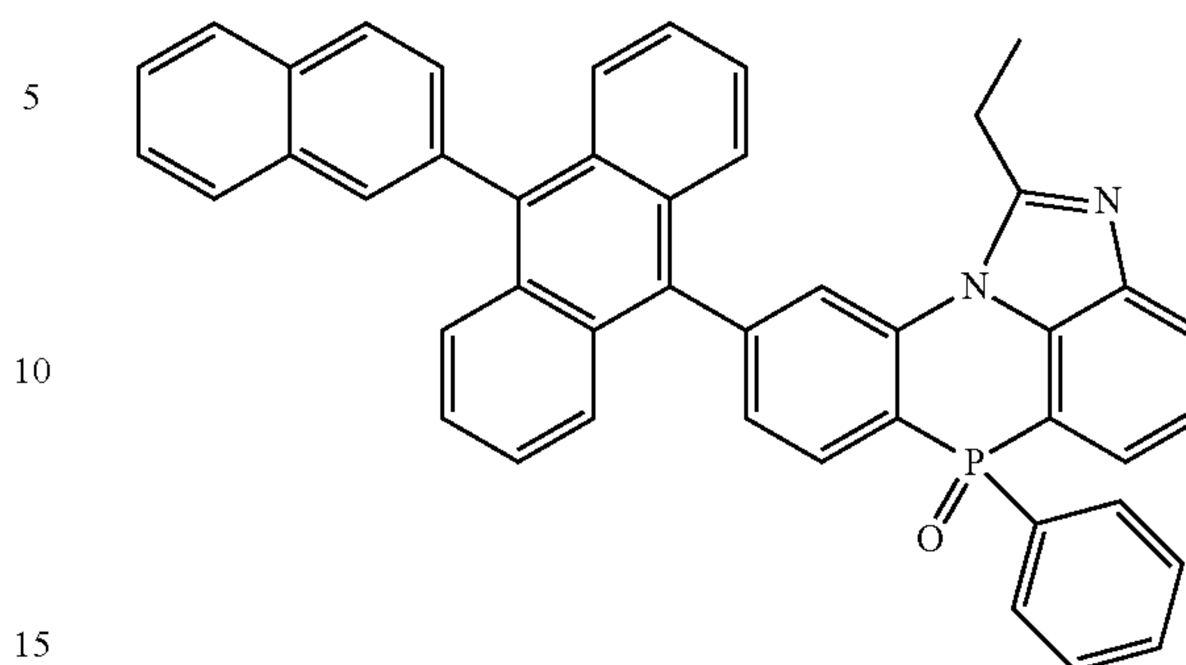
[Chemical Formula 2-7-3]
