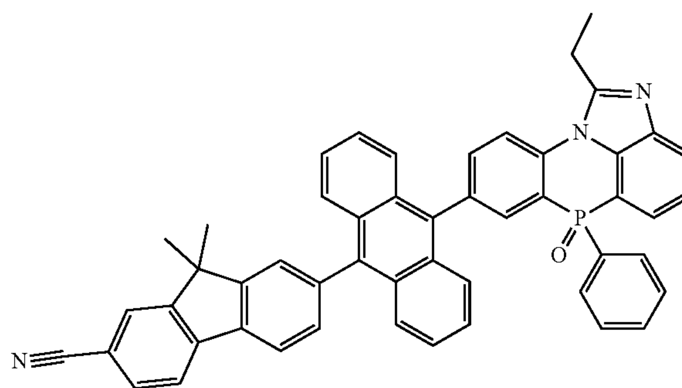
[Chemical Formula 2-3-15]
