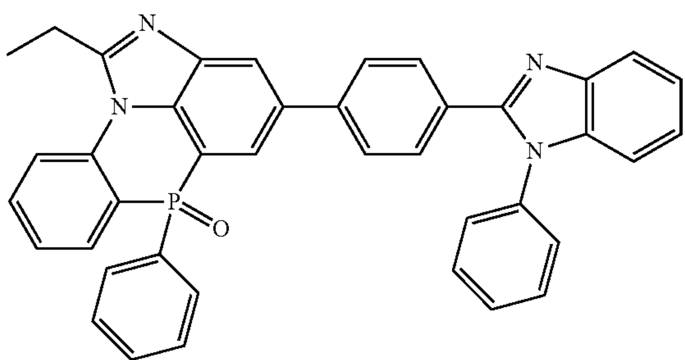
[Chemical Formula 2-10-9]
