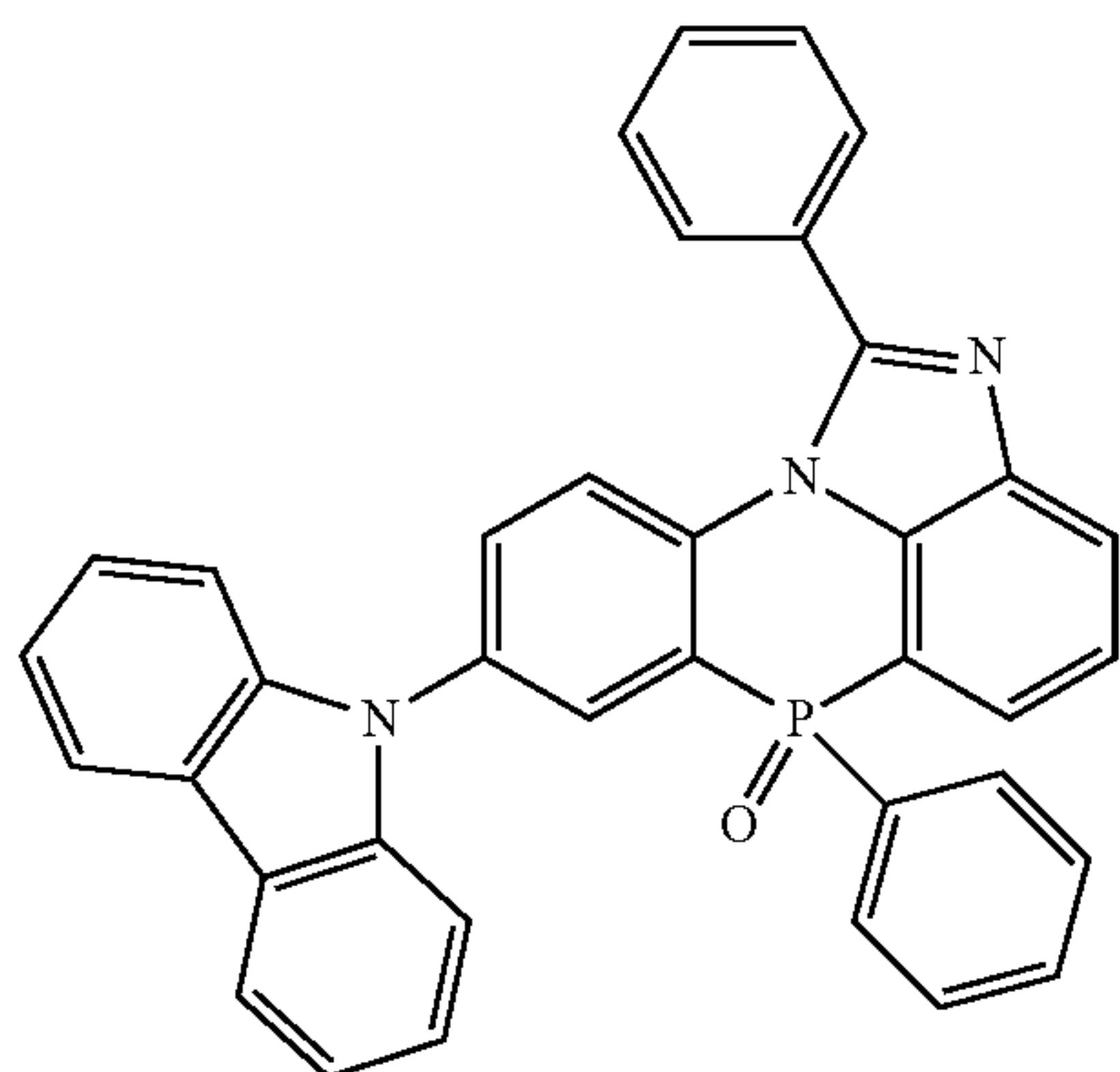
[Chemical Formula 2-4-50]
