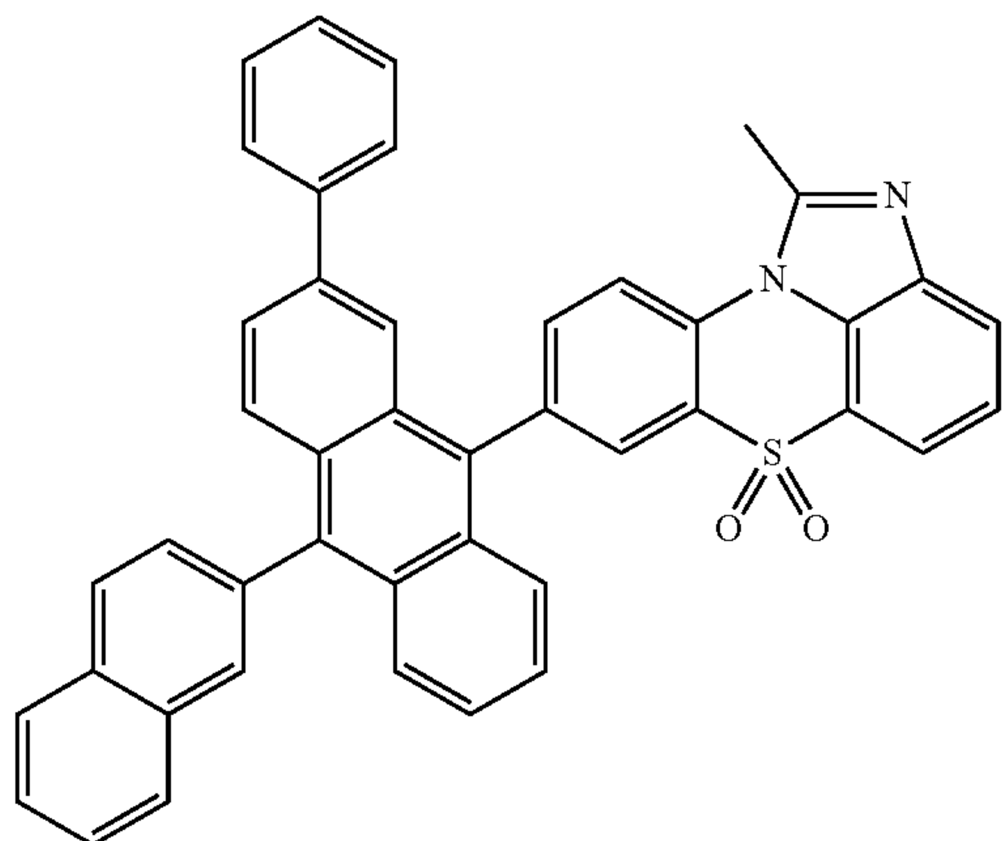
[Chemical Formula 1-2-16]
