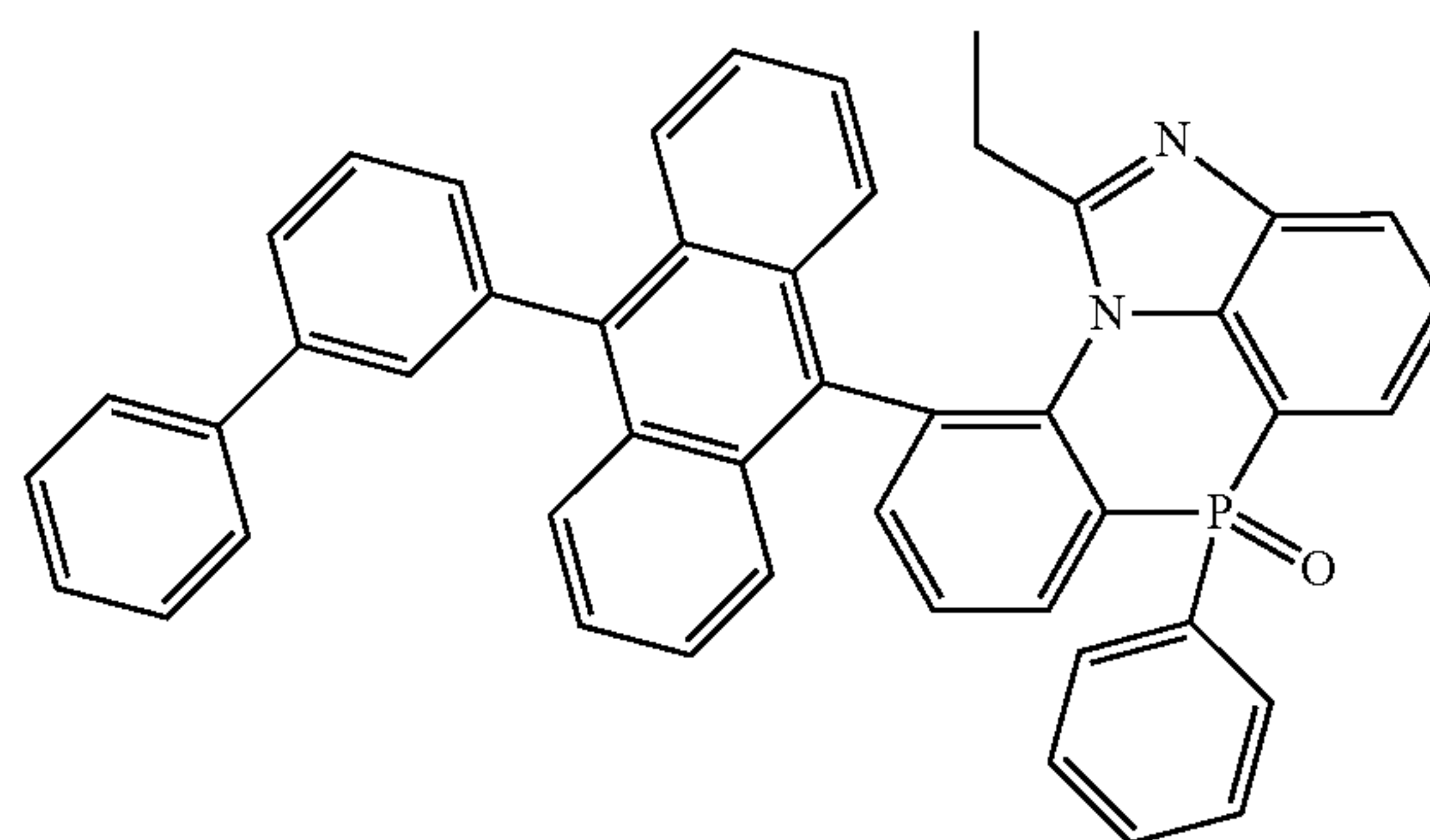
[Chemical Formula 2-8-6]
