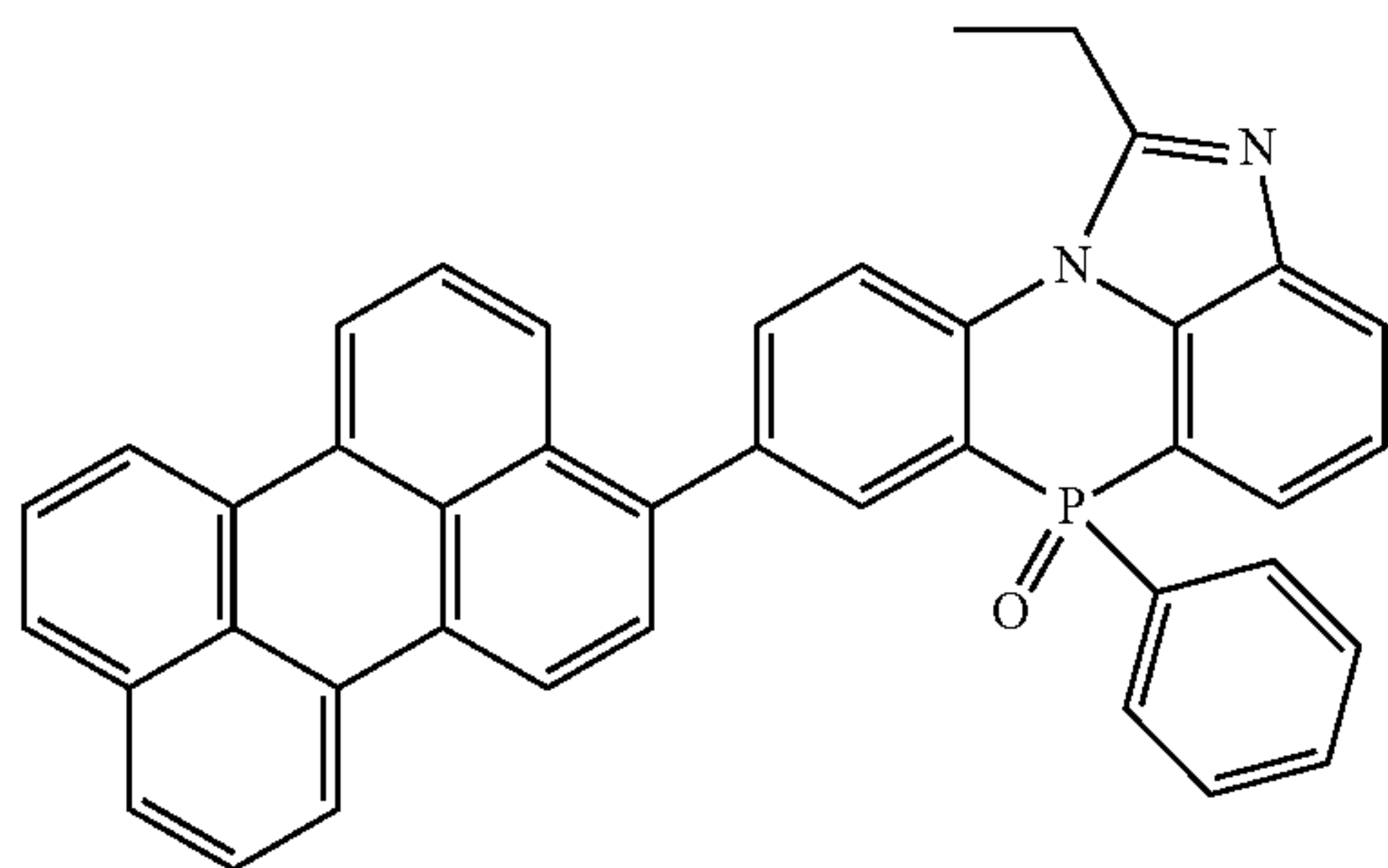
[Chemical Formula 2-3-29]
