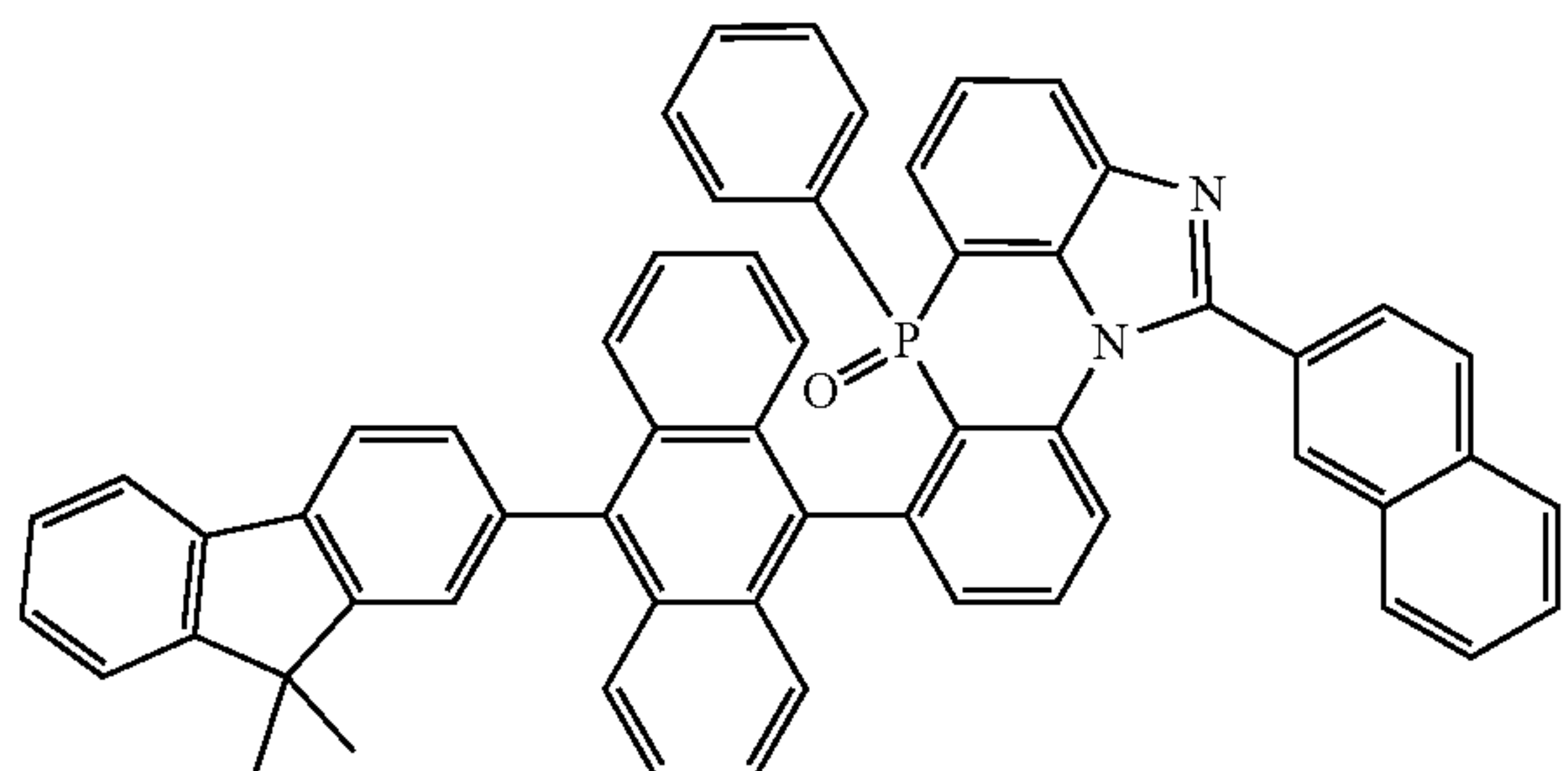
[Chemical Formula 2-6-6]
