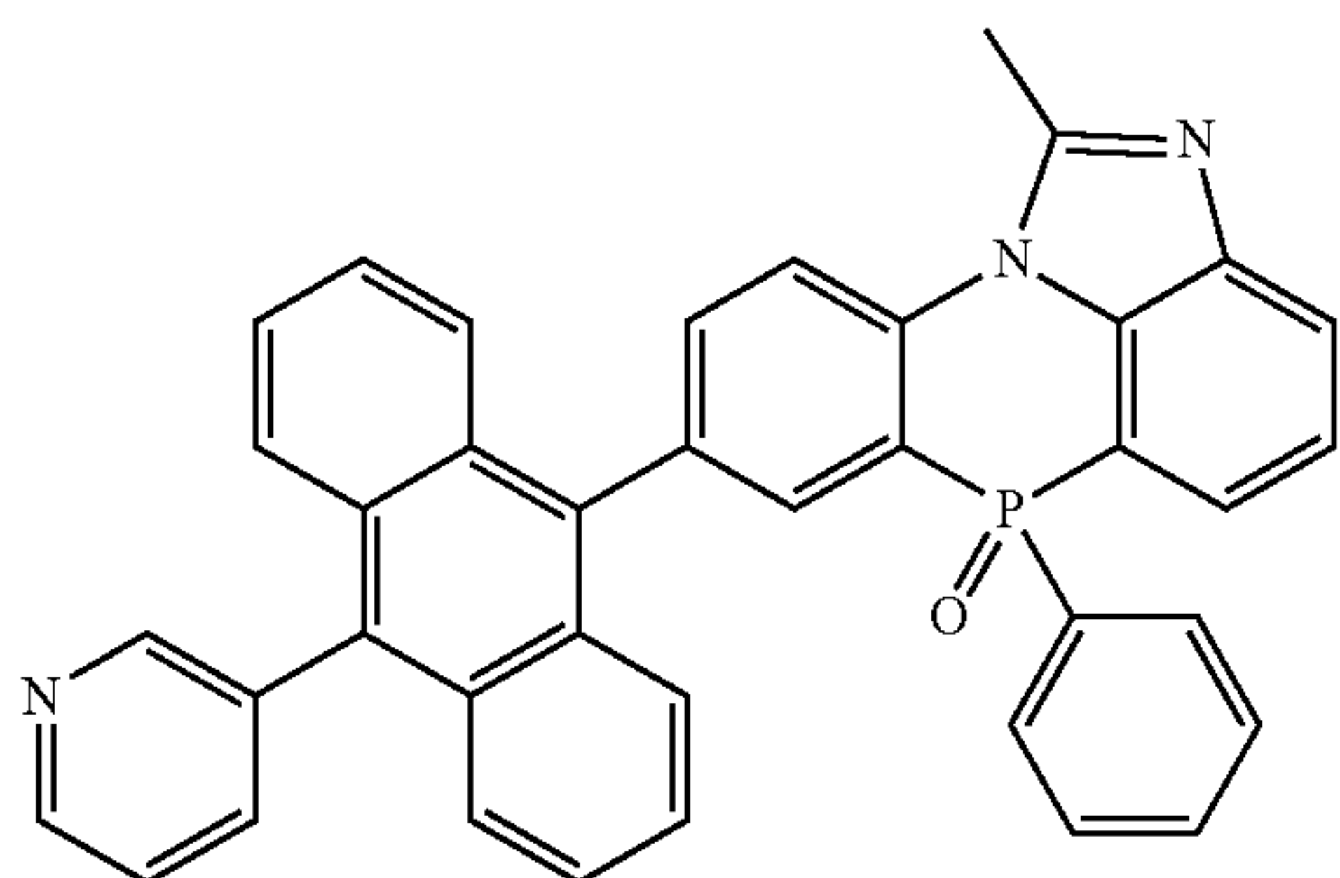
[Chemical Formula 2-2-10]
