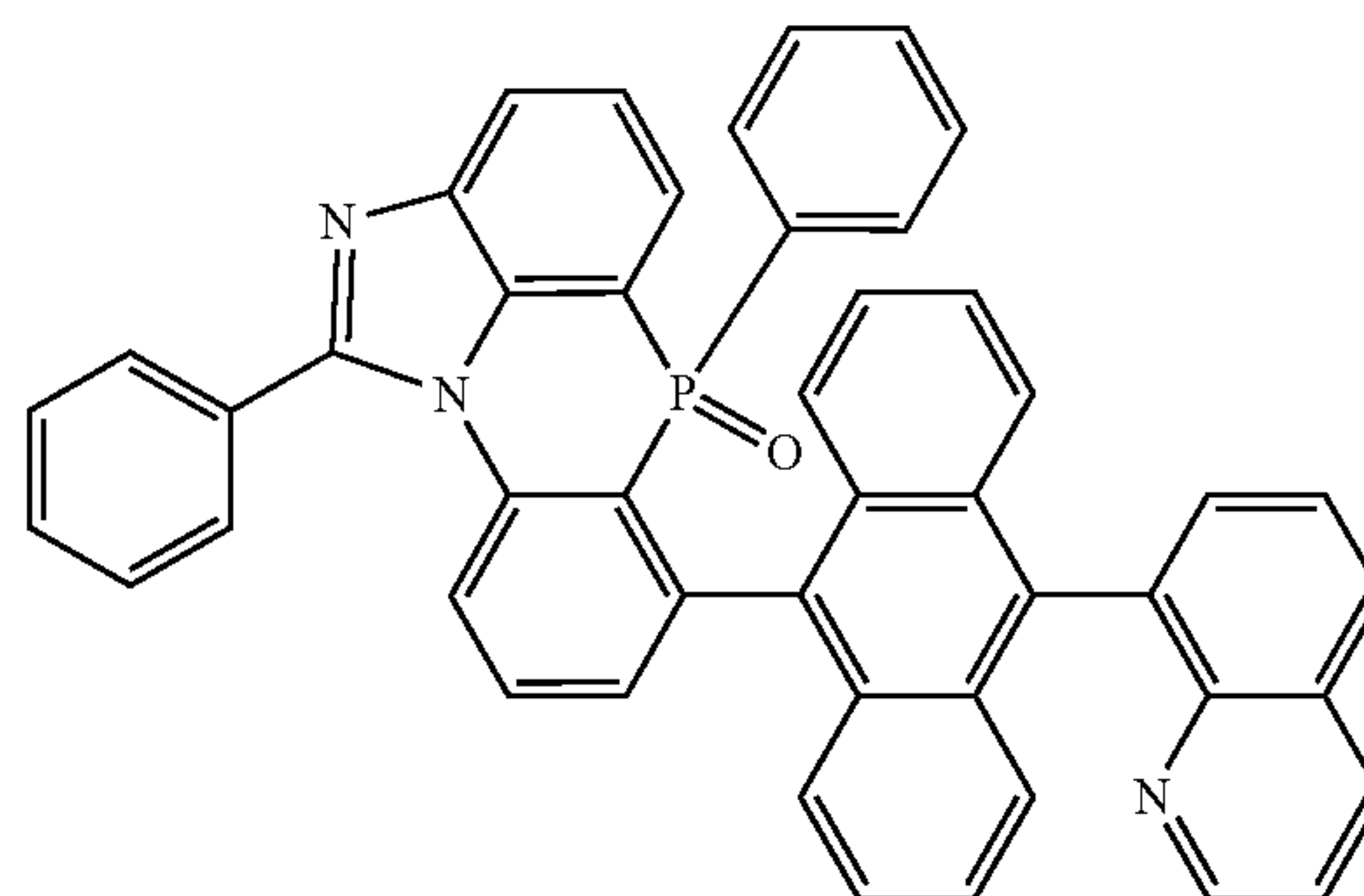
[Chemical Formula 2-6-11]
