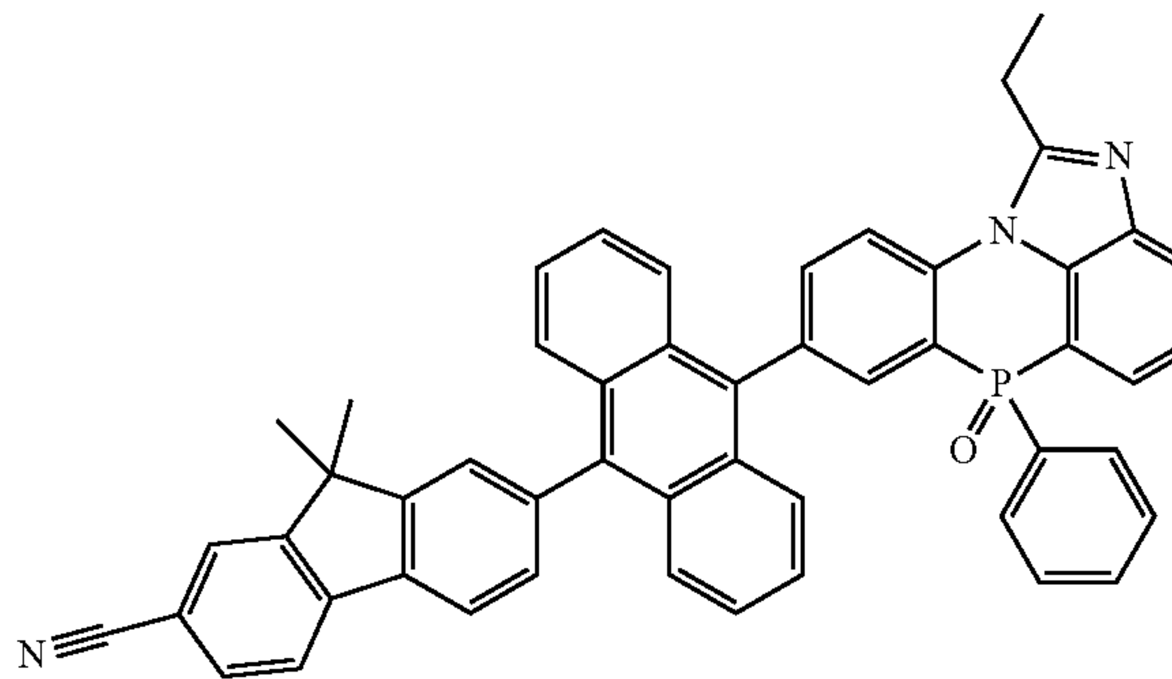
[Chemical Formula 2-3-15]
