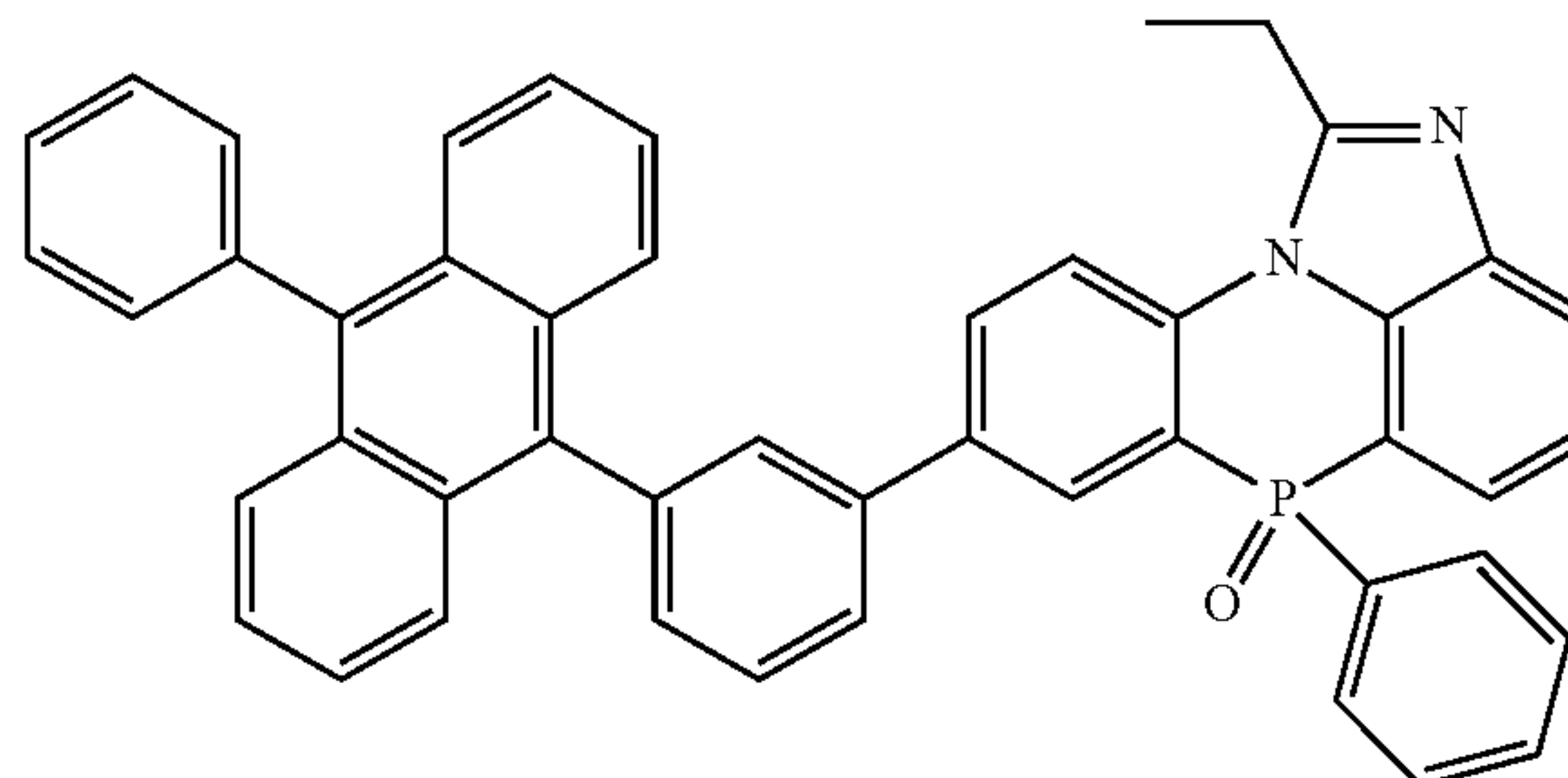
[Chemical Formula 2-3-19]
