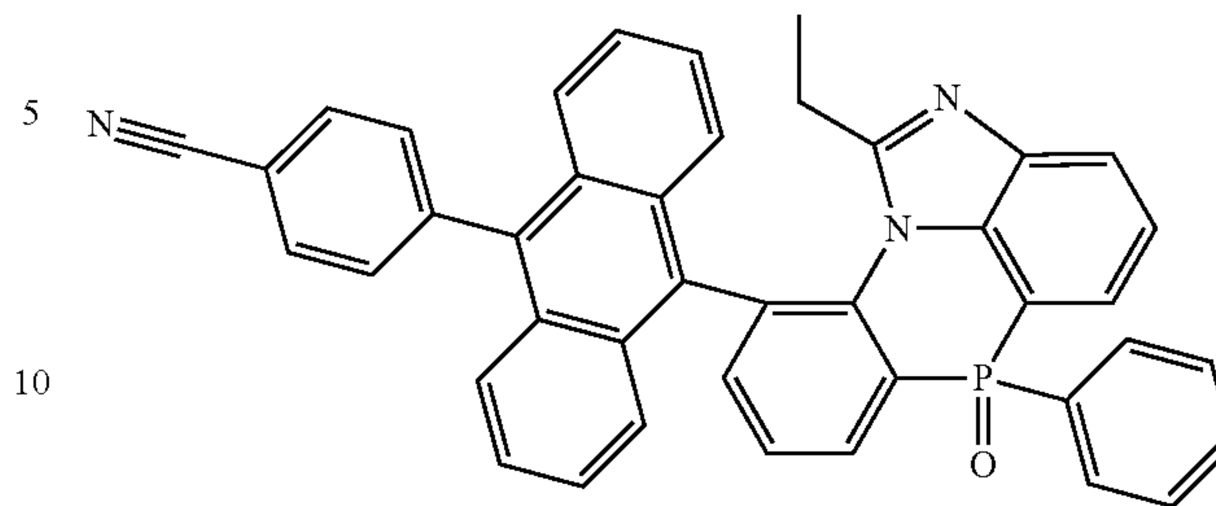
[Chemical Formula 2-8-12]
