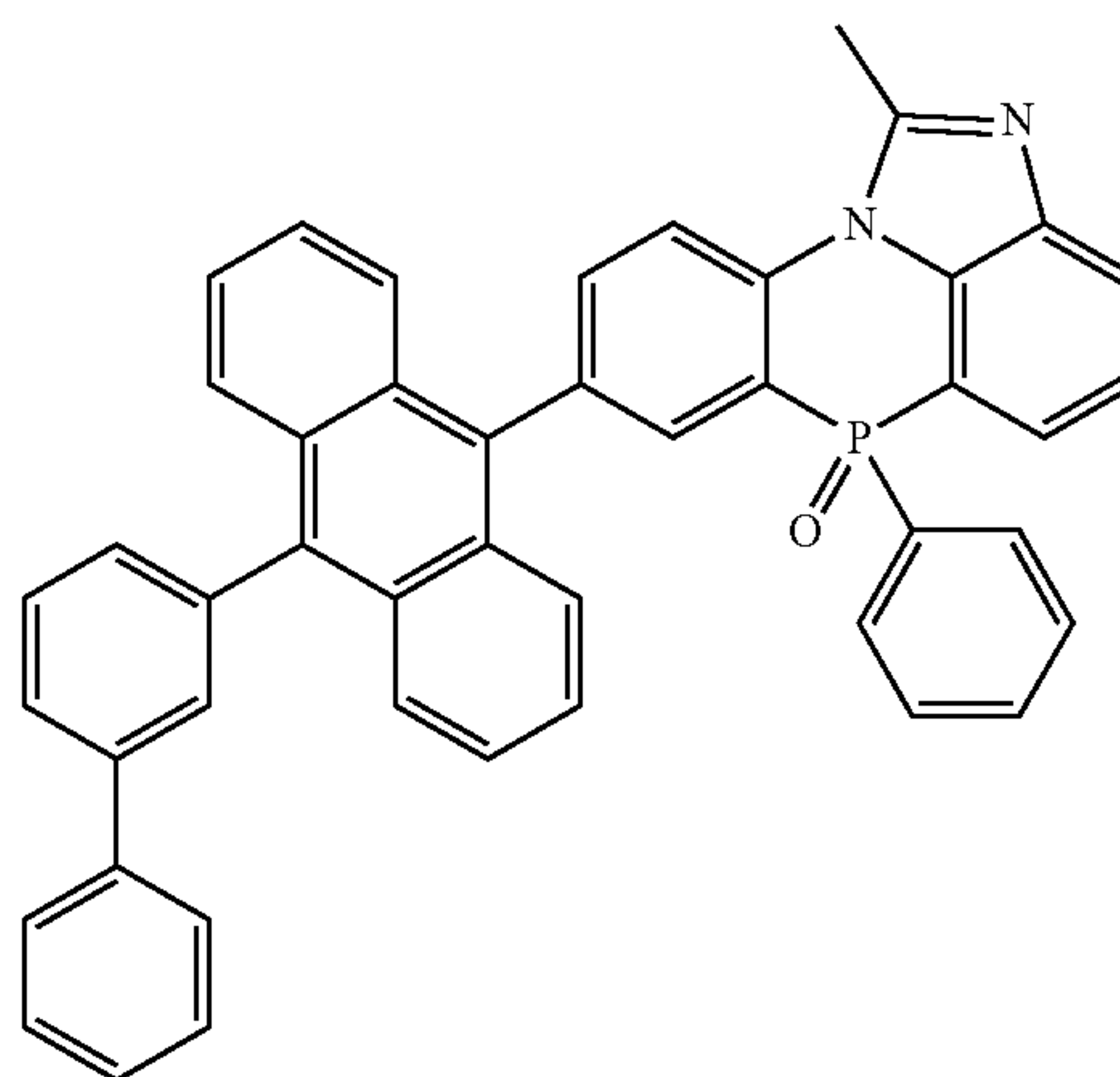
[Chemical Formula 2-2-6]
