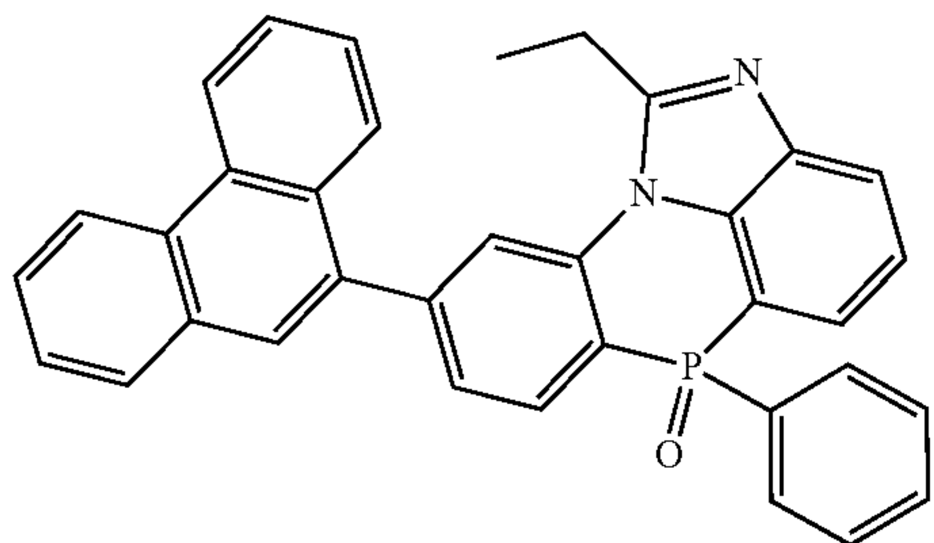
[Chemical Formula 2-7-31]
