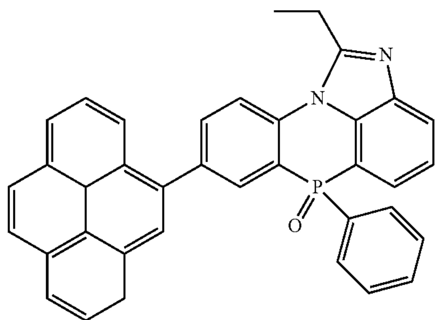
[Chemical Formula 2-3-28]
