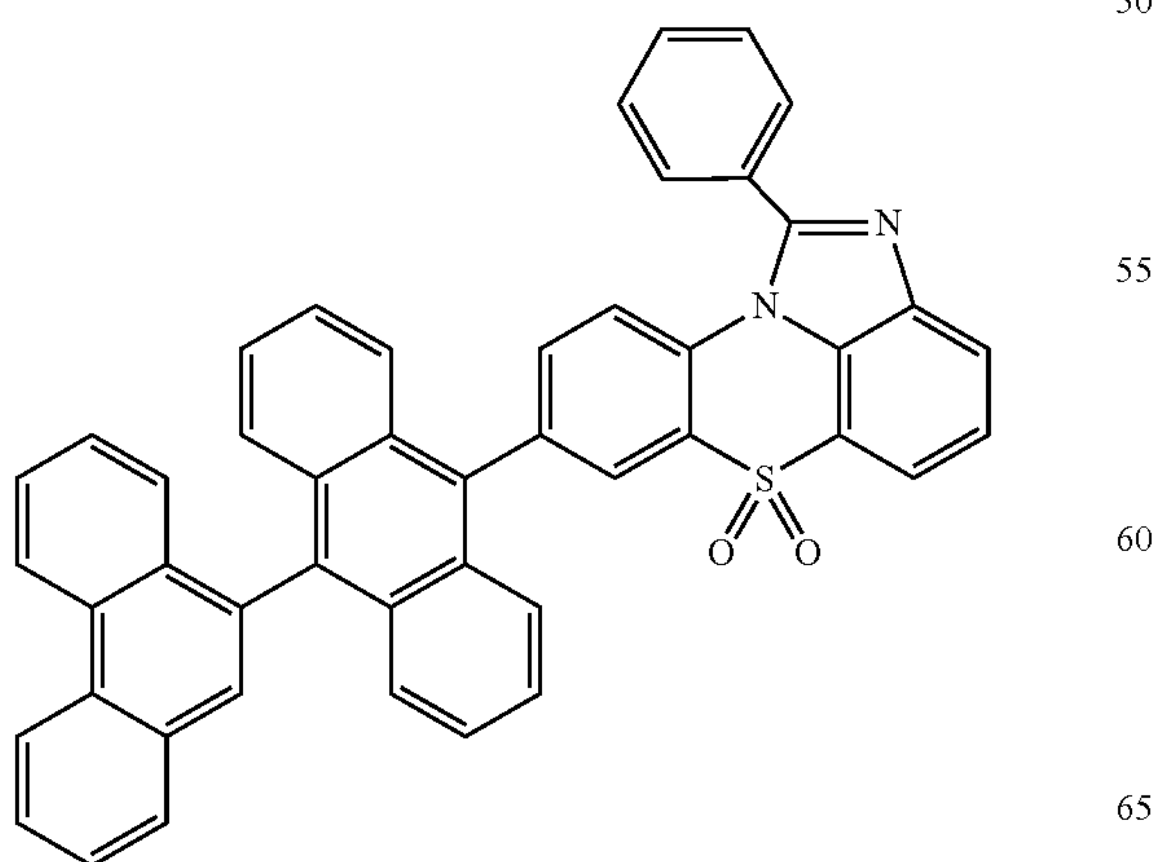
[Chemical Formula 1-4-7]
