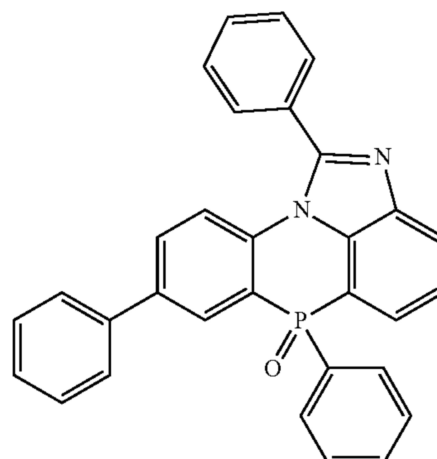
[Chemical Formula 2-4-38]
