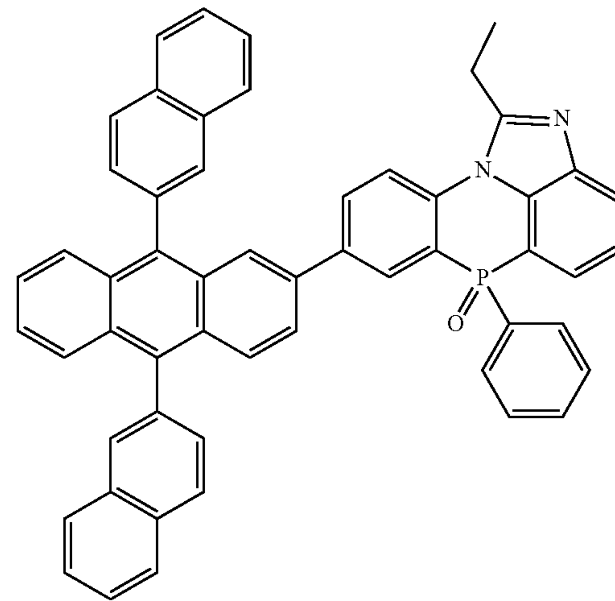
[Chemical Formula 2-3-20]
