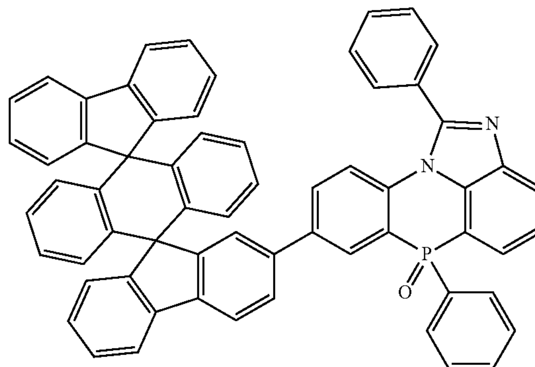
[Chemical Formula 2-4-37]
