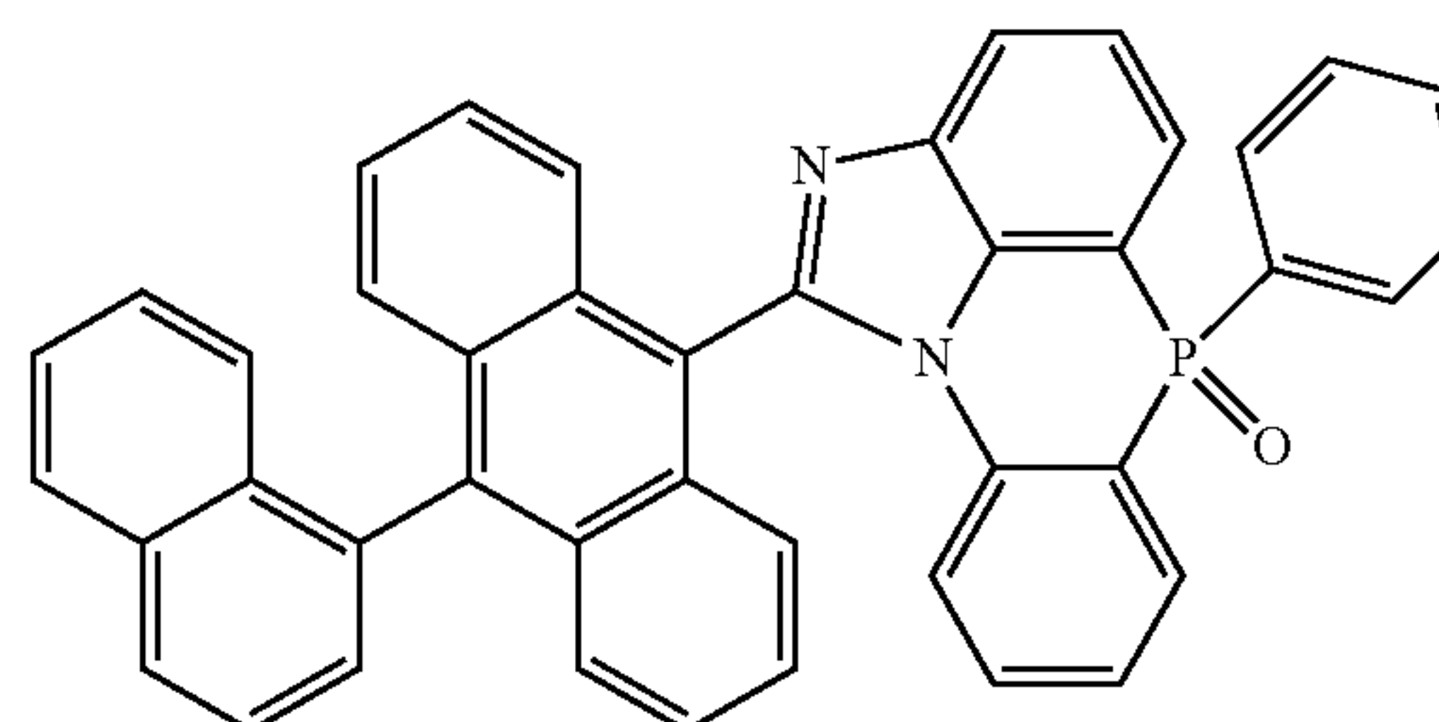
[Chemical Formula 2-5-3]
