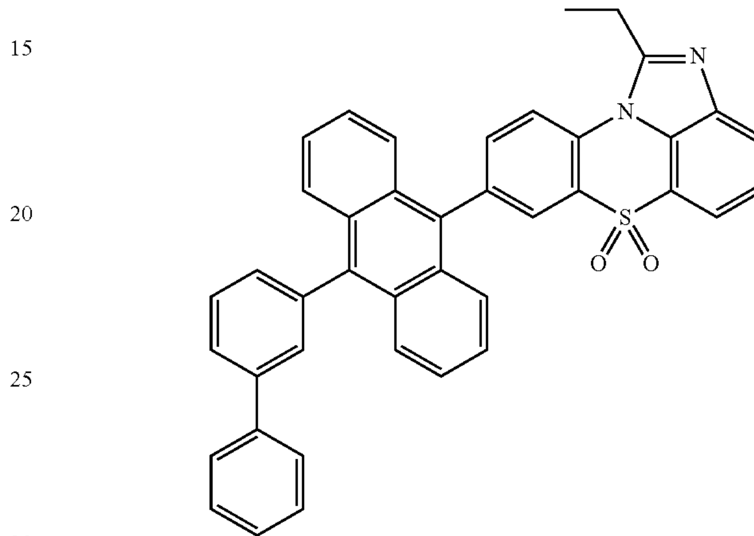
[Chemical Formula 1-3-6]
