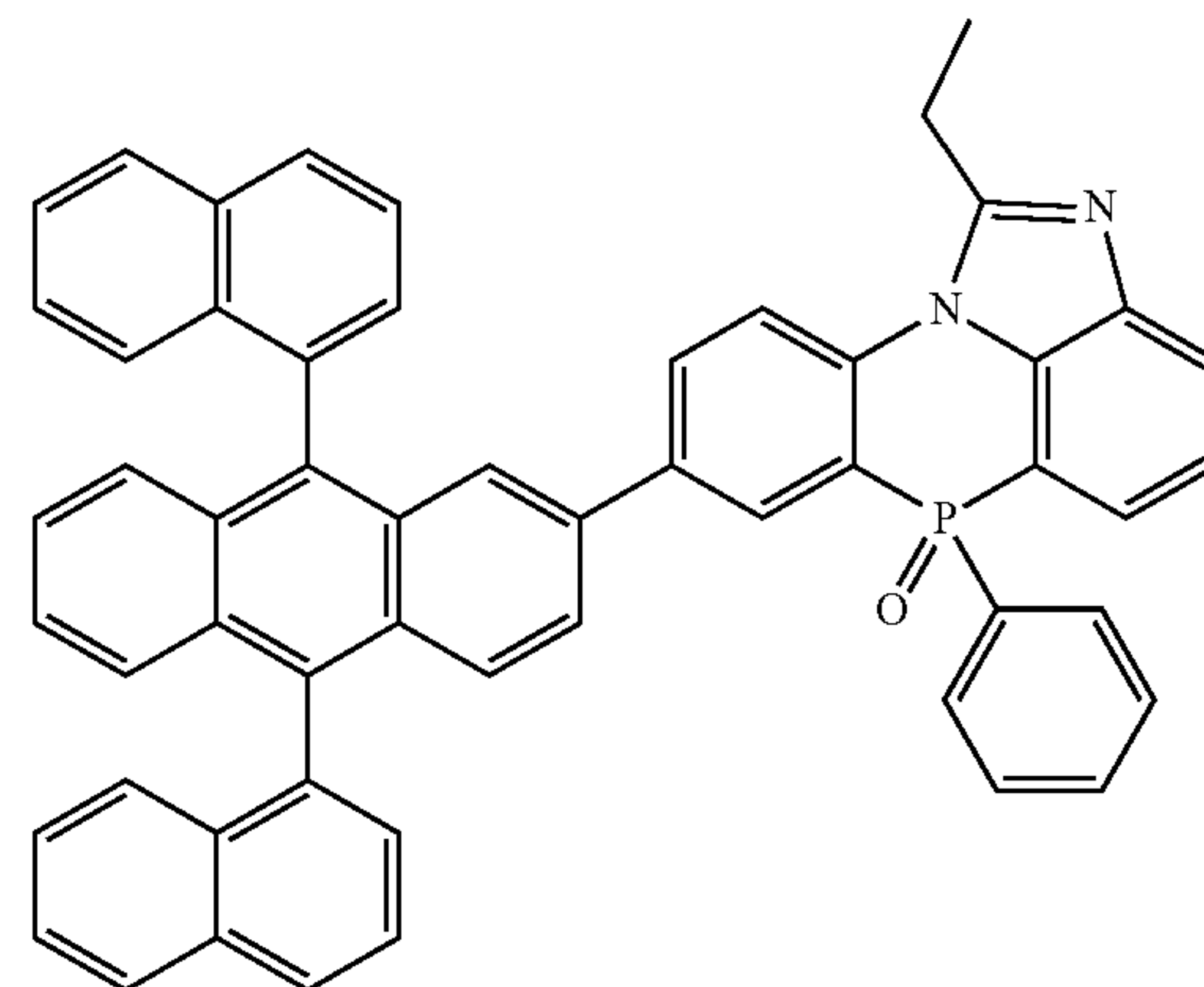
[Chemical Formula 2-3-21]
