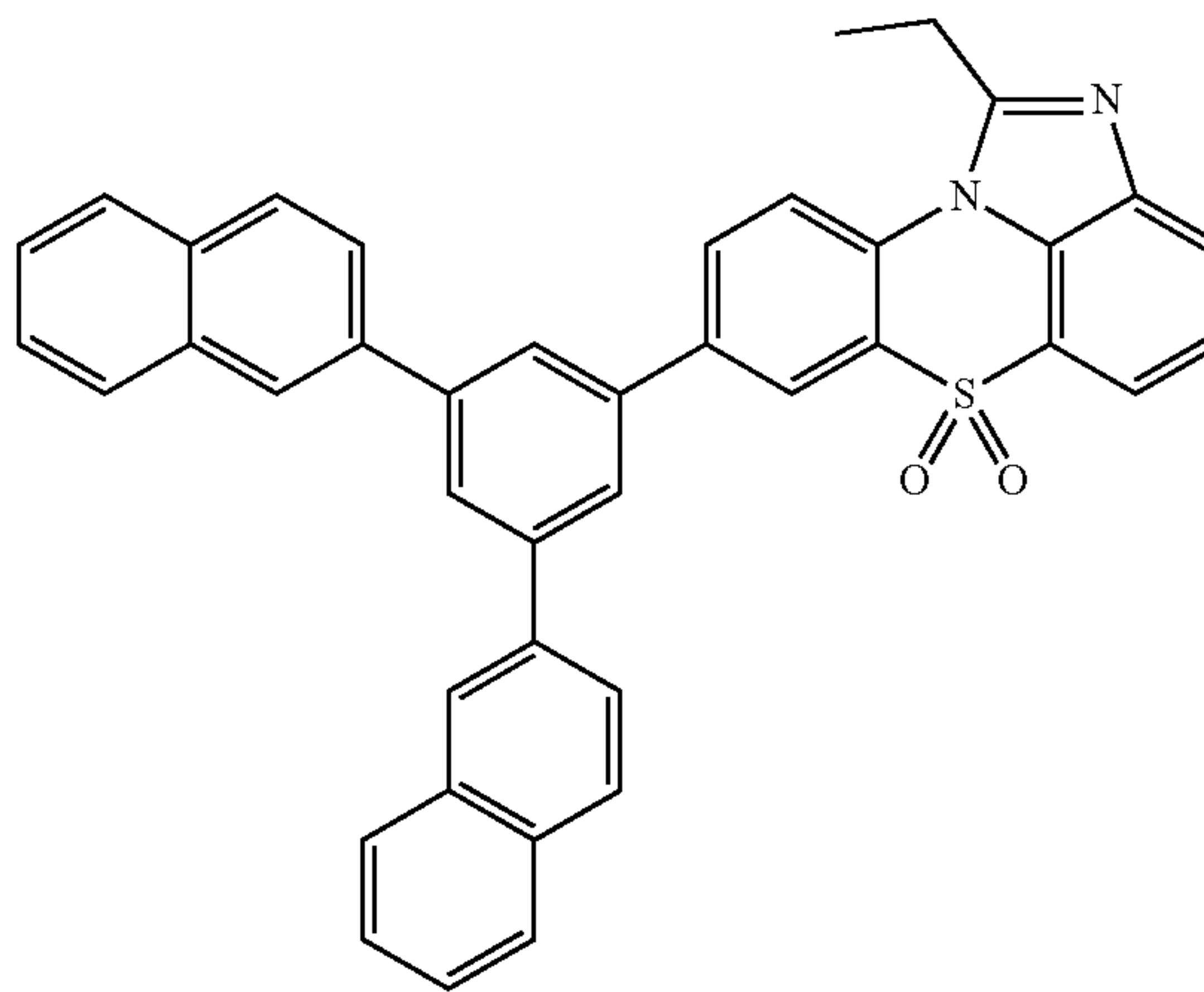
[Chemical Formula 1-3-43]
