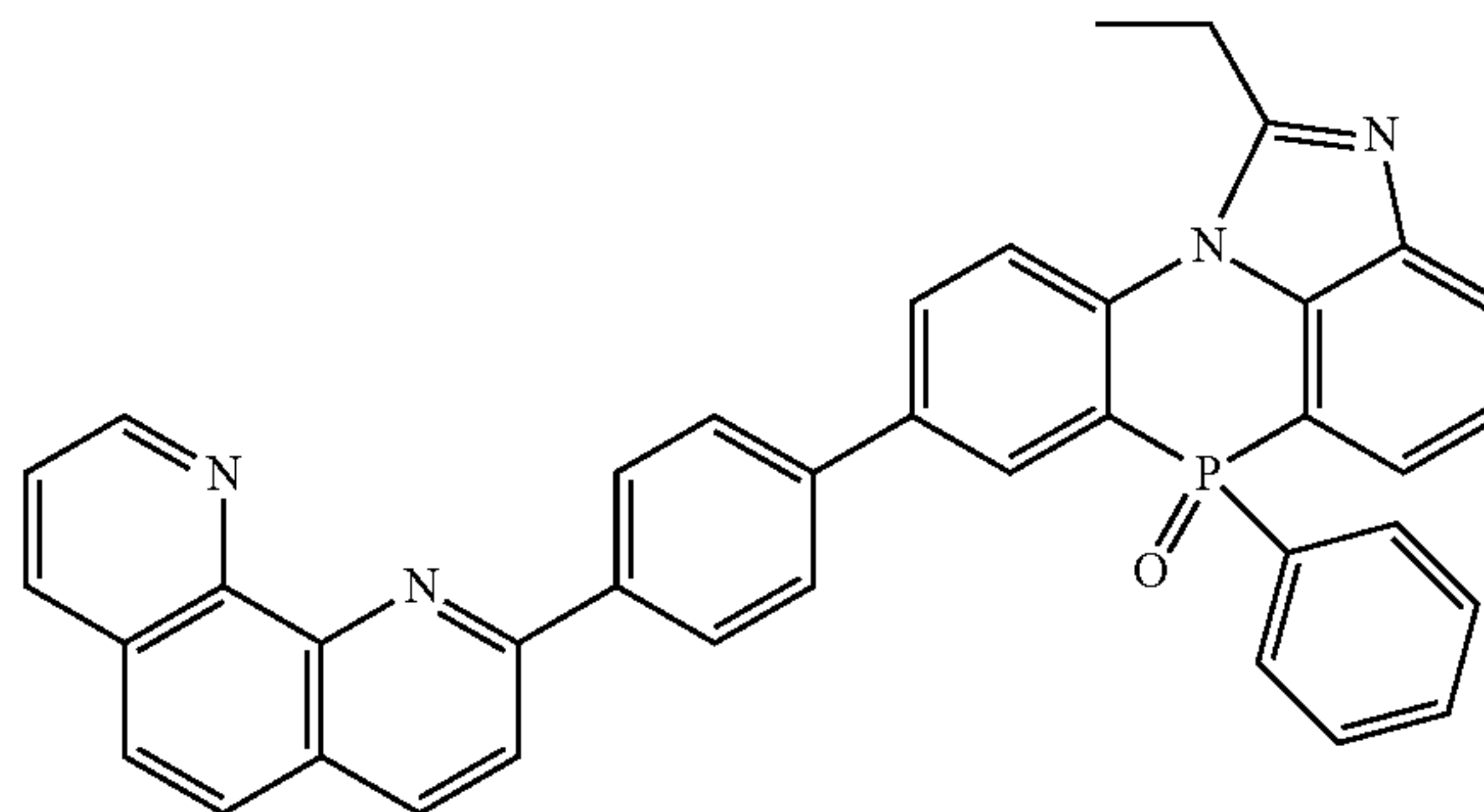
[Chemical Formula 2-3-47]
