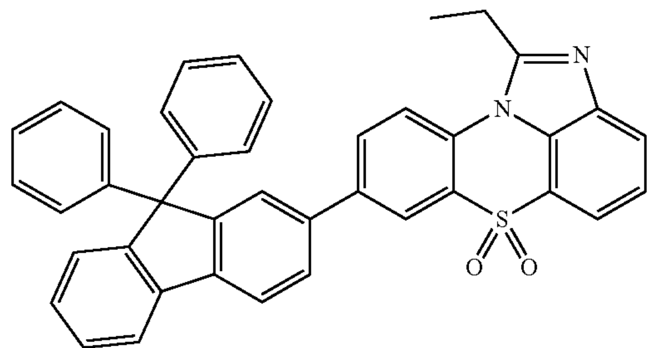
[Chemical Formula 1-3-36]
