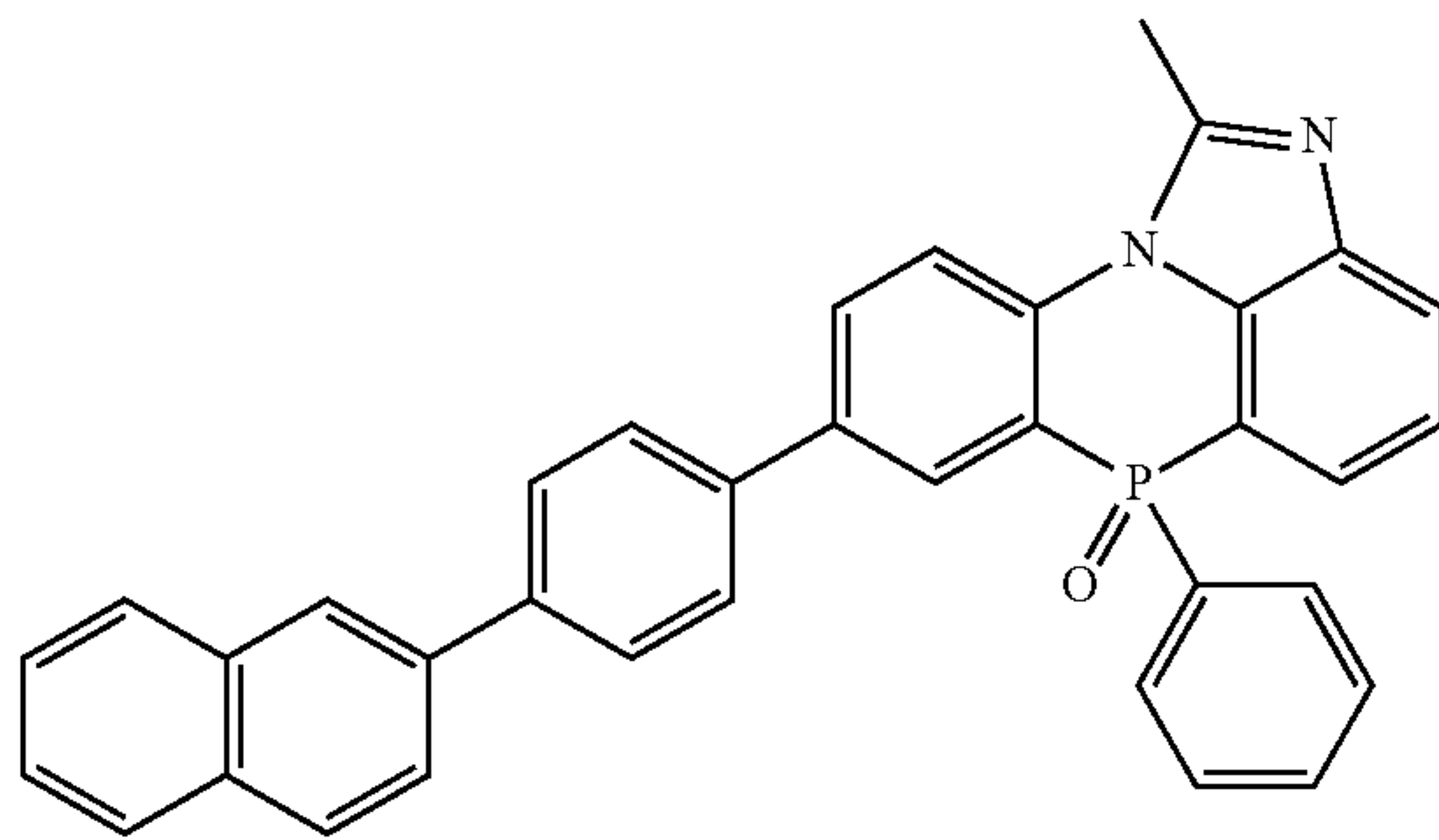
[Chemical Formula 2-2-26]
