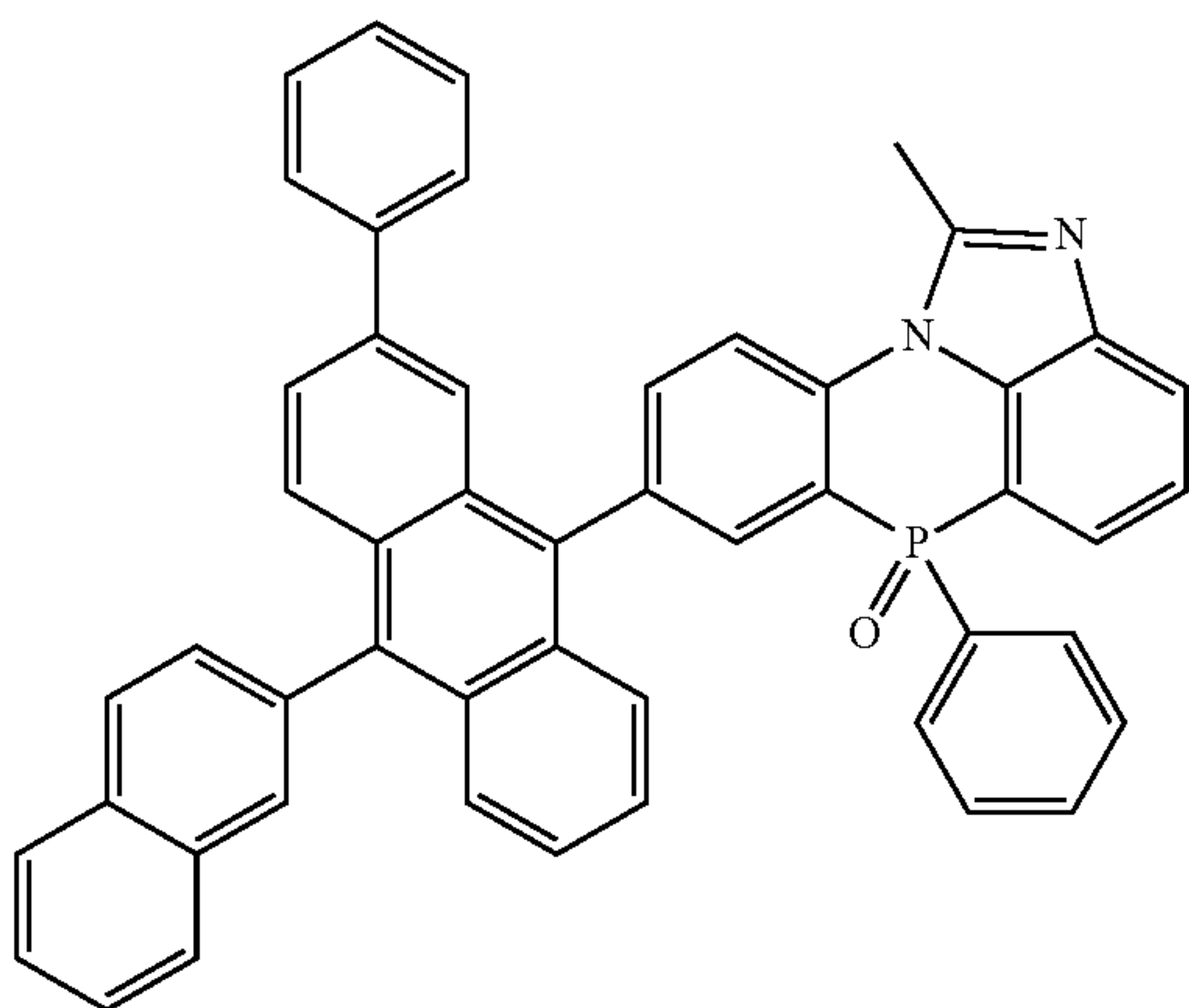
[Chemical Formula 2-2-16]
