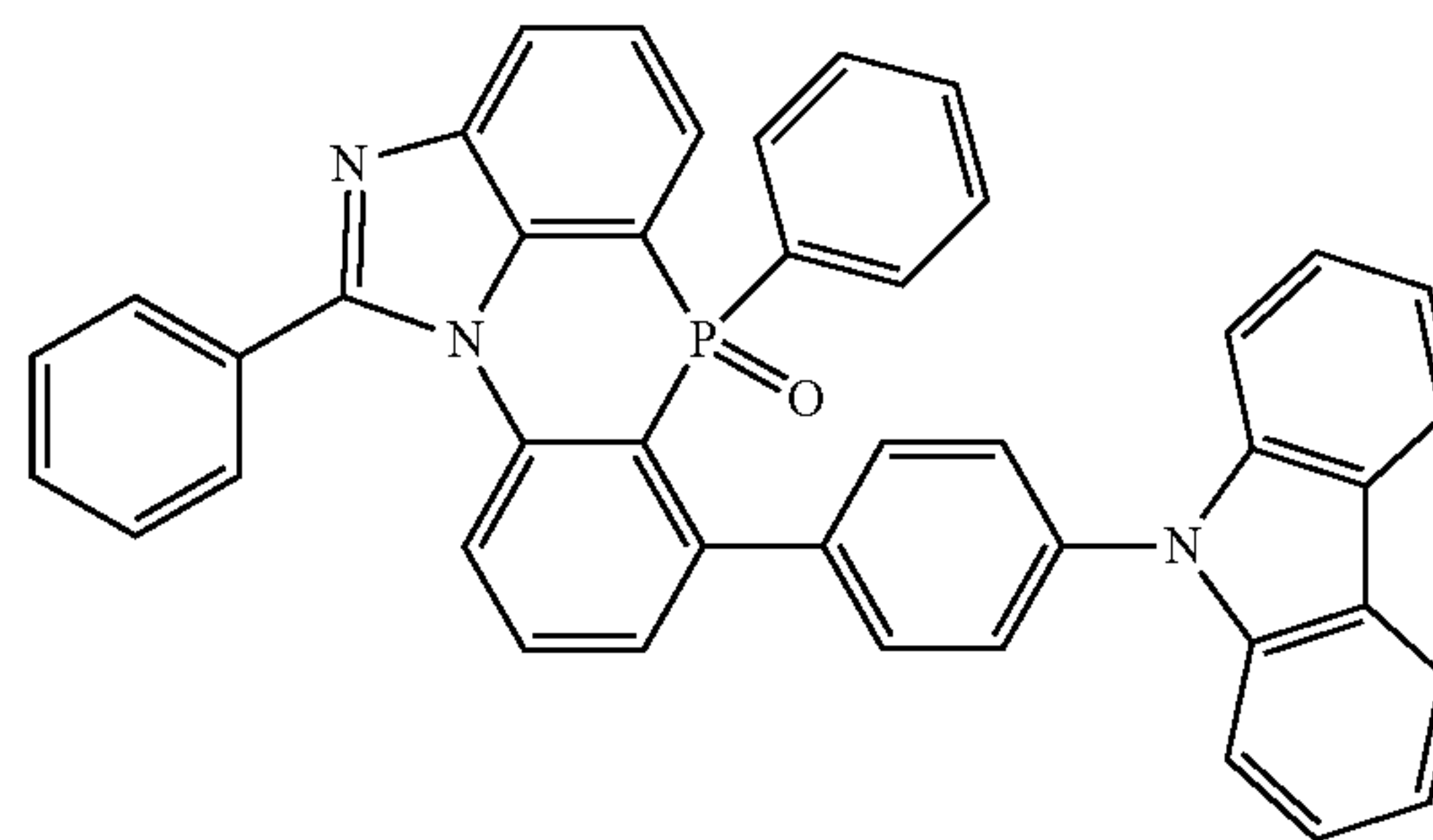
[Chemical Formula 2-6-42]
