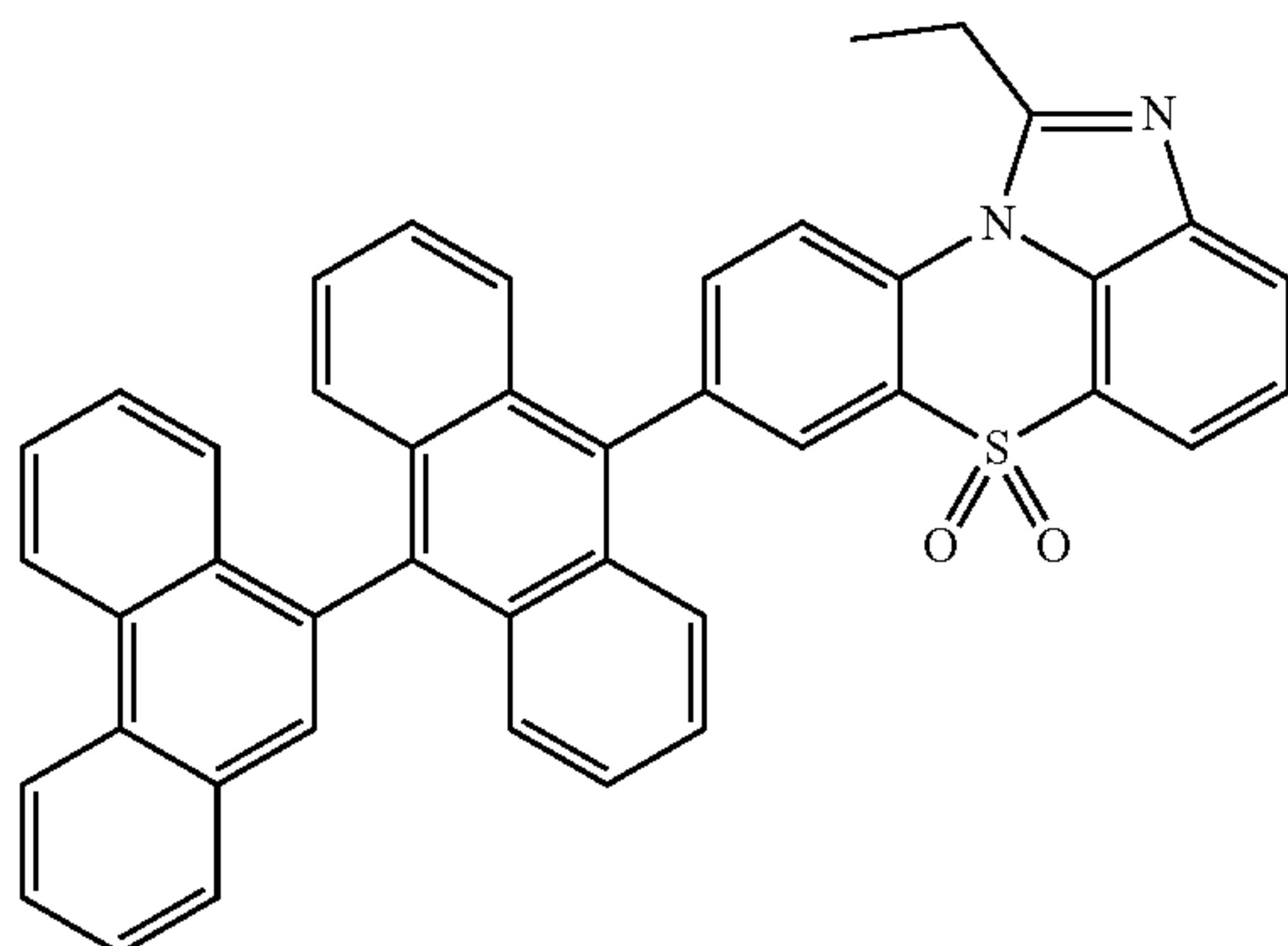
[Chemical Formula 1-3-7]
