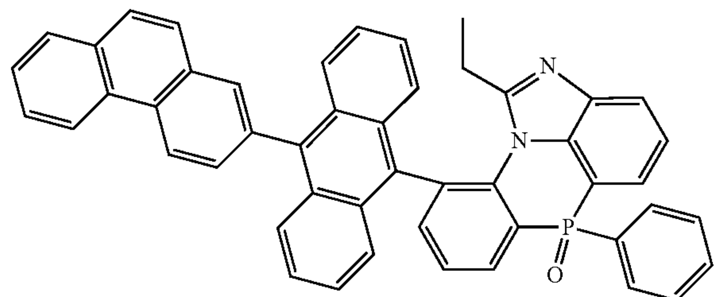
[Chemical Formula 2-8-9]
