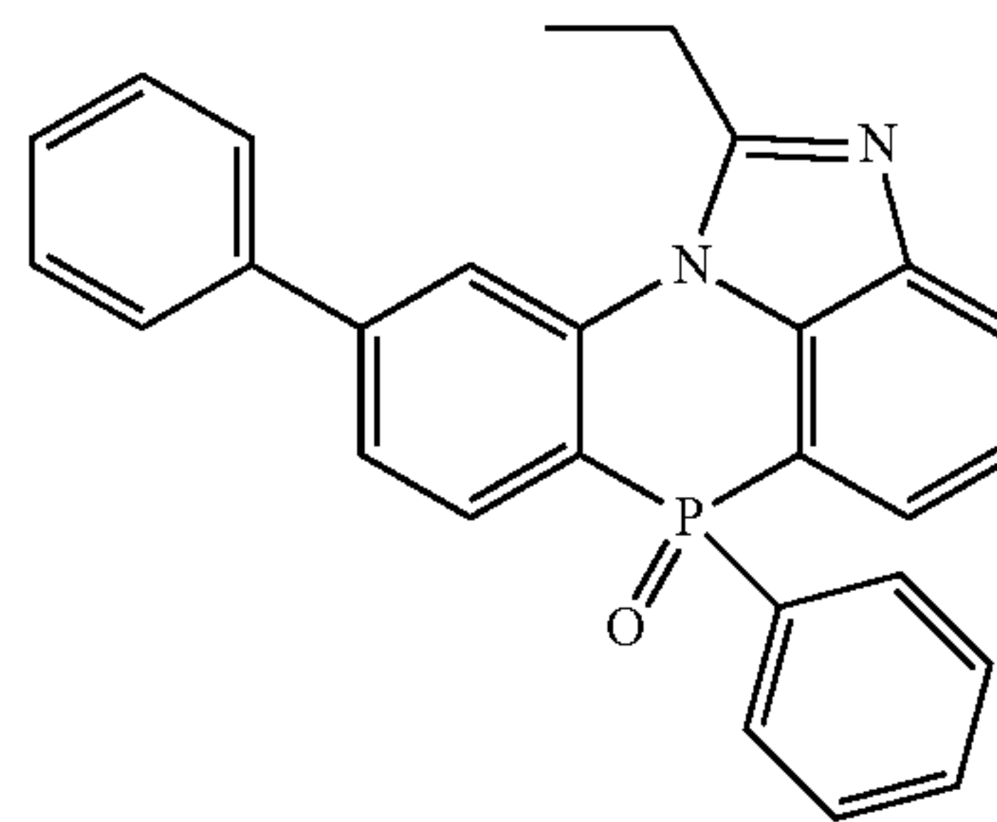
[Chemical Formula 2-7-37]
