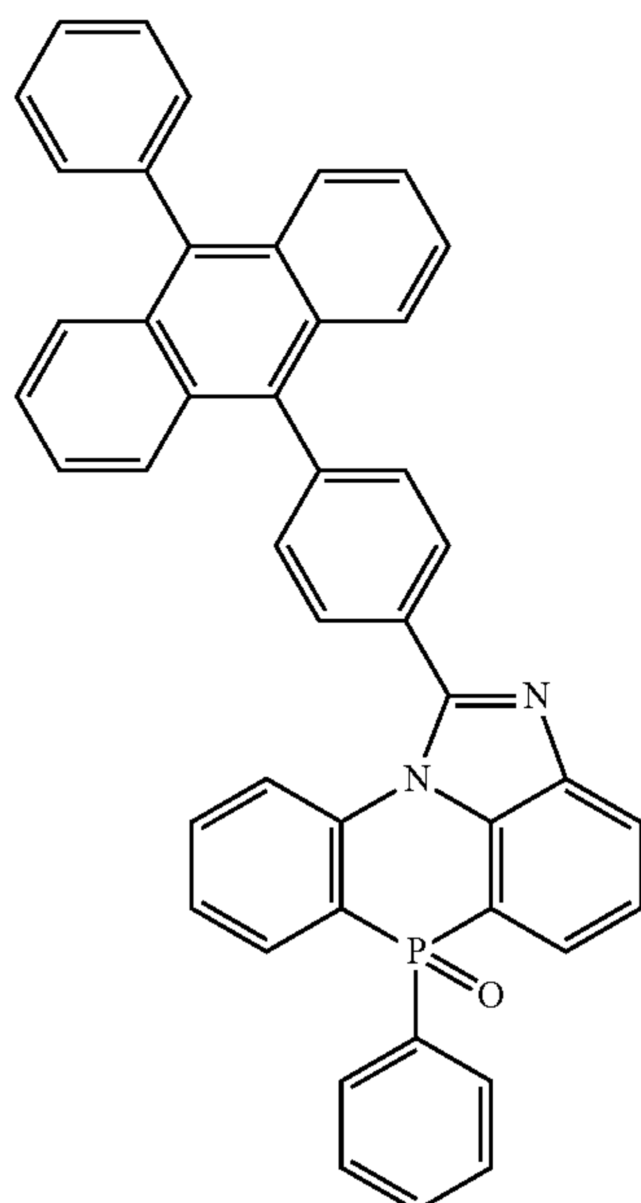
[Chemical Formula 2-5-17]
