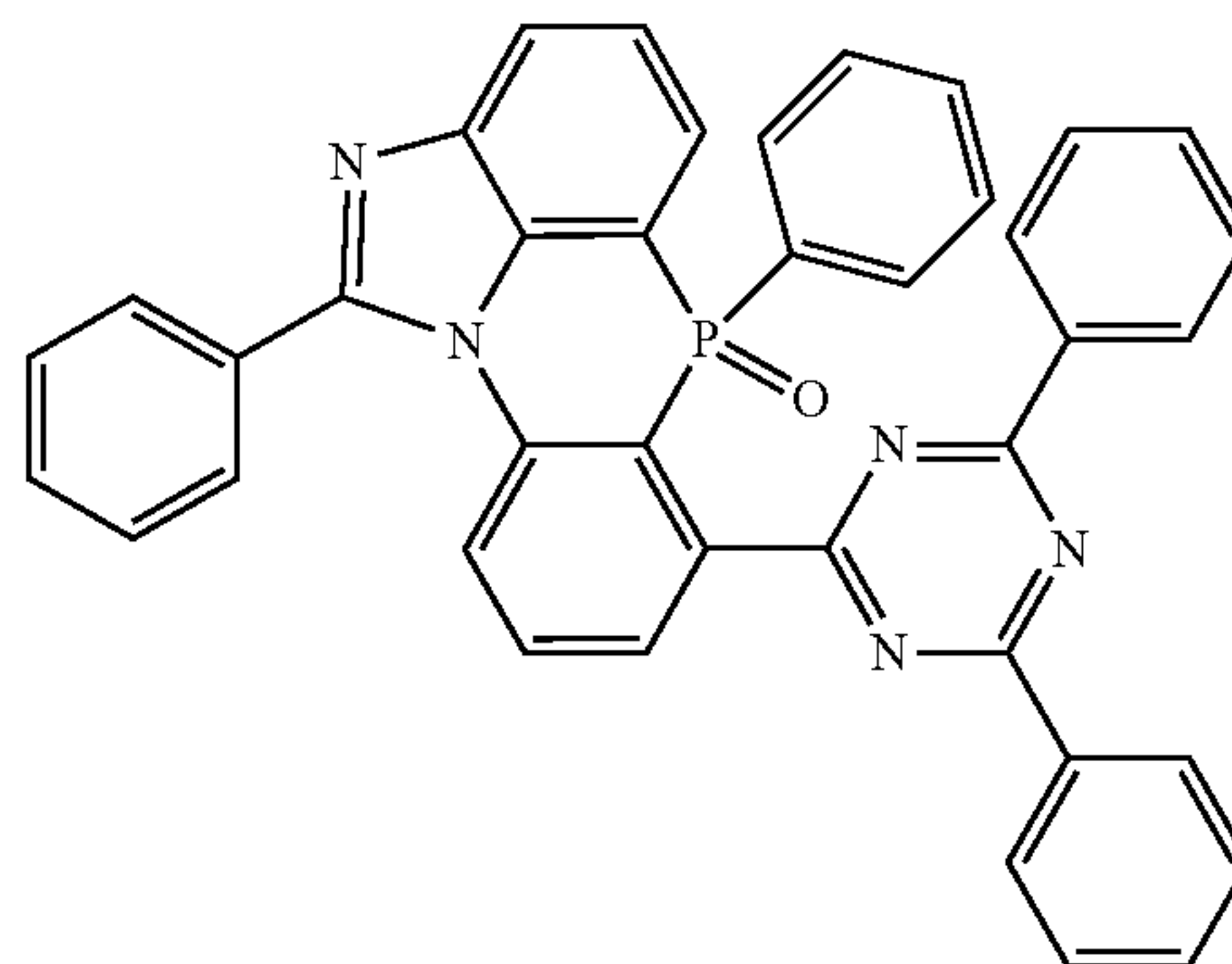
[Chemical Formula 2-6-41]
