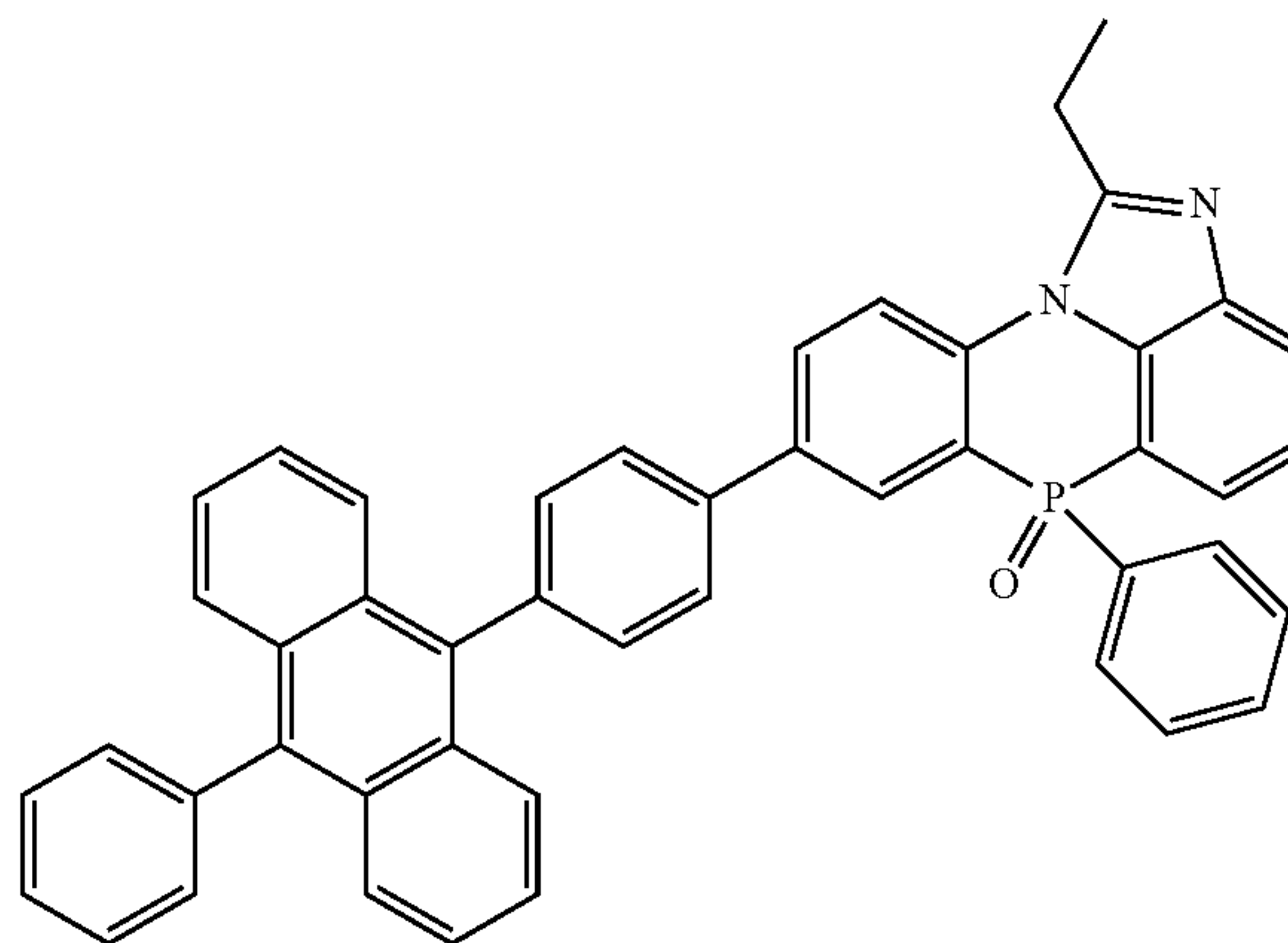
[Chemical Formula 2-3-17]
