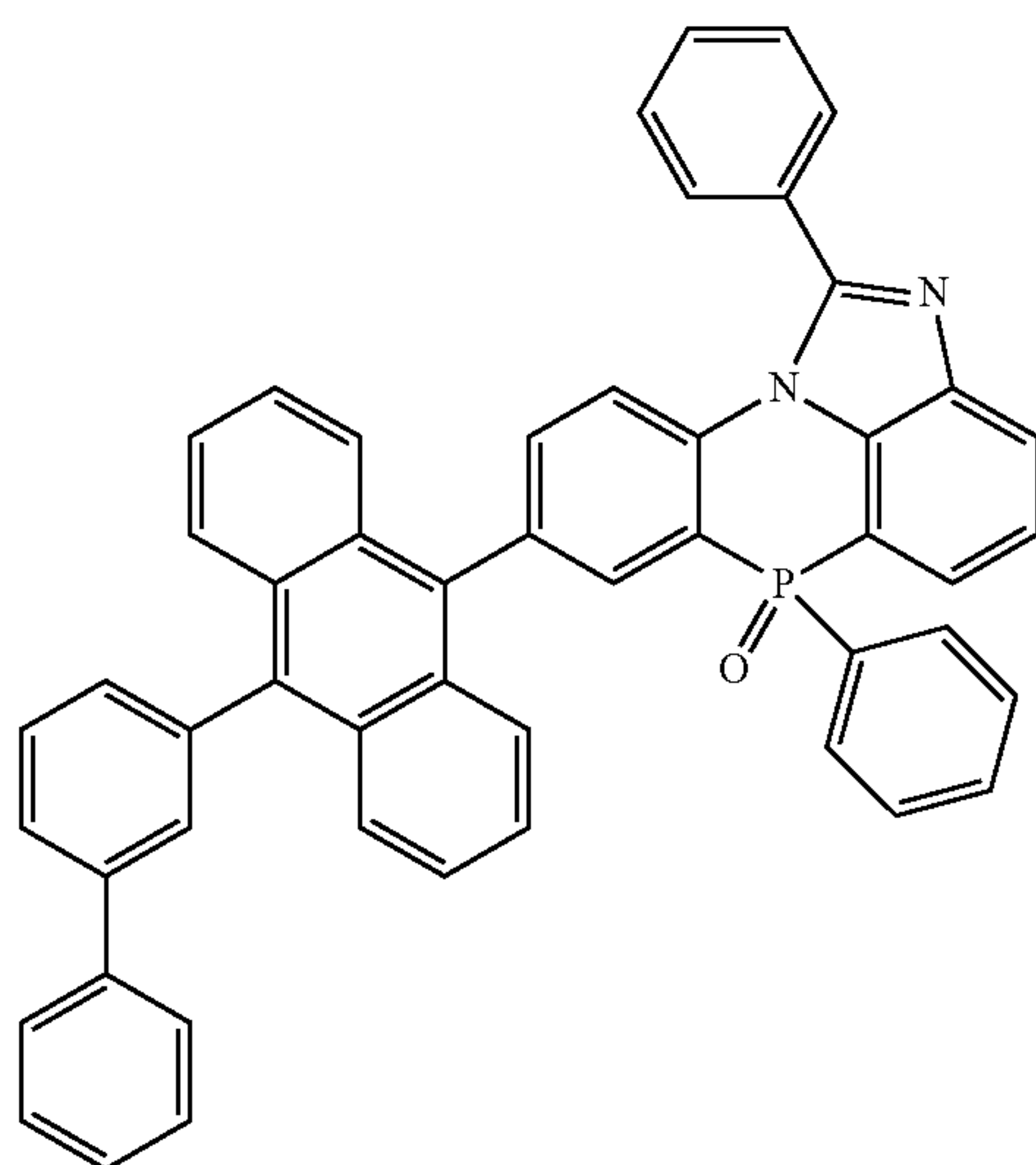
[Chemical Formula 2-4-6]
