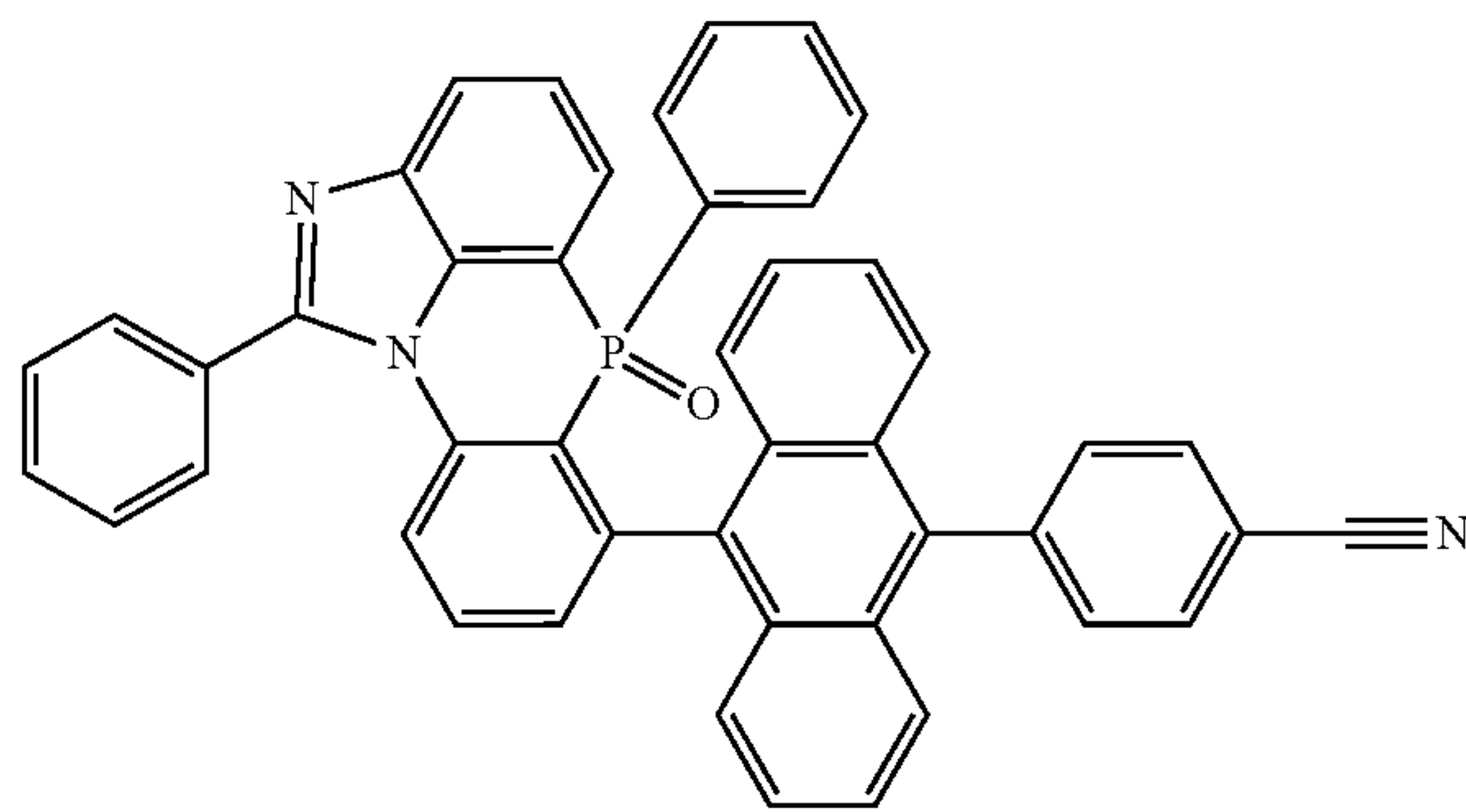
[Chemical Formula 2-6-12]
