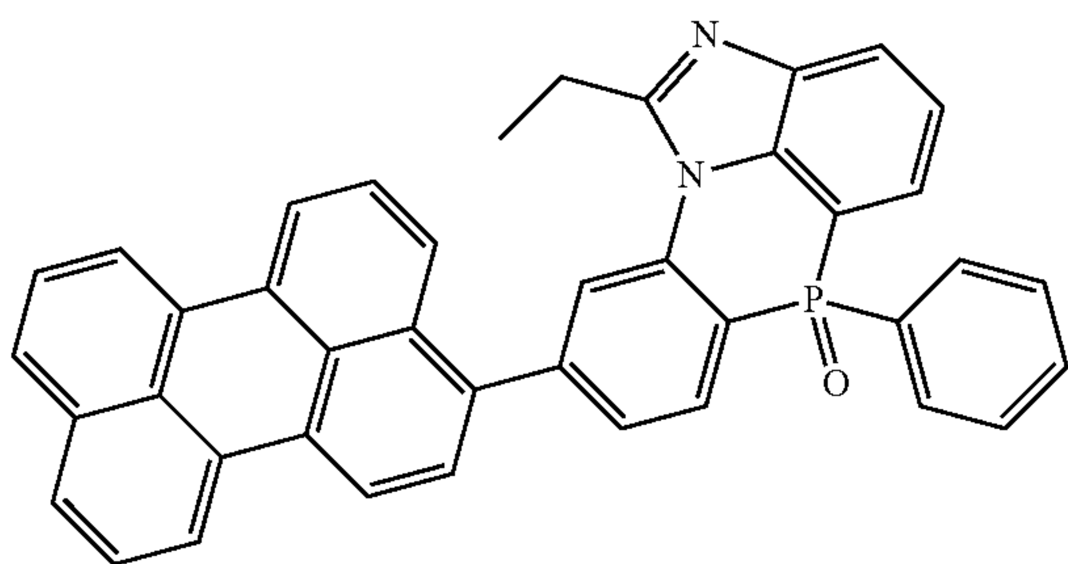
[Chemical Formula 2-7-29]
