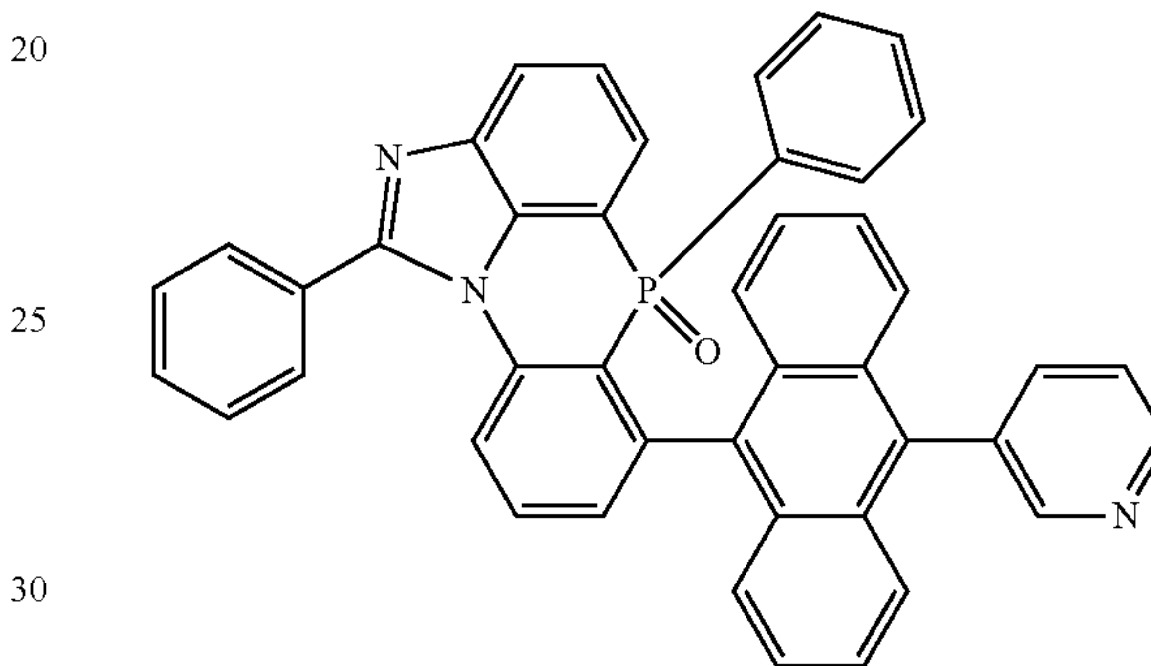
[Chemical Formula 2-6-10]
