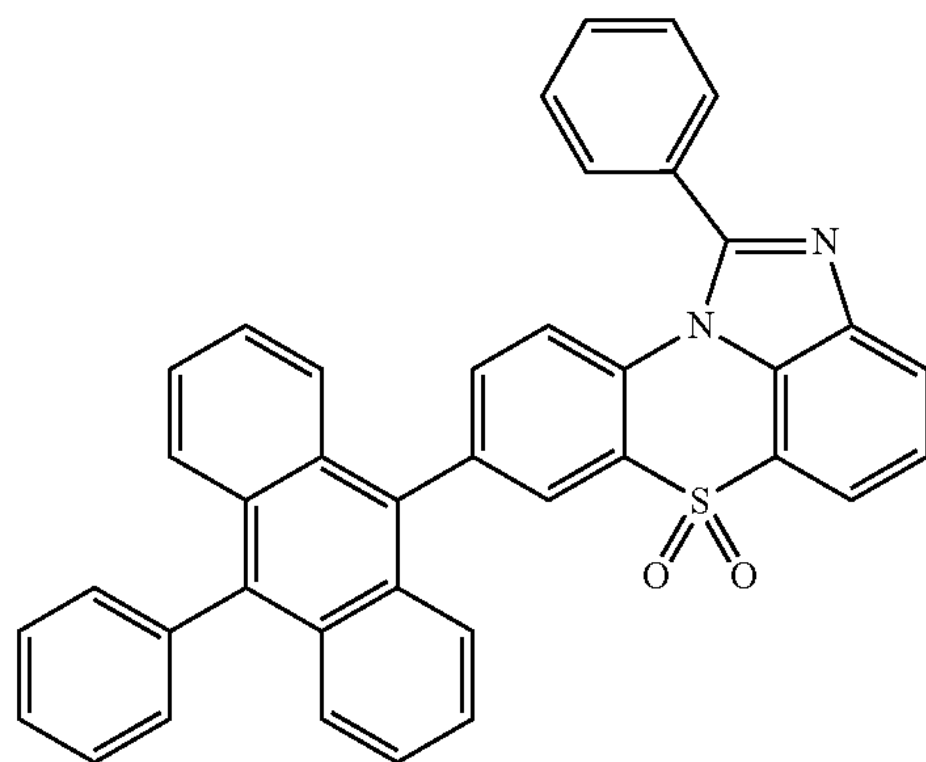
[Chemical Formula 1-4-1]
