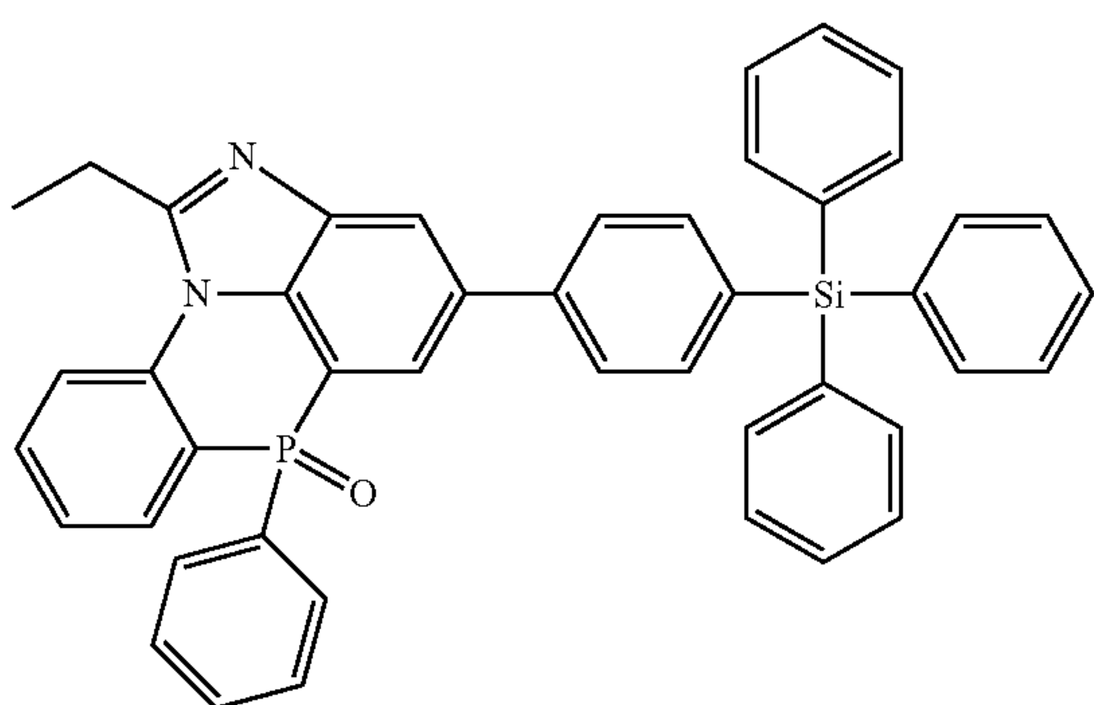
[Chemical Formula 2-10-12]
