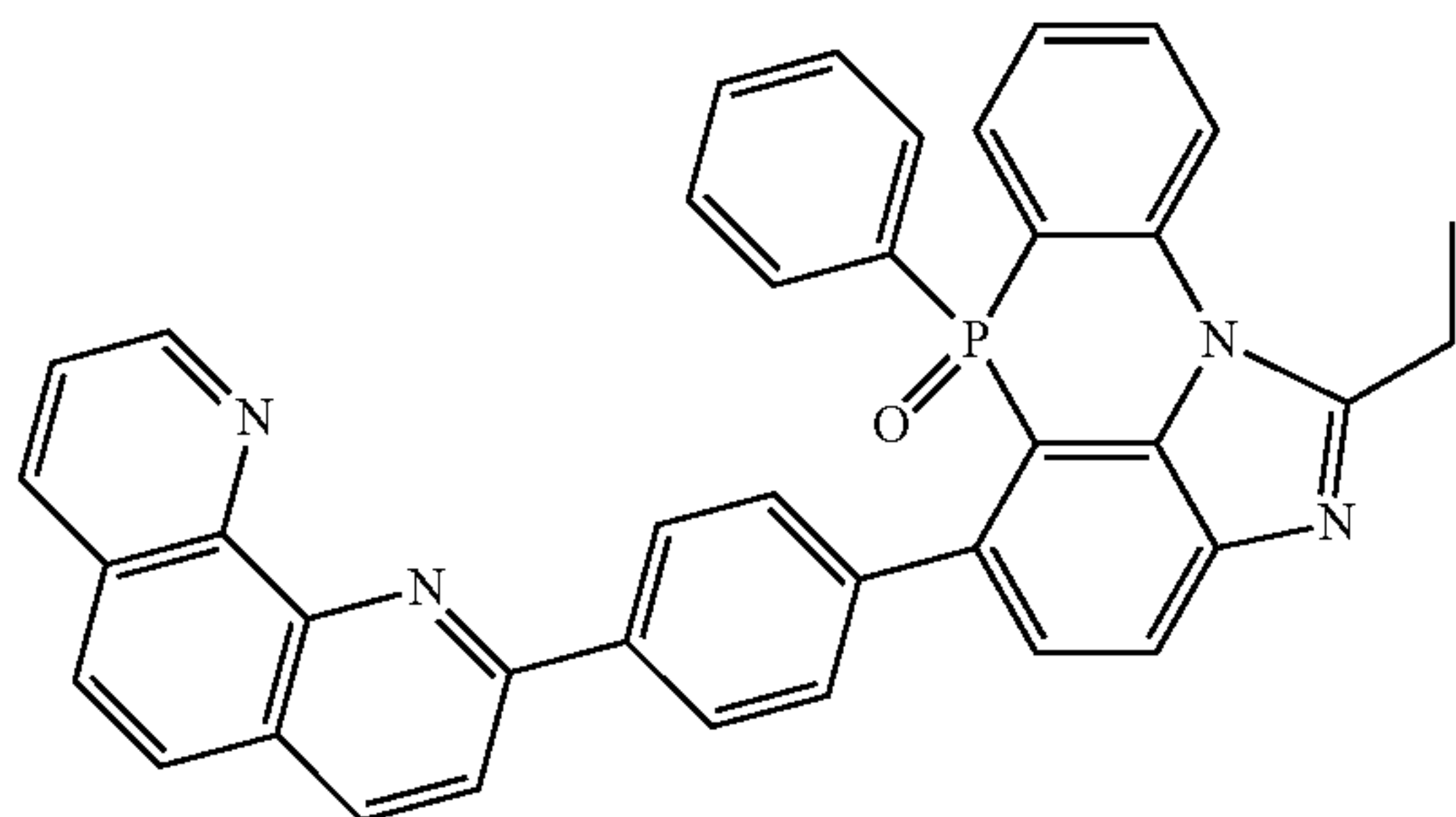
[Chemical Formula 2-9-11]
