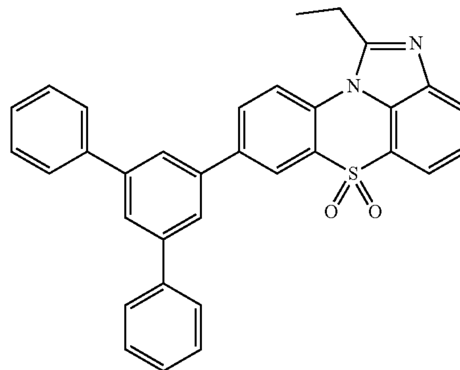
[Chemical Formula 1-3-40]
