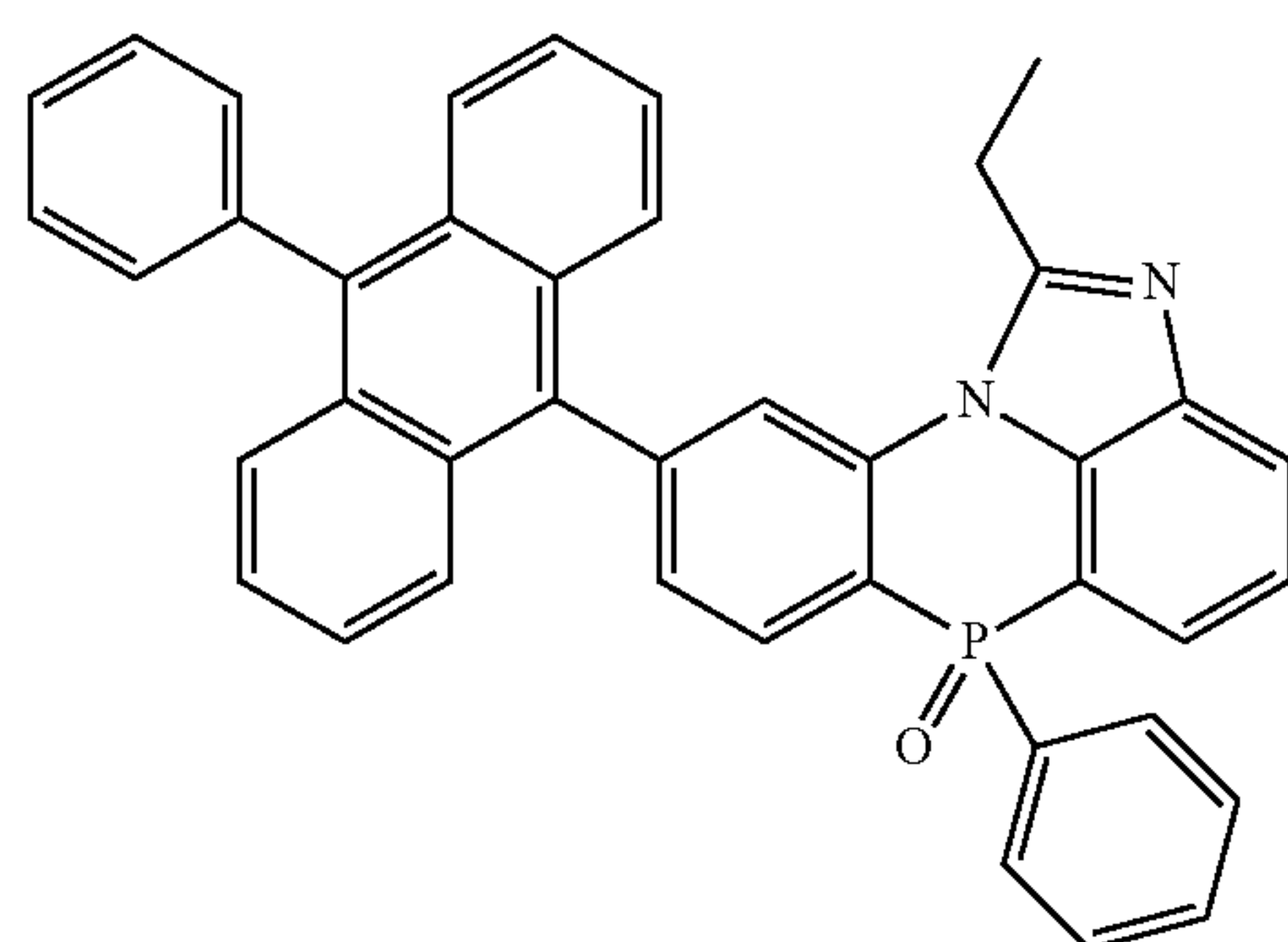
[Chemical Formula 2-7-1]
