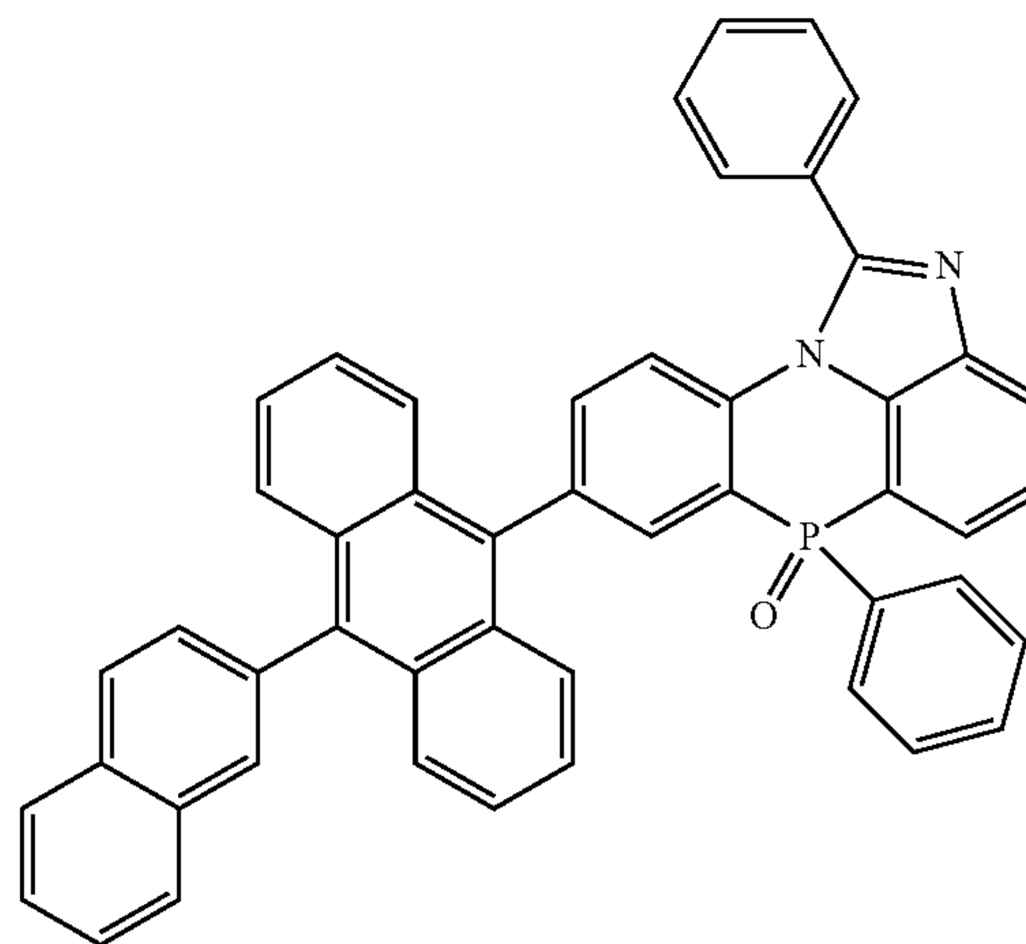
[Chemical Formula 2-4-2]
