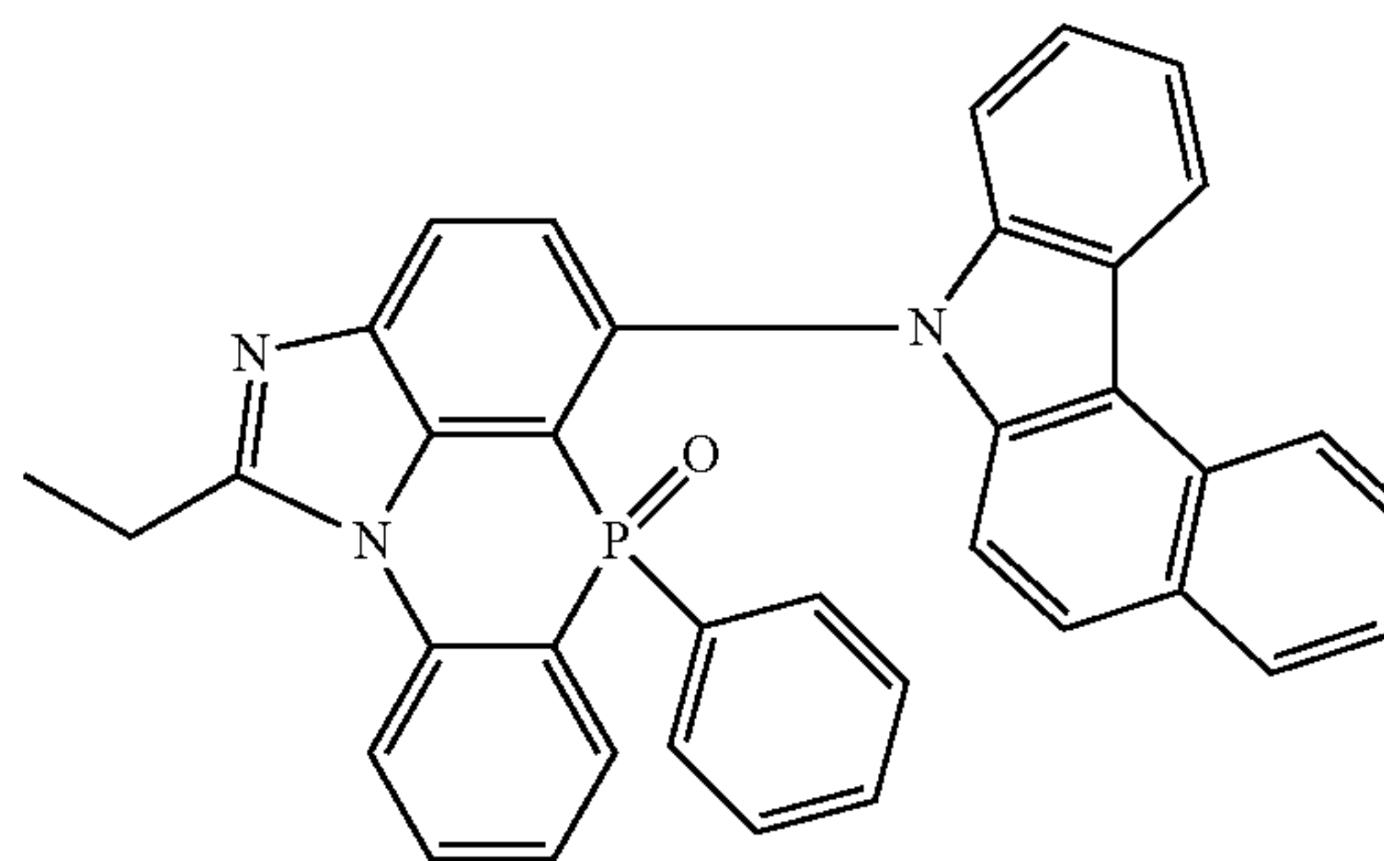
[Chemical Formula 2-9-16]
