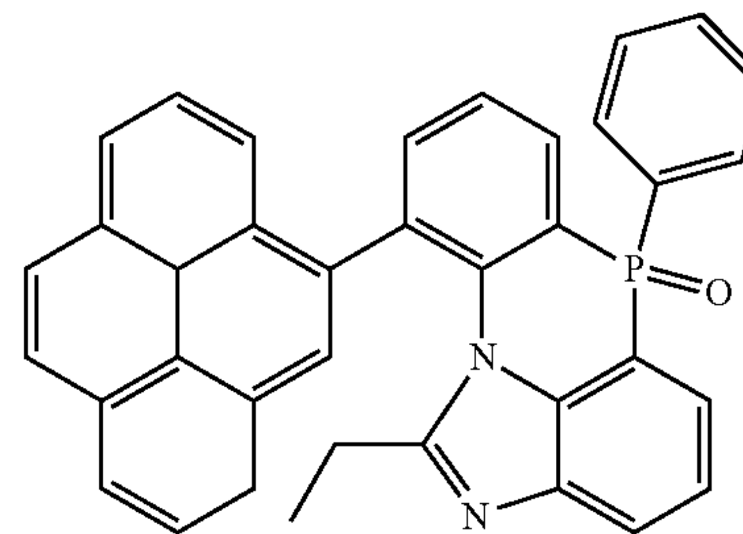
[Chemical Formula 2-8-28]
