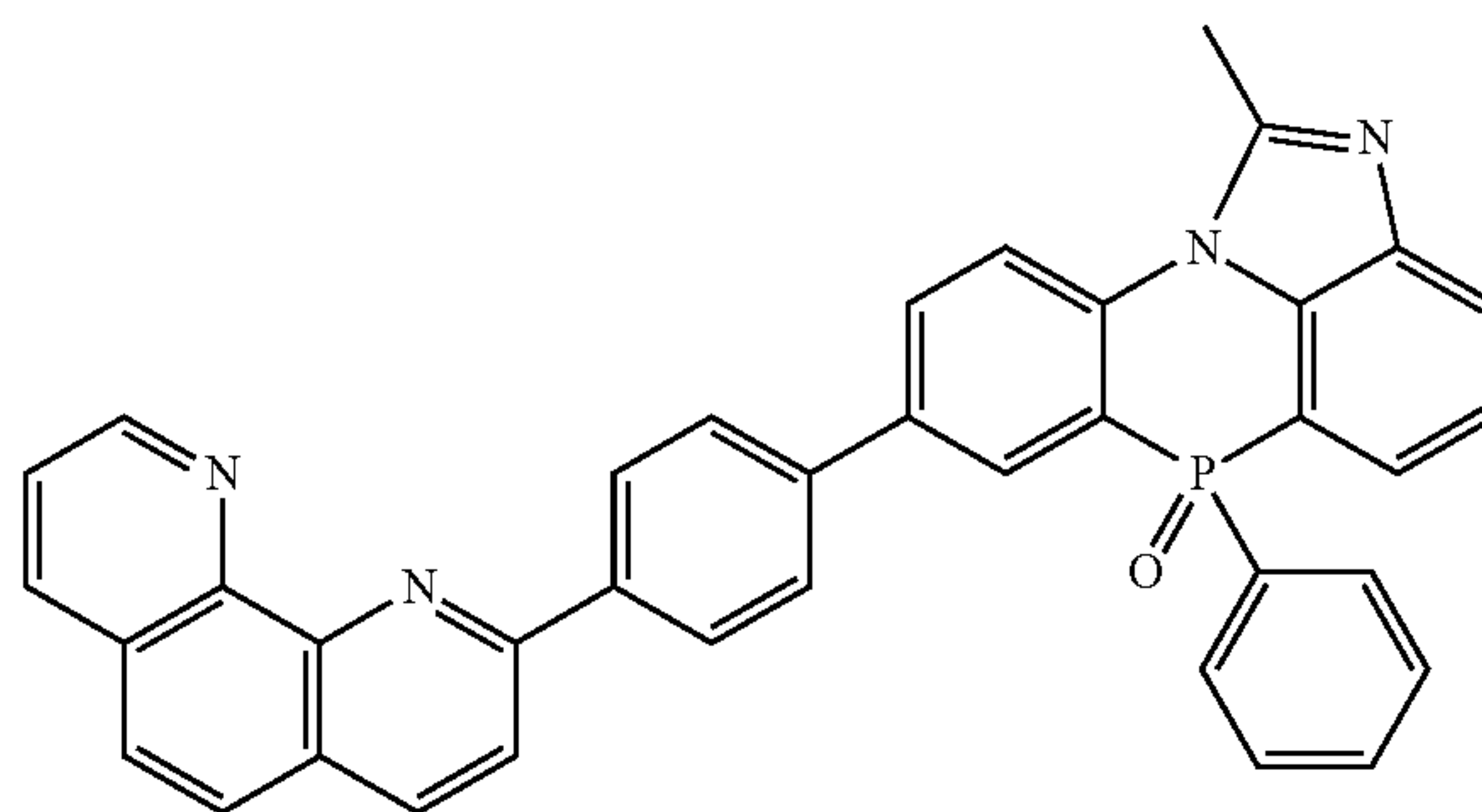
[Chemical Formula 2-2-47]
