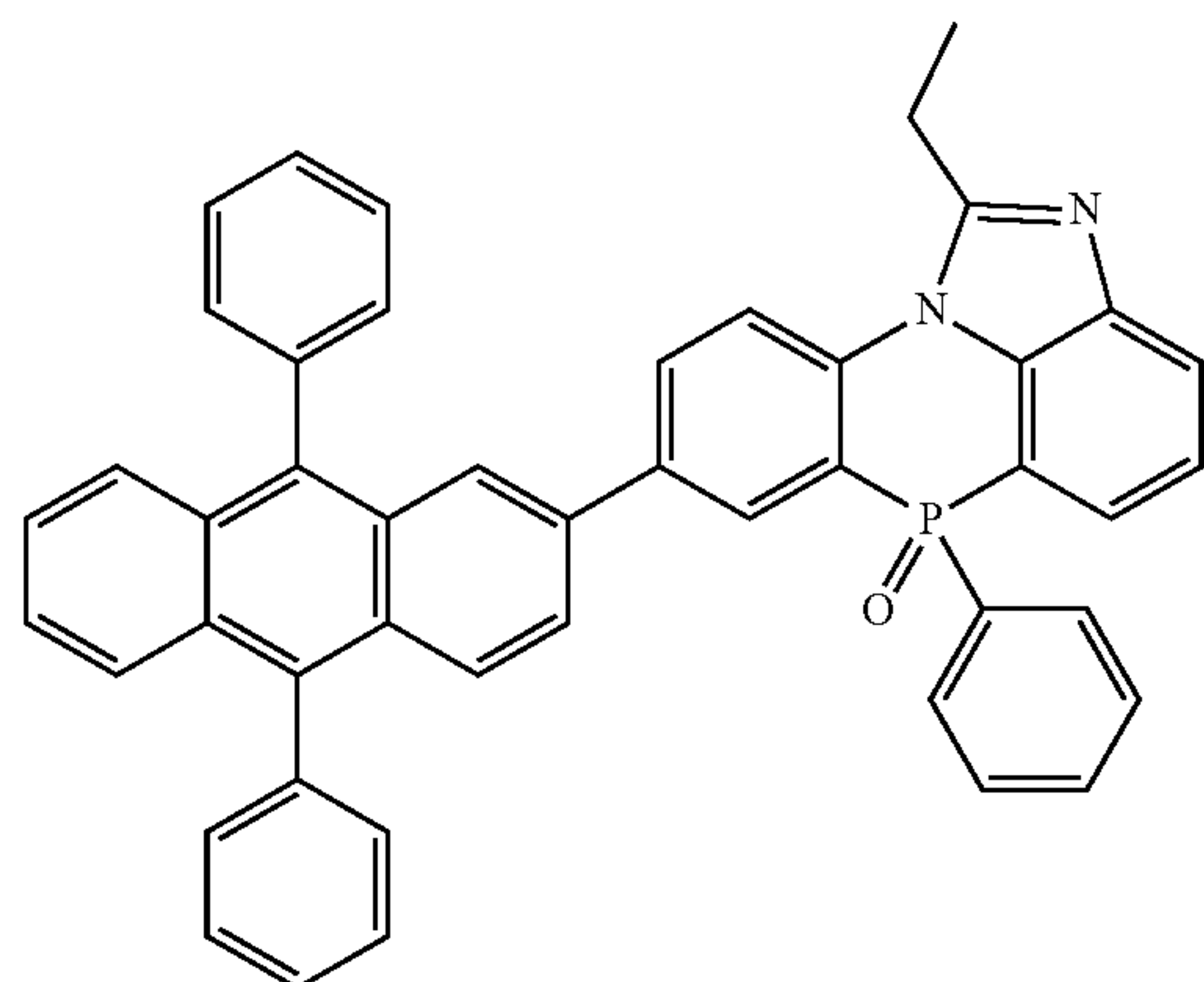
[Chemical Formula 2-3-19]
