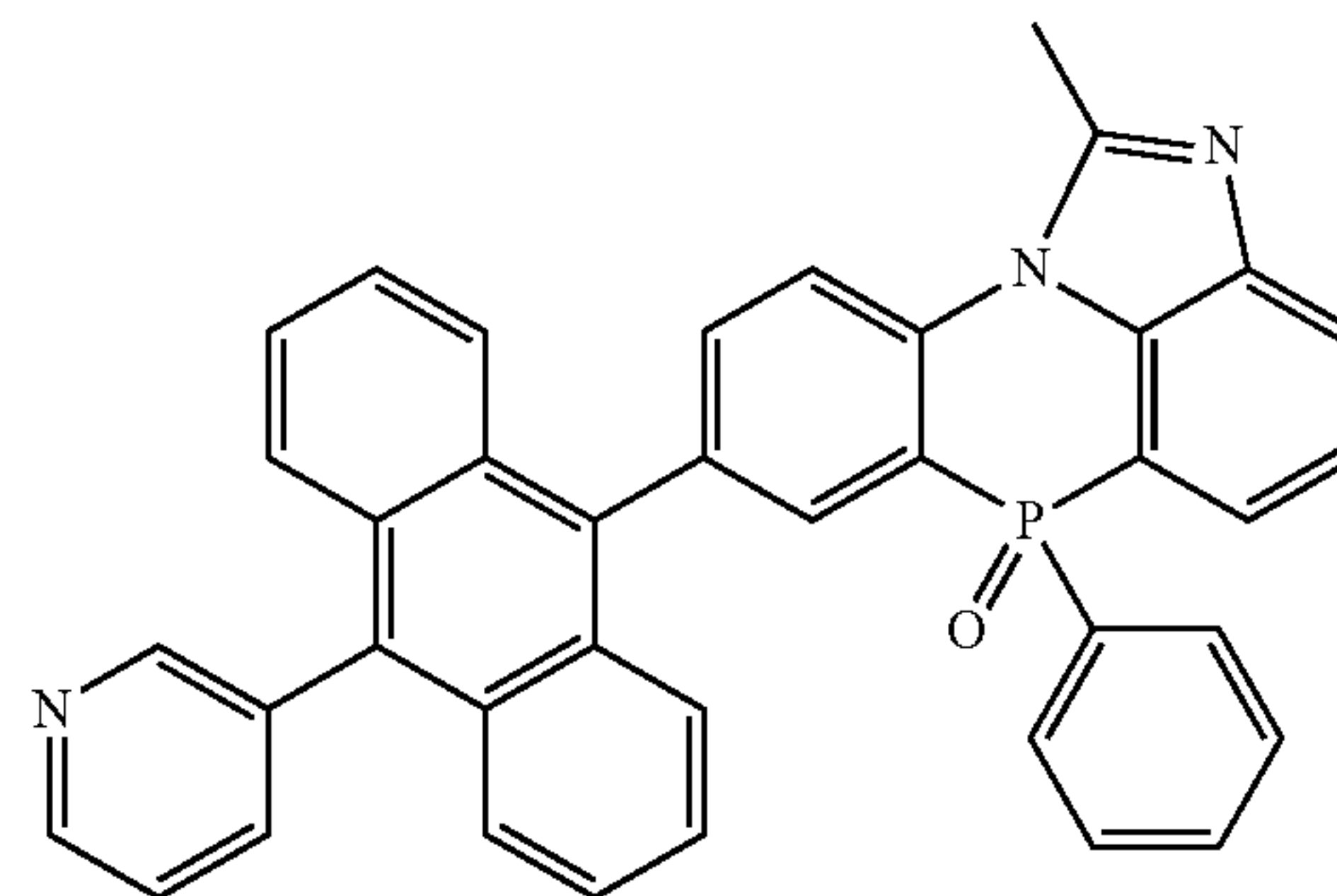
[Chemical Formula 2-2-10]
