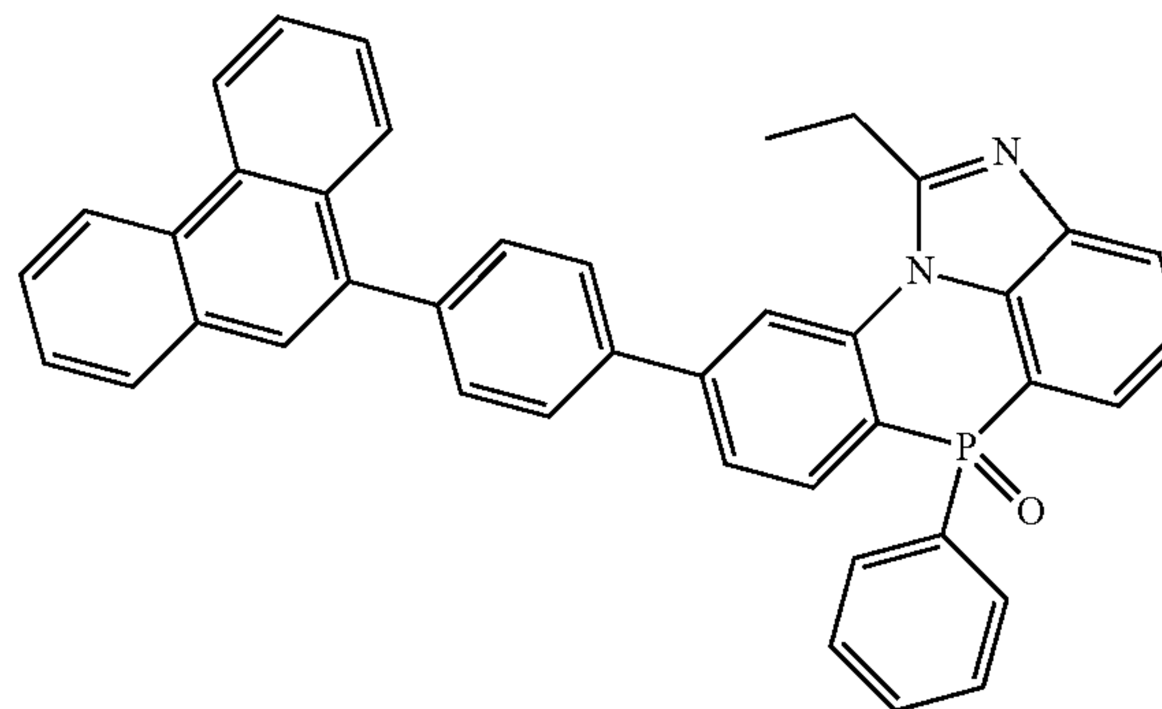
[Chemical Formula 2-7-32]
