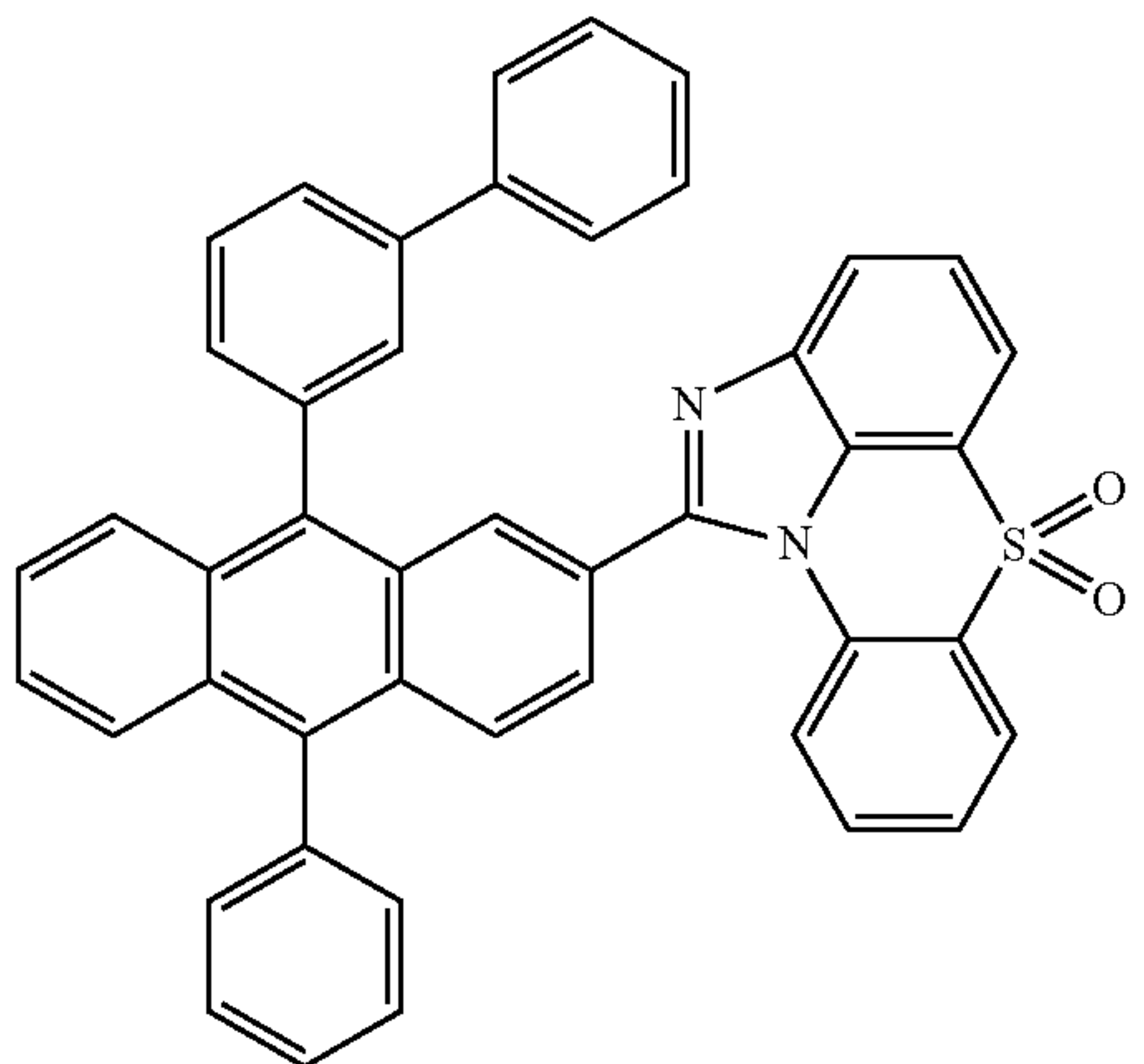
[Chemical Formula 1-5-24]
