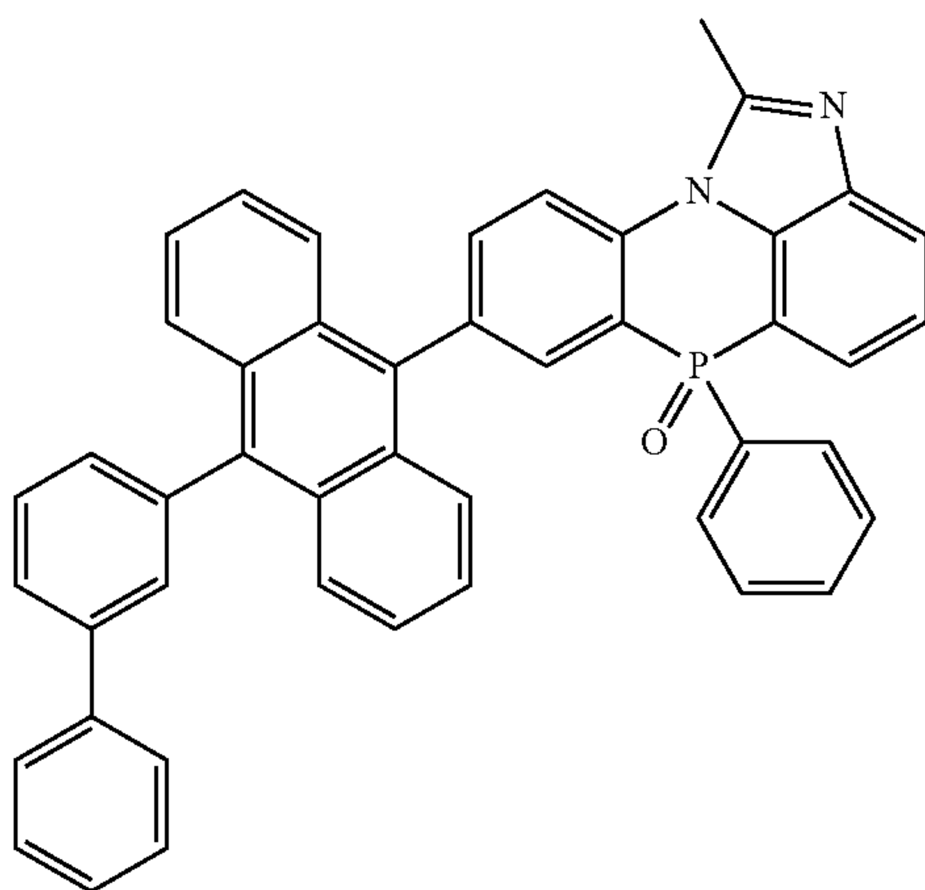
[Chemical Formula 2-2-6]
