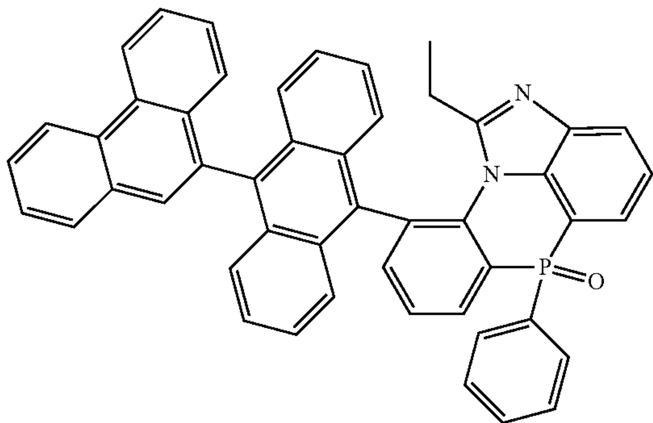
[Chemical Formula 2-8-7]
