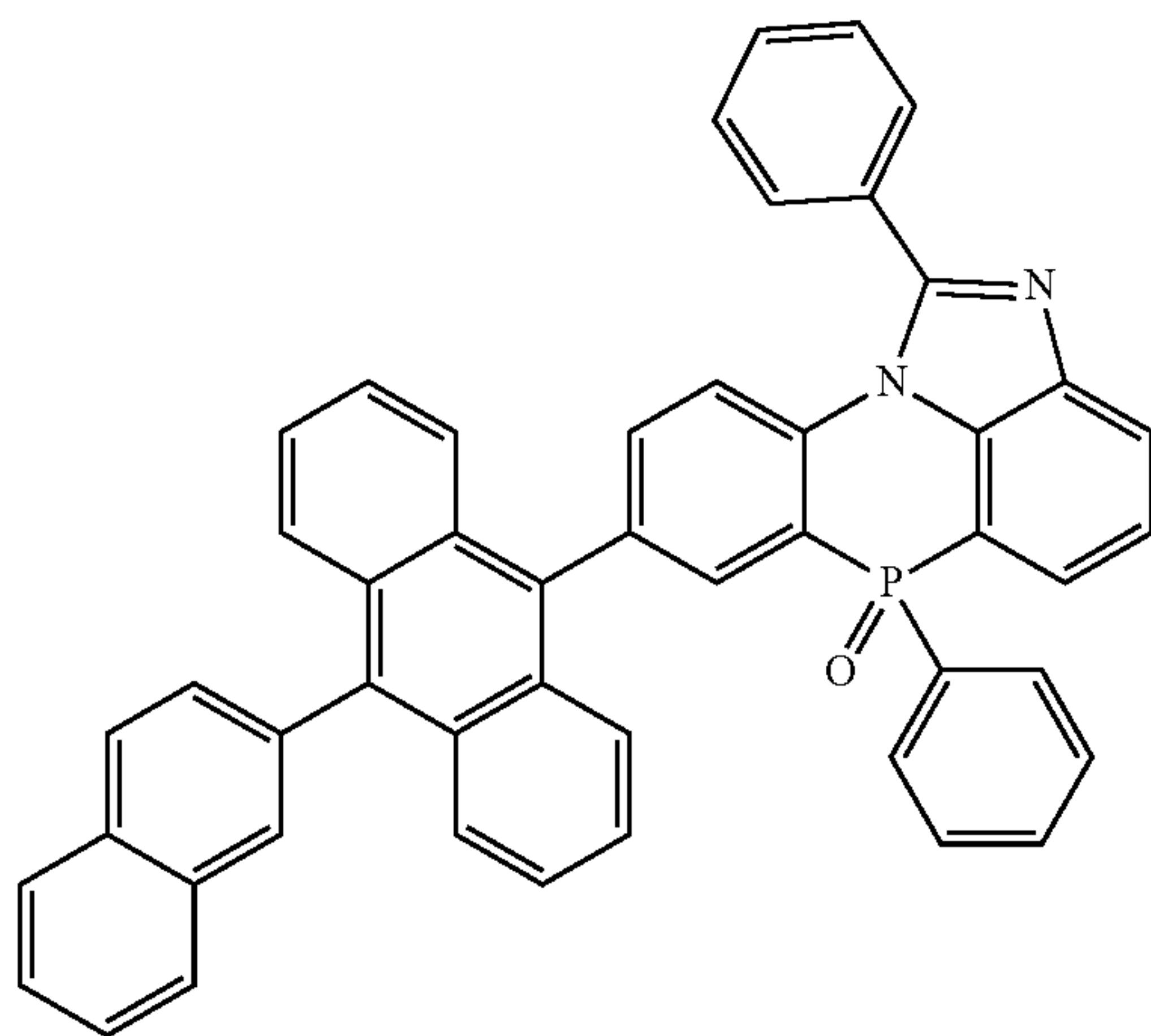
[Chemical Formula 2-4-2]
