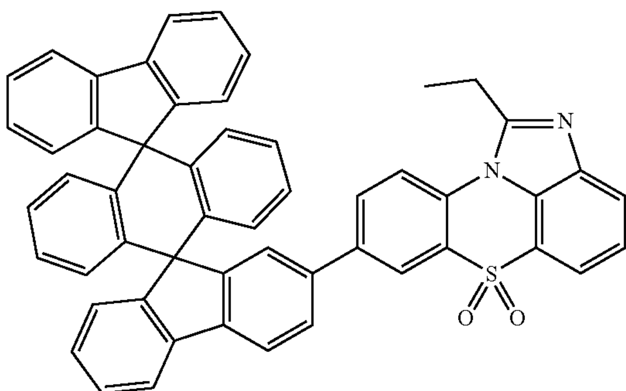
[Chemical Formula 1-3-37]
