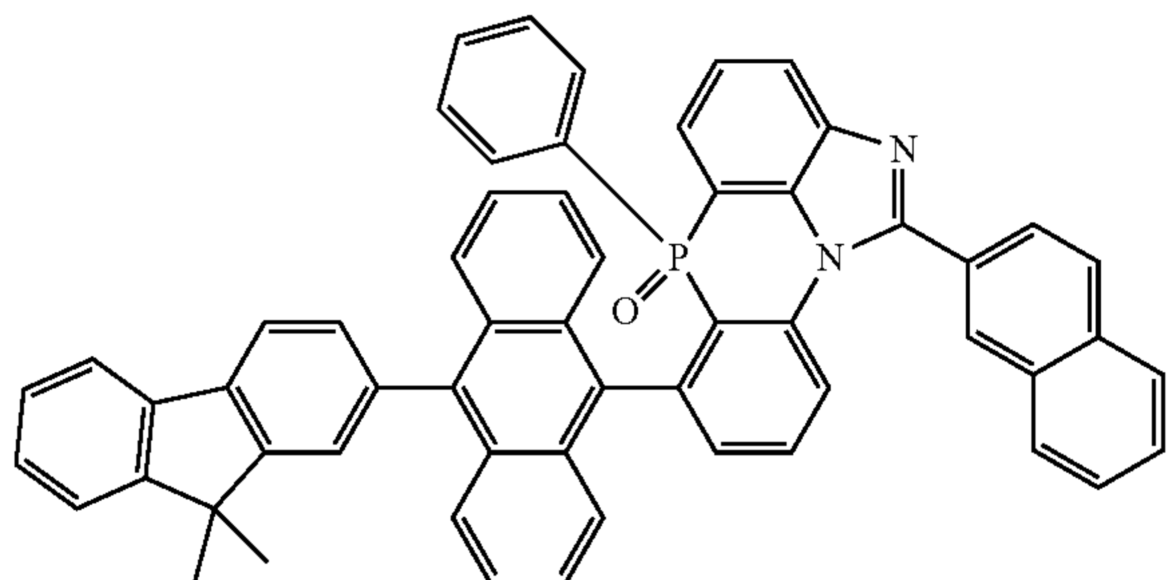
[Chemical Formula 2-6-6]
