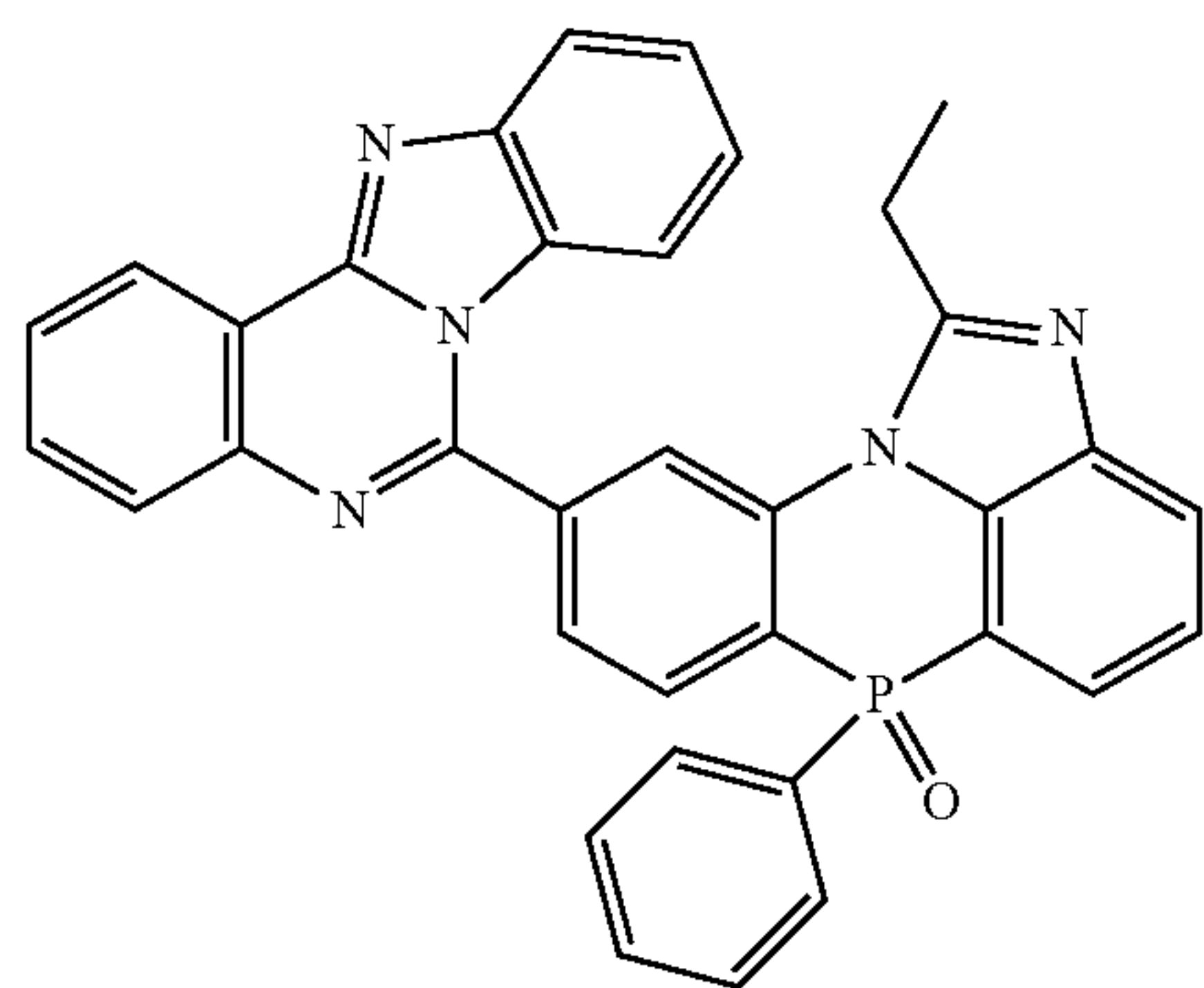
[Chemical Formula 2-7-53]
