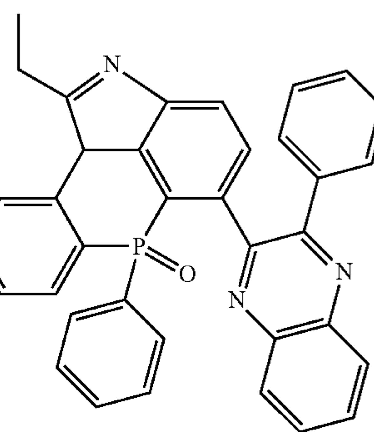
[Chemical Formula 2-9-14]
