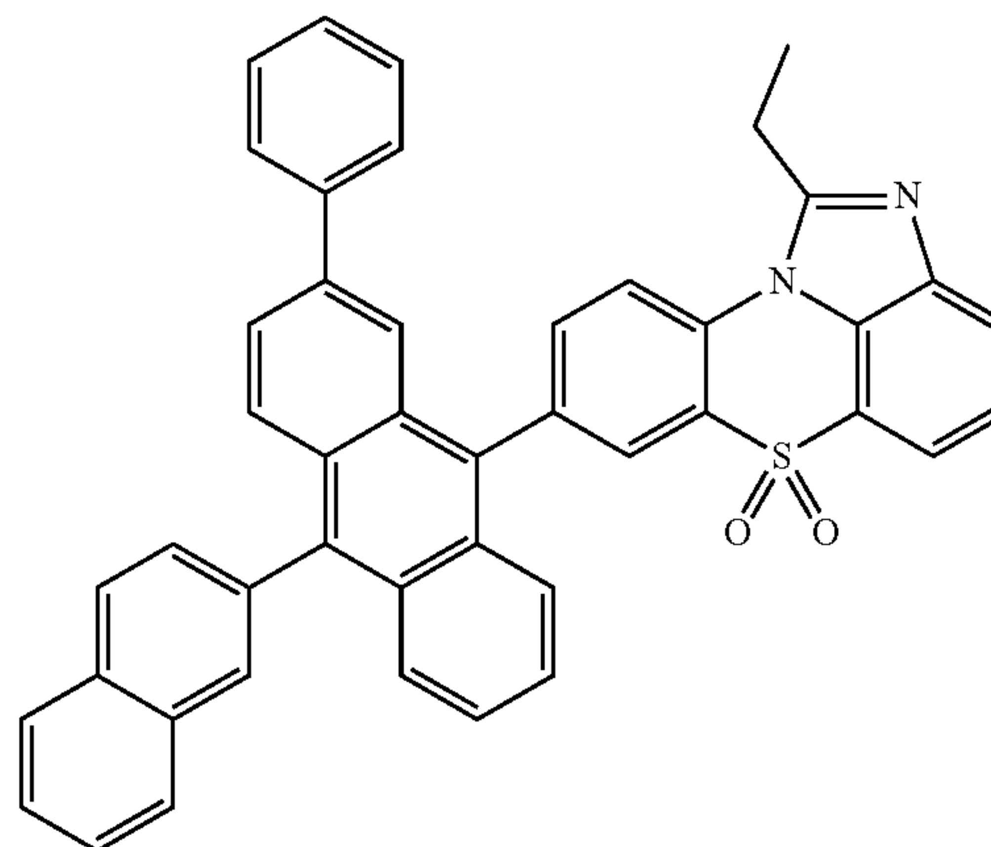
[Chemical Formula 1-3-16]
