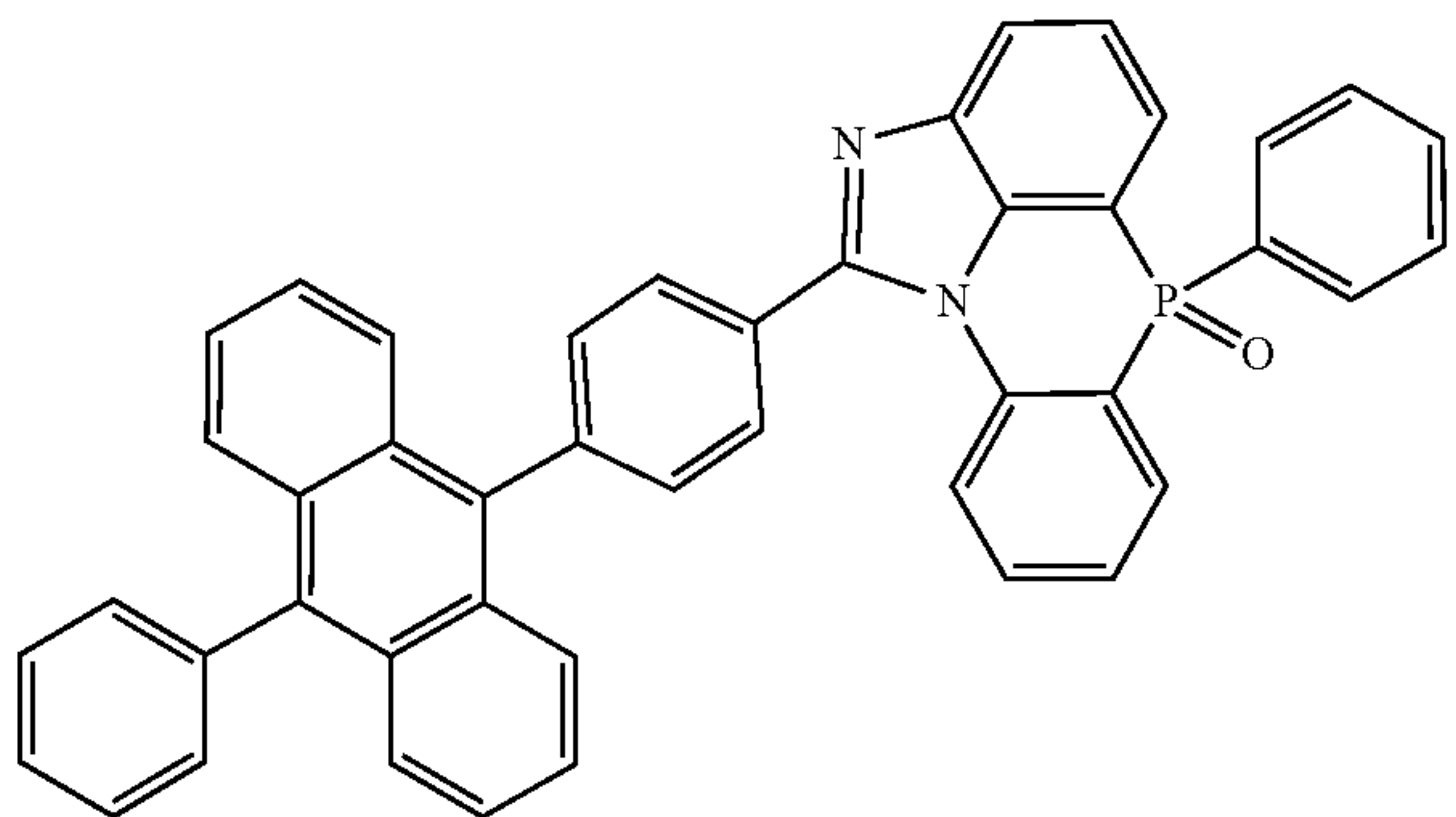
[Chemical Formula 2-5-17]
