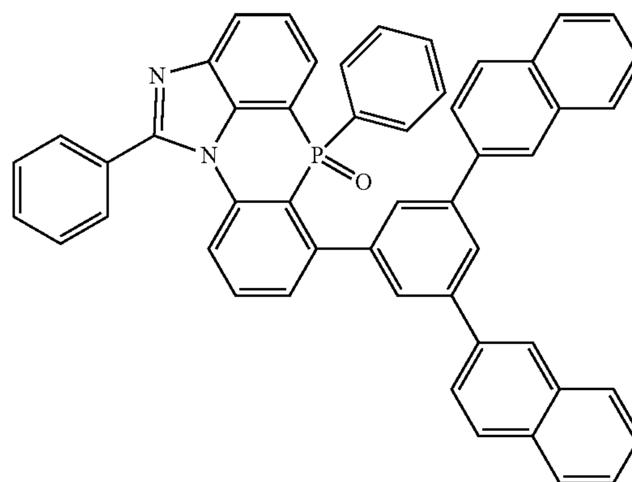
[Chemical Formula 2-6-43]
