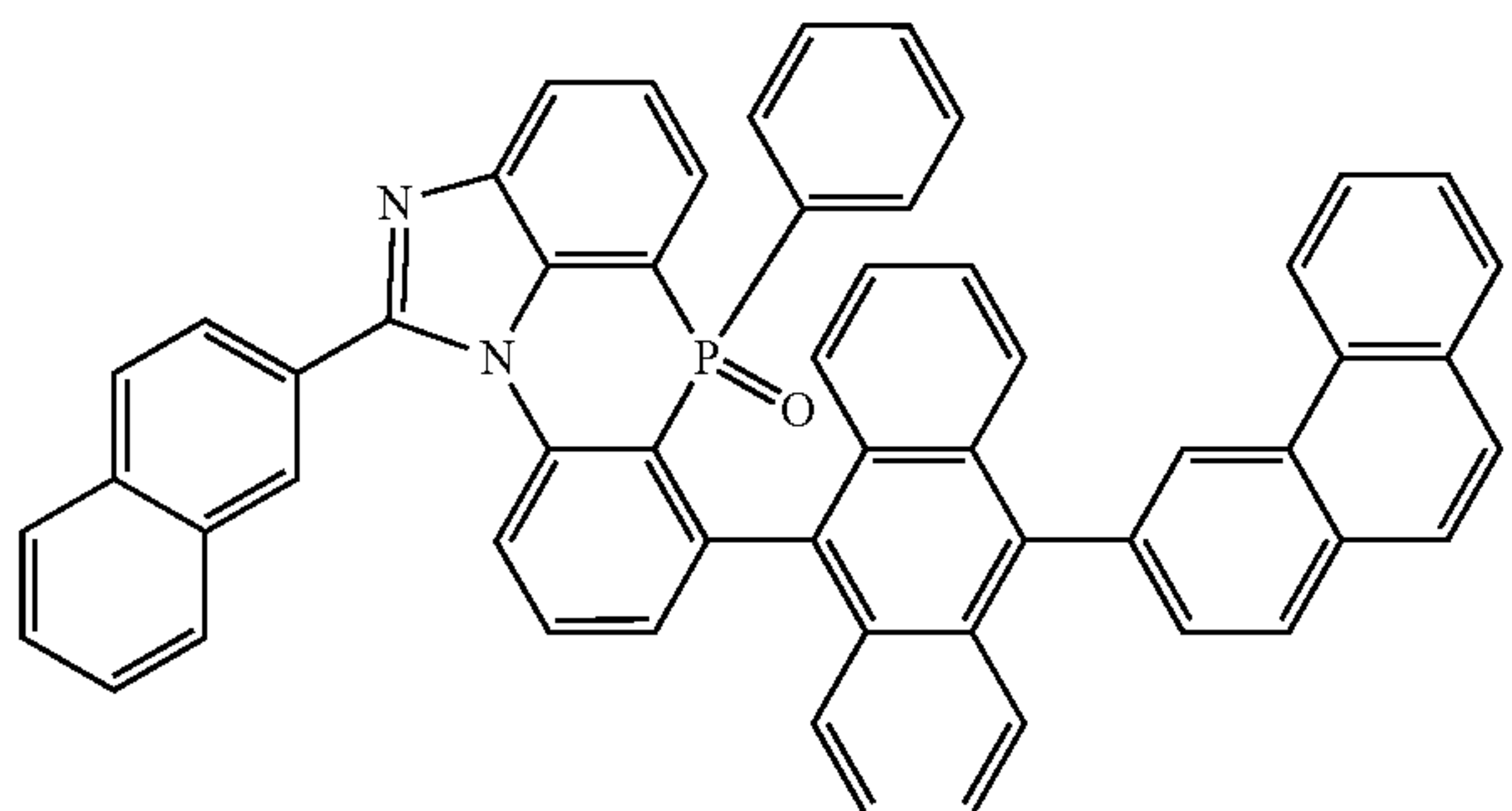
[Chemical Formula 2-6-9]
