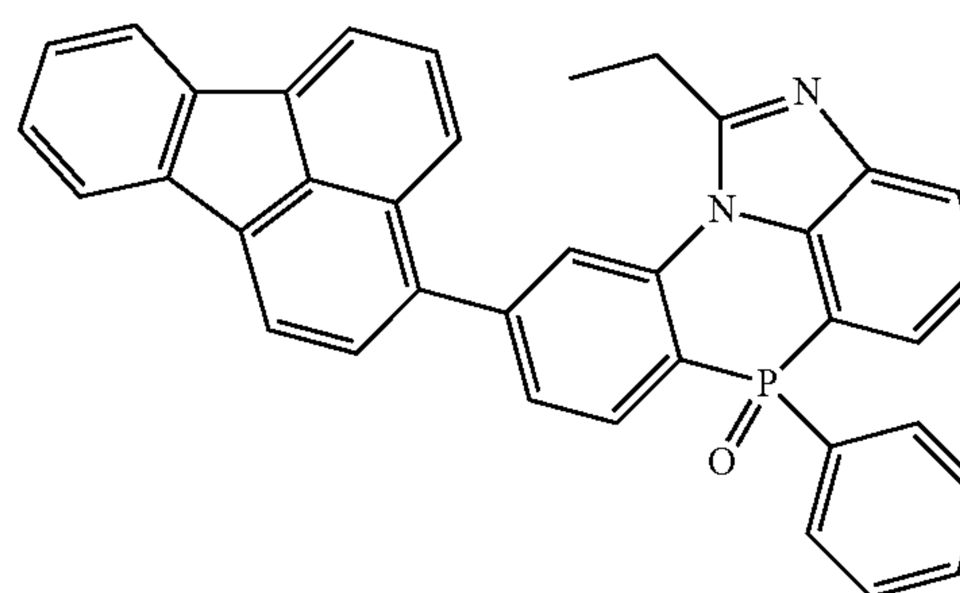
[Chemical Formula 2-7-30]
