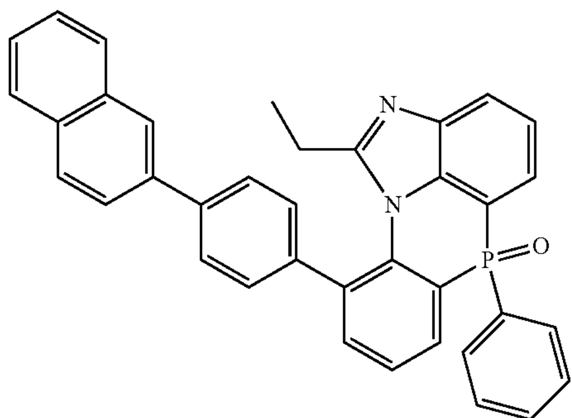
[Chemical Formula 2-8-26]
