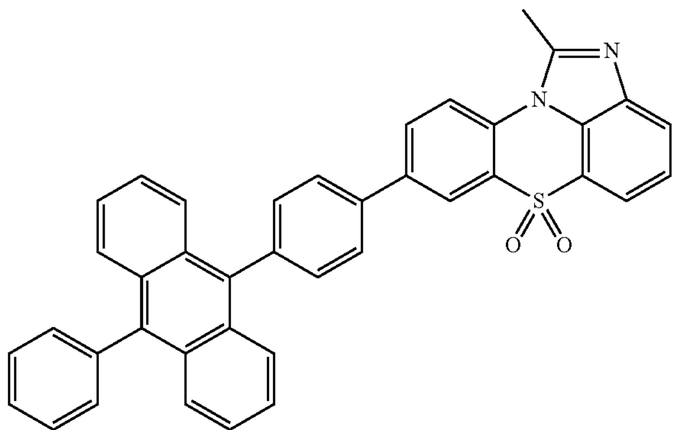
[Chemical Formula 1-2-17]
