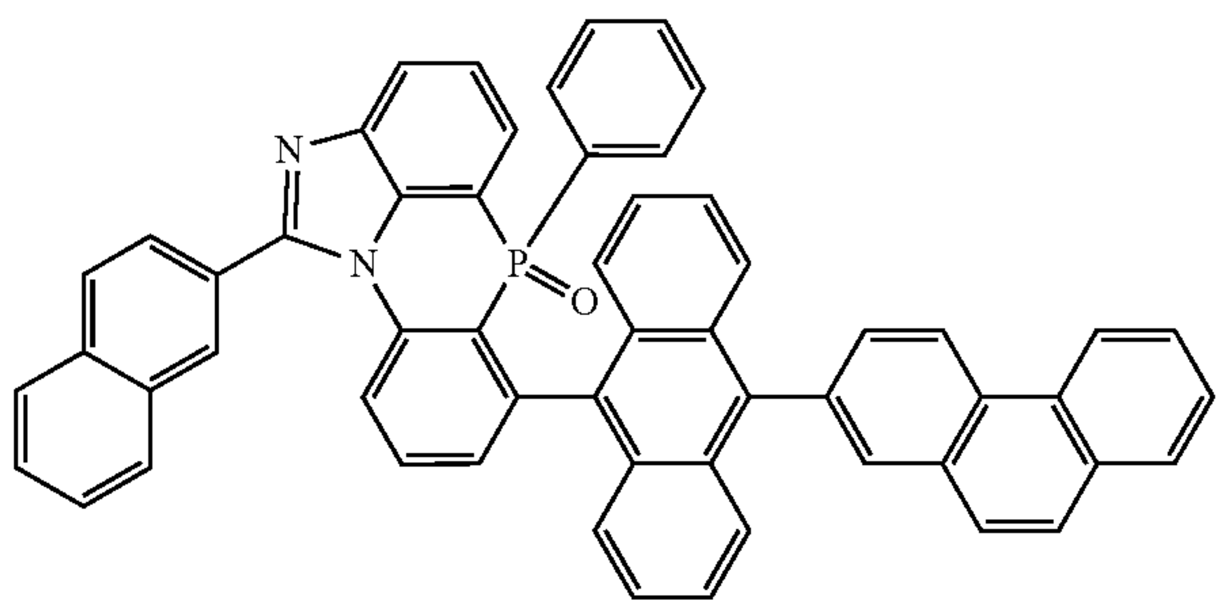
[Chemical Formula 2-6-9]
