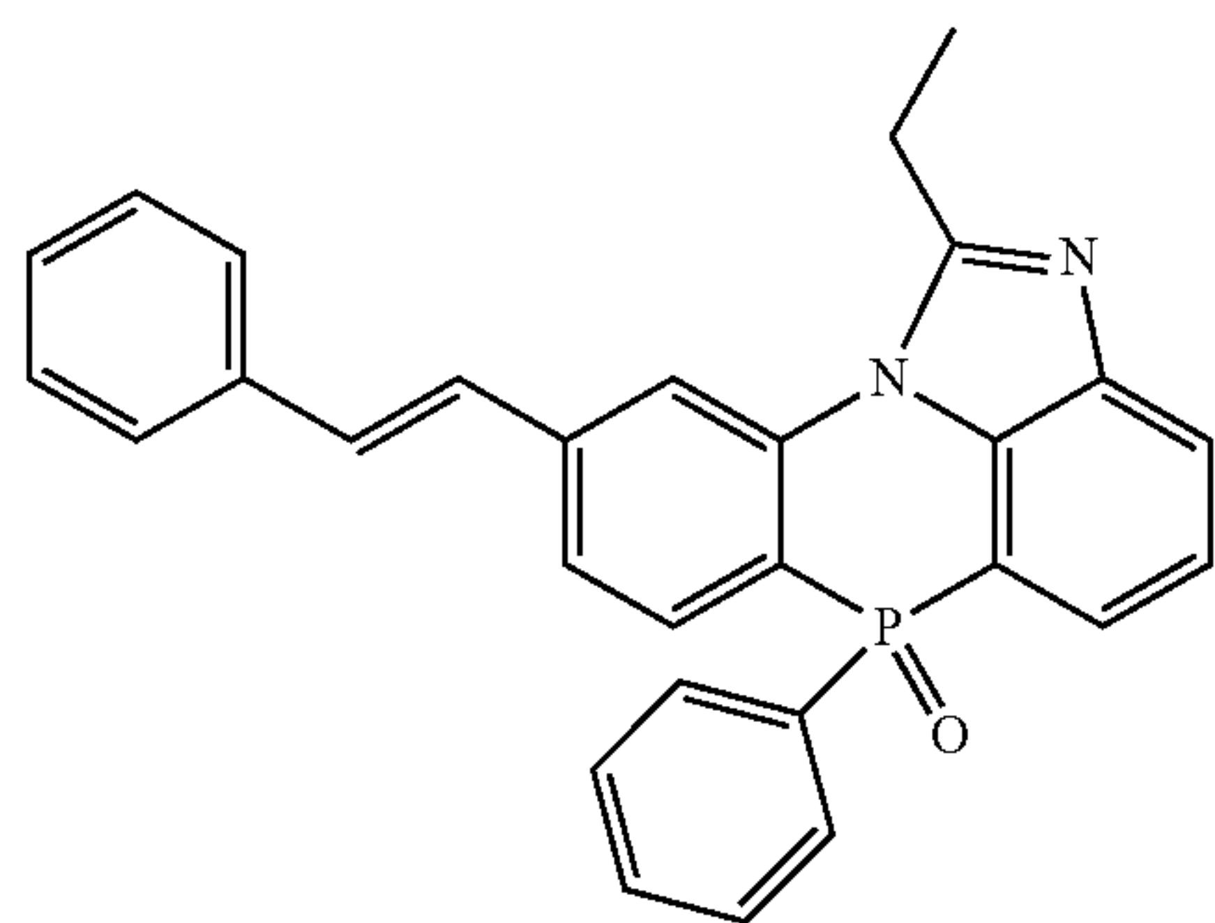
[Chemical Formula 2-8-1]
