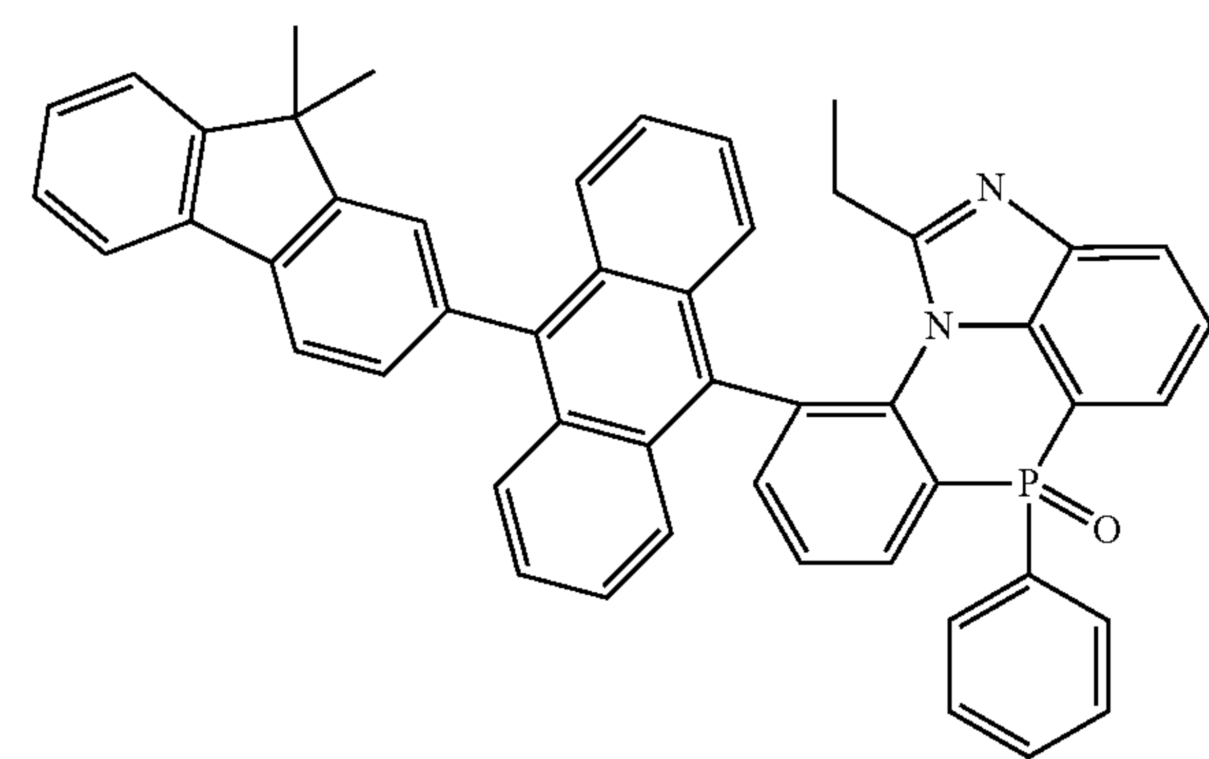
[Chemical Formula 2-8-5]
