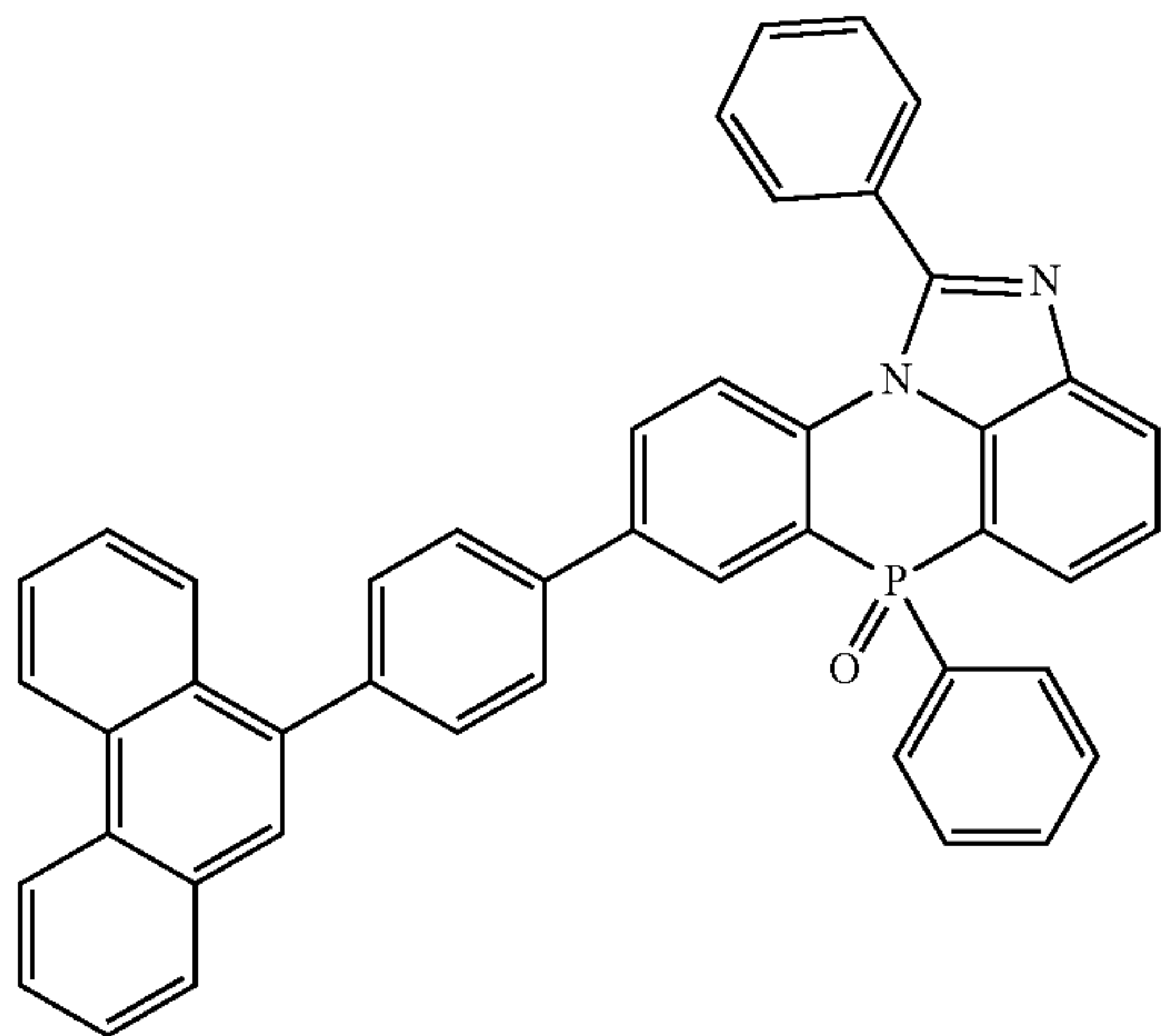
[Chemical Formula 2-4-33]
