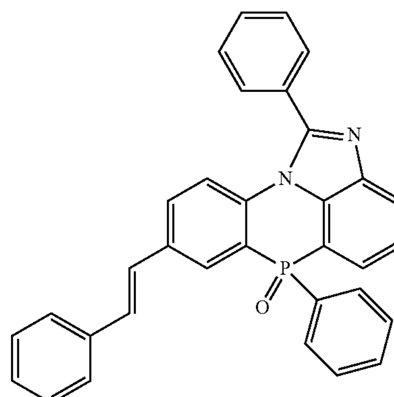
[Chemical Formula 2-4-54]
