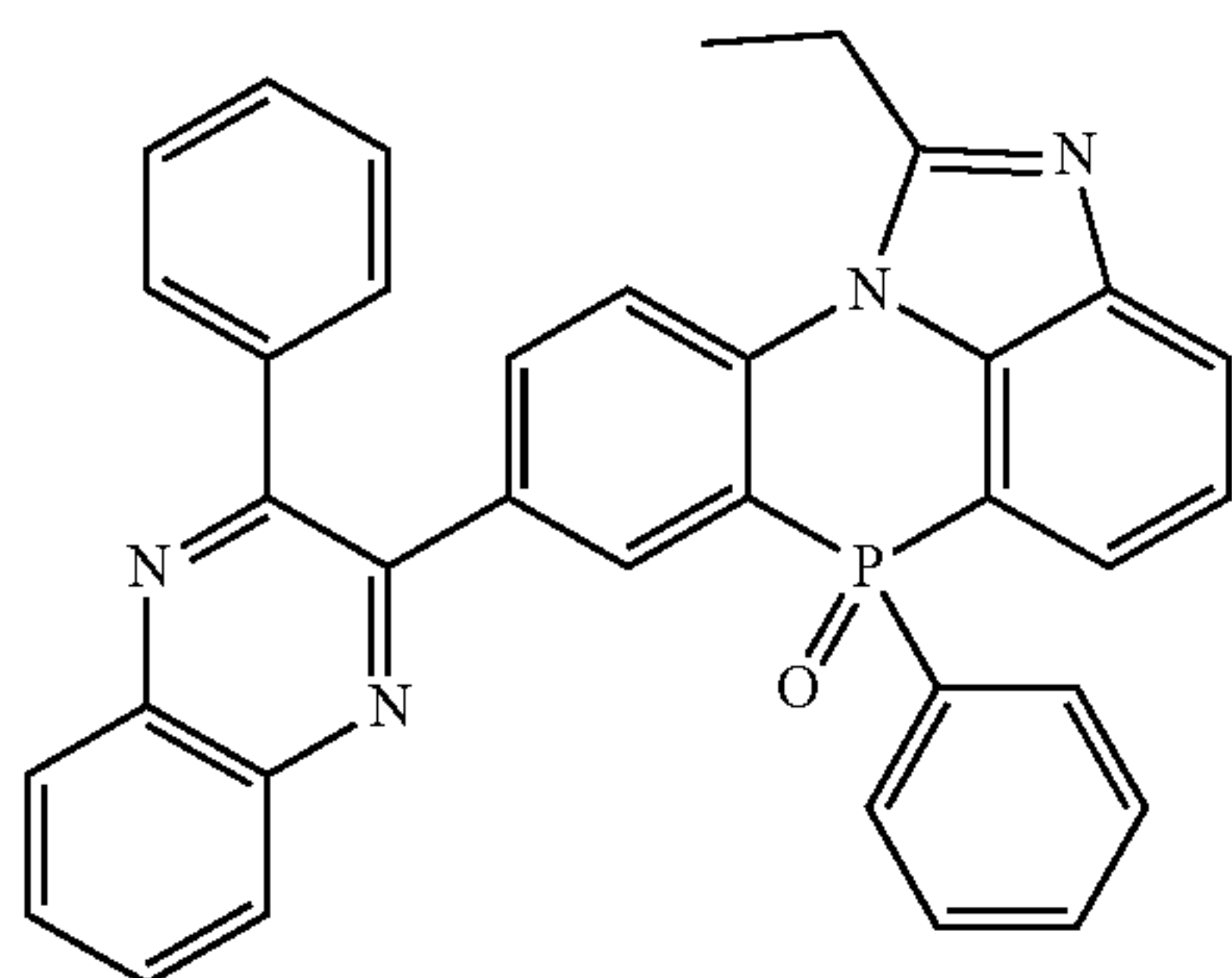
[Chemical Formula 2-3-49]
