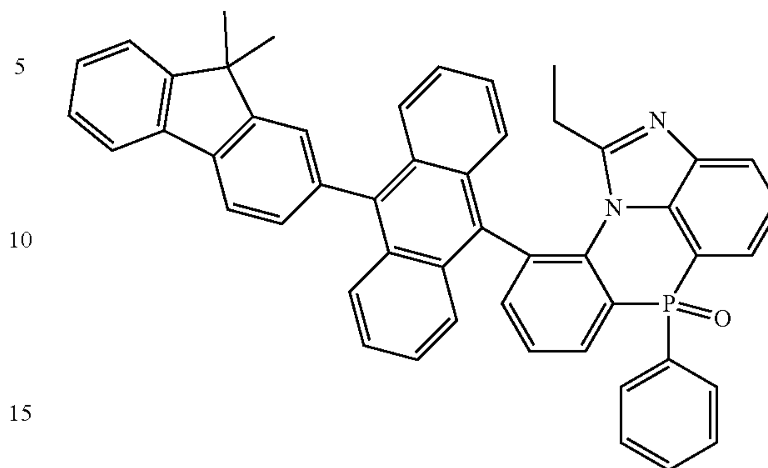
[Chemical Formula 2-8-5]
