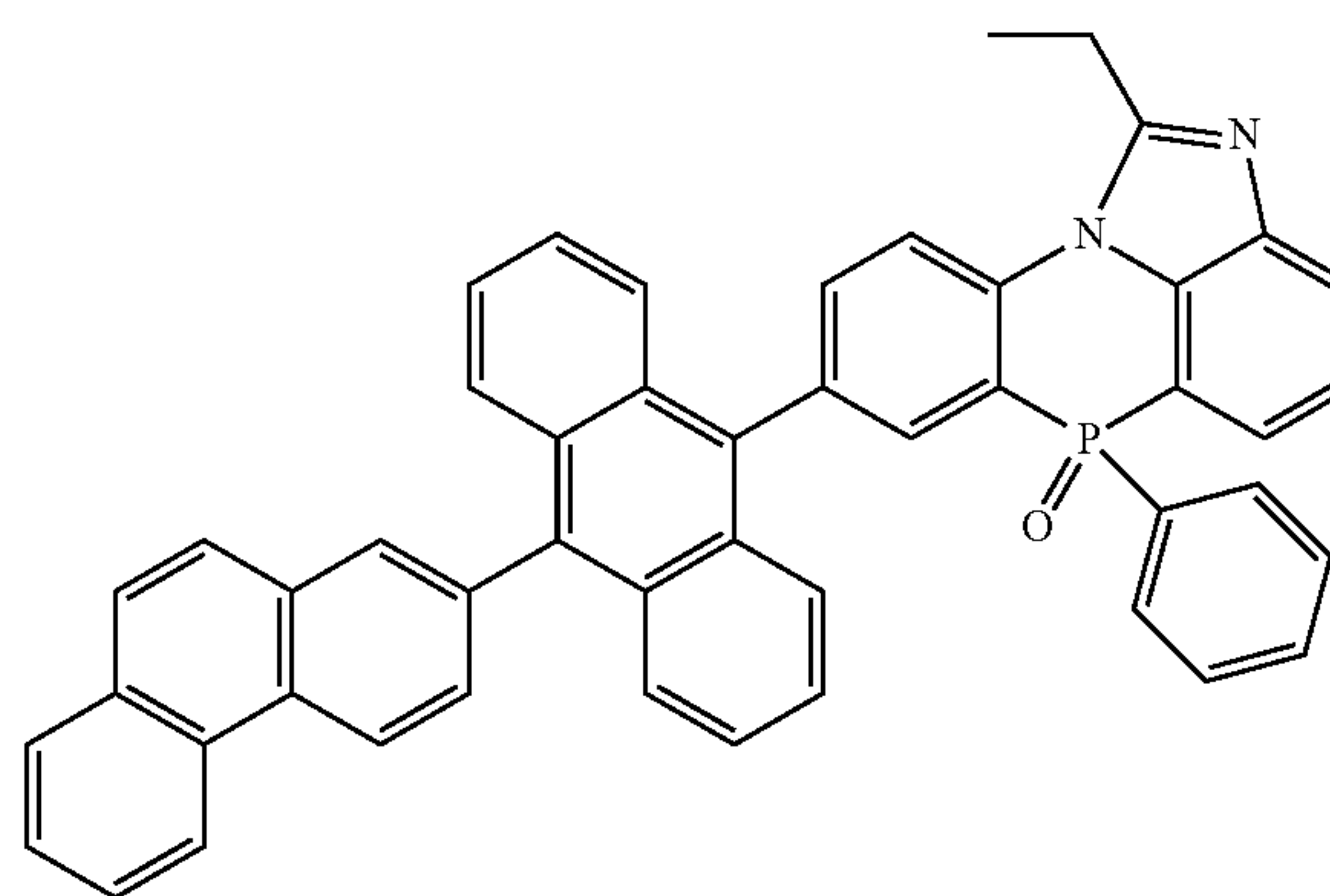
[Chemical Formula 2-3-9]
