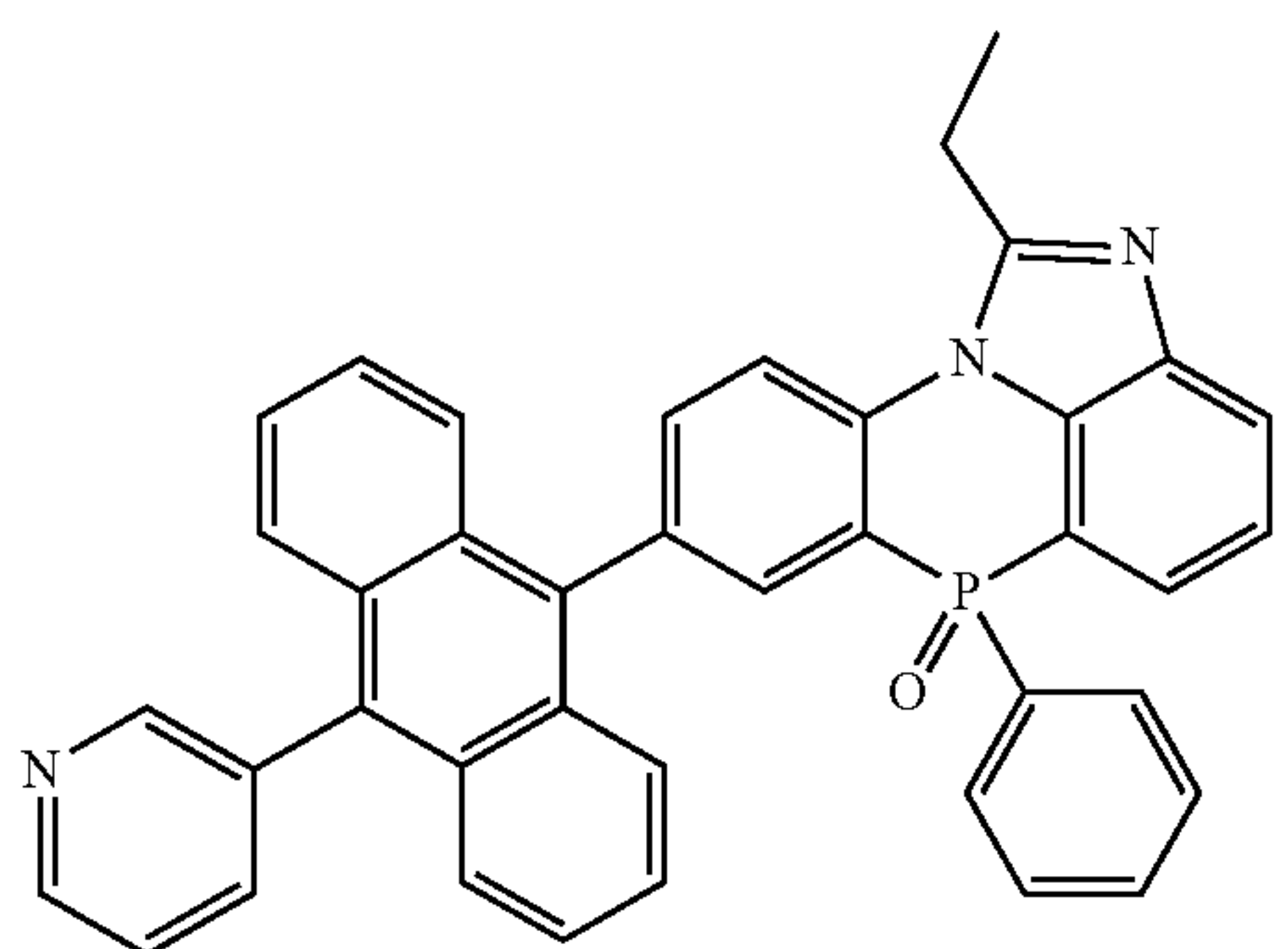
[Chemical Formula 2-3-10]
