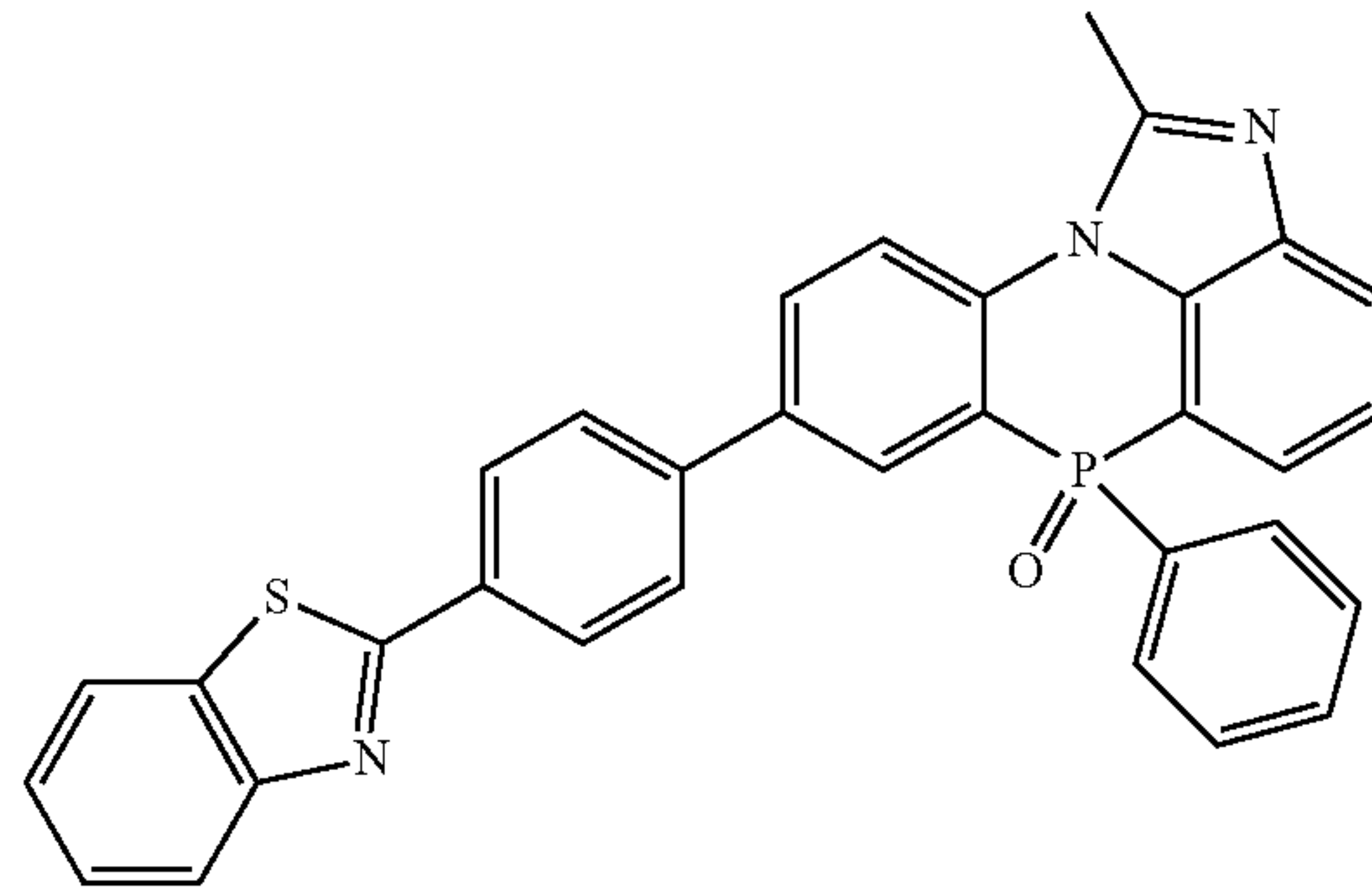
[Chemical Formula 2-2-46]
