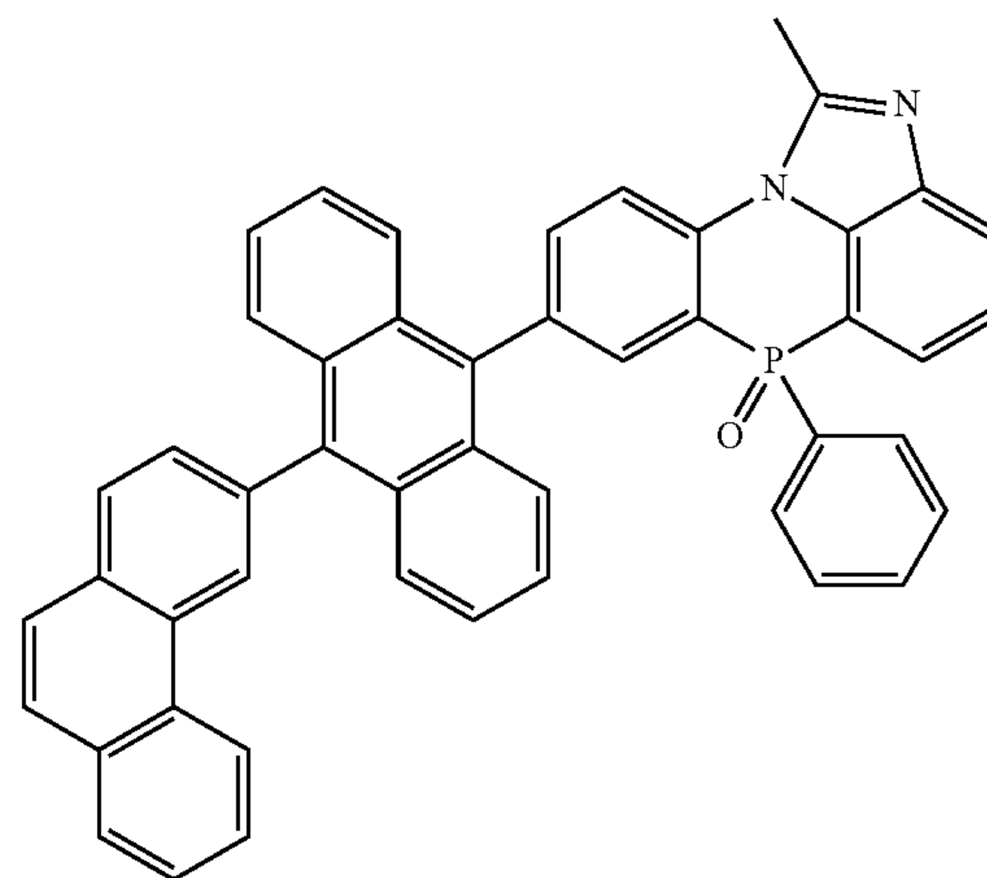
[Chemical Formula 2-2-8]
