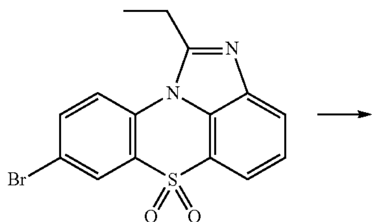
[Compound 2-B]
