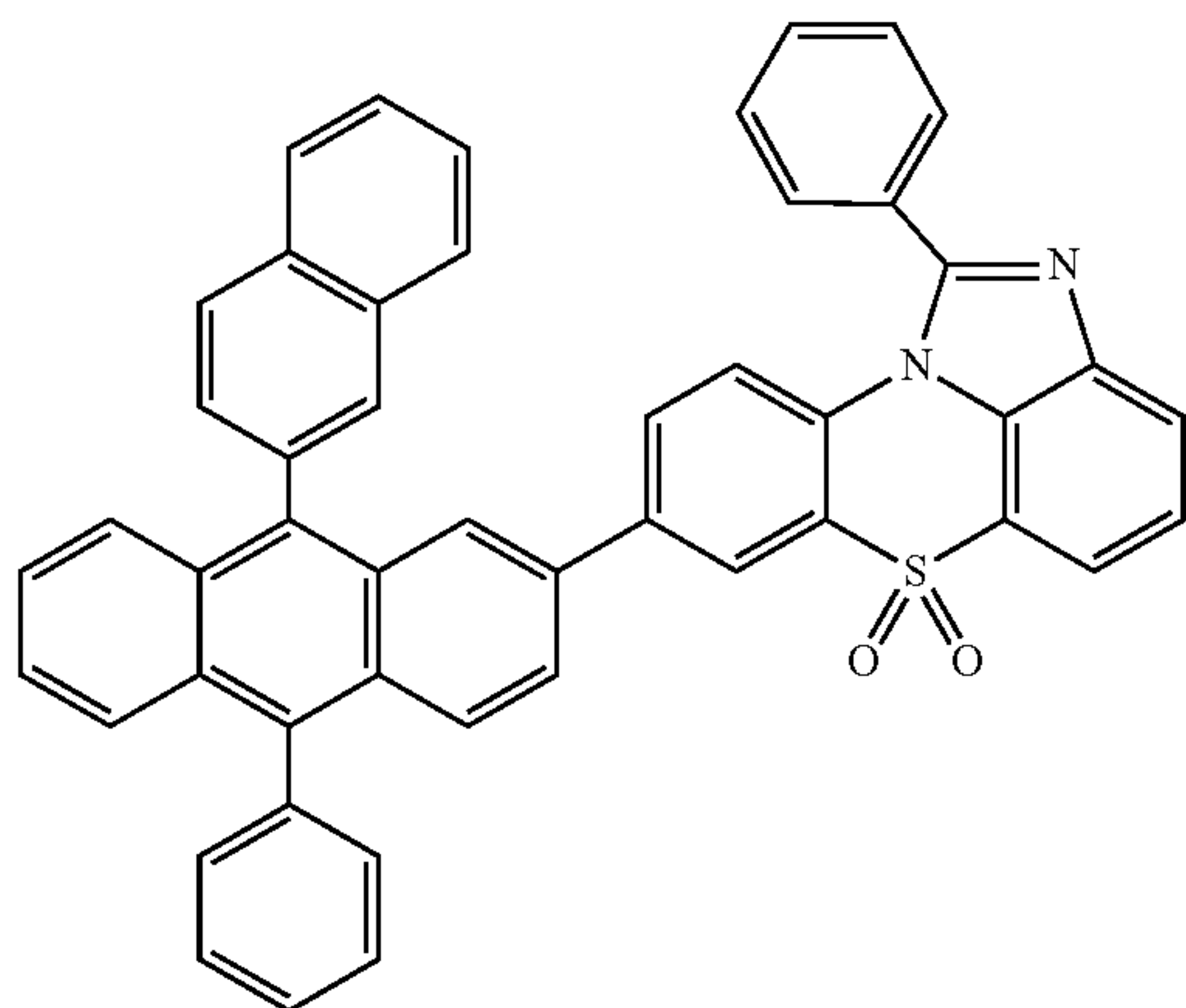
[Chemical Formula 1-4-23]
