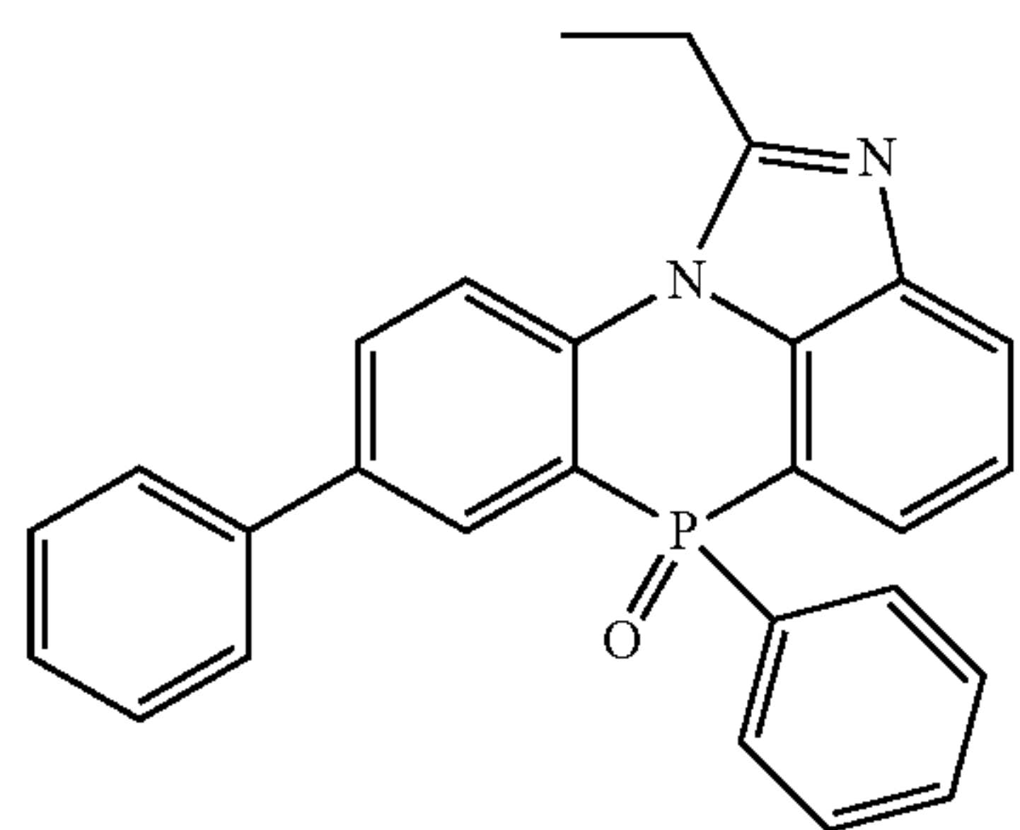
[Chemical Formula 2-3-38]
