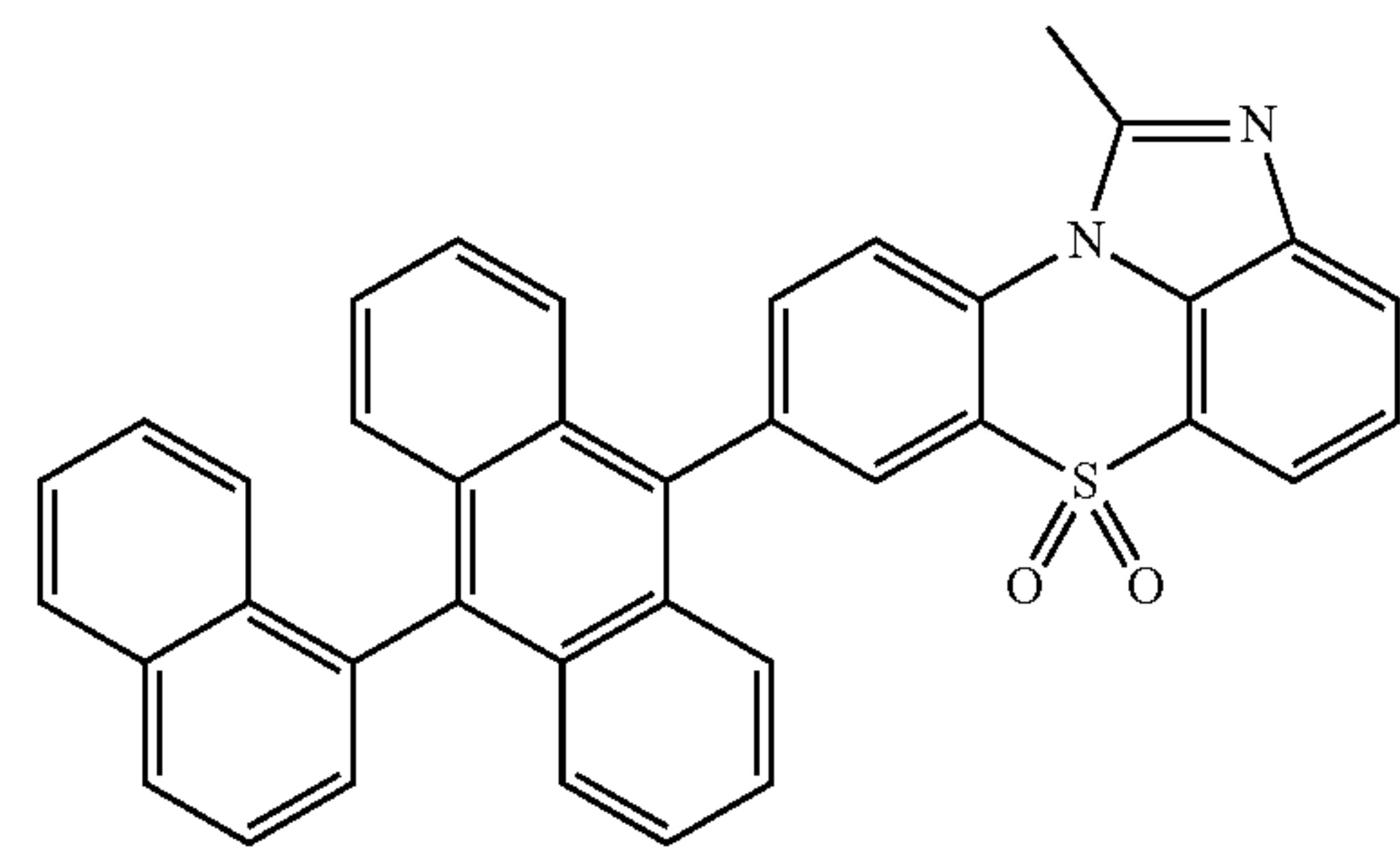
[Chemical Formula 1-2-3]
