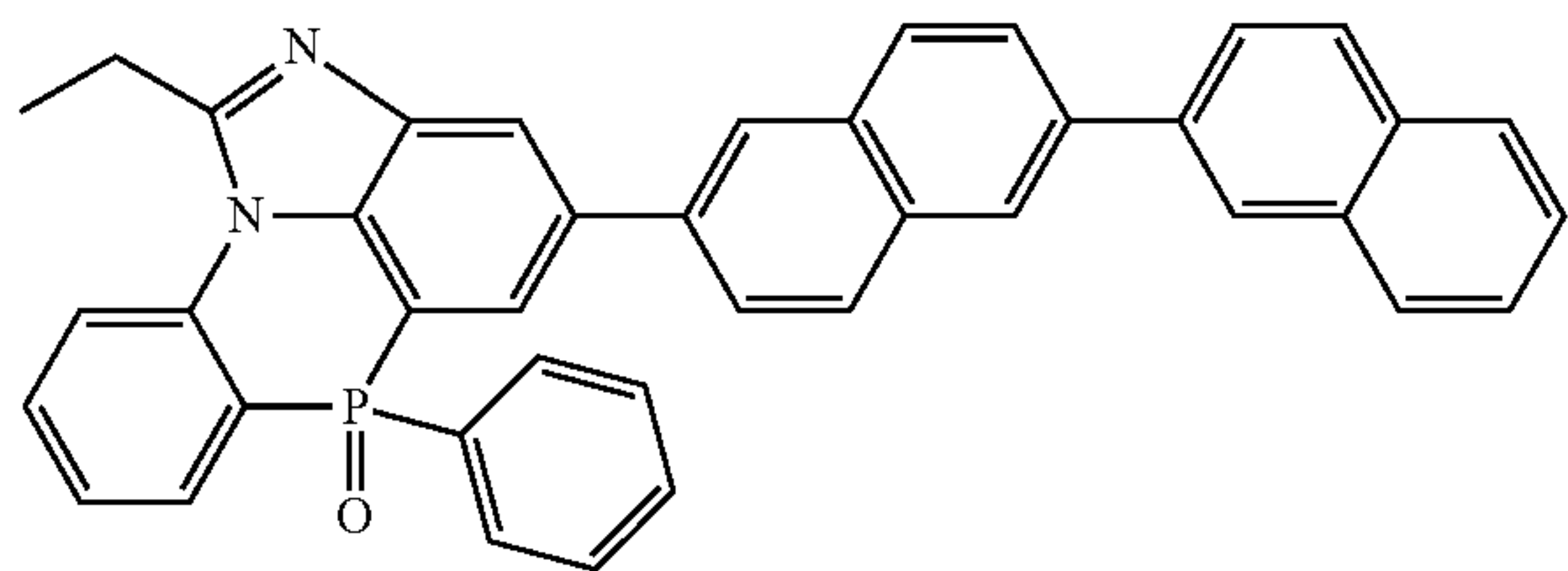
[Chemical Formula 2-10-8]
