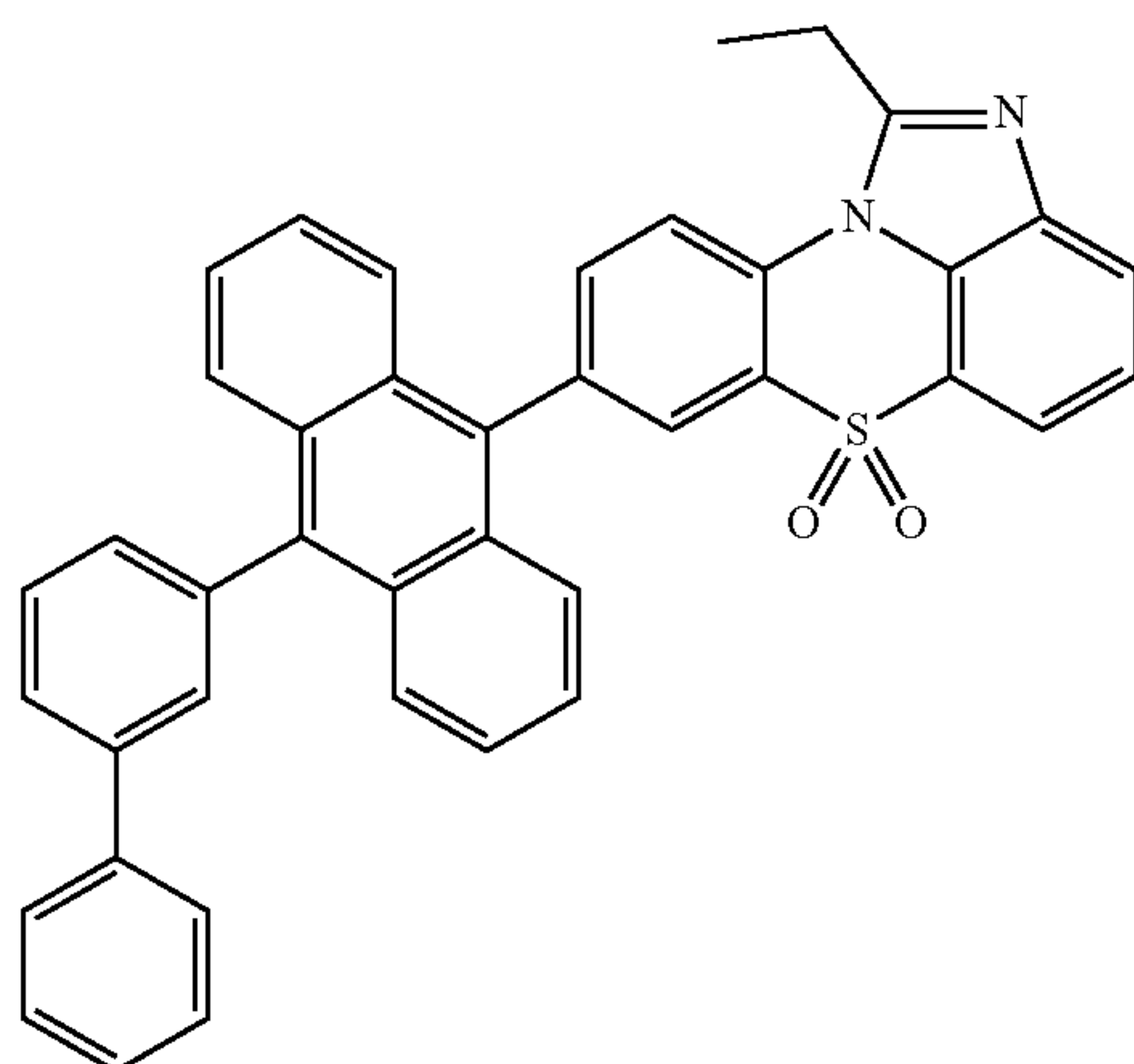
[Chemical Formula 1-3-7]
