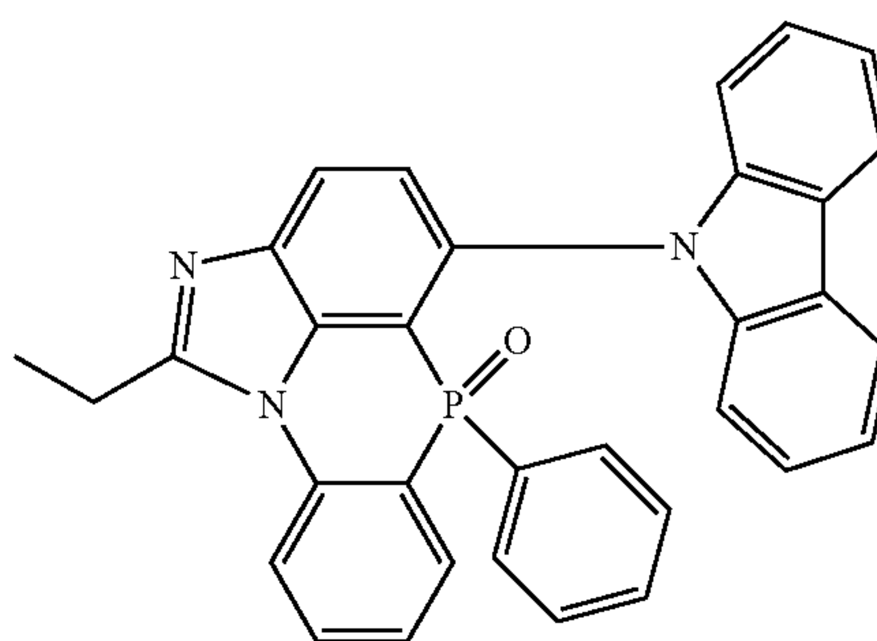
[Chemical Formula 2-9-15]
