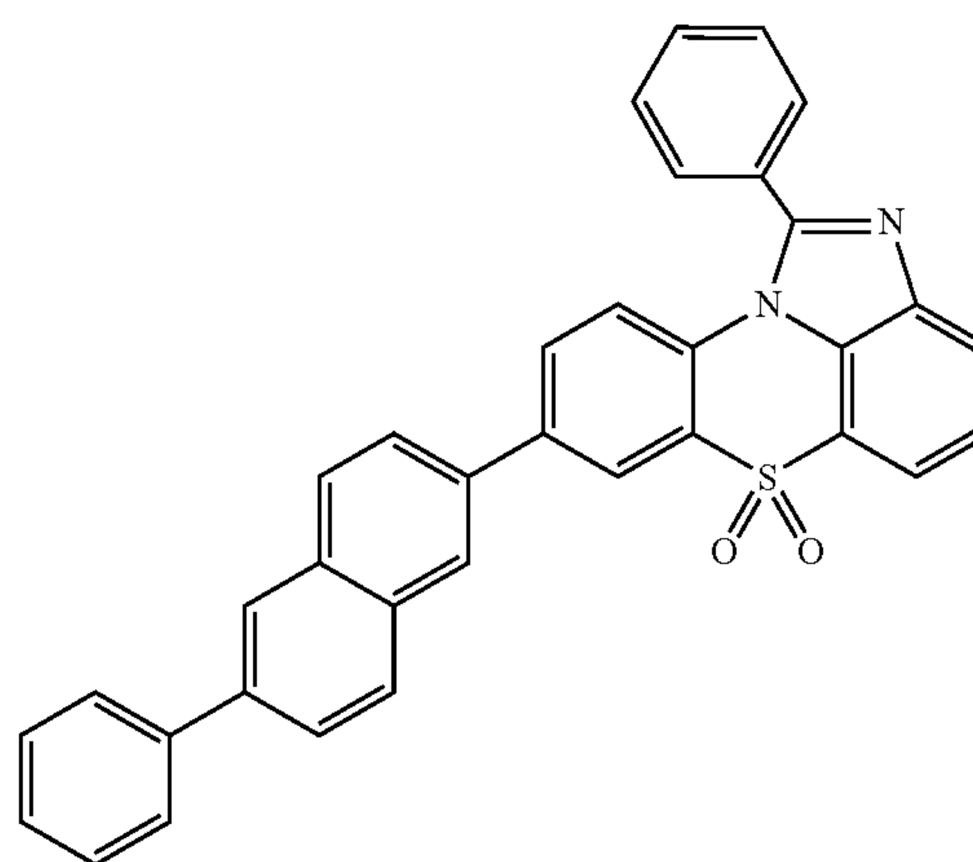
[Chemical Formula 1-4-28]
