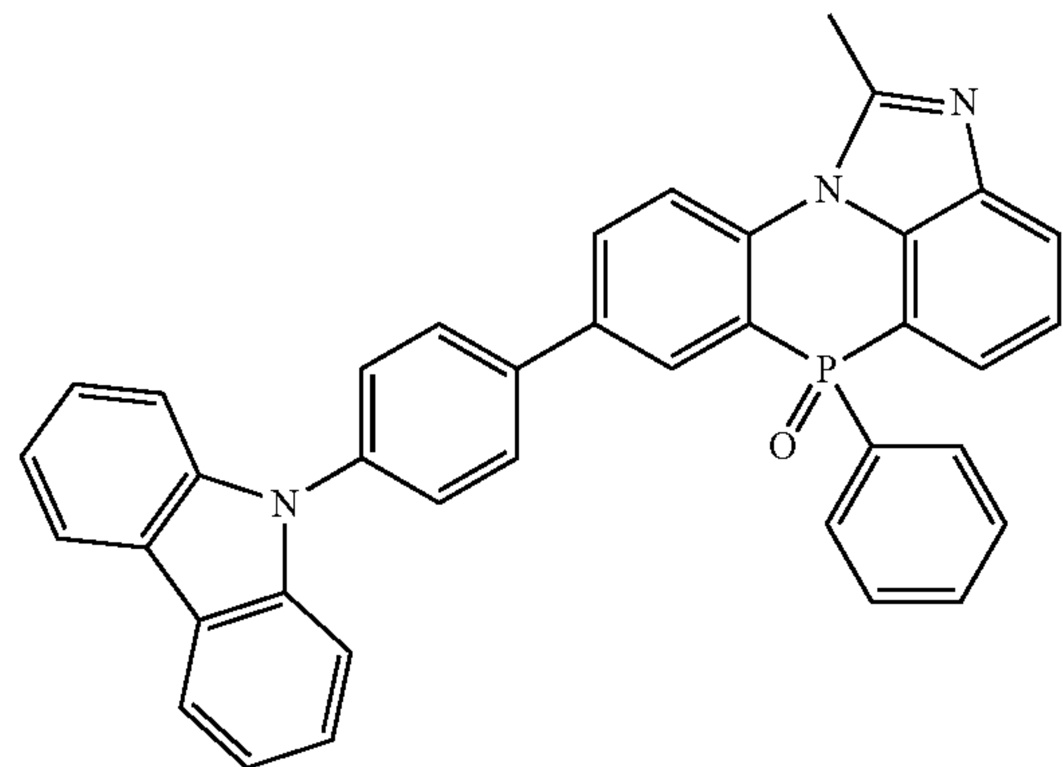
[Chemical Formula 2-2-42]
