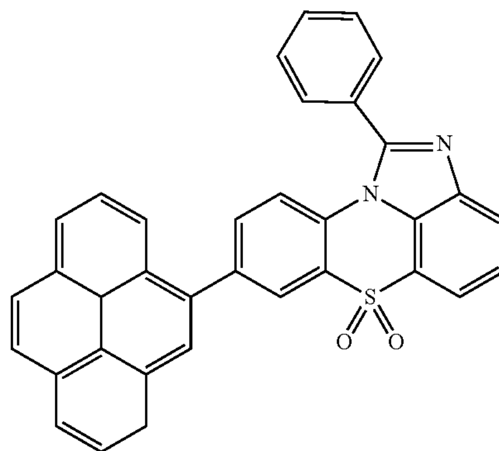
[Chemical Formula 1-4-29]
