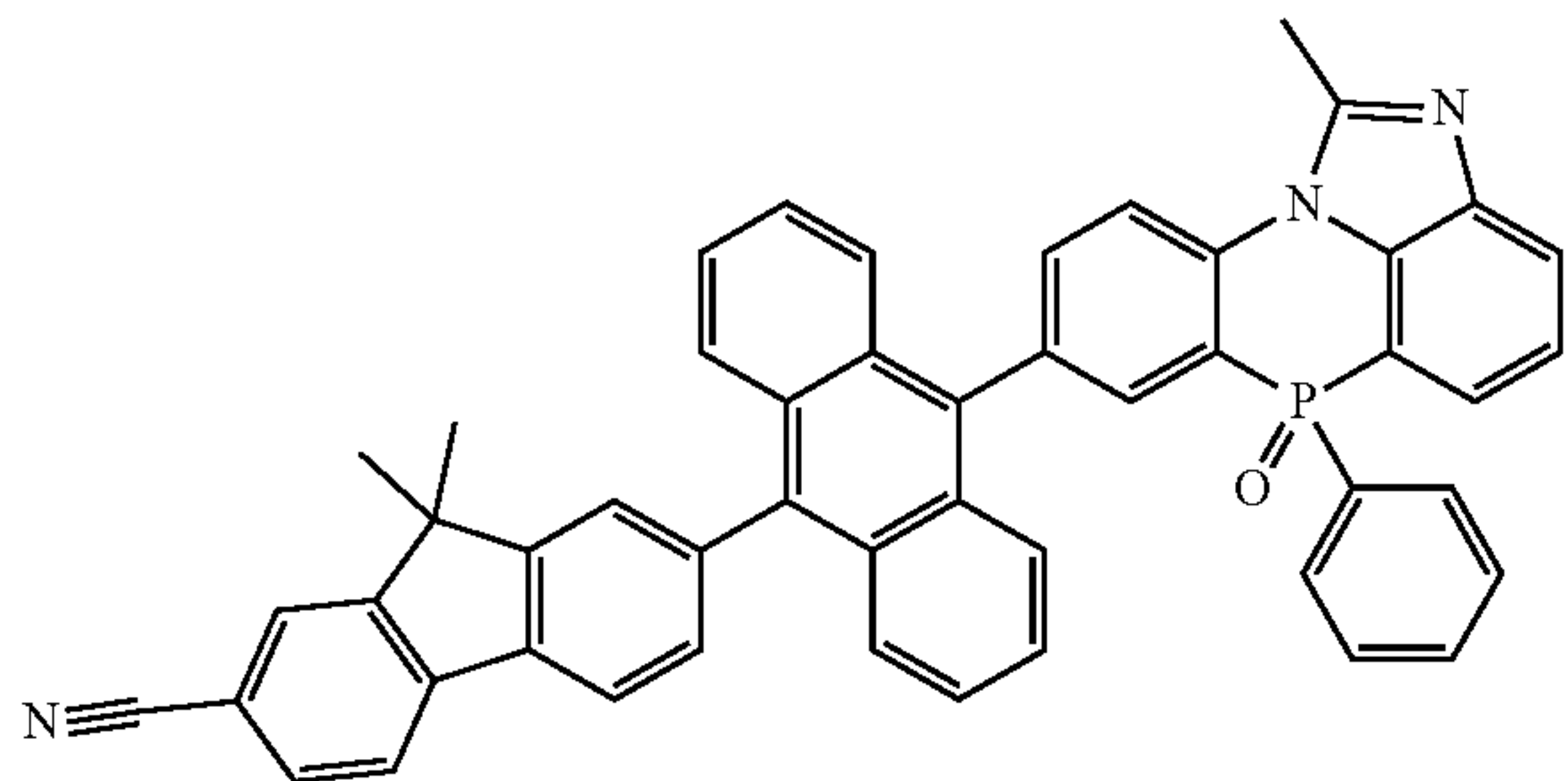
[Chemical Formula 2-2-15]
