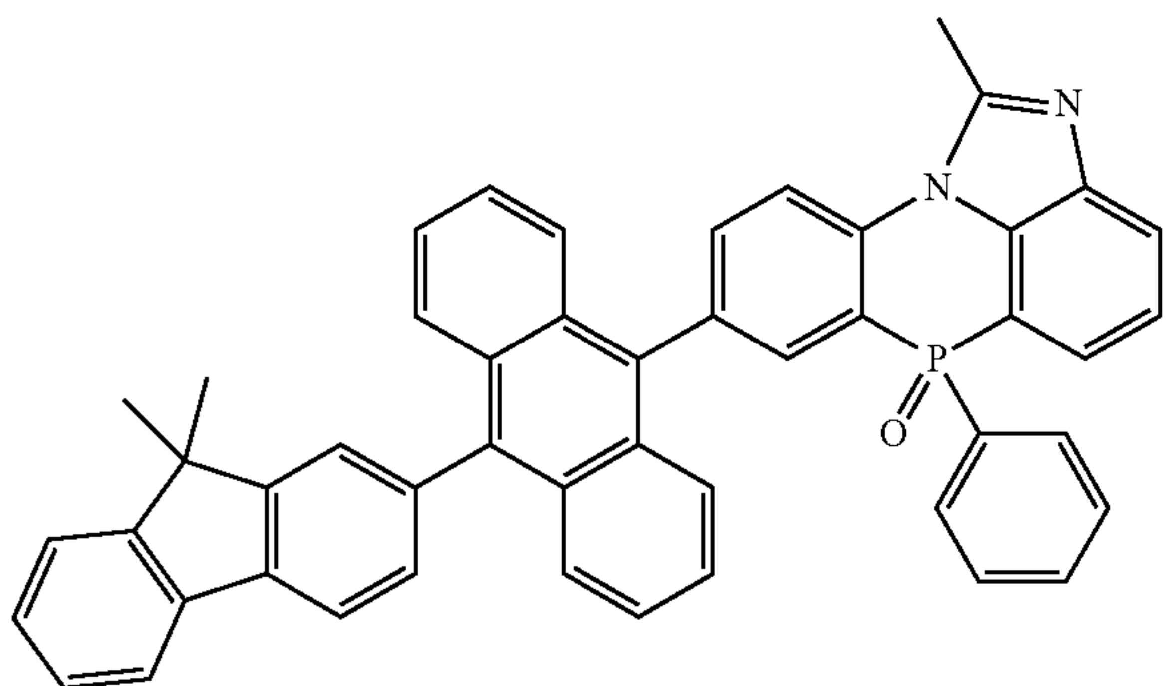
[Chemical Formula 2-2-5]
