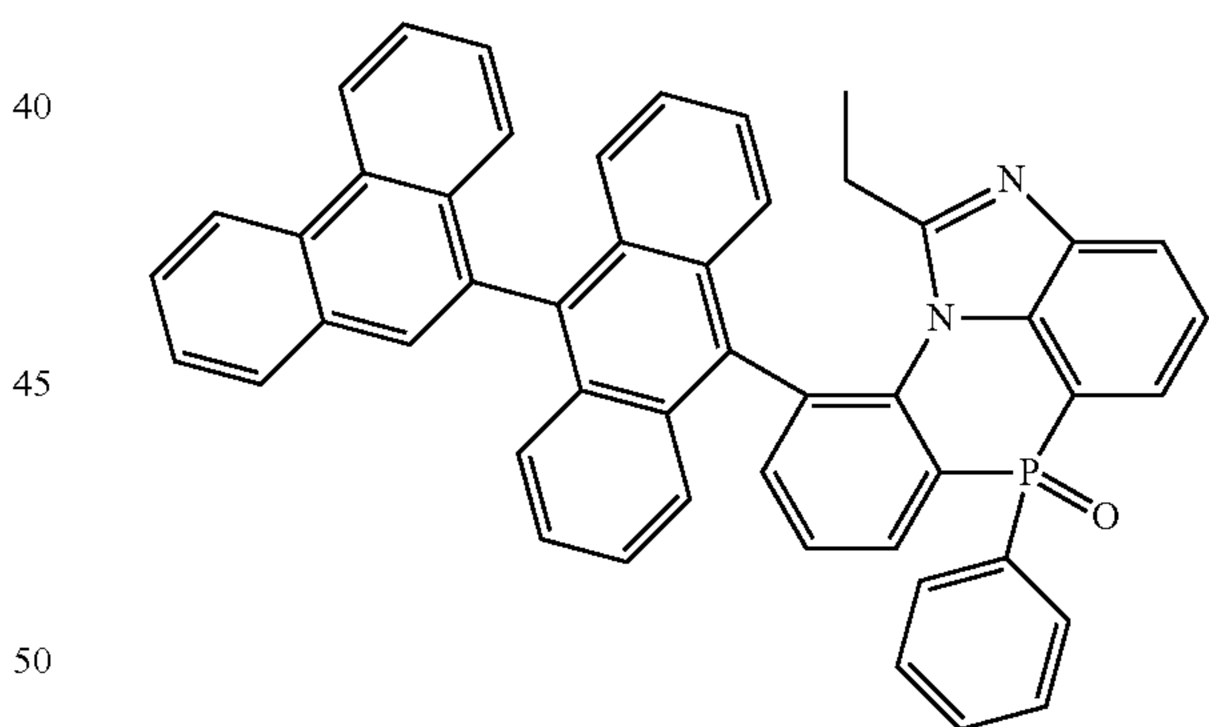
[Chemical Formula 2-8-7]
