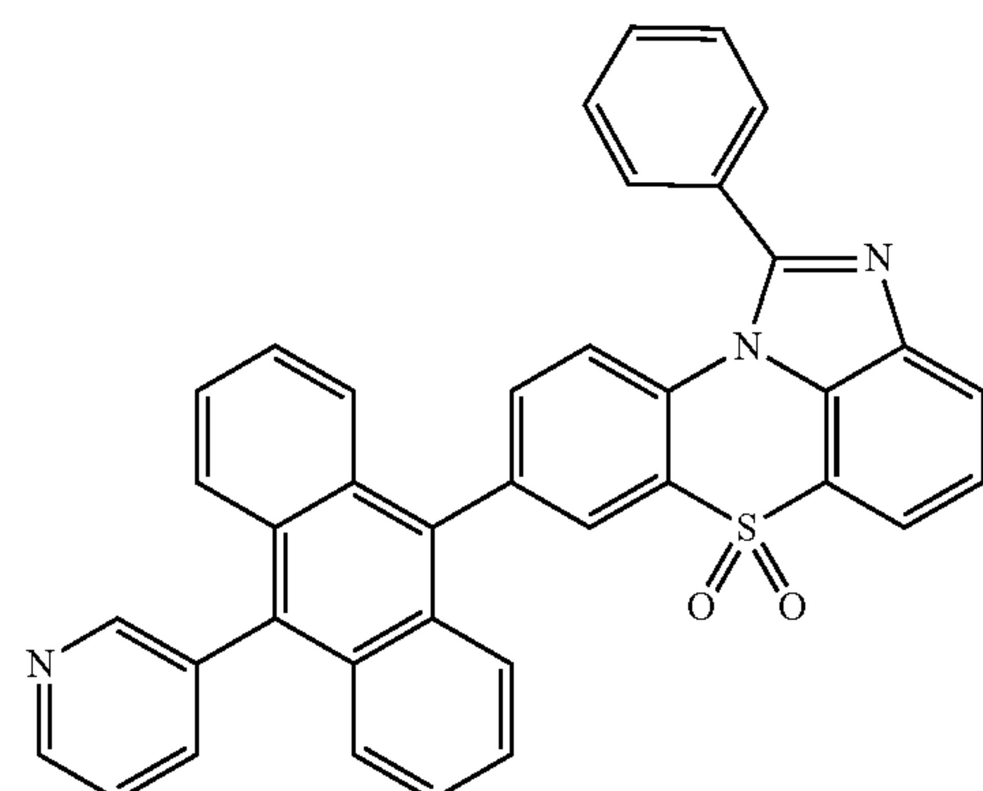
[Chemical Formula 1-4-10]
