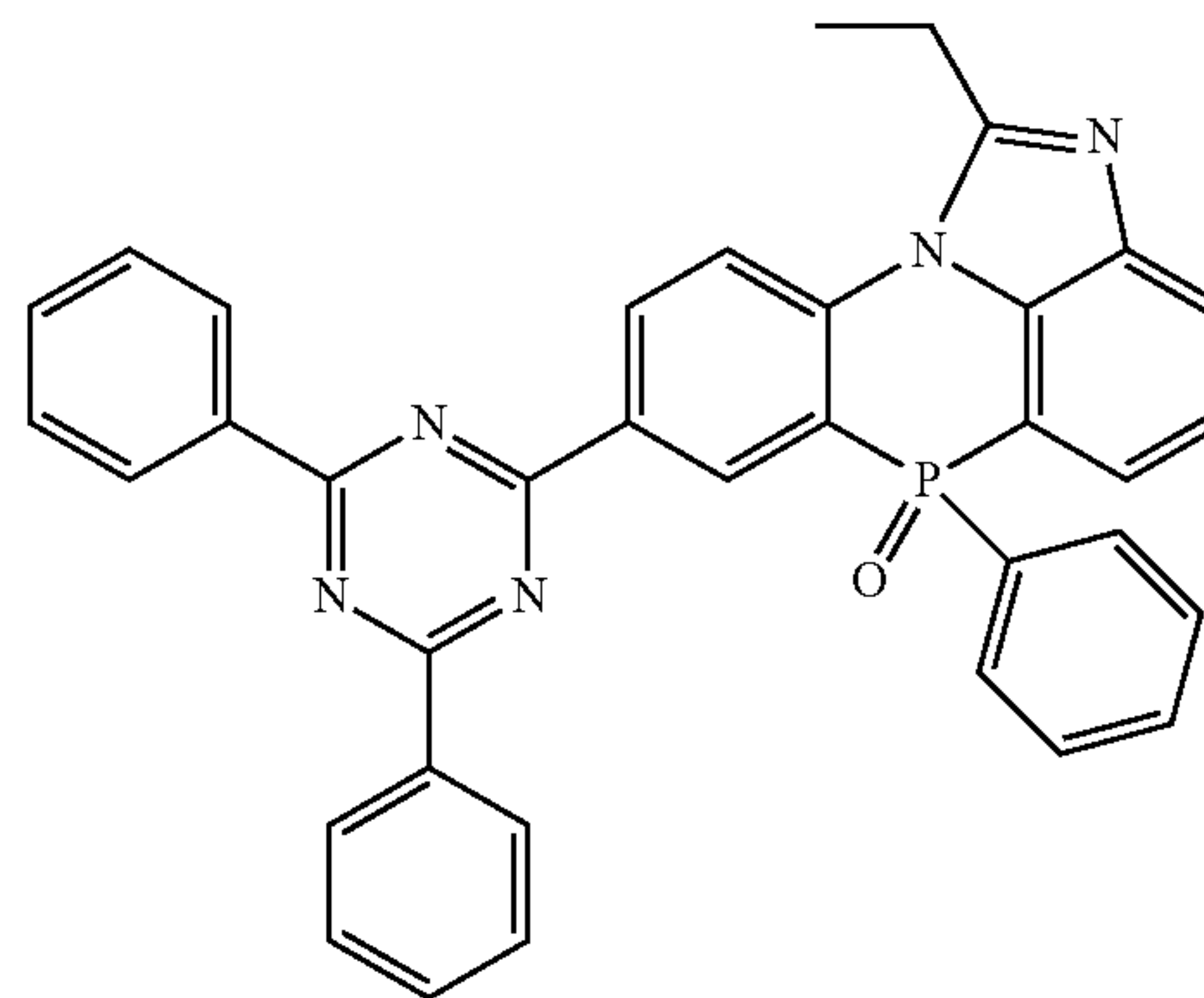
[Chemical Formula 2-3-42]
