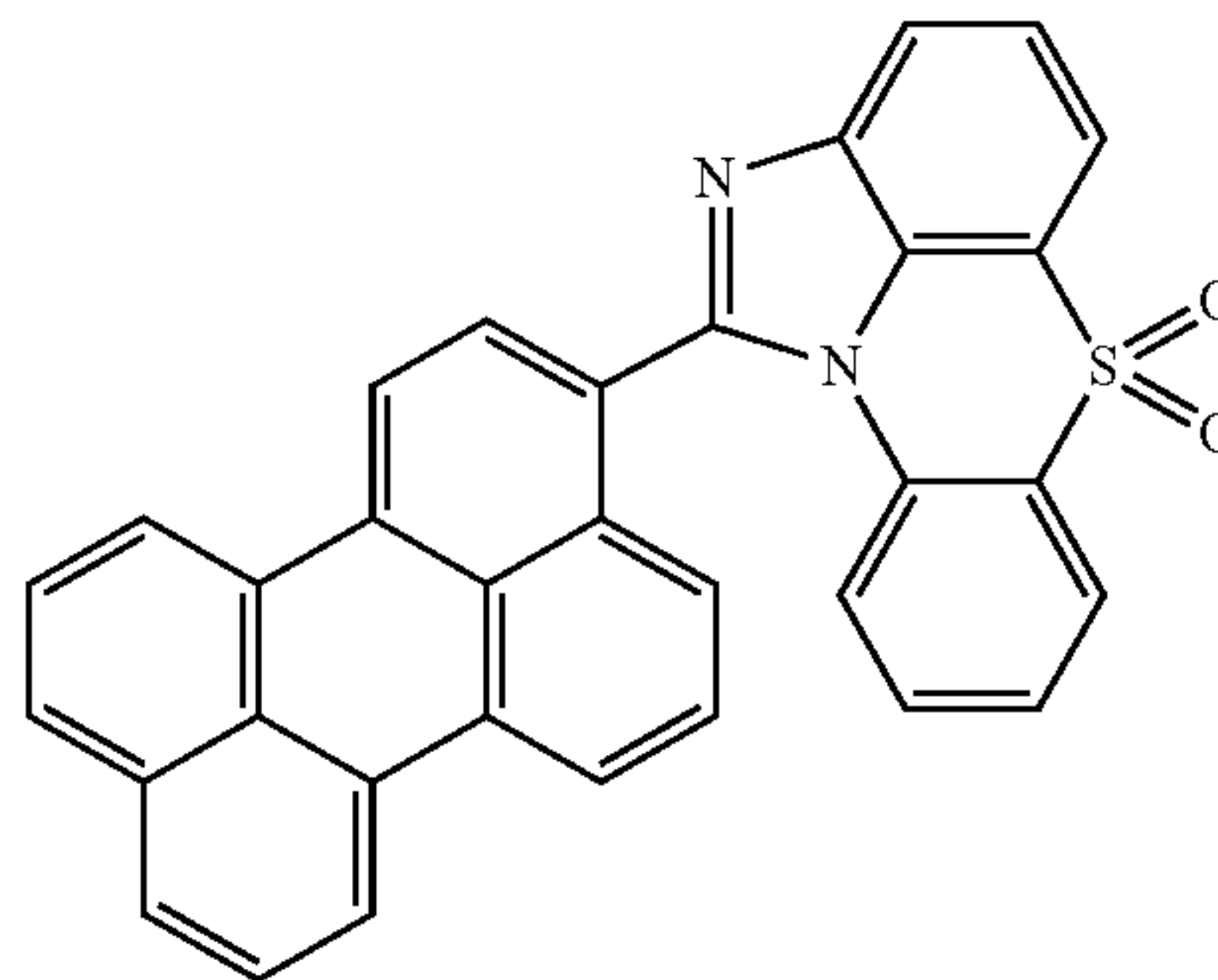
[Chemical Formula 1-5-29]
