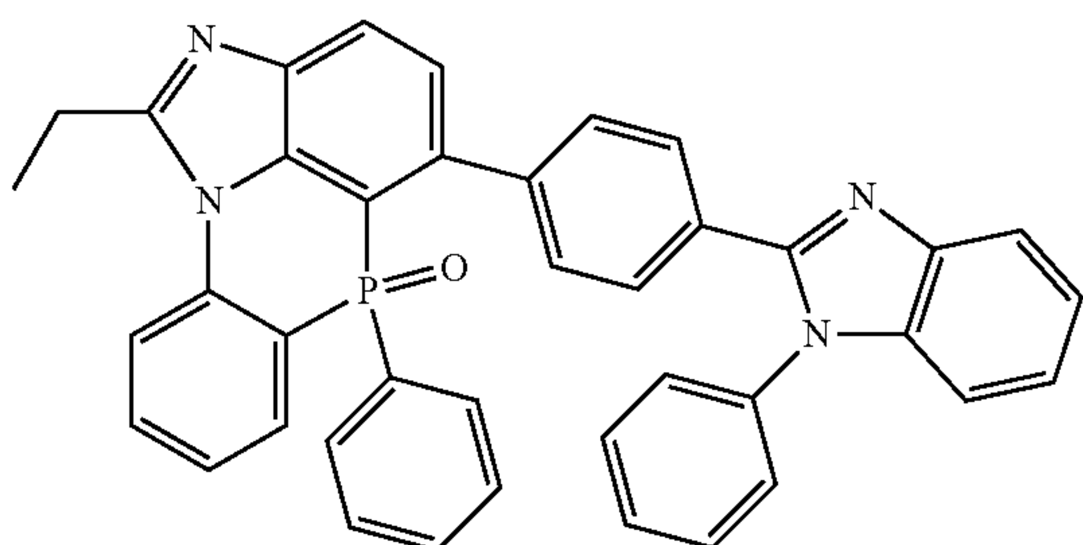
[Chemical Formula 2-9-9]
