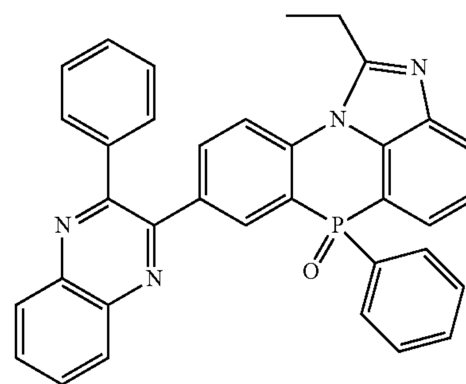
[Chemical Formula 2-3-49]
