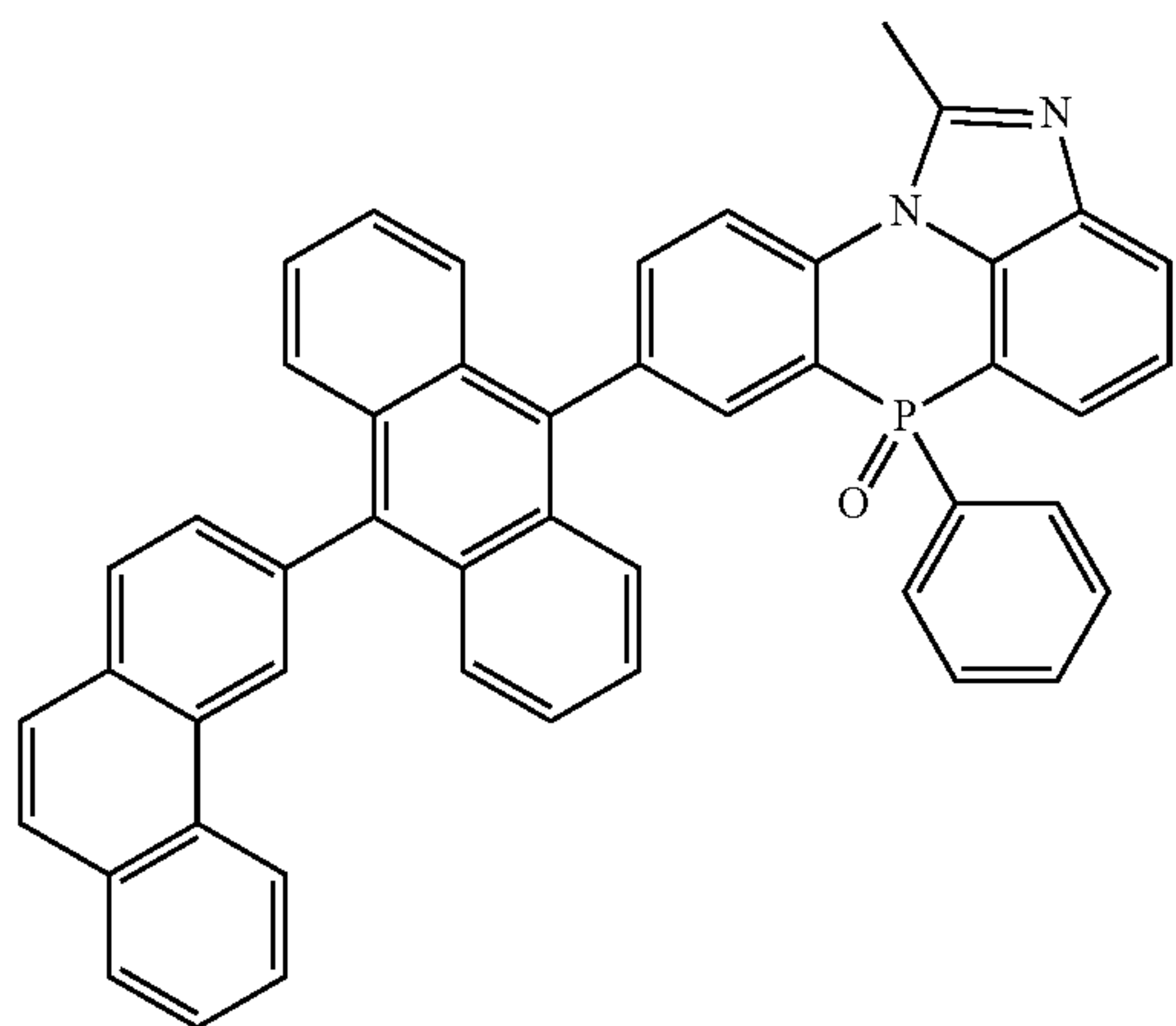
[Chemical Formula 2-2-8]
