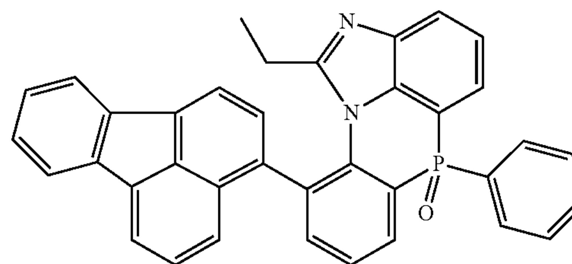
[Chemical Formula 2-8-30]
