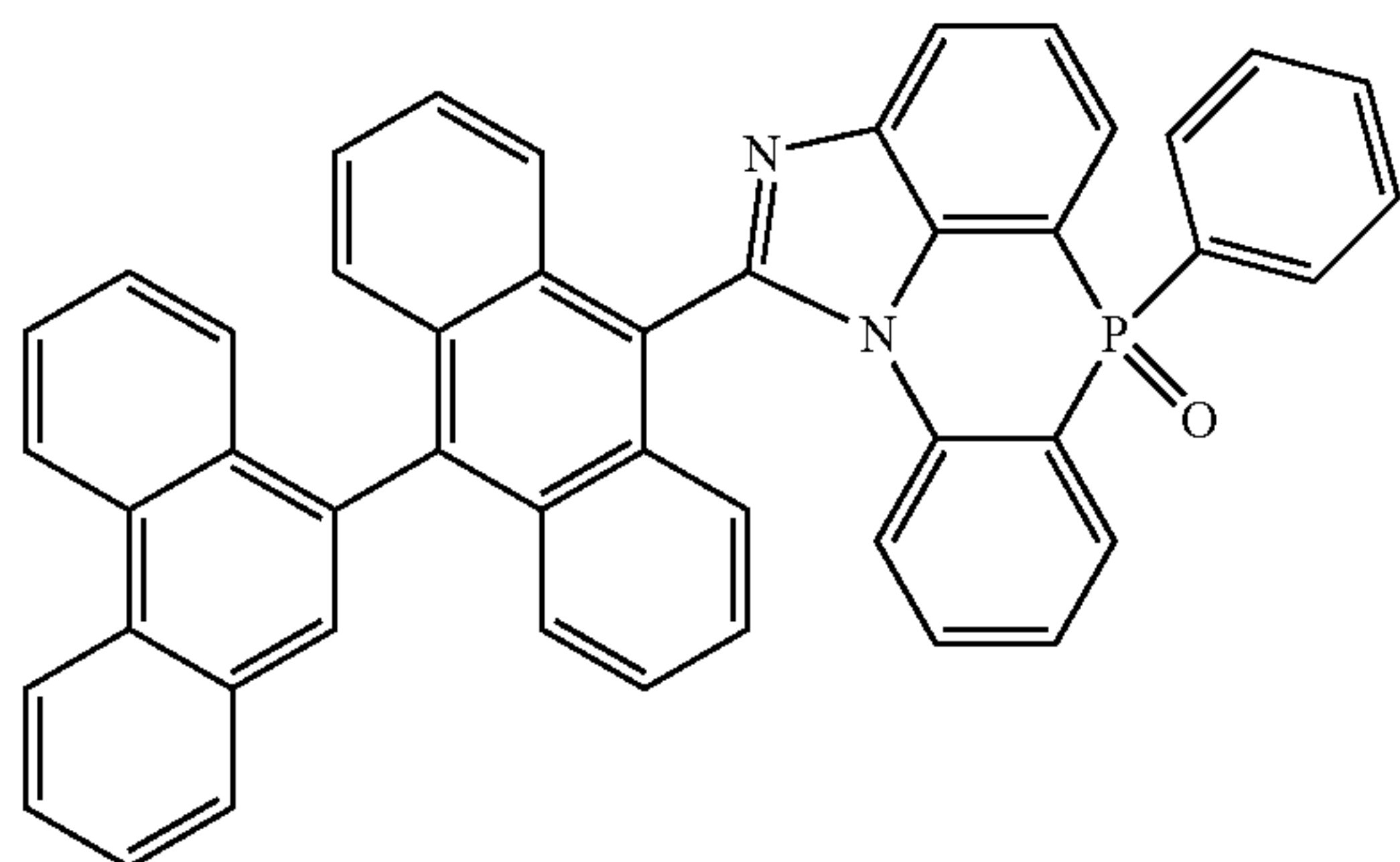
[Chemical Formula 2-5-7]
