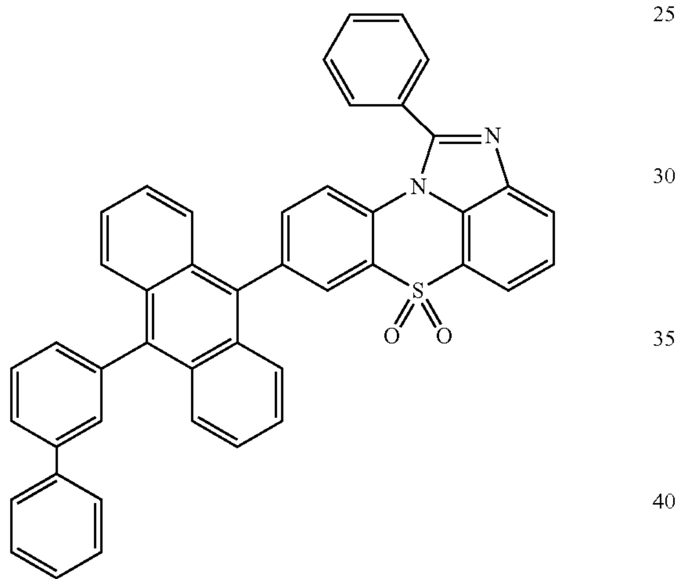
[Chemical Formula 1-4-6]
