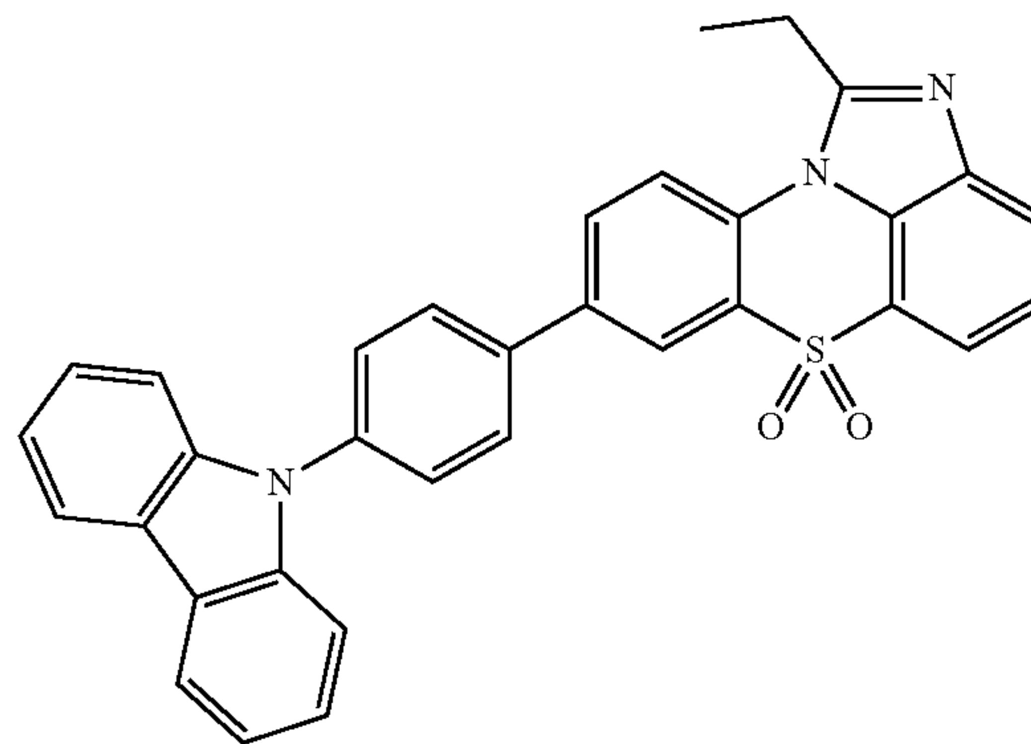
[Chemical Formula 1-3-43]
