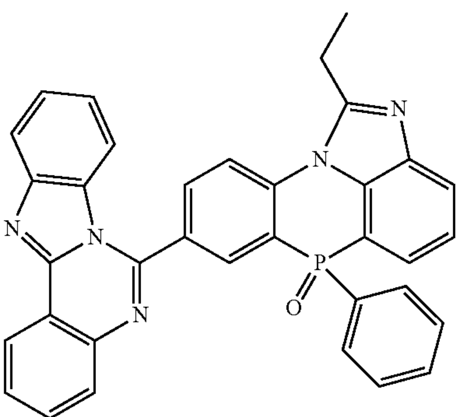
[Chemical Formula 2-3-53]
