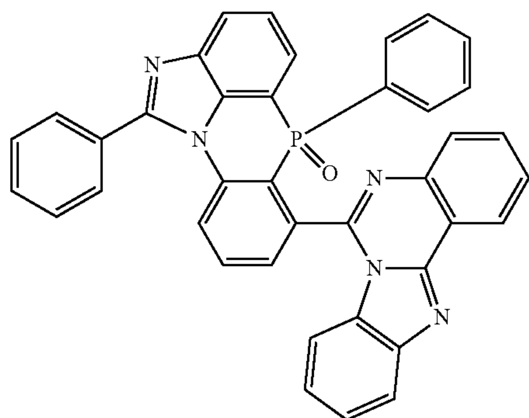
[Chemical Formula 2-6-54]
