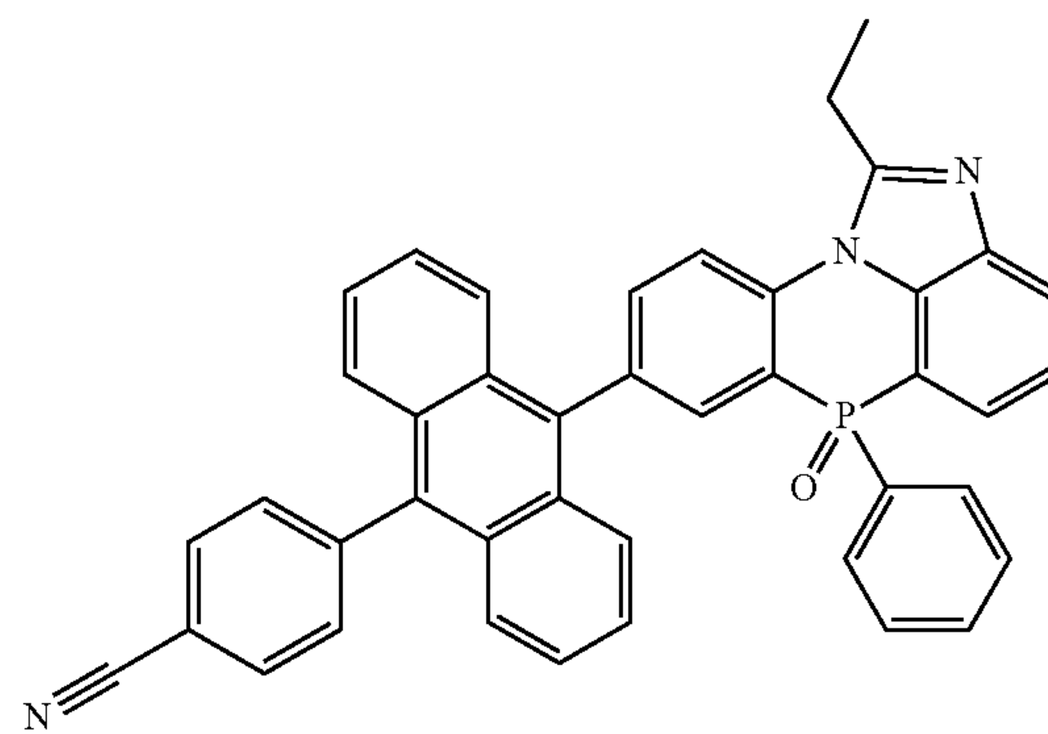
[Chemical Formula 2-3-12]
