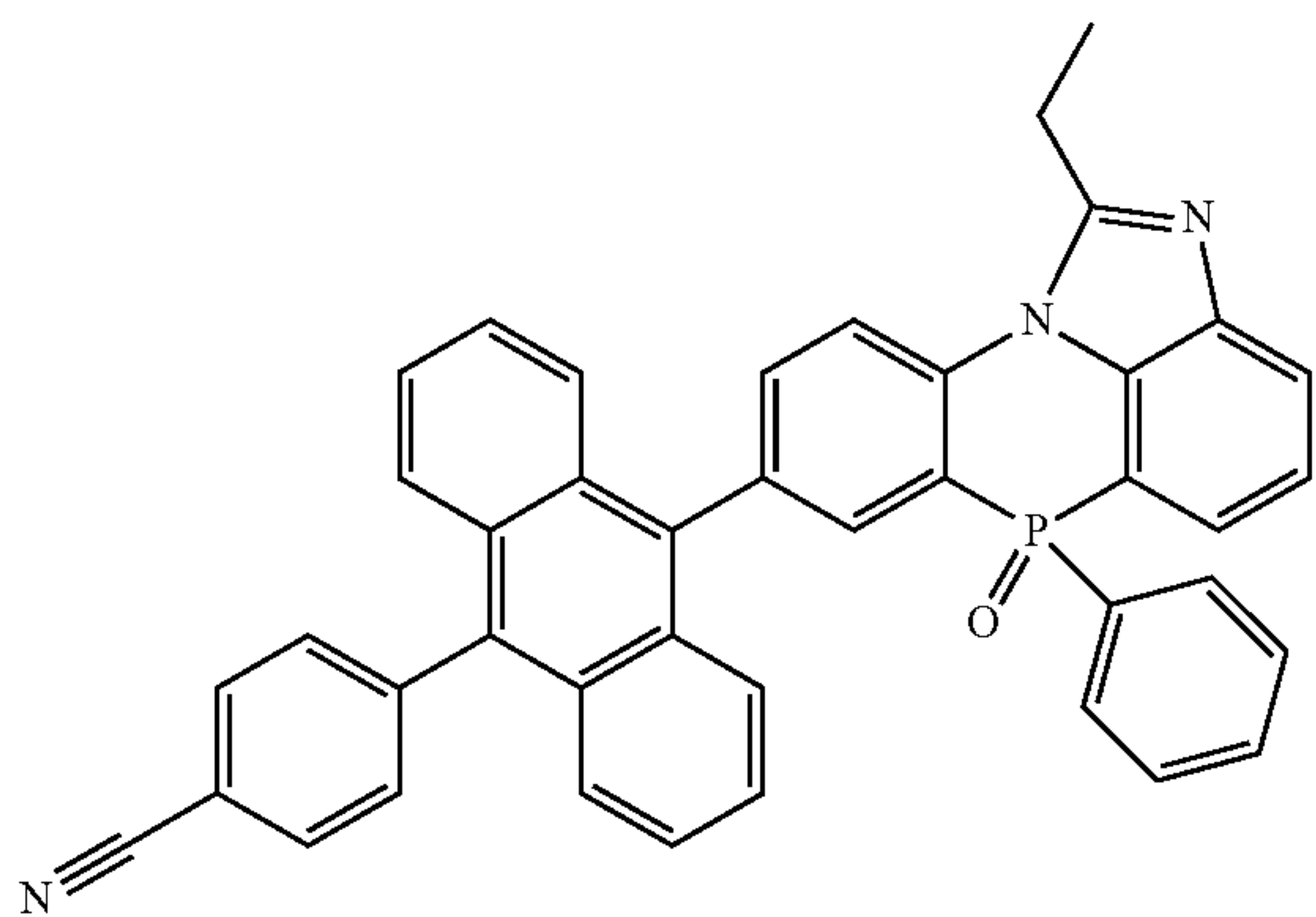
[Chemical Formula 2-3-13]
