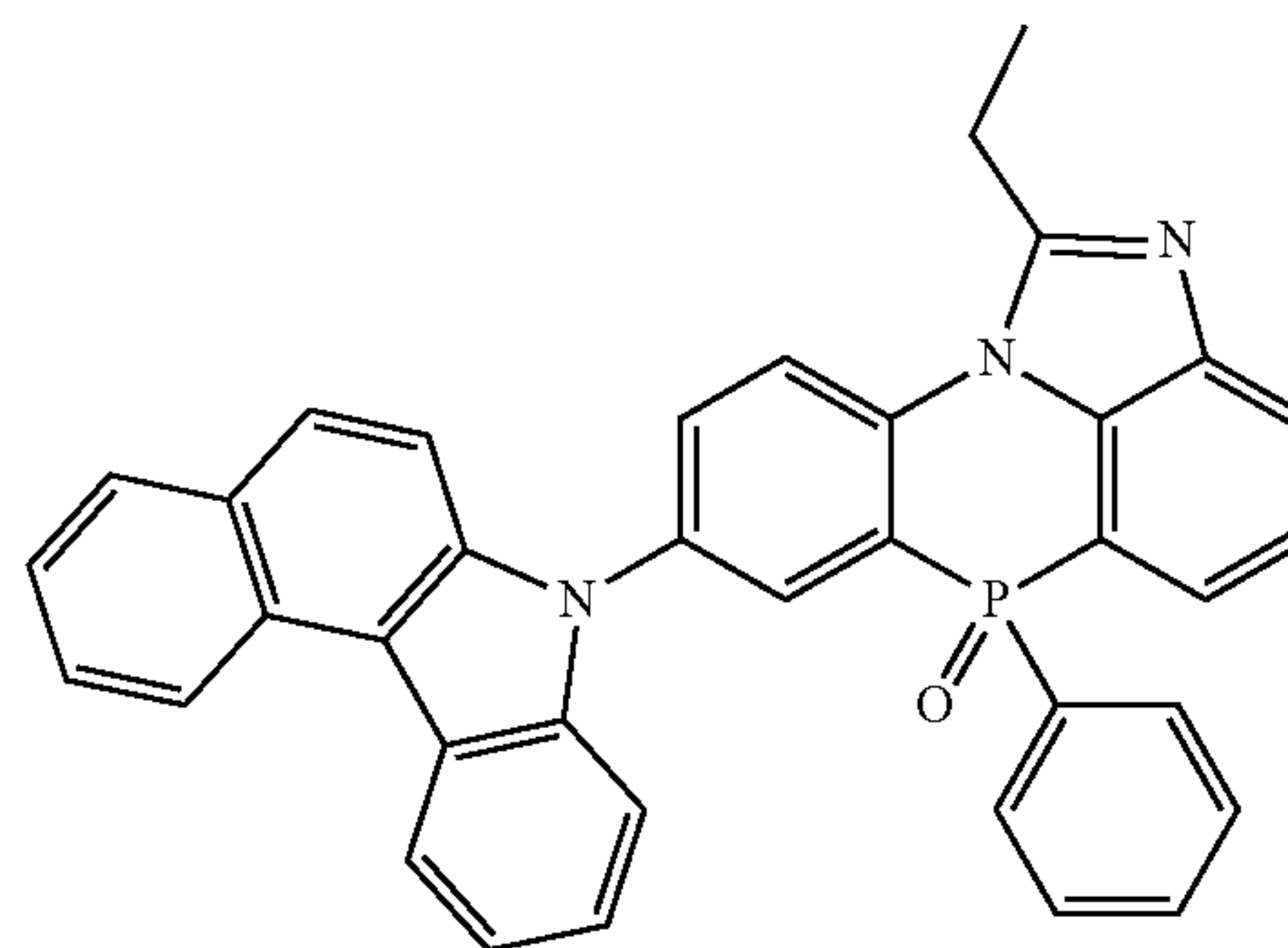
[Chemical Formula 2-3-51]
