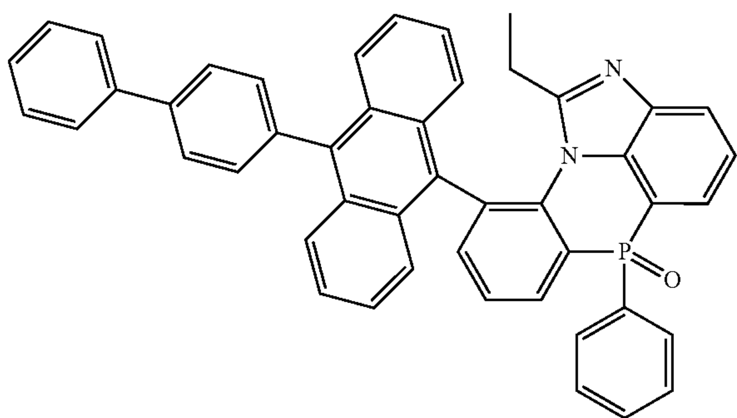
[Chemical Formula 2-8-4]
