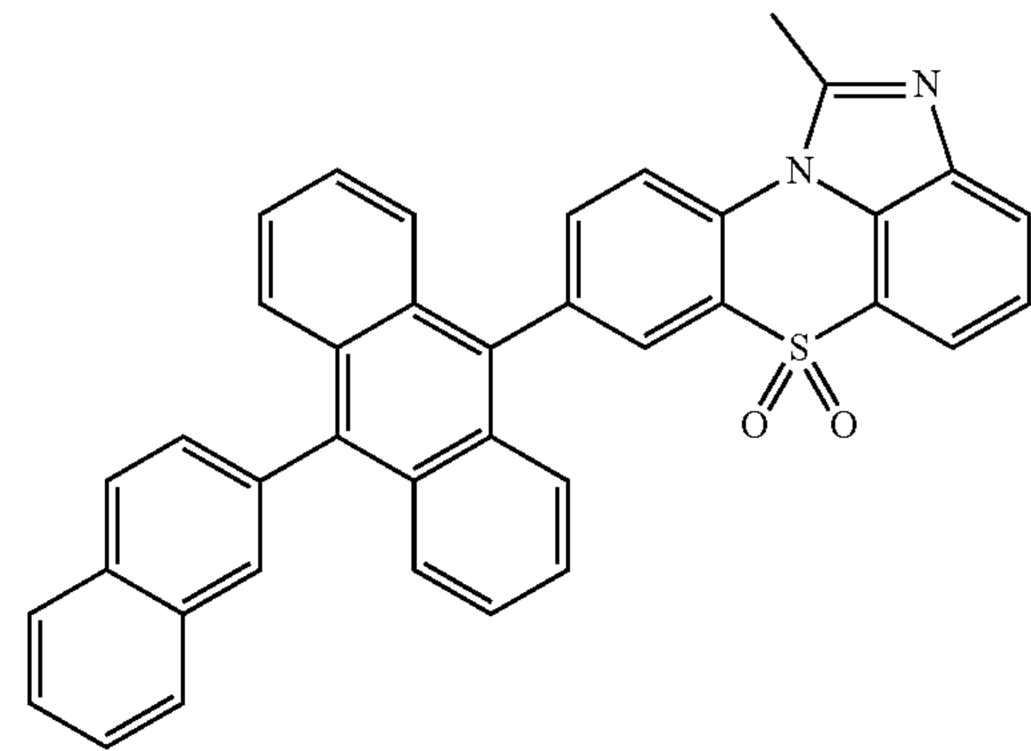
[Chemical Formula 1-2-2]
