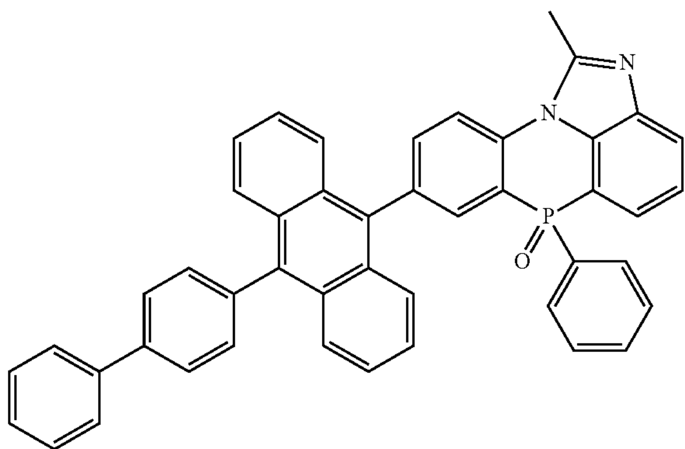
[Chemical Formula 2-2-4]
