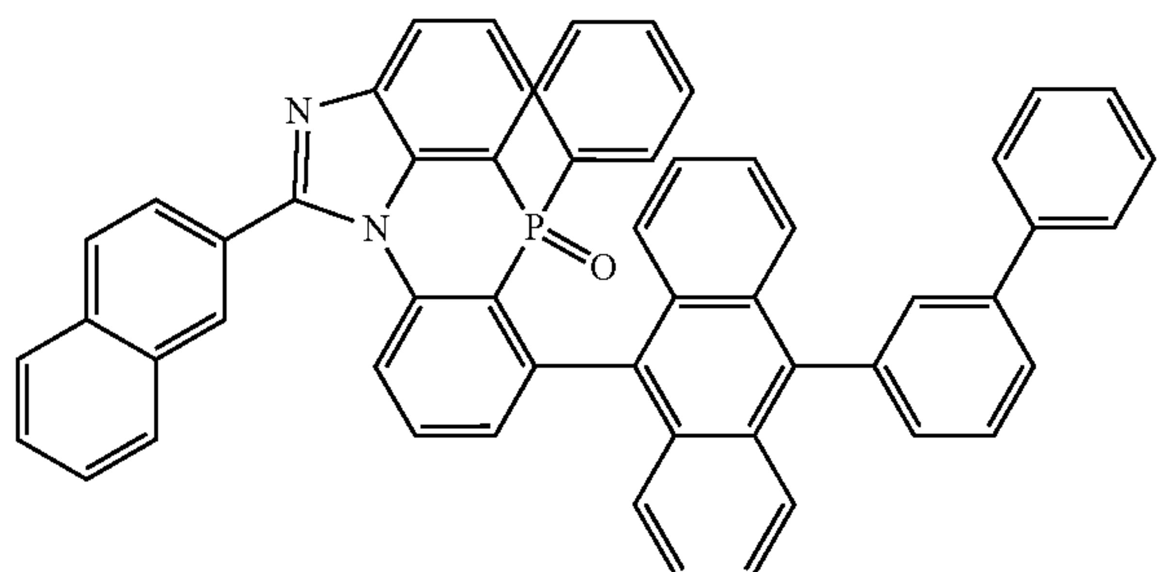
[Chemical Formula 2-6-7]
