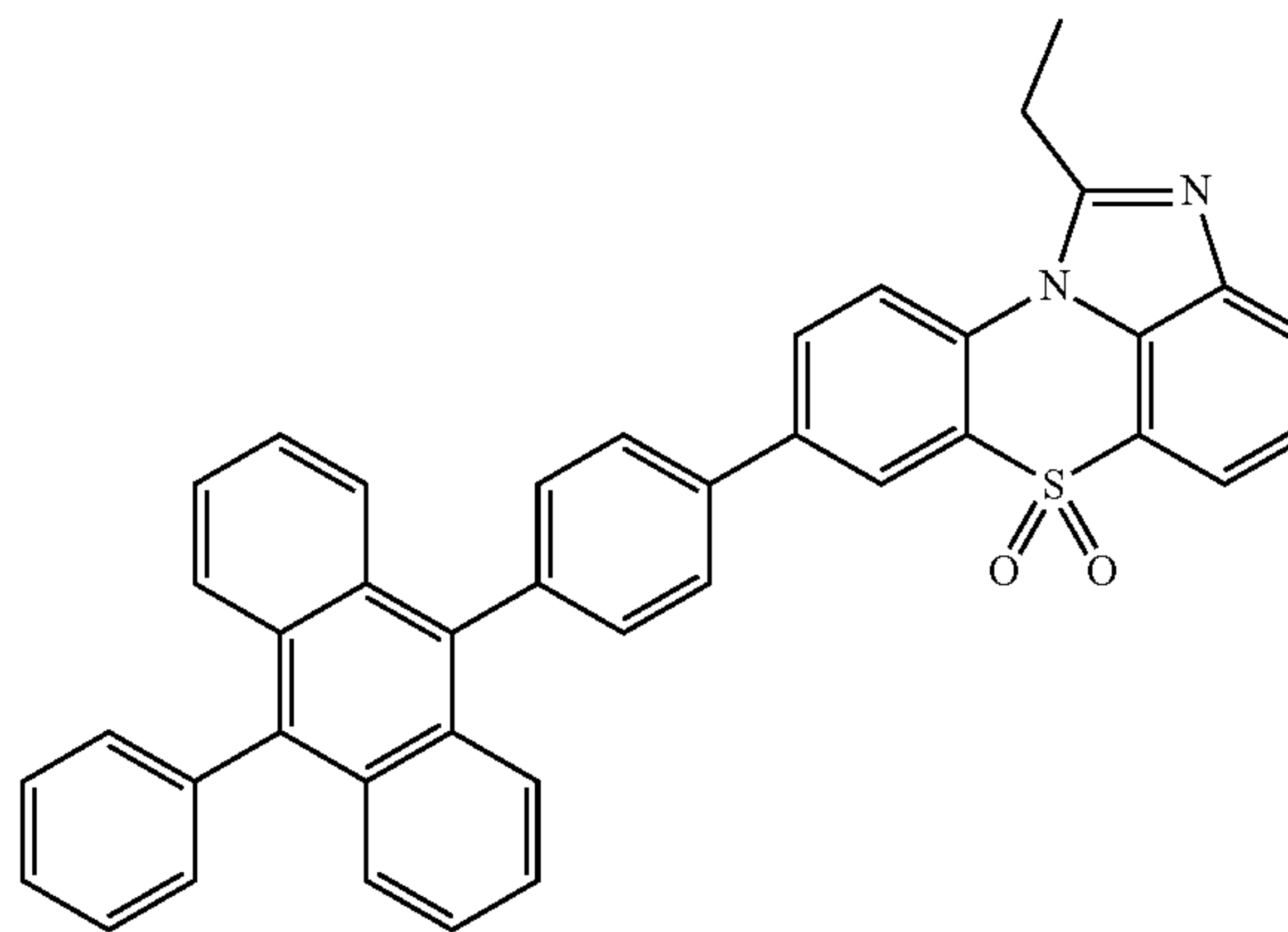
[Chemical Formula 1-3-17]
