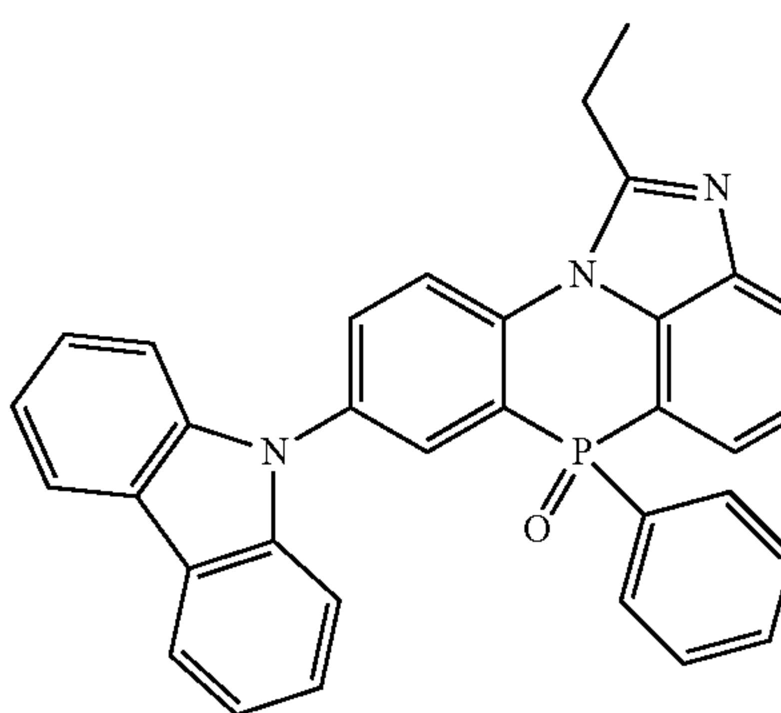
[Chemical Formula 2-3-50]
