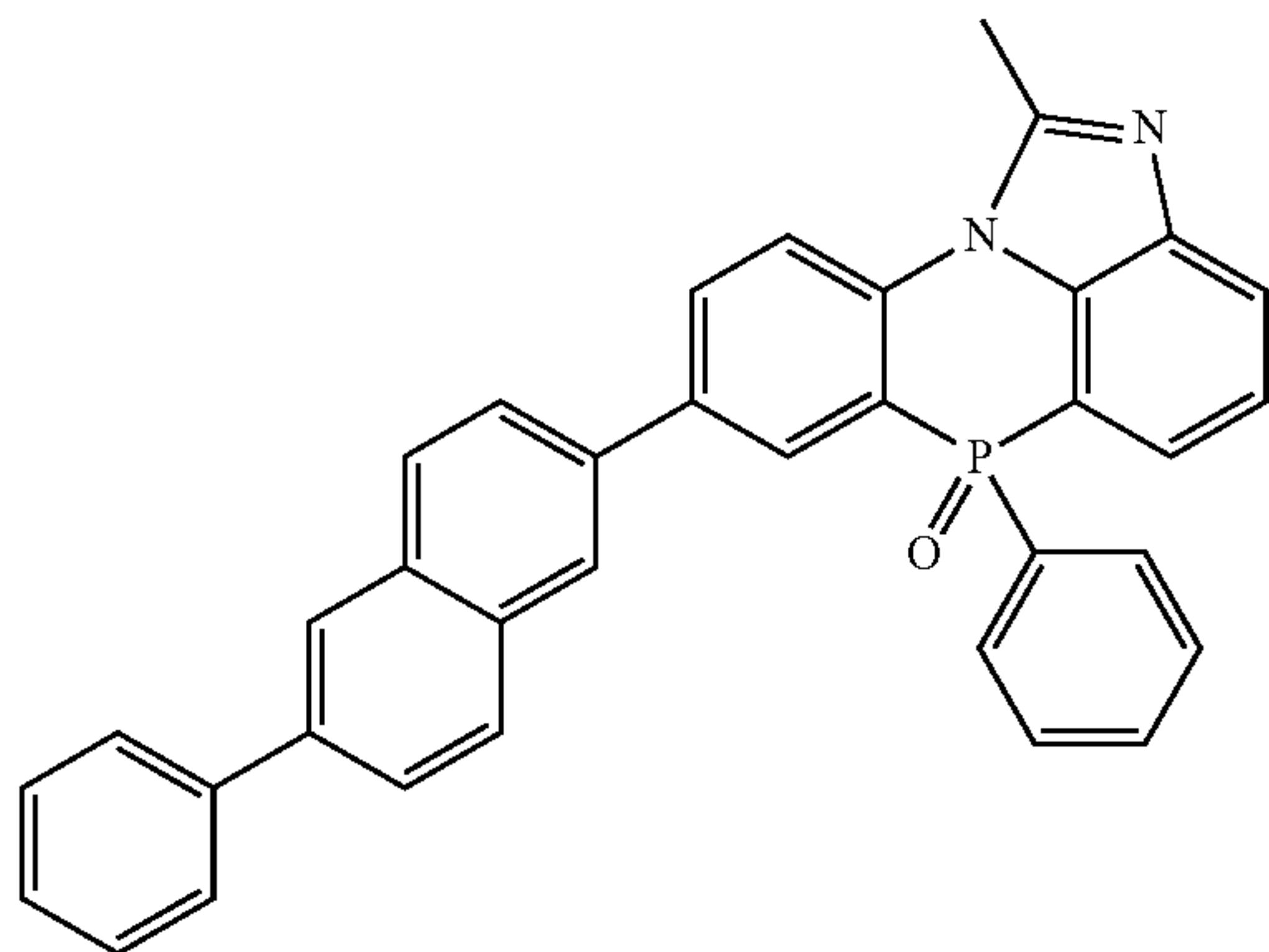
[Chemical Formula 2-2-27]
