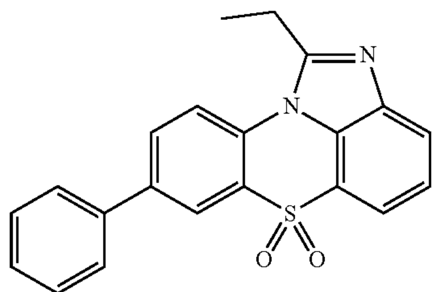
[Chemical Formula 1-3-38]
