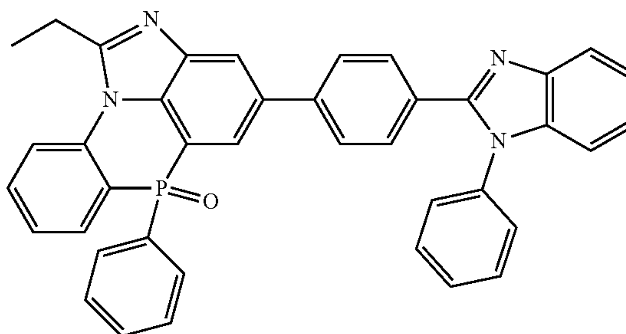
[Chemical Formula 2-10-9]
