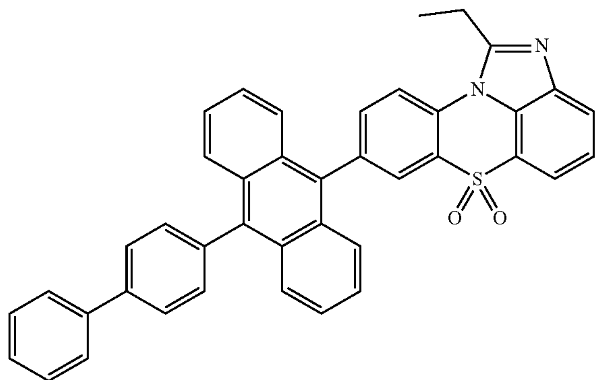
[Chemical Formula 1-3-4]
