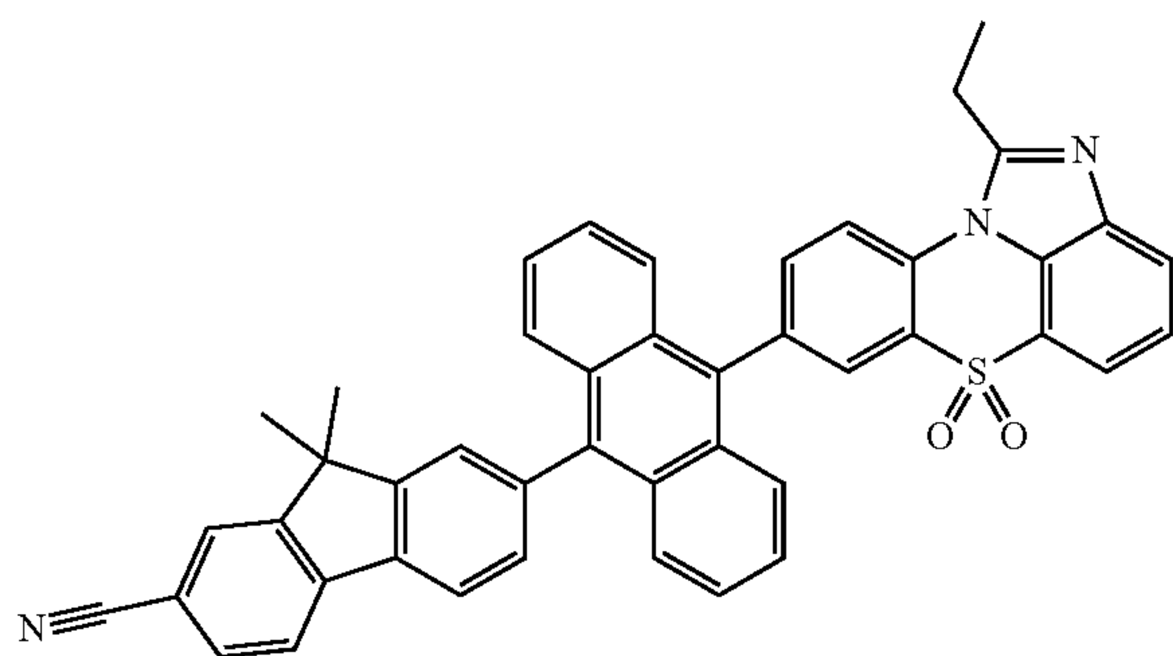
[Chemical Formula 1-3-15]
