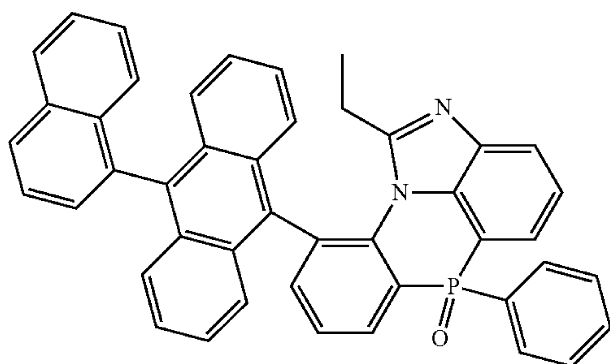
[Chemical Formula 2-8-4]
