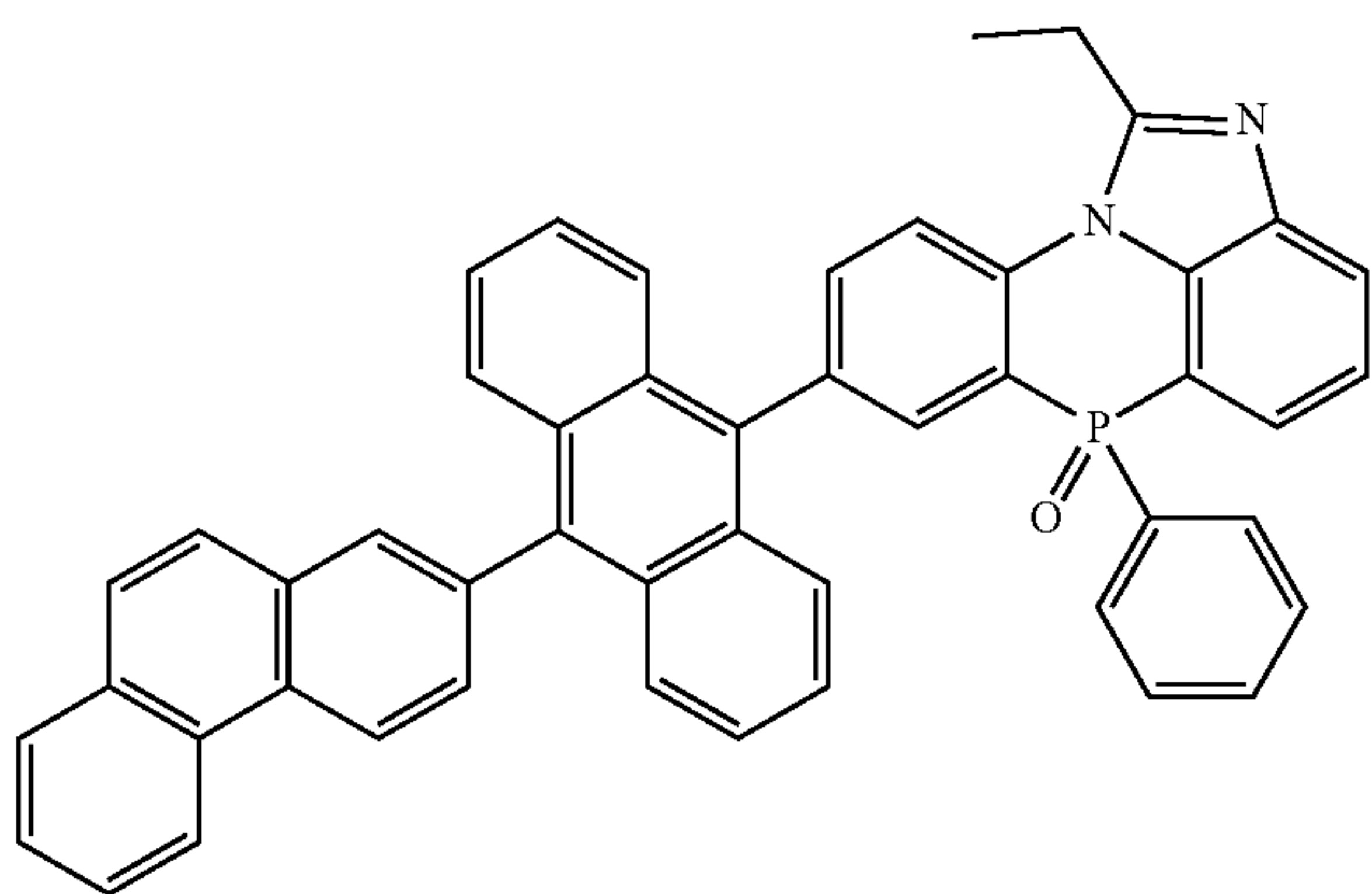
[Chemical Formula 2-3-9]
