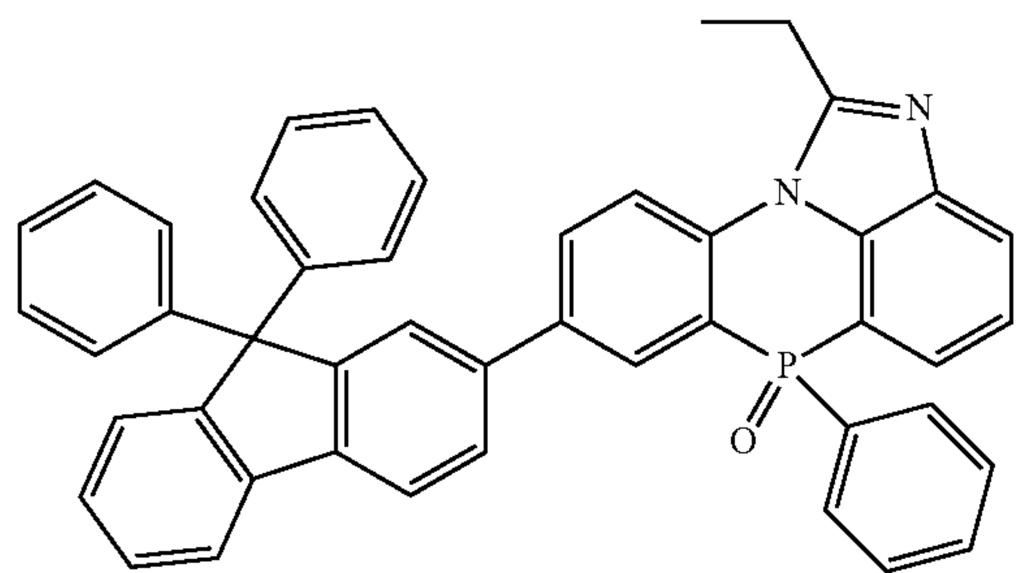
[Chemical Formula 2-3-36]
