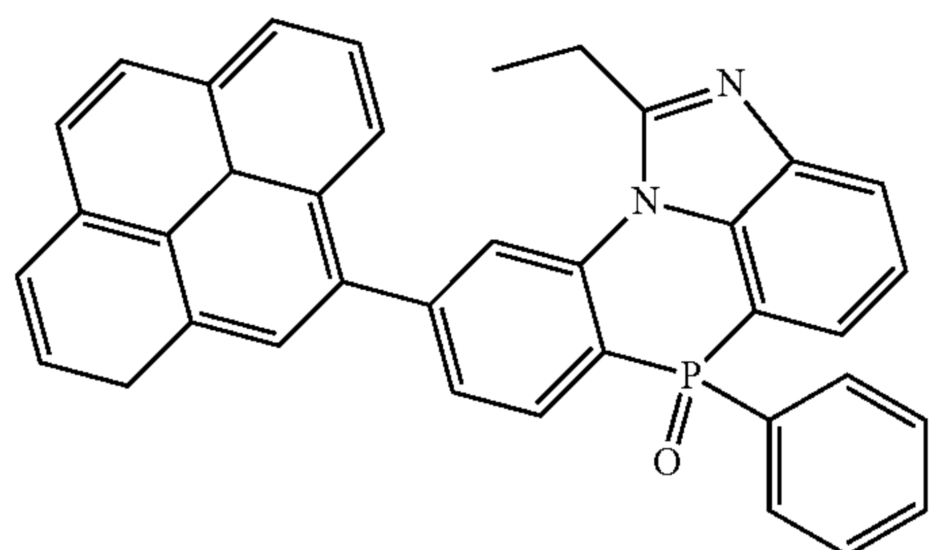
[Chemical Formula 2-7-28]
