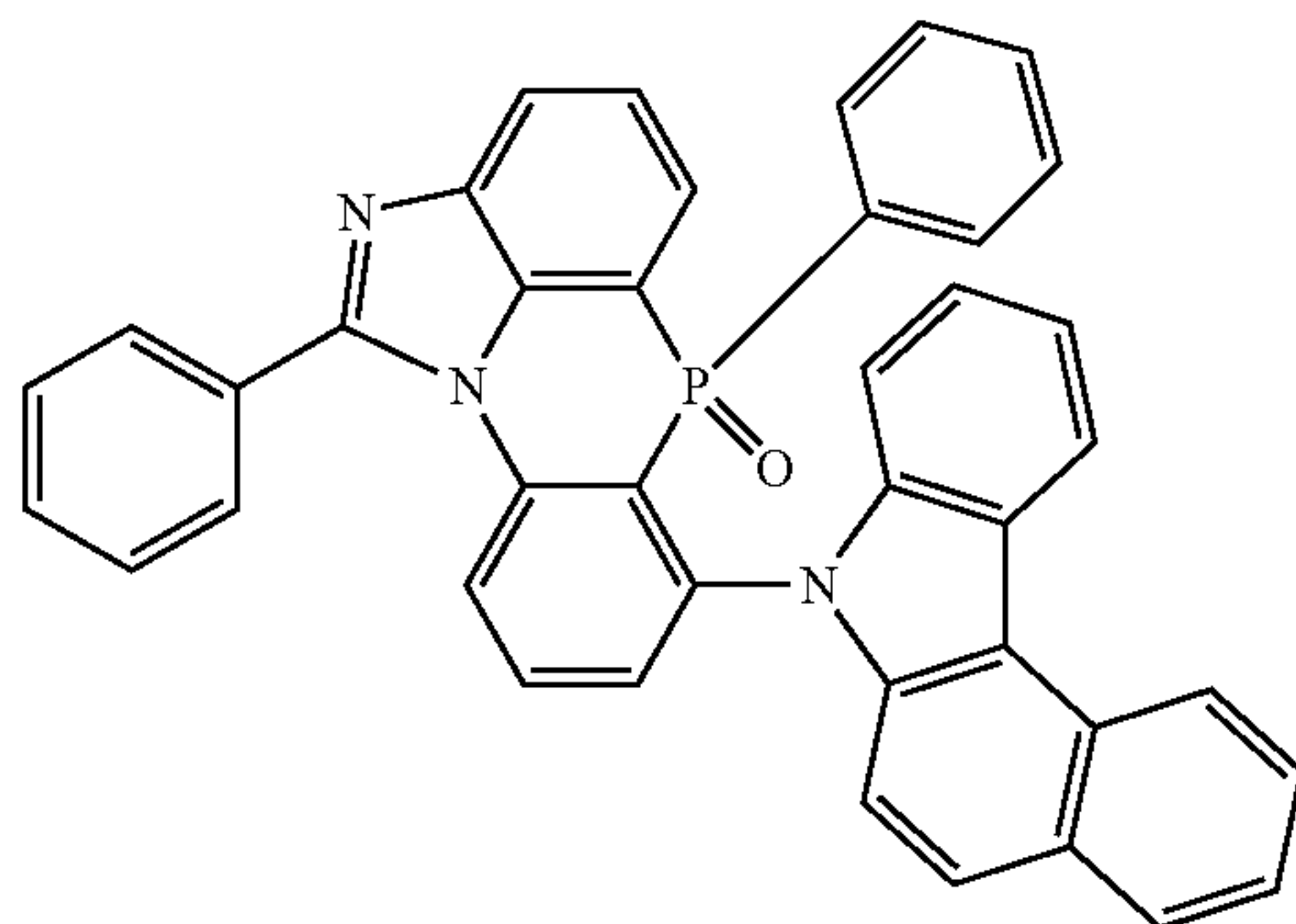
[Chemical Formula 2-6-52]
