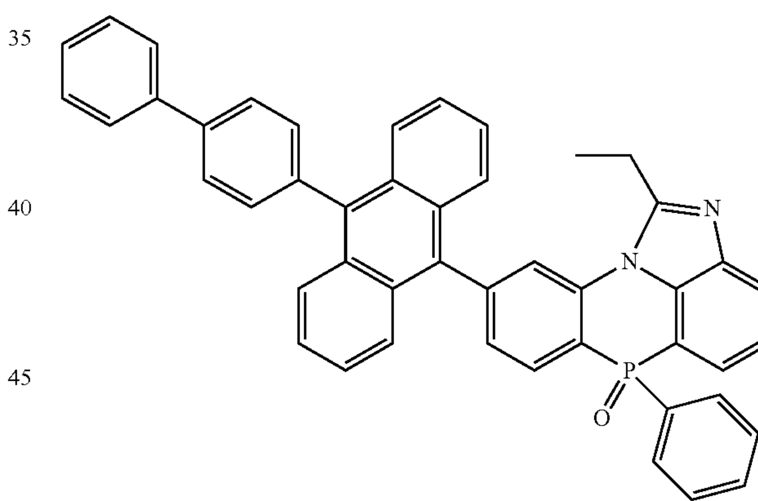
[Chemical Formula 2-7-5]
