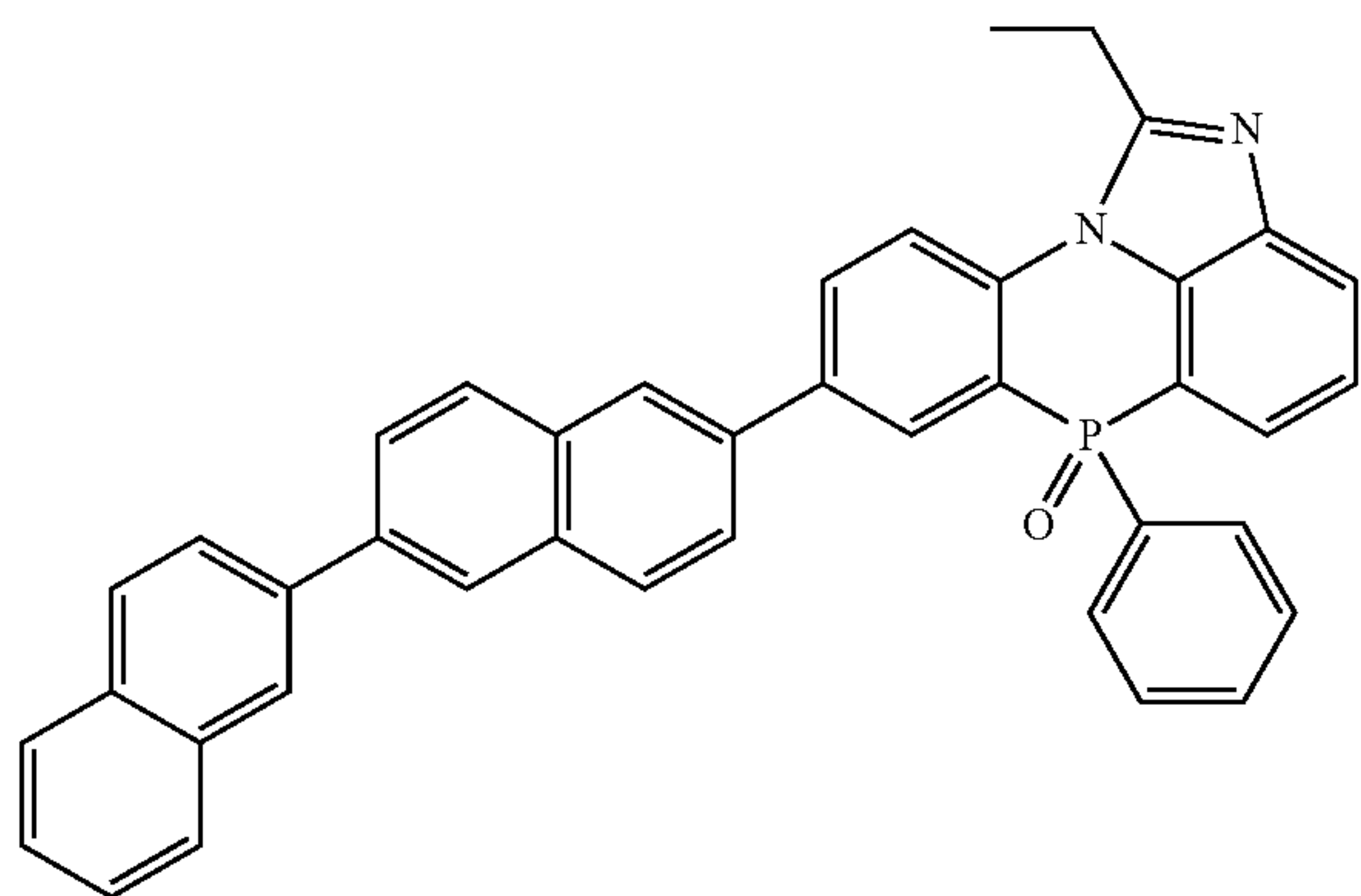
[Chemical Formula 2-3-44]
