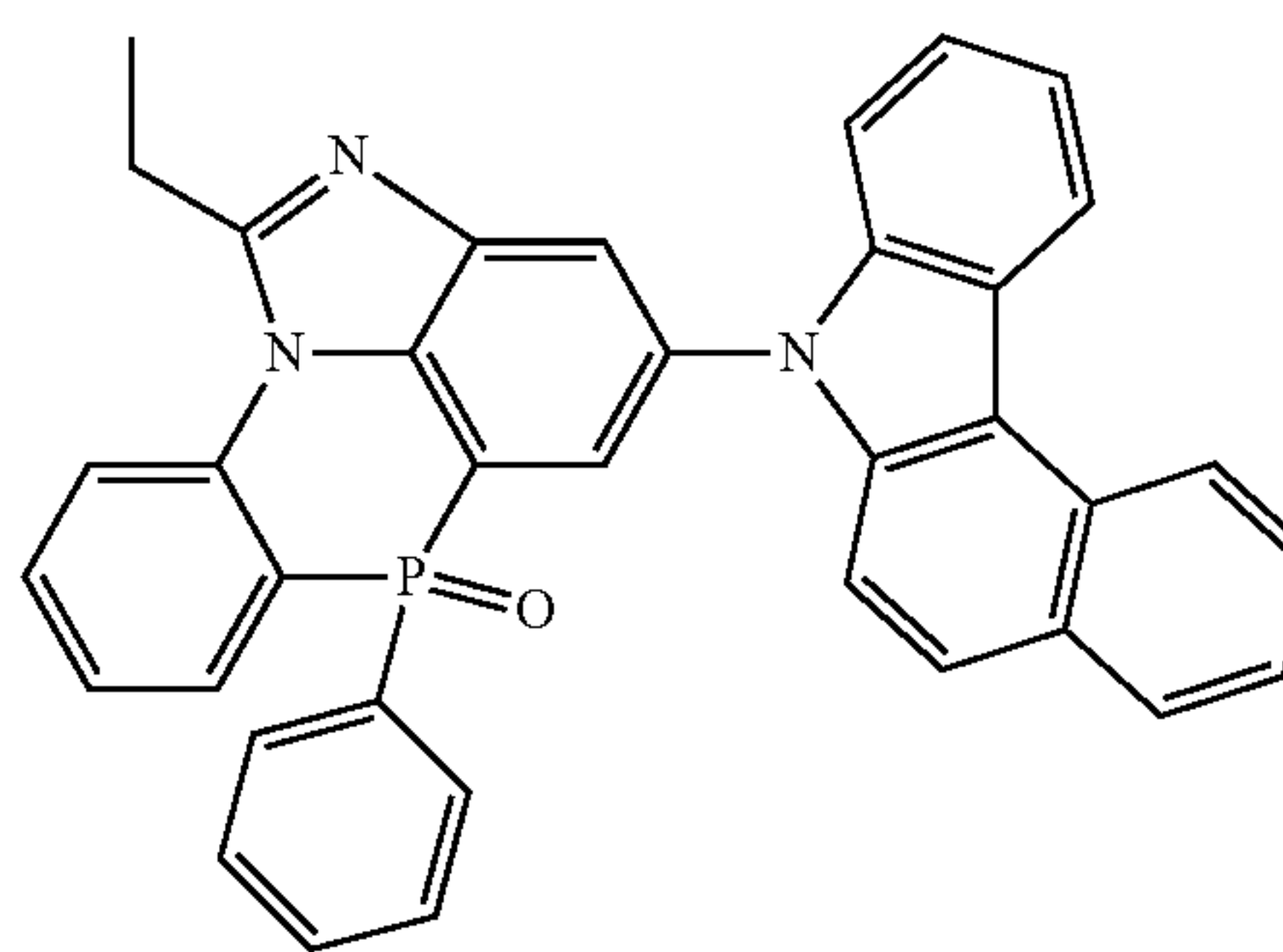
[Chemical Formula 2-10-15]
