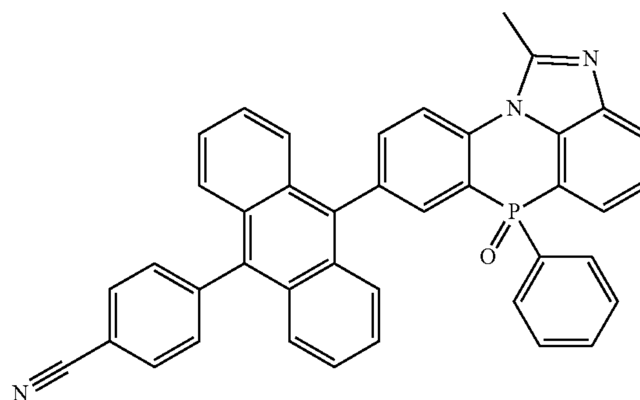
[Chemical Formula 2-2-12]
