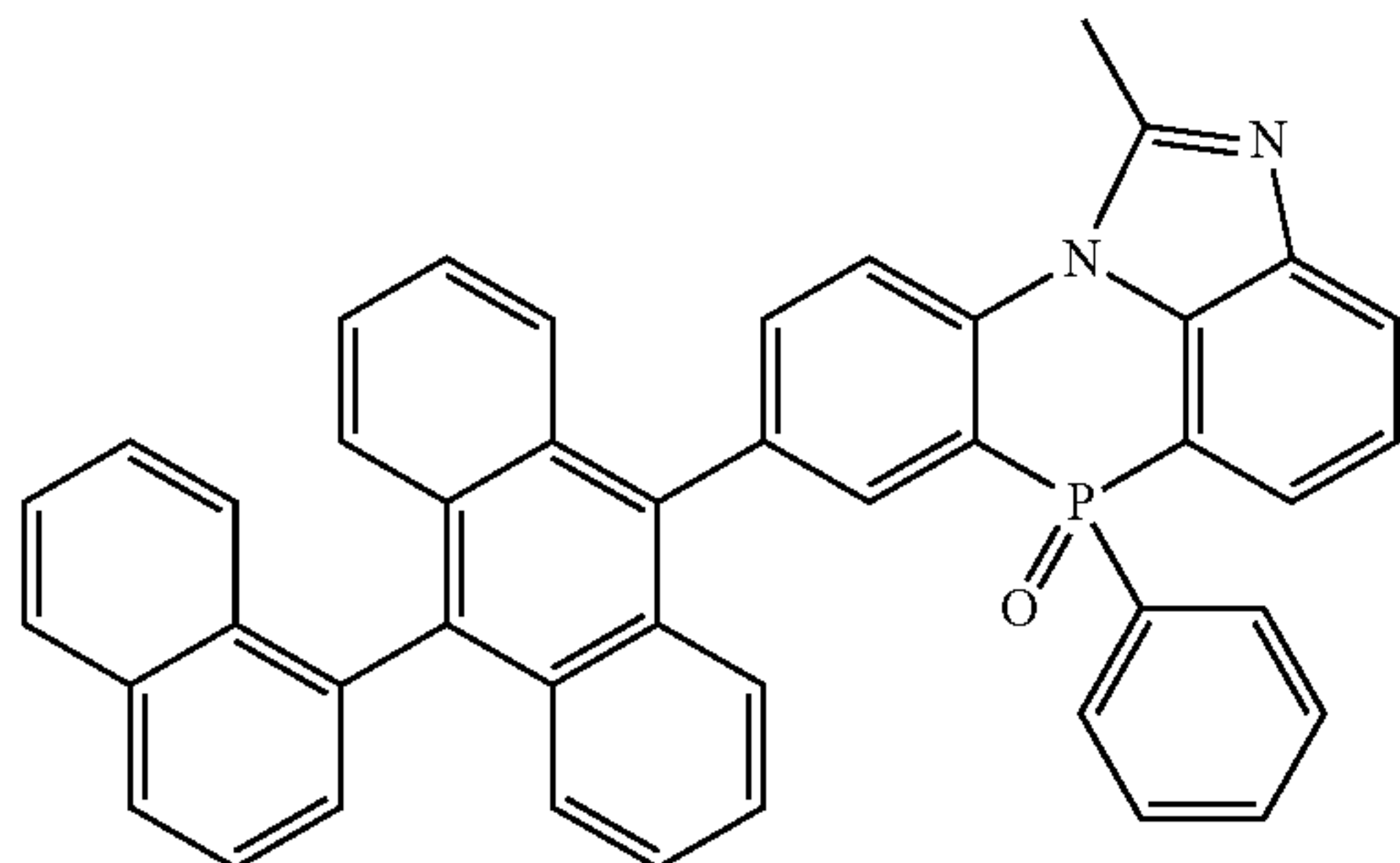
[Chemical Formula 2-2-3]
