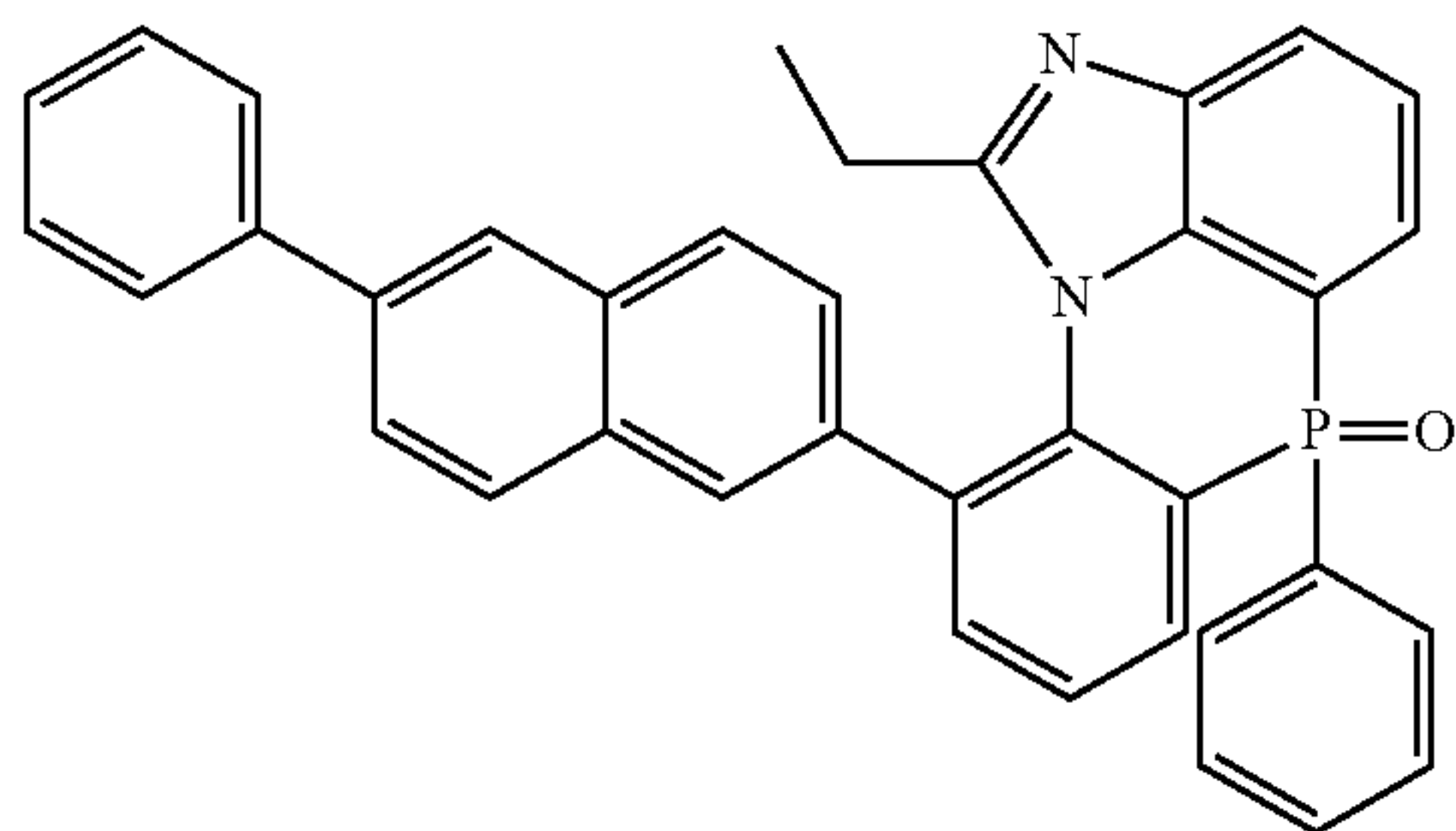
[Chemical Formula 2-8-27]
