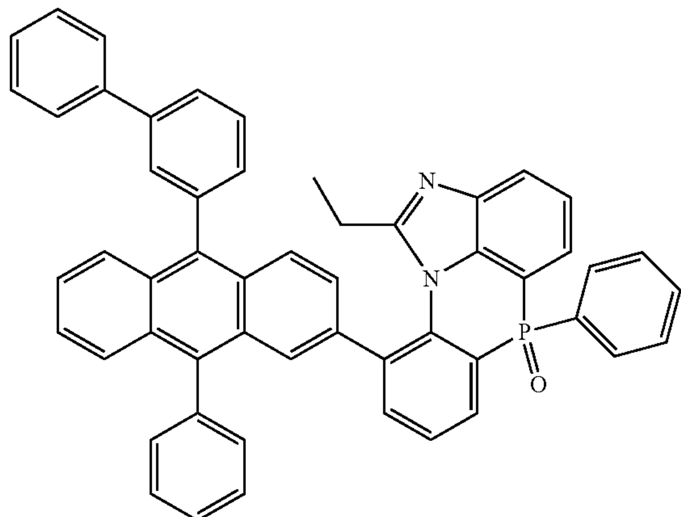
[Chemical Formula 2-8-24]
