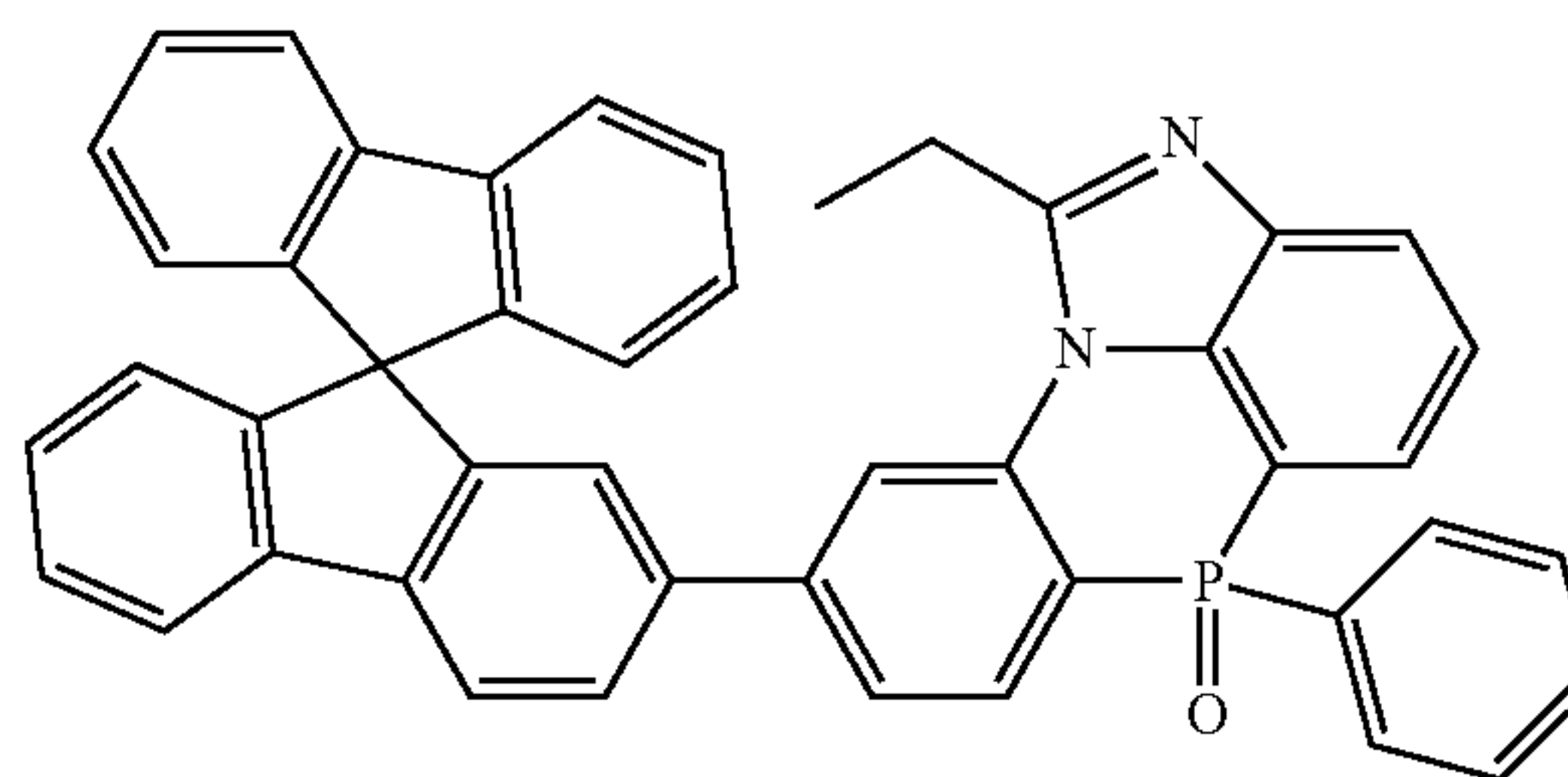
[Chemical Formula 2-7-34]
