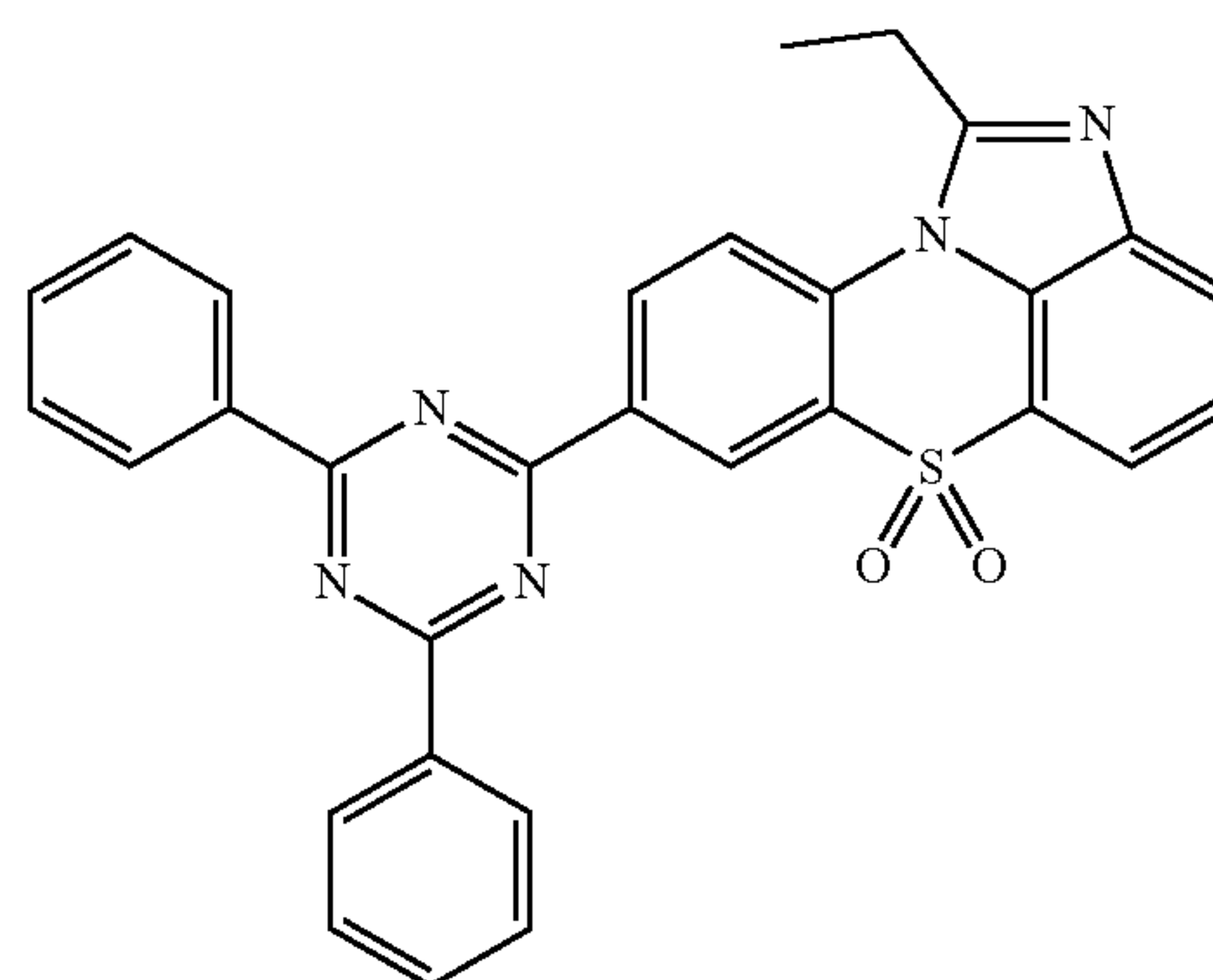
[Chemical Formula 1-3-42]
