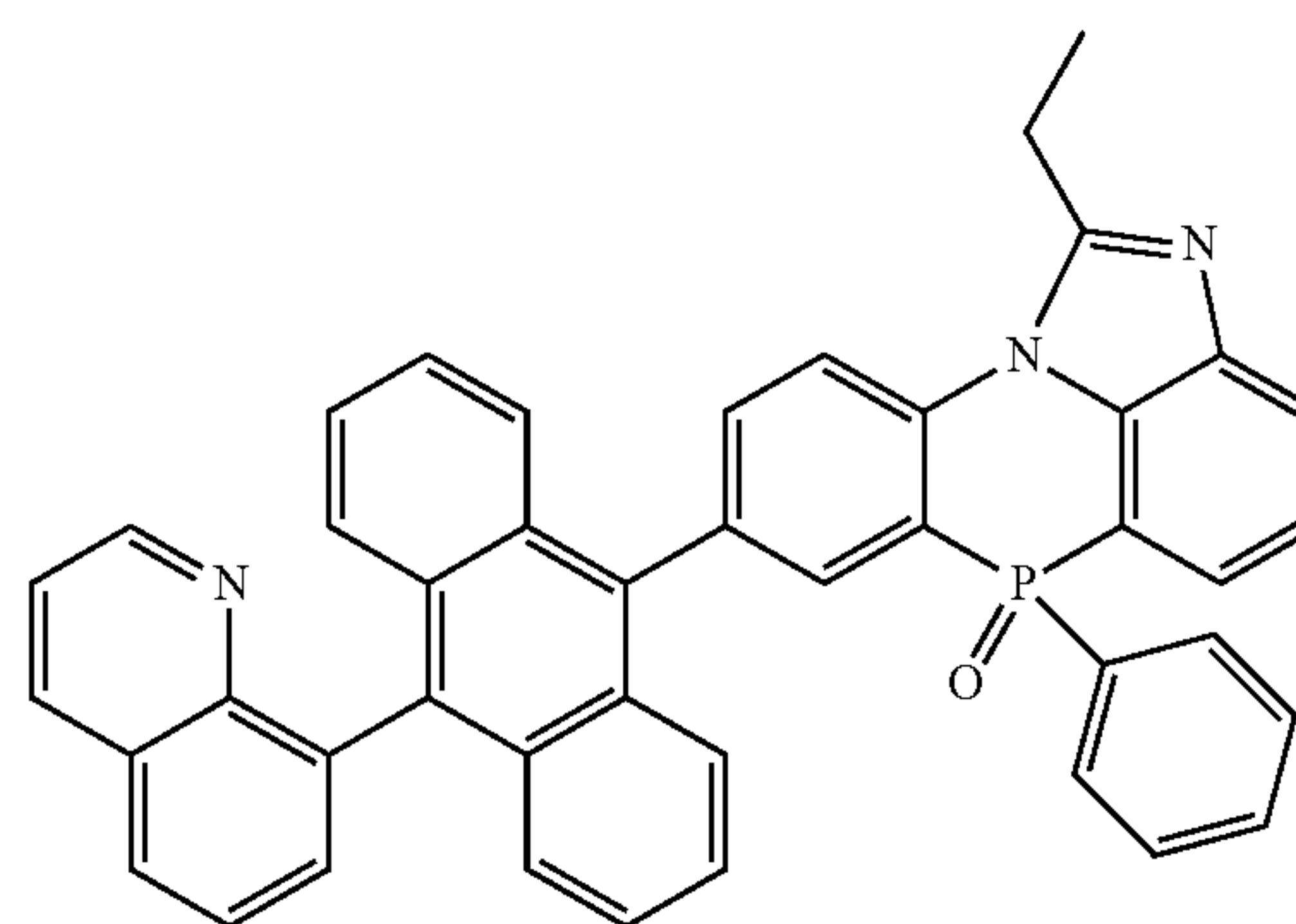
[Chemical Formula 2-3-11]
