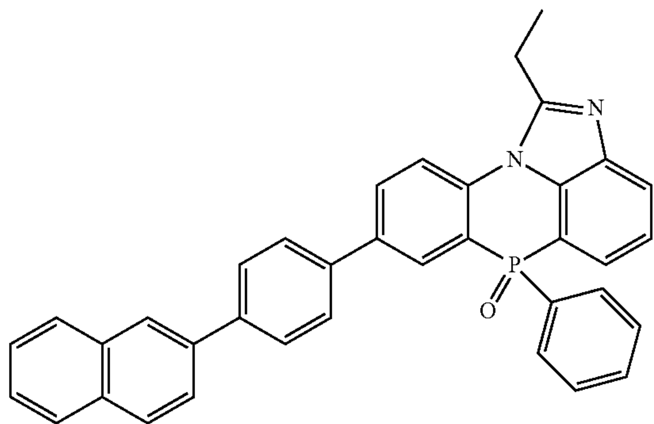
[Chemical Formula 2-3-26]
