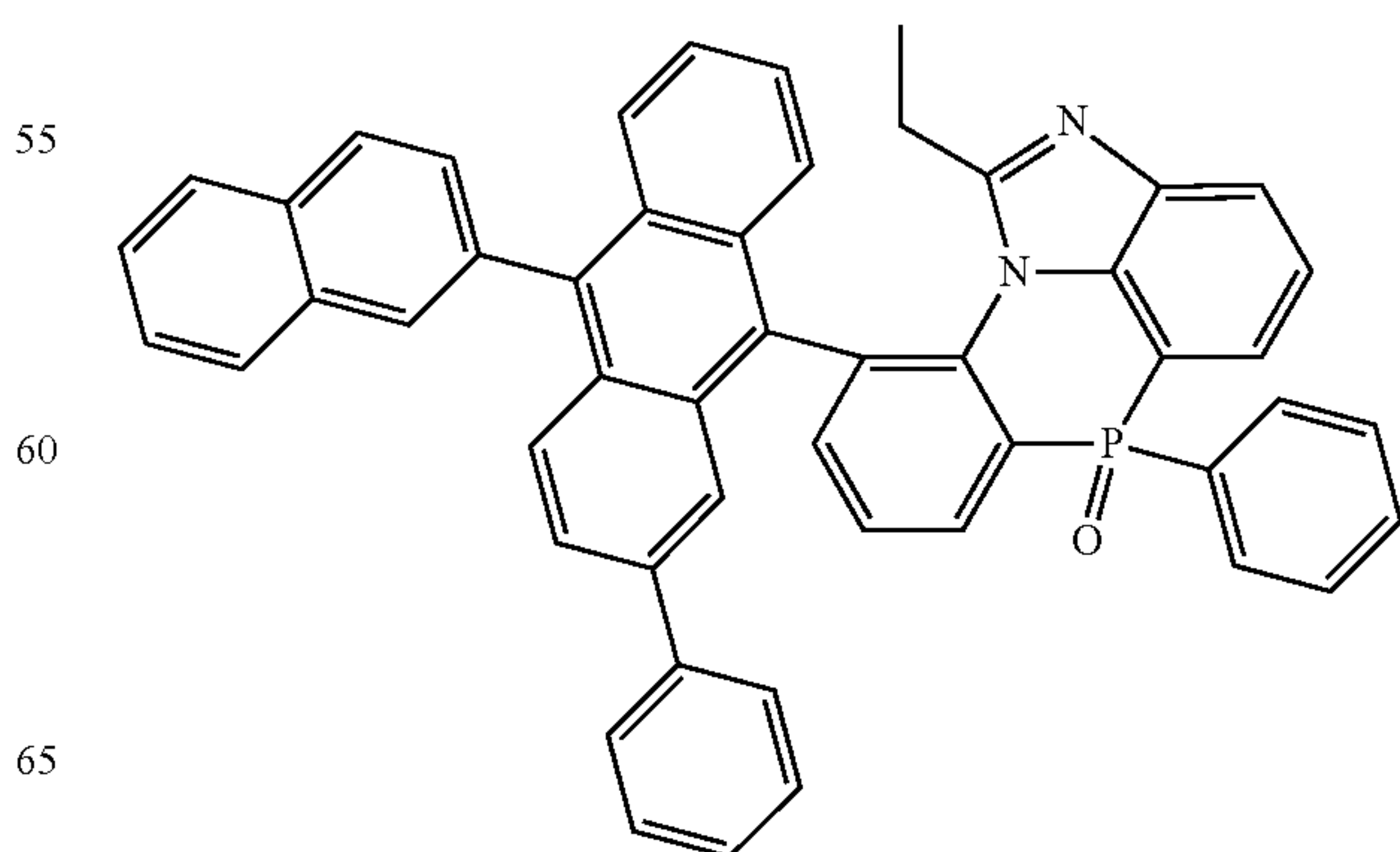
[Chemical Formula 2-8-16]
