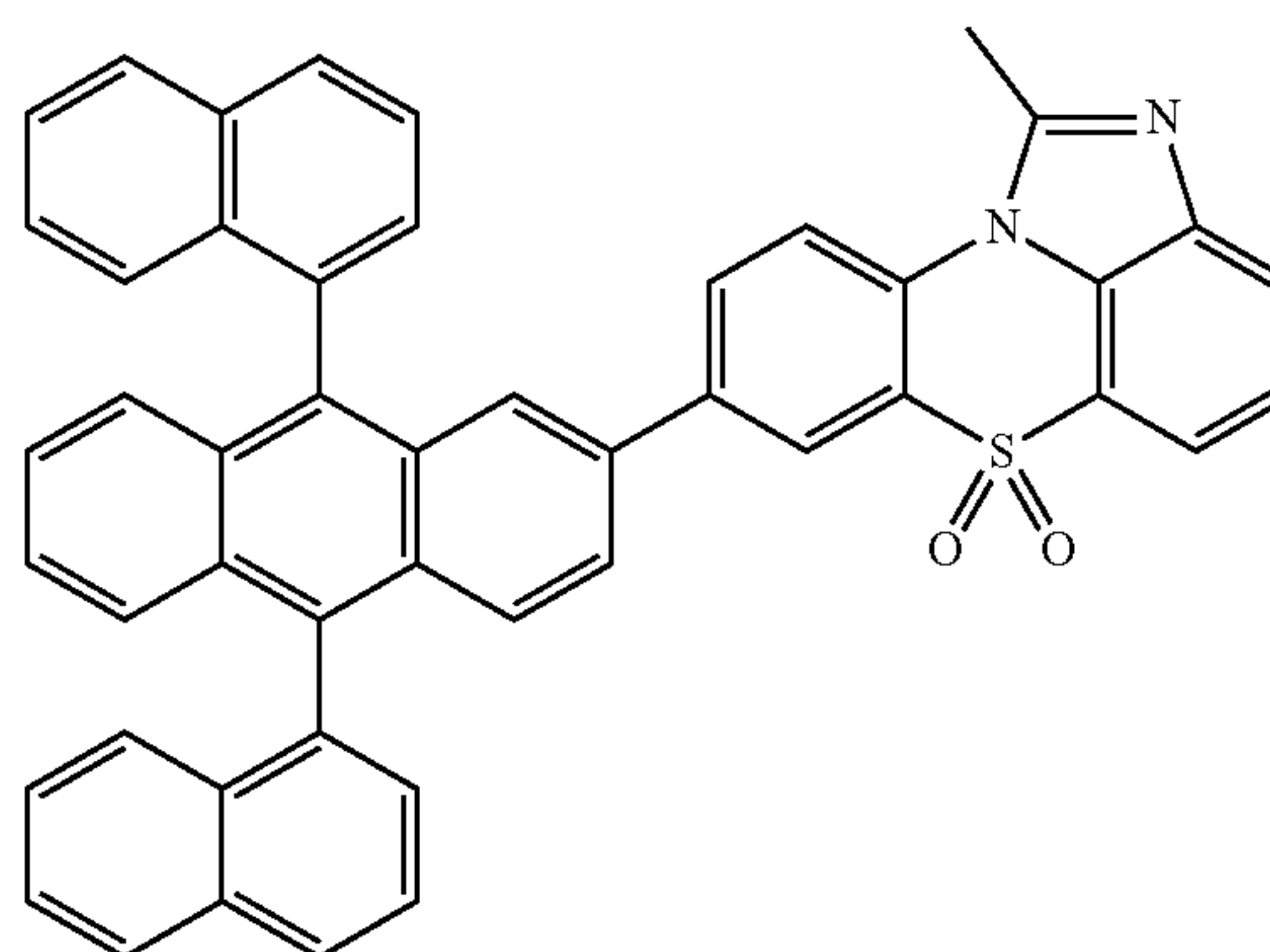
[Chemical Formula 1-2-21]
