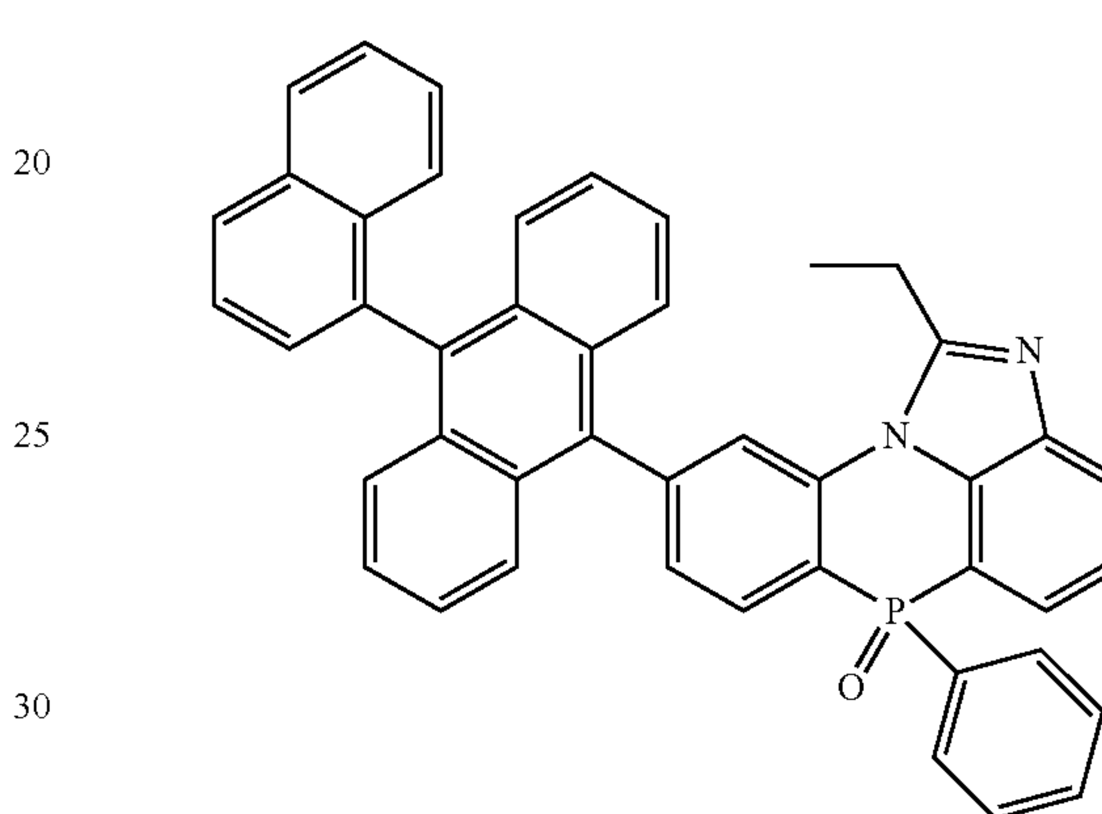
[Chemical Formula 2-7-4]
