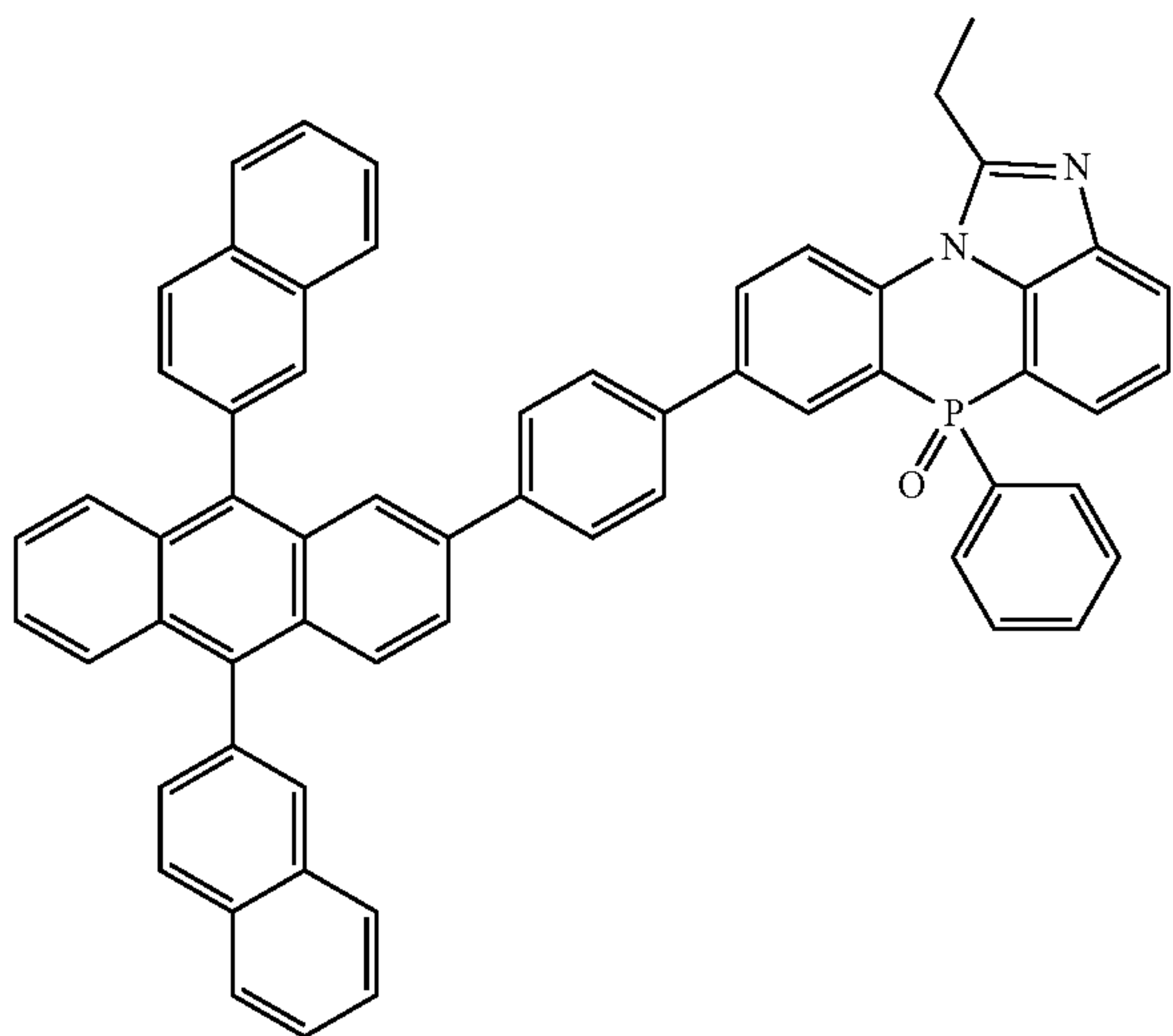
[Chemical Formula 2-3-25]
