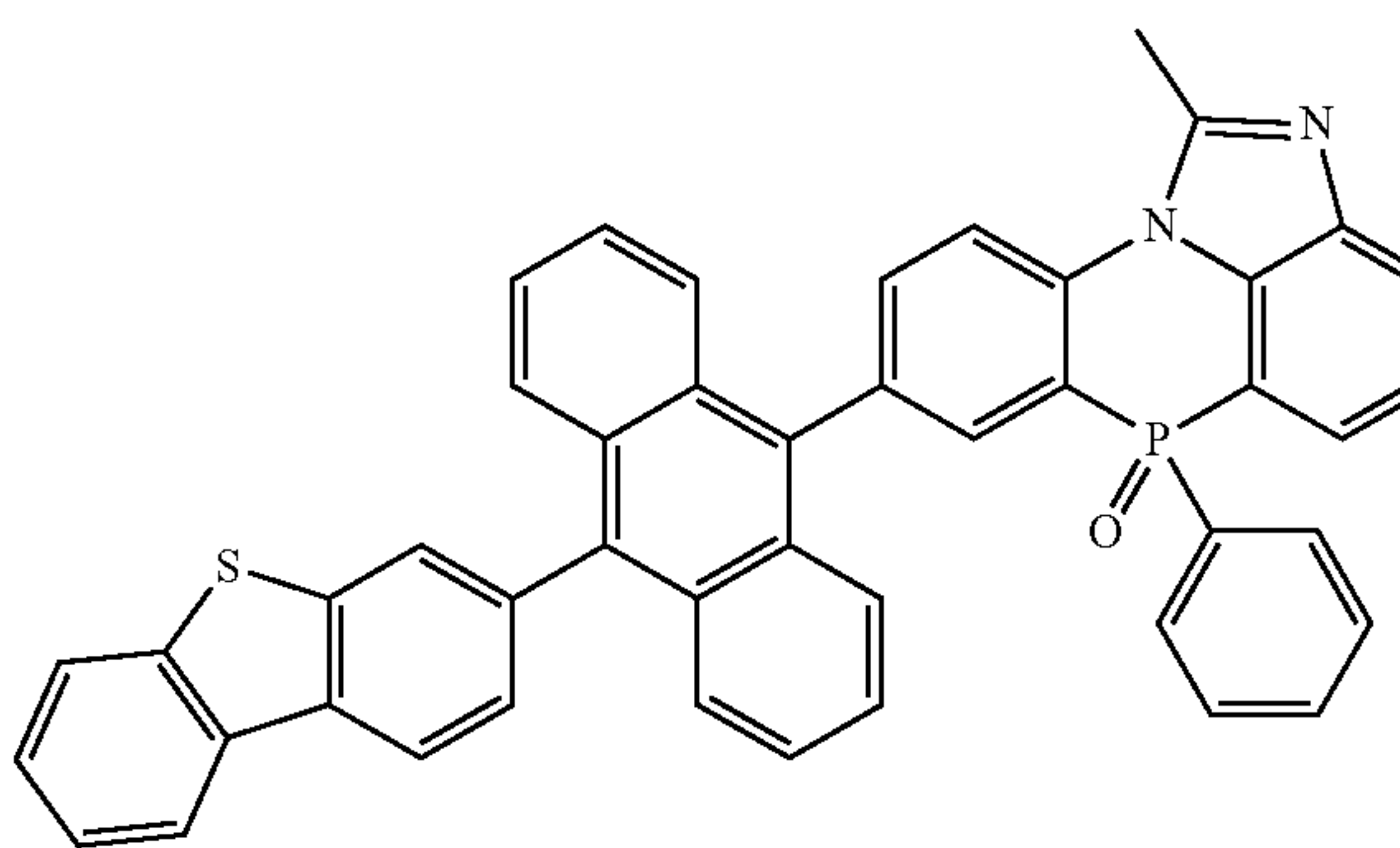
[Chemical Formula 2-2-14]
