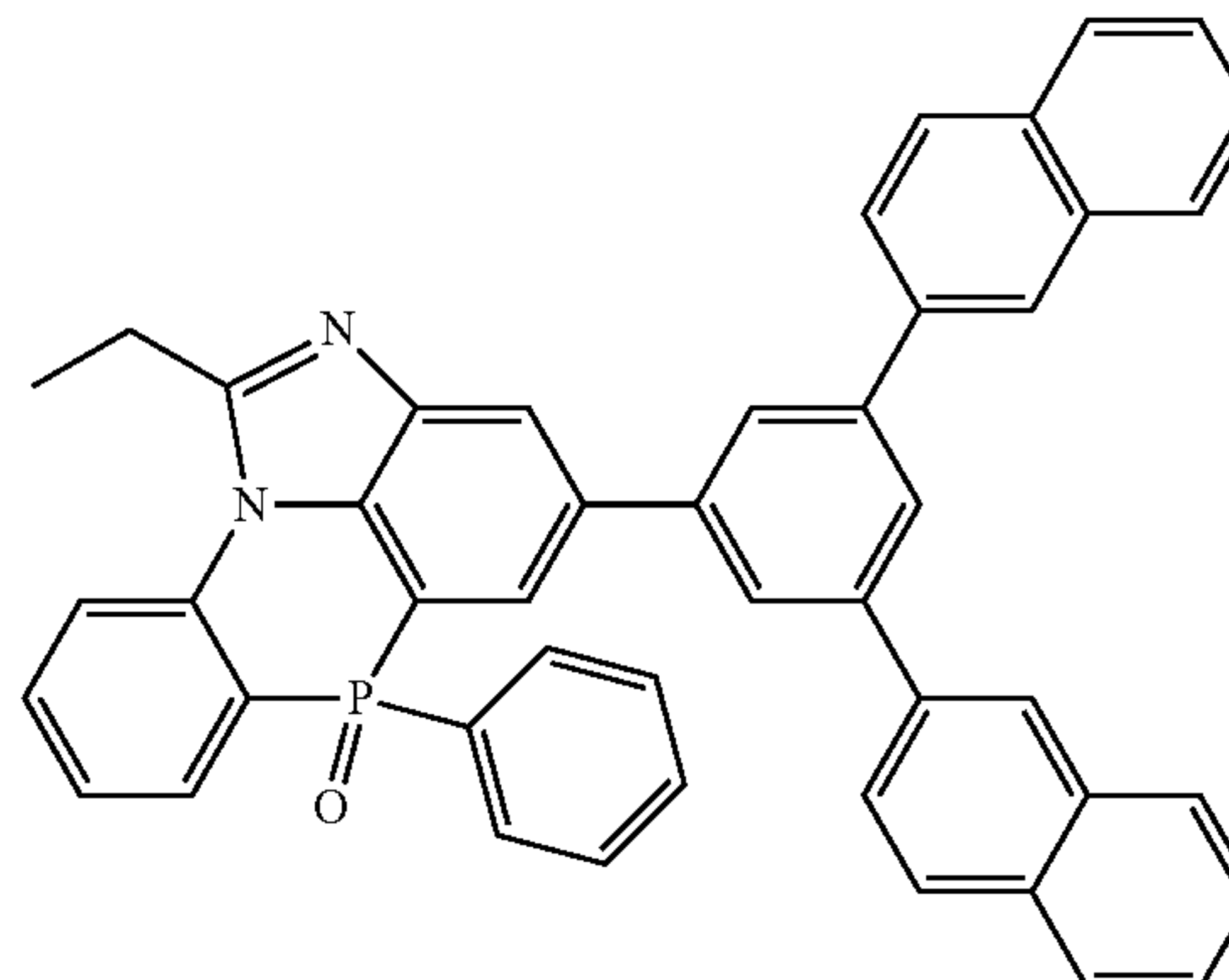
[Chemical Formula 2-10-7]
