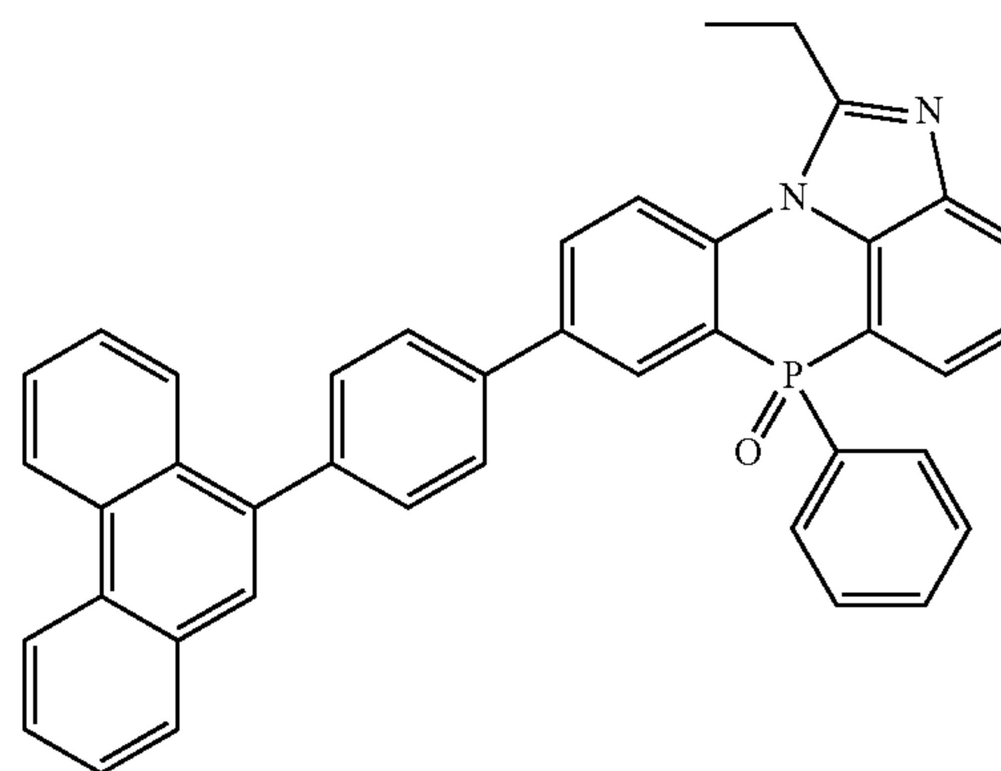
[Chemical Formula 2-3-32]
