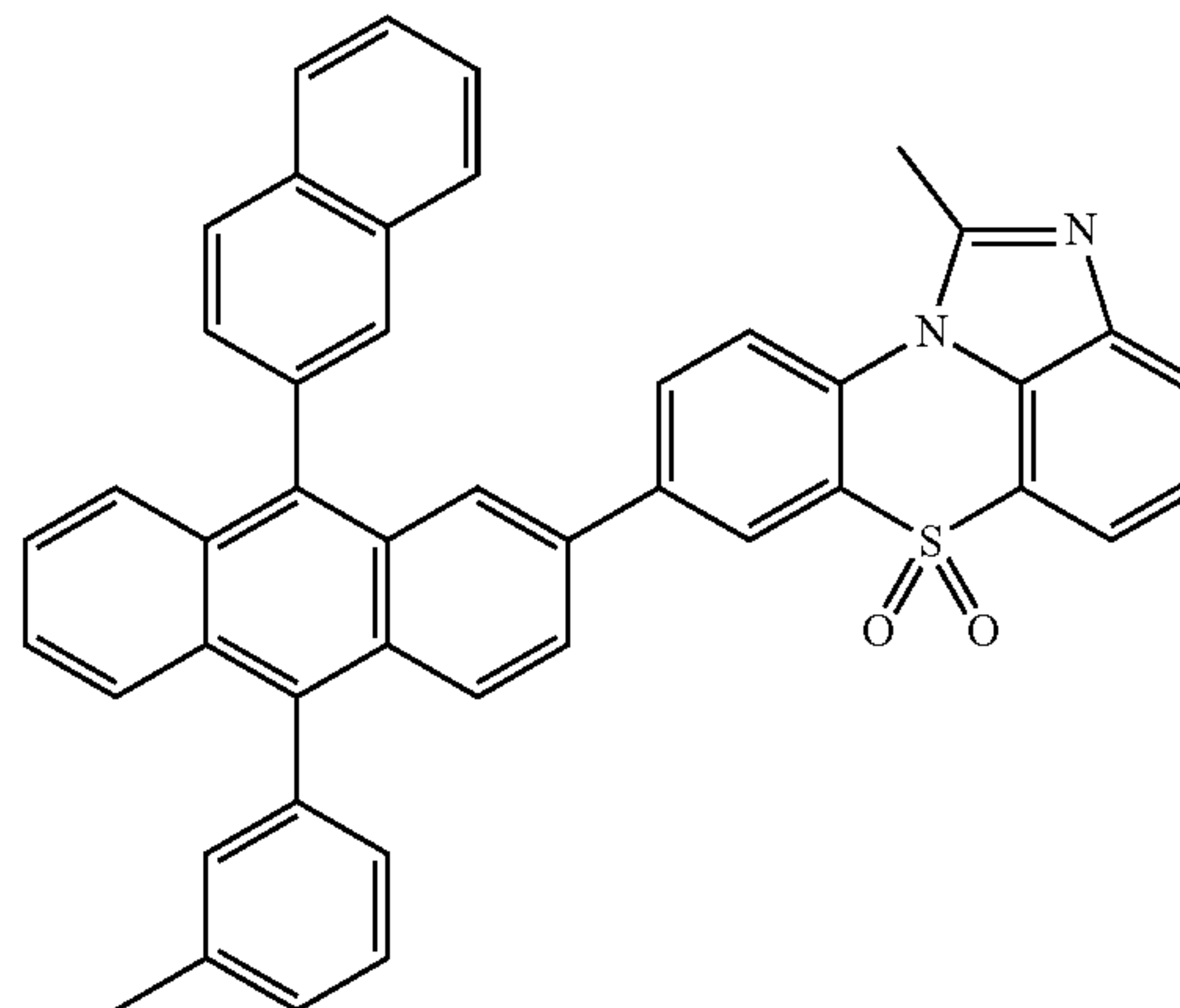
[Chemical Formula 1-2-20]
