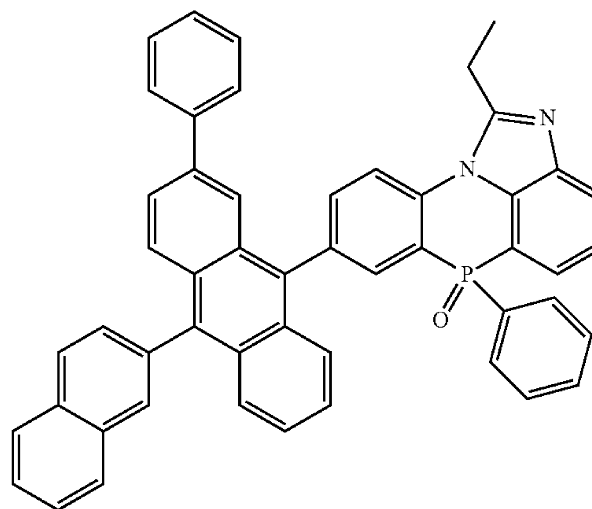
[Chemical Formula 2-3-16]
