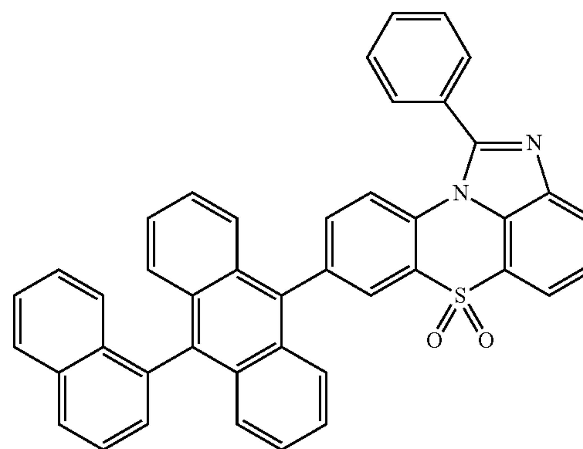
[Chemical Formula 1-4-3]
