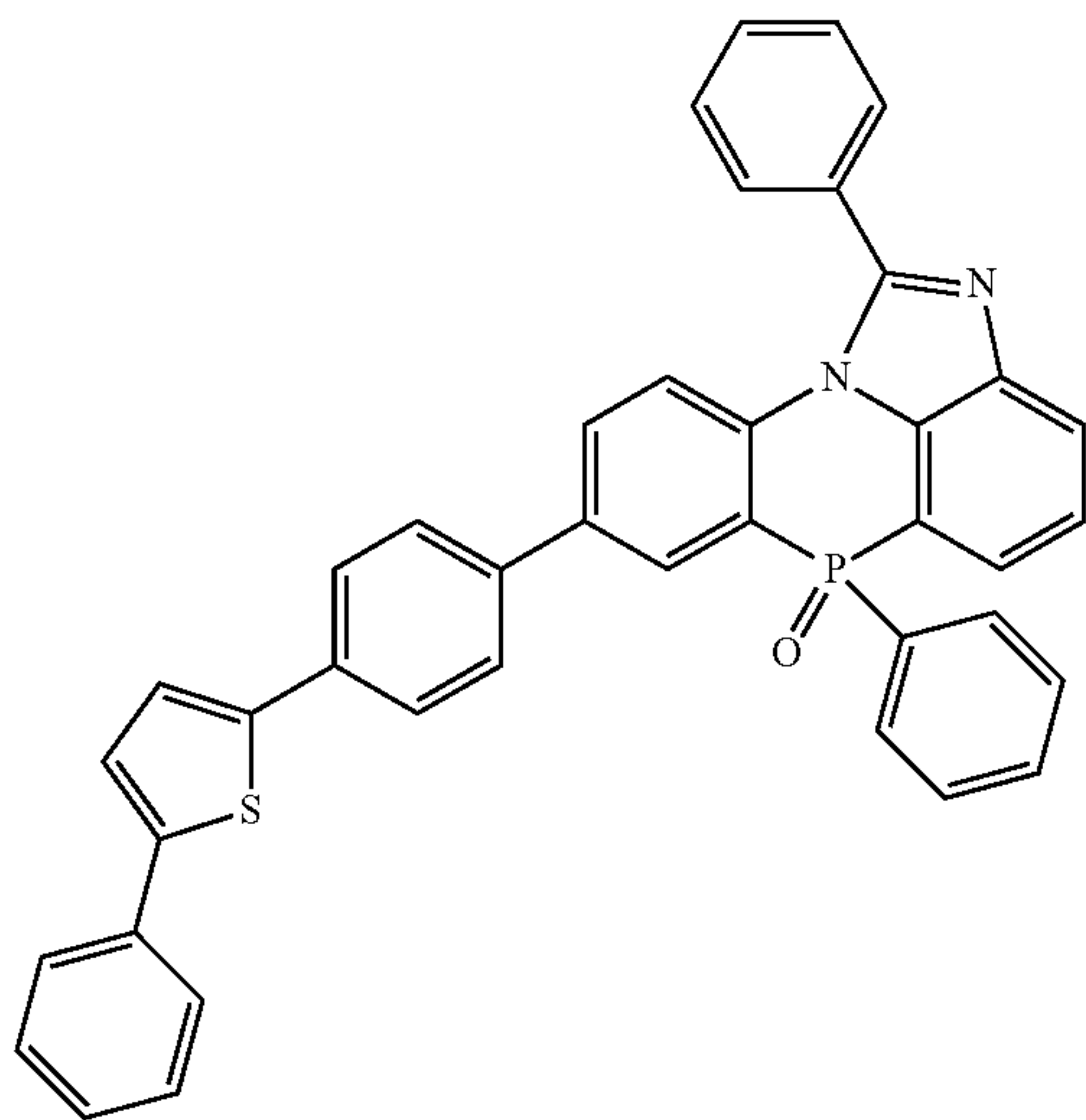
[Chemical Formula 2-4-39]
