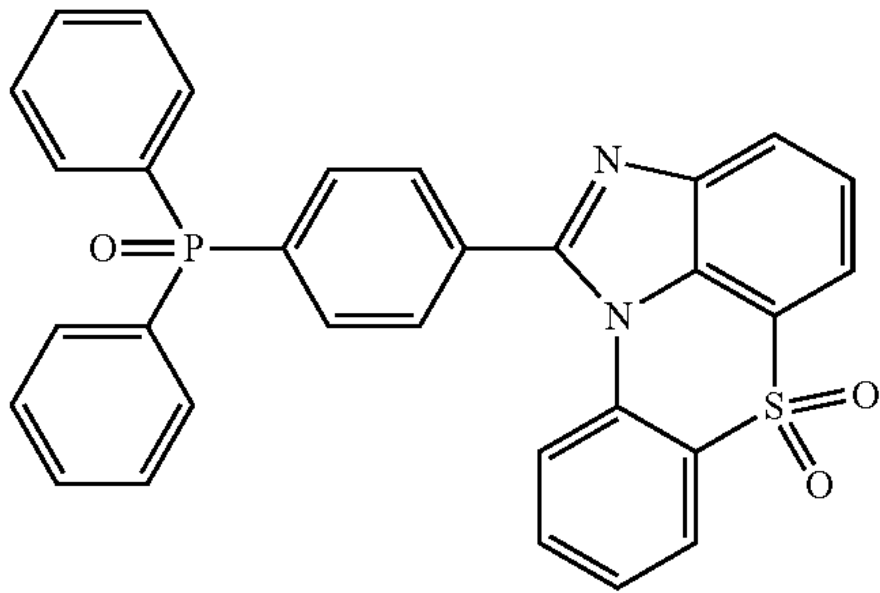
[Chemical Formula 1-12-4]
