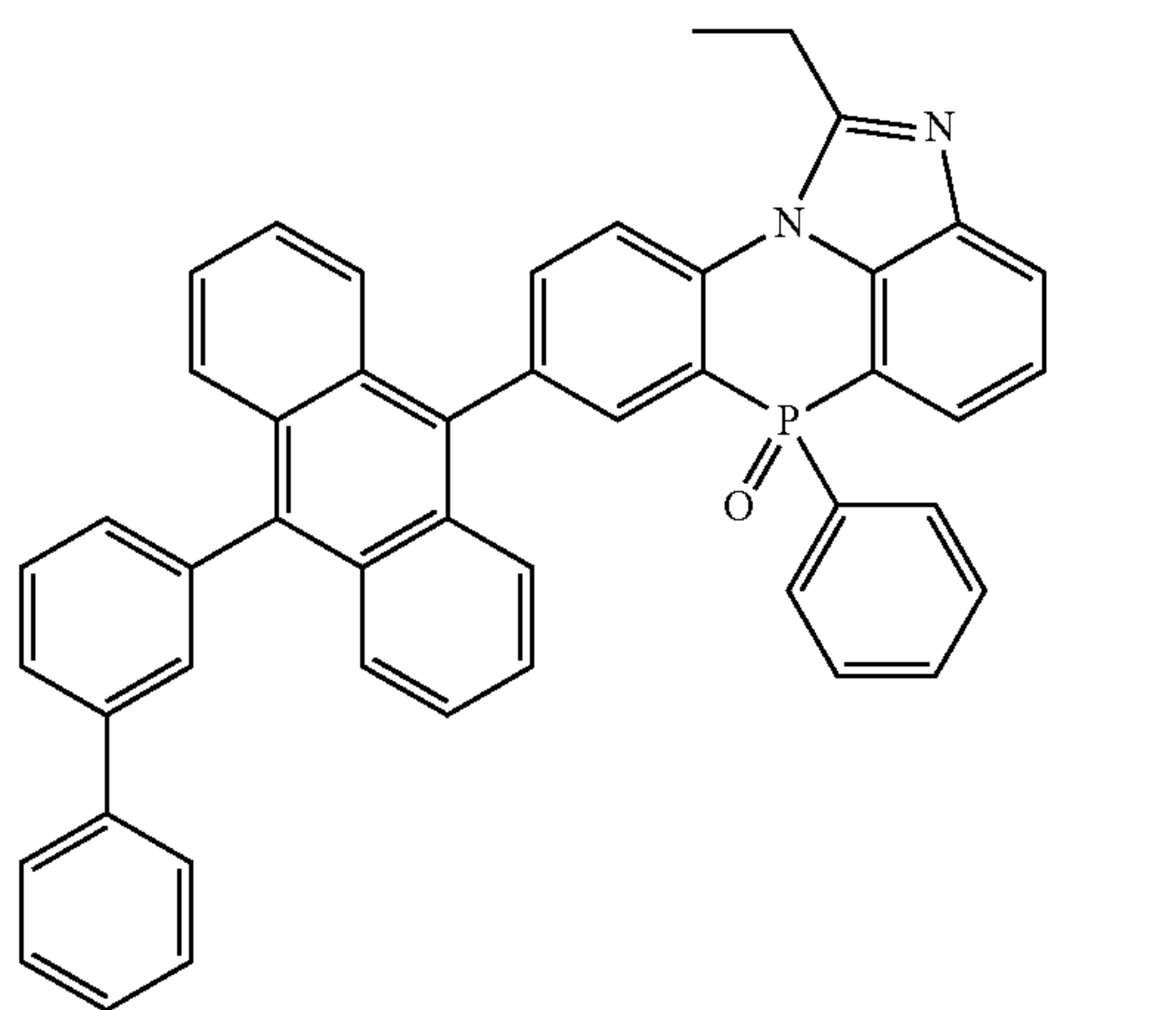
[Chemical Formula 2-3-7]
