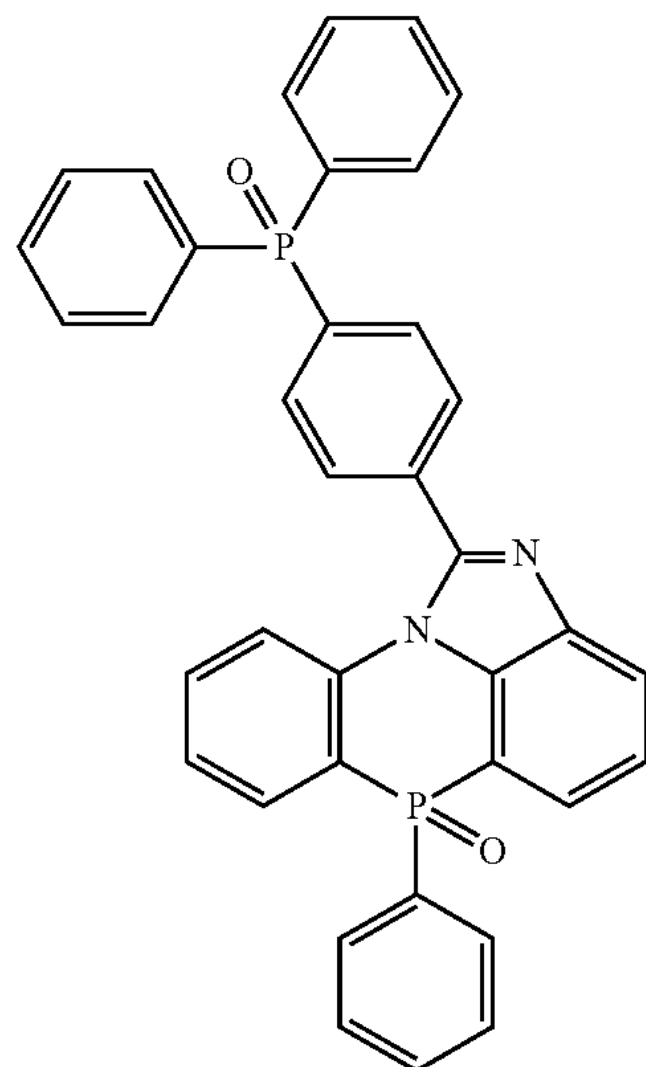
[Chemical Formula 2-12-3]
