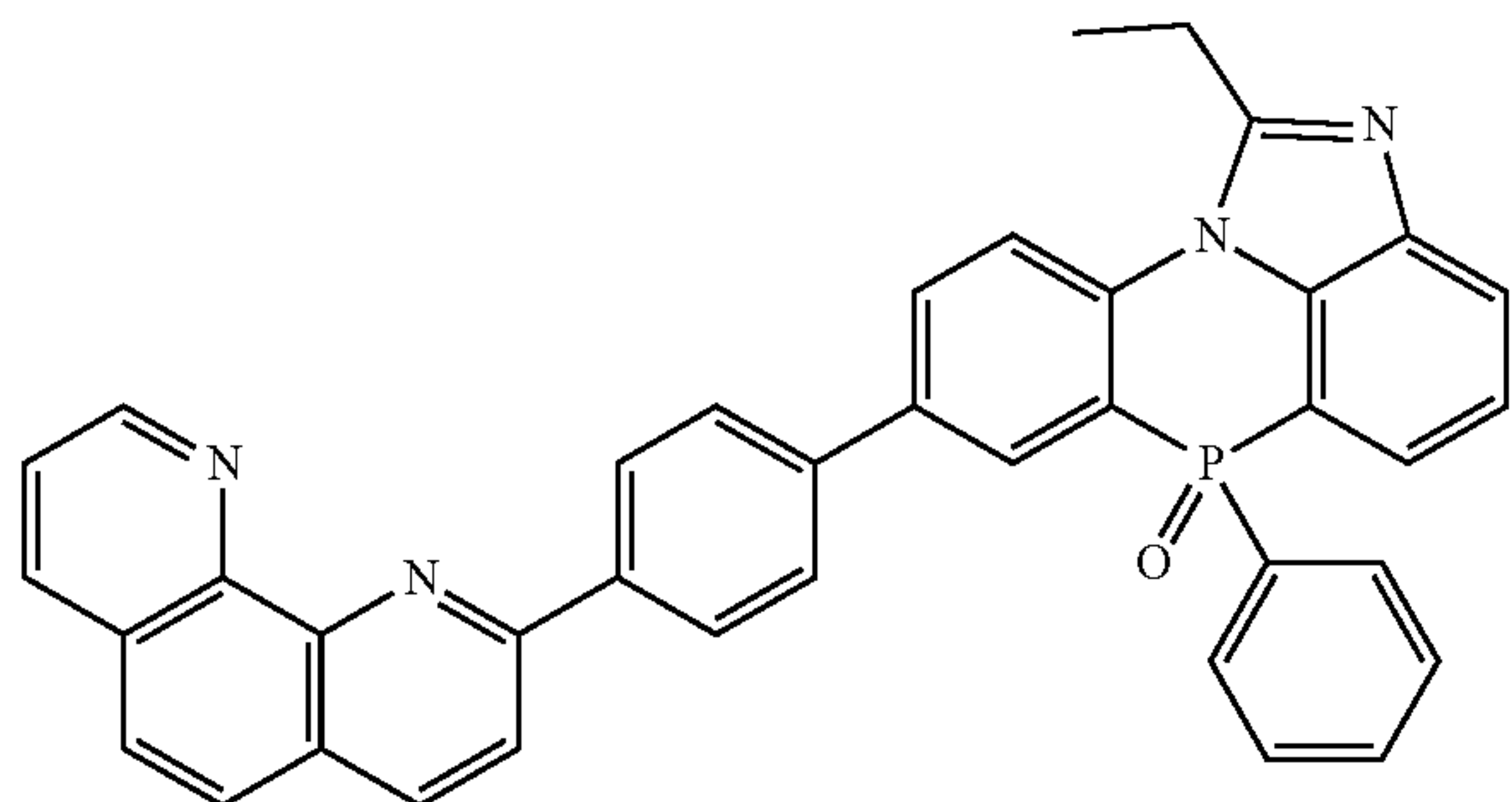
[Chemical Formula 2-3-47]
