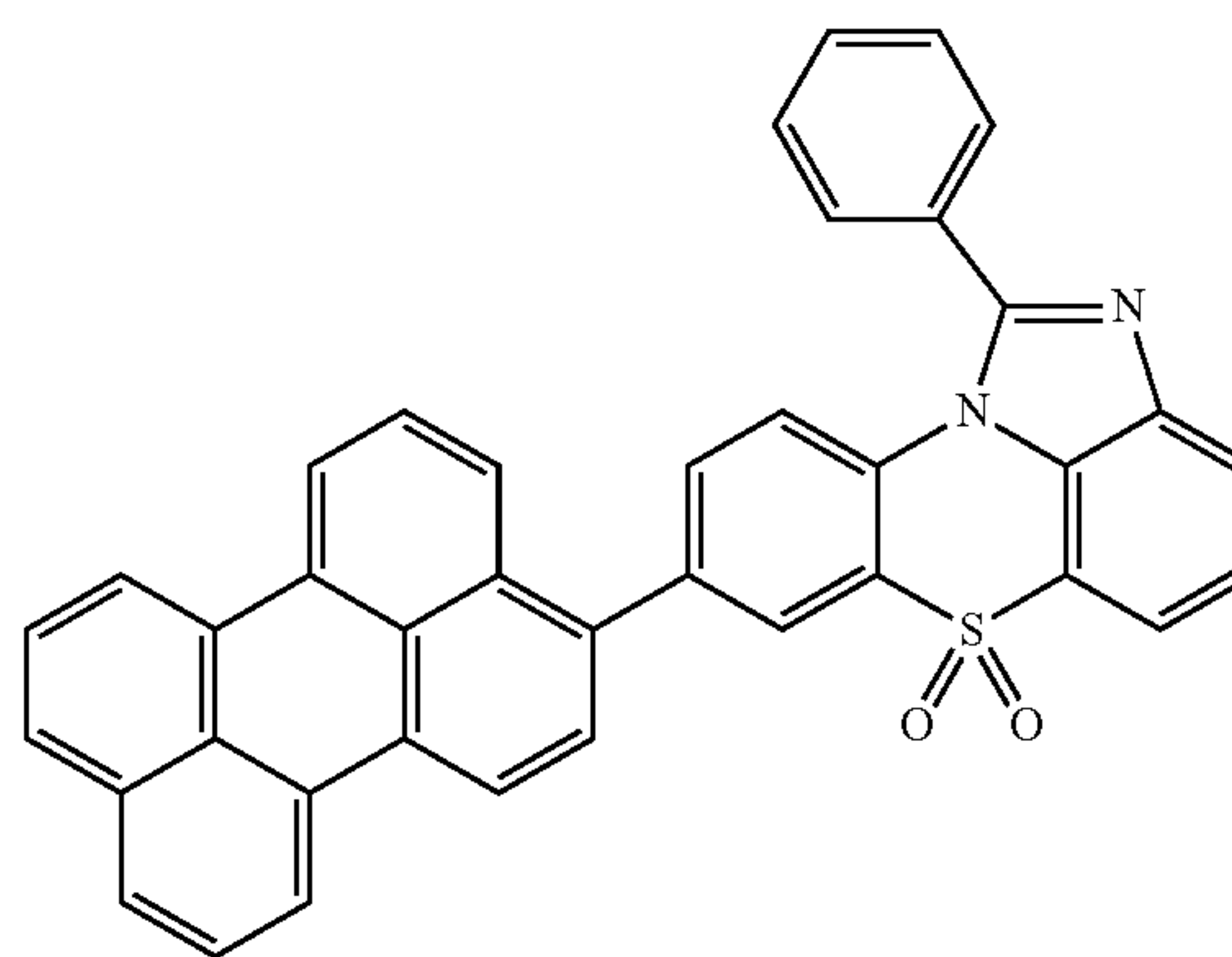
[Chemical Formula 1-4-29]
