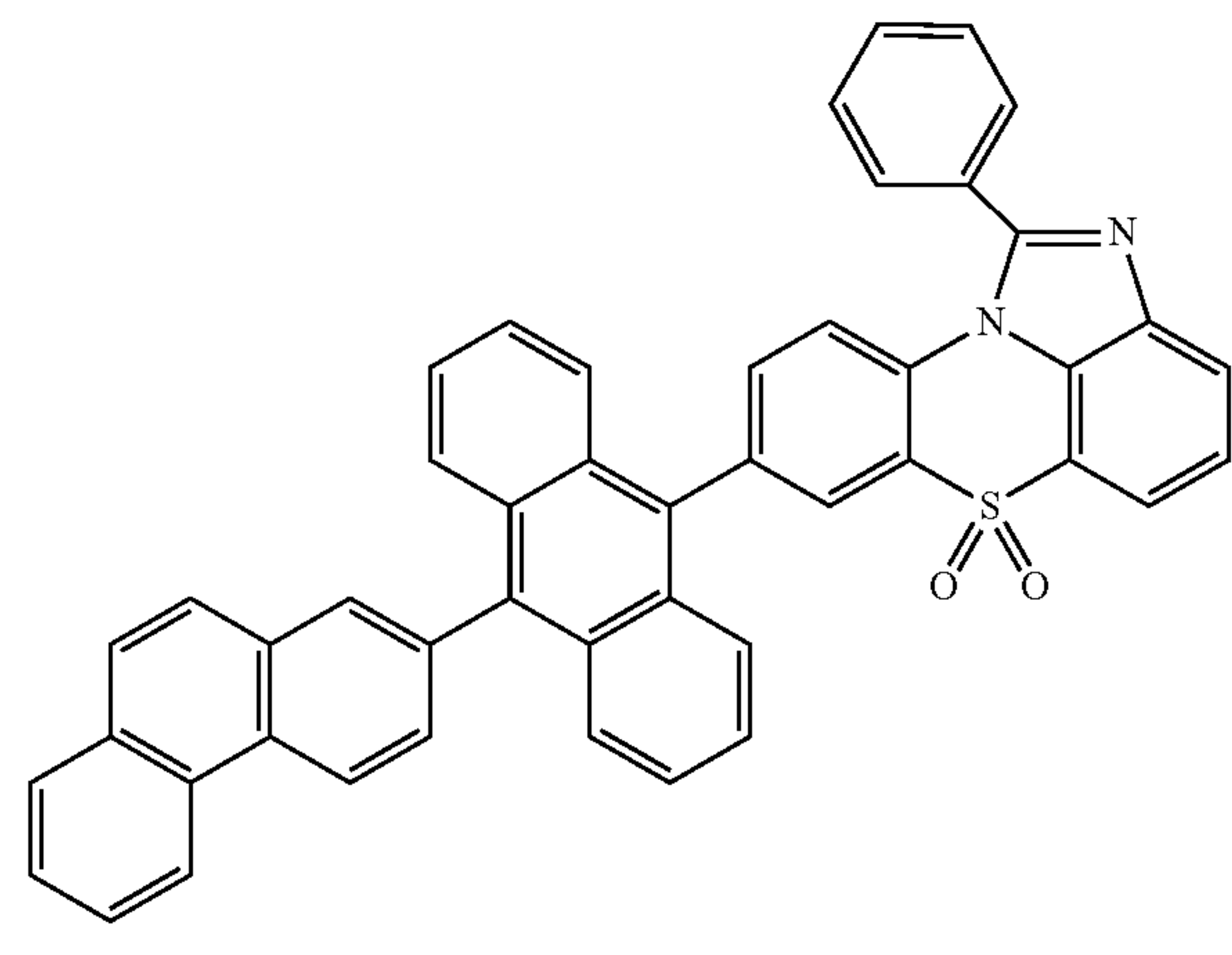
[Chemical Formula 1-4-9]
