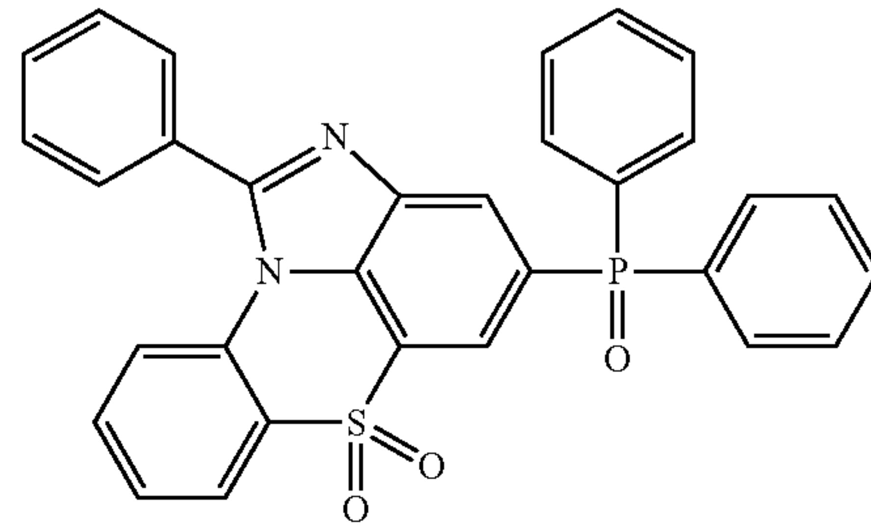
[Chemical Formula 1-12-8]
