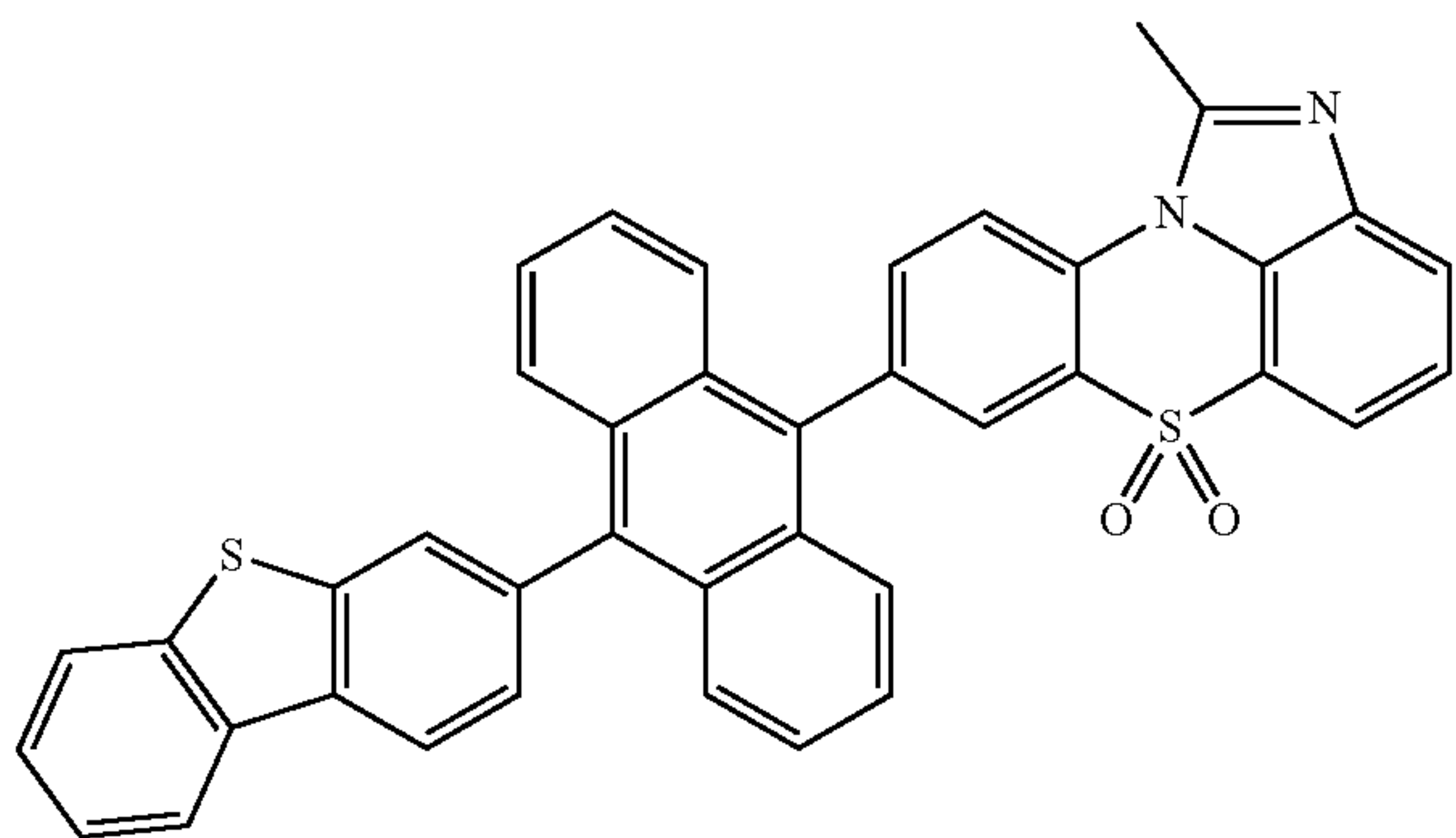
[Chemical Formula 1-2-14]
