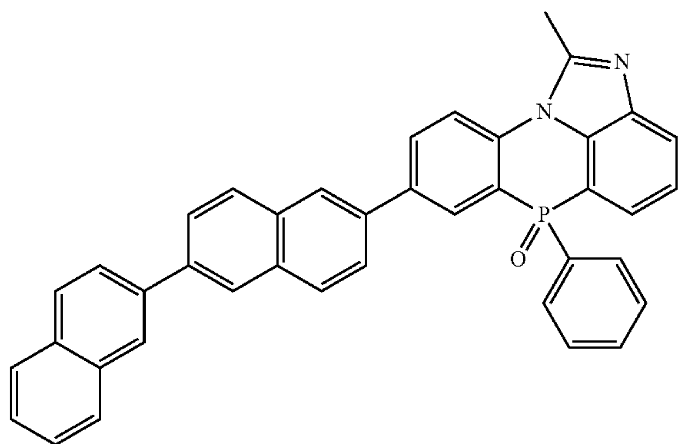
[Chemical Formula 2-2-45]
