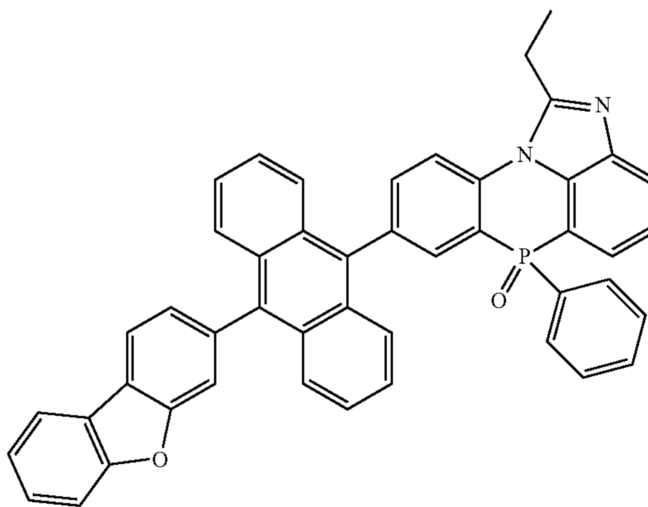
[Chemical Formula 2-3-13]
