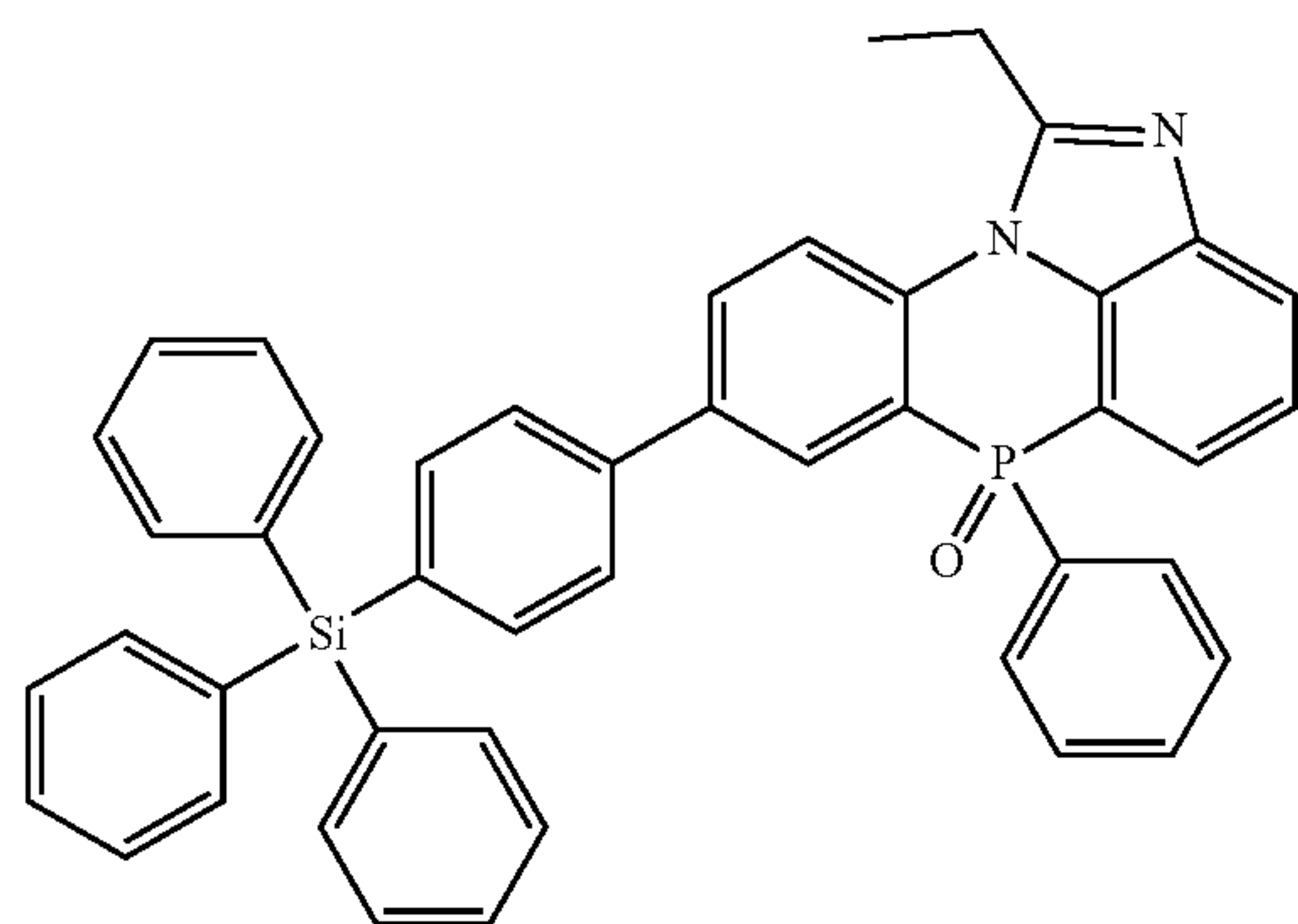
[Chemical Formula 2-3-48]
