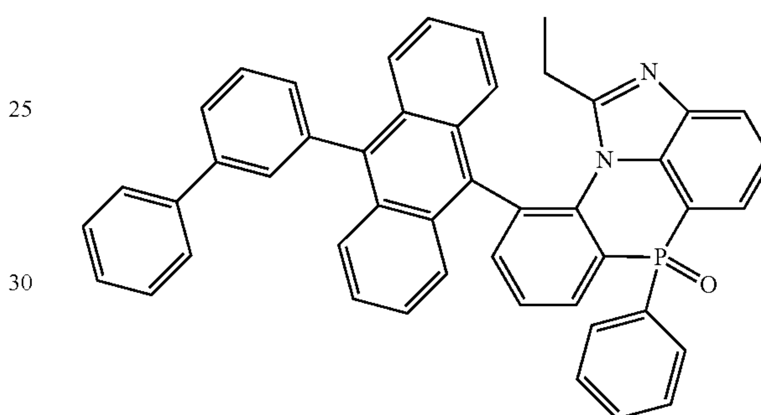
[Chemical Formula 2-8-6]
