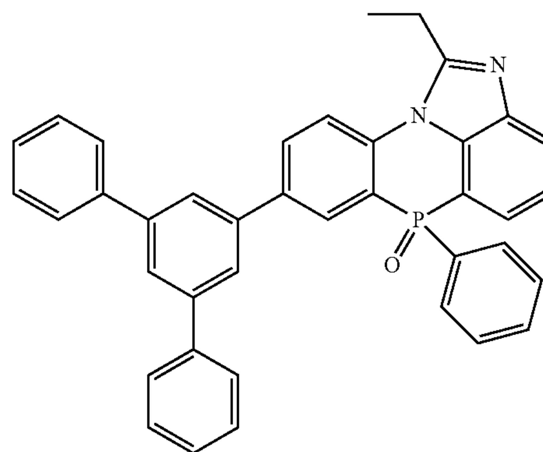
[Chemical Formula 2-3-41]
