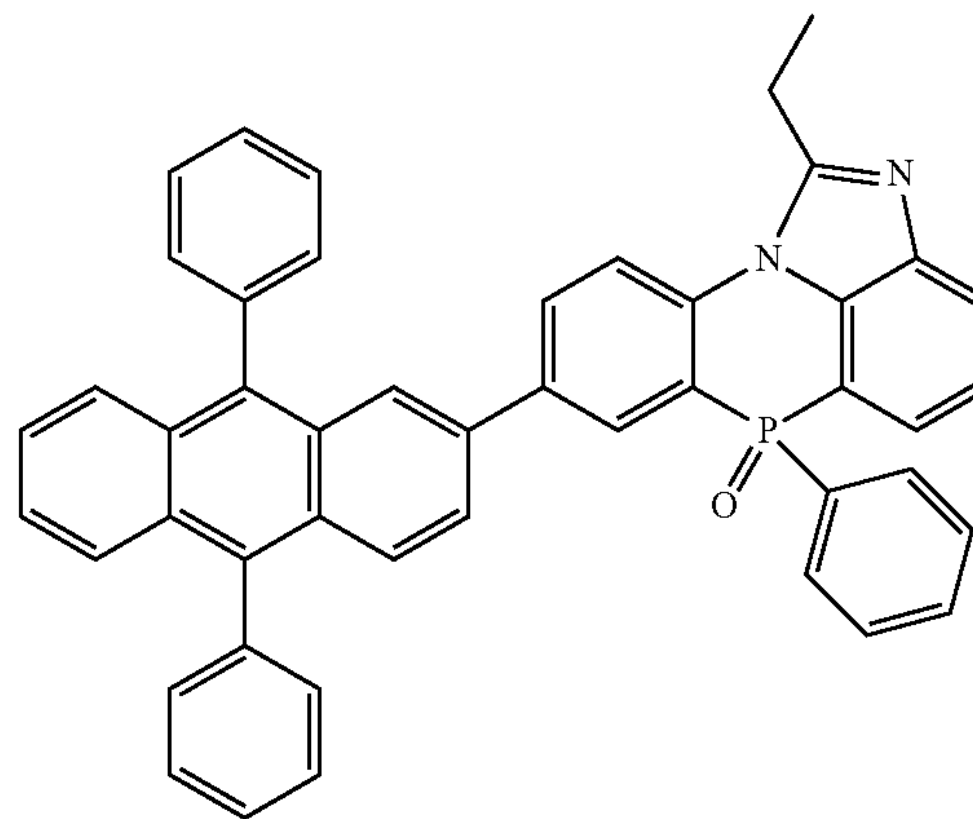
[Chemical Formula 2-3-19]
