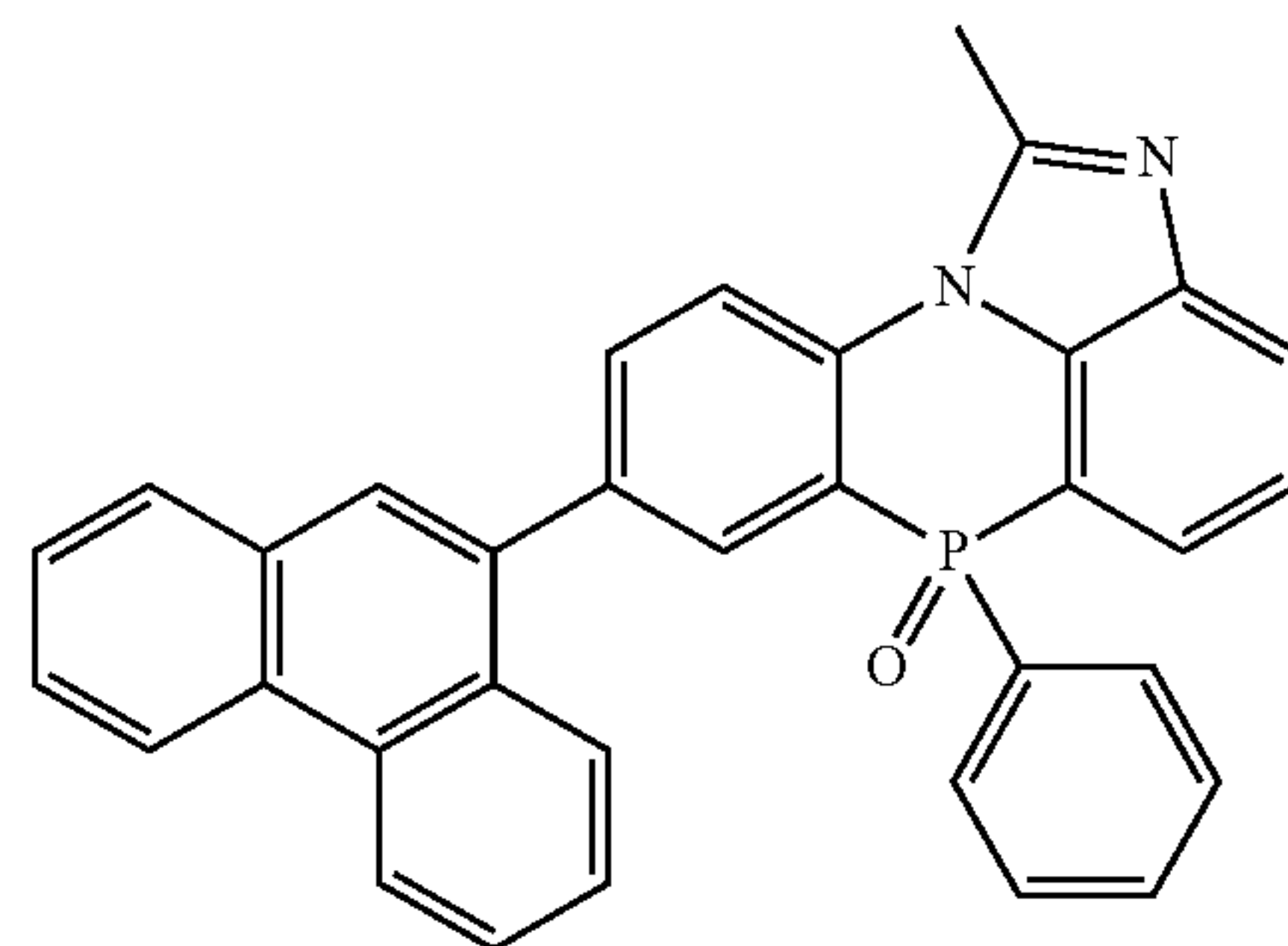
[Chemical Formula 2-2-31]
