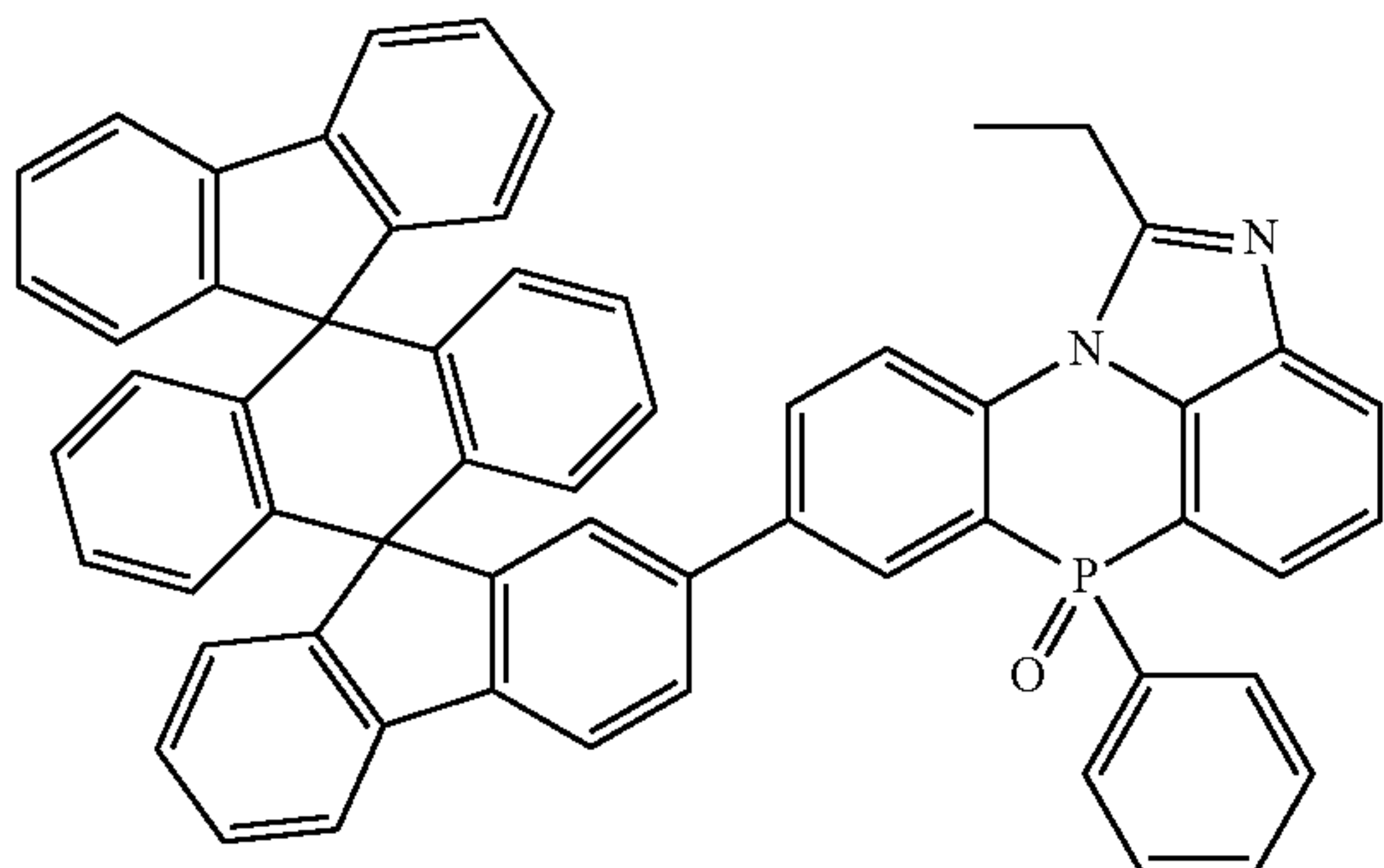
[Chemical Formula 2-3-36]
