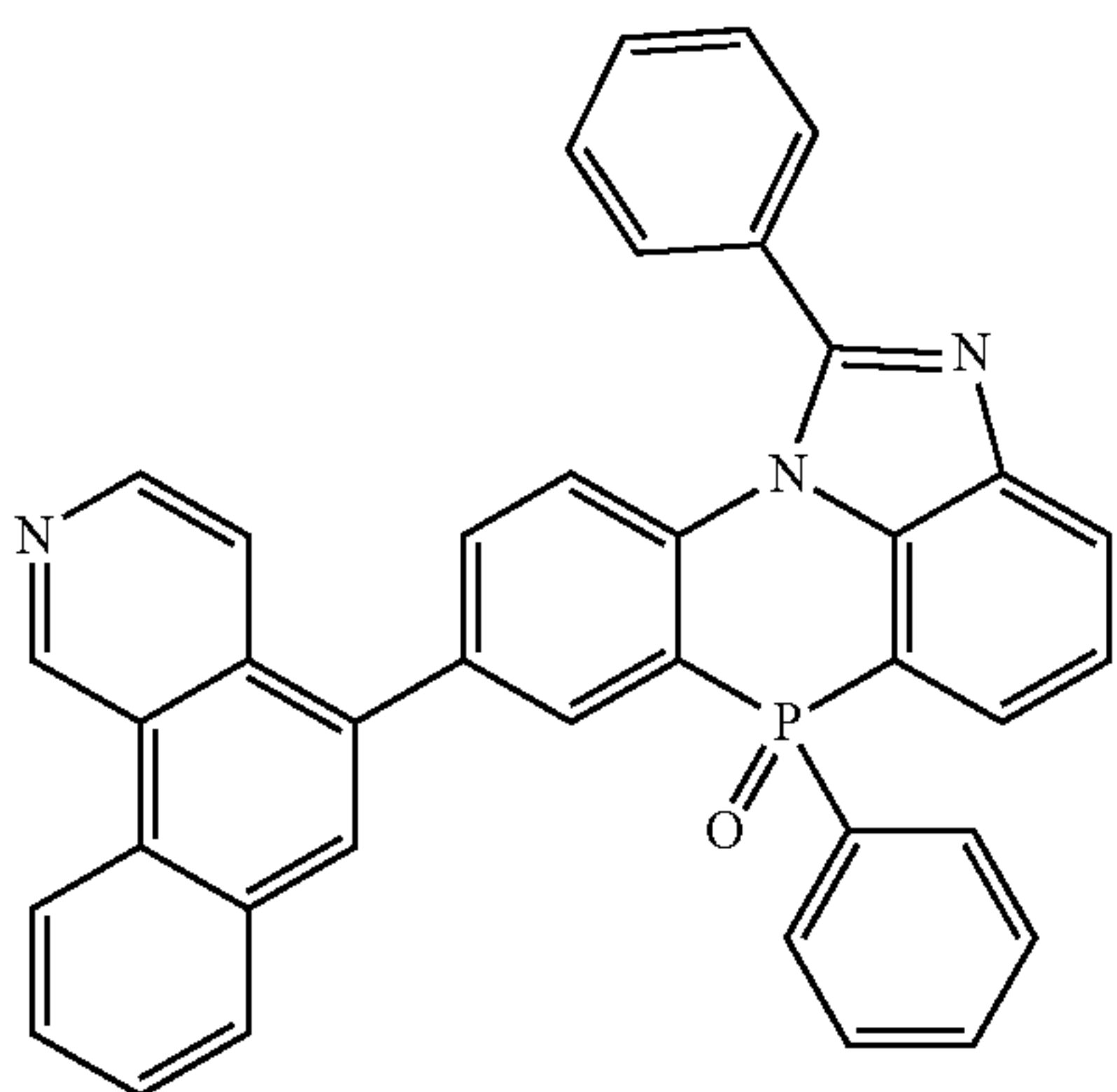
[Chemical Formula 2-4-34]
