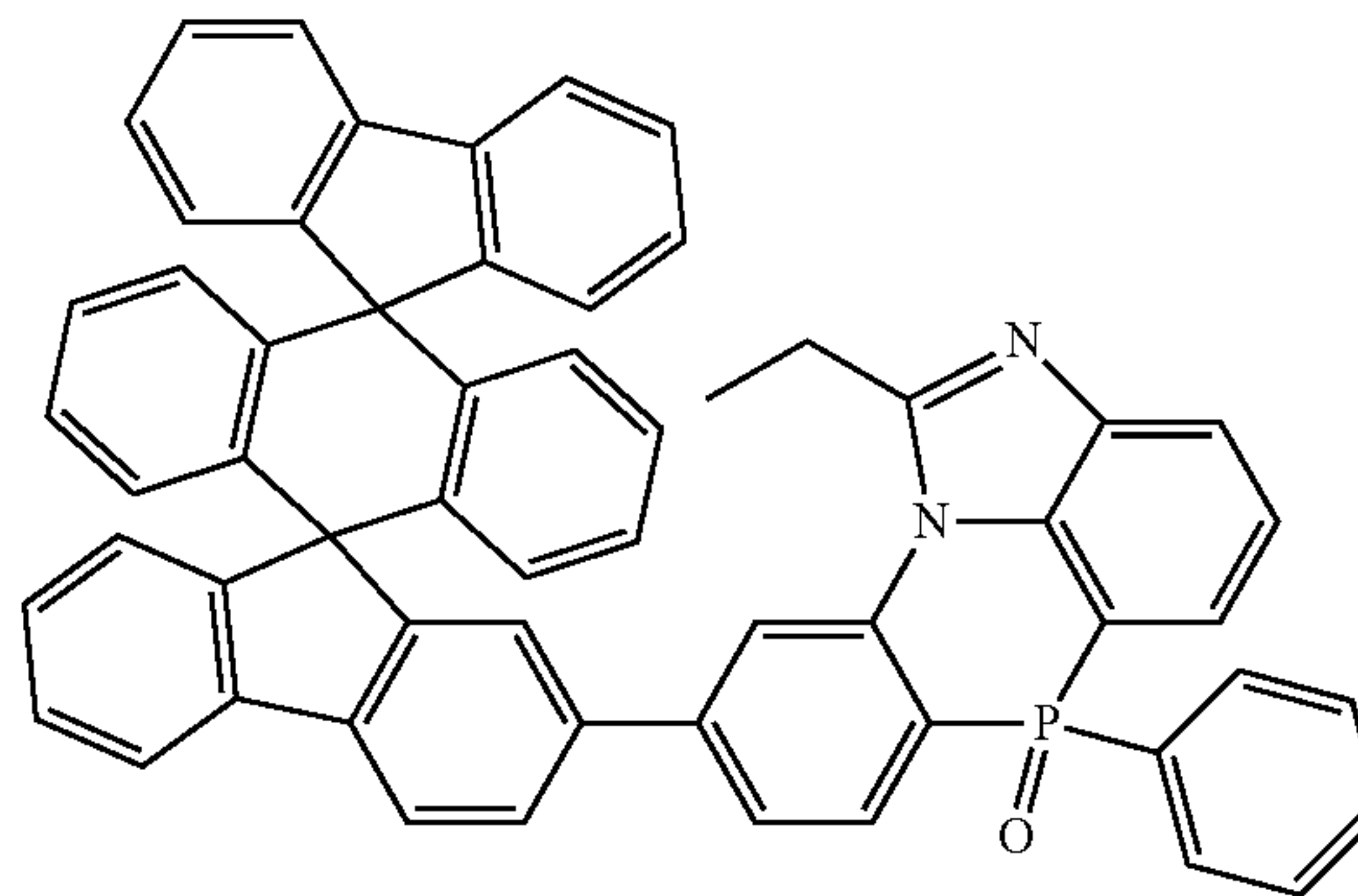
[Chemical Formula 2-7-36]
