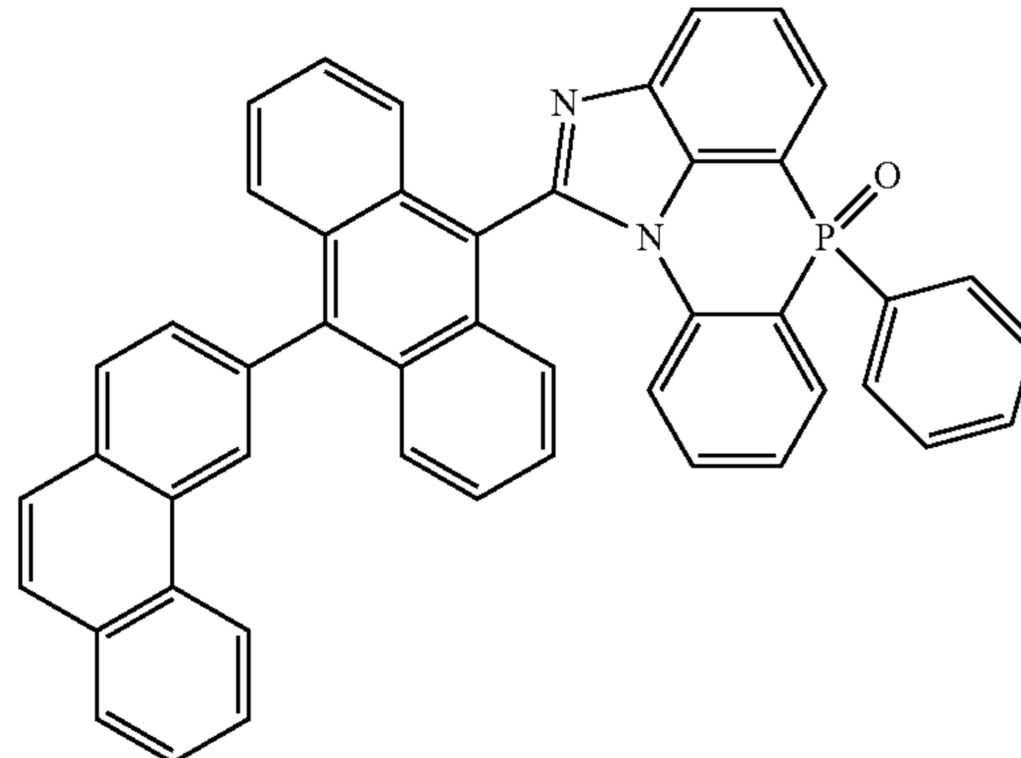
[Chemical Formula 2-5-9]
