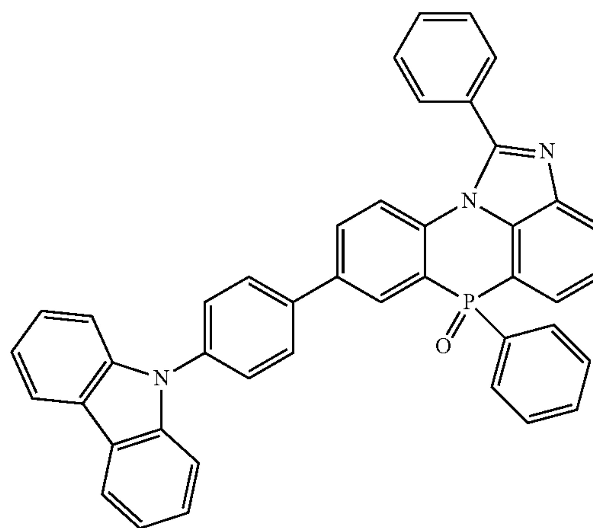
[Chemical Formula 2-4-42]
