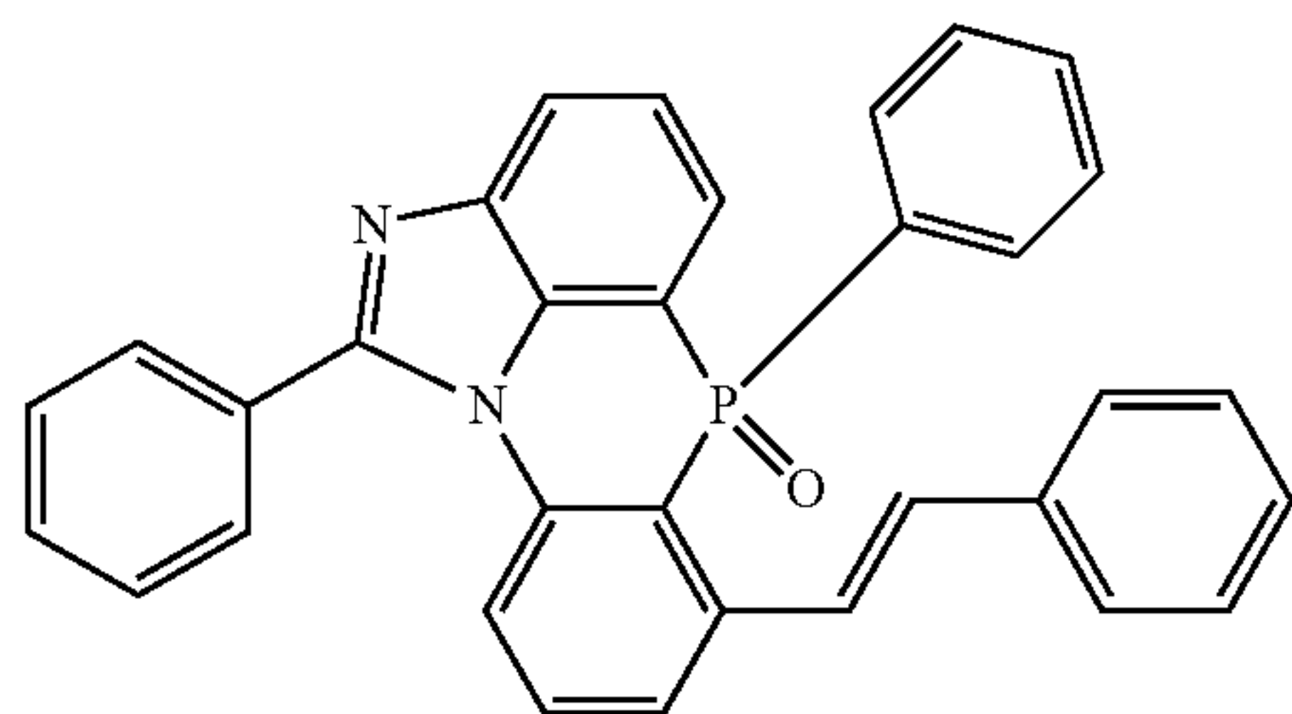
[Chemical Formula 2-7-1]
