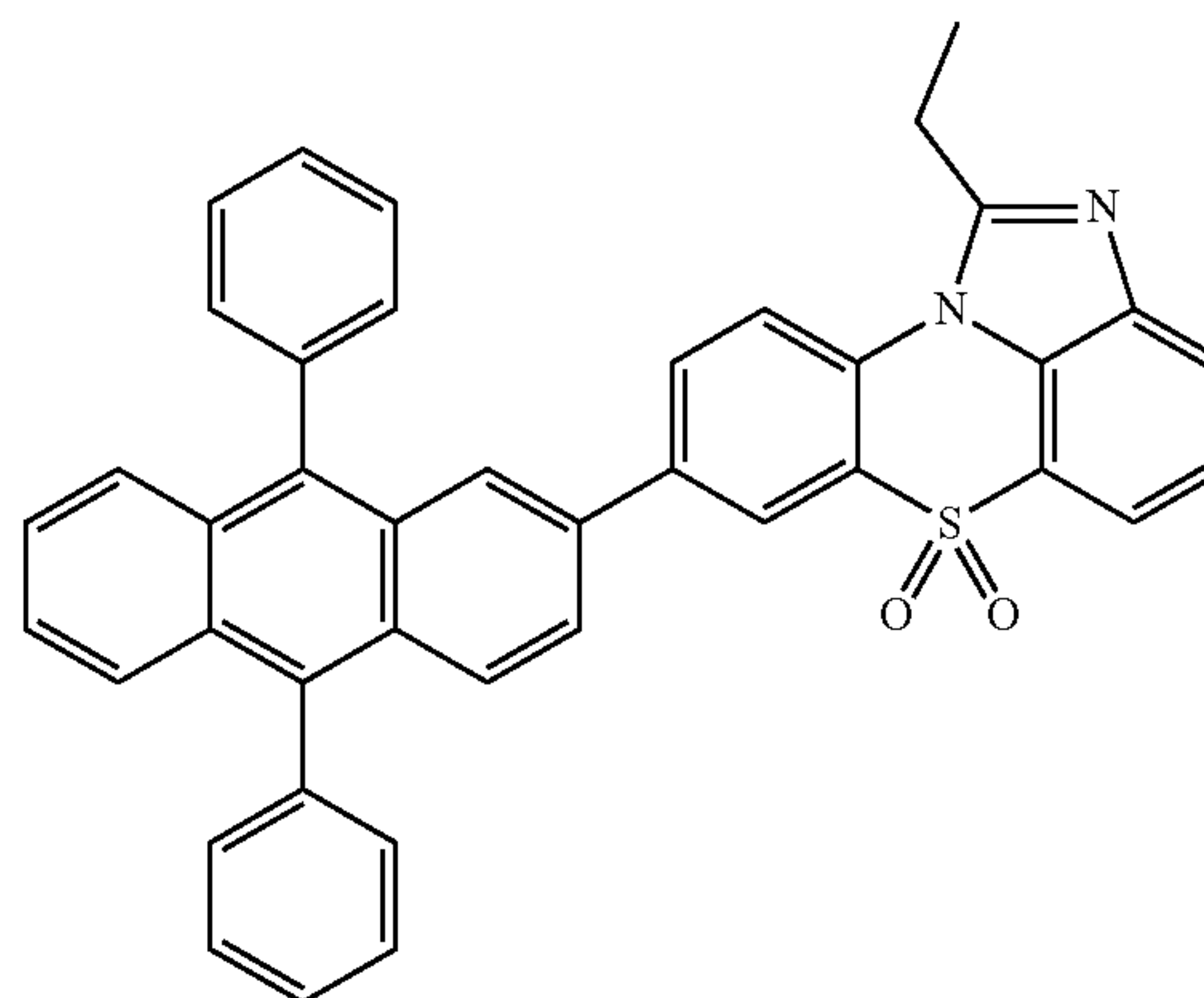
[Chemical Formula 1-3-19]
