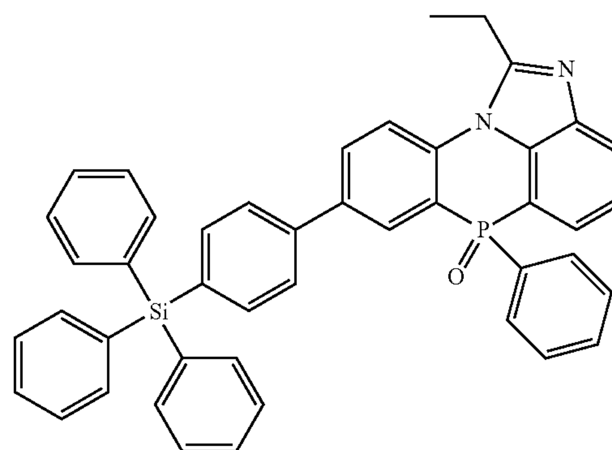
[Chemical Formula 2-3-48]
