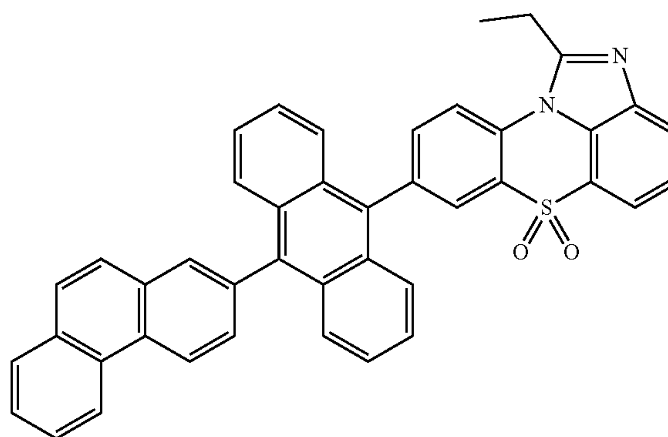
[Chemical Formula 1-3-9]
