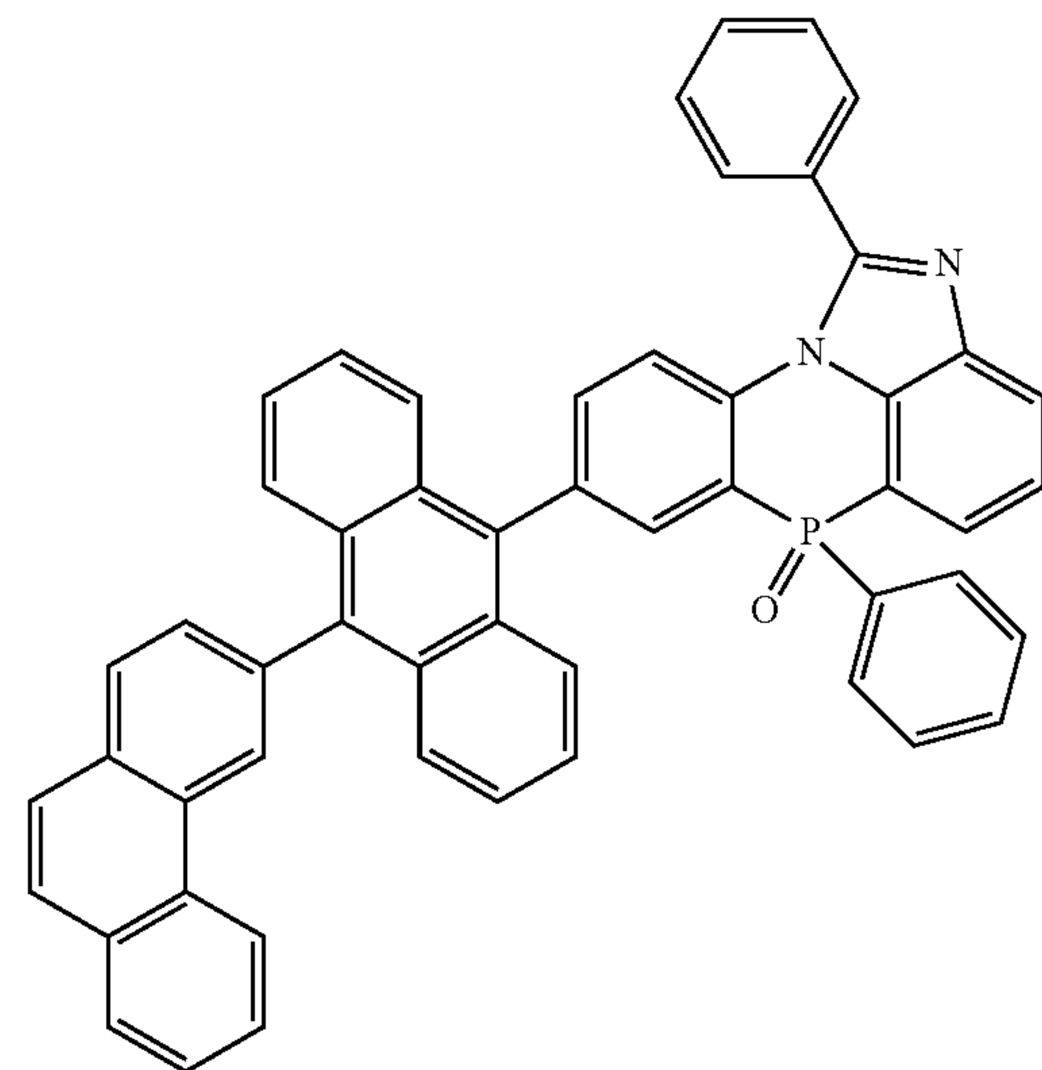
[Chemical Formula 2-4-8]
