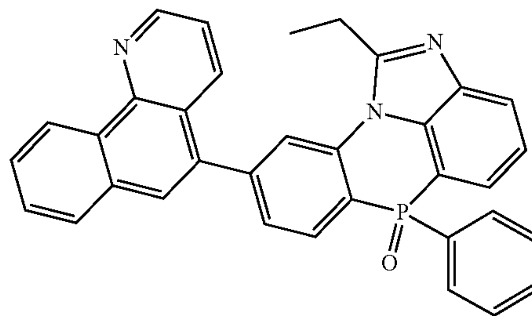
[Chemical Formula 2-7-33]
