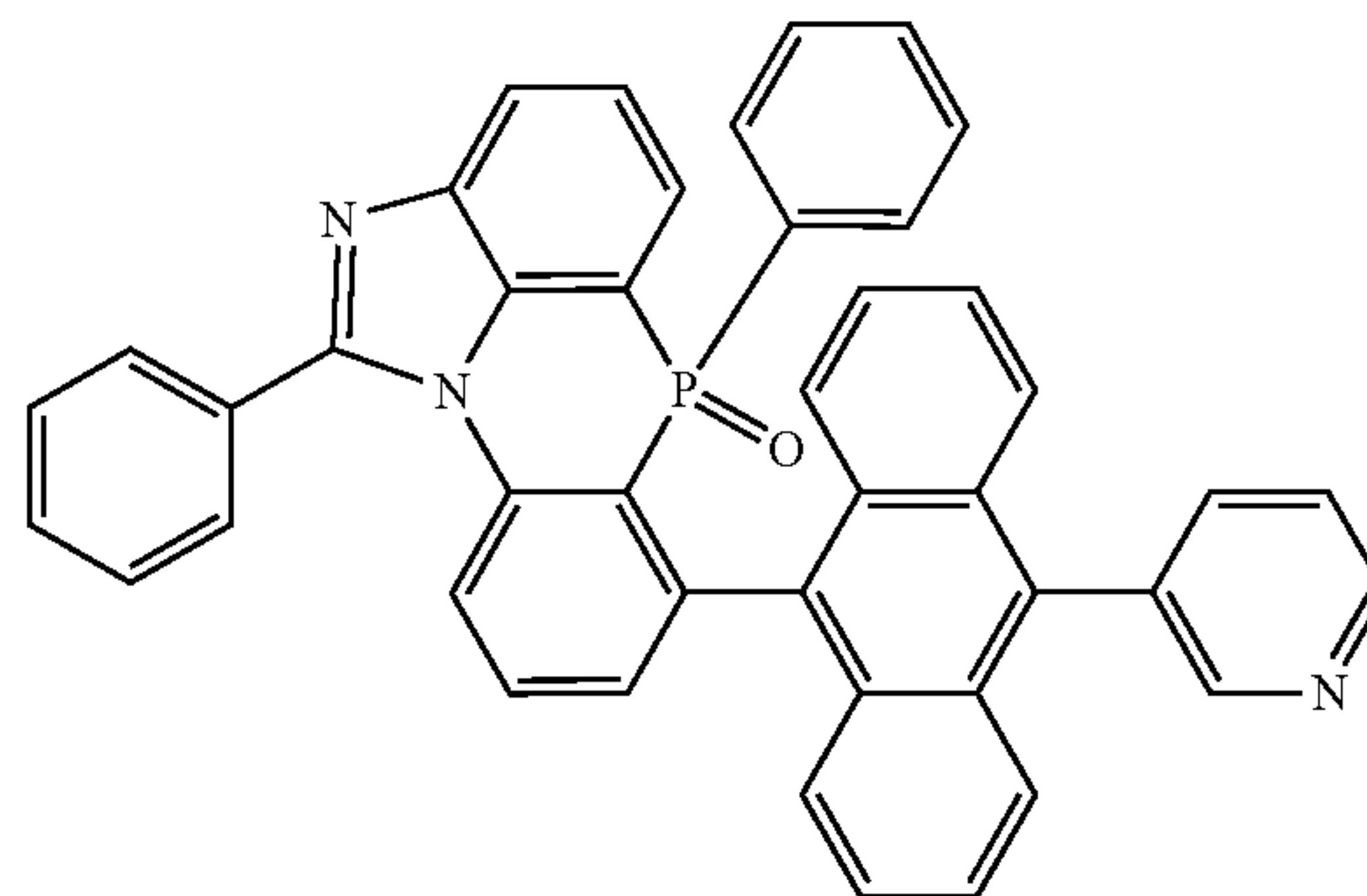
[Chemical Formula 2-6-10]
