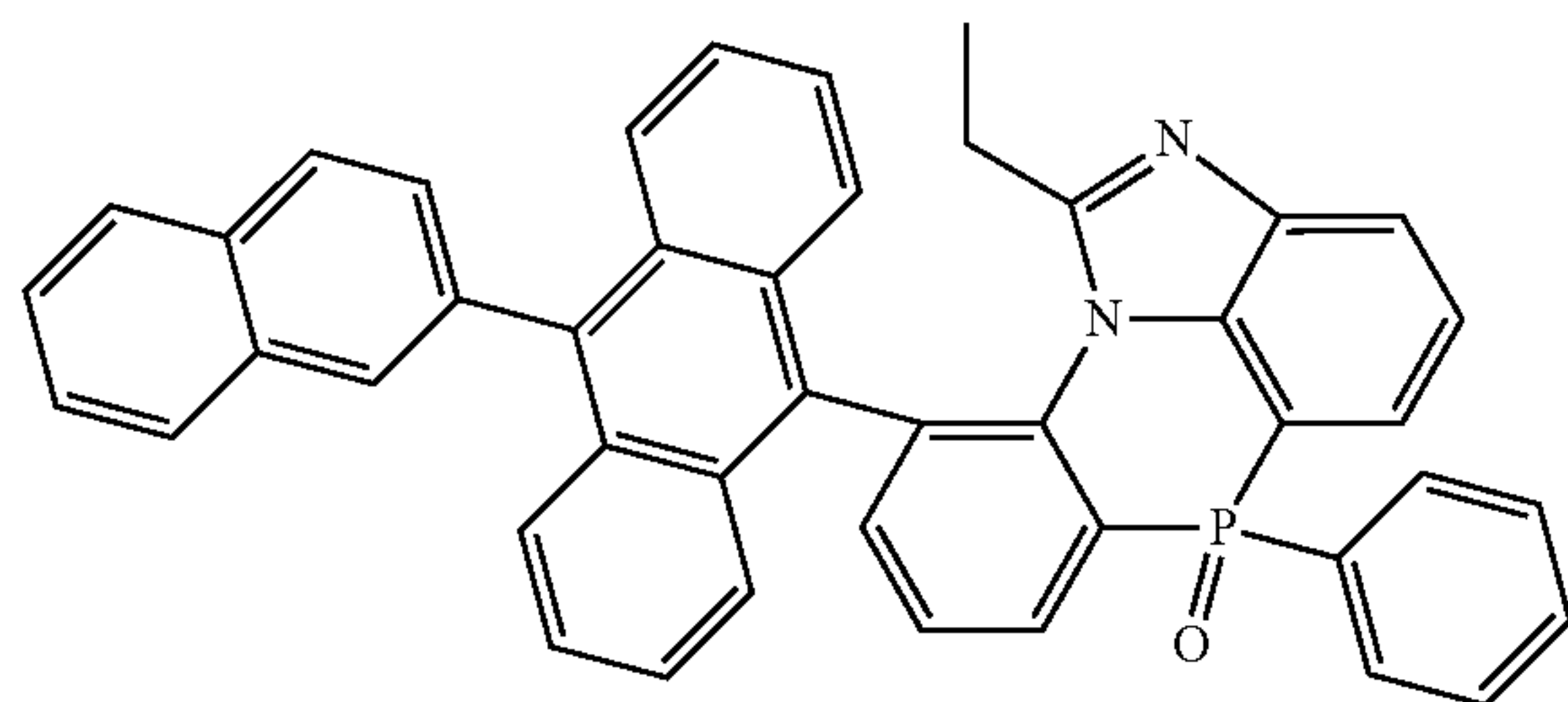
[Chemical Formula 2-8-2]
