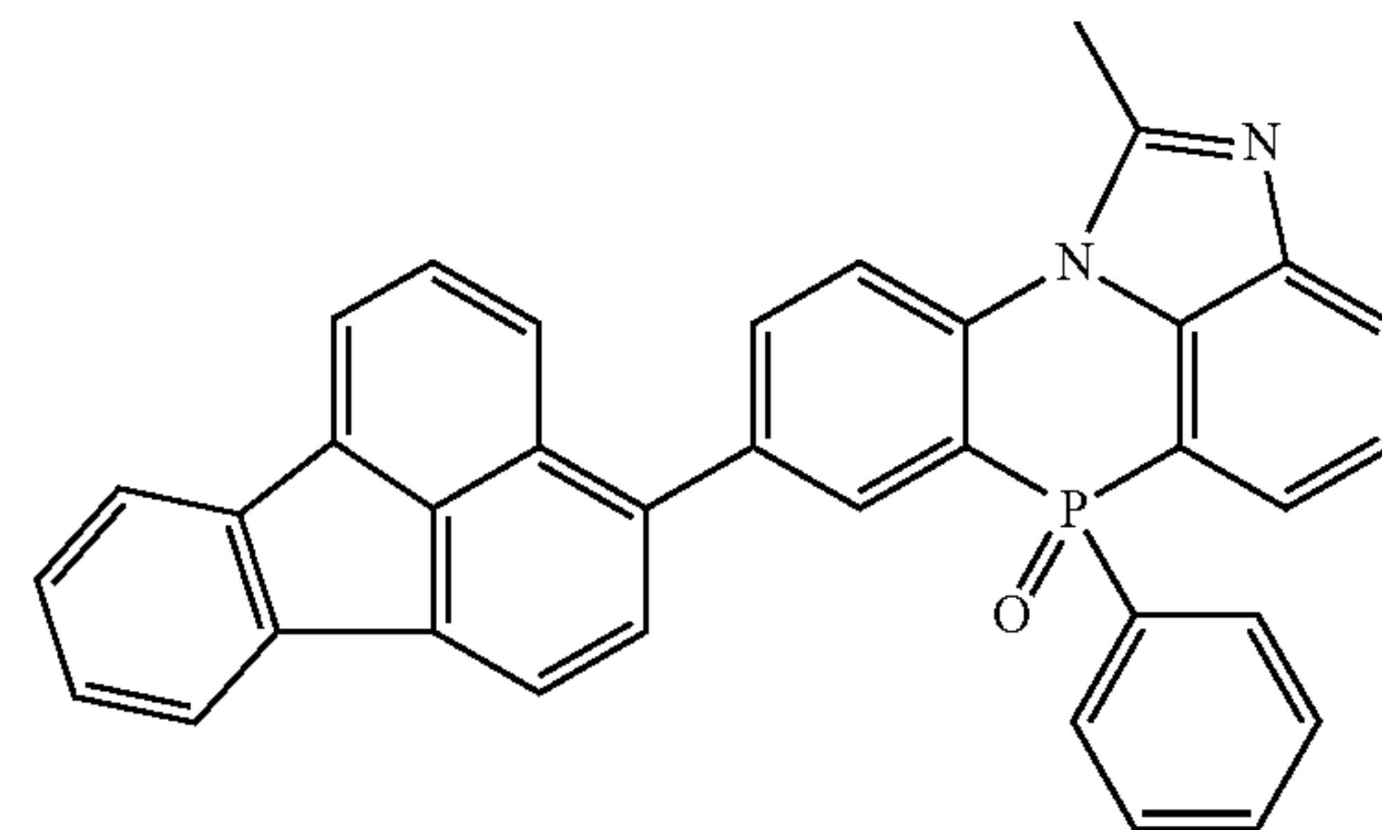
[Chemical Formula 2-2-30]
