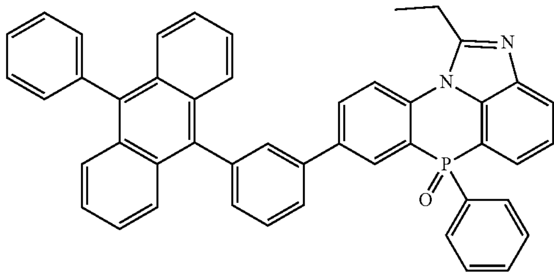
[Chemical Formula 2-3-19]
