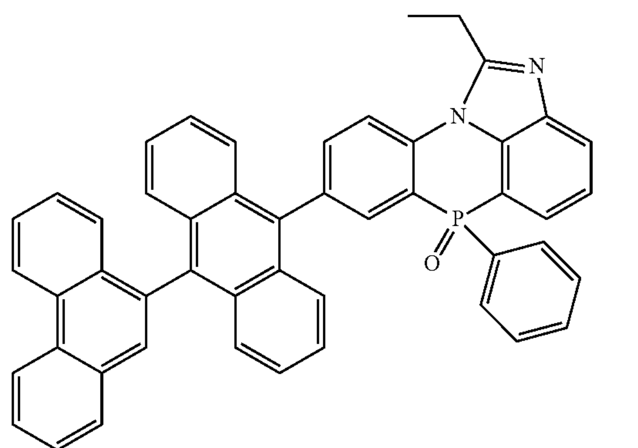
[Chemical Formula 2-3-7]
