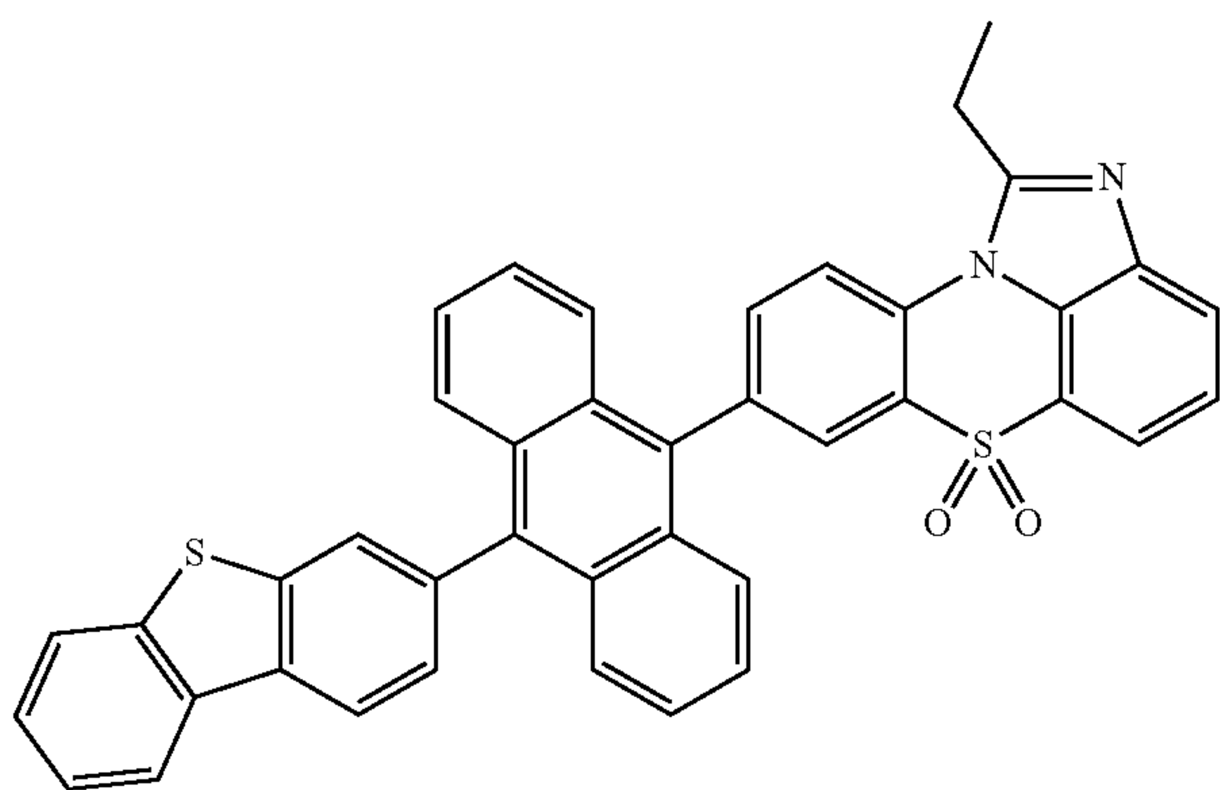
[Chemical Formula 1-3-14]
