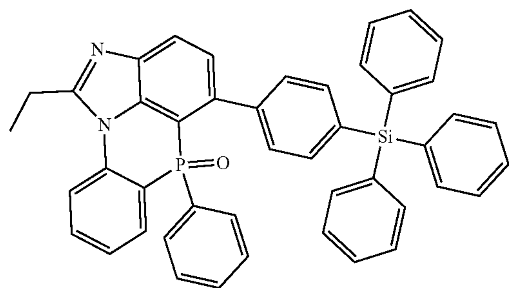
[Chemical Formula 2-9-13]
