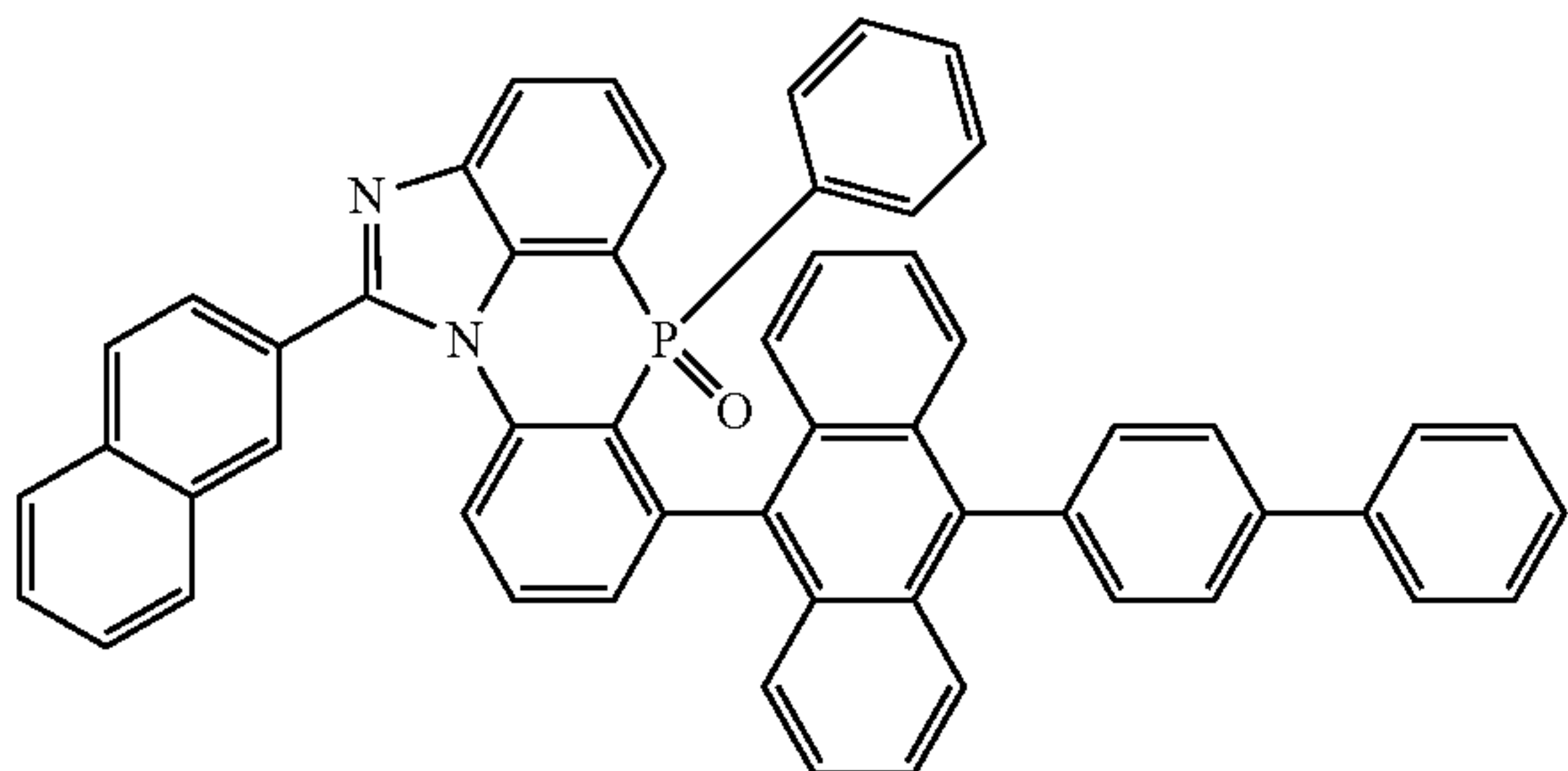
[Chemical Formula 2-6-5] 15
