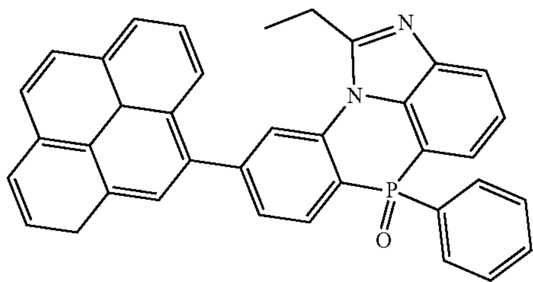
[Chemical Formula 2-7-28]
