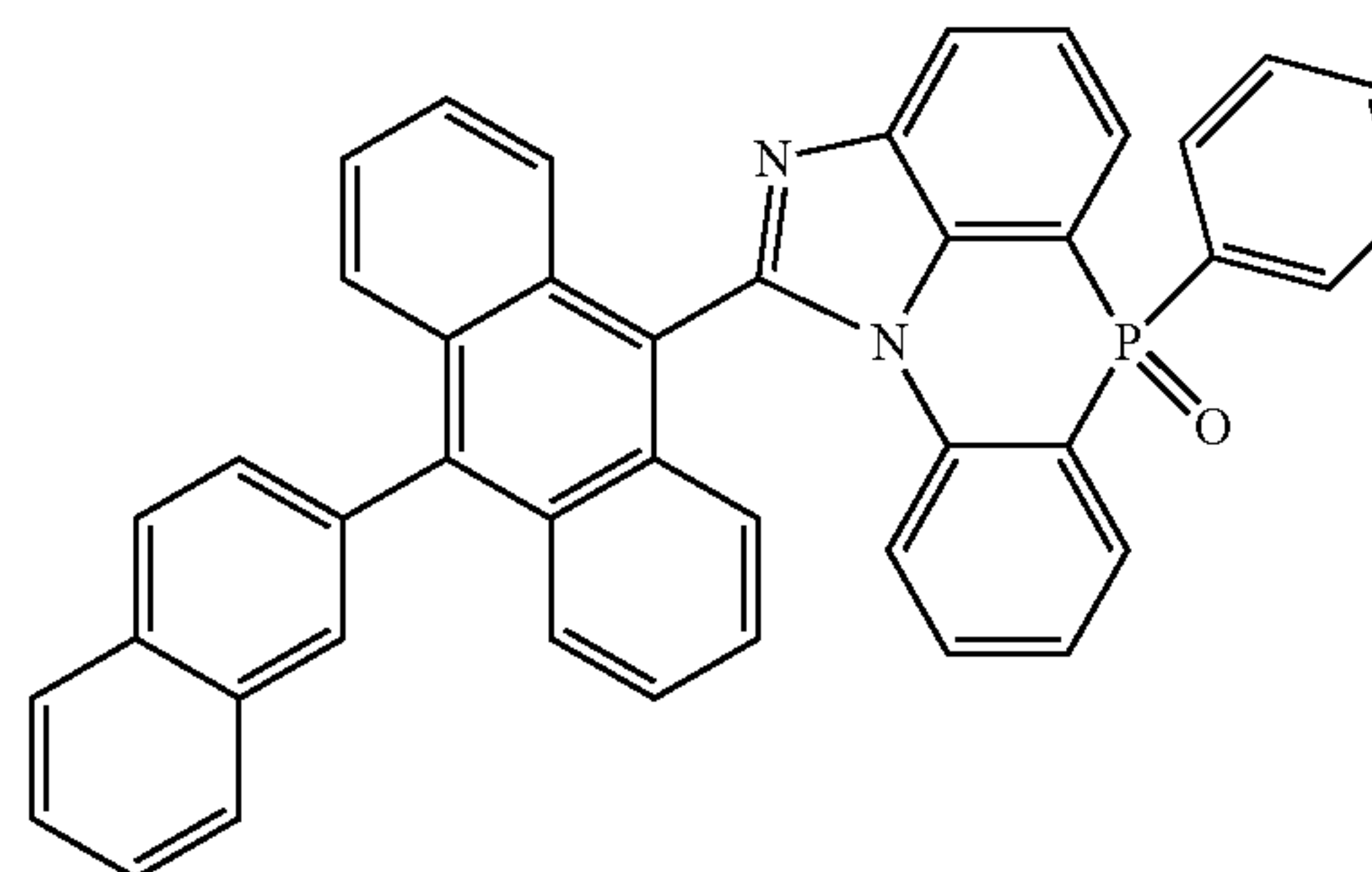
[Chemical Formula 2-5-2]
