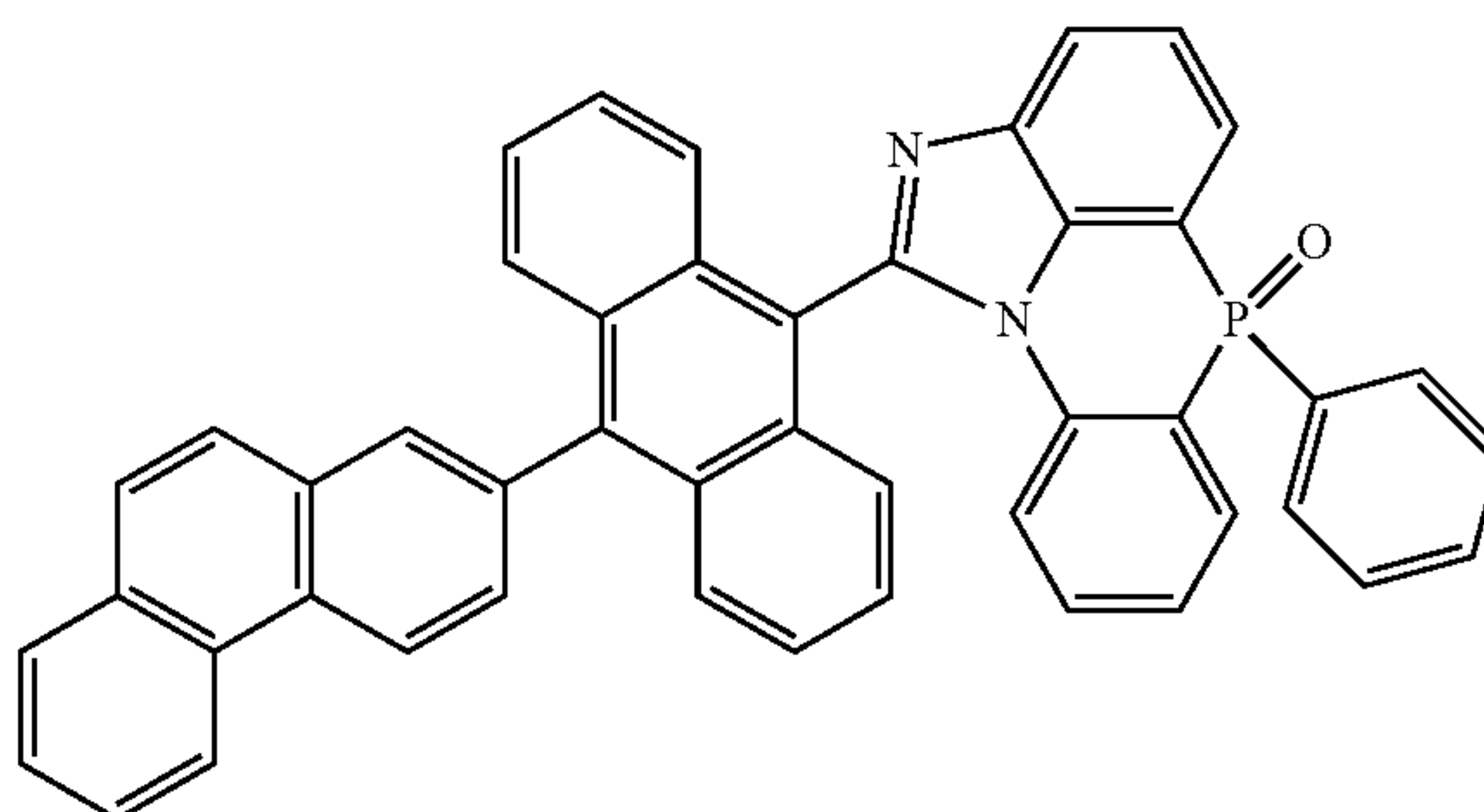
[Chemical Formula 2-5-10]
