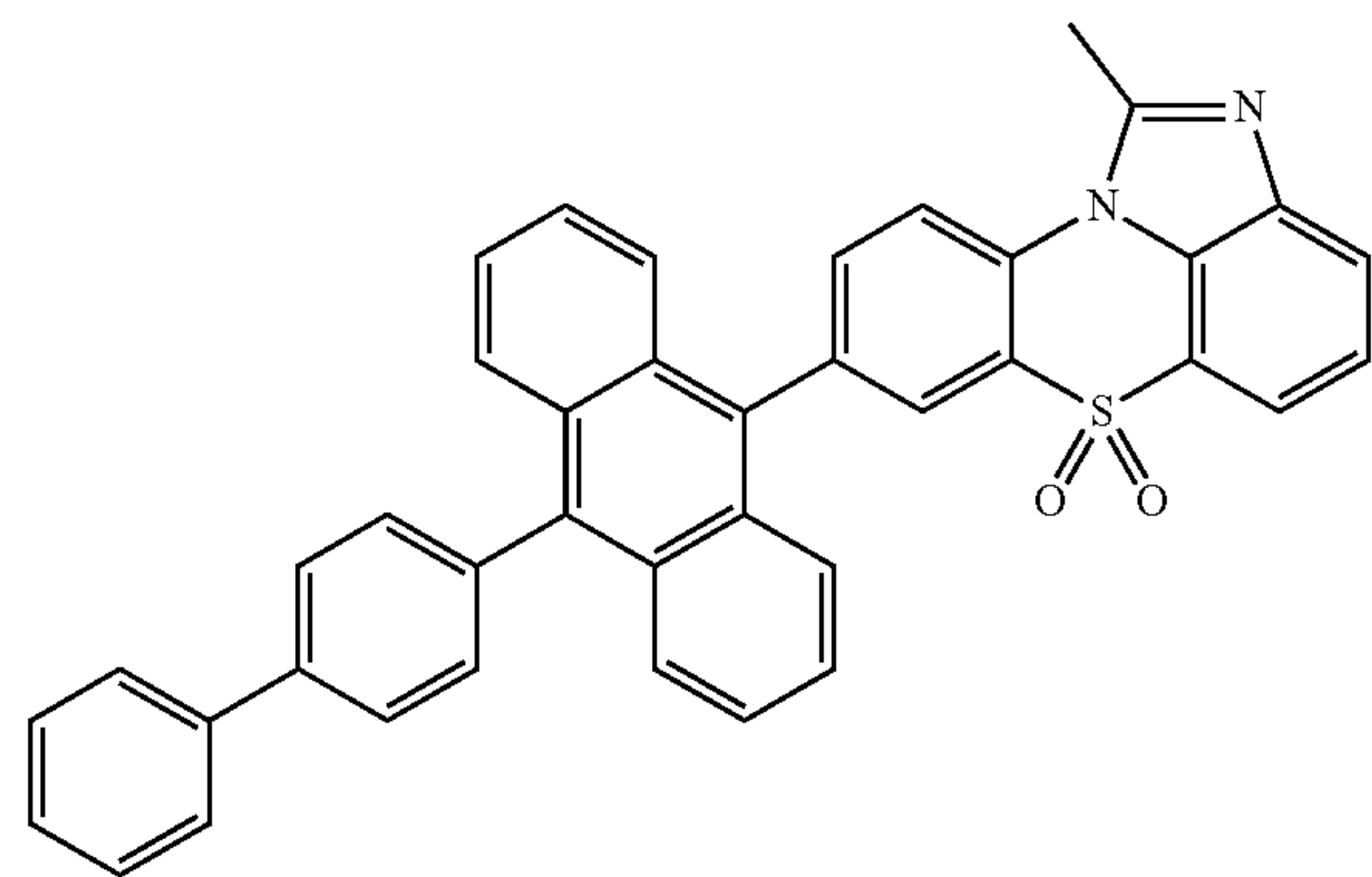
[Chemical Formula 1-2-4]
