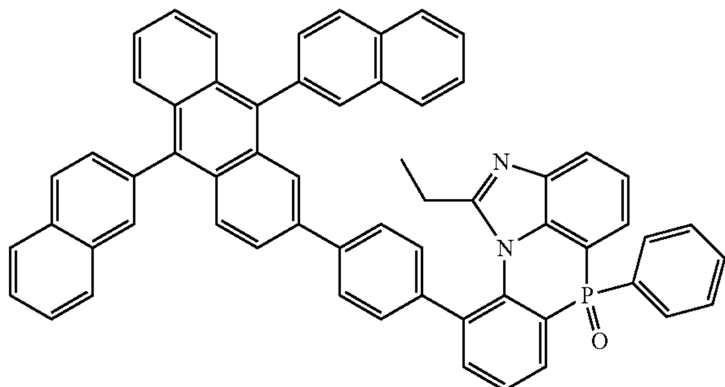
[Chemical Formula 2-8-25]
