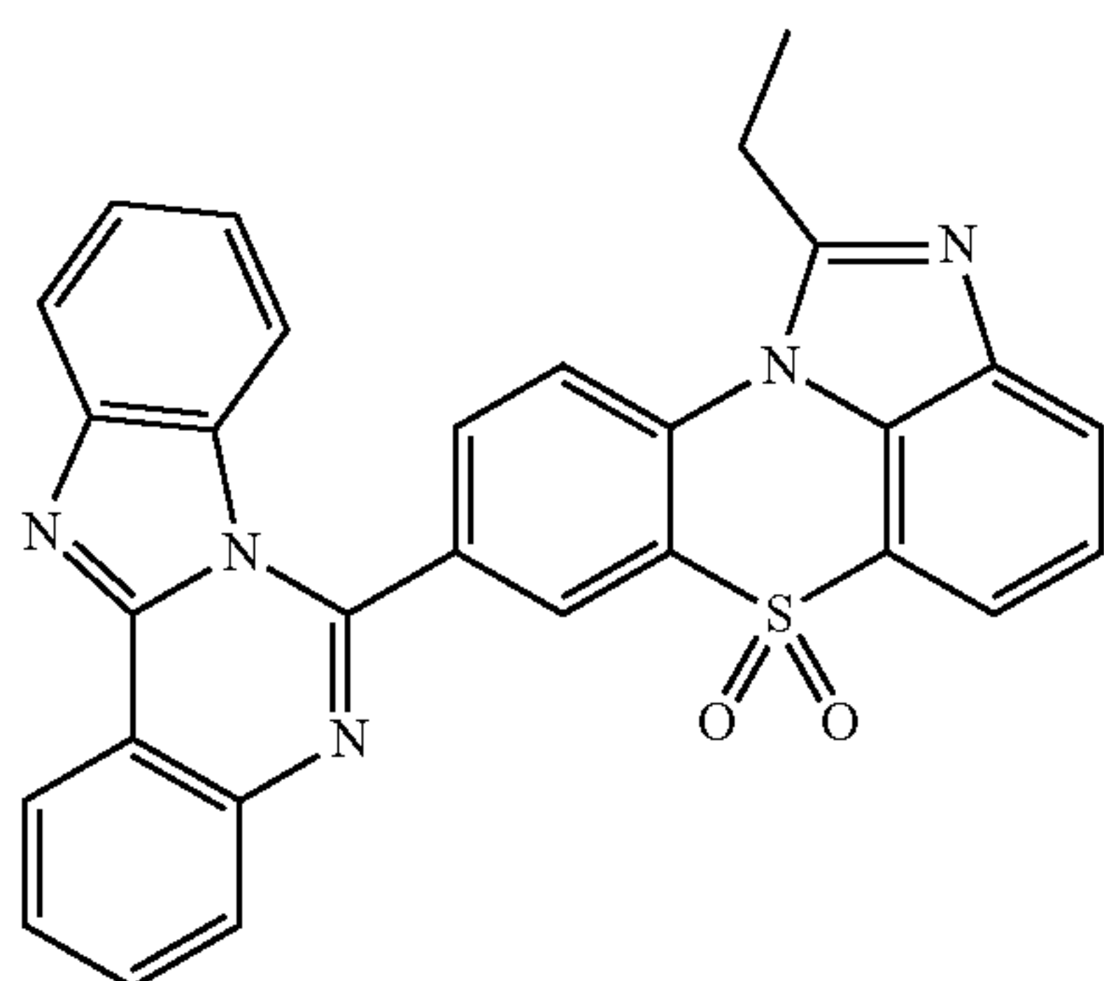
[Chemical Formula 1-3-53]
