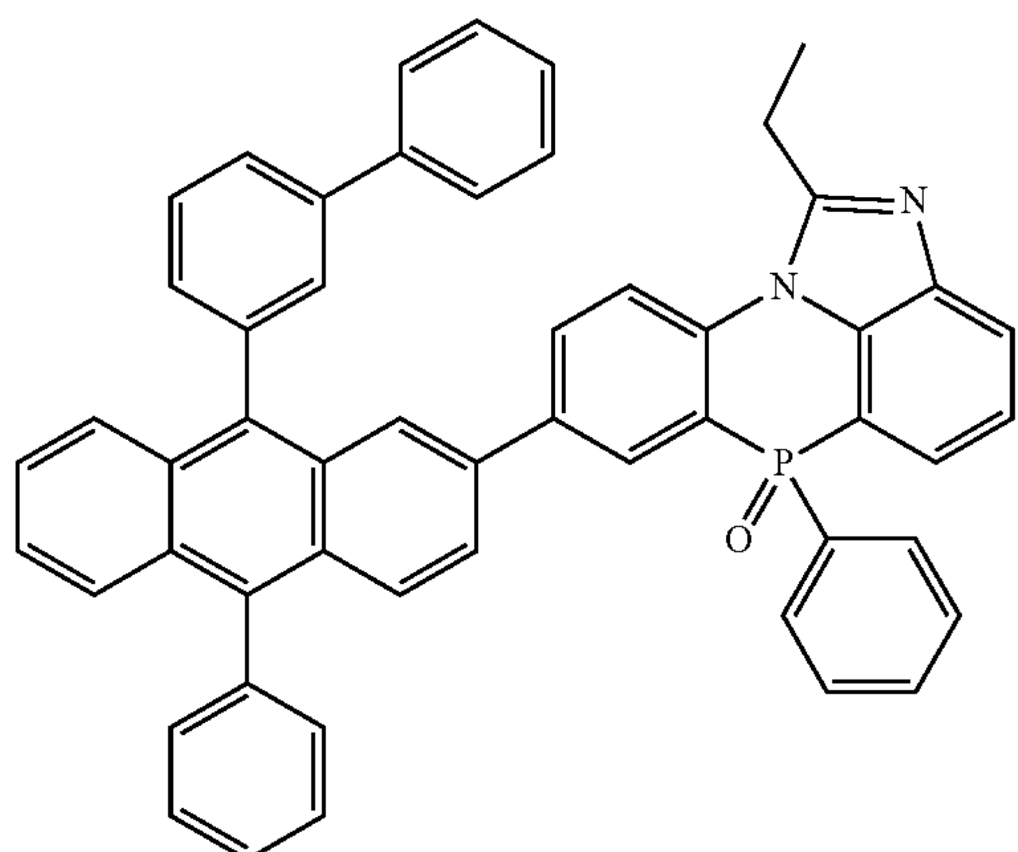
[Chemical Formula 2-3-24]
