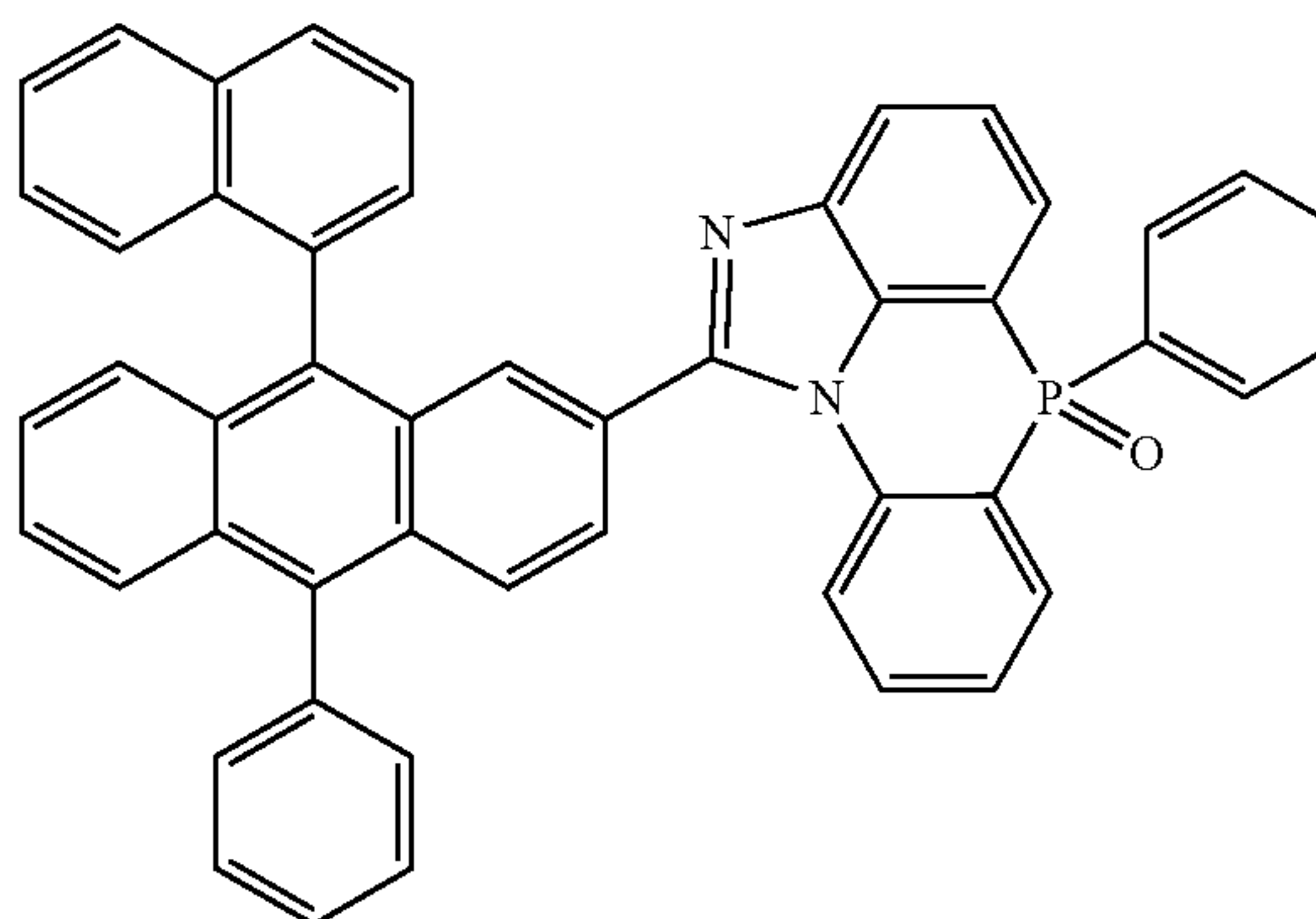
[Chemical Formula 2-5-22]
