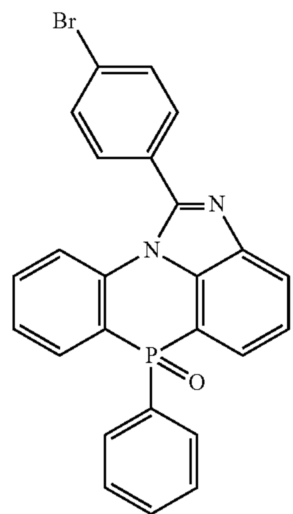
[Compound 2-1-G]
