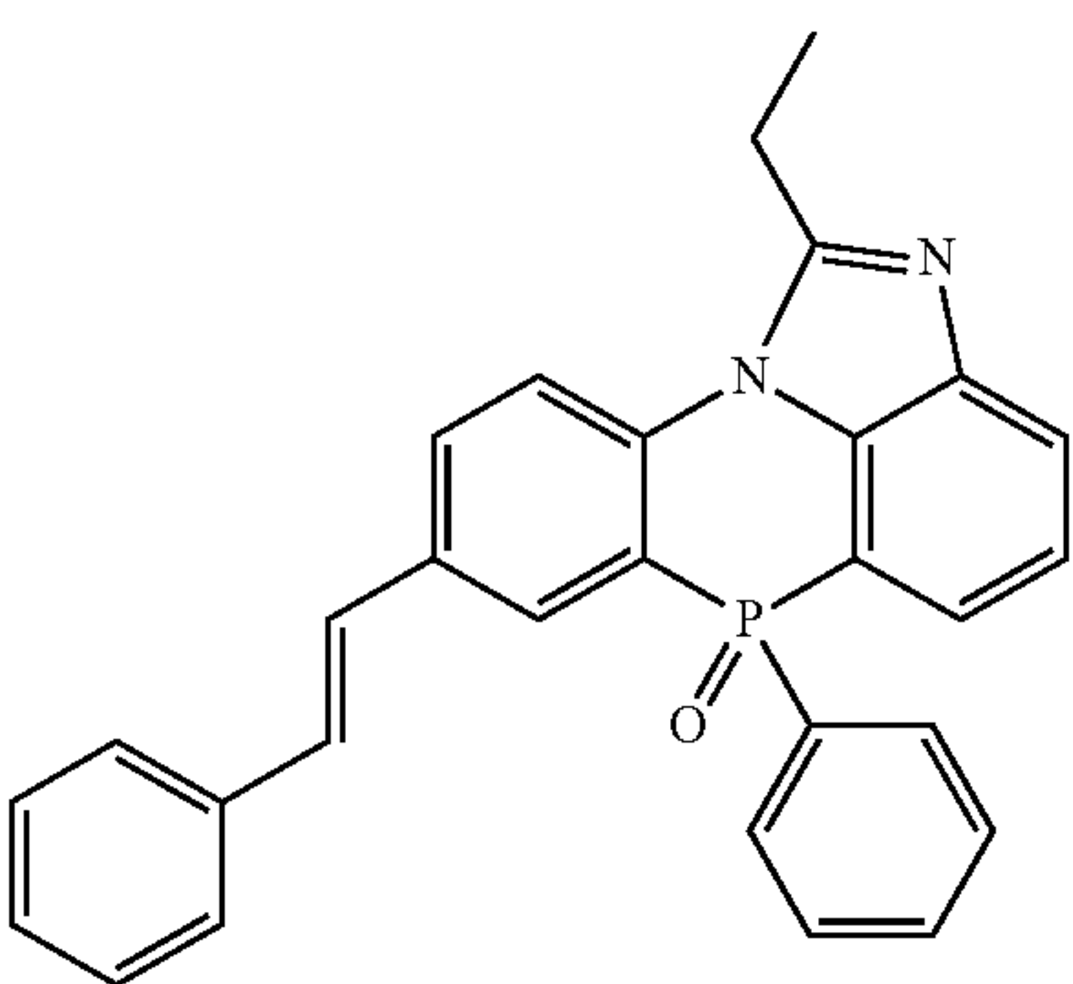
[Chemical Formula 2-3-54]
