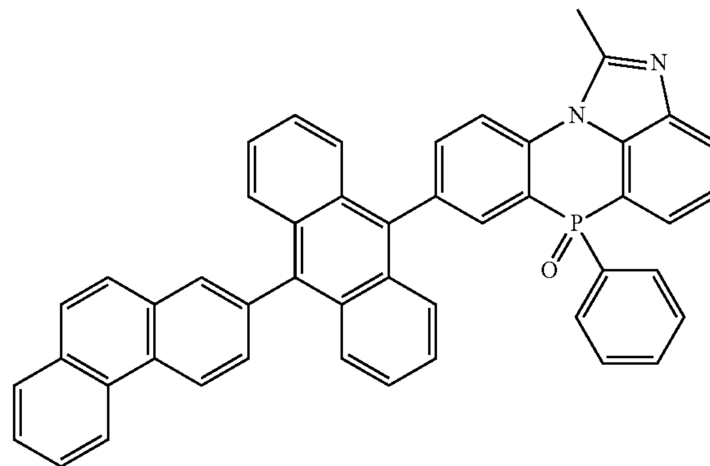
[Chemical Formula 2-2-10]
