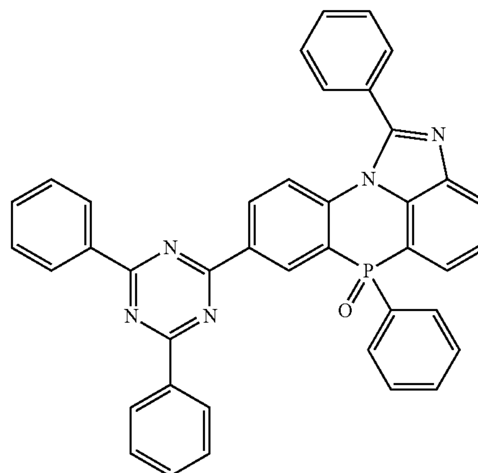
[Chemical Formula 2-4-41]
