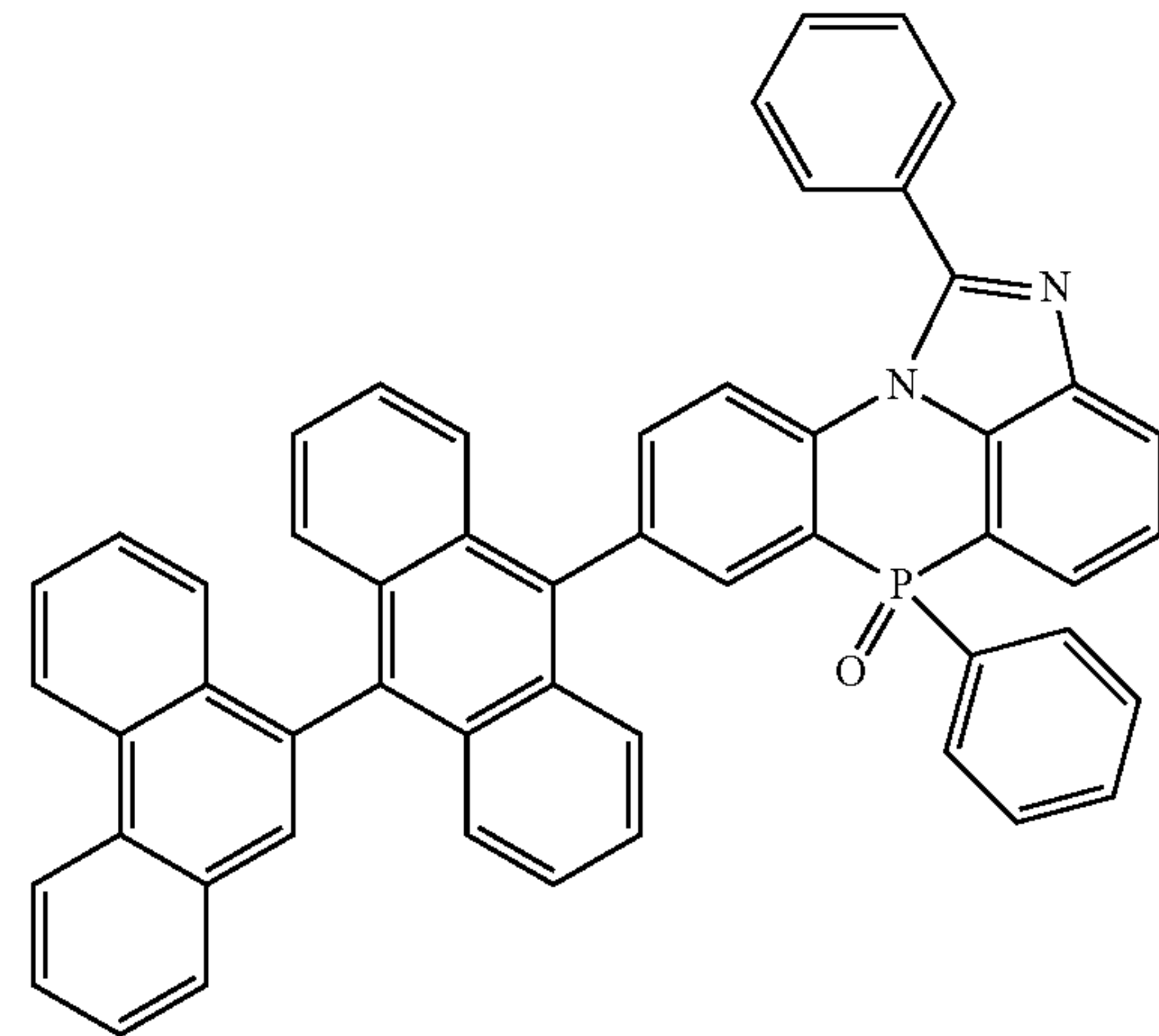
[Chemical Formula 2-4-7]
