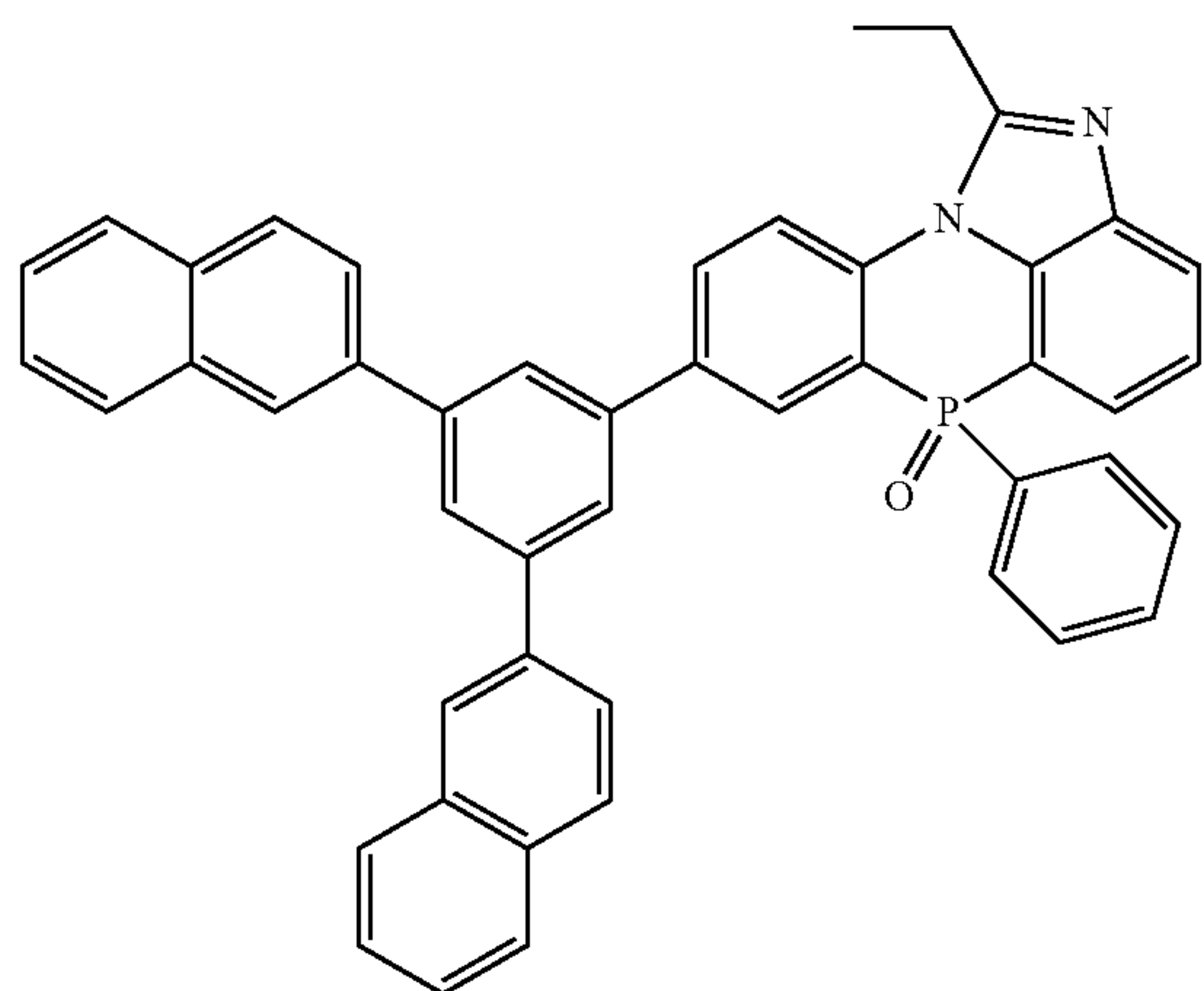
[Chemical Formula 2-3-43]
