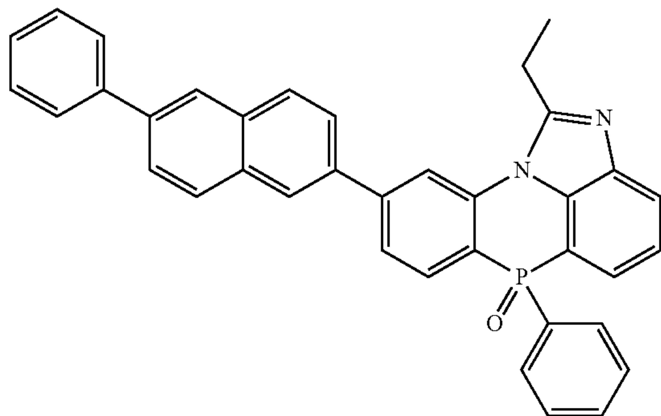
[Chemical Formula 2-7-27]
