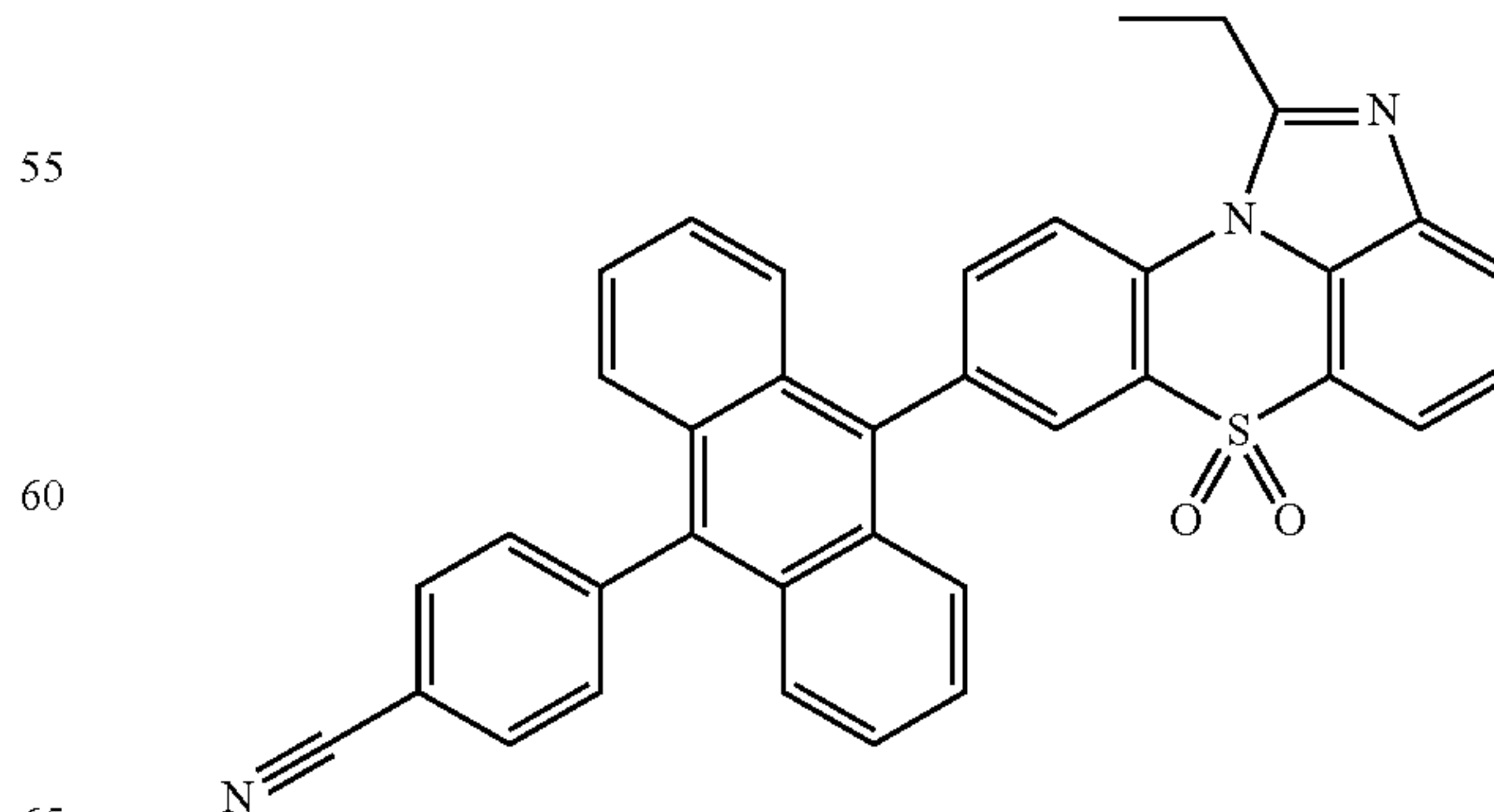
[Chemical Formula 1-3-12]
