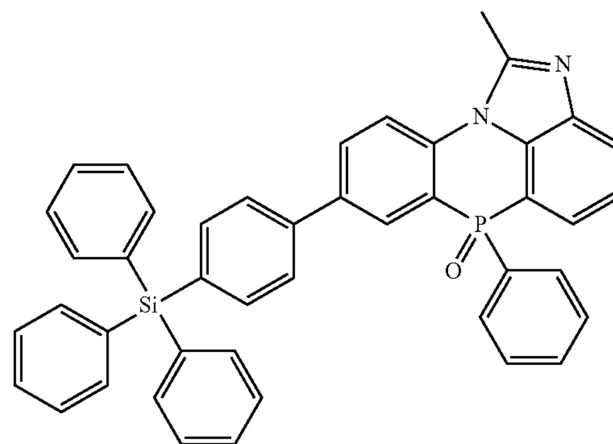
Chemical Formula 2-2-48]
