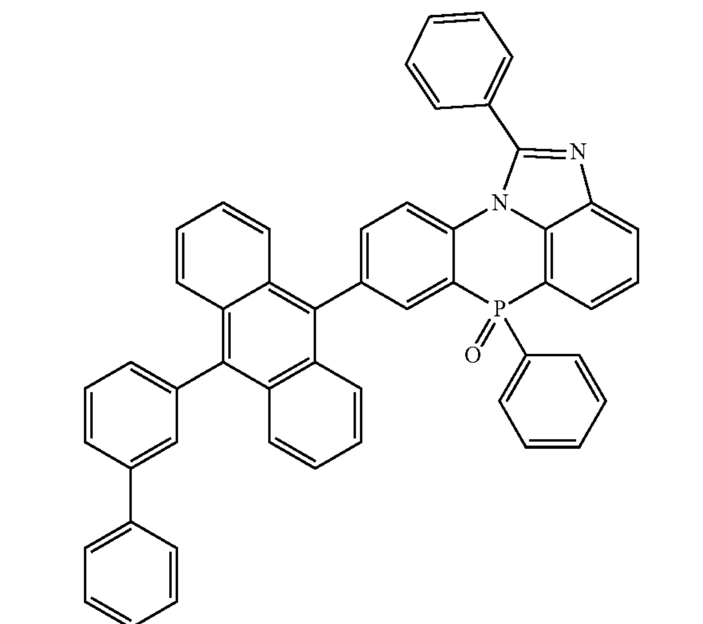
[Chemical Formula 2-4-6]
