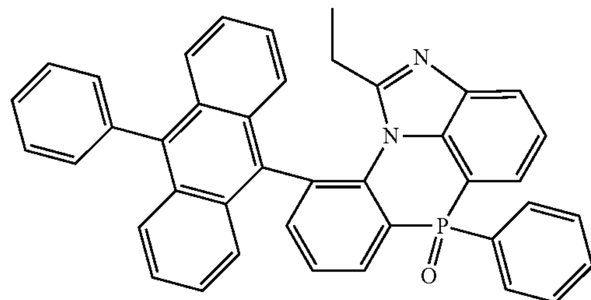
[Chemical Formula 2-8-2]
