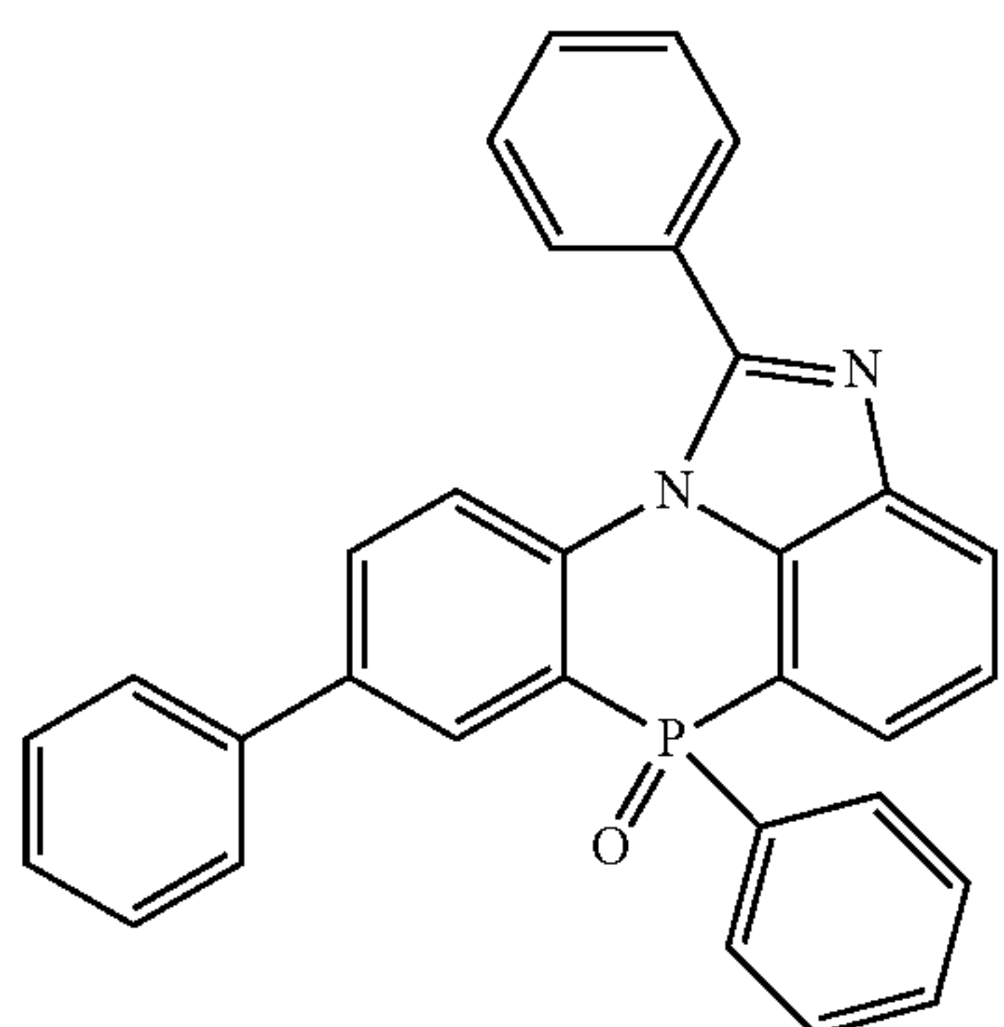
[Chemical Formula 2-4-38]
