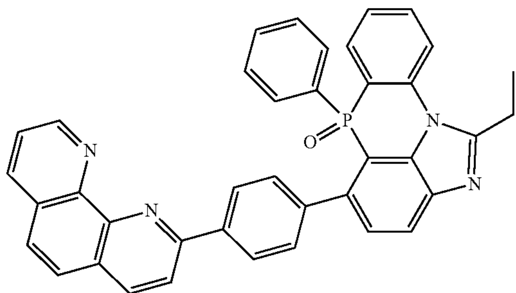
[Chemical Formula 2-9-12]
