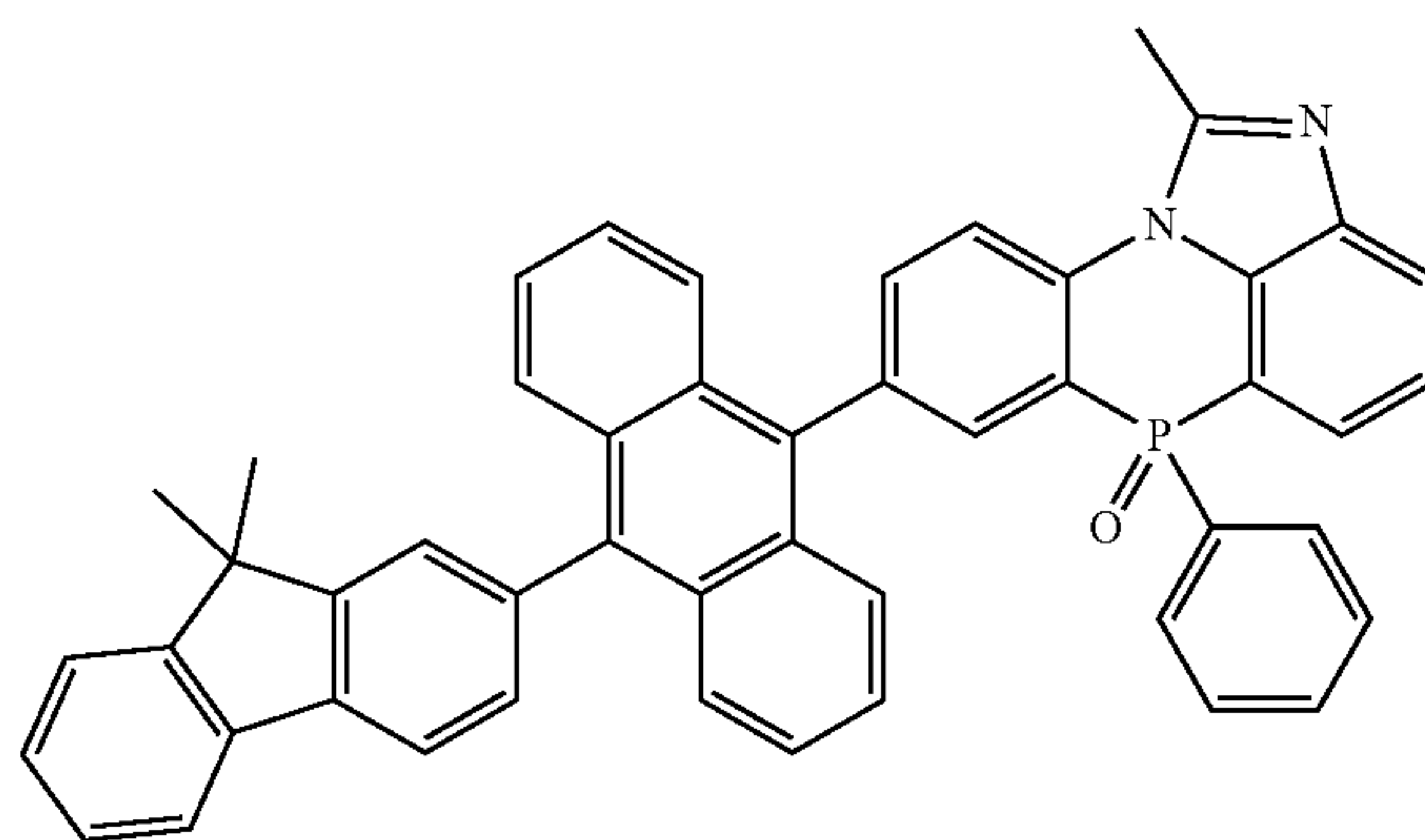
[Chemical Formula 2-2-5]
