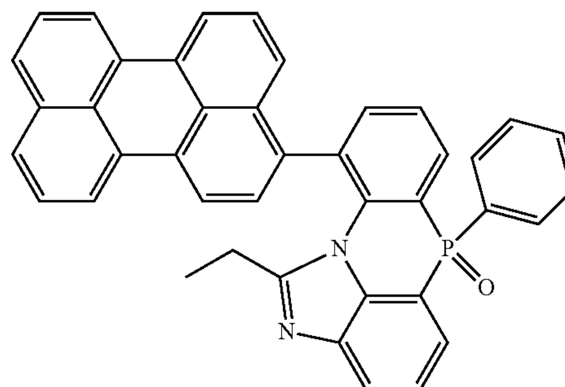
[Chemical Formula 2-8-29]
