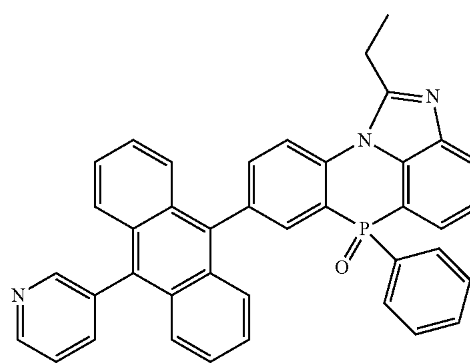
[Chemical Formula 2-3-11]
