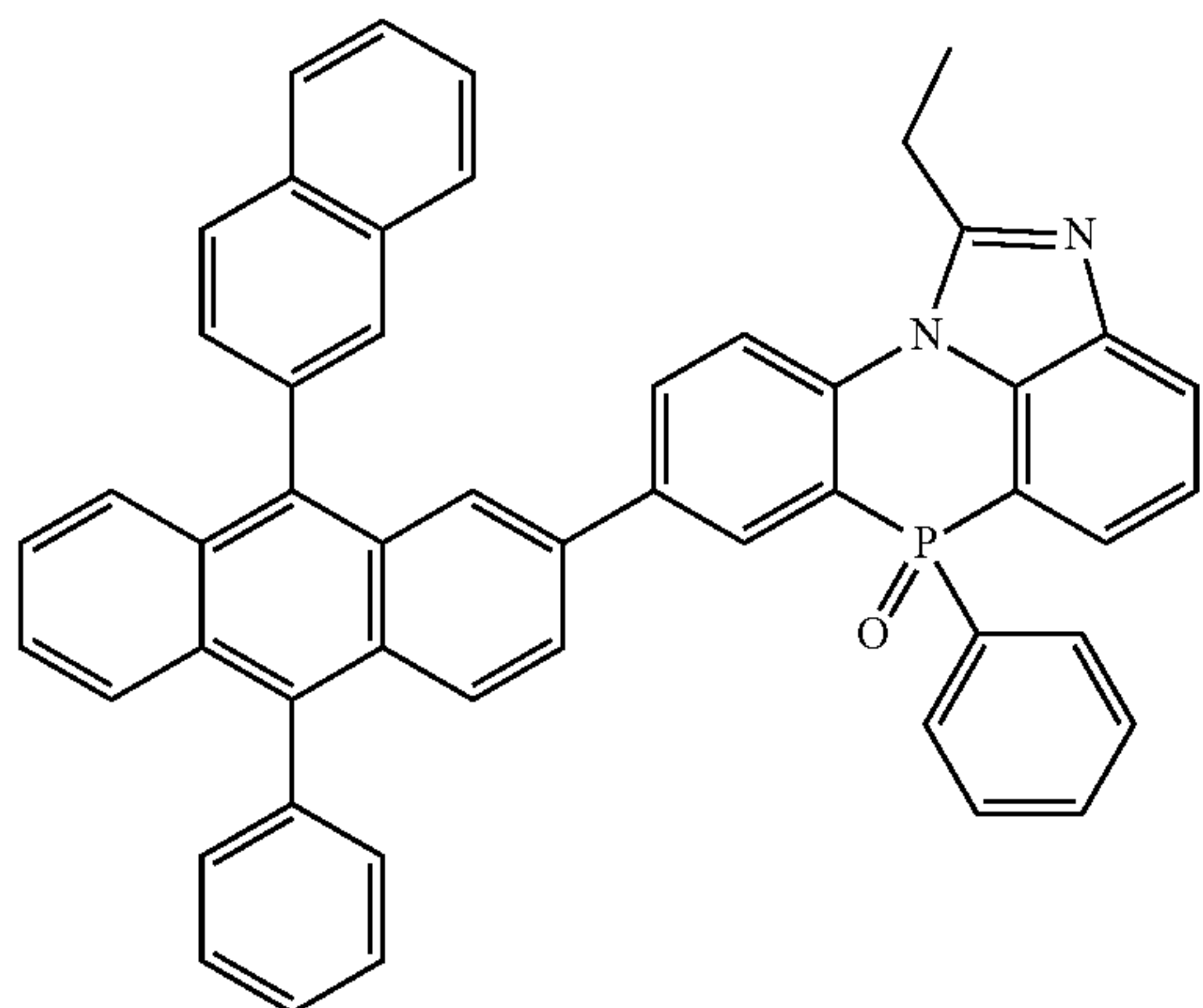
[Chemical Formula 2-3-23]
