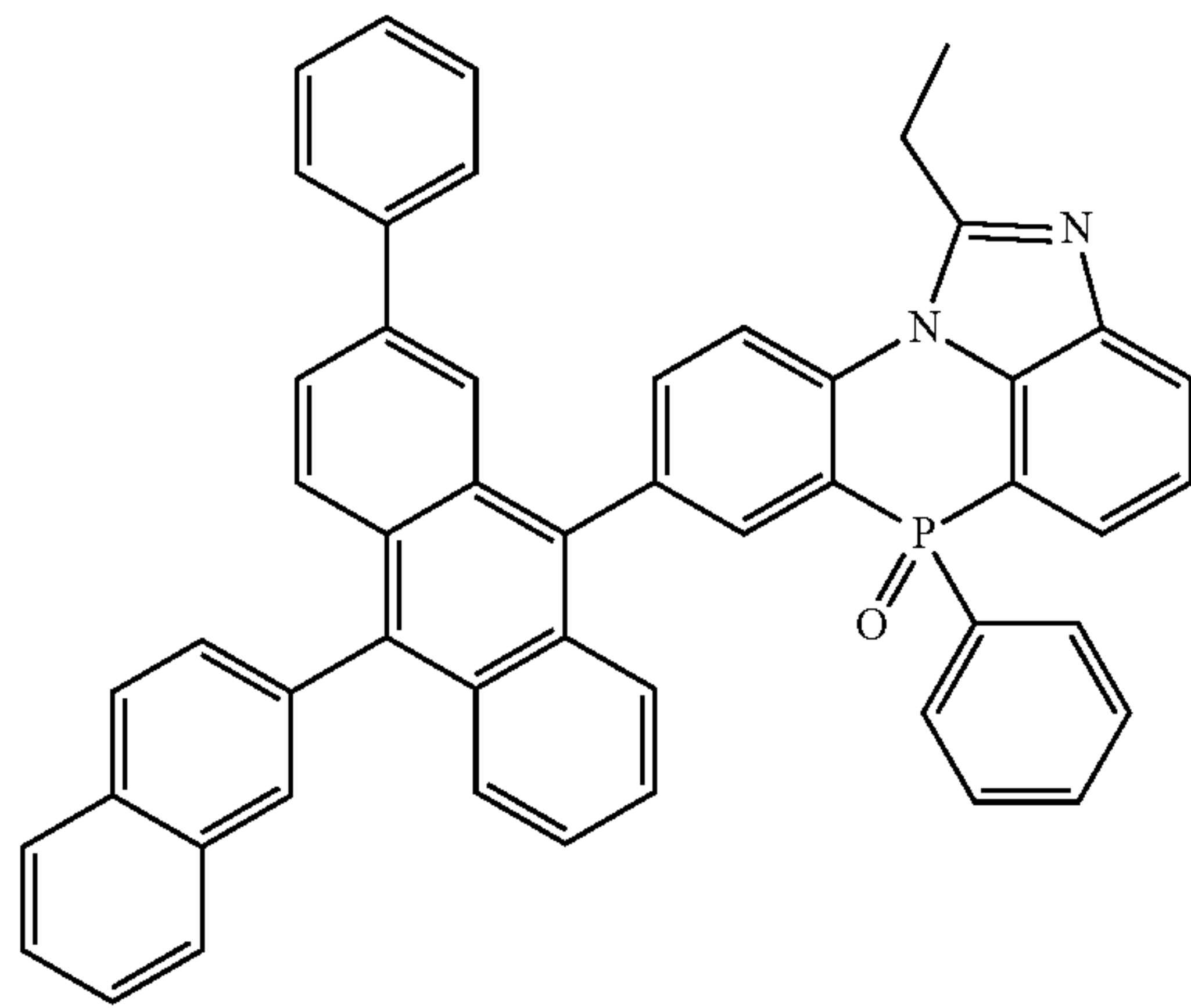
[Chemical Formula 2-3-16]
