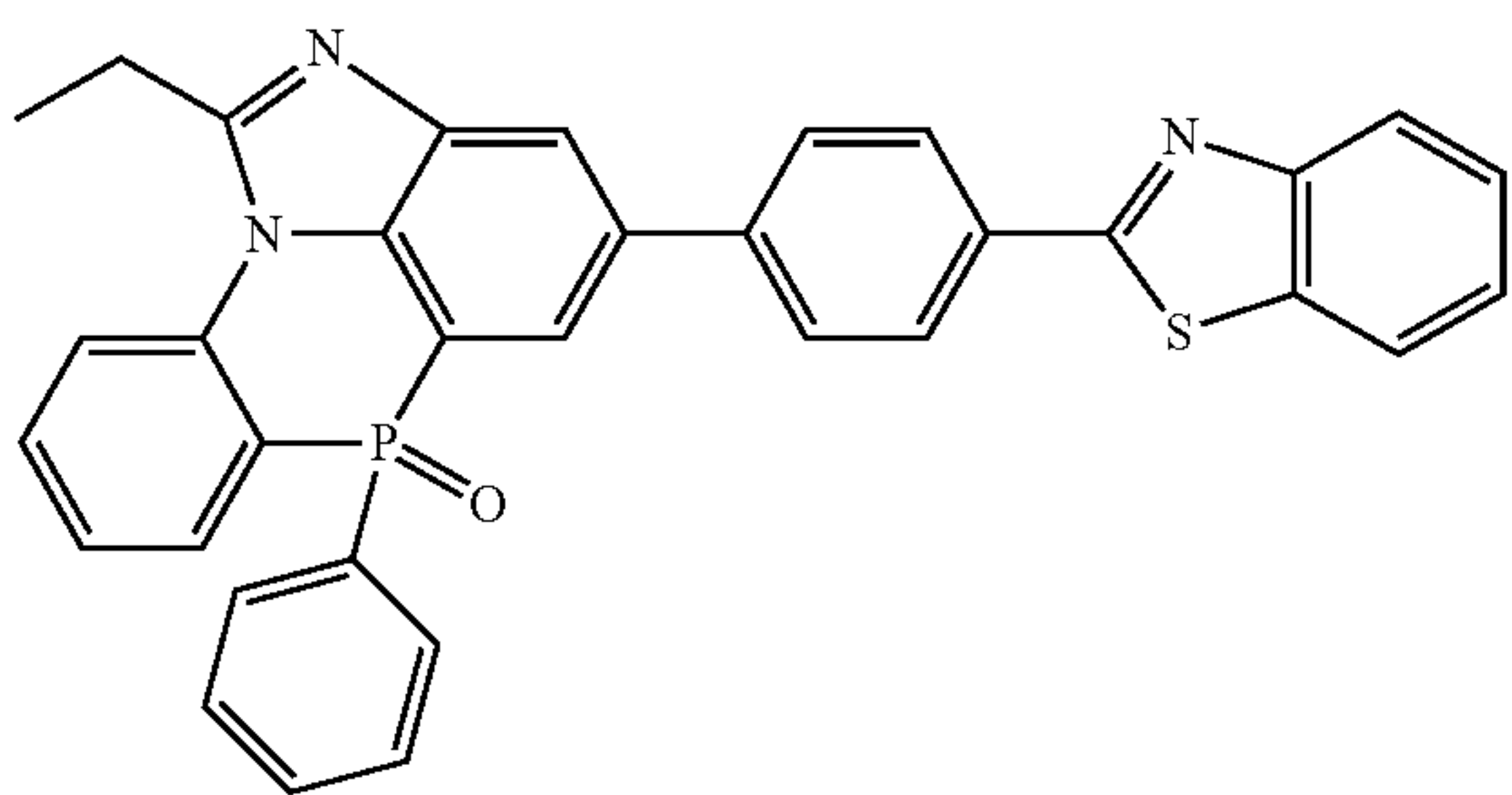
[Chemical Formula 2-10-10]
