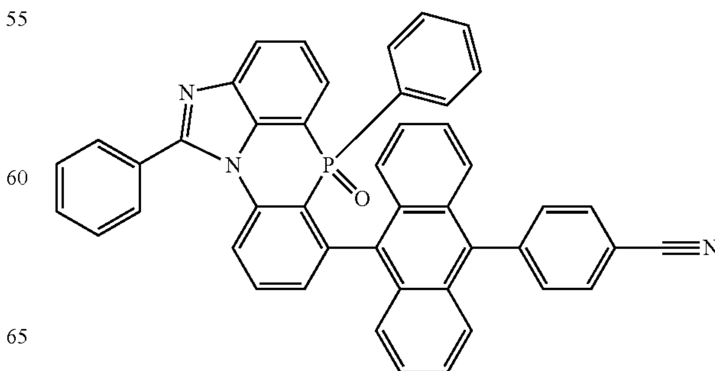
[Chemical Formula 2-6-12]
