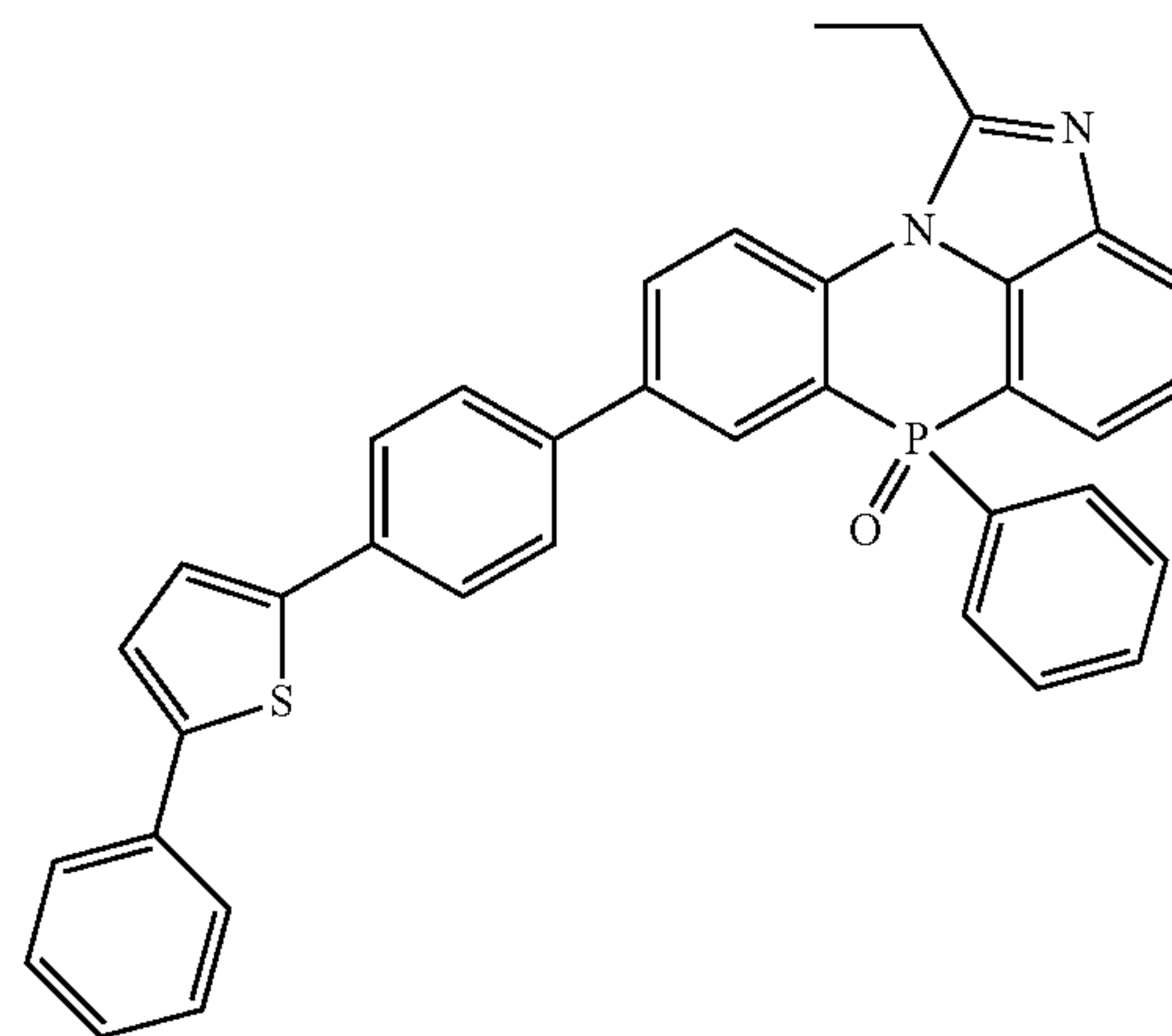
[Chemical Formula 2-3-40]
