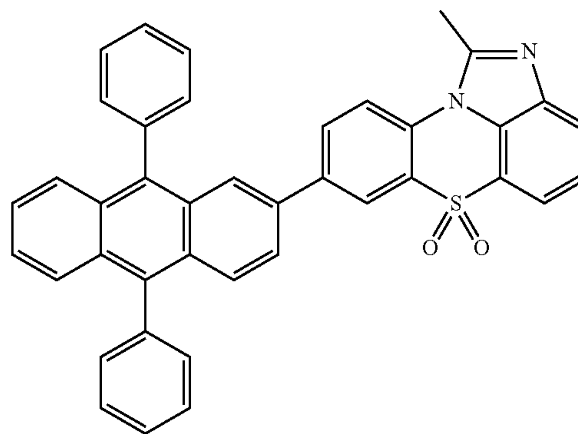
[Chemical Formula 1-2-19]
