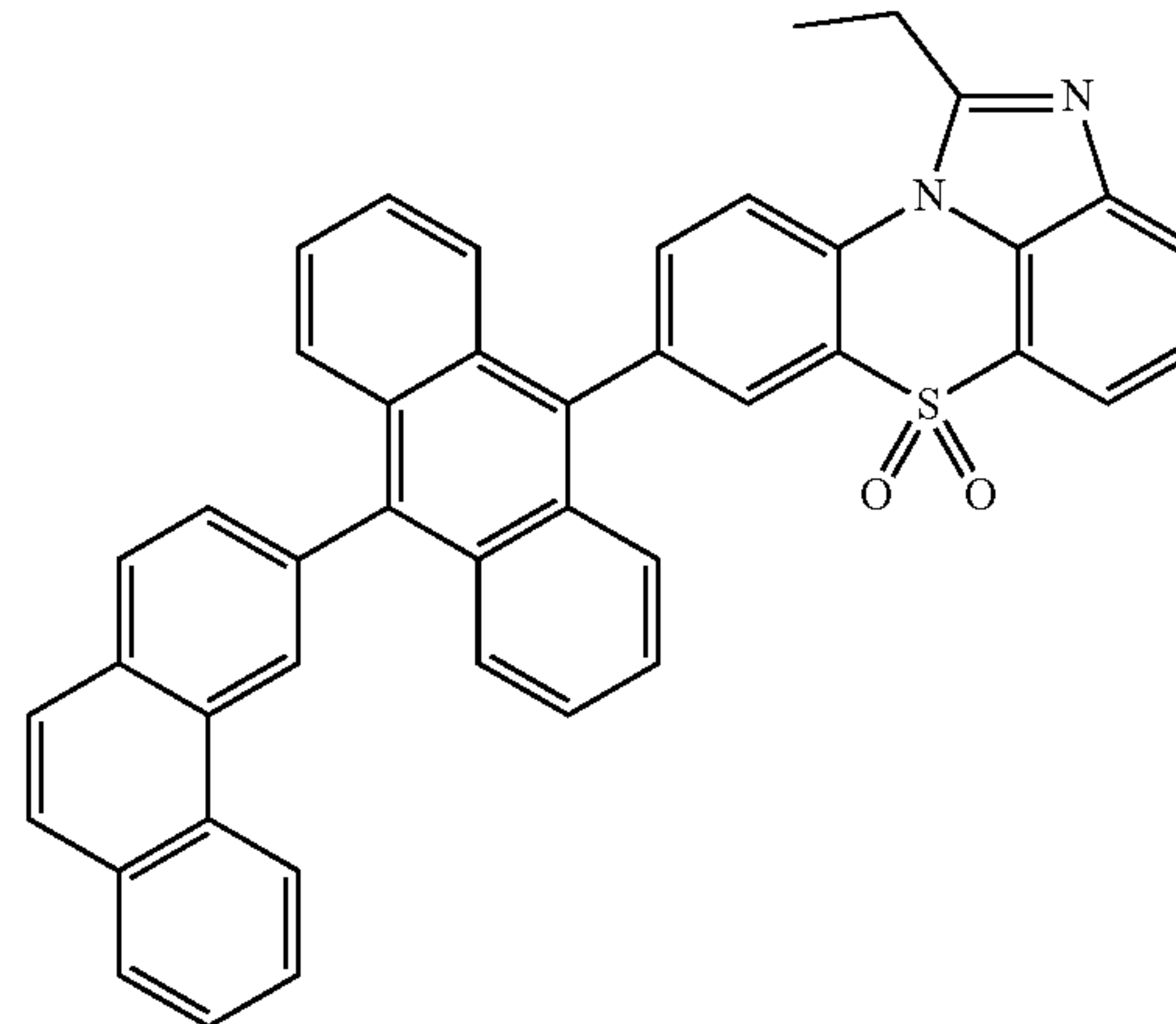
[Chemical Formula 1-3-9]
