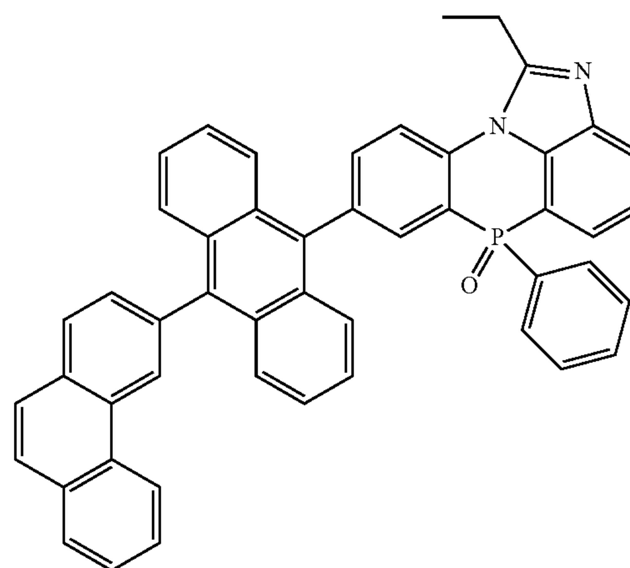
[Chemical Formula 2-3-8]
