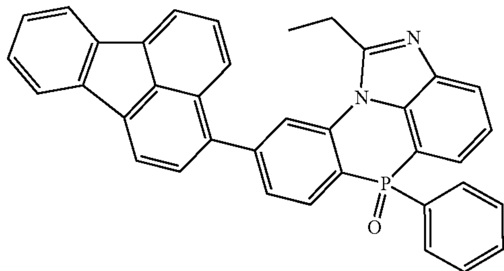
[Chemical Formula 2-7-30]
