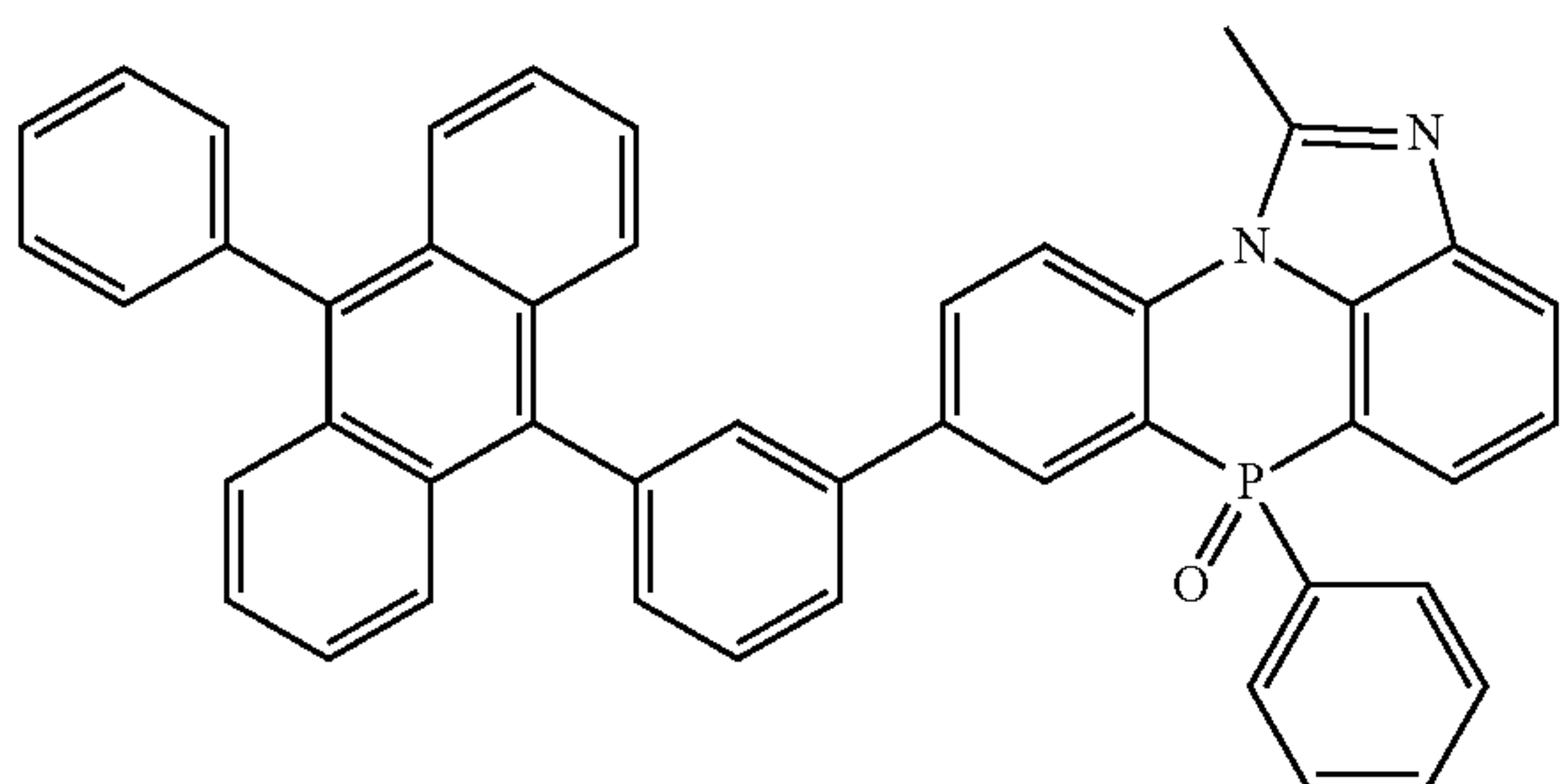
[Chemical Formula 2-2-18]
