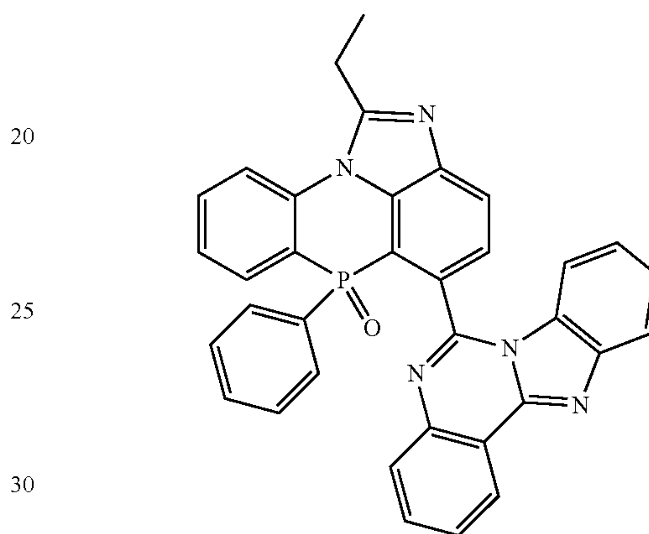
[Chemical Formula 2-9-17]
