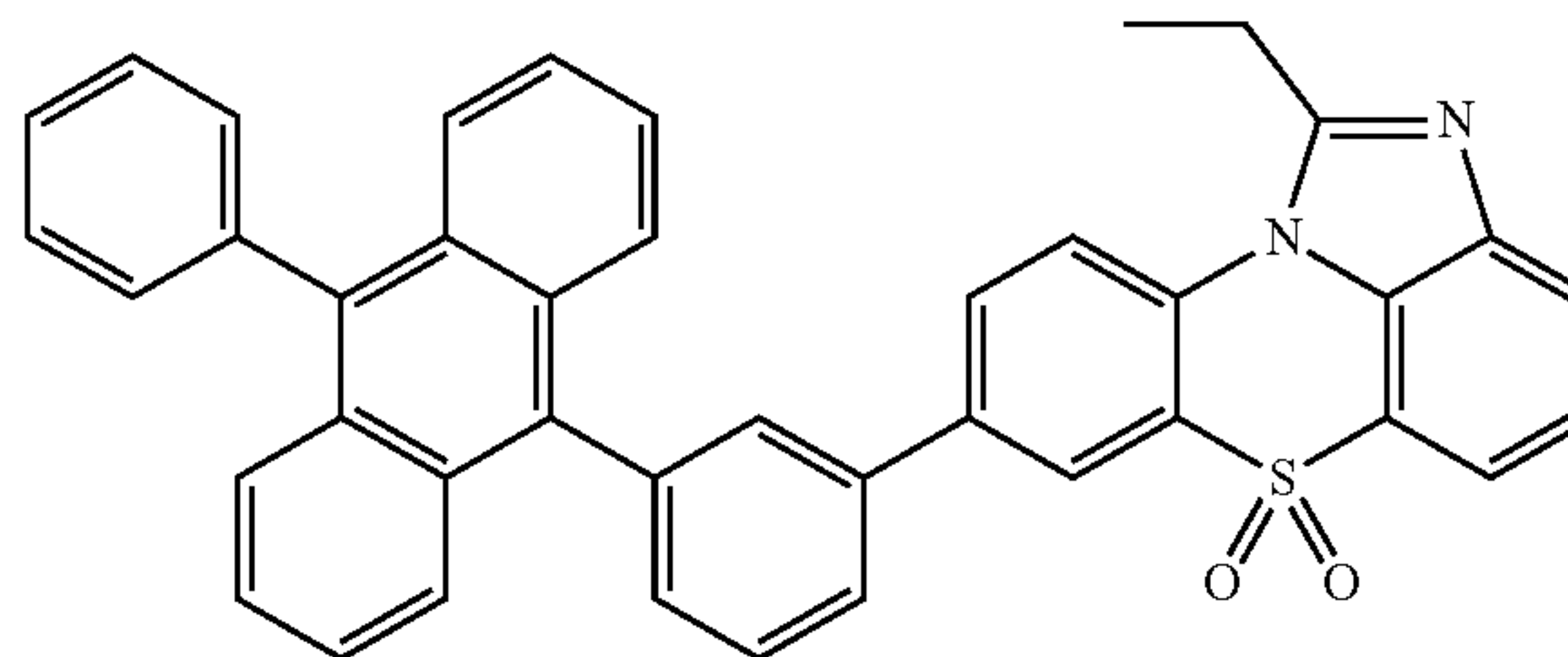
[Chemical Formula 1-3-18]
