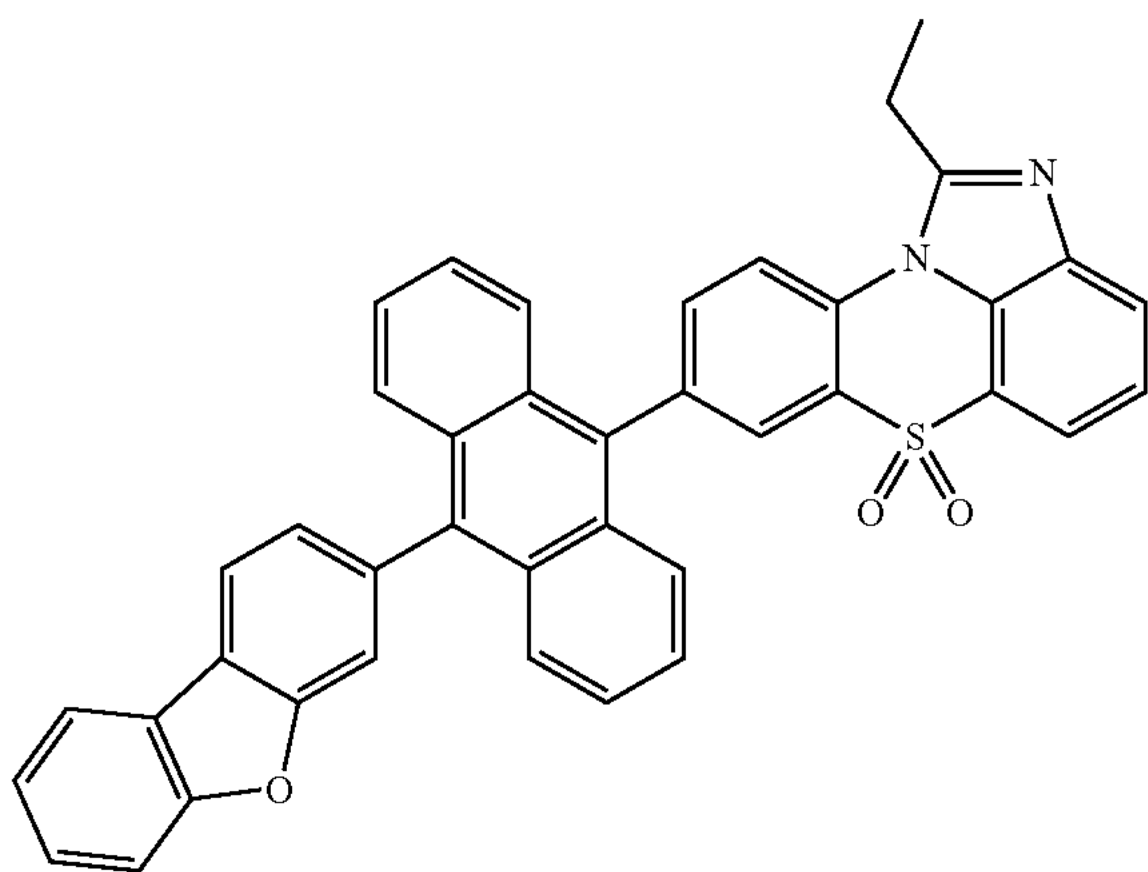
[Chemical Formula 1-3-13]
