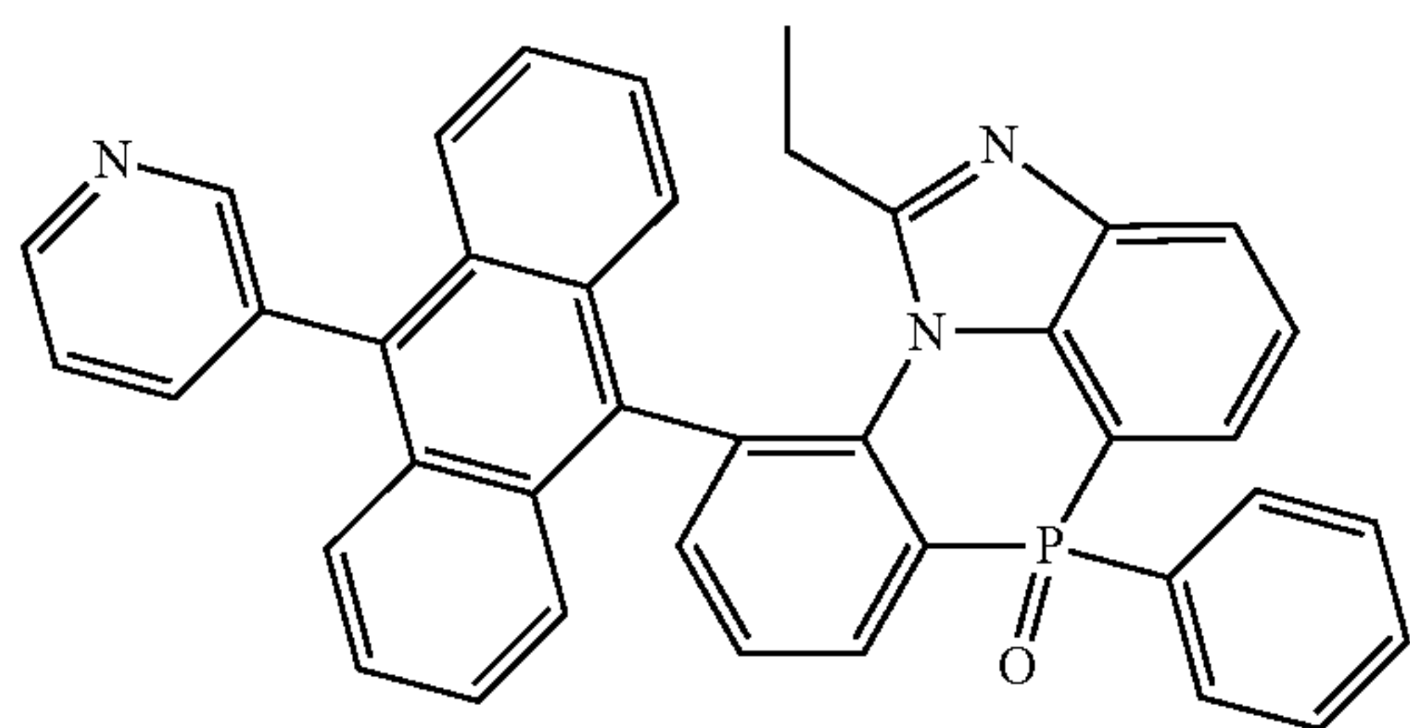
[Chemical Formula 2-8-10]
