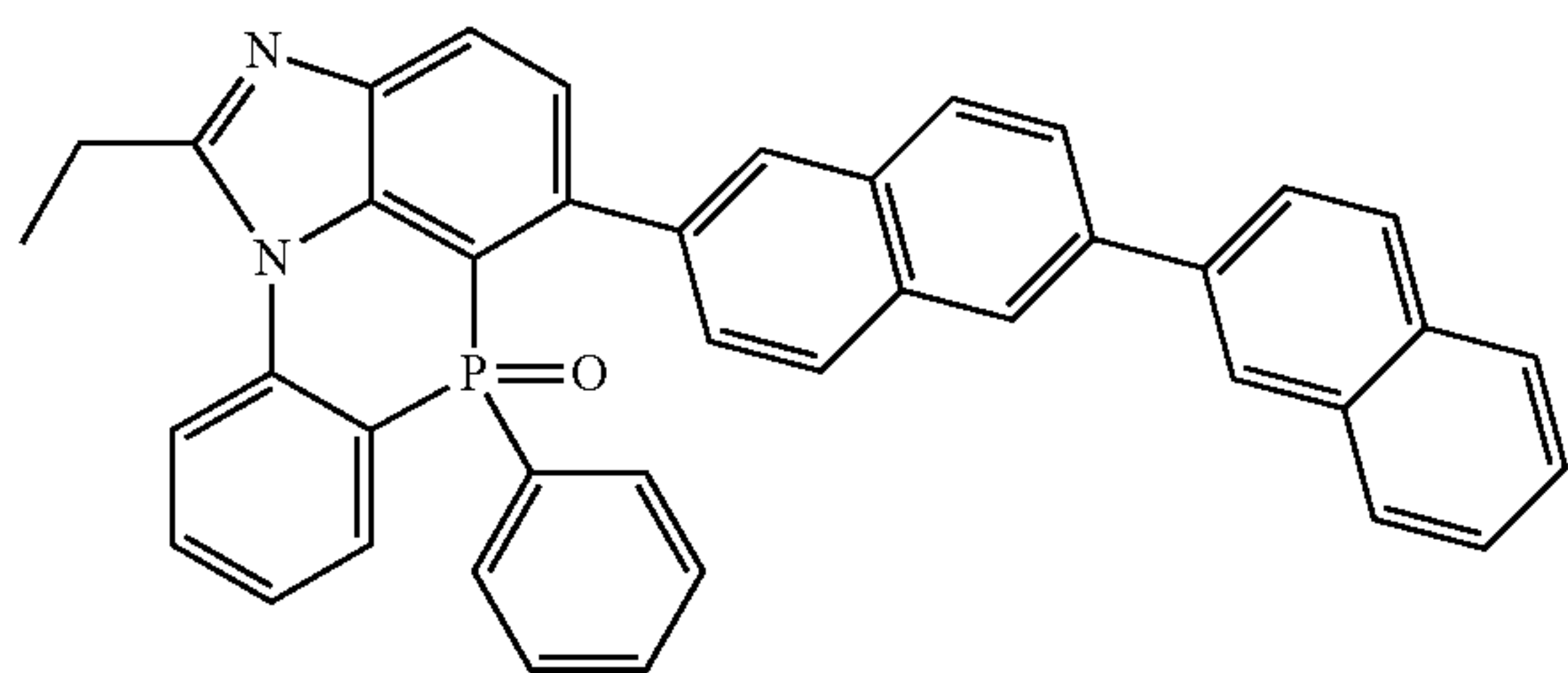
[Chemical Formula 2-9-8]
