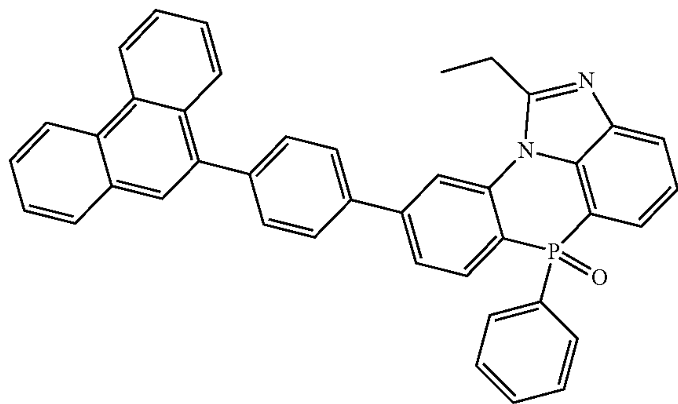
[Chemical Formula 2-7-32]
