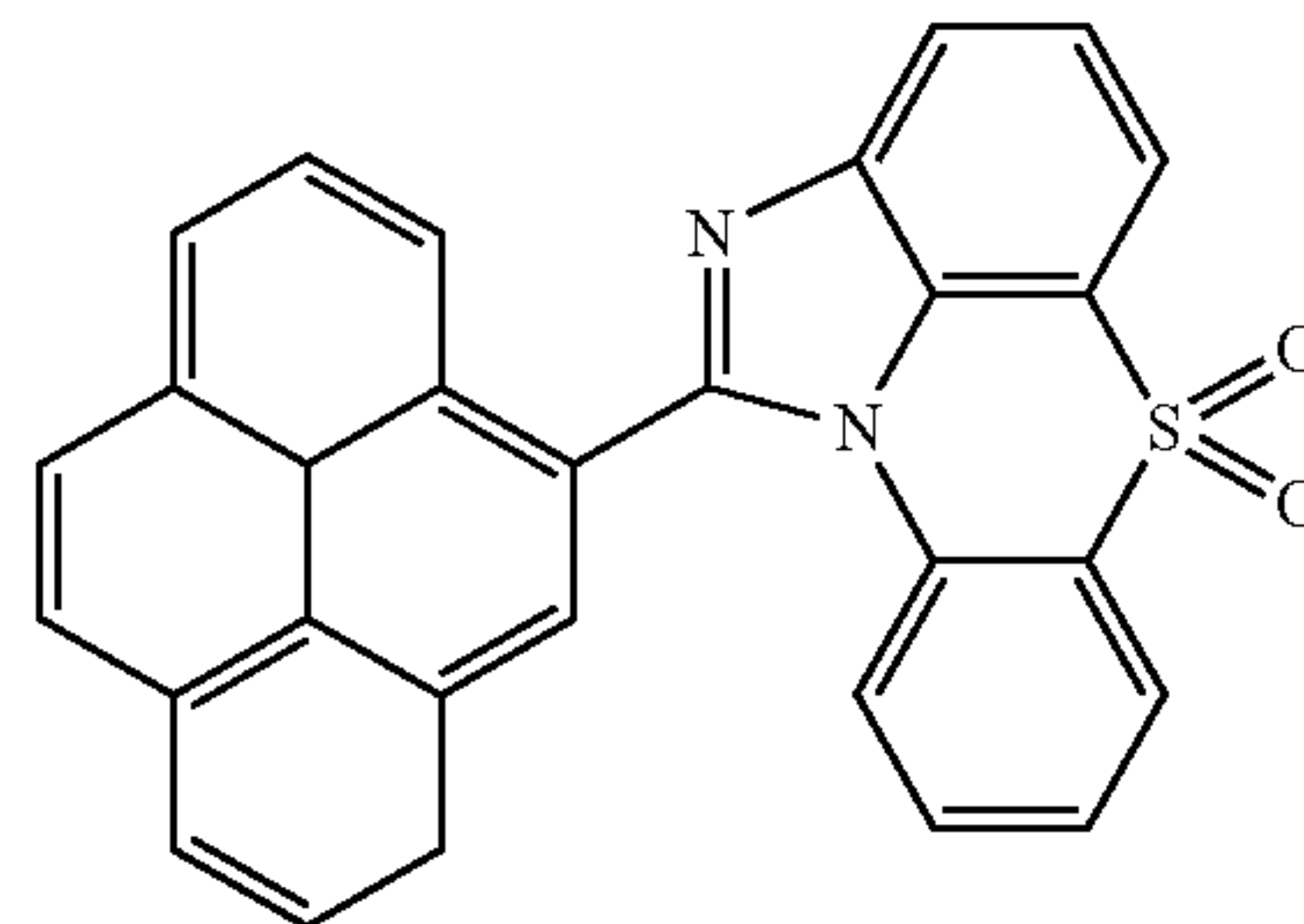
[Chemical Formula 1-5-28]
