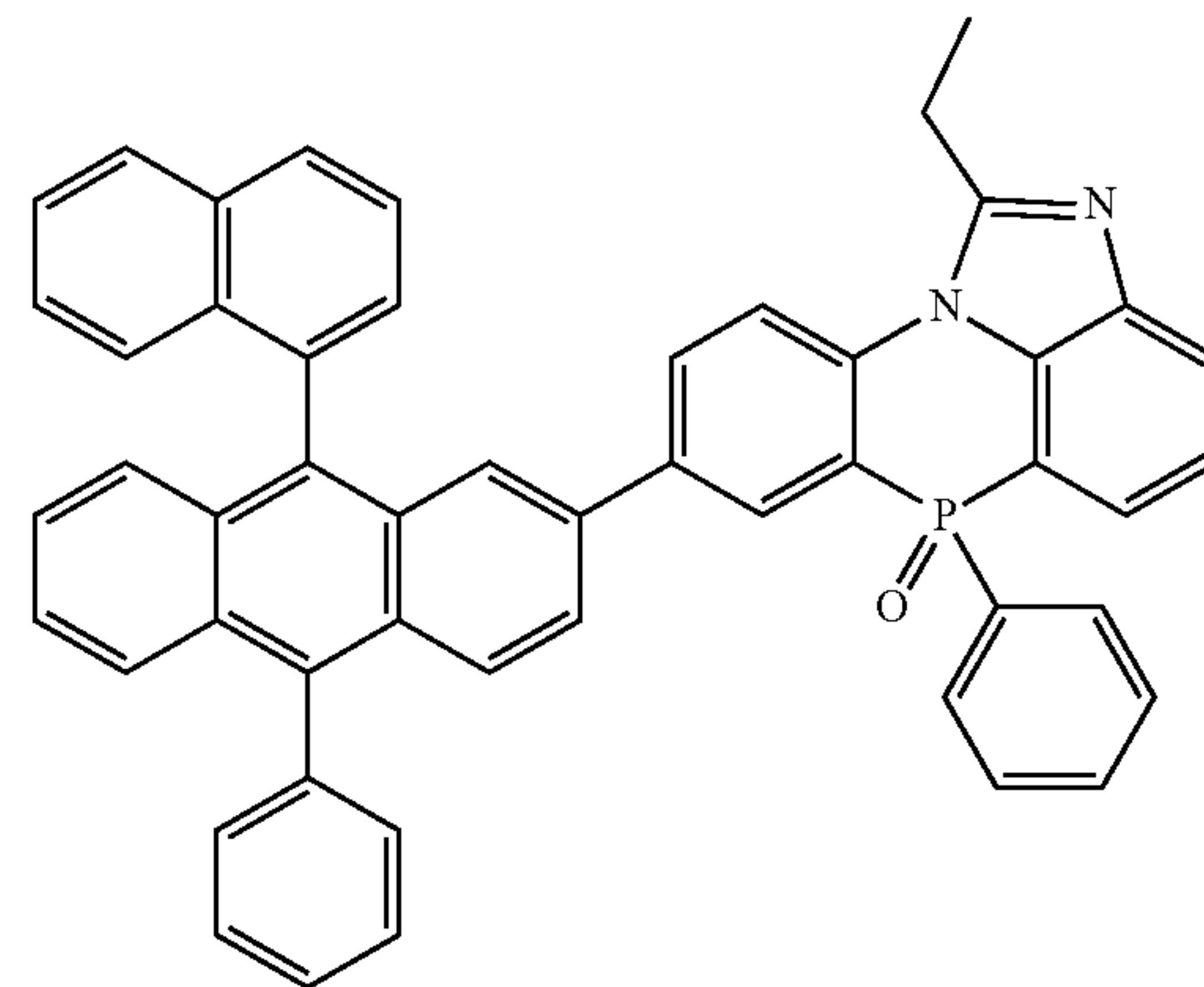
[Chemical Formula 2-3-22]
