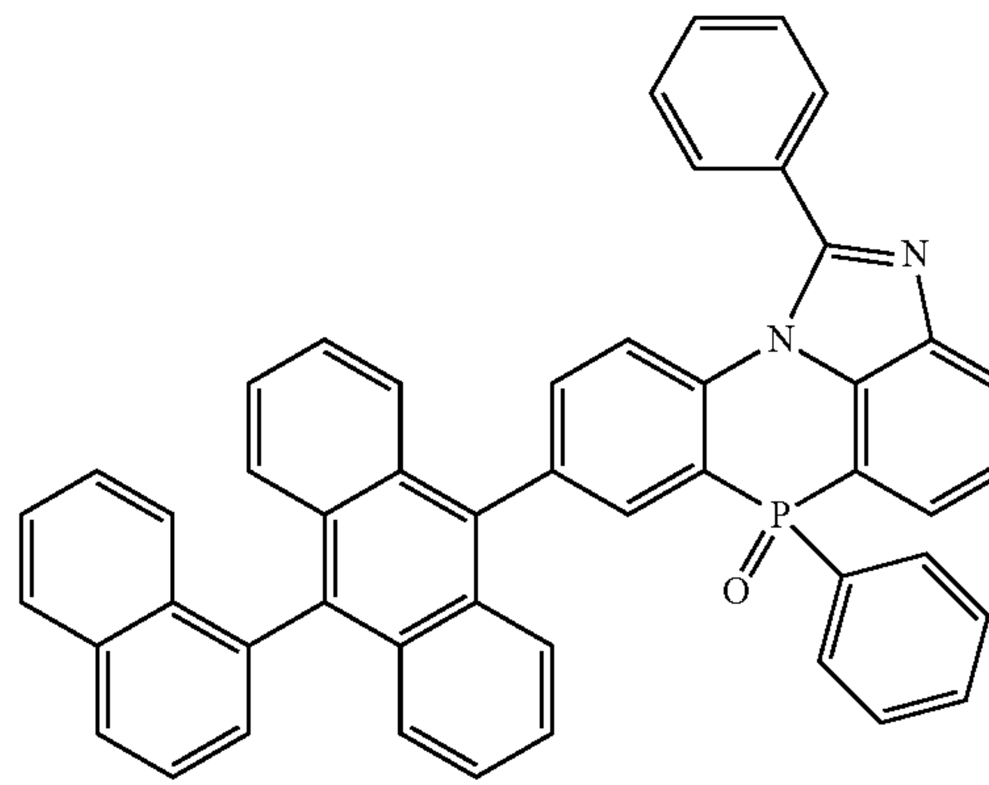
[Chemical Formula 2-4-3]
