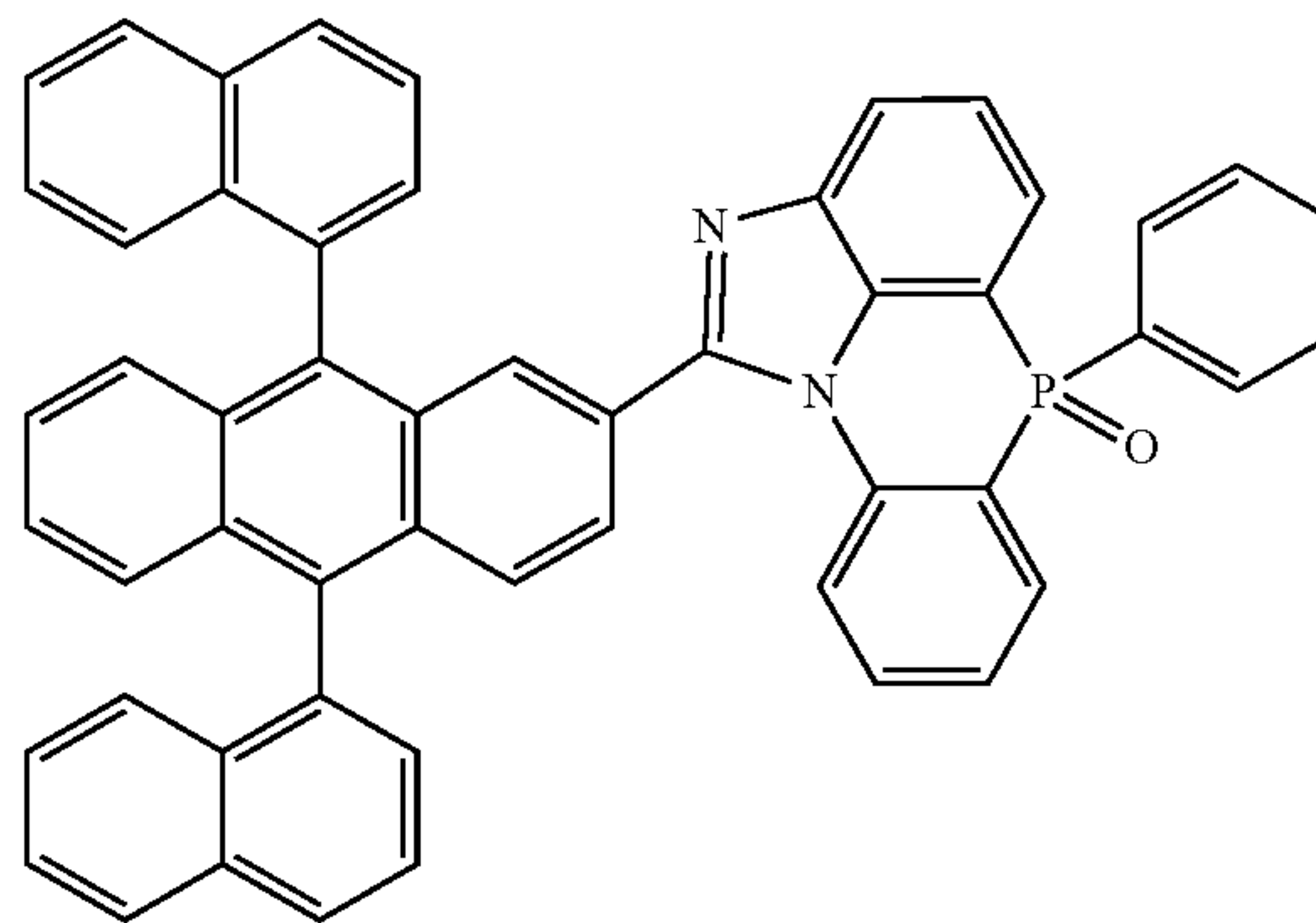
[Chemical Formula 2-5-21]
