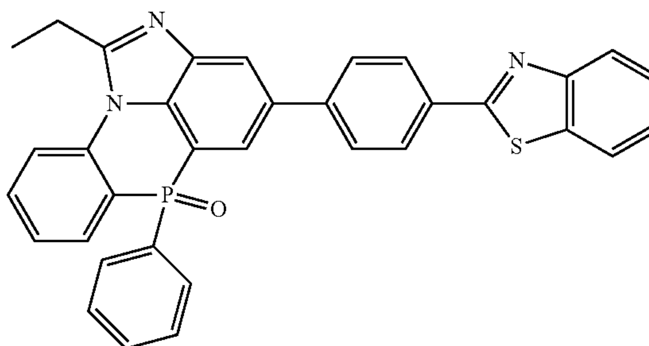
[Chemical Formula 2-10-11]
