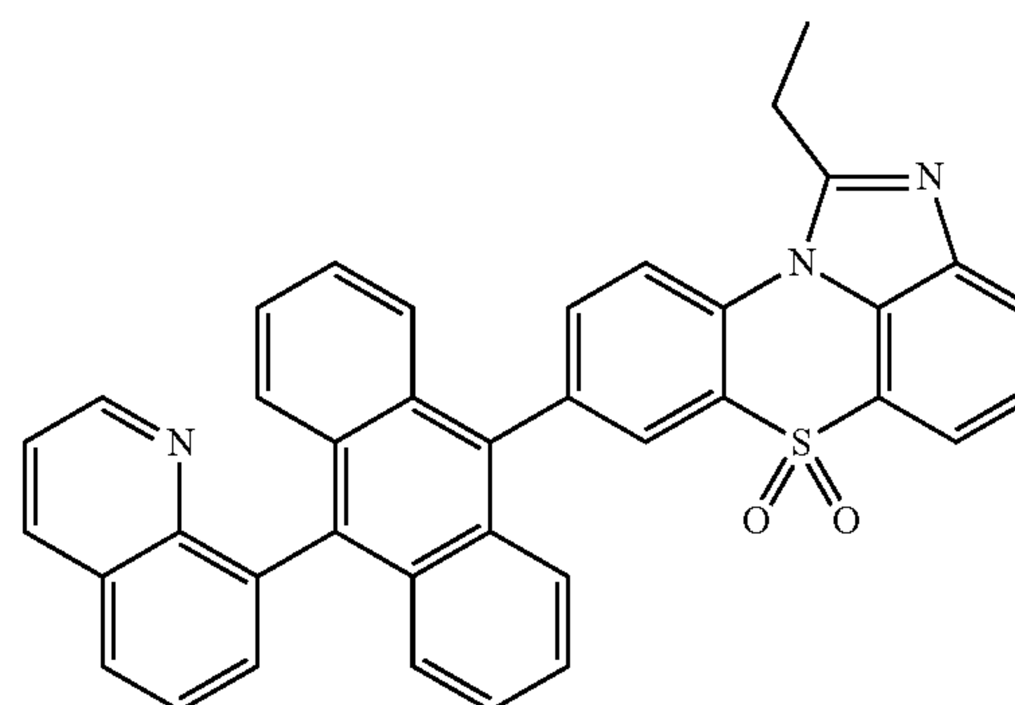
[Chemical Formula 1-3-11]
