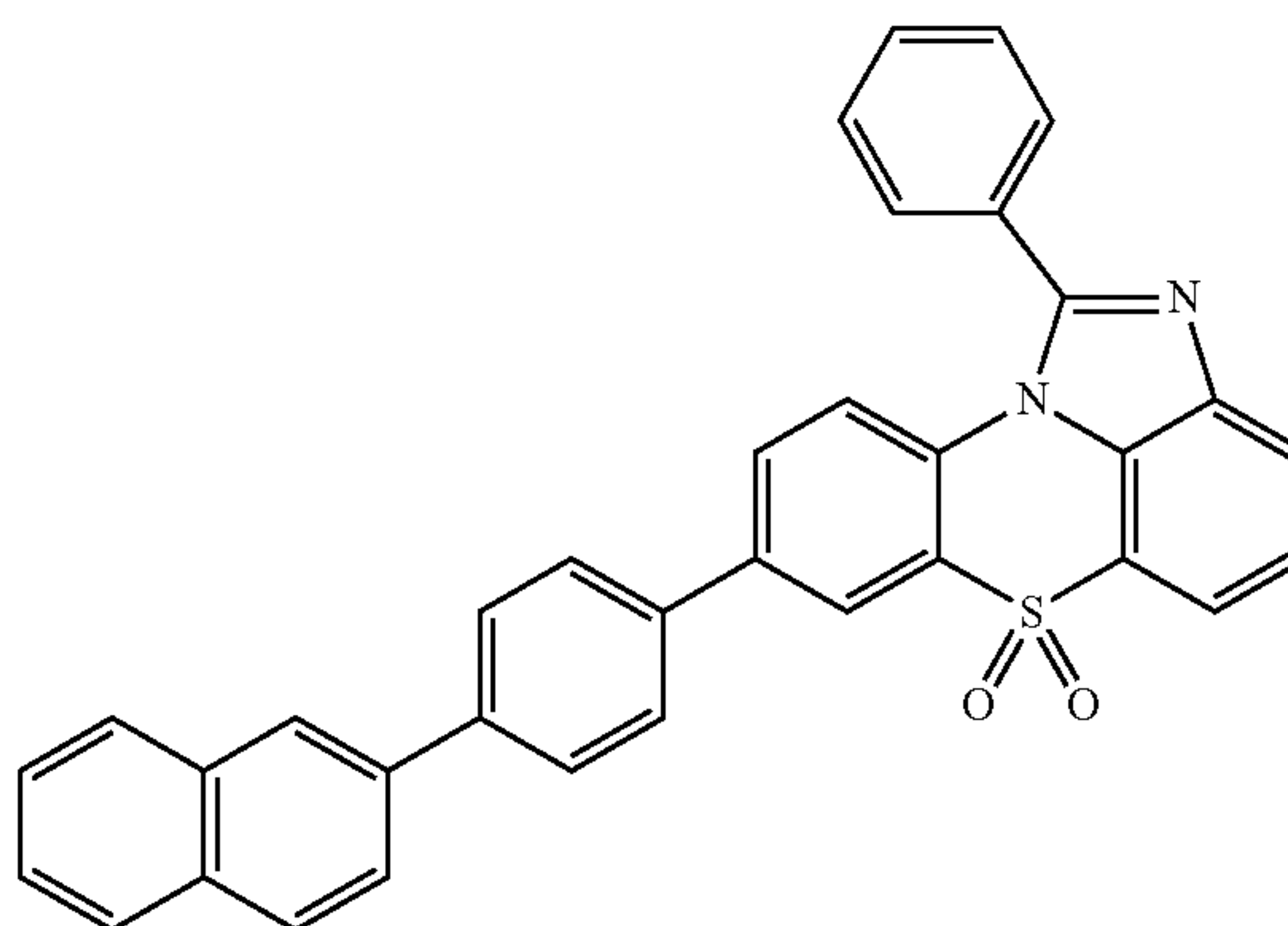
[Chemical Formula 1-4-27]
