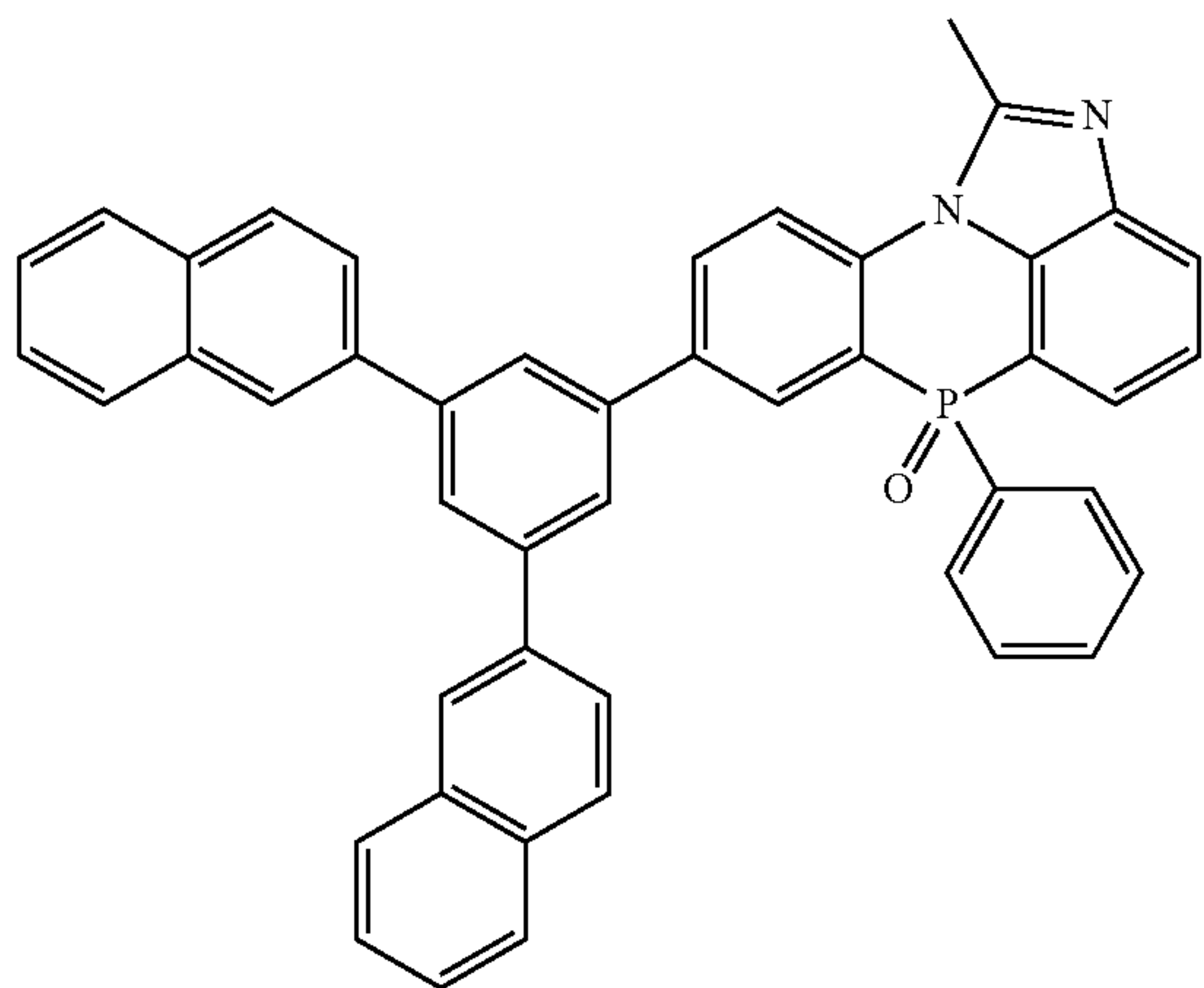
[Chemical Formula 2-2-44]
