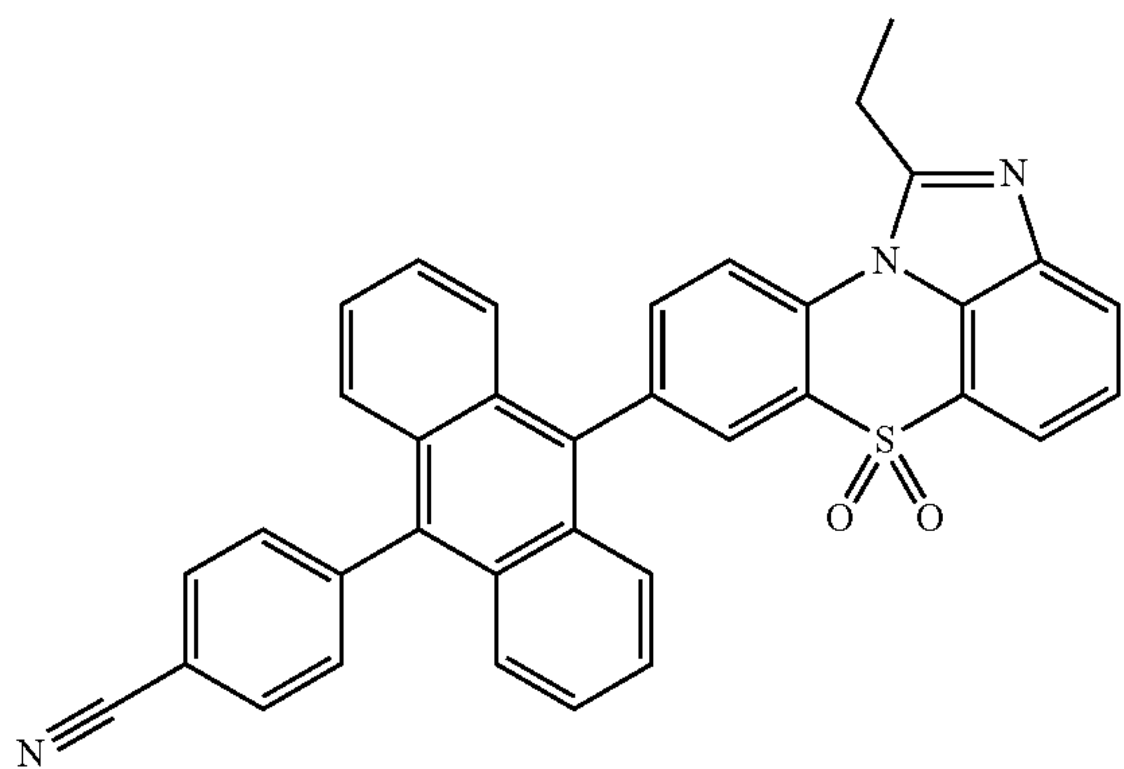
[Chemical Formula 1-3-13]
