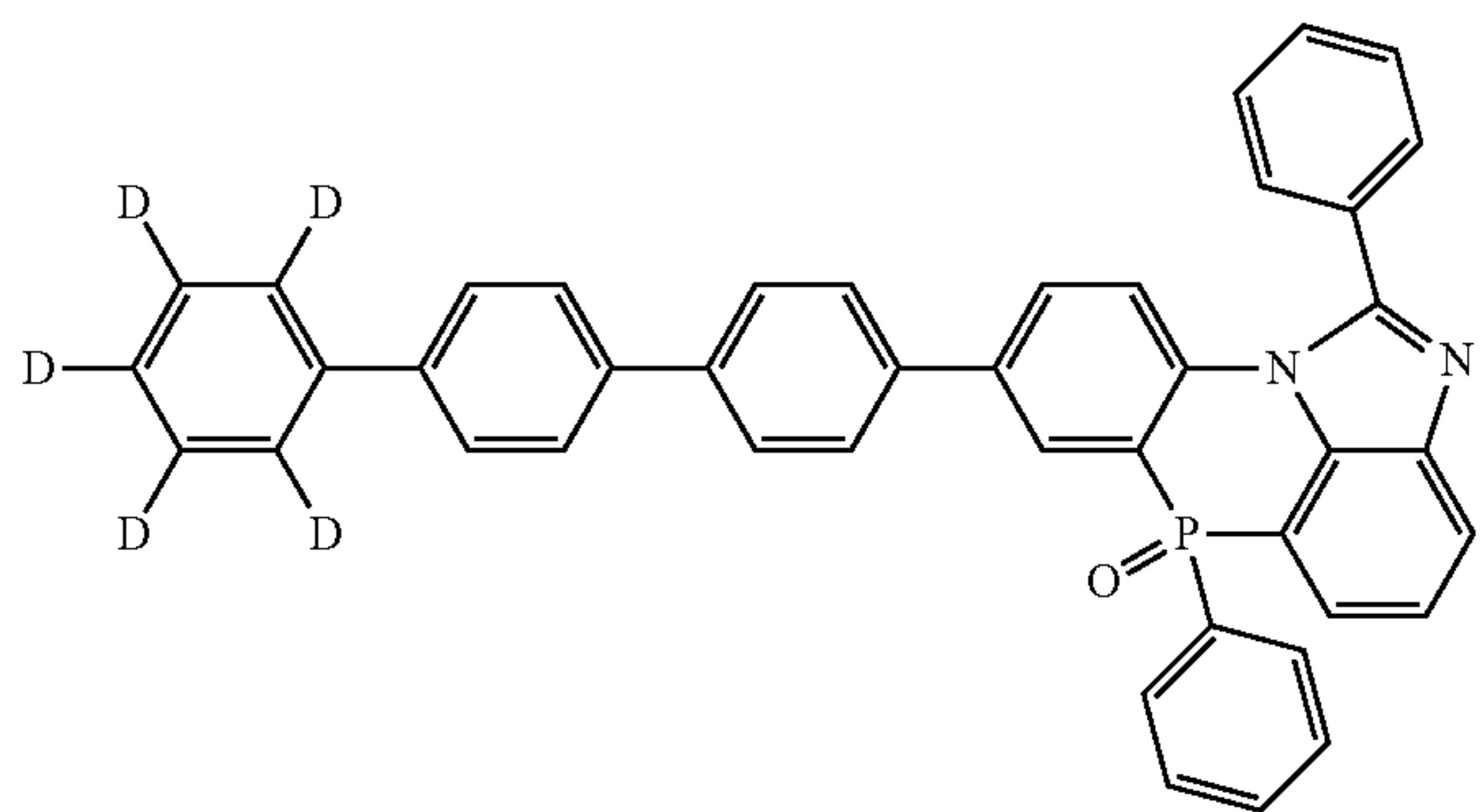
[Chemical Formula 2-4-52]
