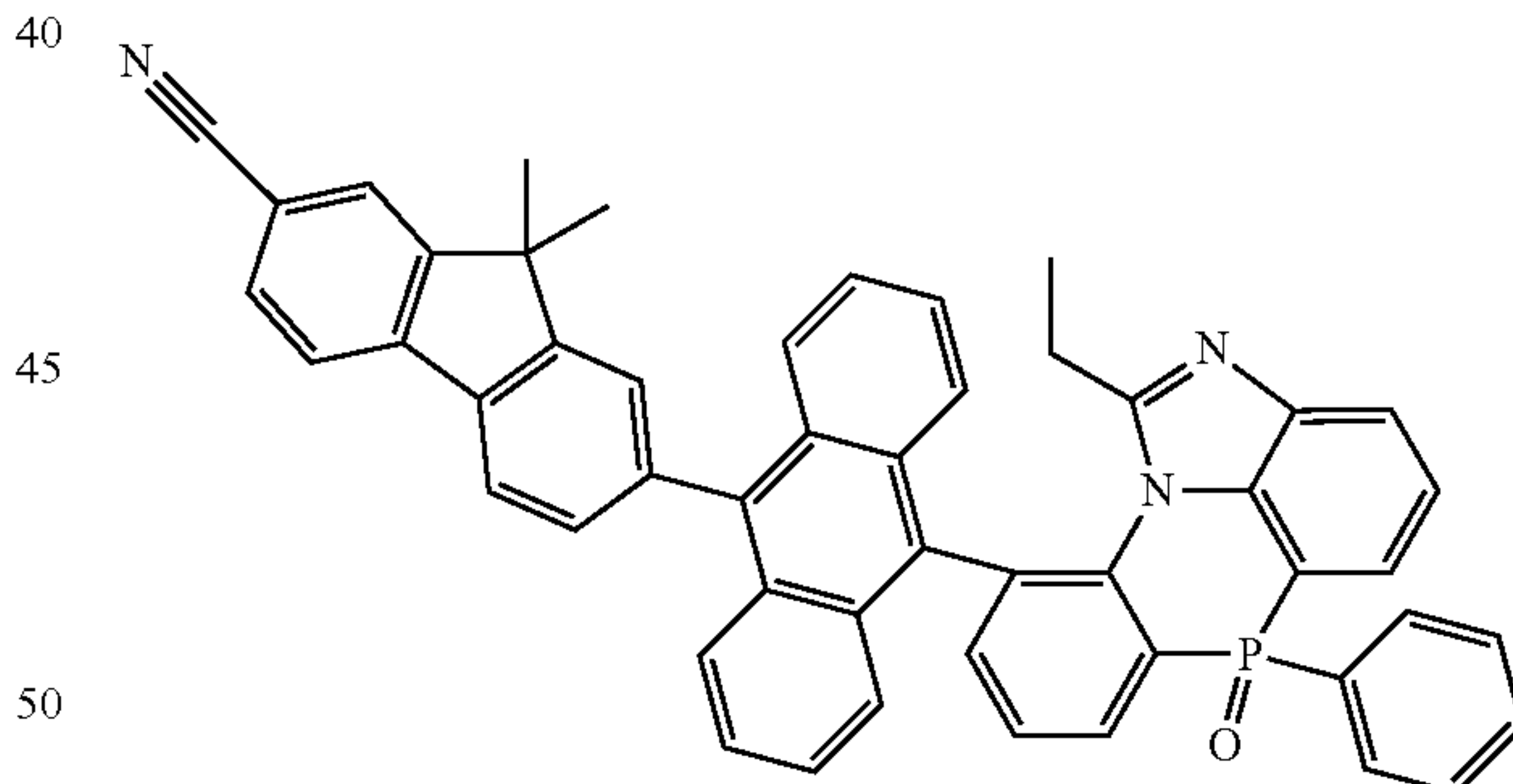
[Chemical Formula 2-8-16]
