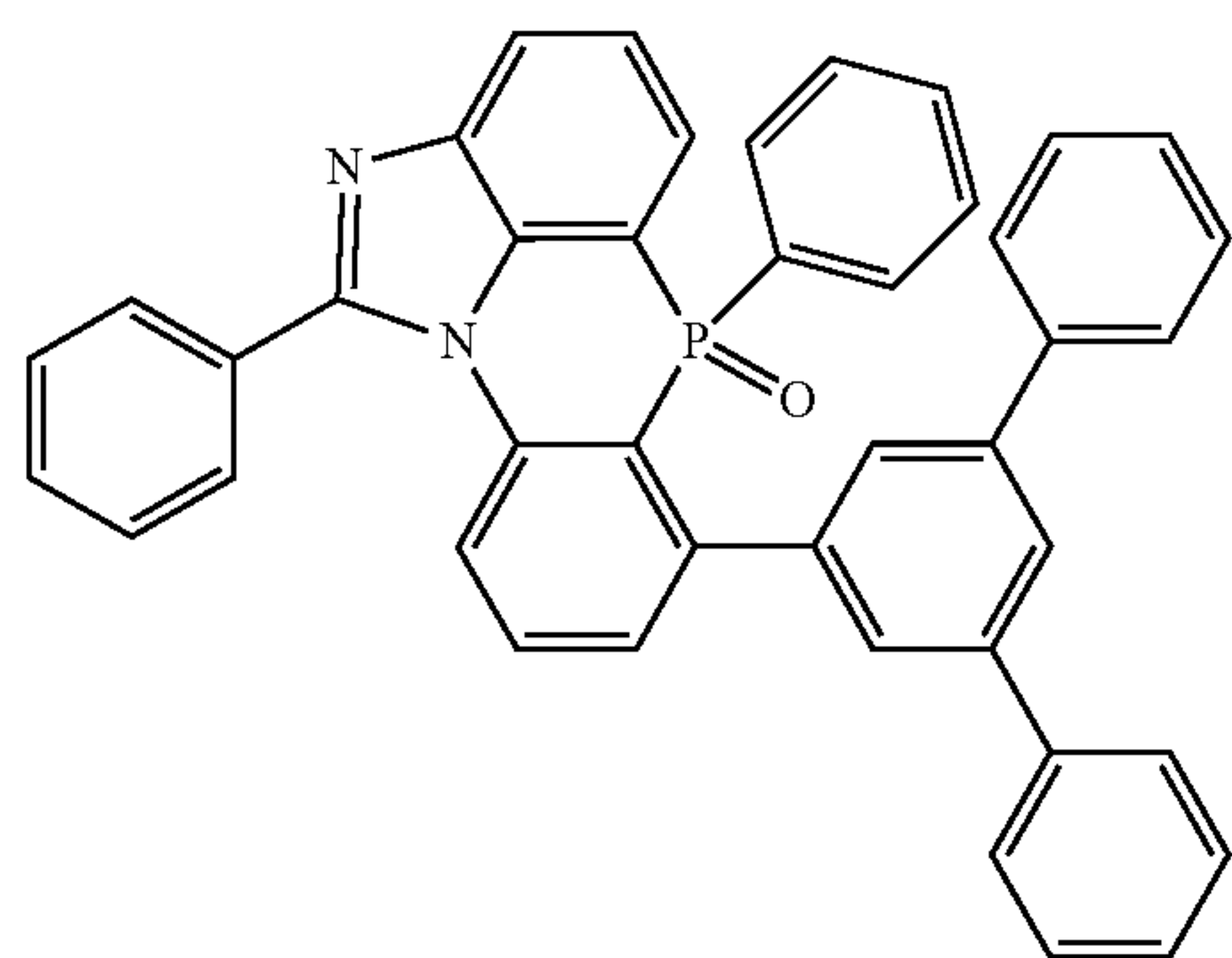
[Chemical Formula 2-6-40]
