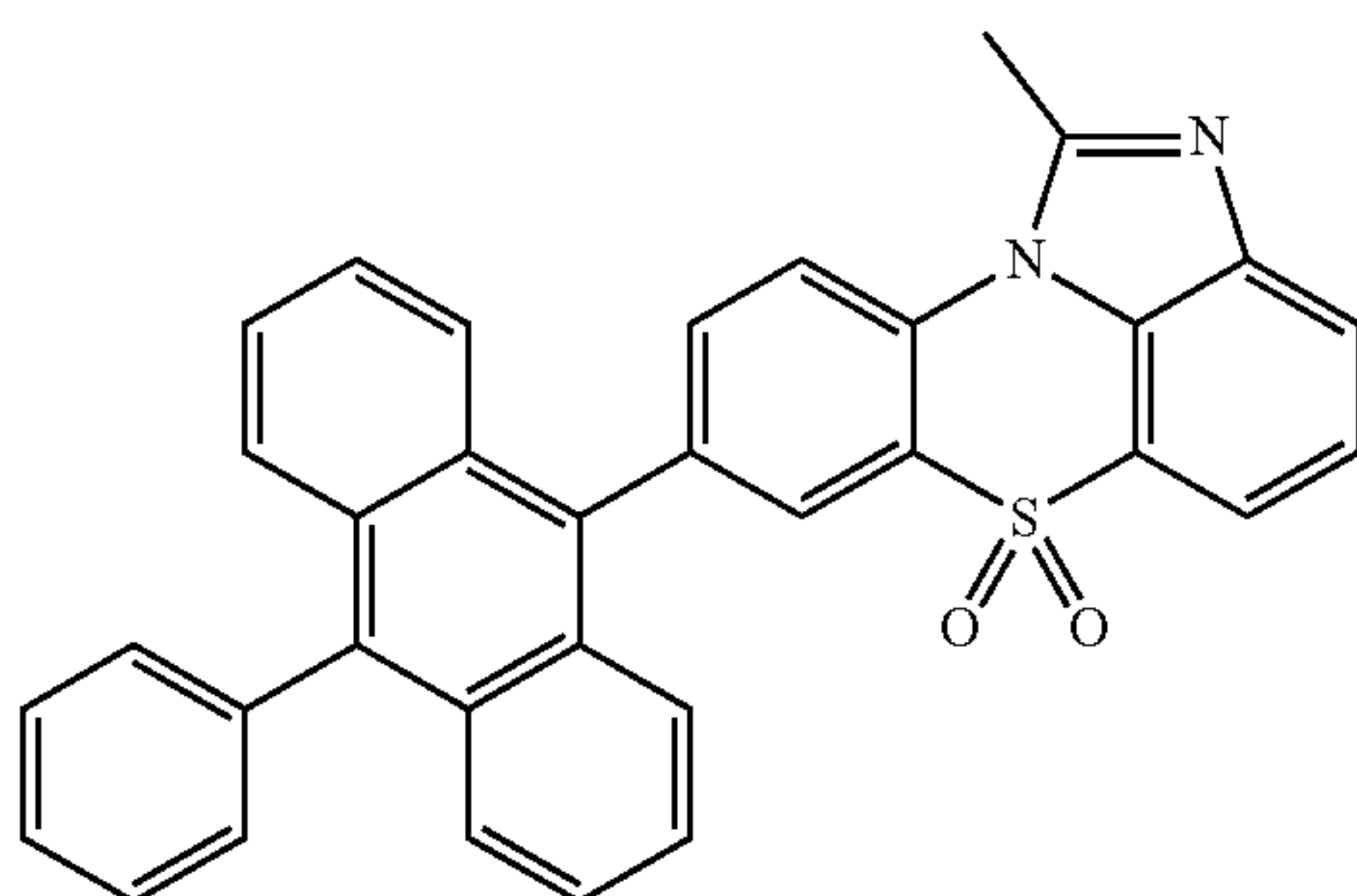
[Chemical Formula 1-2-1]
