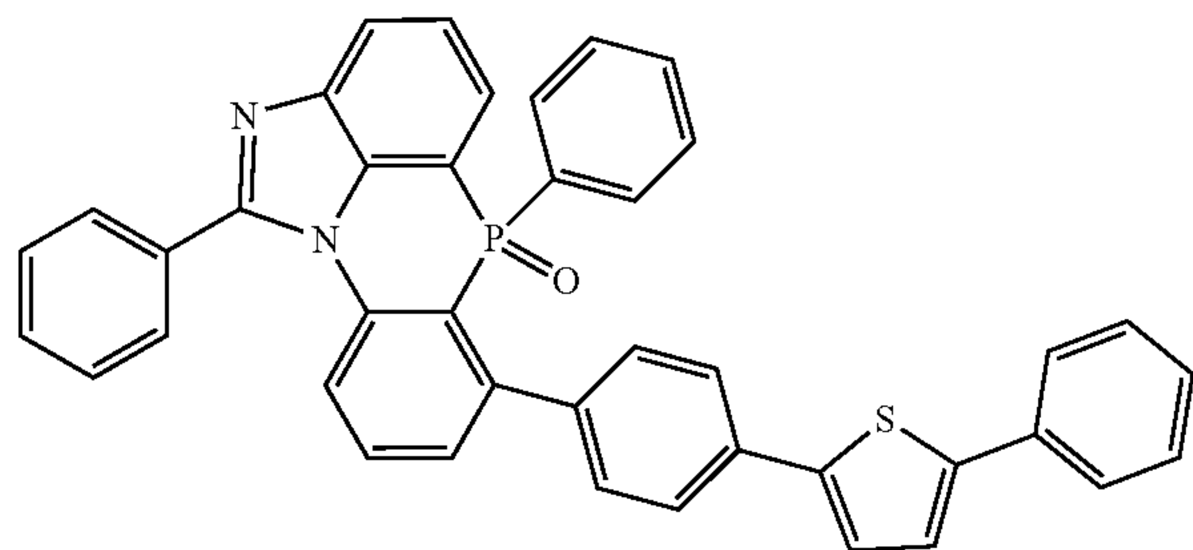
[Chemical Formula 2-6-39]
