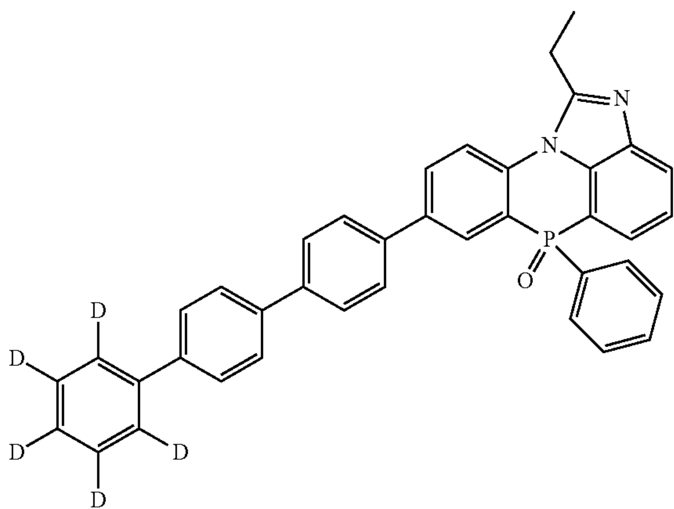
[Chemical Formula 2-3-52]
