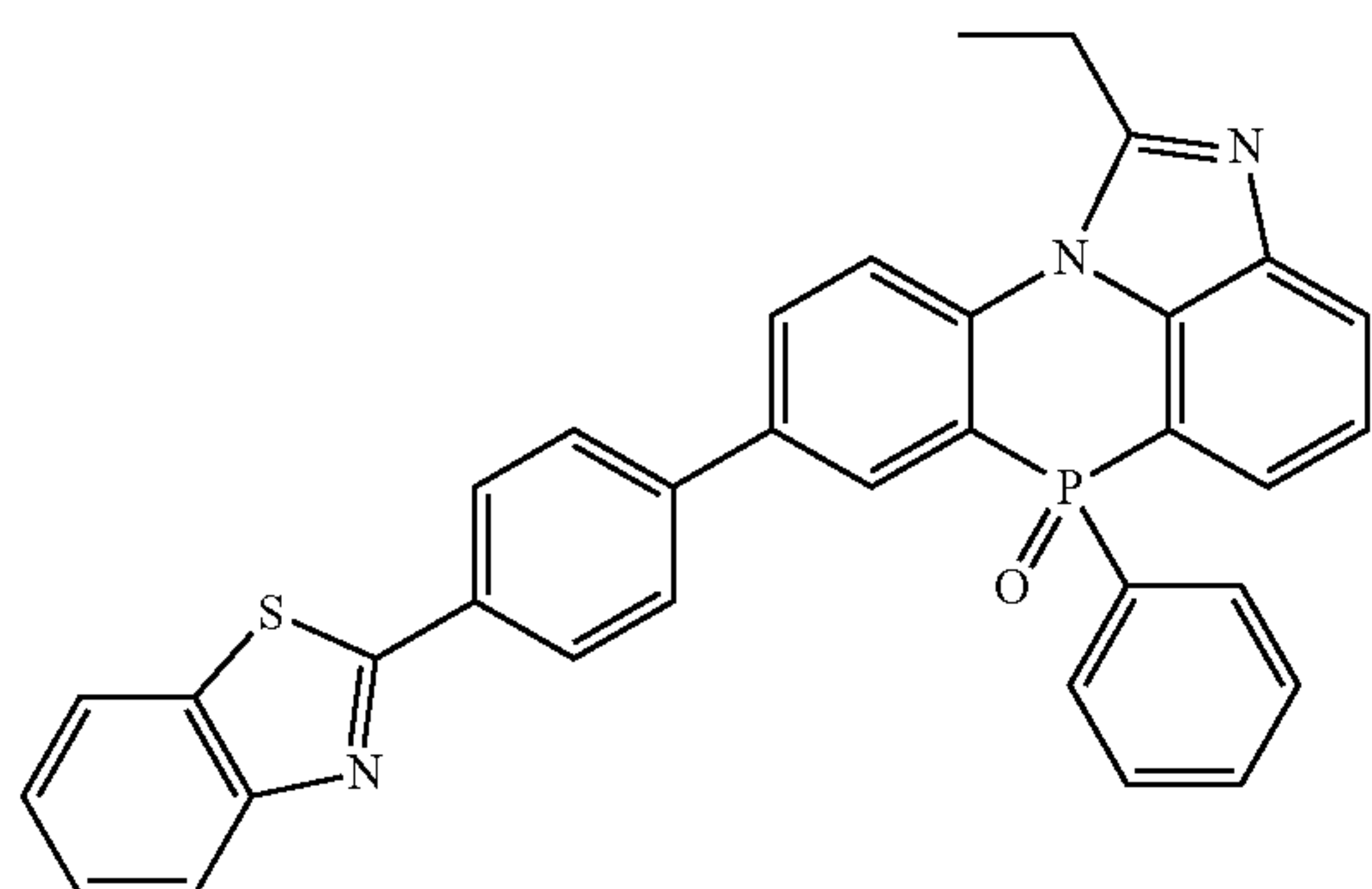
[Chemical Formula 2-3-46]
