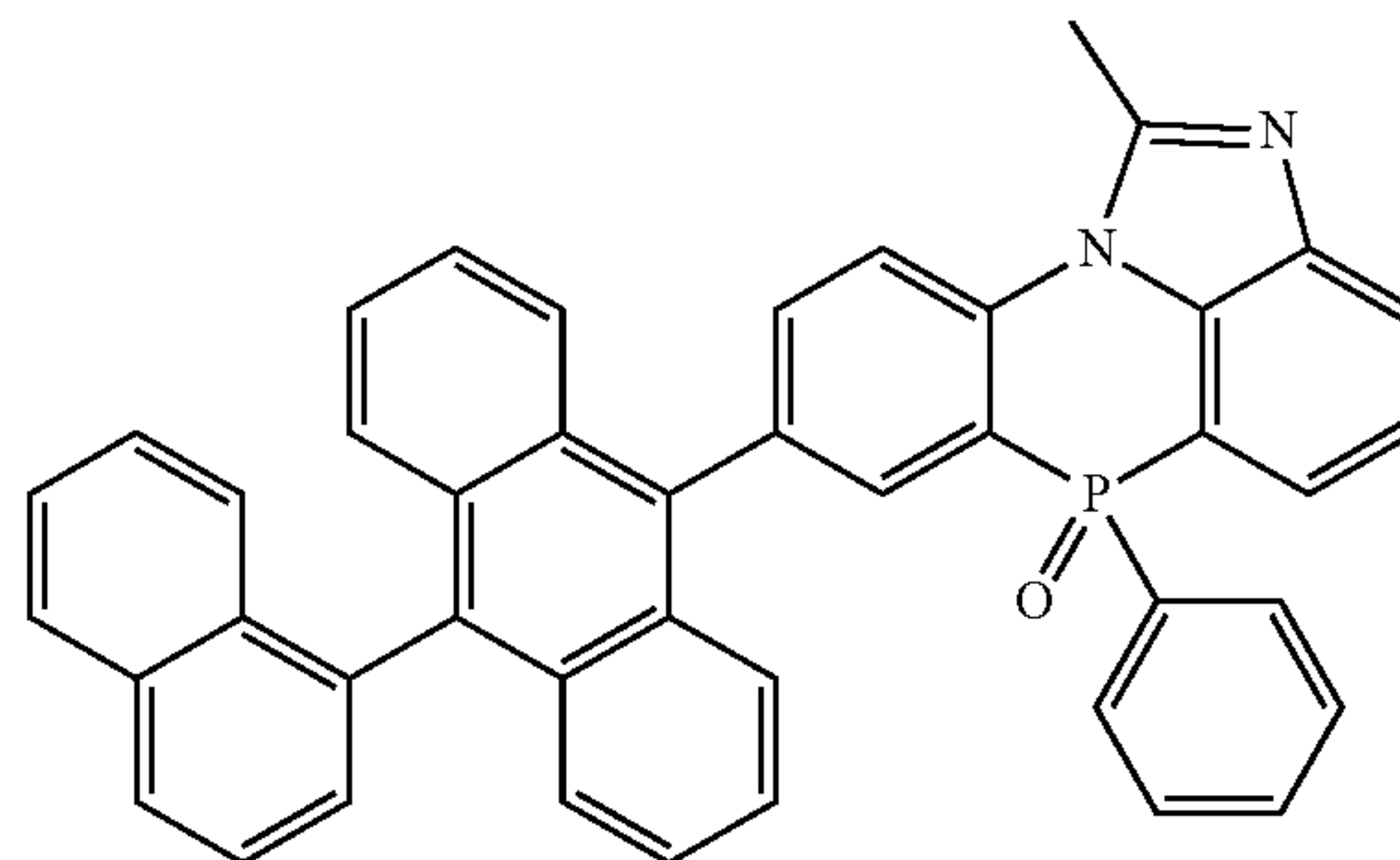
[Chemical Formula 2-2-3]
