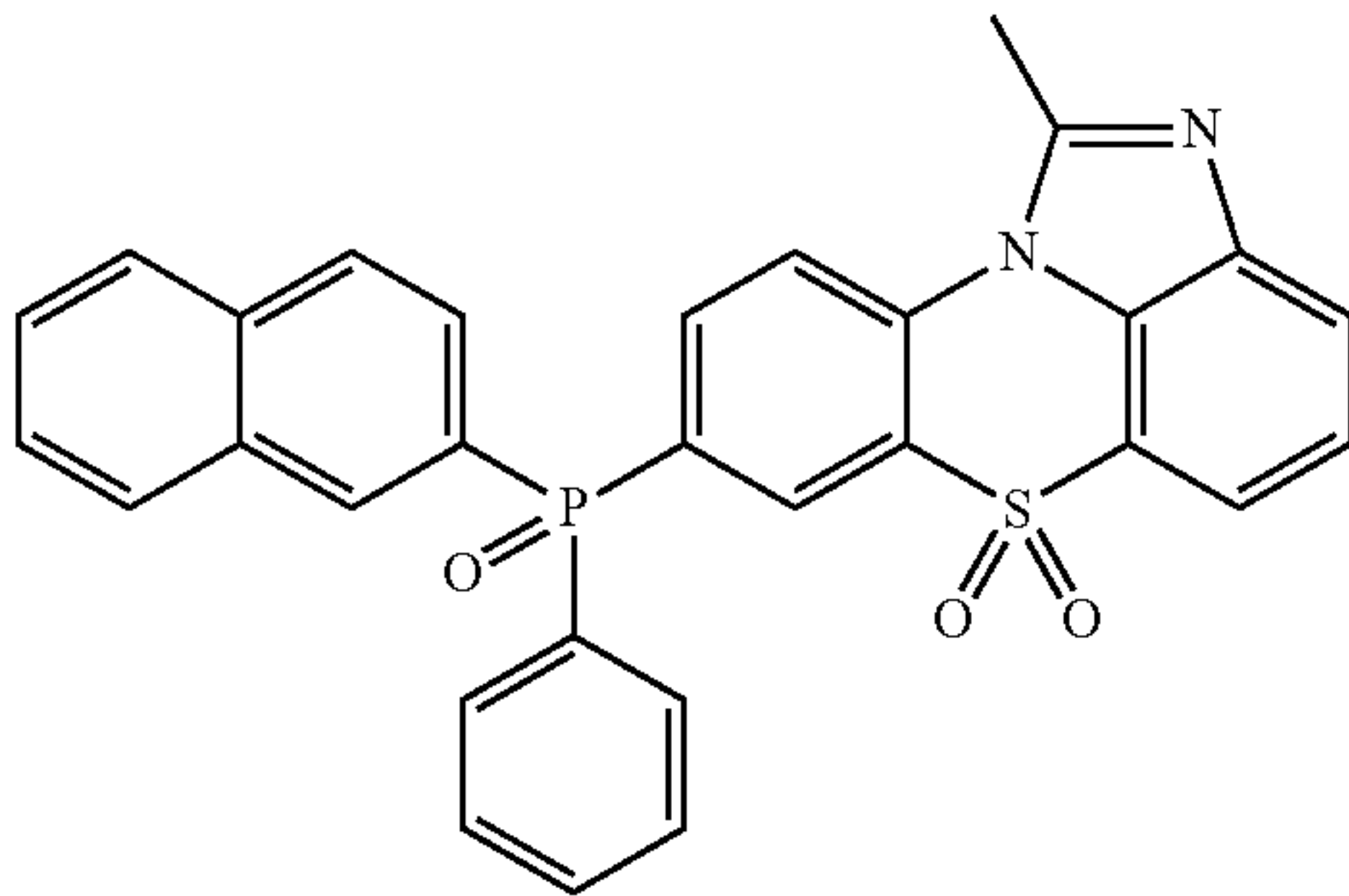
[Chemical Formula 1-12-5]
