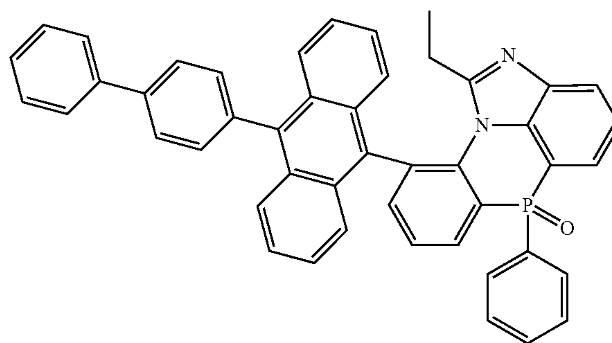
[Chemical Formula 2-8-4]
