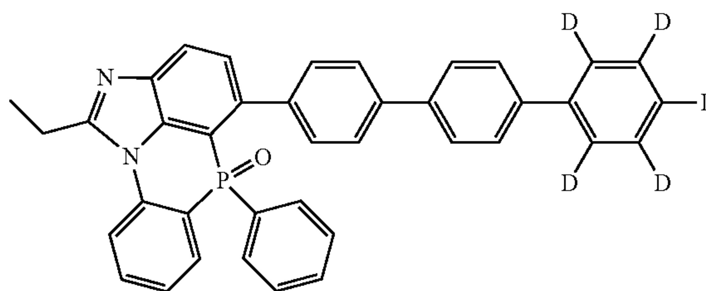
[Chemical Formula 2-9-16]
