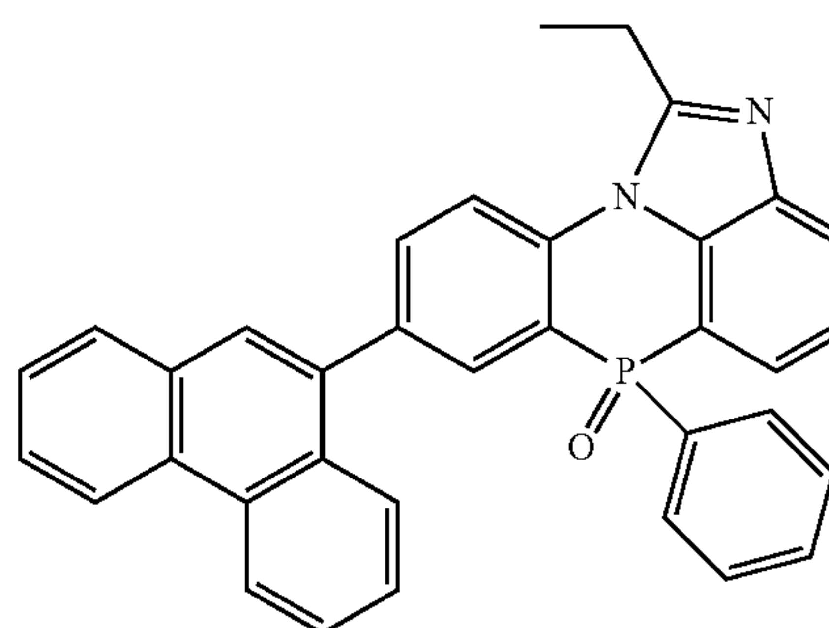
[Chemical Formula 2-3-31]
