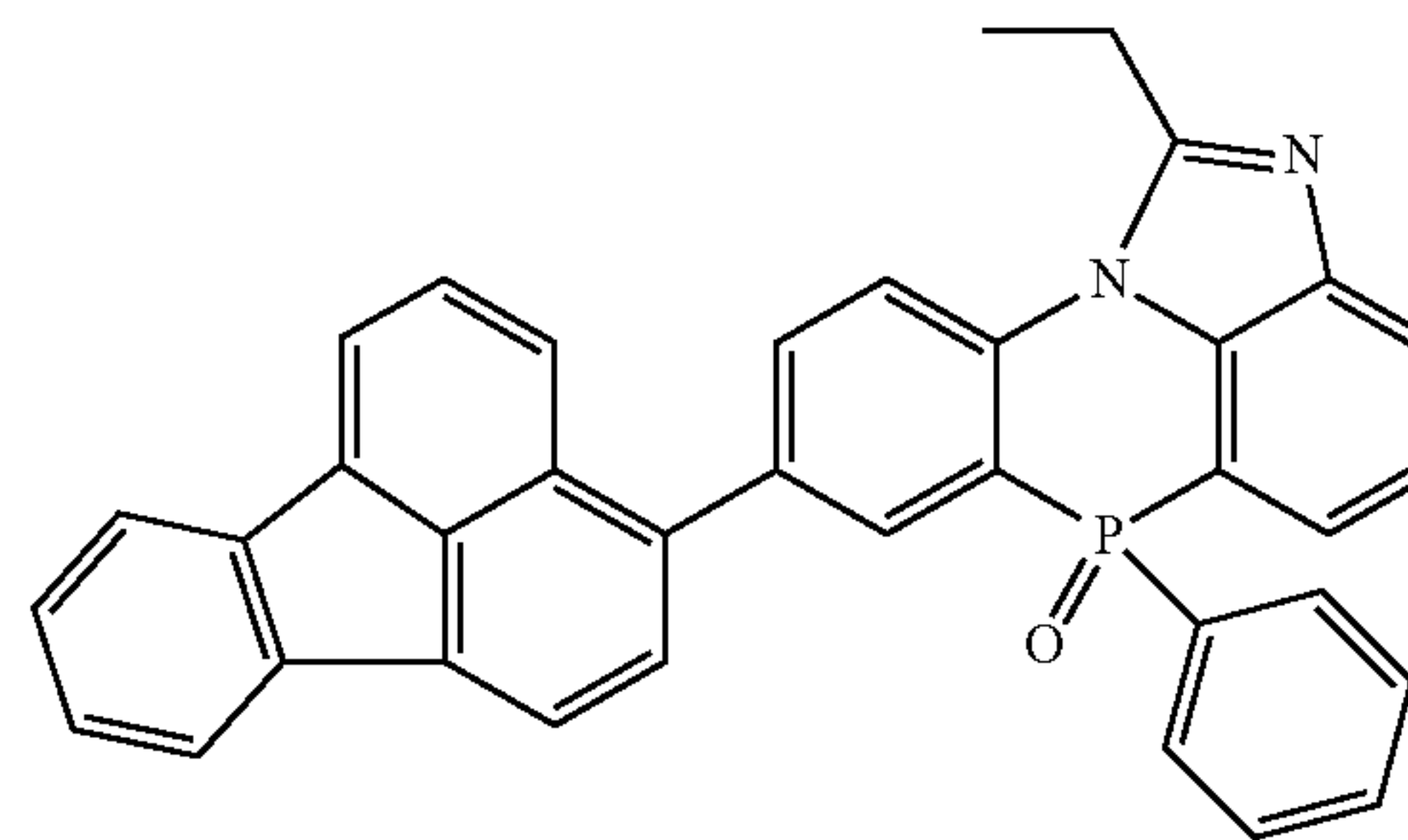
[Chemical Formula 2-3-30]
