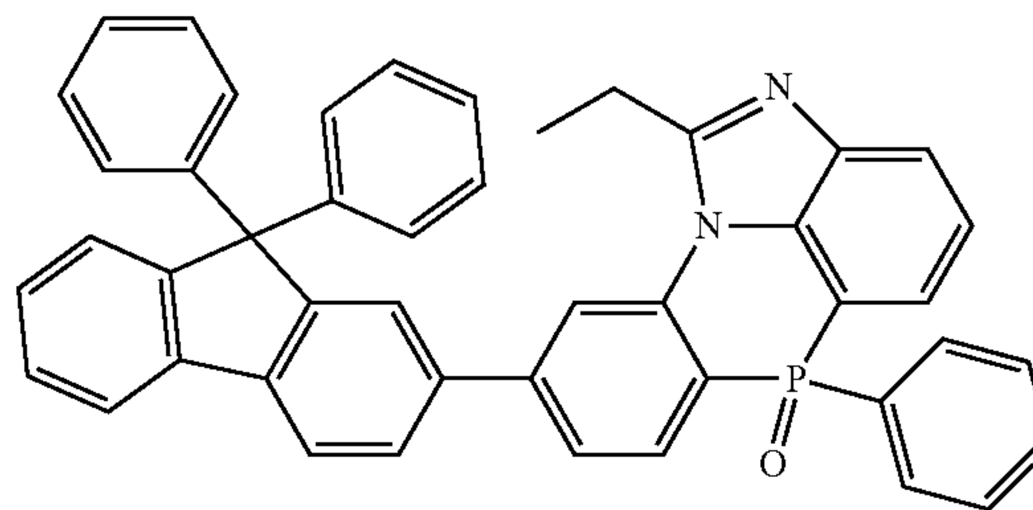
[Chemical Formula 2-7-35]
