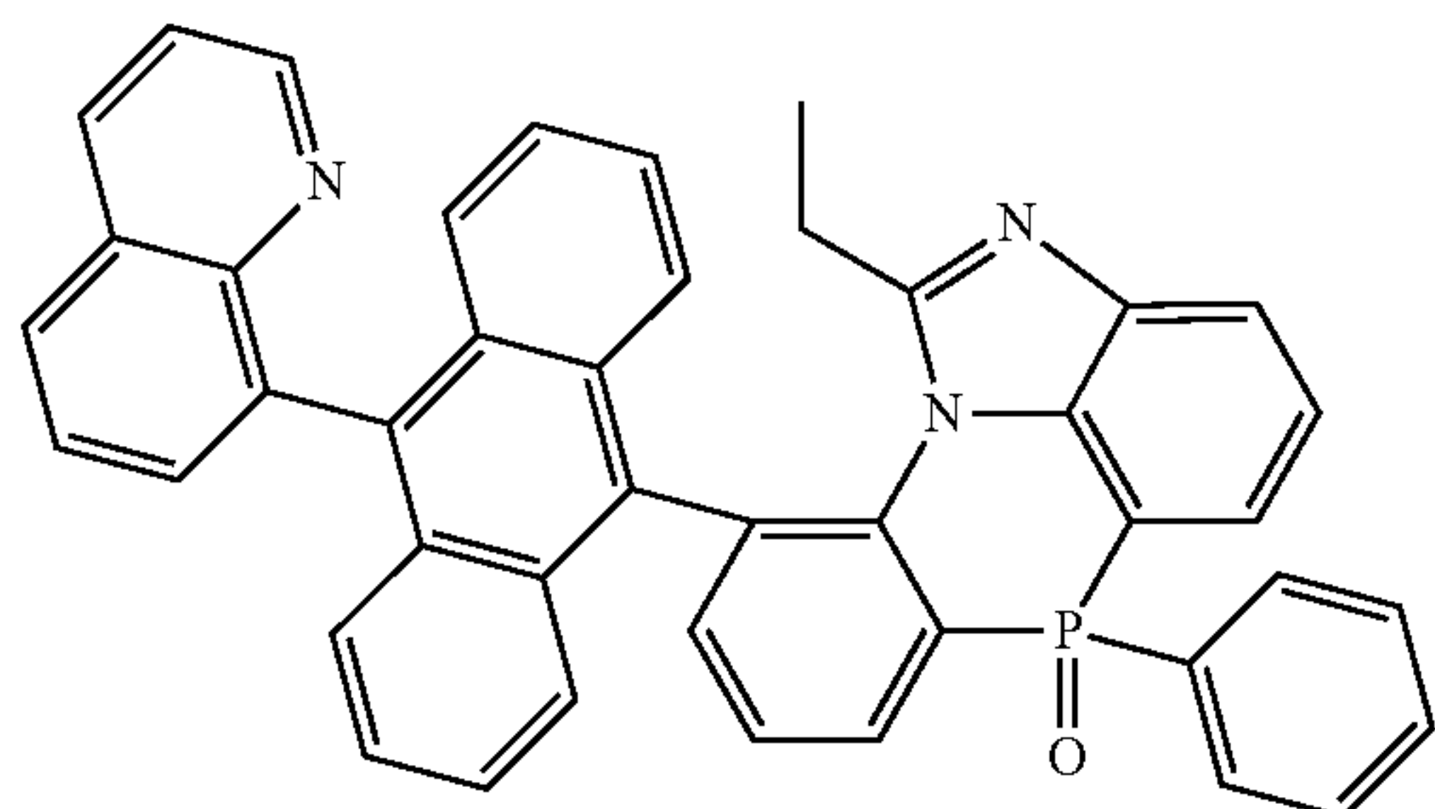
[Chemical Formula 2-8-11]
