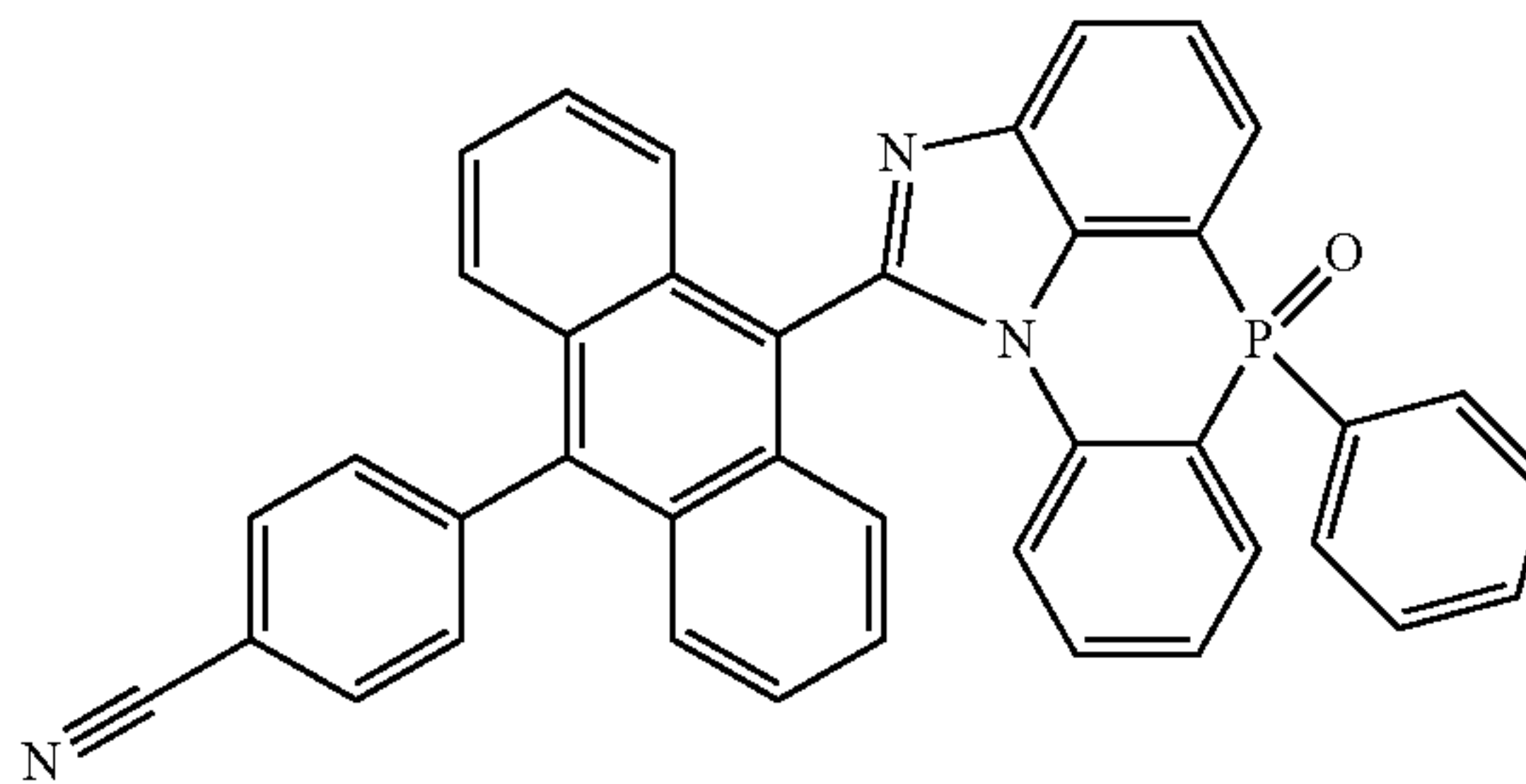
[Chemical Formula 2-5-12]
