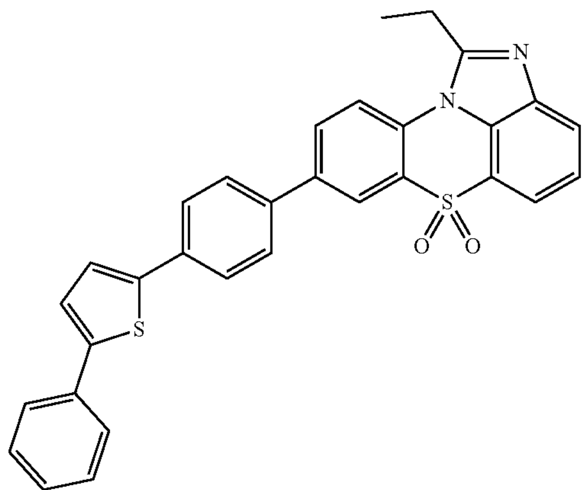
[Chemical Formula 1-3-39]
