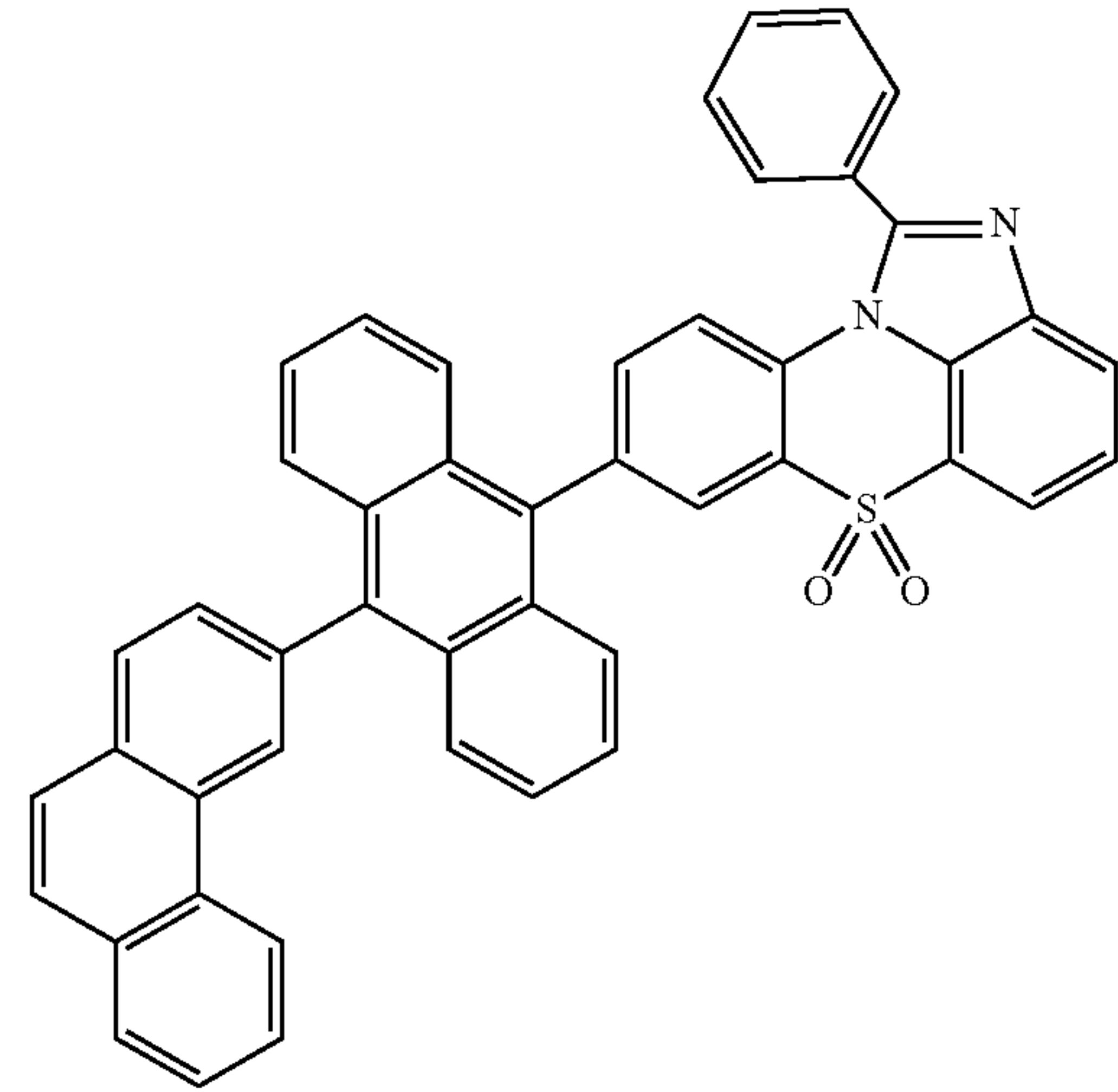
[Chemical Formula 1-4-8]
