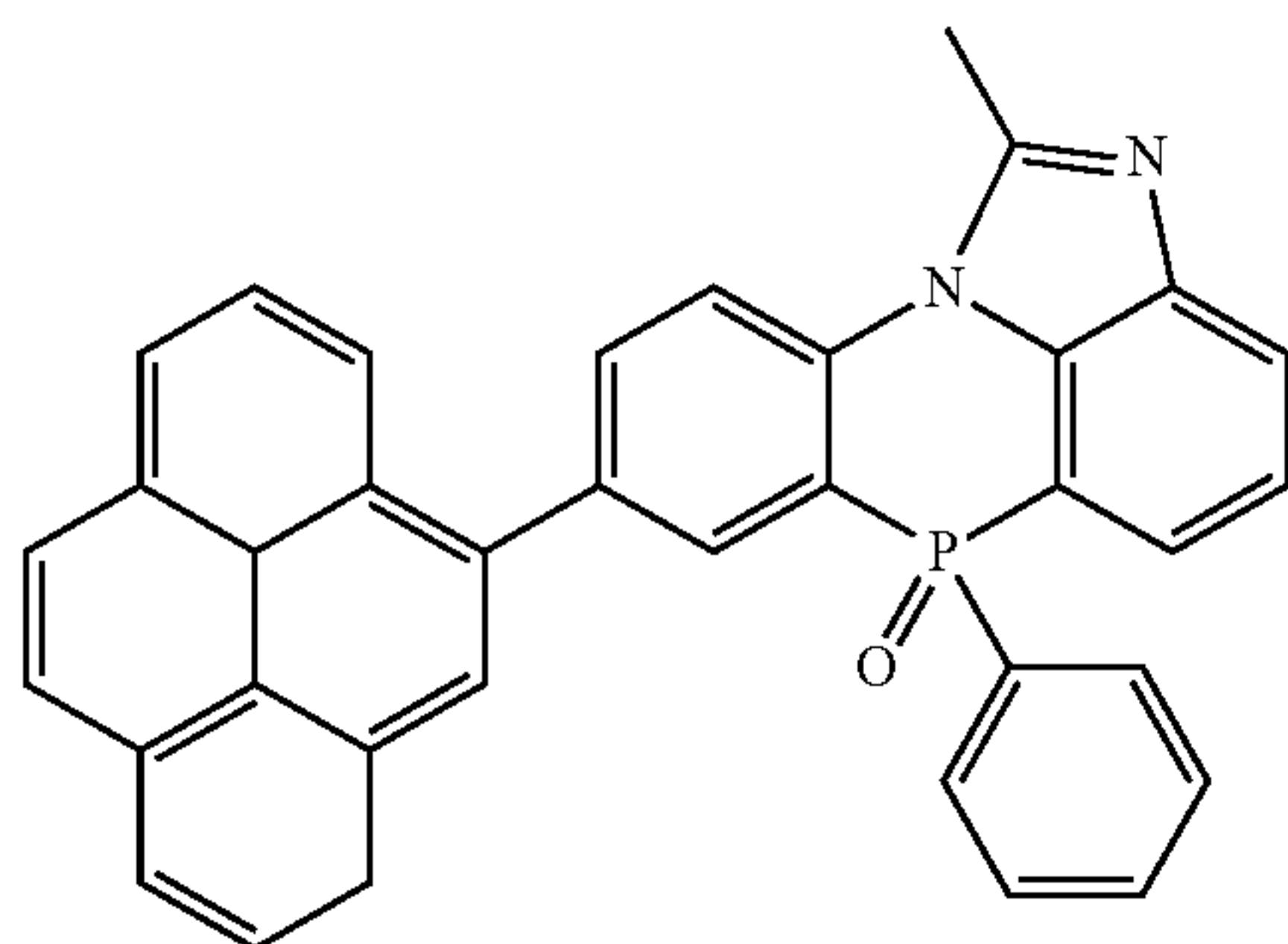
[Chemical Formula 2-2-28]
