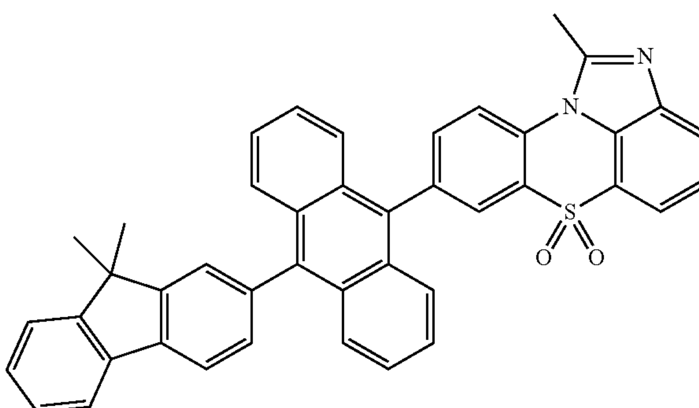
[Chemical Formula 1-2-5]
