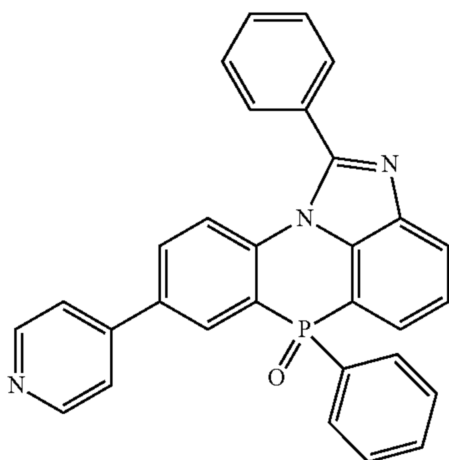
[Chemical Formula 2-4-39]
