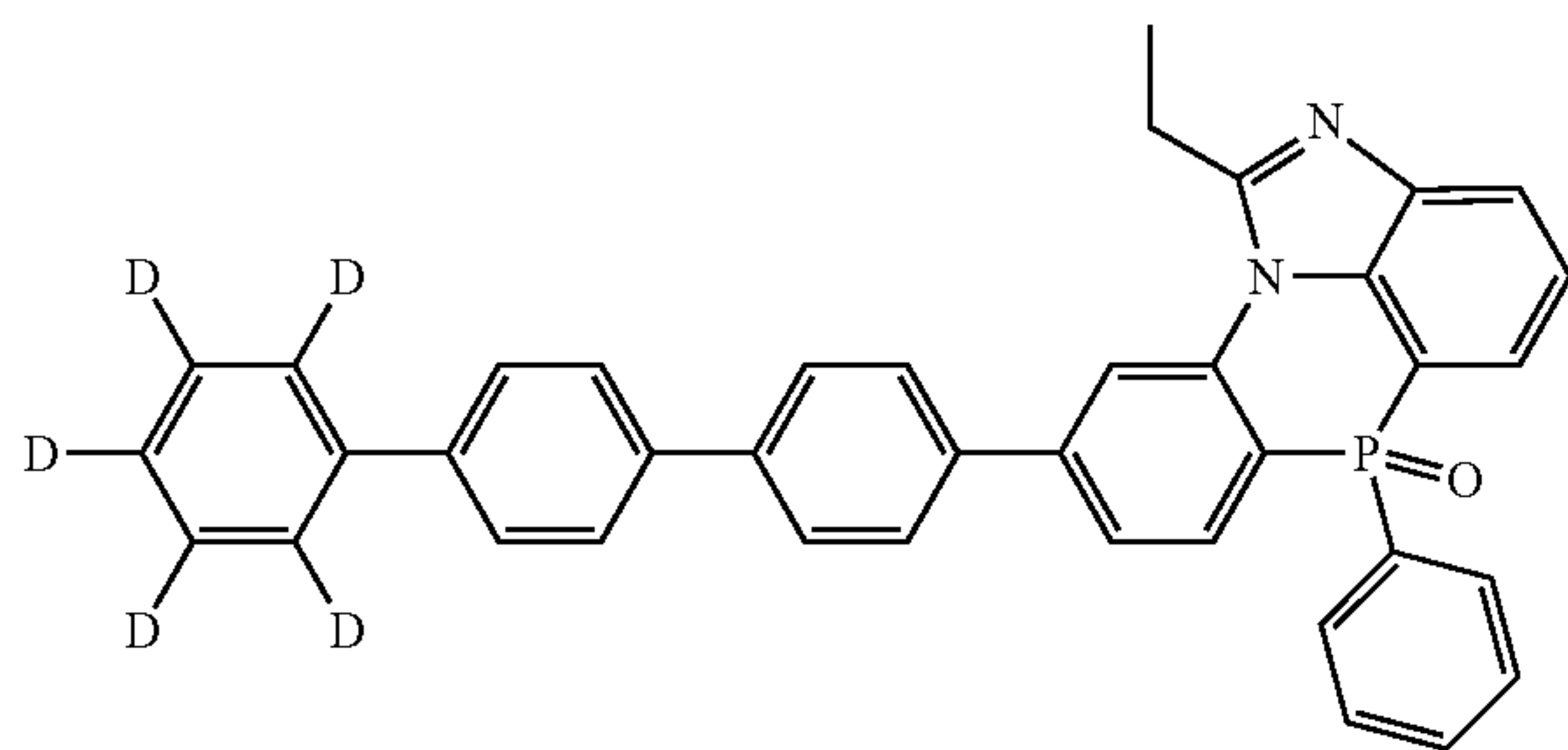
[Chemical Formula 2-7-53]
