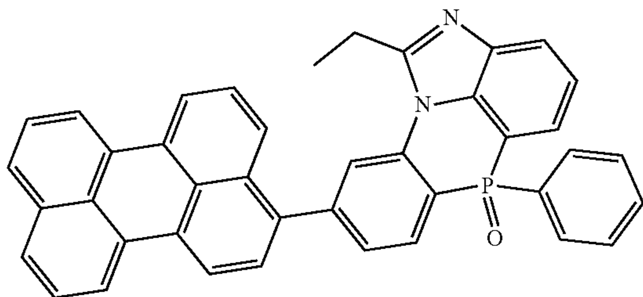
[Chemical Formula 2-7-29]
