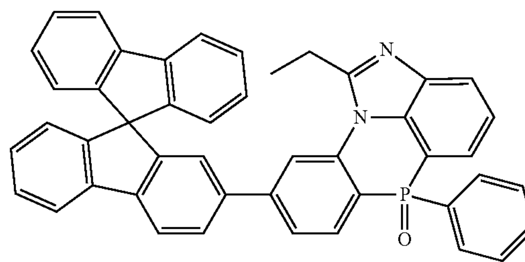
[Chemical Formula 2-7-34]
