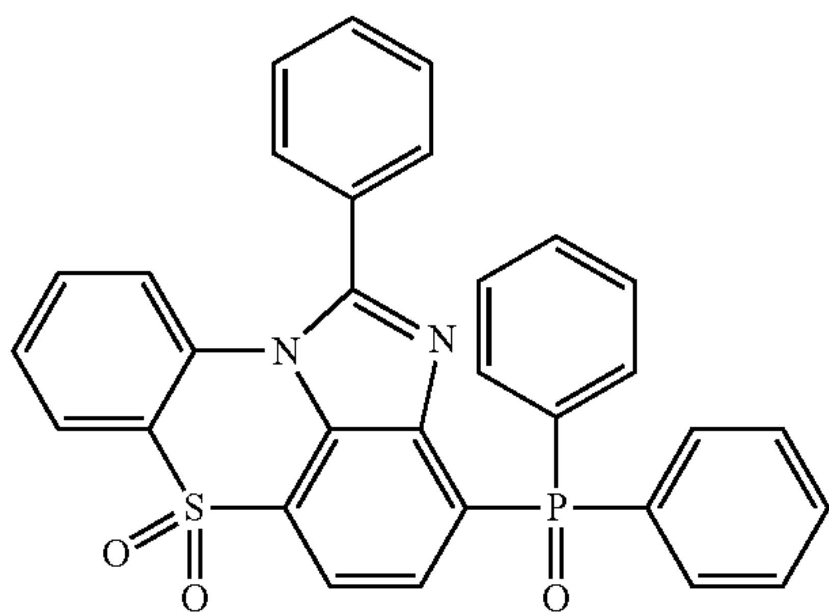
[Chemical Formula 1-12-7]
