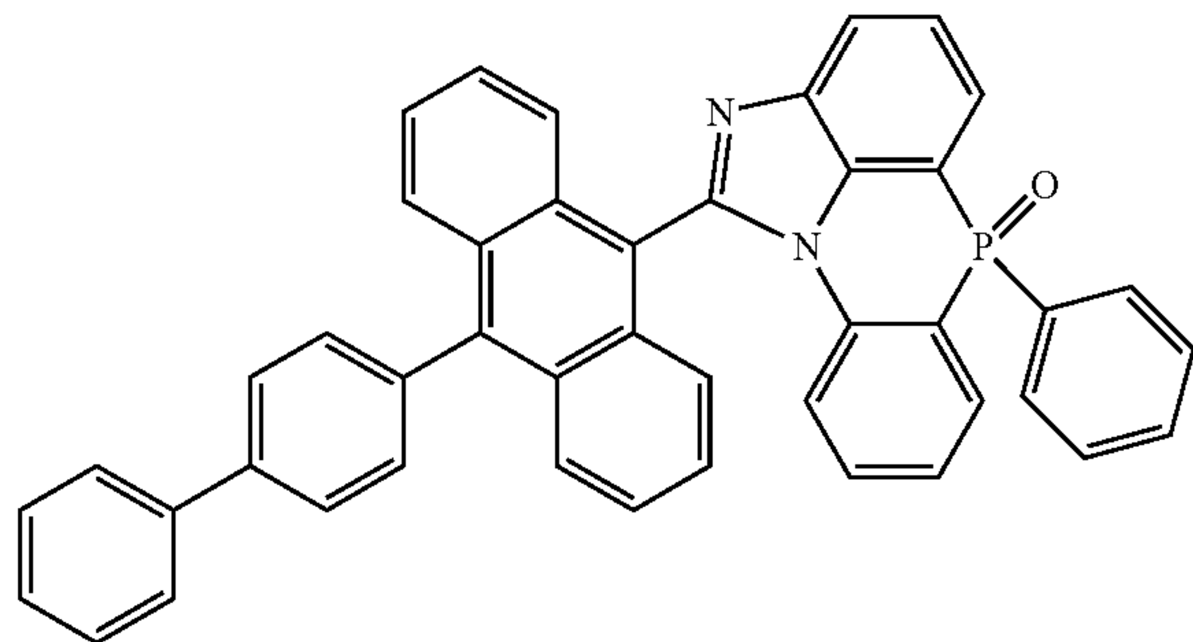
[Chemical Formula 2-5-4]
