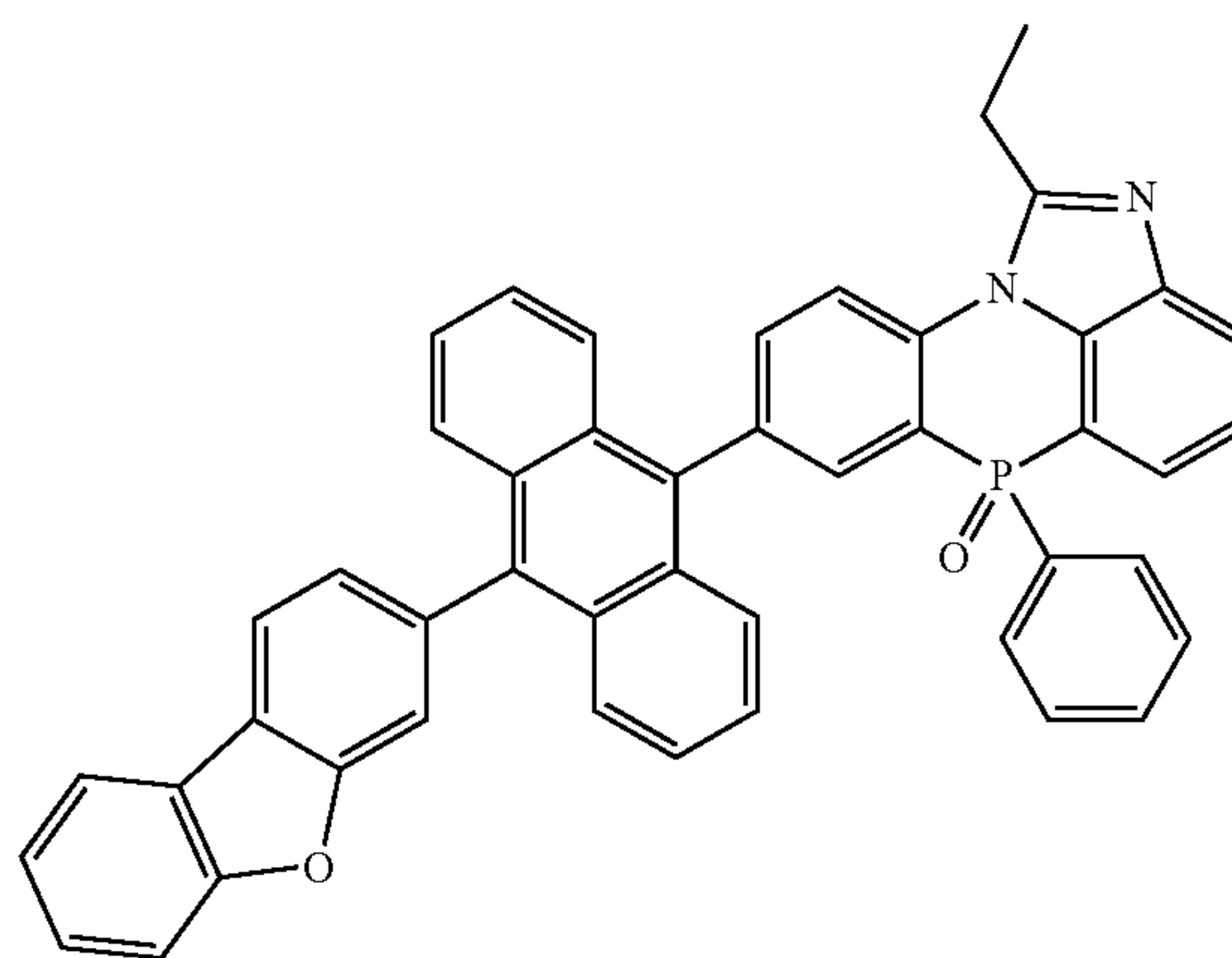
[Chemical Formula 2-3-13]
