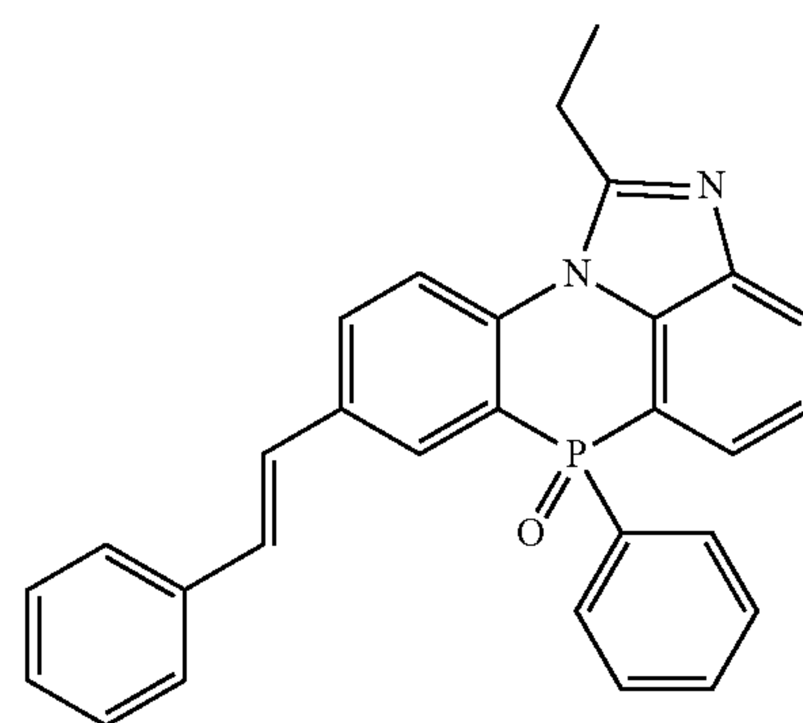
[Chemical Formula 2-3-54]
