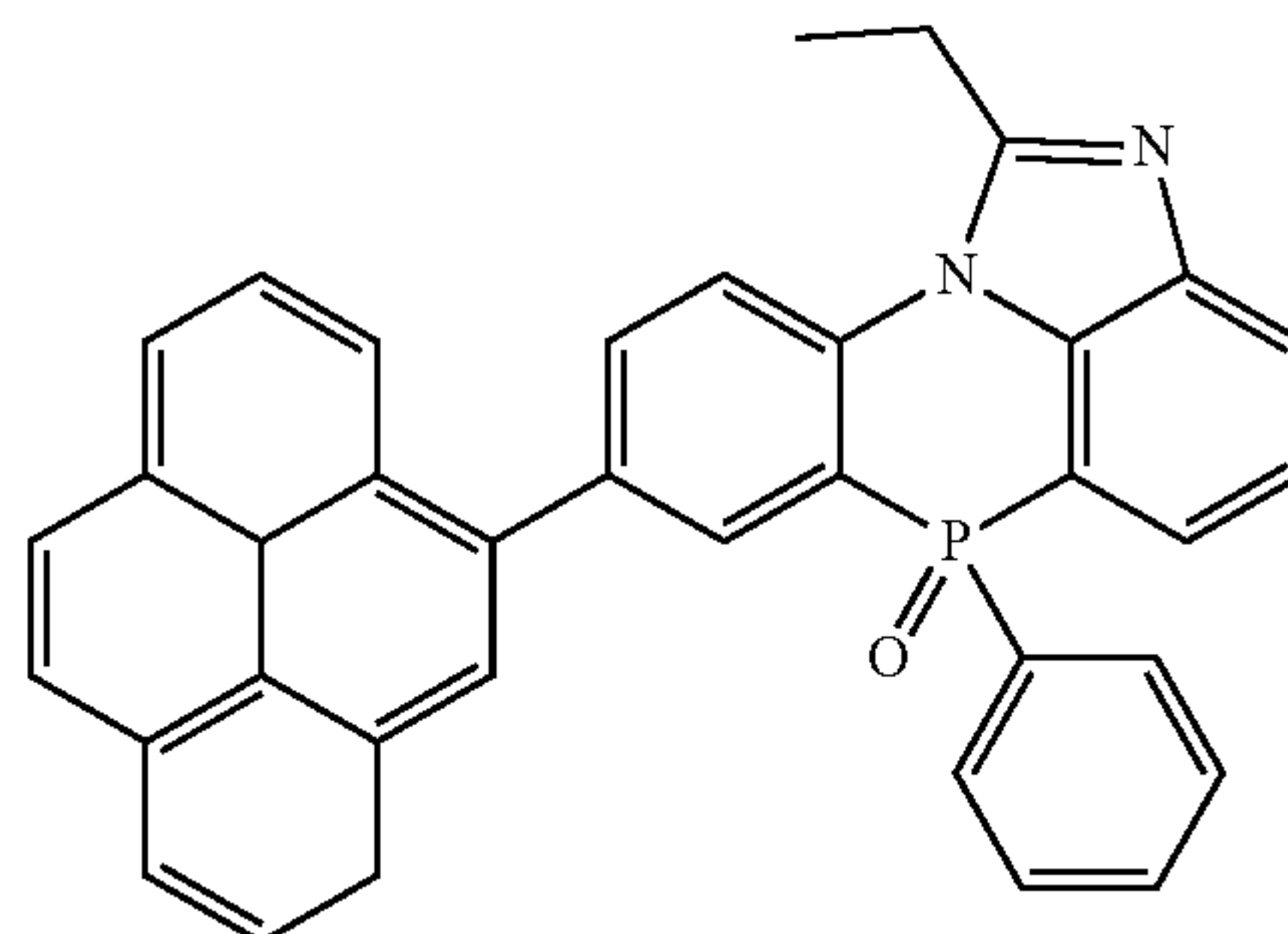
[Chemical Formula 2-3-28]
