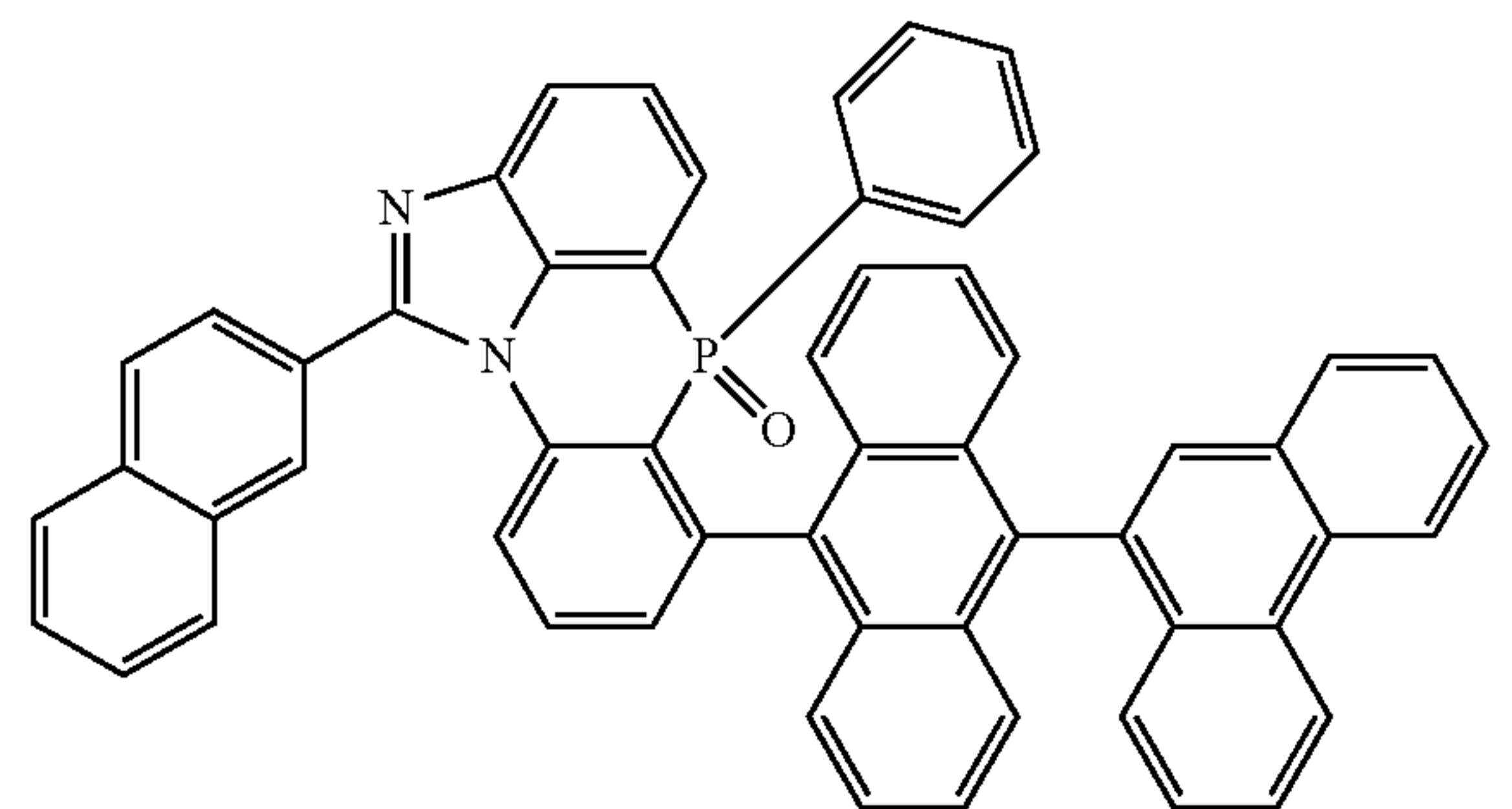
[Chemical Formula 2-6-8]
