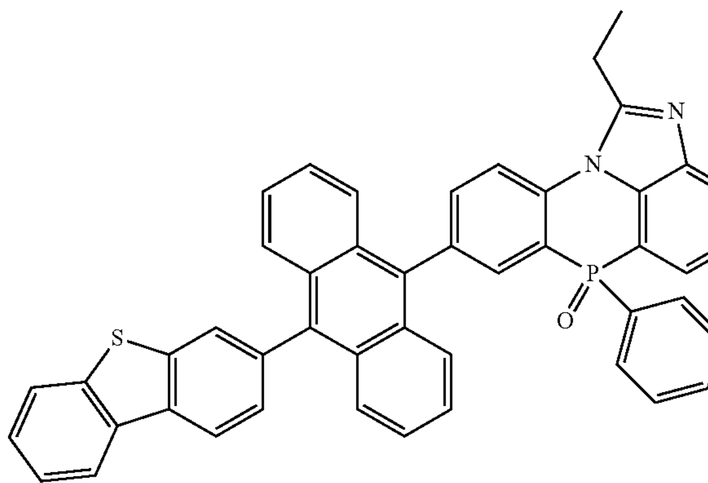
[Chemical Formula 2-3-15]
