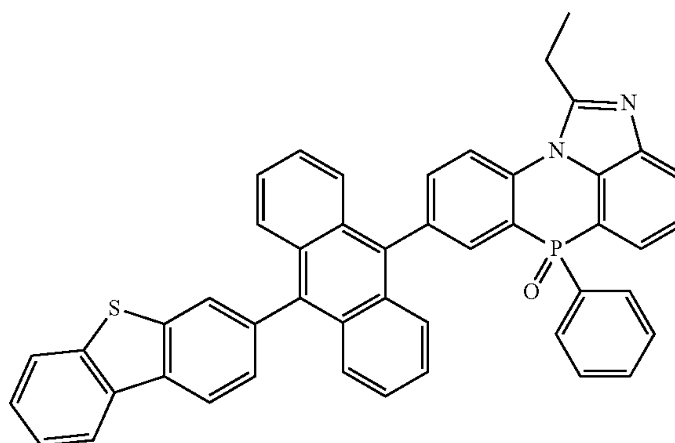
[Chemical Formula 2-3-14]
