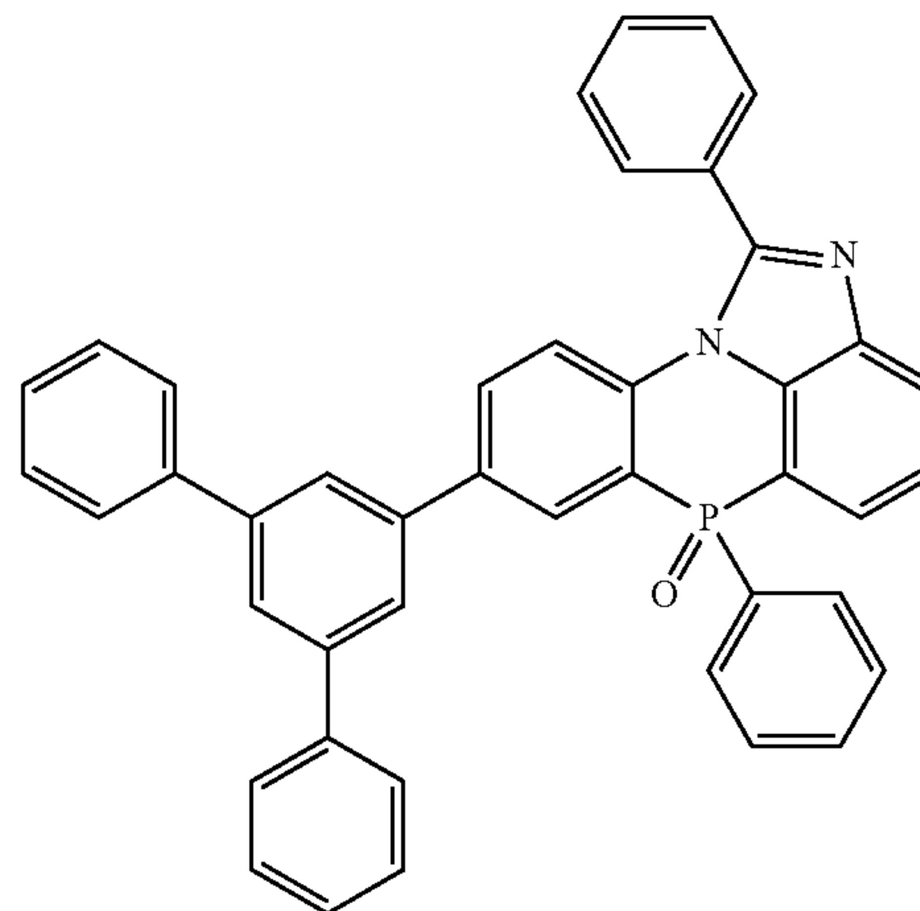
[Chemical Formula 2-4-40]
