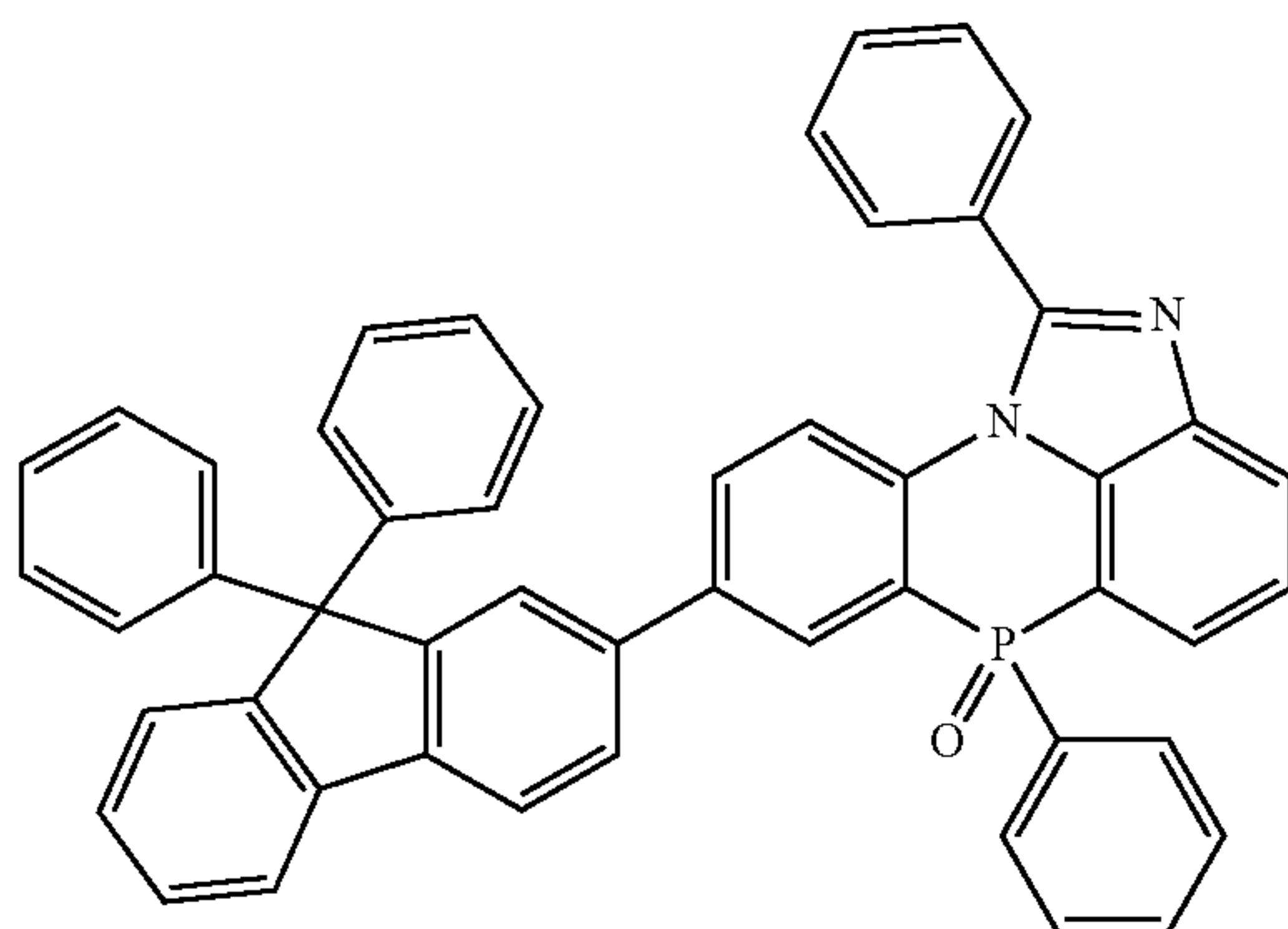
[Chemical Formula 2-4-35]
