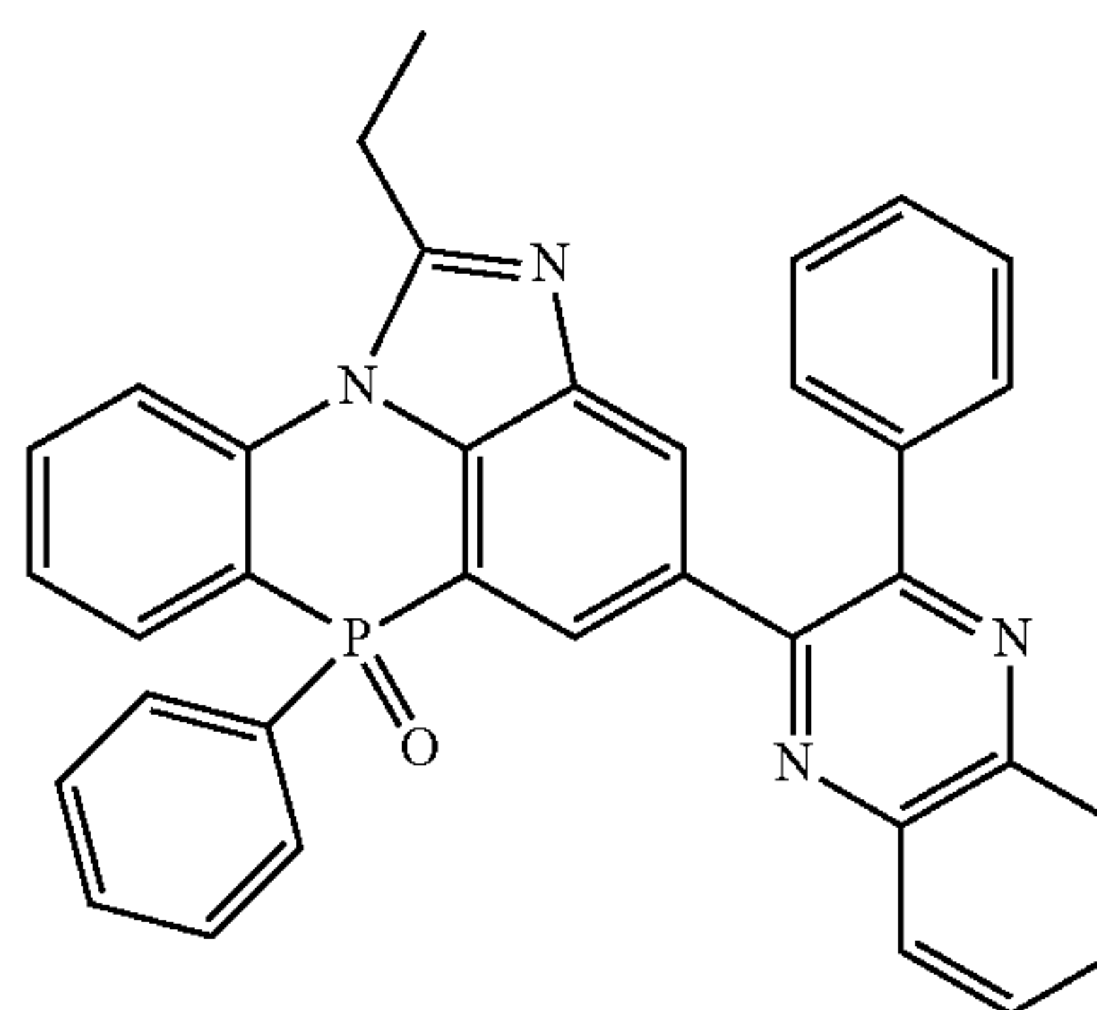
[Chemical Formula 2-10-13]
