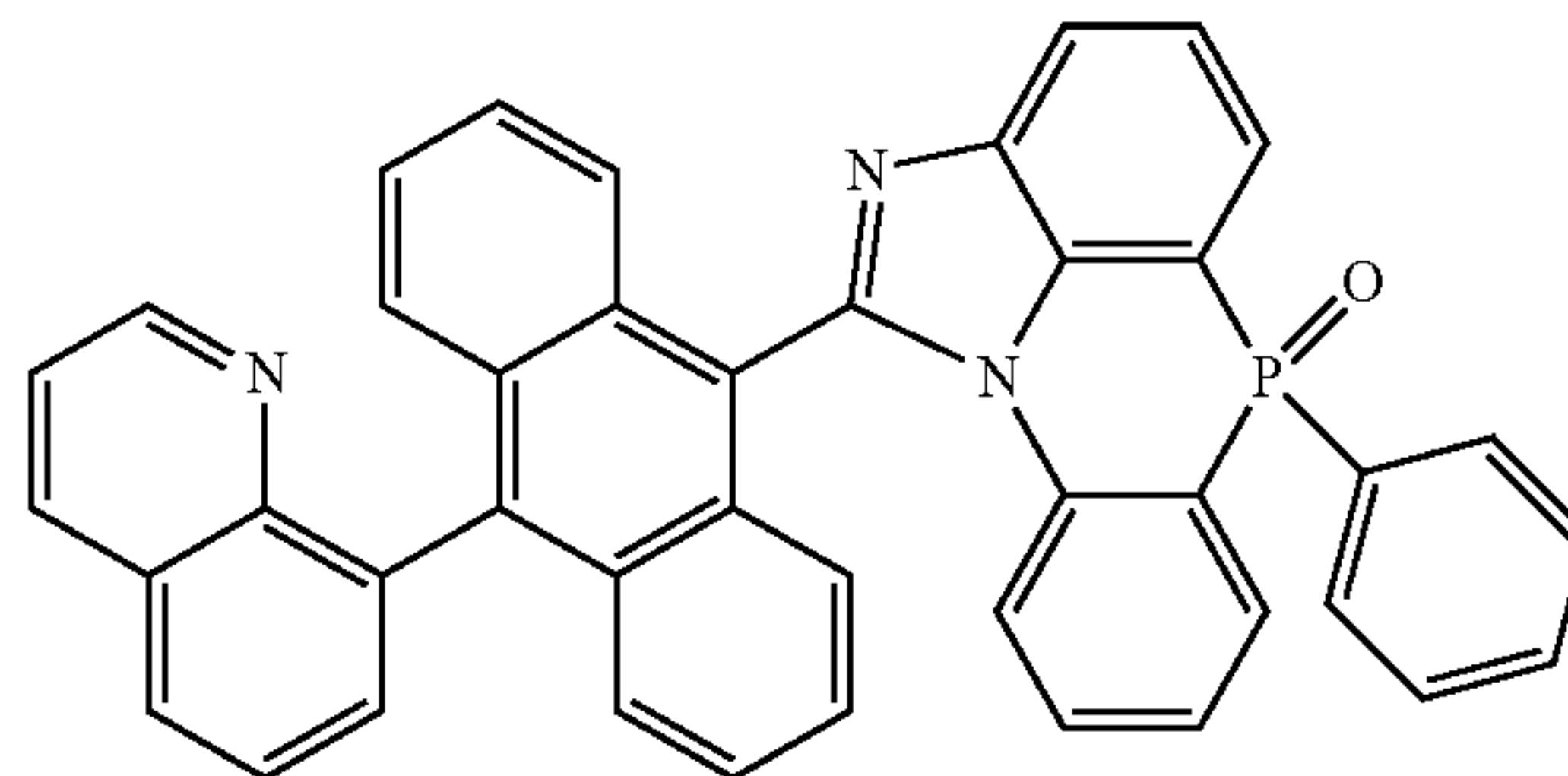
[Chemical Formula 2-5-12]
