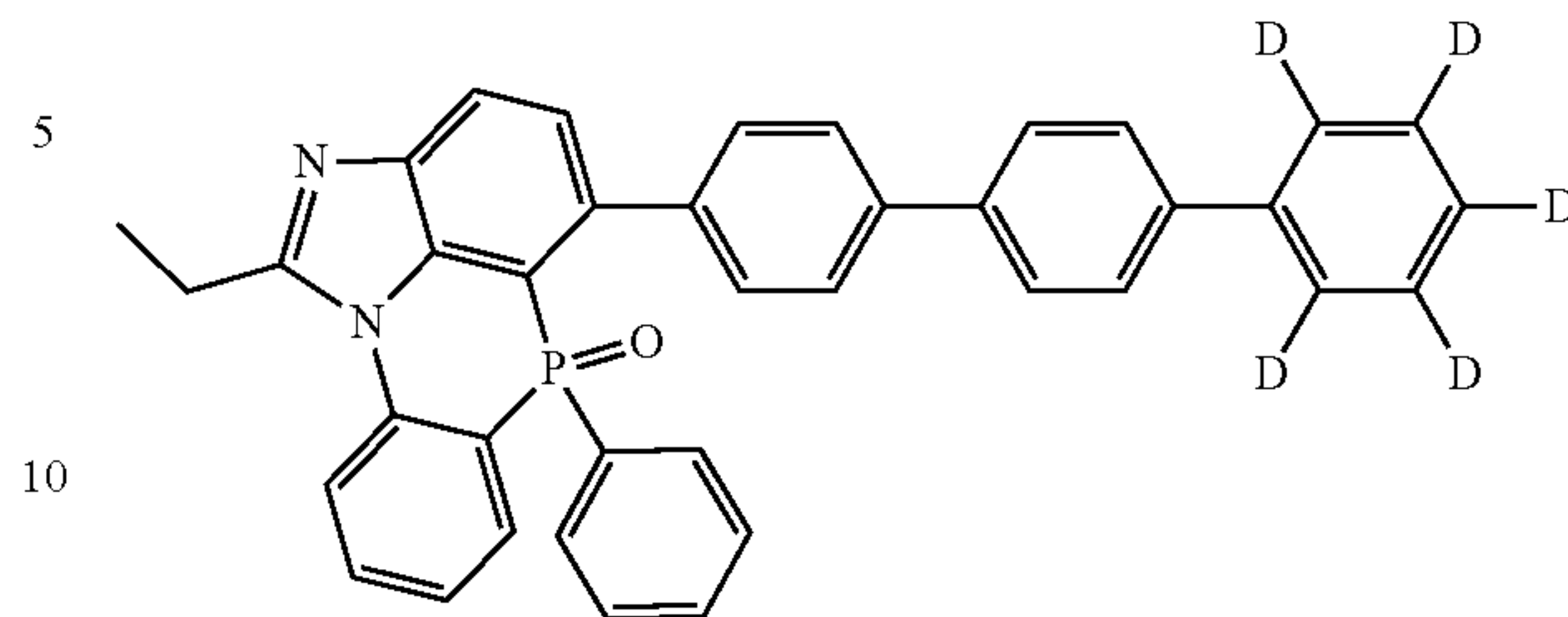
[Chemical Formula 2-9-16]
