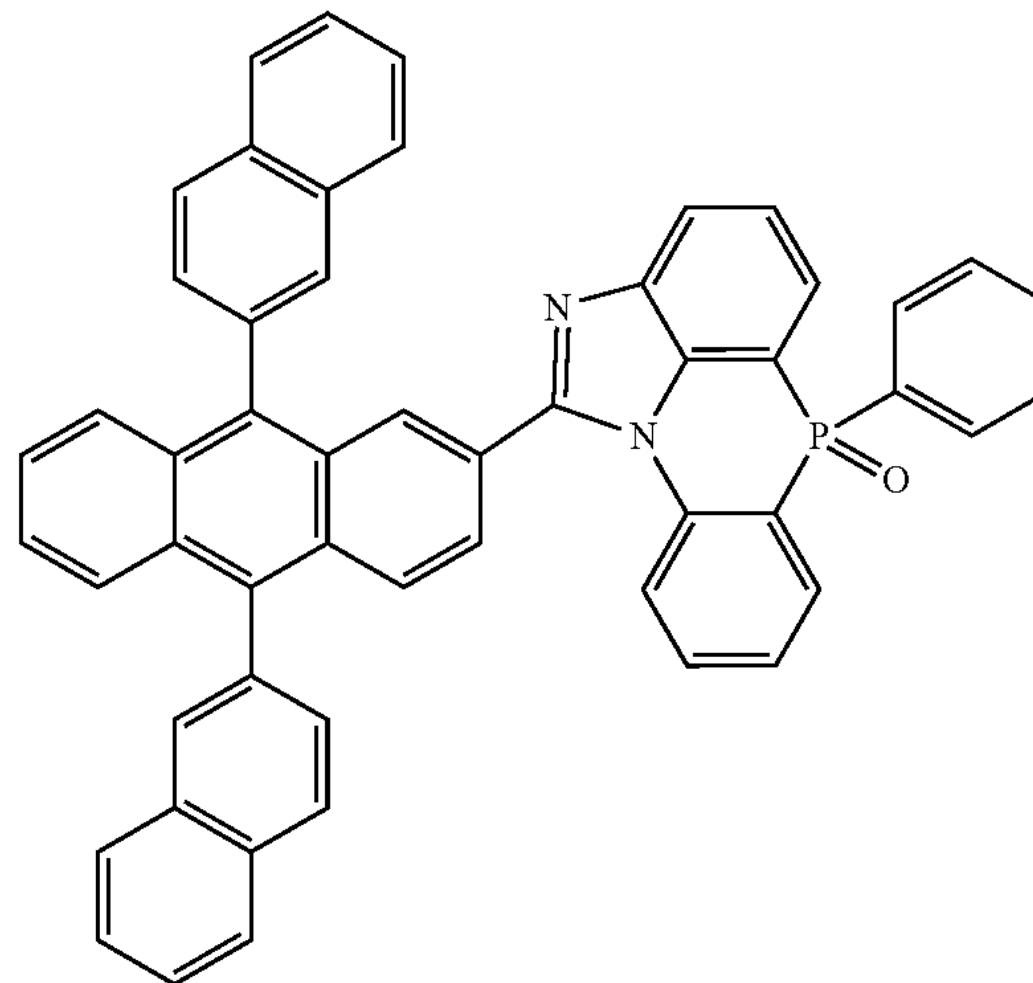
[Chemical Formula 2-5-20]
