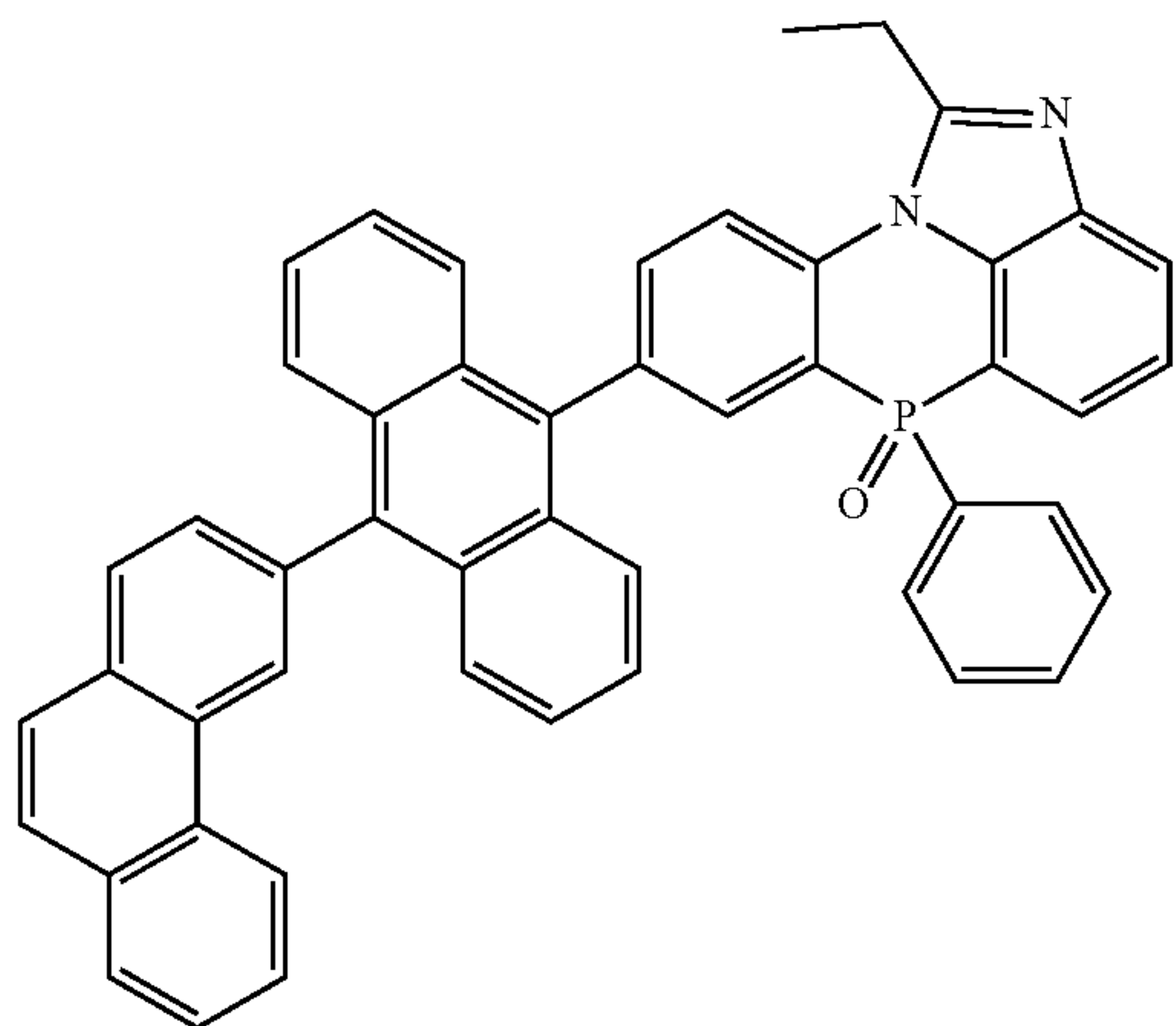
[Chemical Formula 2-3-8]
