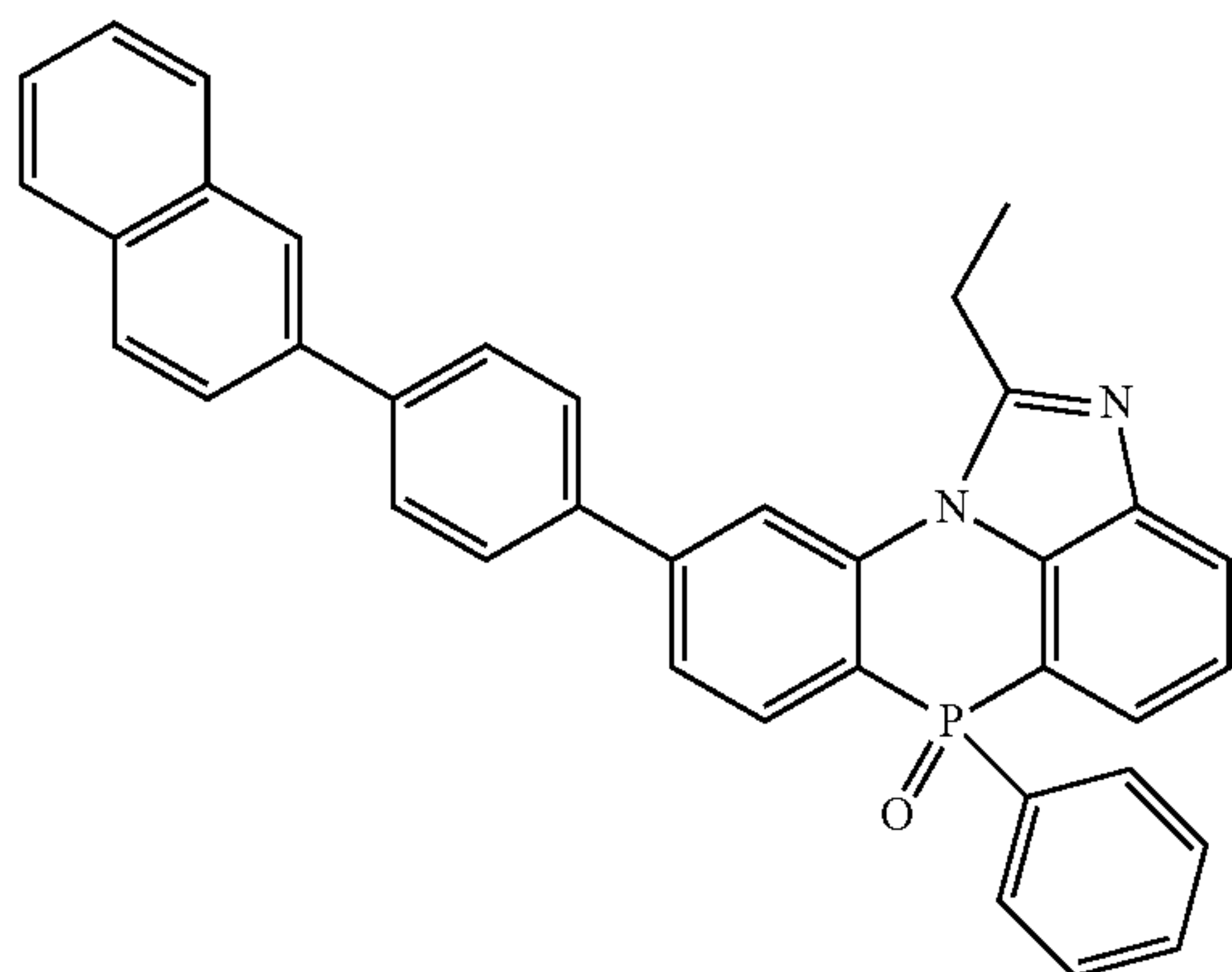
[Chemical Formula 2-7-26]
