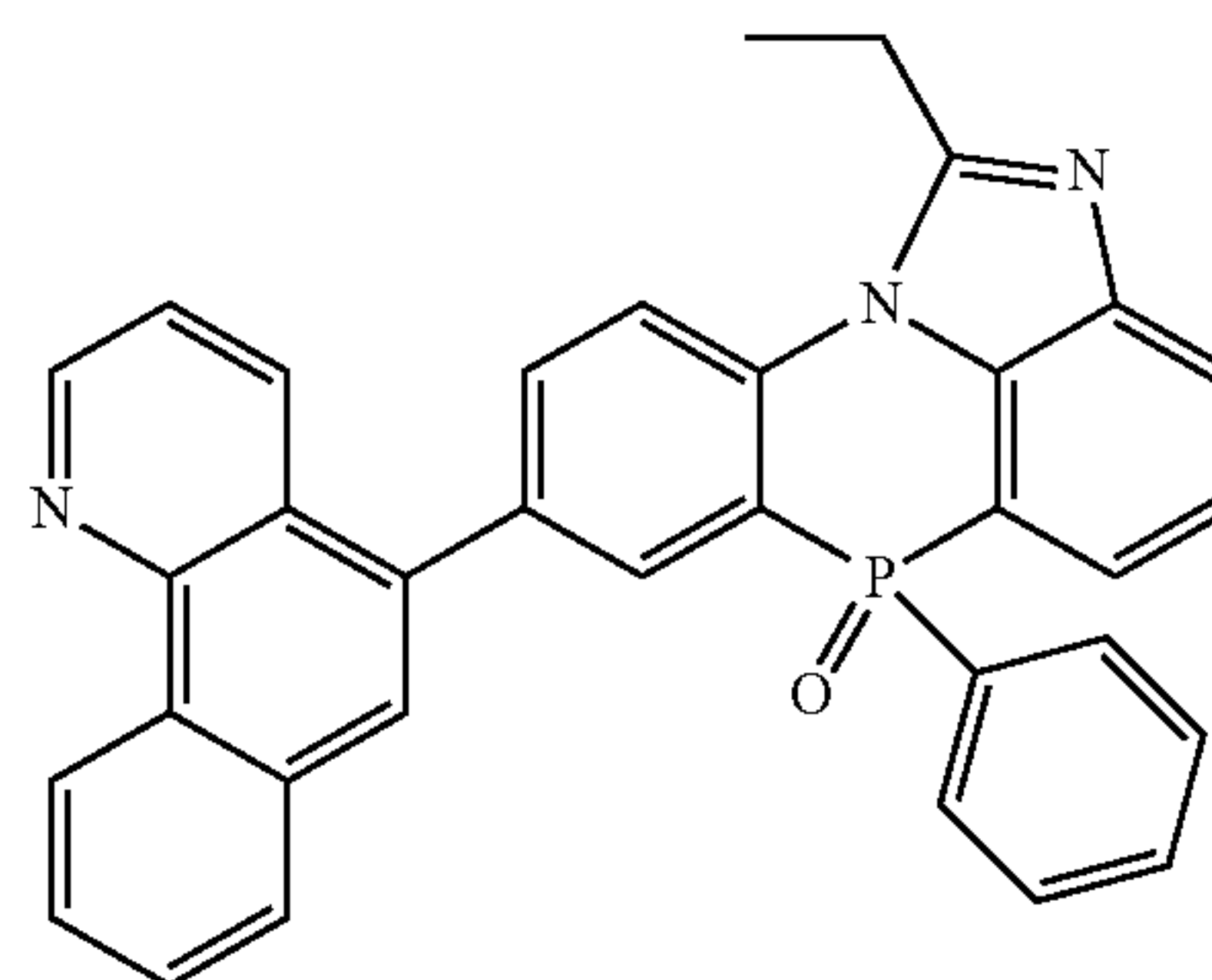
[Chemical Formula 2-3-33]
