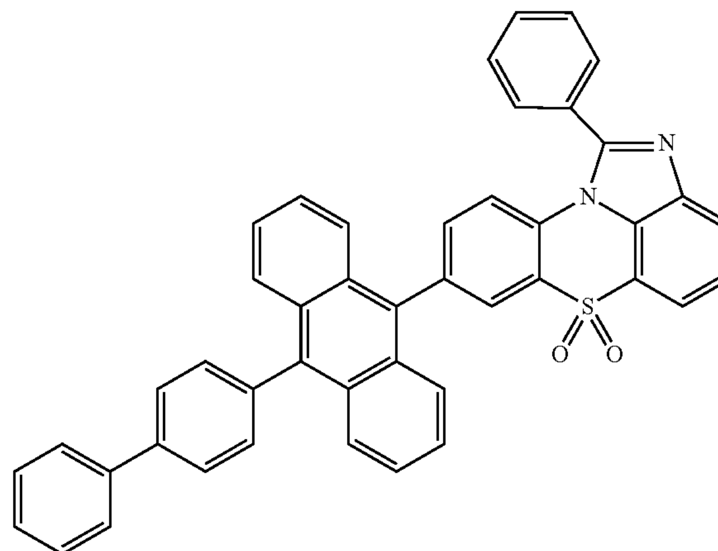
[Chemical Formula 1-4-4]
