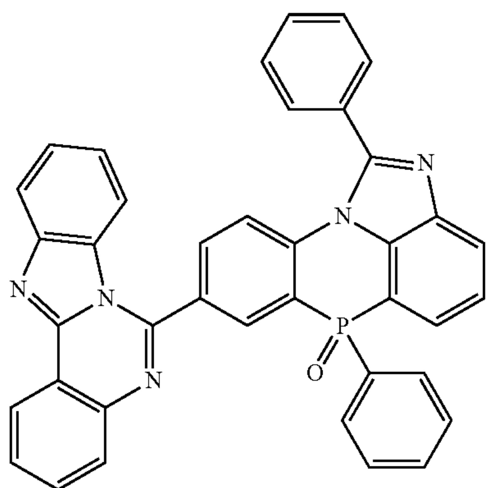
[Chemical Formula 2-4-53]
