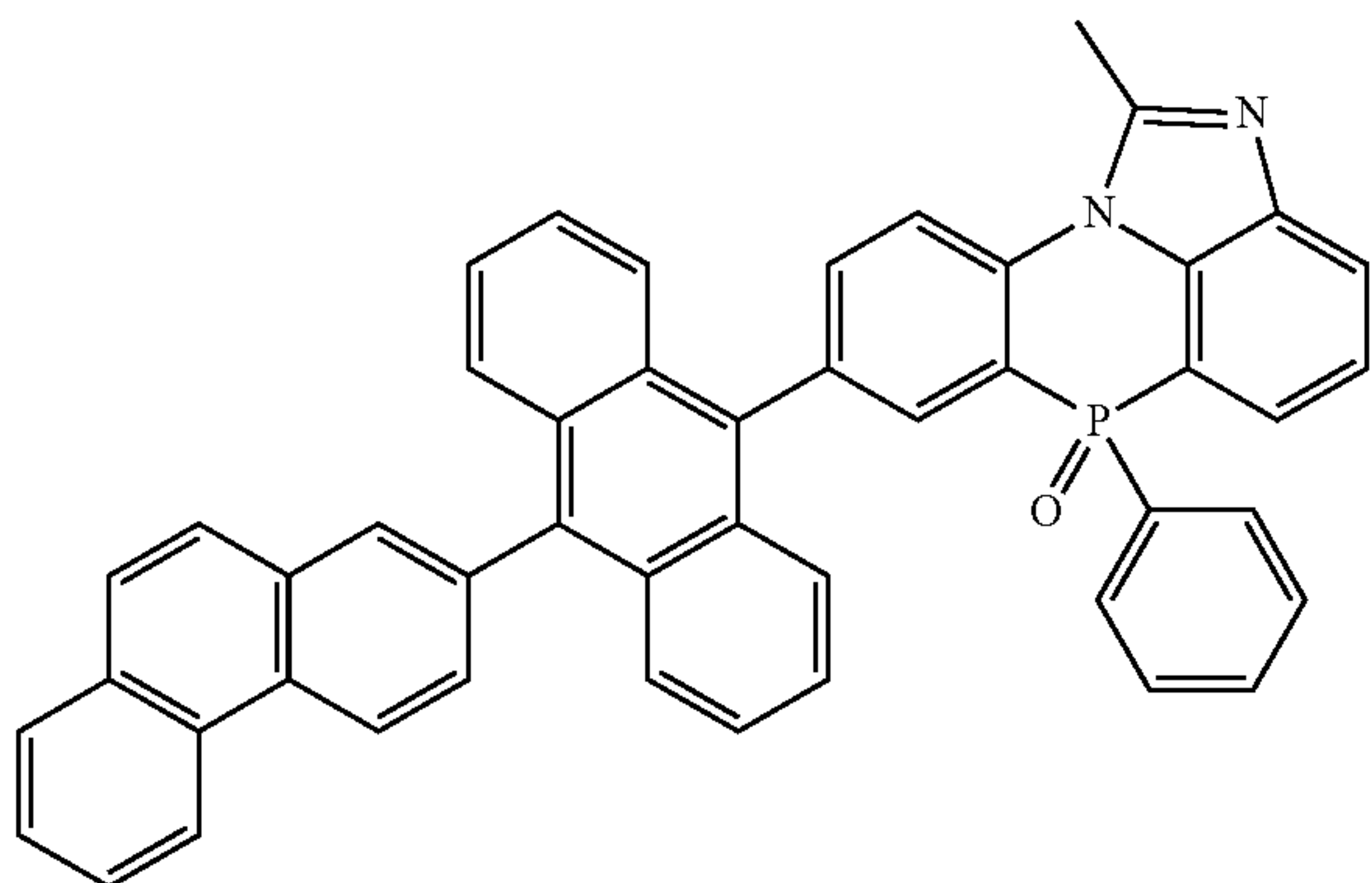
[Chemical Formula 2-2-9]
