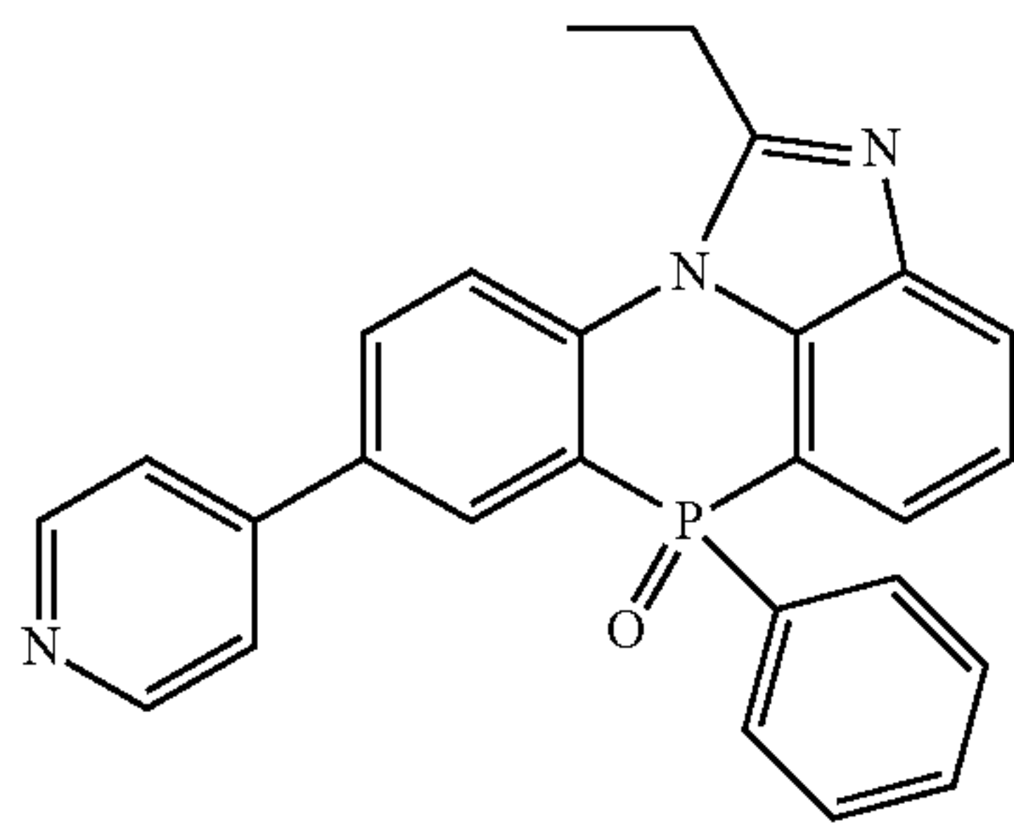
[Chemical Formula 2-3-38]
