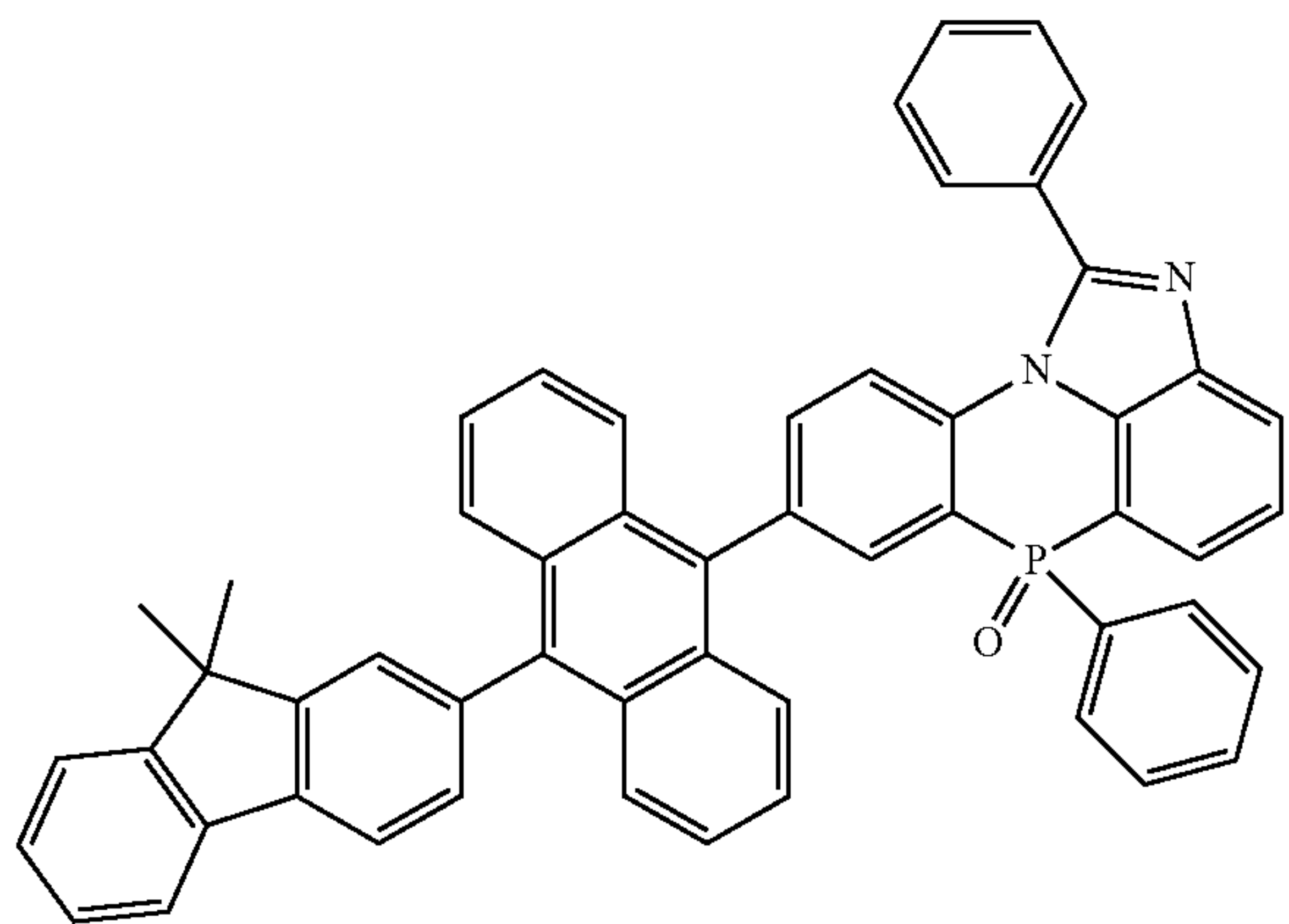
[Chemical Formula 2-4-5]
