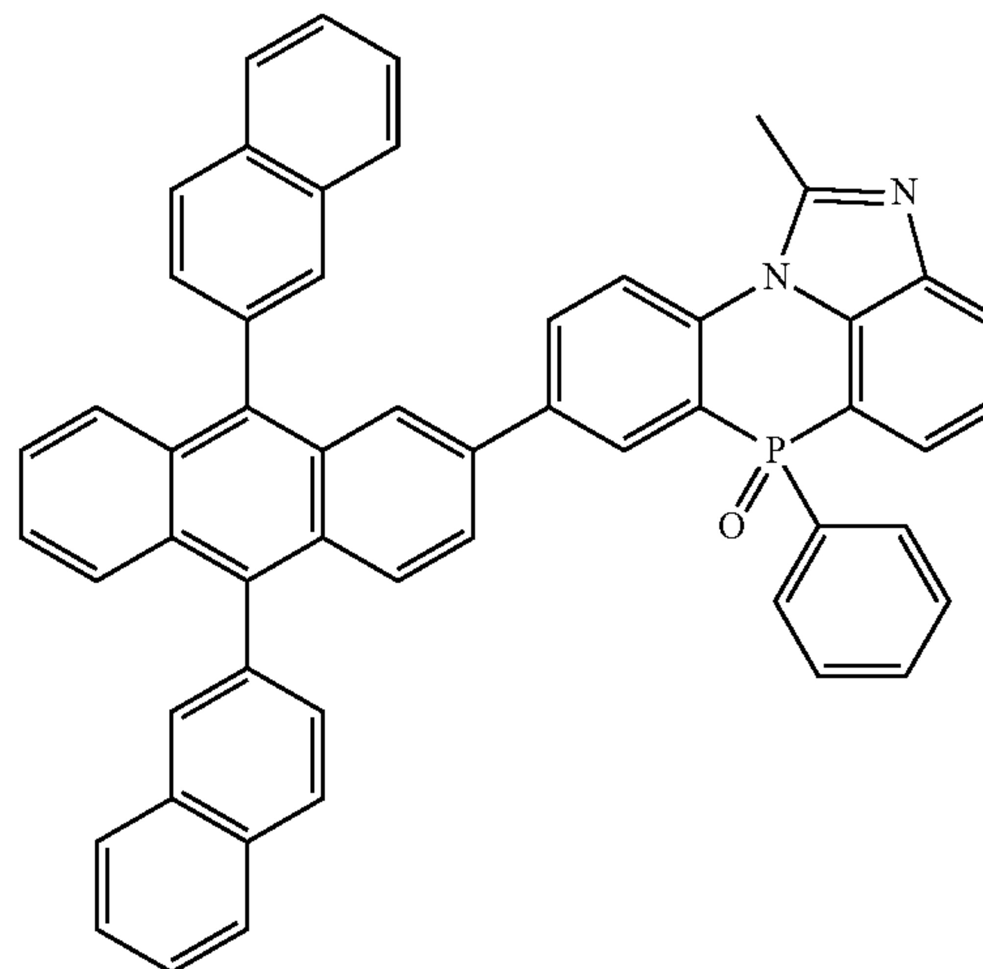
[Chemical Formula 2-2-20]
