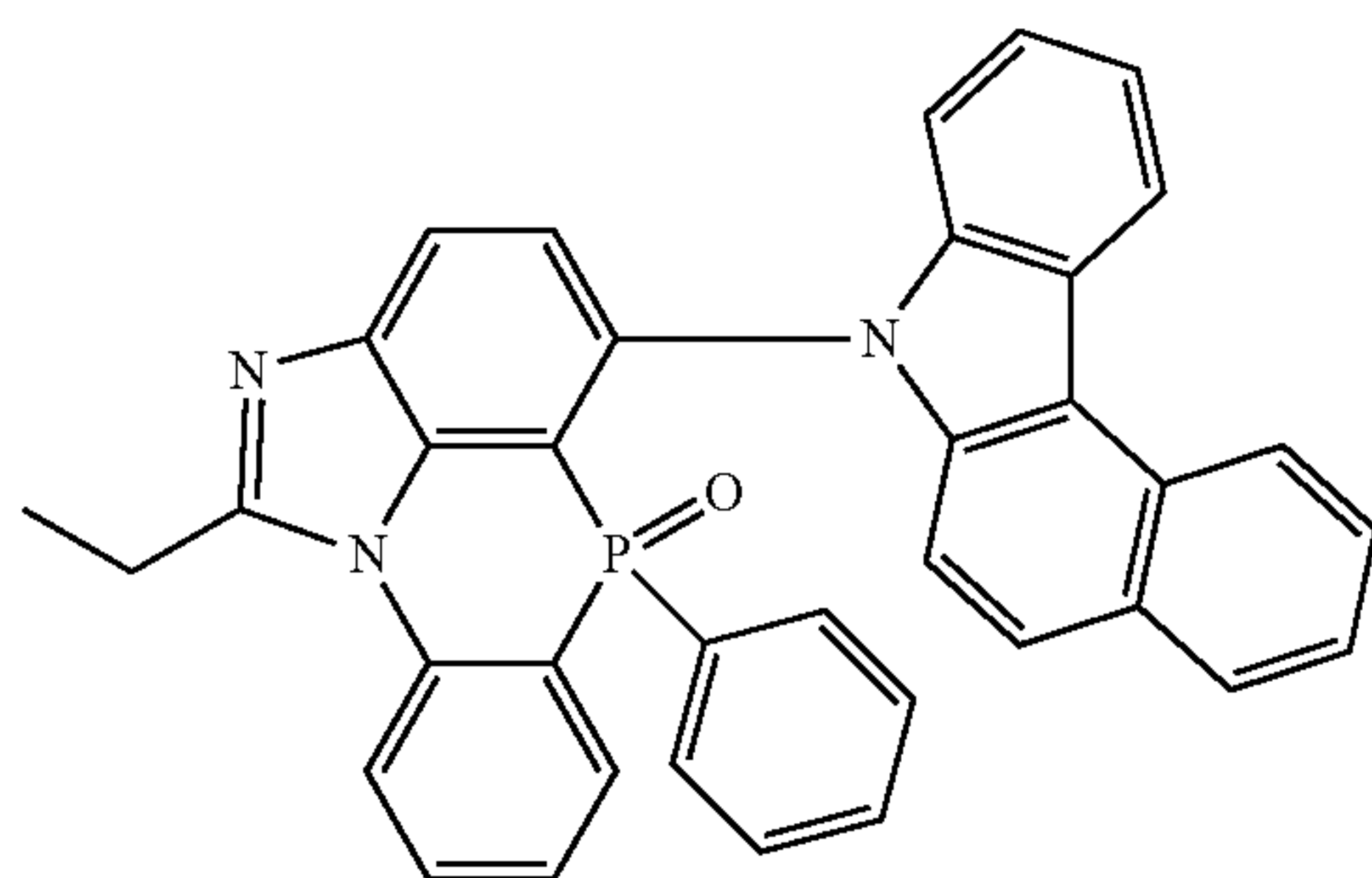
[Chemical Formula 2-9-15]
