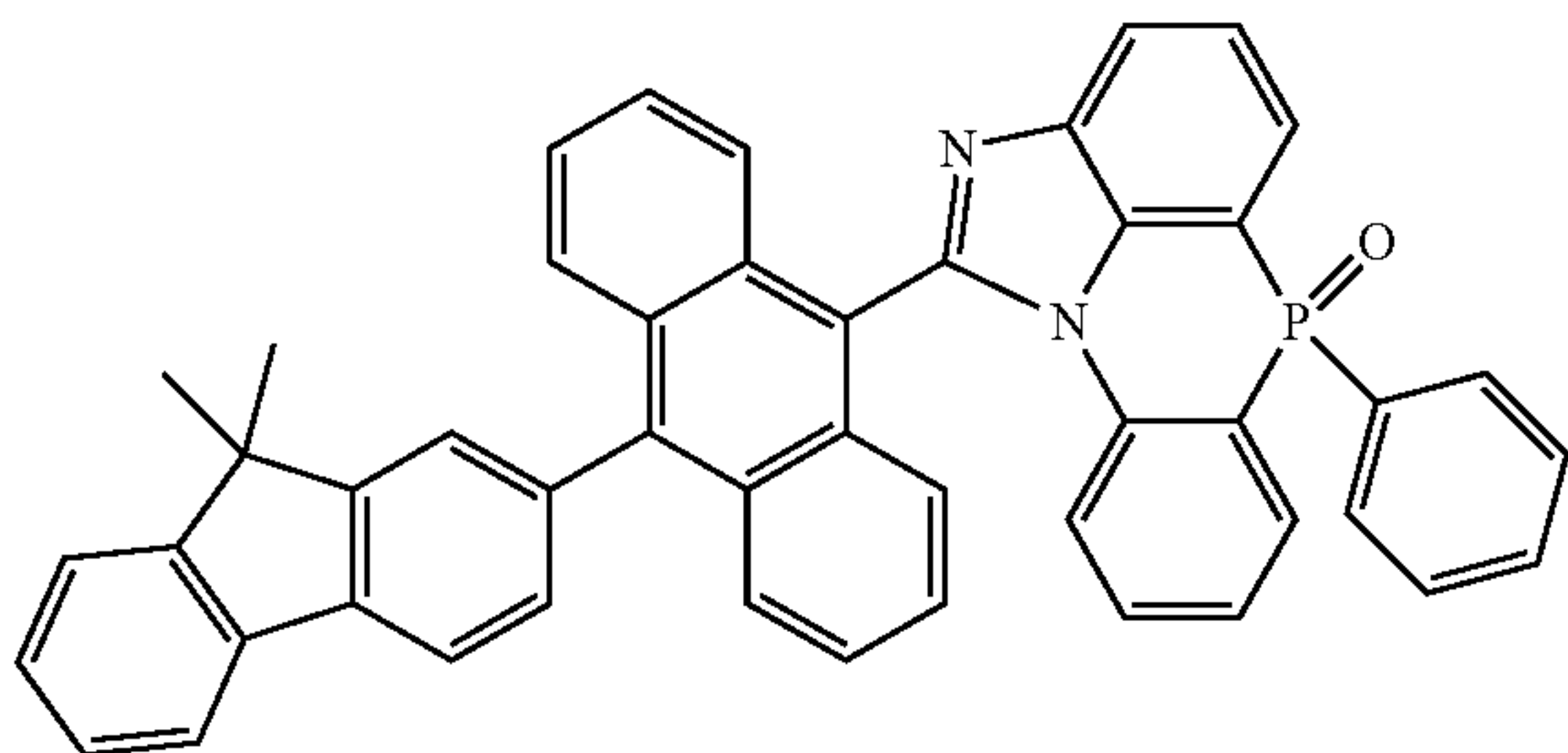
[Chemical Formula 2-5-5]
