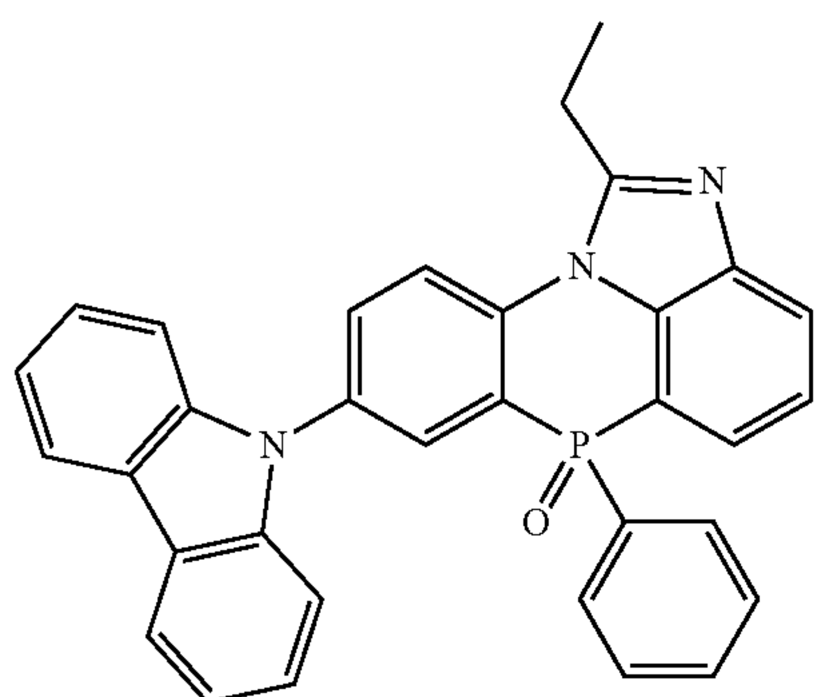
[Chemical Formula 2-3-50]
