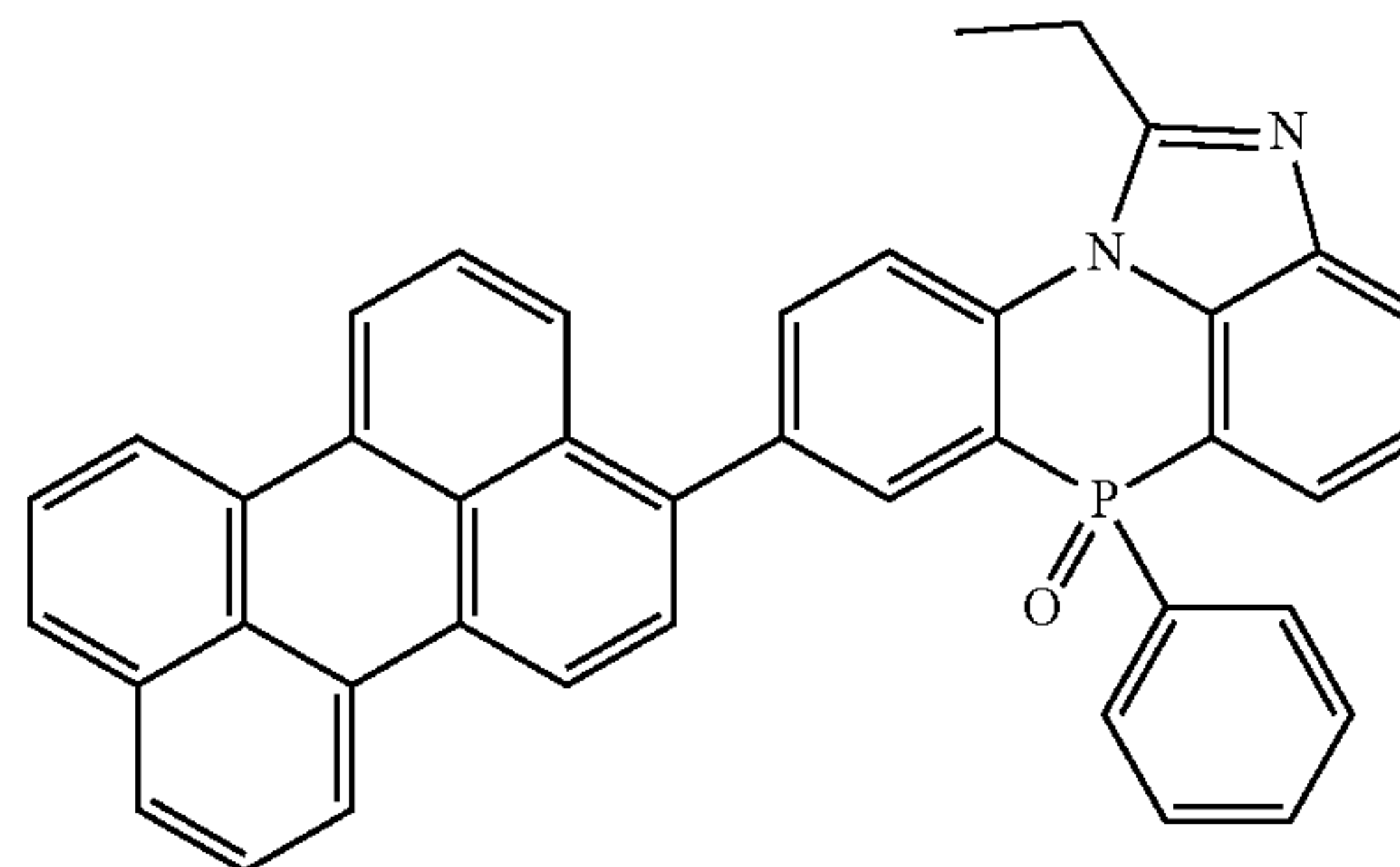
[Chemical Formula 2-3-29]
