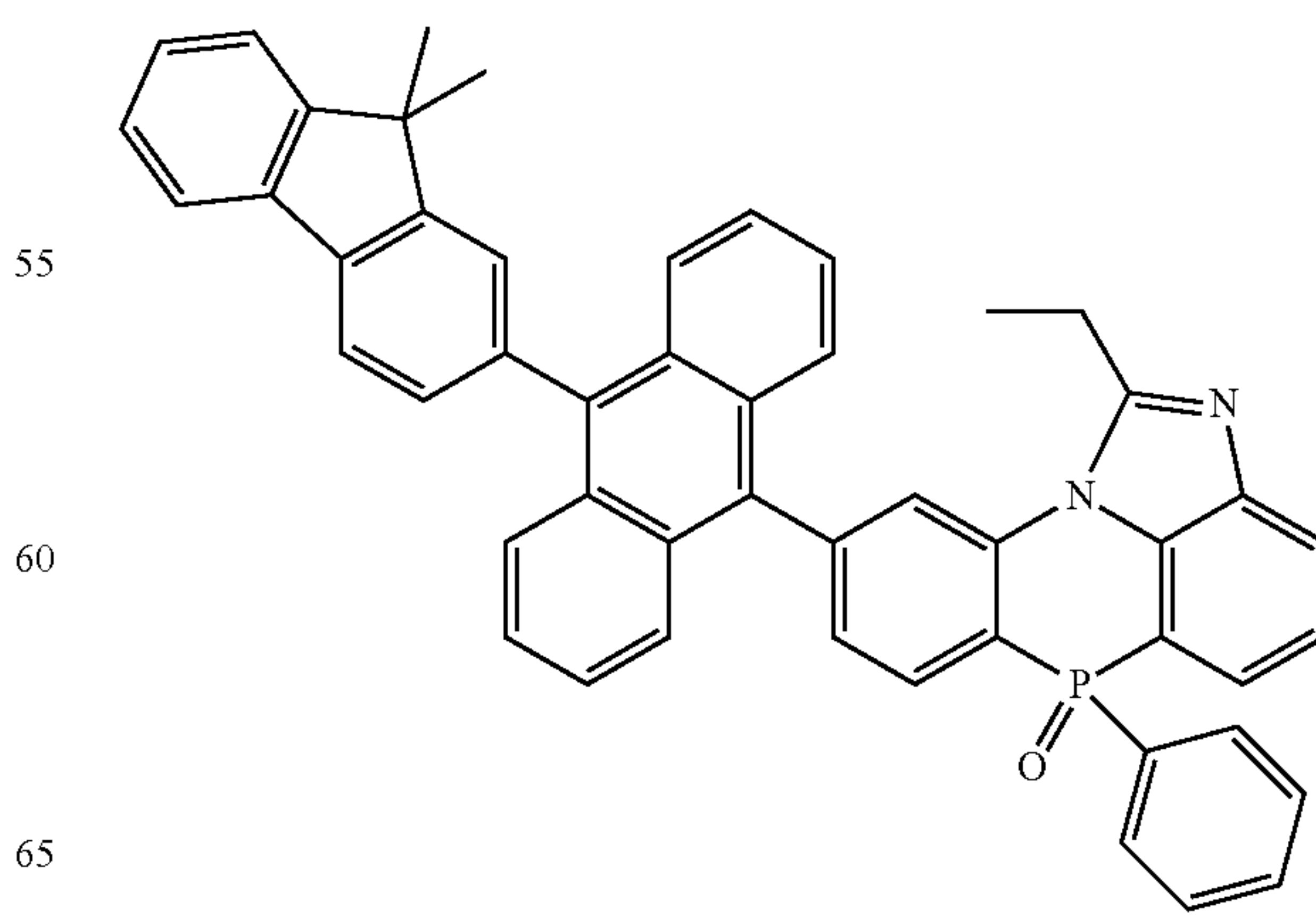
[Chemical Formula 2-7-5]
