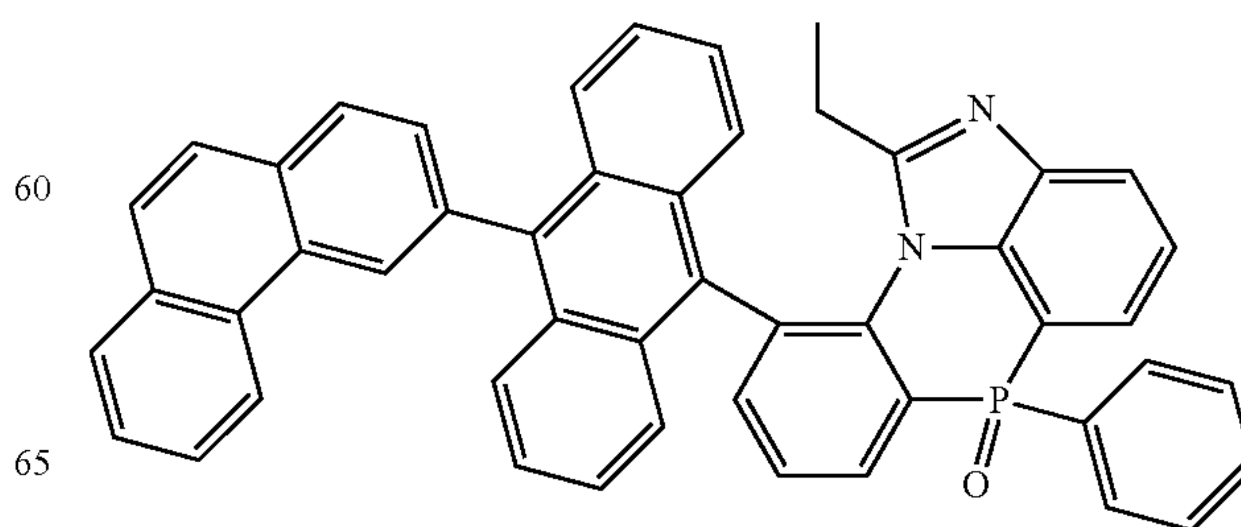
[Chemical Formula 2-8-8]
