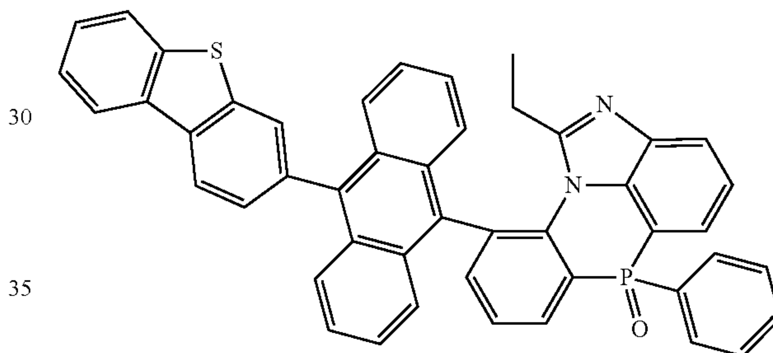
[Chemical Formula 2-8-14]
