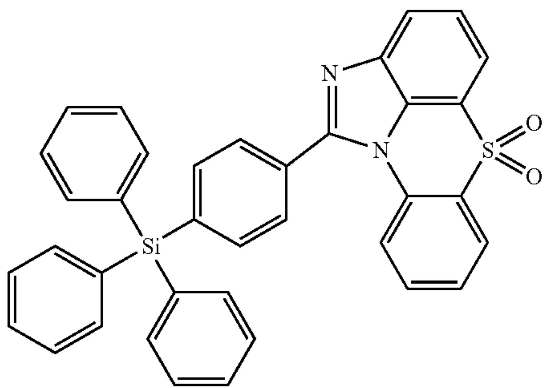
[Chemical Formula 1-1-8]
