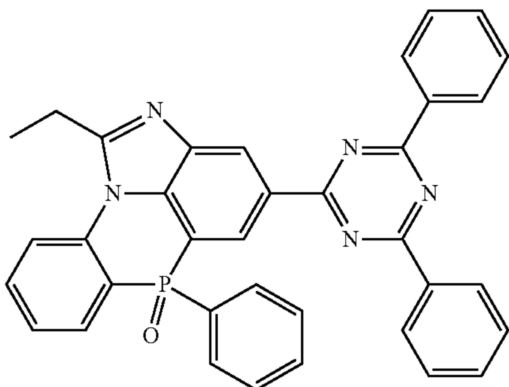
[Chemical Formula 2-10-5]
