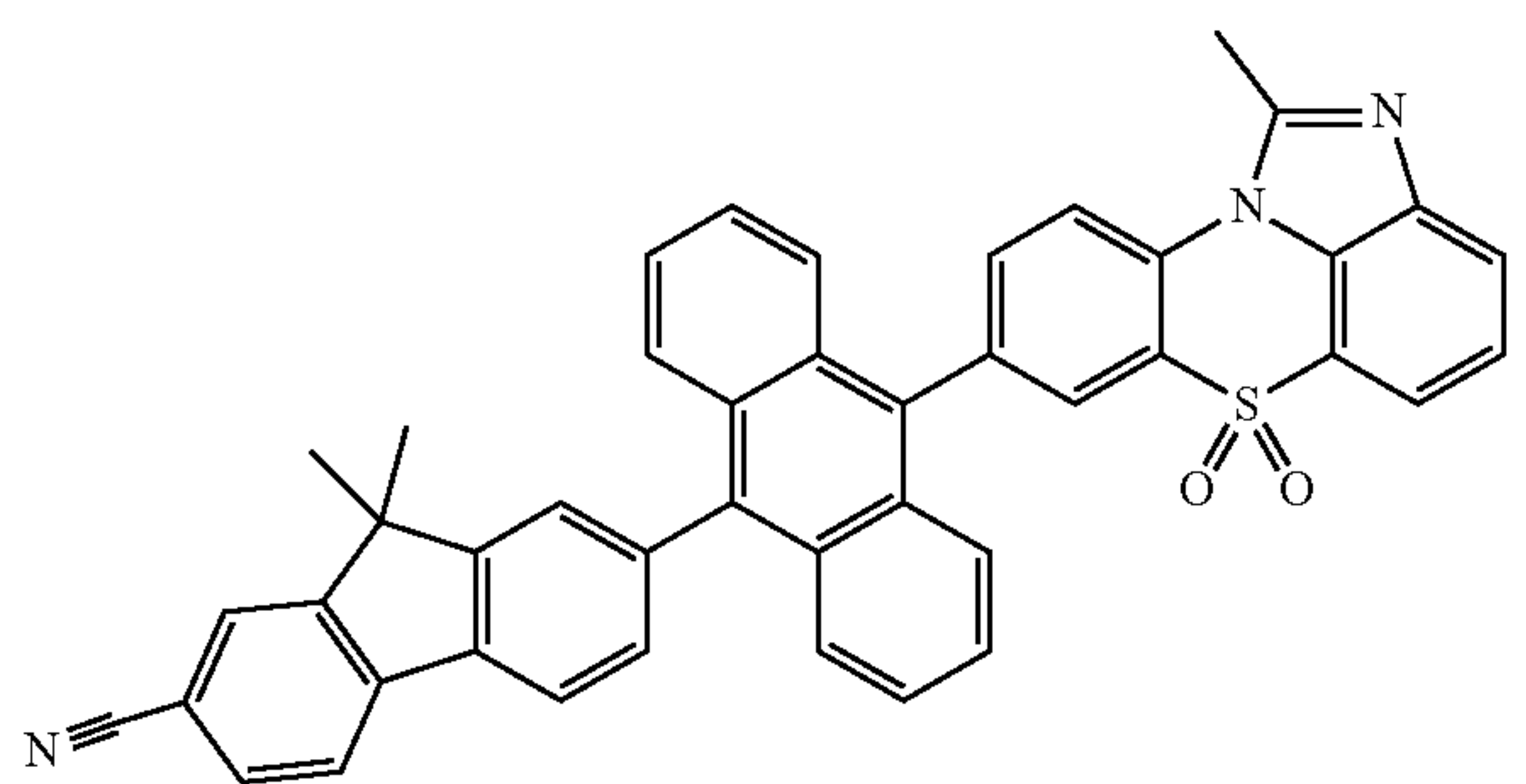
[Chemical Formula 1-2-15]
