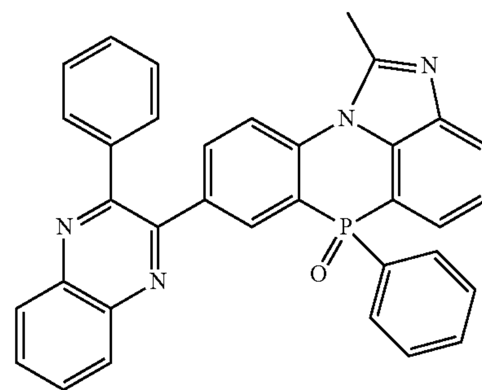
[Chemical Formula 2-2-49]
