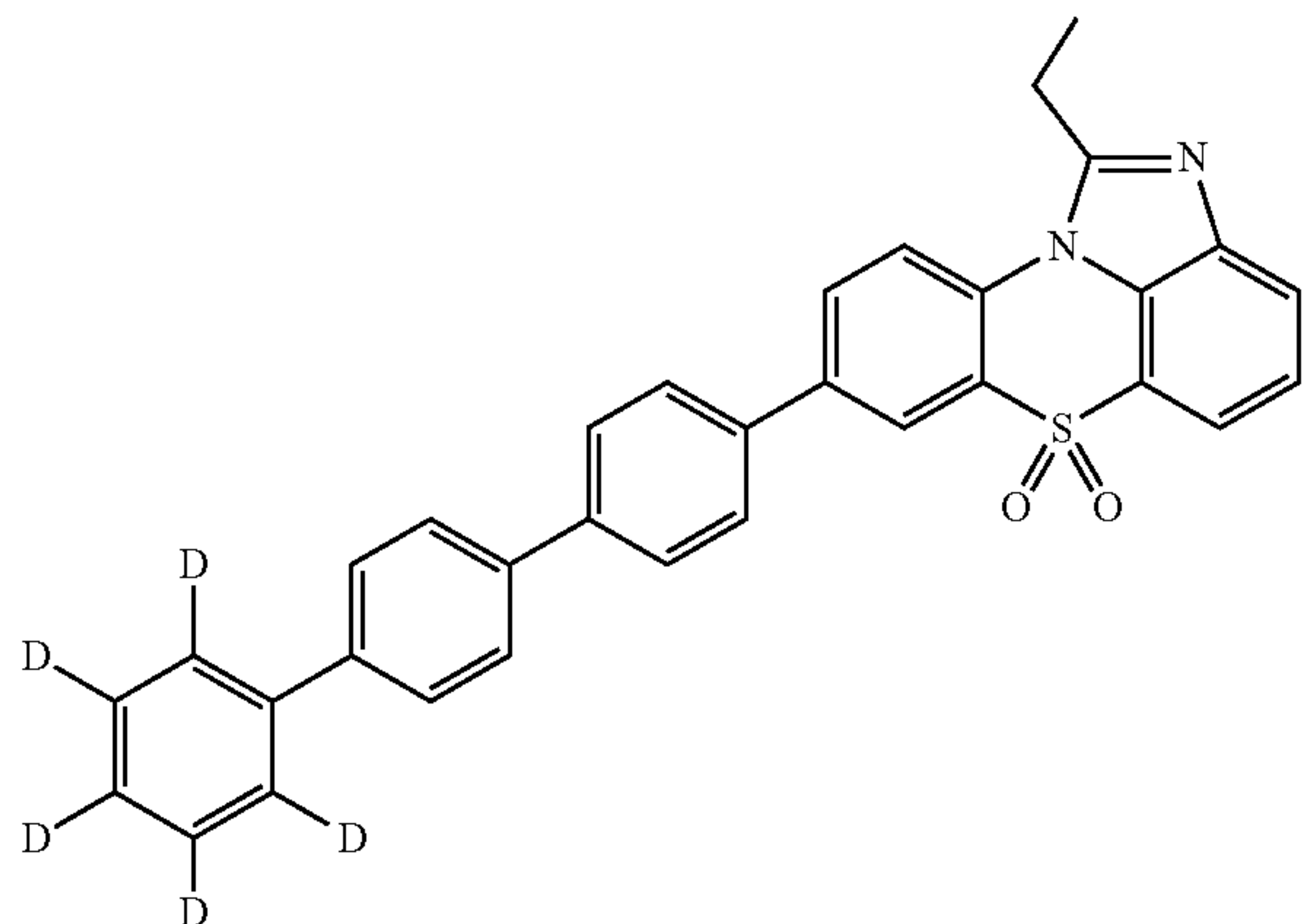
[Chemical Formula 1-3-52]
