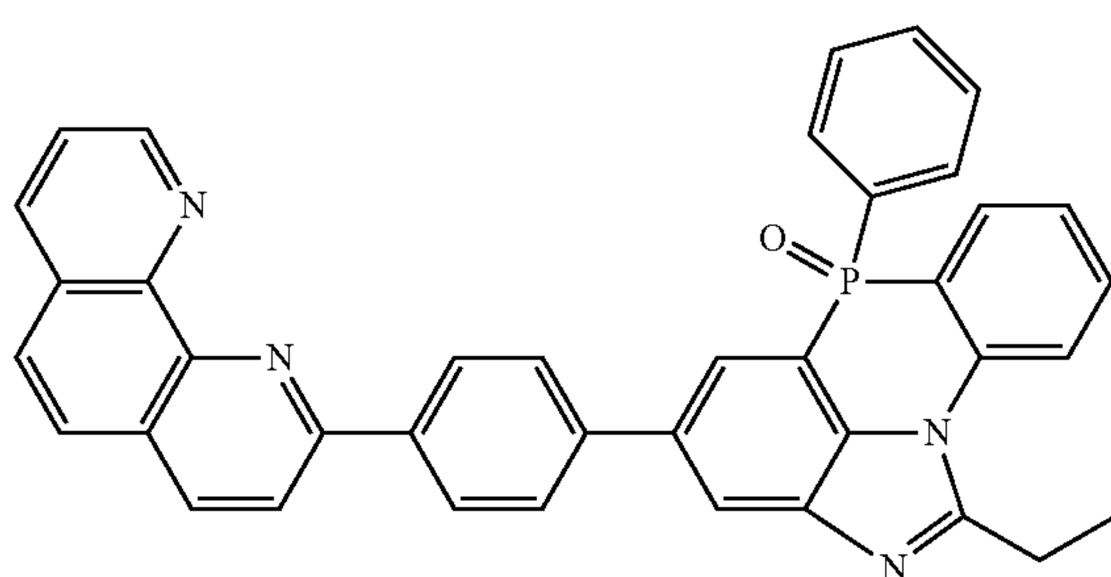
[Chemical Formula 2-10-12]
