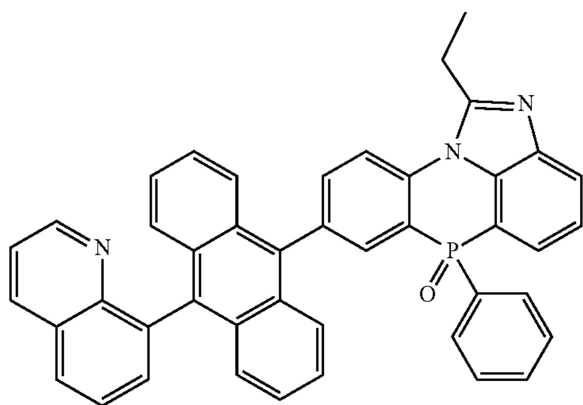
[Chemical Formula 2-3-11]
