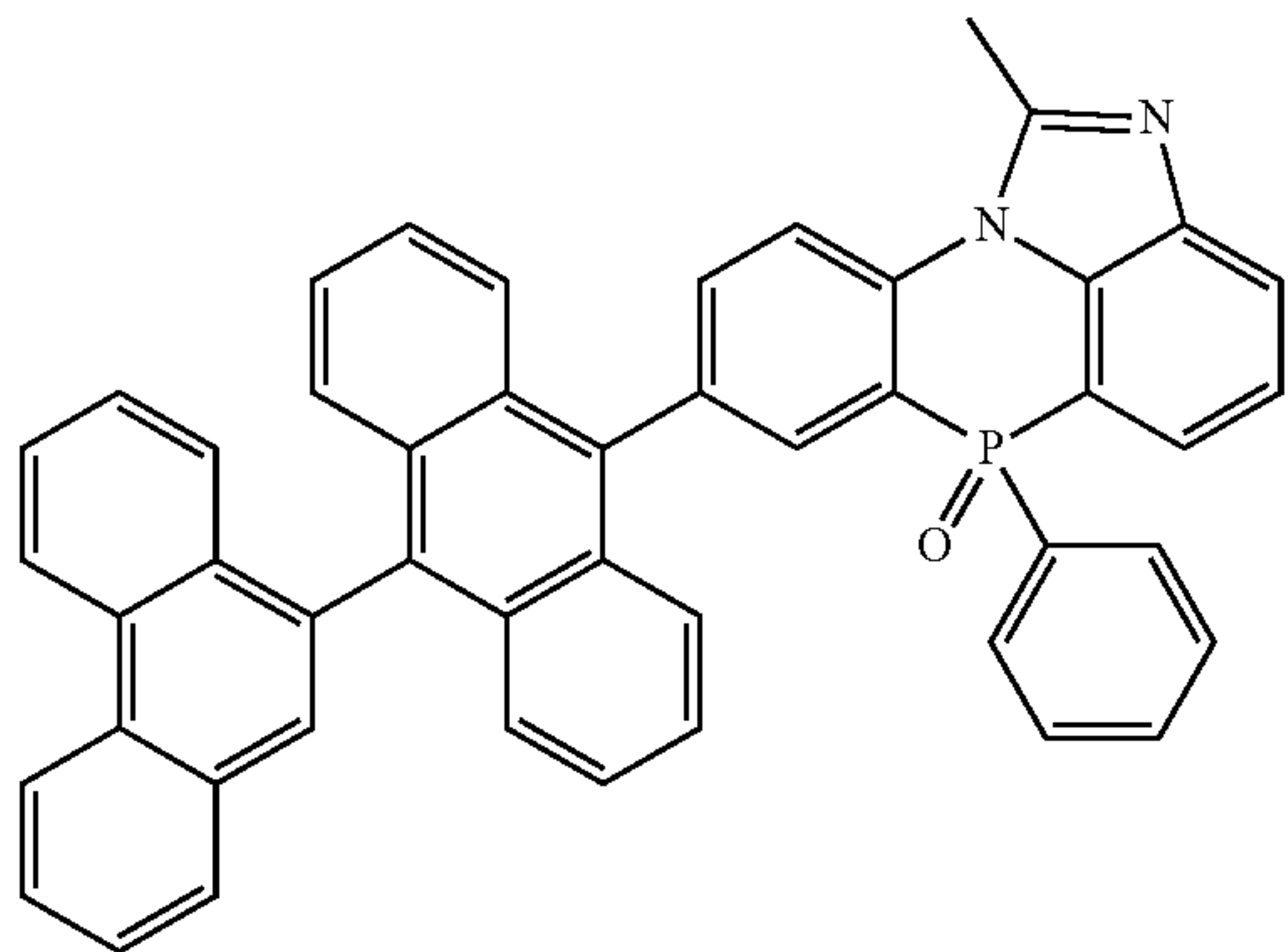
[Chemical Formula 2-2-8]
