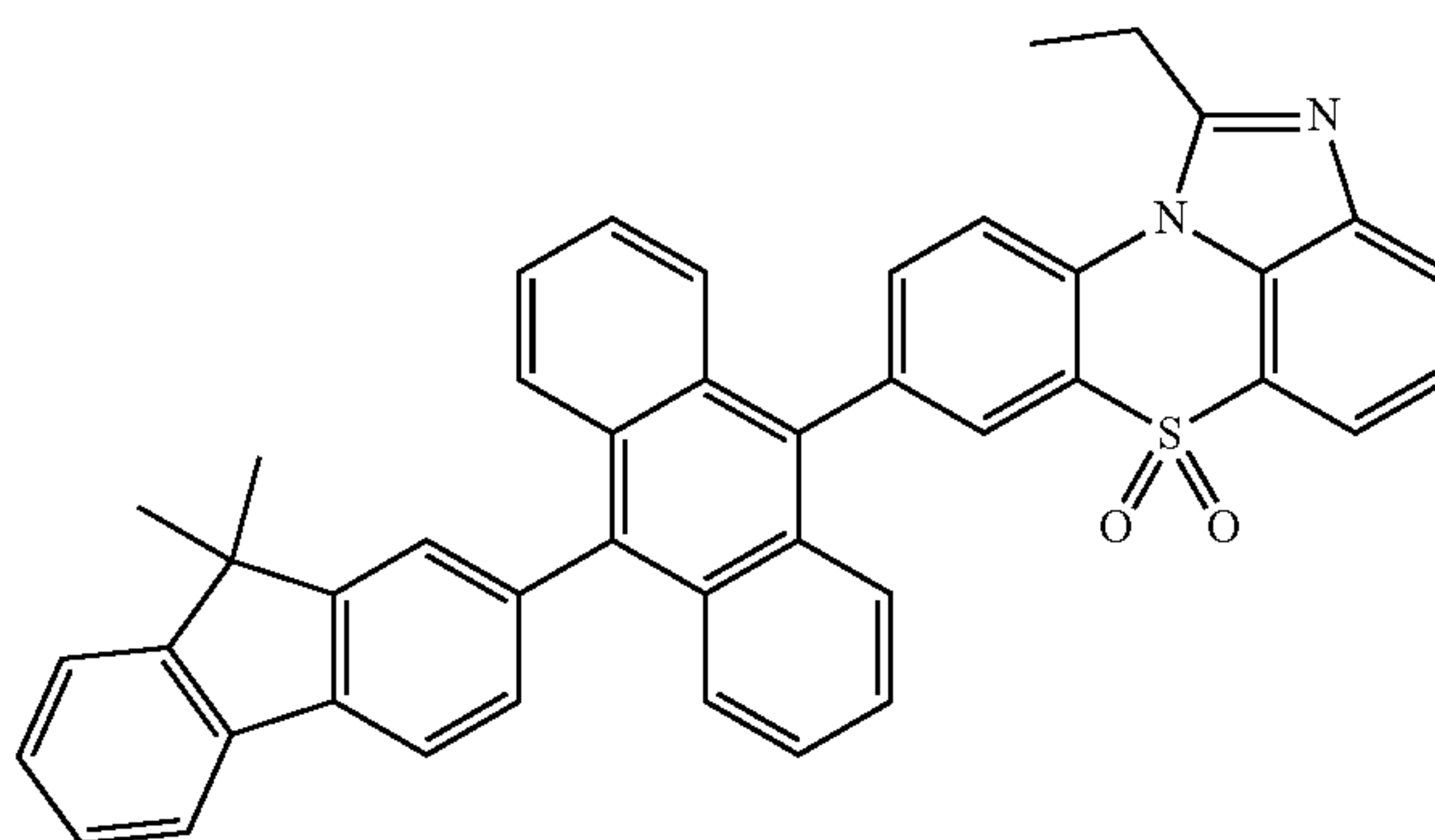
[Chemical Formula 1-3-5]
