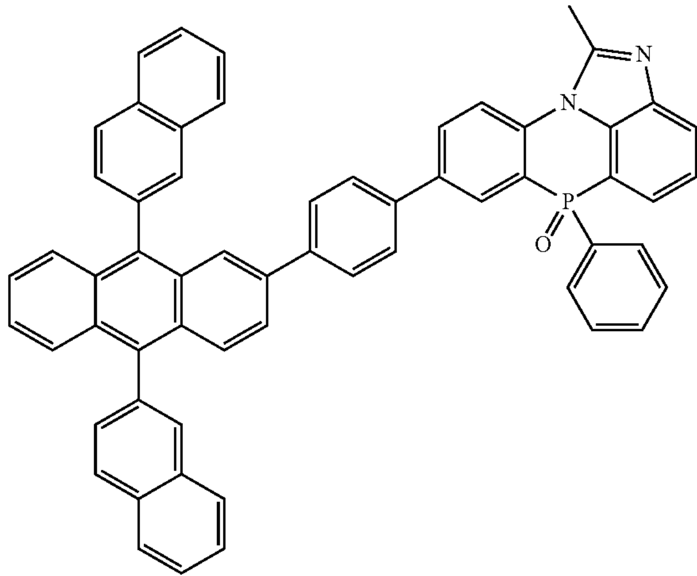
[Chemical Formula 2-2-25]
