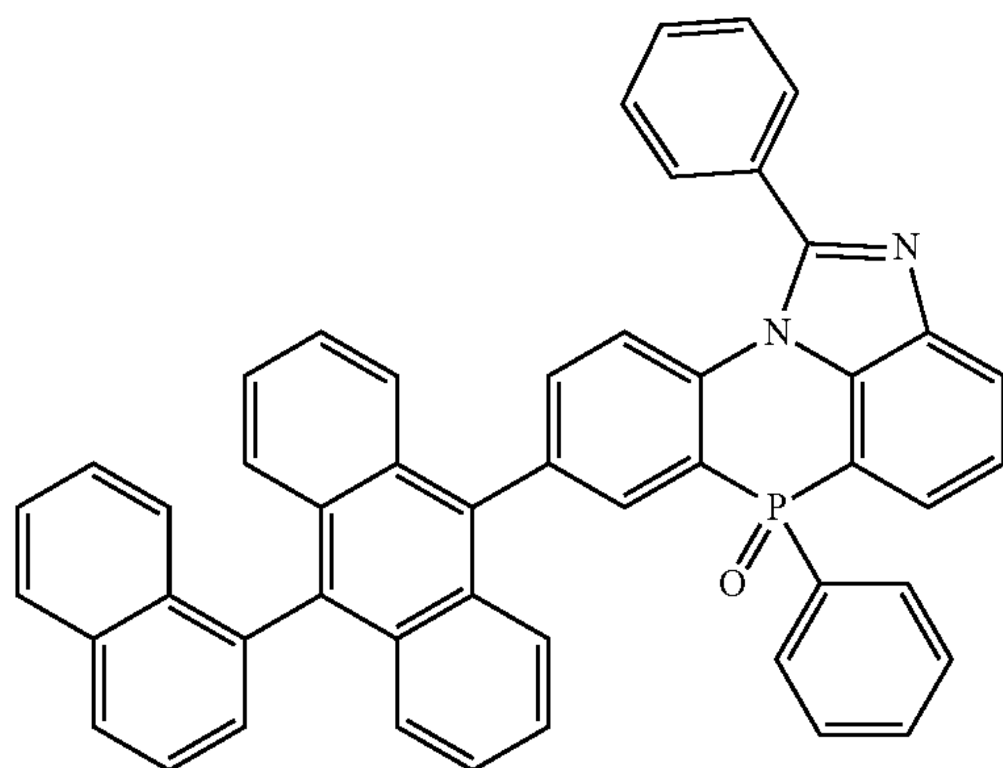
[Chemical Formula 2-4-3]
