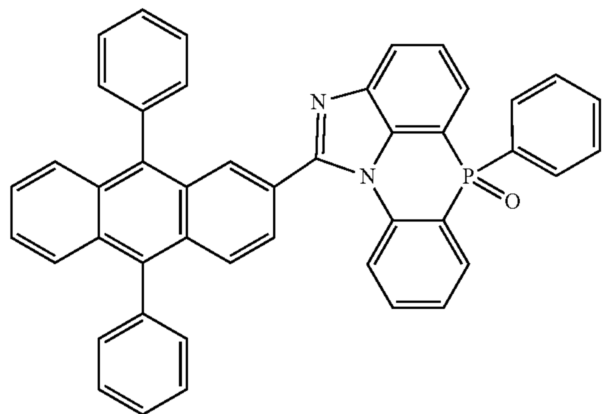
[Chemical Formula 2-5-19]
