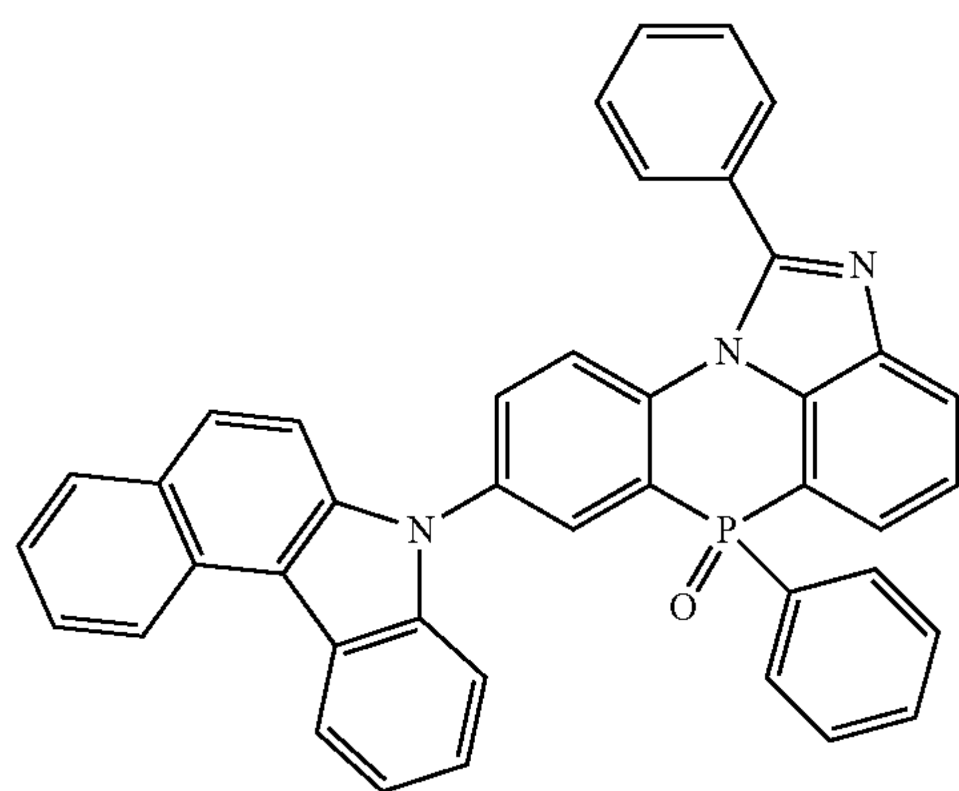
[Chemical Formula 2-4-52]
