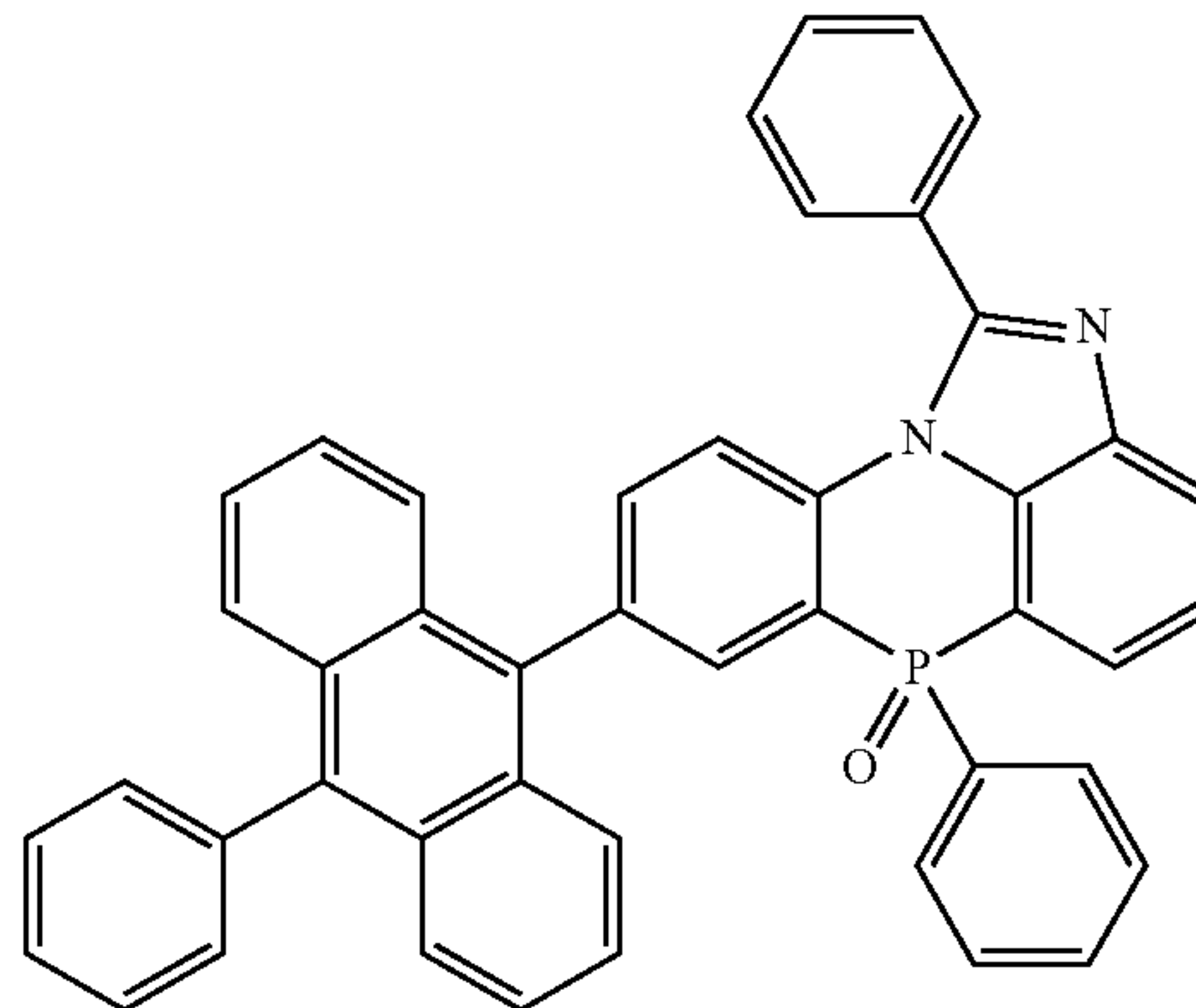
[Chemical Formula 2-4-1]
