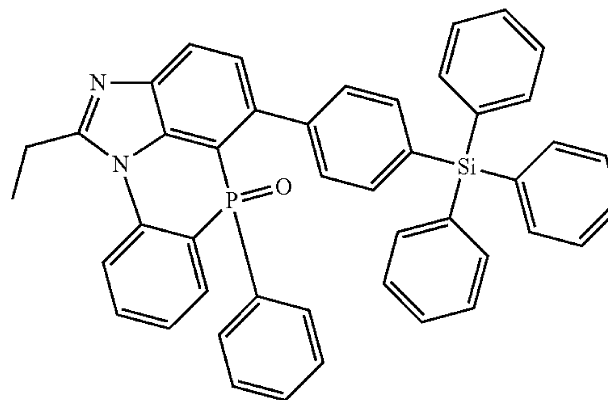
[Chemical Formula 2-9-13]
