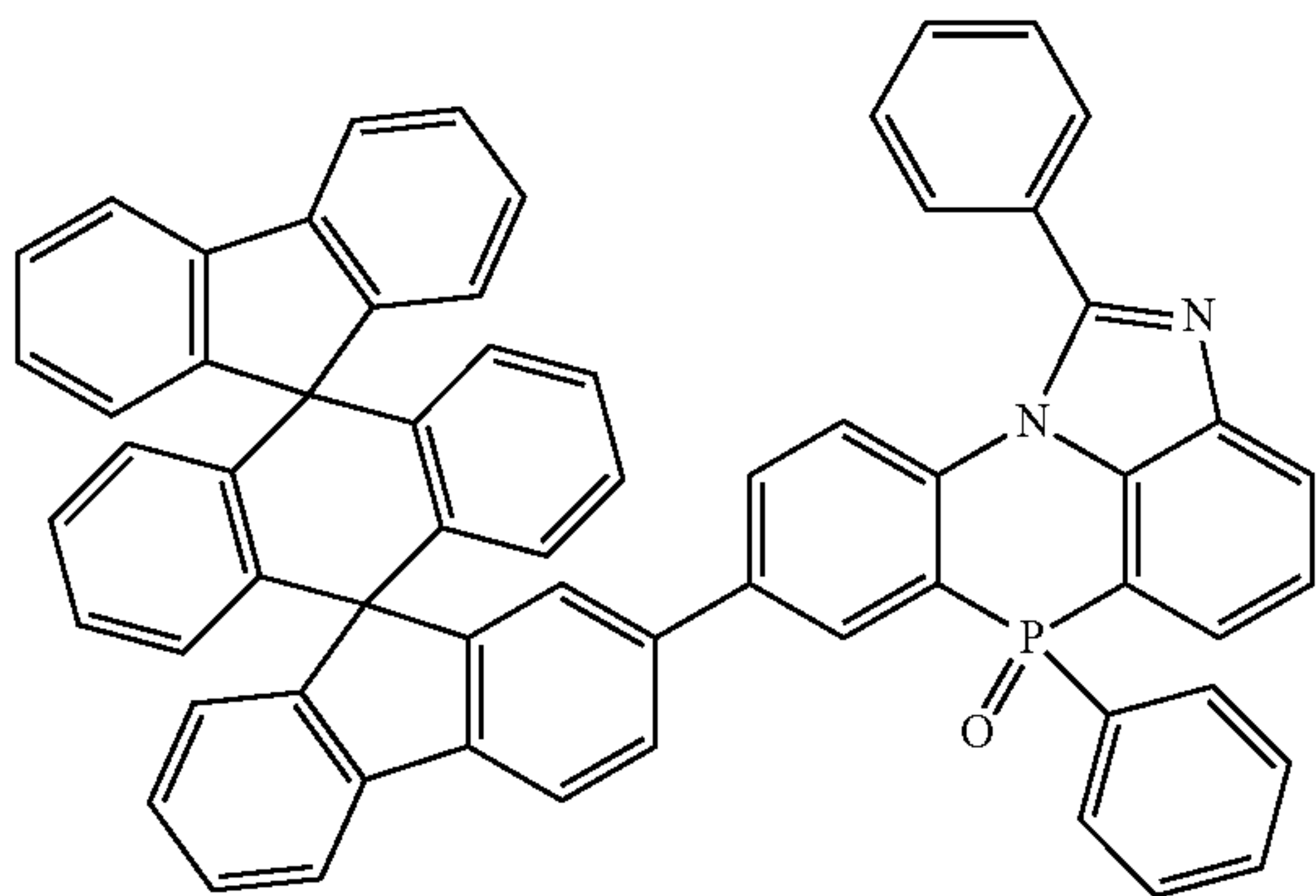
[Chemical Formula 2-4-37]
