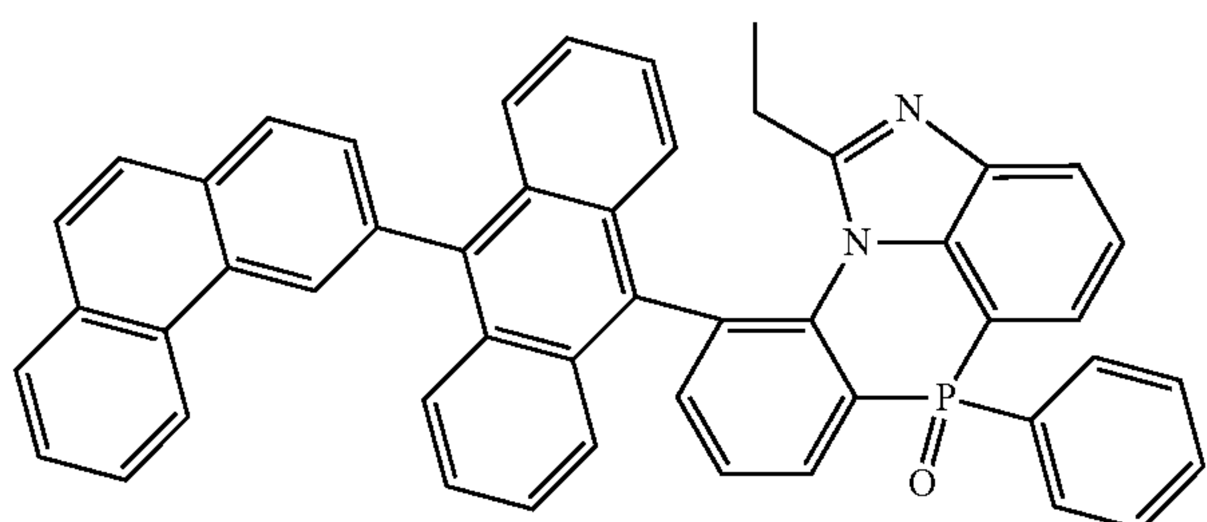
[Chemical Formula 2-8-8]
