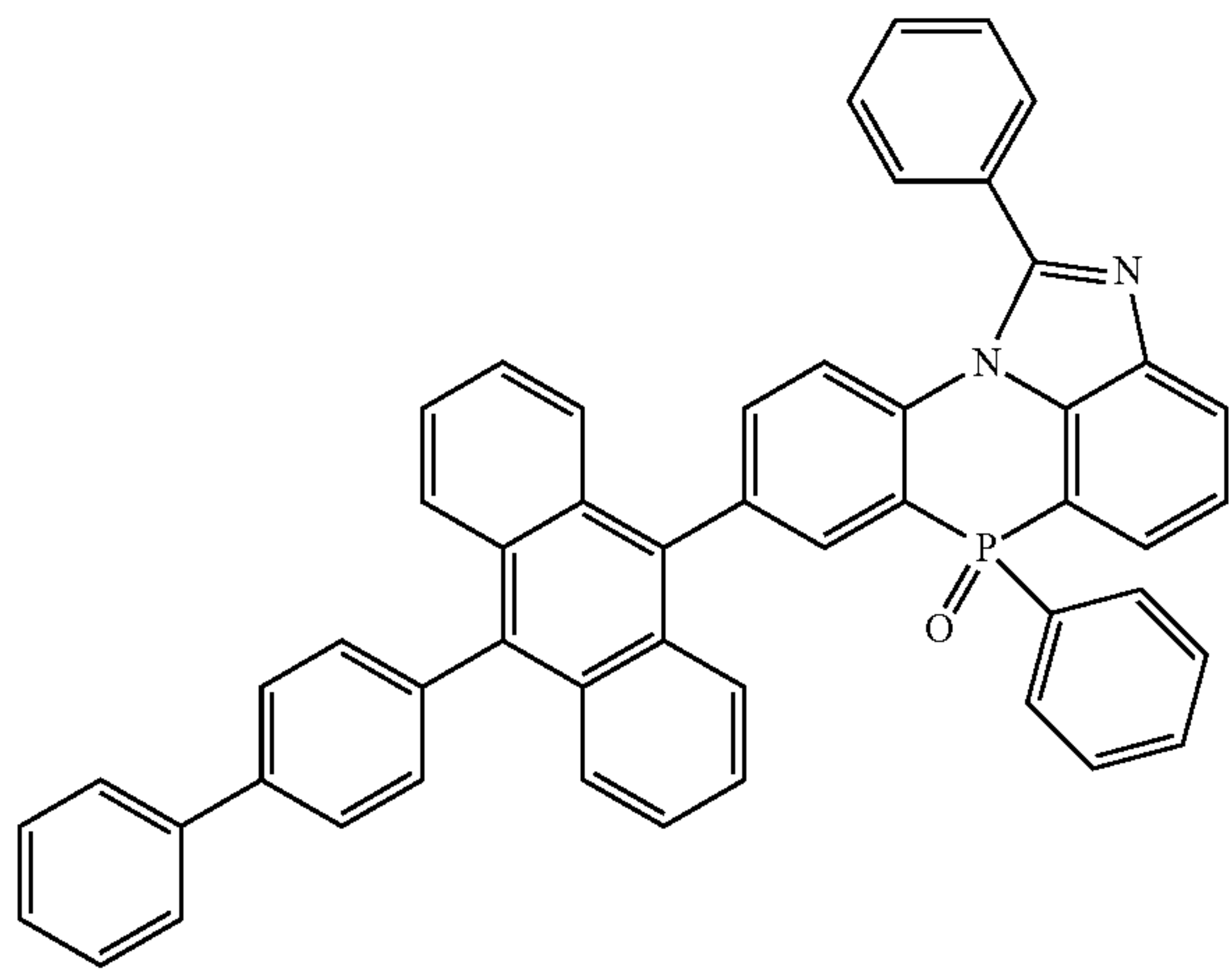
[Chemical Formula 2-4-4]
