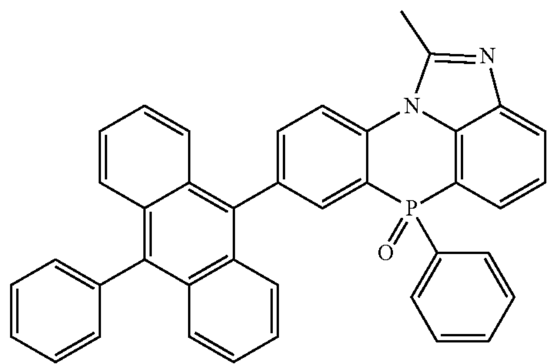
[Chemical Formula 2-2-1]
