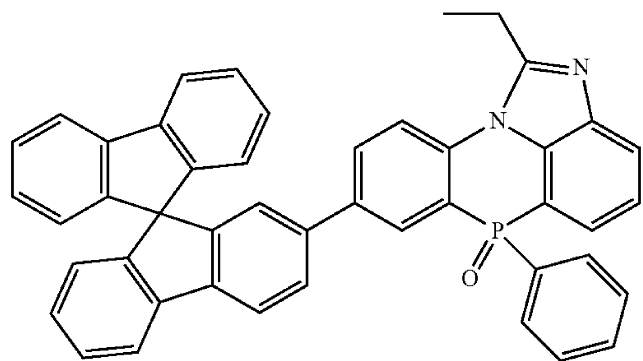
[Chemical Formula 2-3-34]
