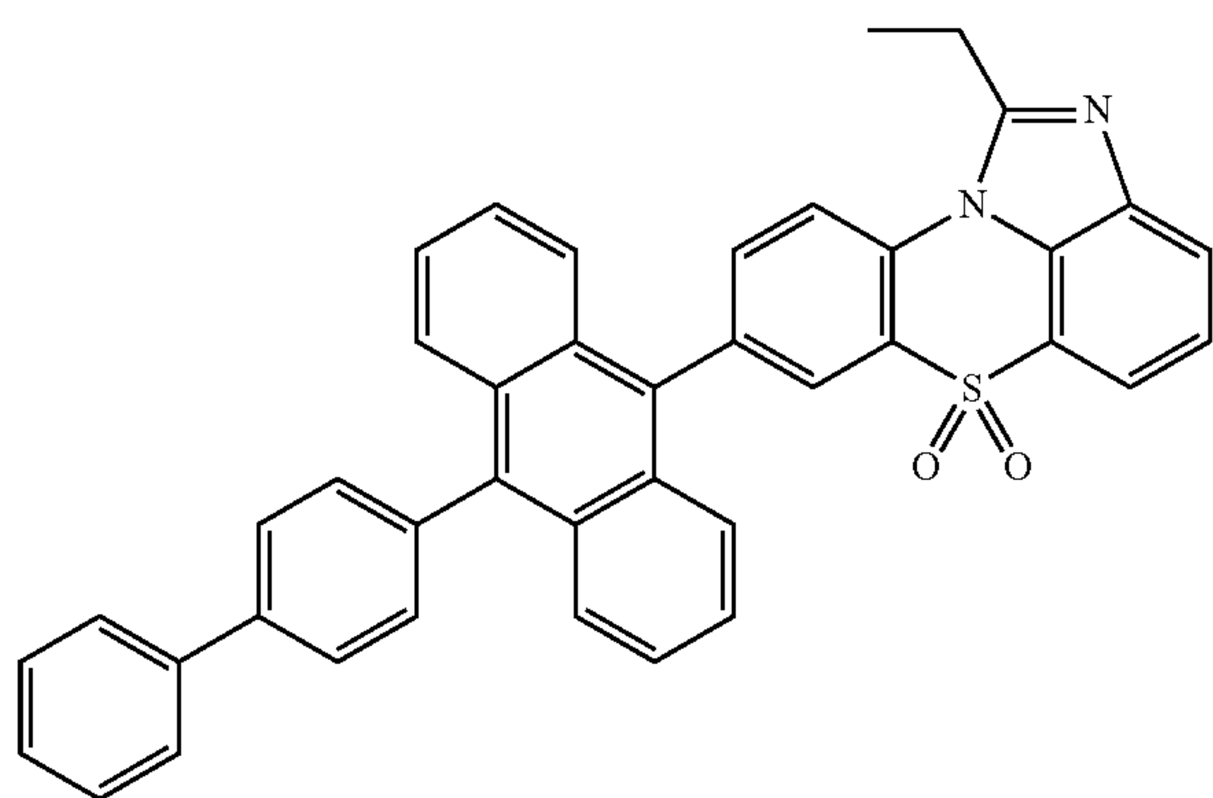
[Chemical Formula 1-3-4]
