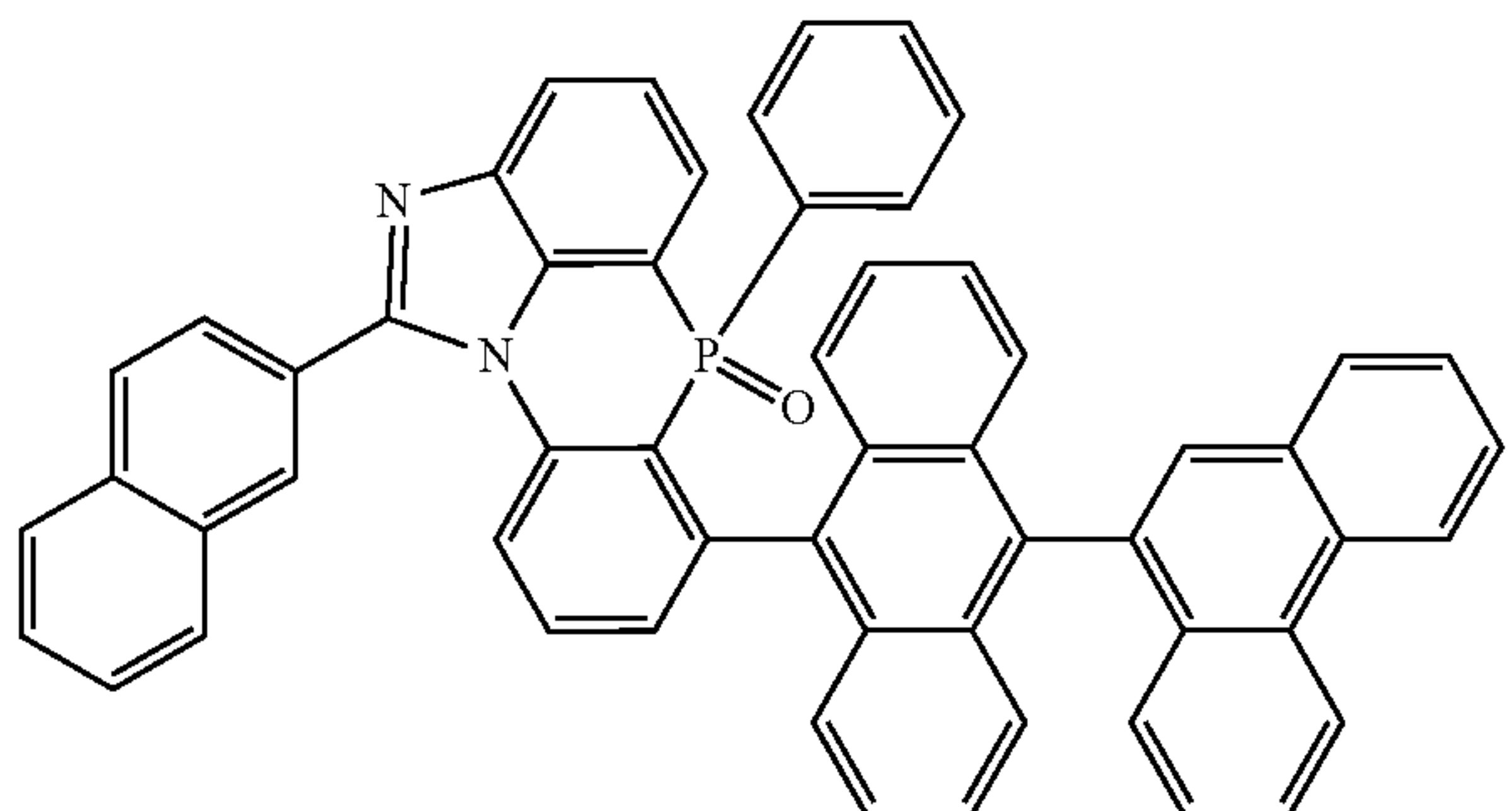
[Chemical Formula 2-6-8]
