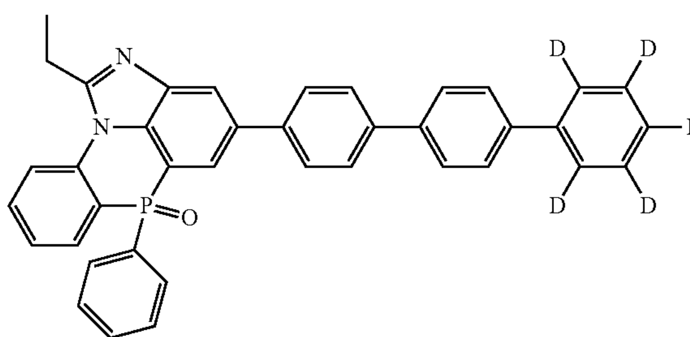
[Chemical Formula 2-10-16]
