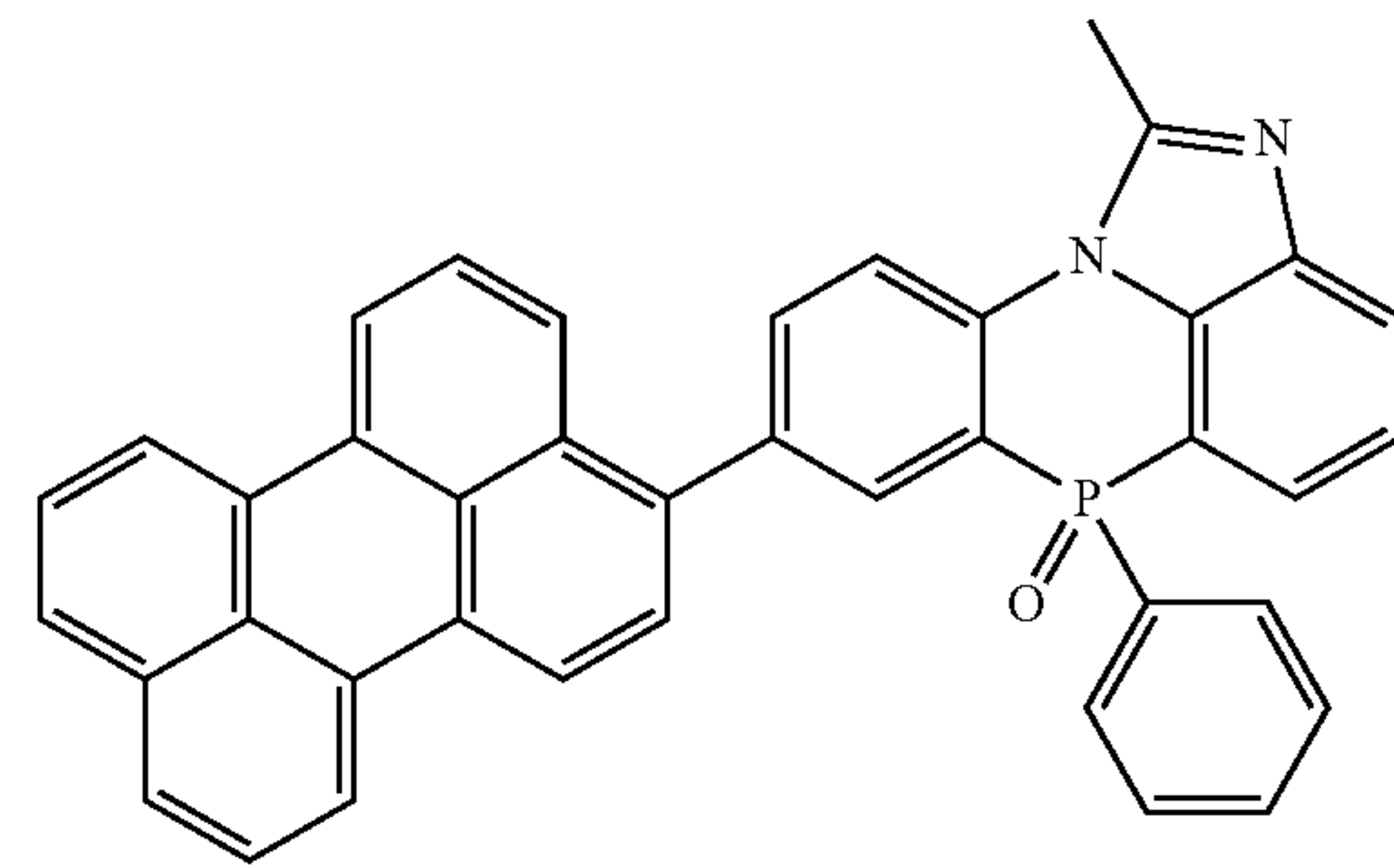
[Chemical Formula 2-2-29]
