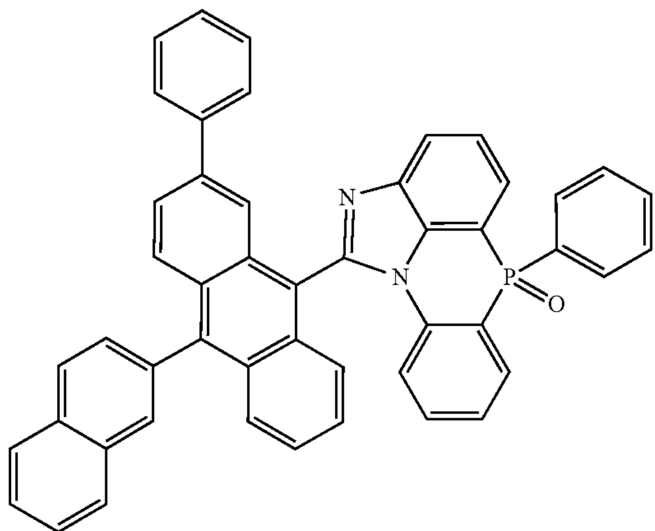
[Chemical Formula 2-5-16]
