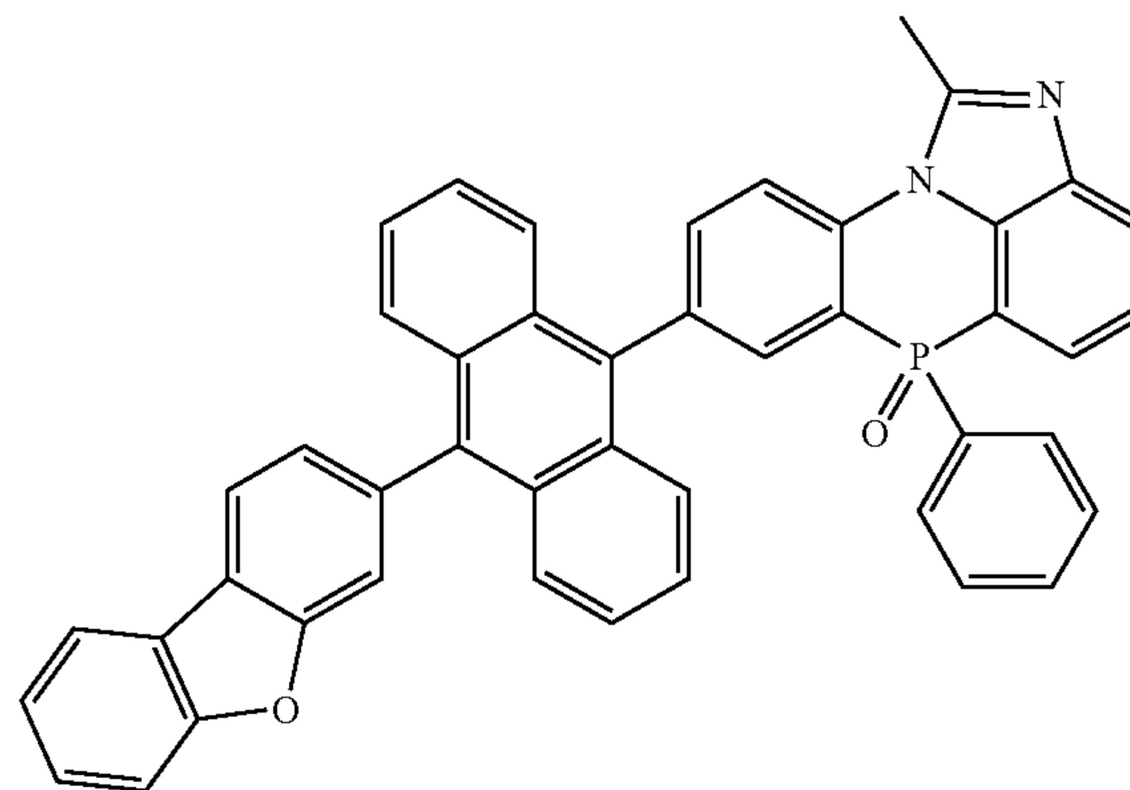
[Chemical Formula 2-2-13]
