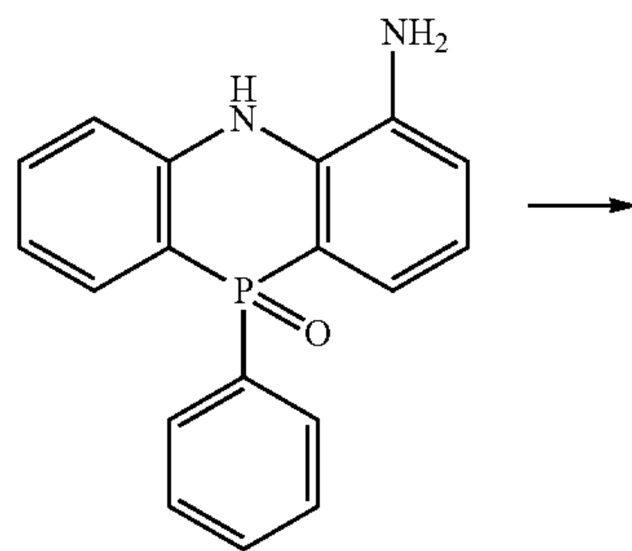
[Compound 2-1-F]
