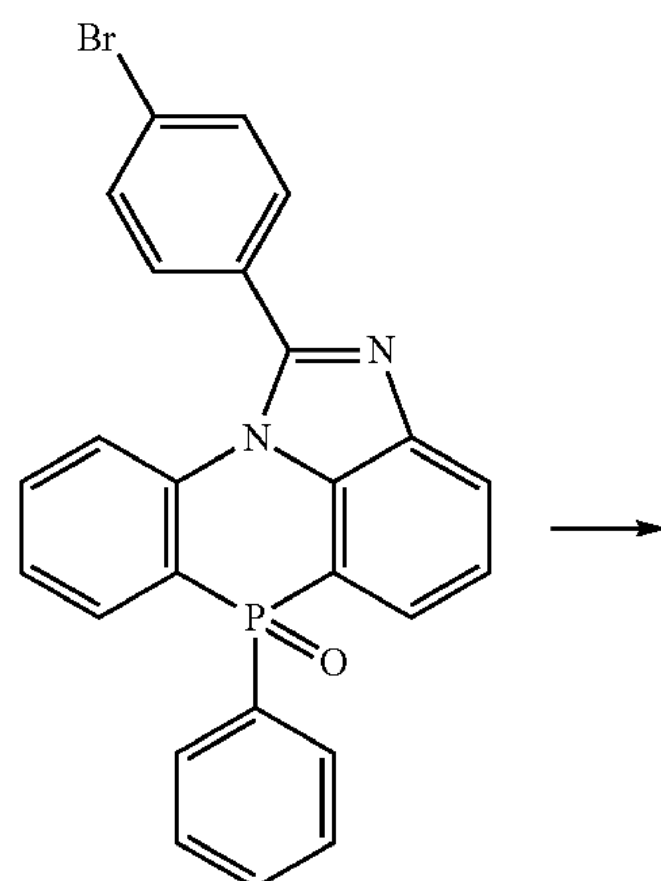
[Compound 2-1-G]
