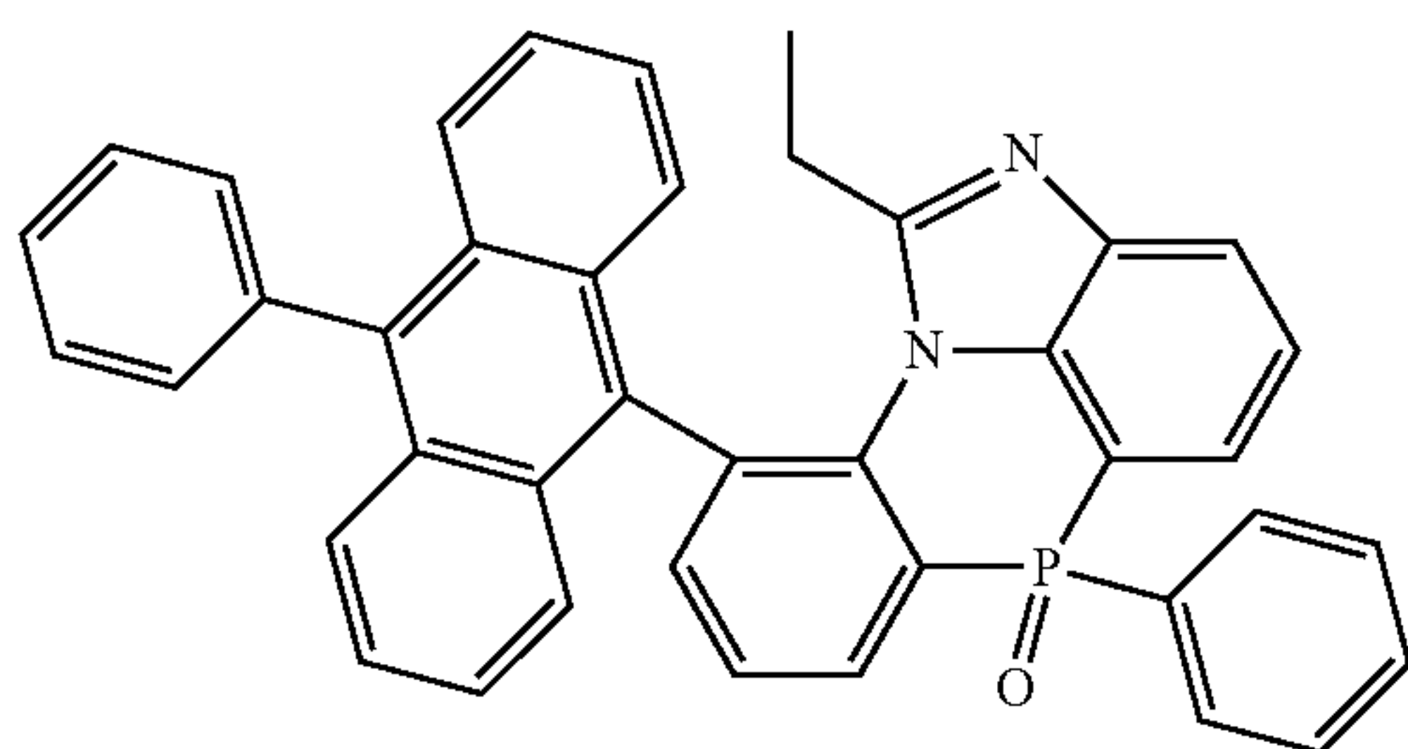
[Chemical Formula 2-8-1]
