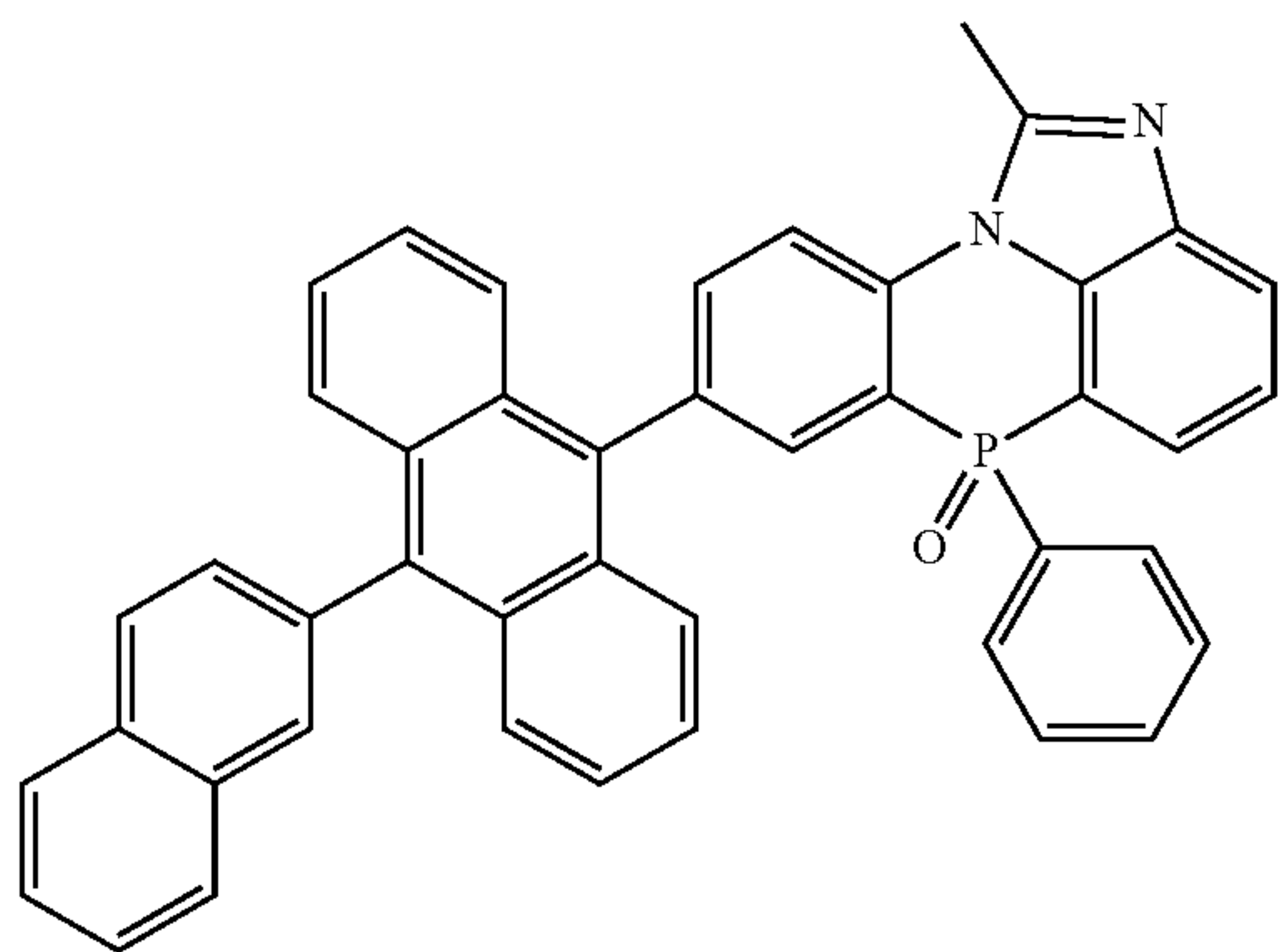
[Chemical Formula 2-2-2]
