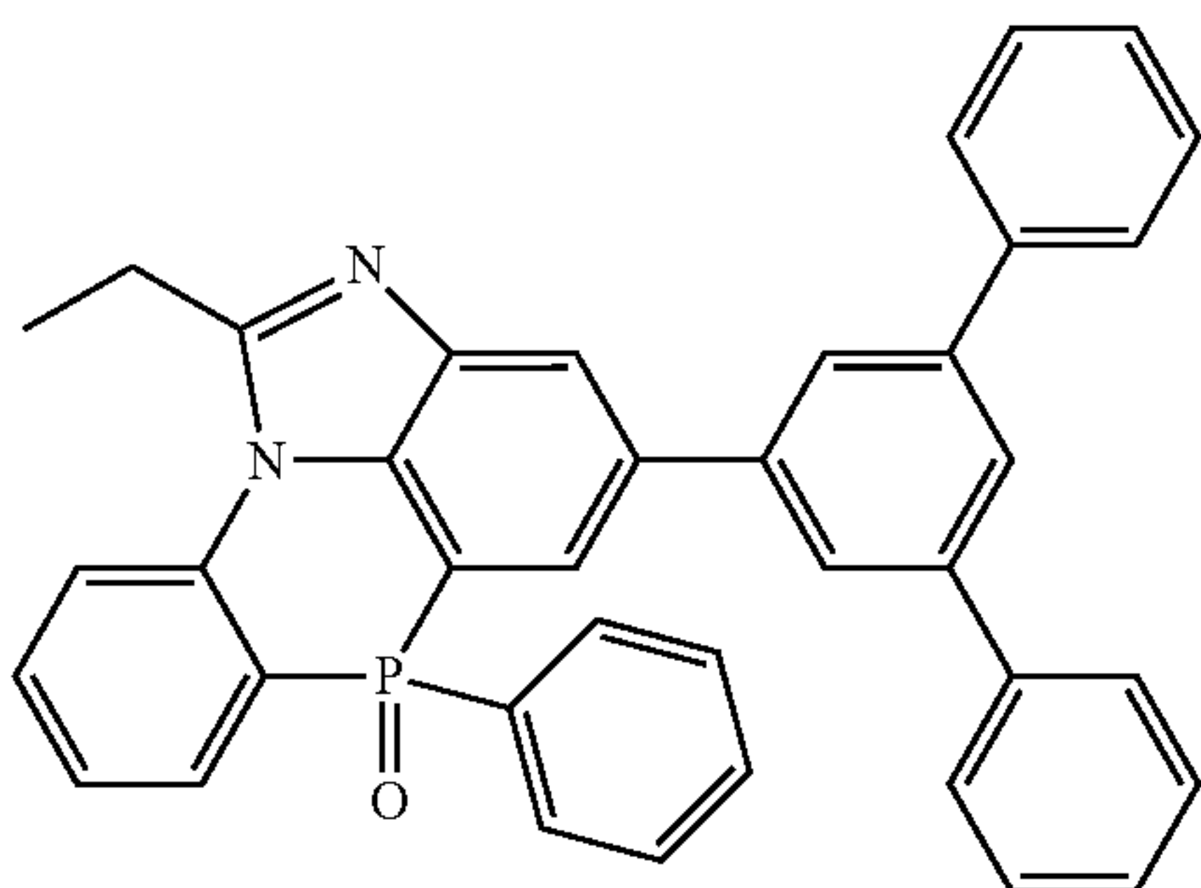
[Chemical Formula 2-10-4]
