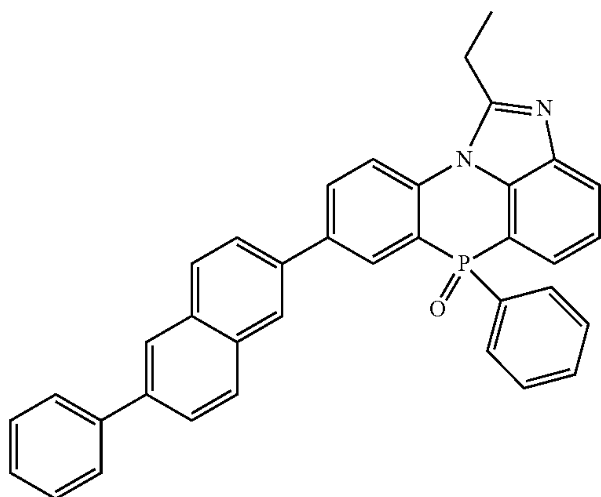
[Chemical Formula 2-3-27]
