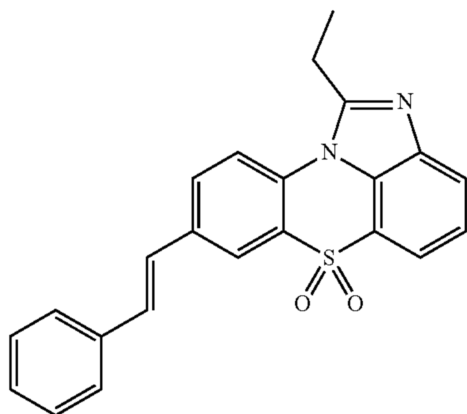
[Chemical Formula 1-3-54]
