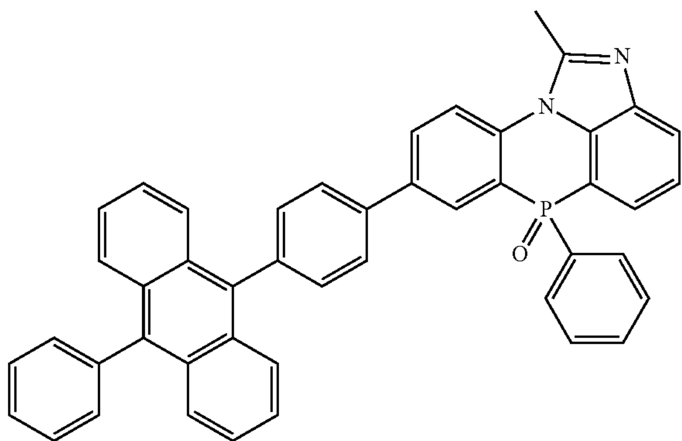
[Chemical Formula 2-2-17]
