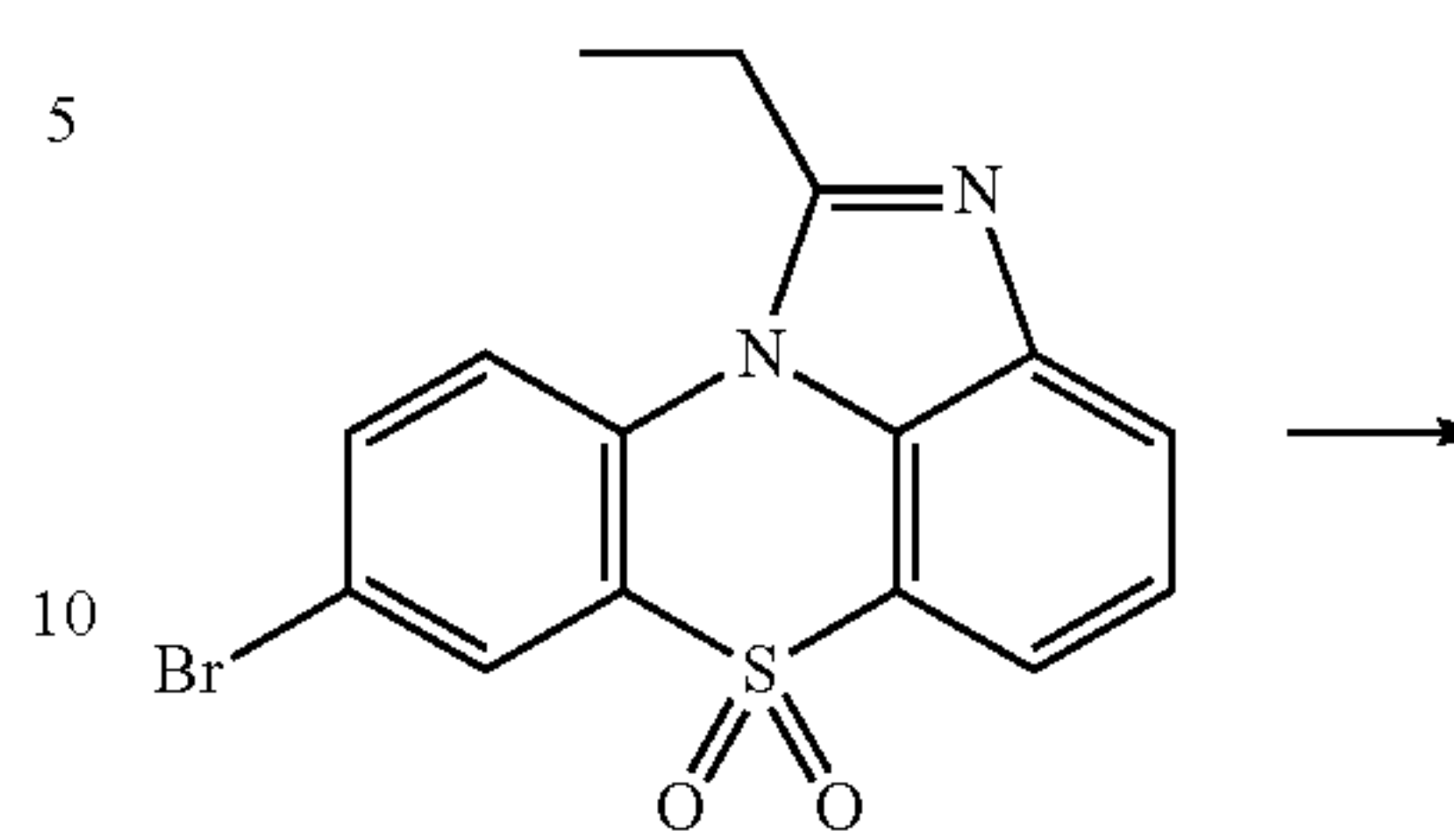
[Compound 2-B]
