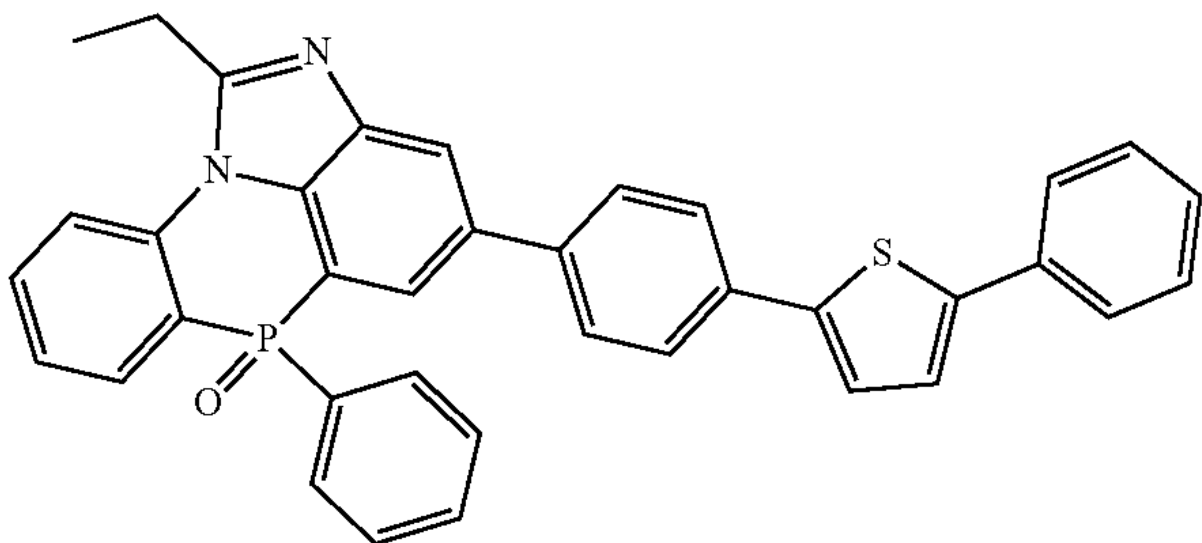
[Chemical Formula 2-10-3]
