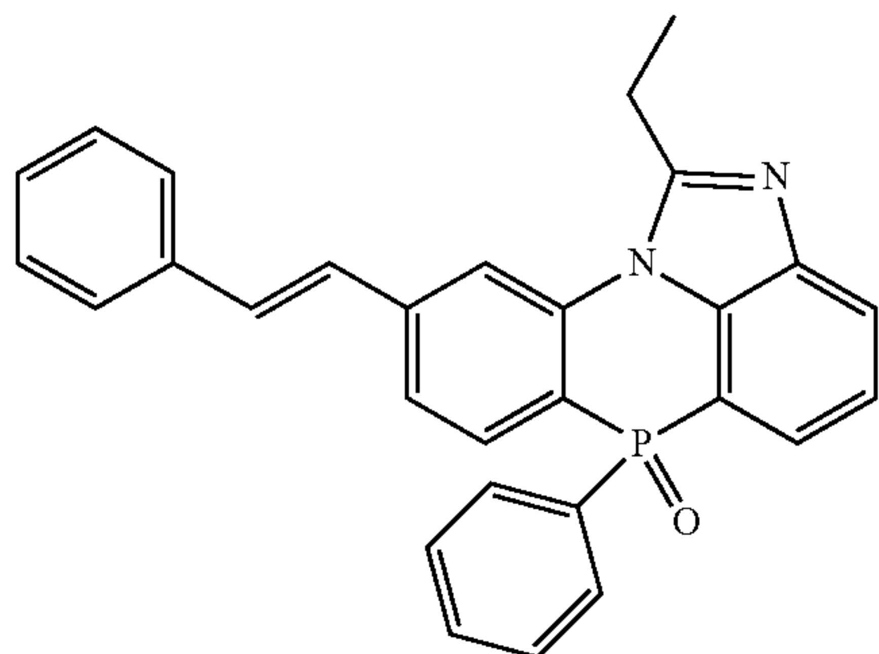
[Chemical Formula 2-7-54]
