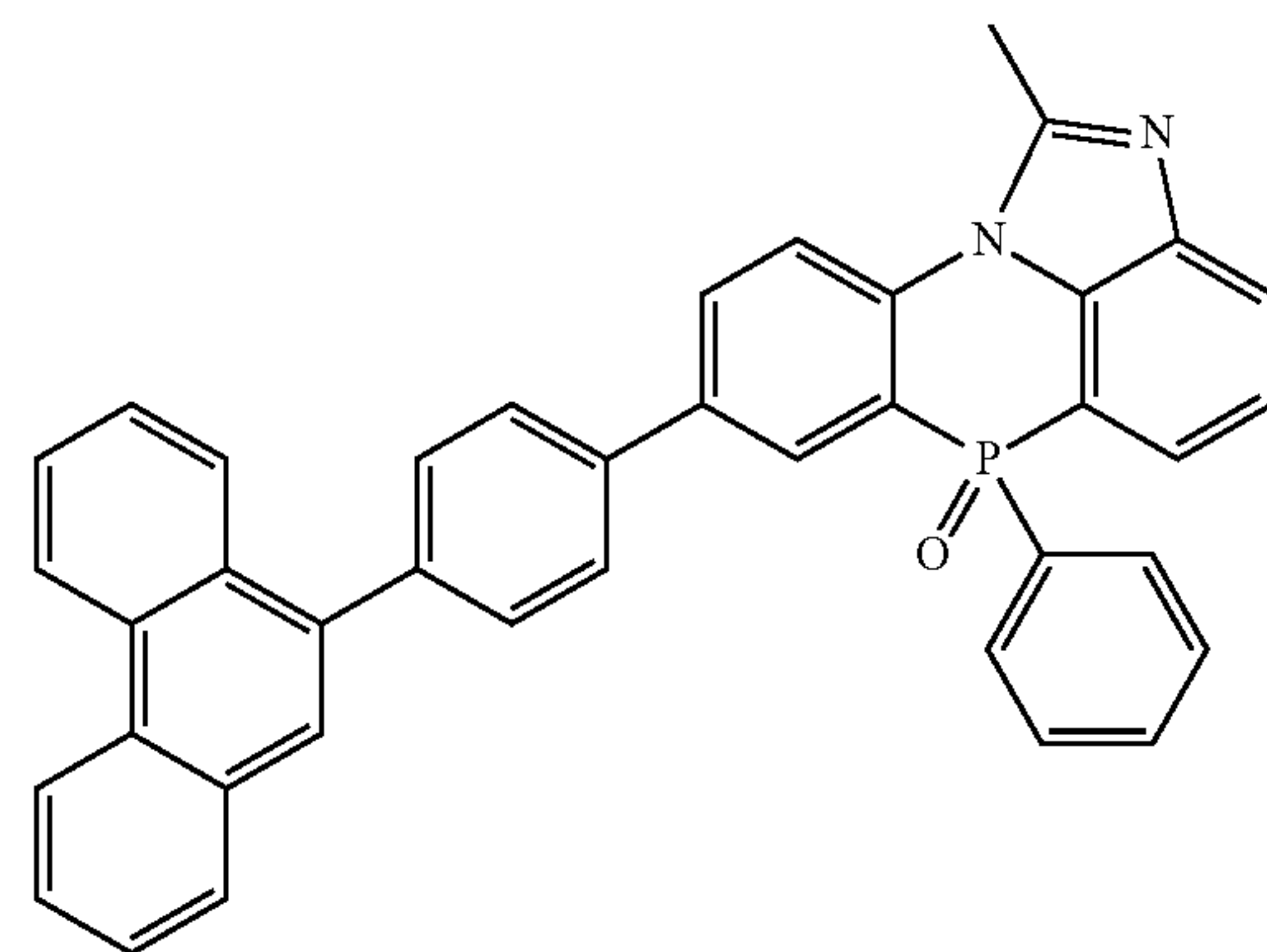
[Chemical Formula 2-2-32]
