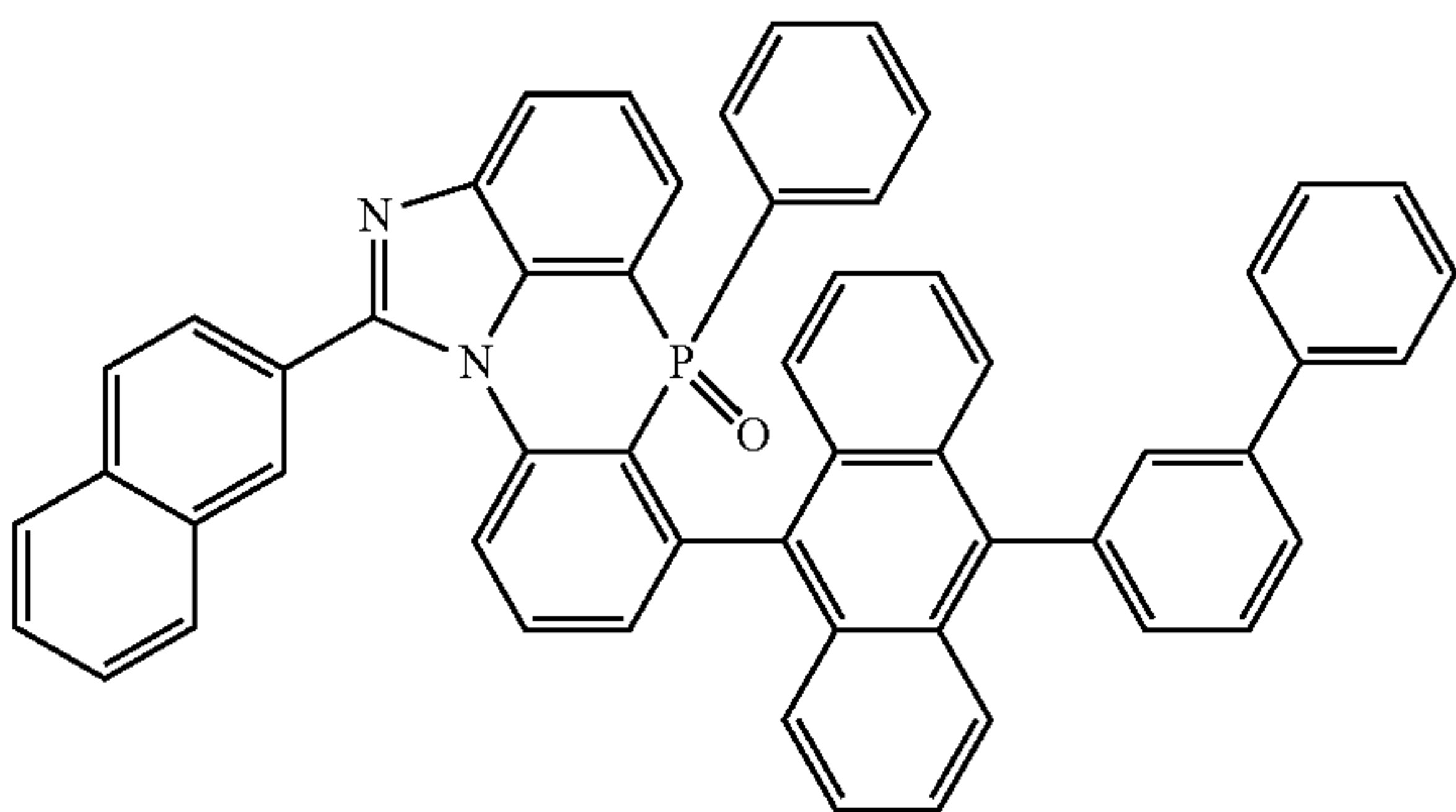
[Chemical Formula 2-6-7]
