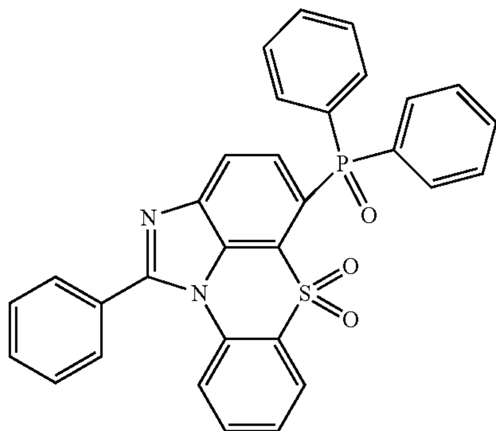
[Chemical Formula 1-12-7]
