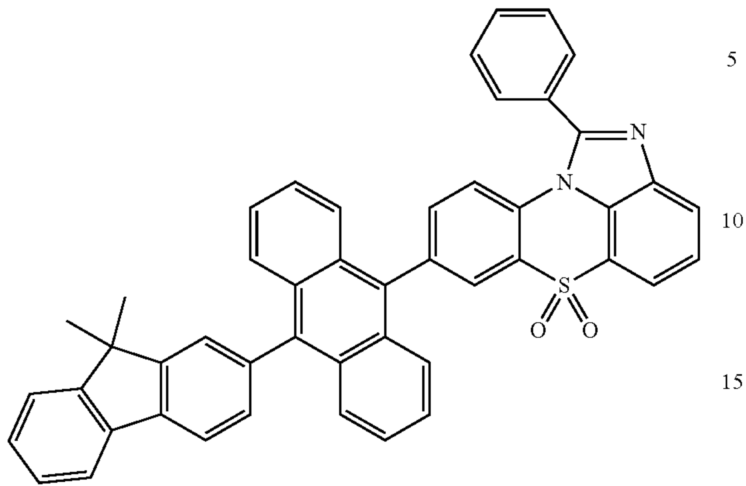
[Chemical Formula 1-4-5]
