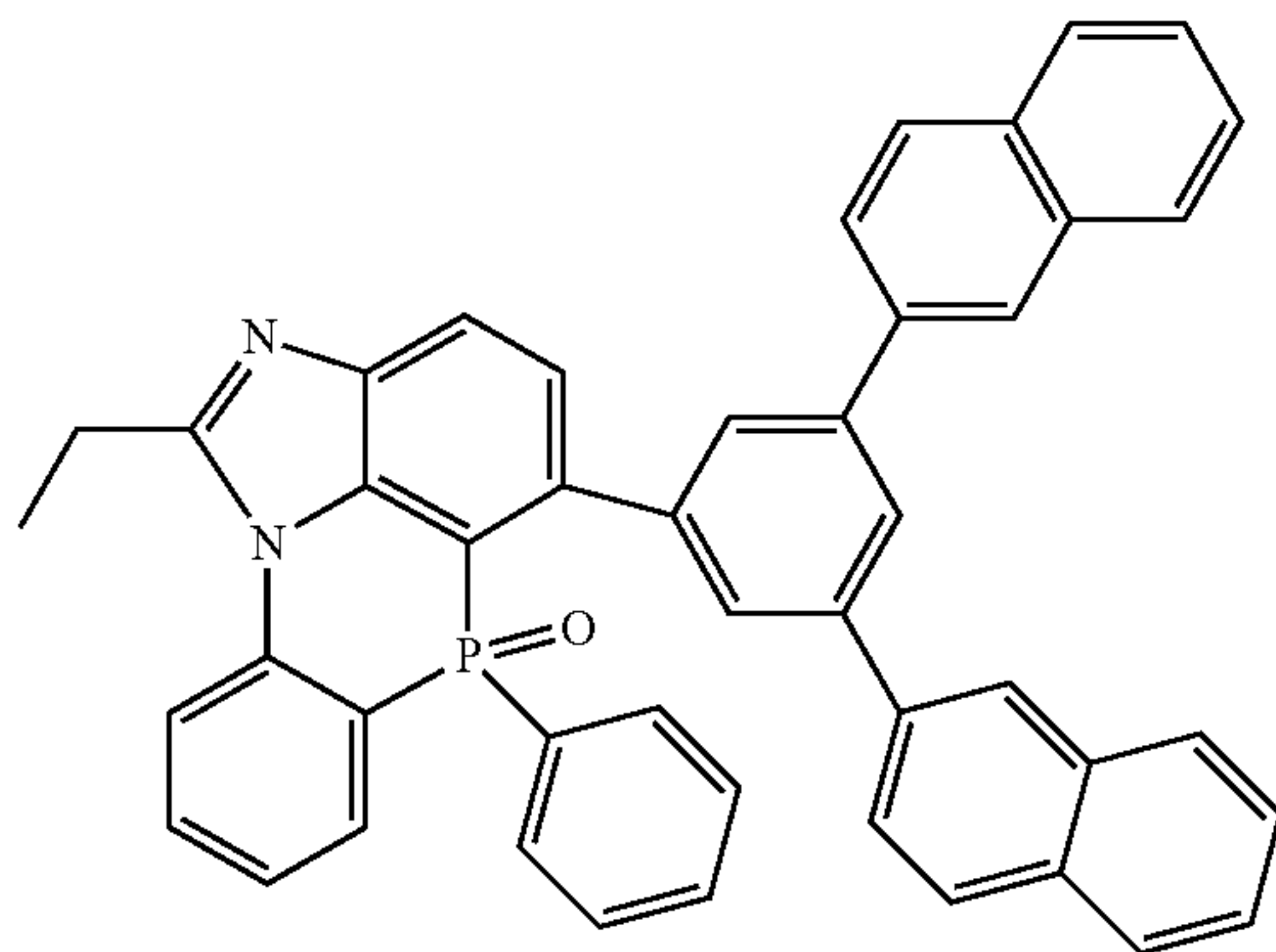
[Chemical Formula 2-9-8]
