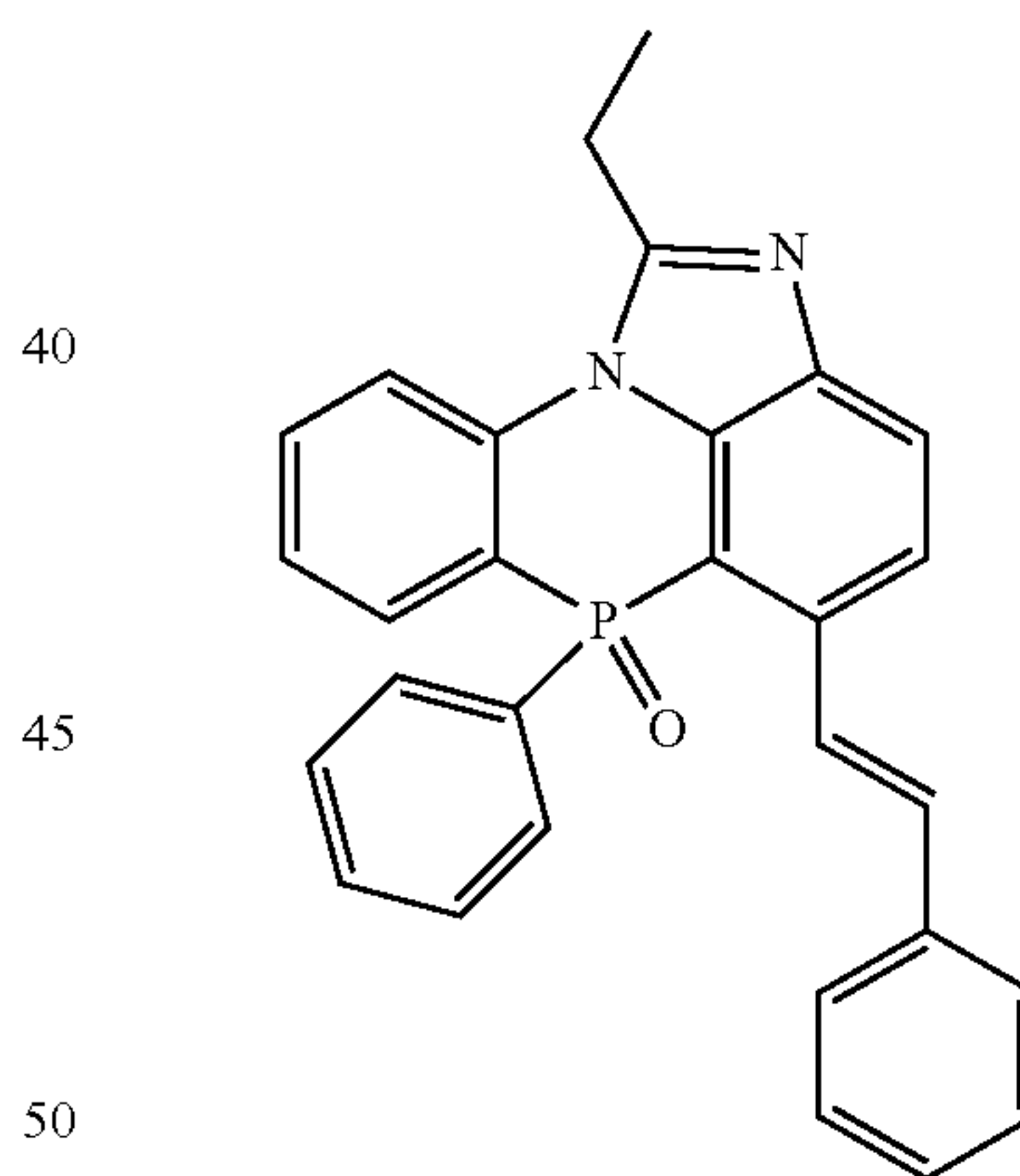
[Chemical Formula 2-9-14]
