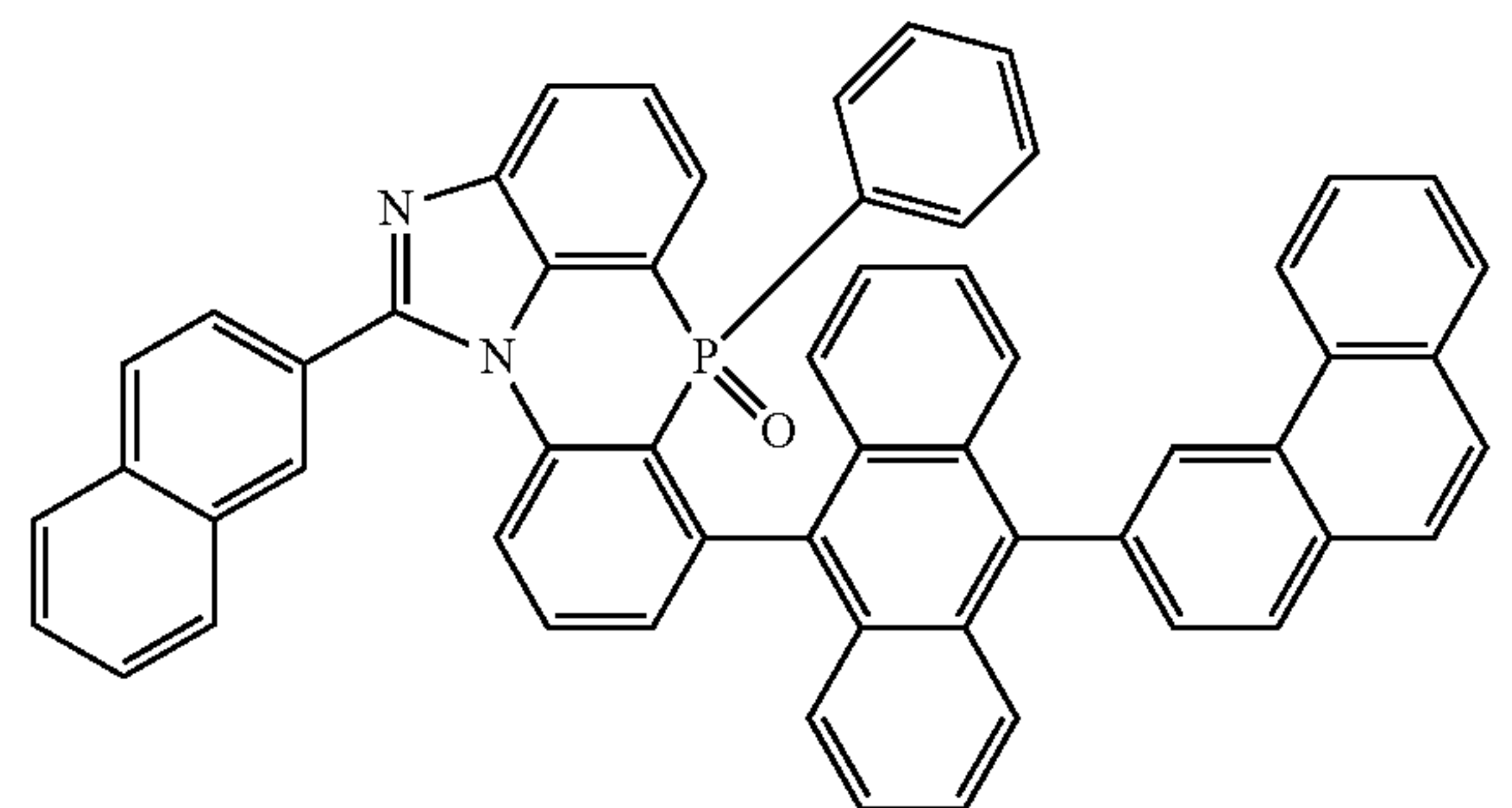
[Chemical Formula 2-6-8]
