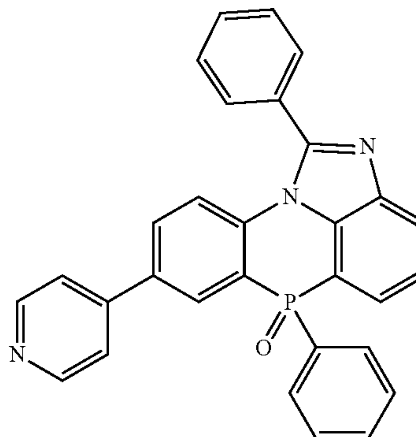
[Chemical Formula 2-4-39]
