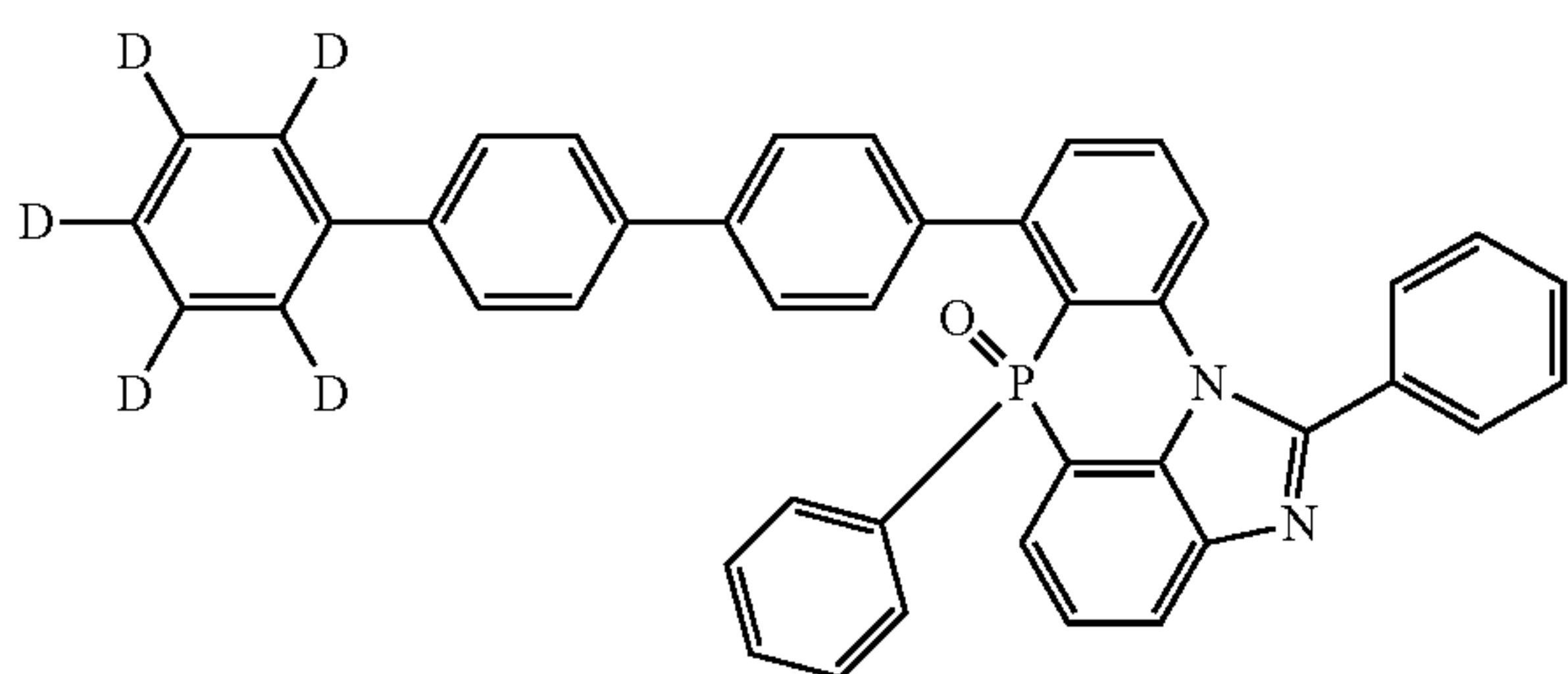
[Chemical Formula 2-6-53]
