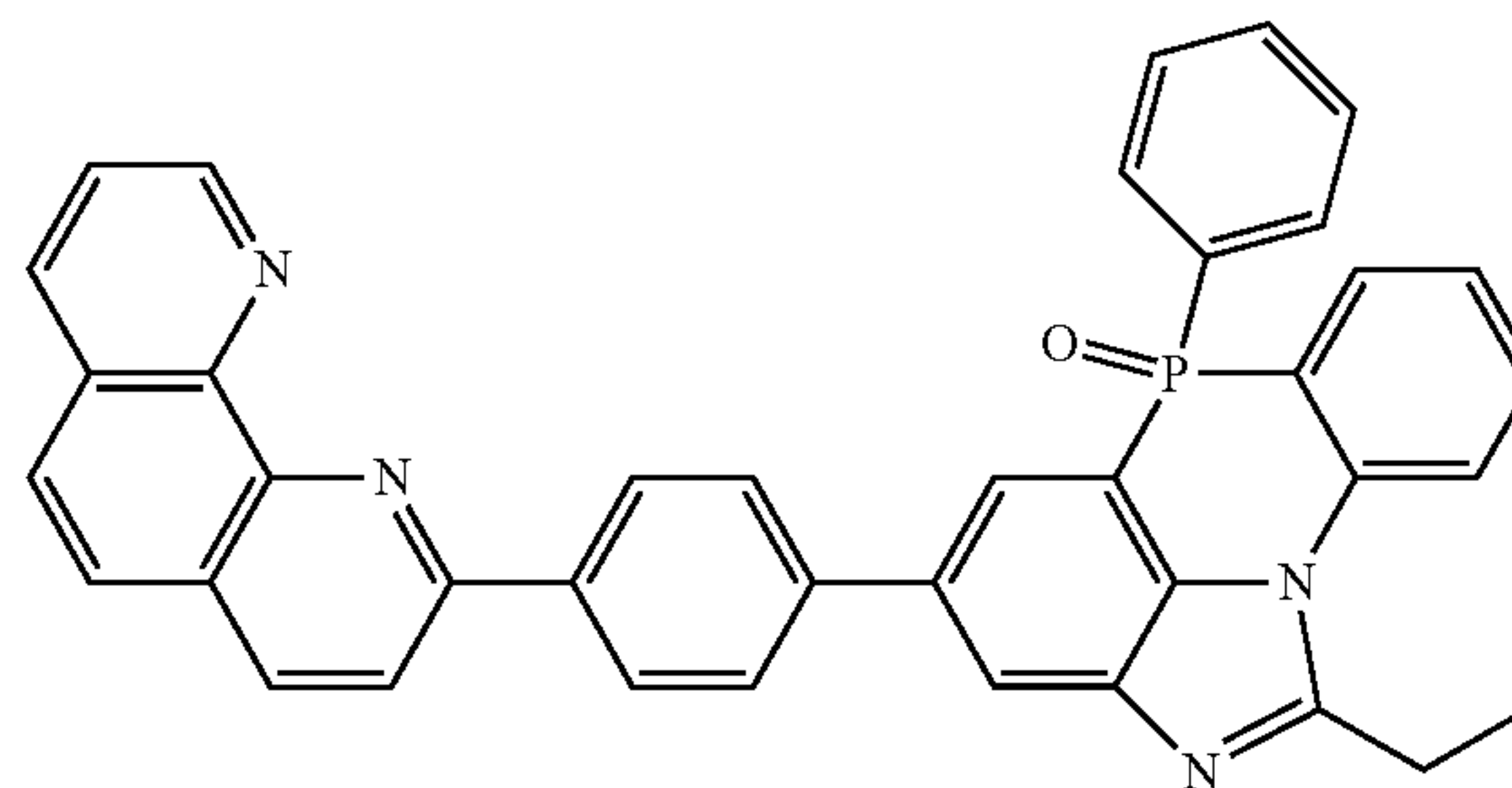
[Chemical Formula 2-10-11]
