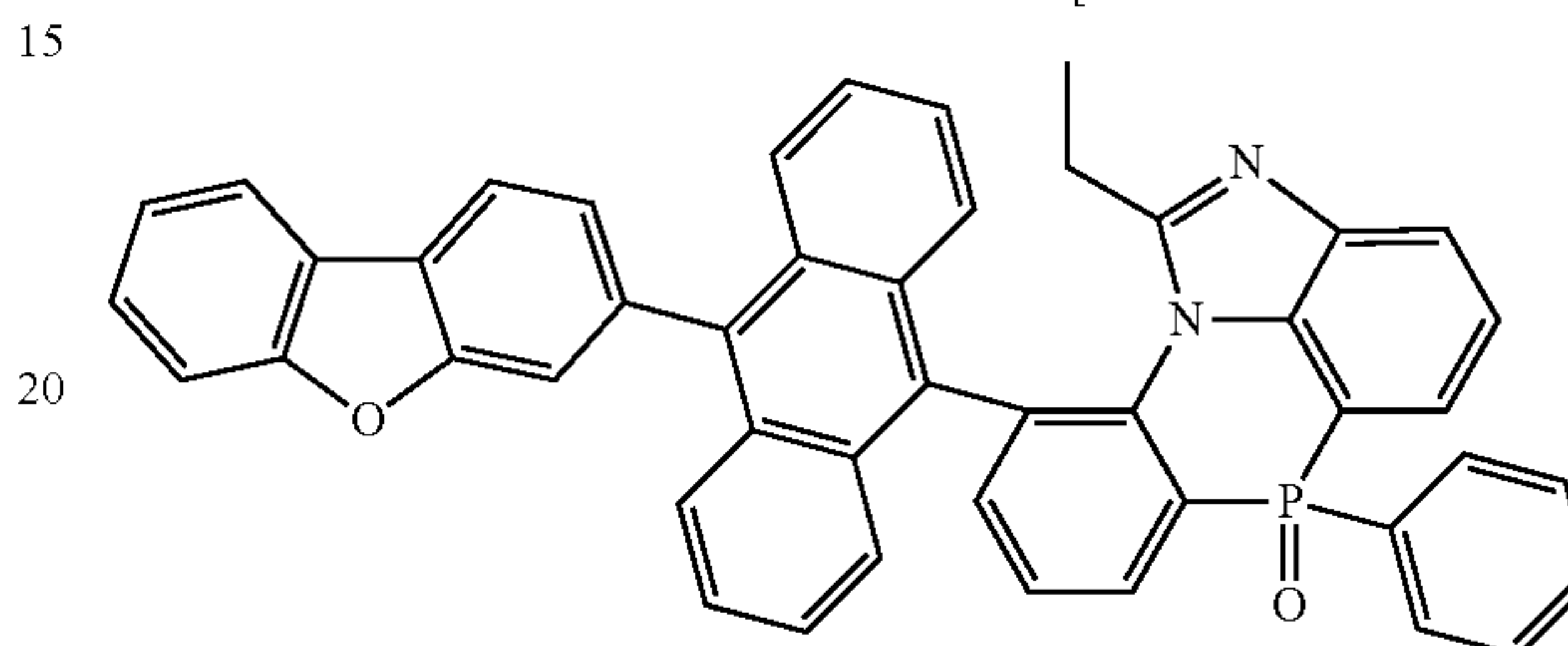
[Chemical Formula 2-8-13]
