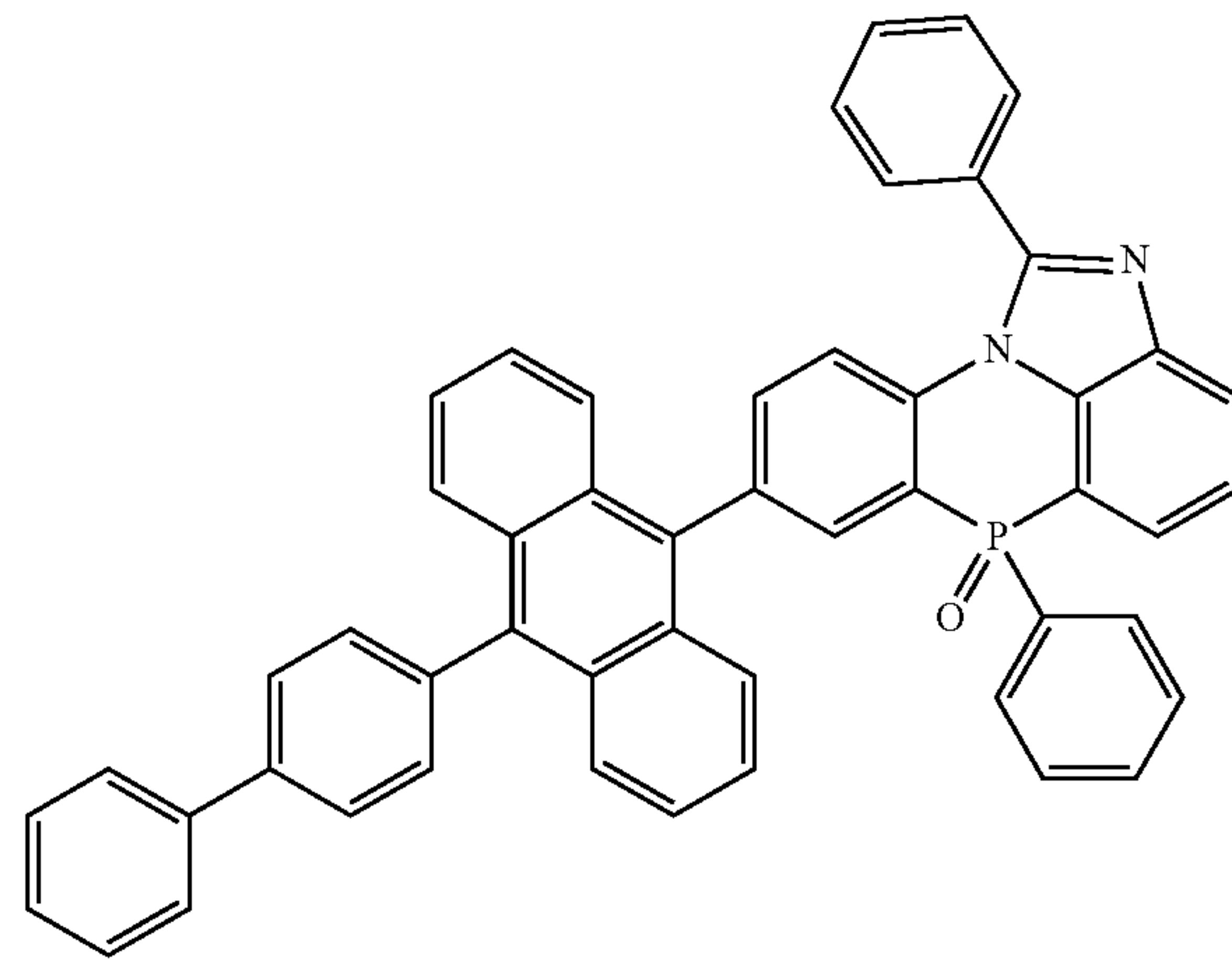
[Chemical Formula 2-4-4]
