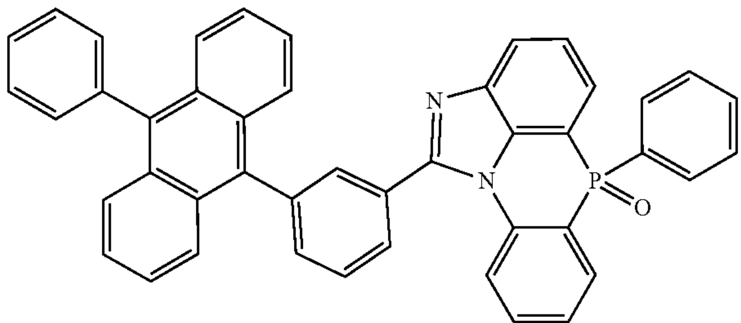
[Chemical Formula 2-5-18]
