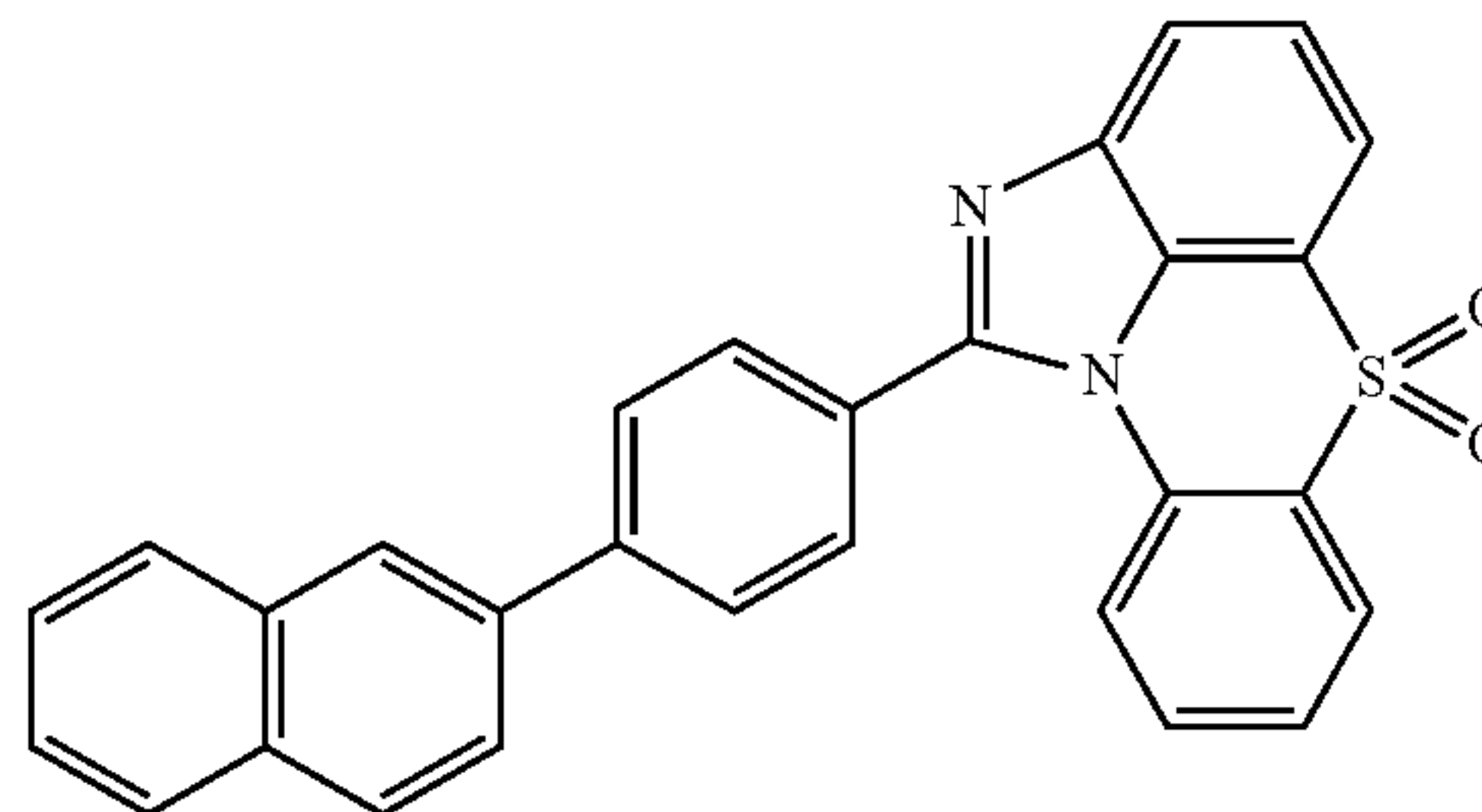
[Chemical Formula 1-5-26]
