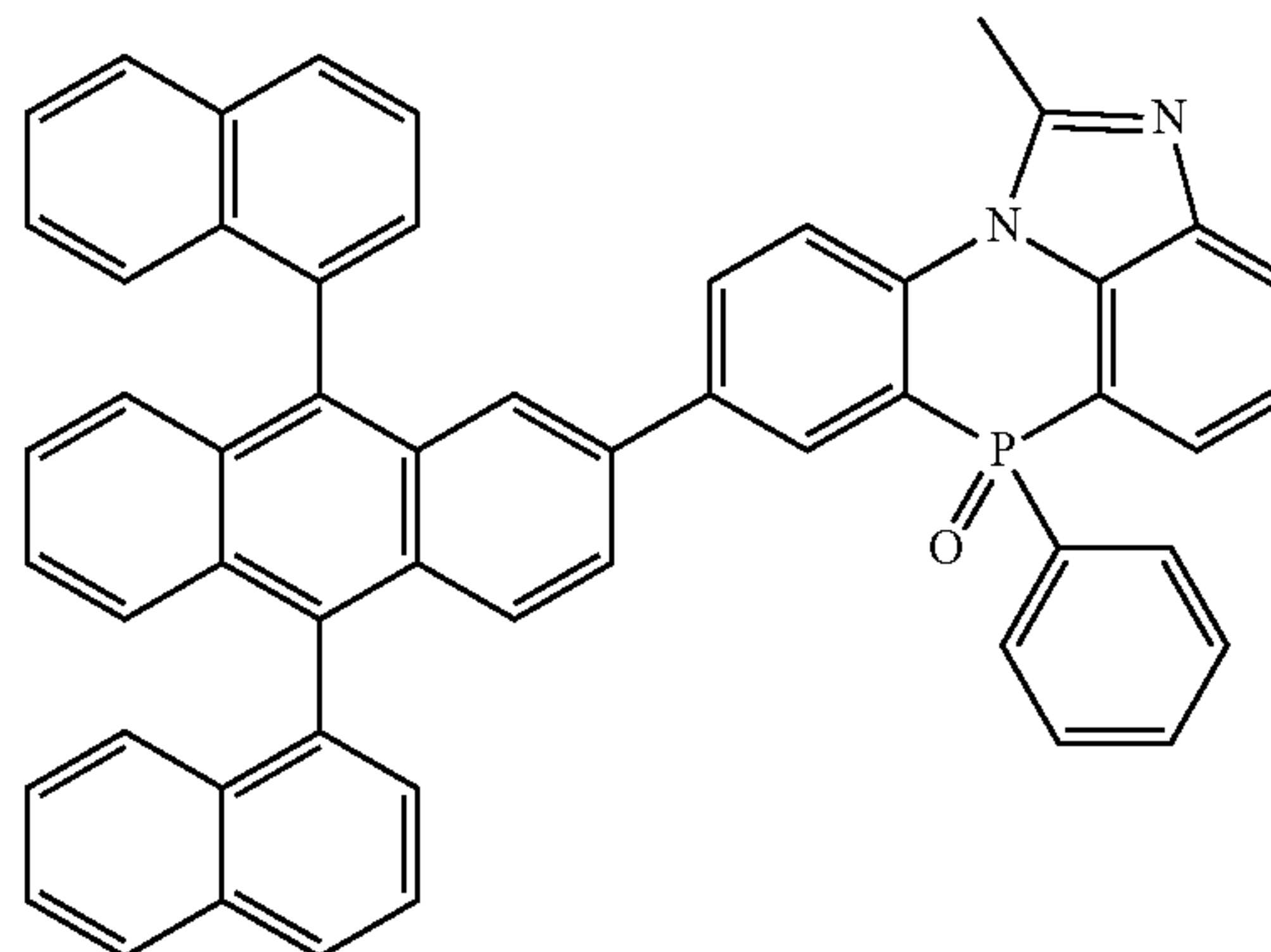
[Chemical Formula 2-2-21]
