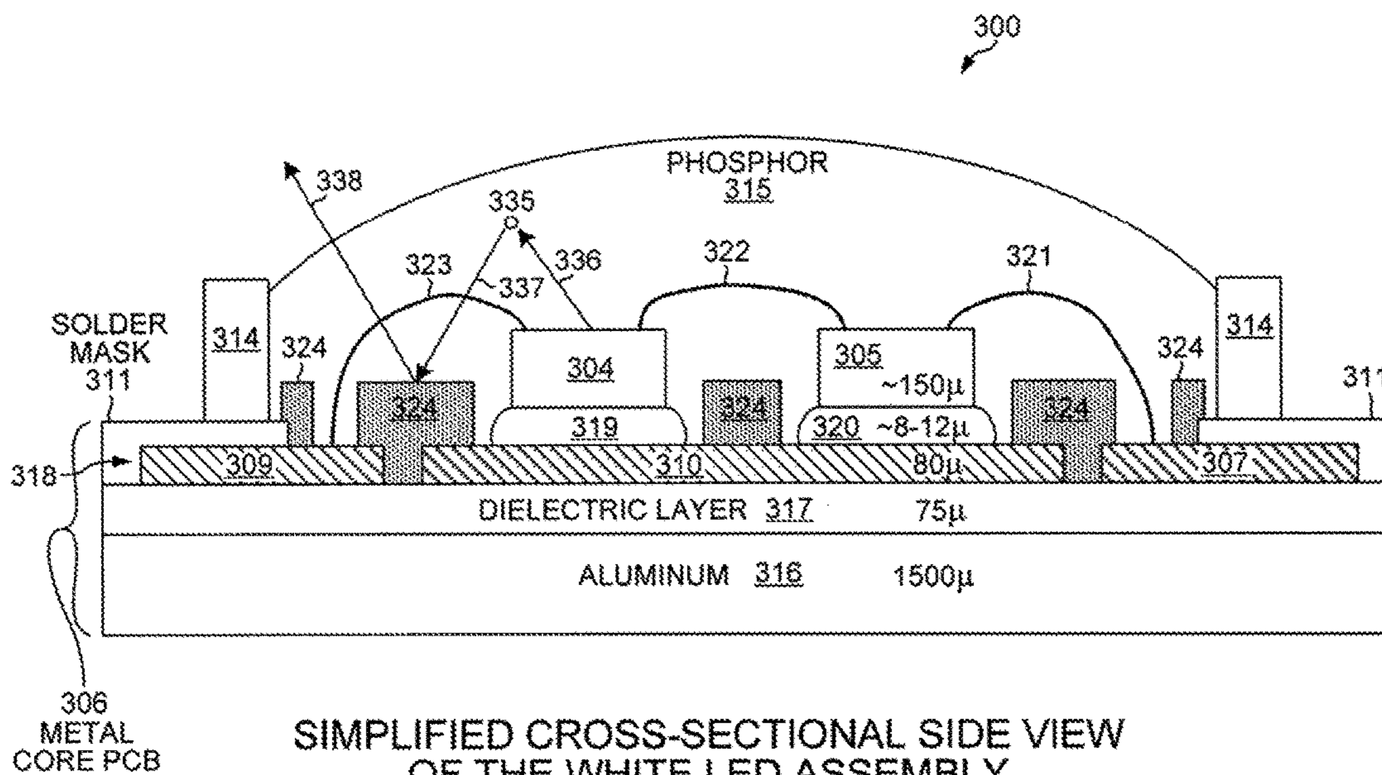
FIG. 40 (PRIOR ART)
