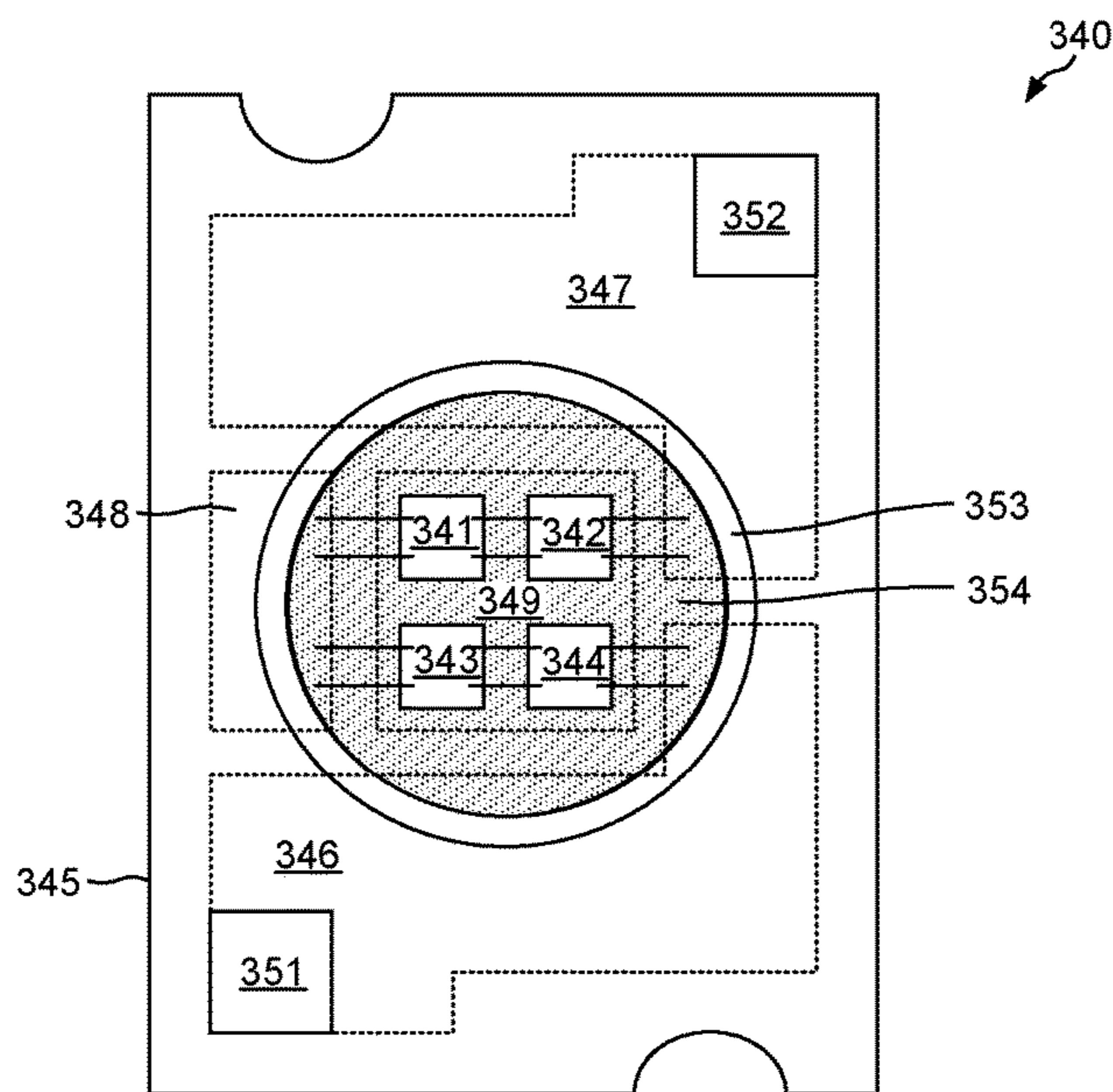
TOP-DOWN VIEW OF A WHITE LED ASSEMBLY
