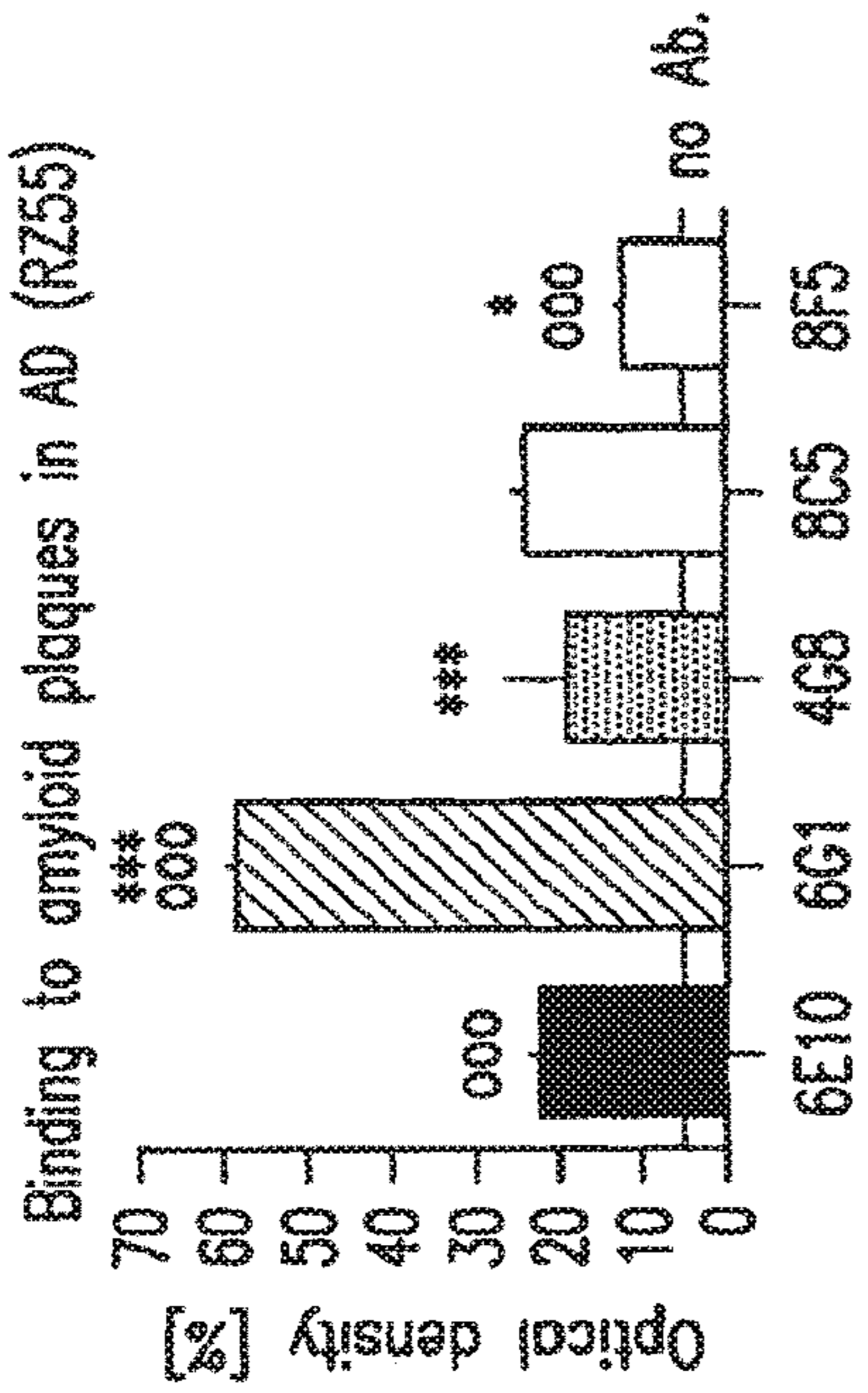
Antibody FIG.7F
