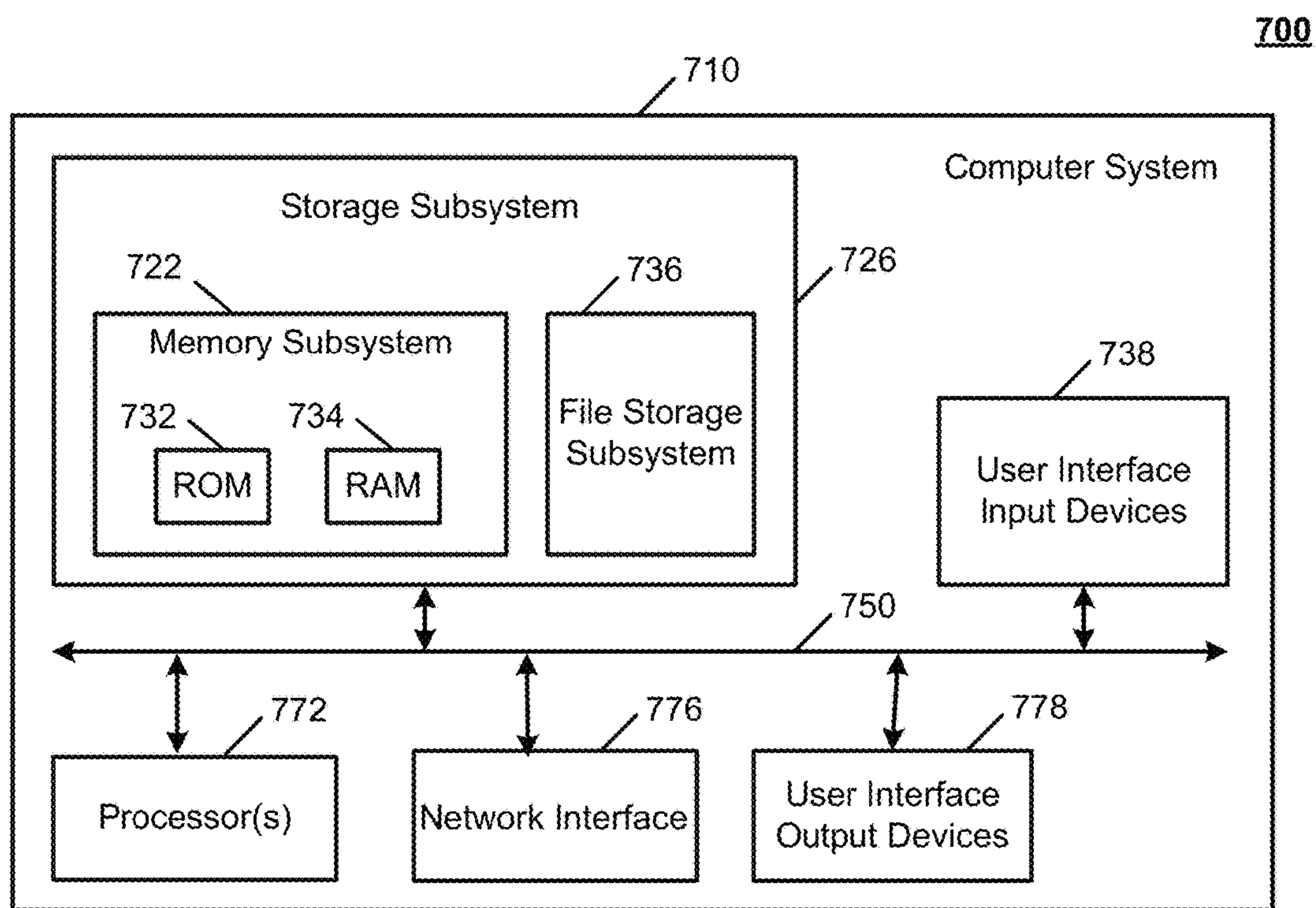
FIG. 7 – Computer System
