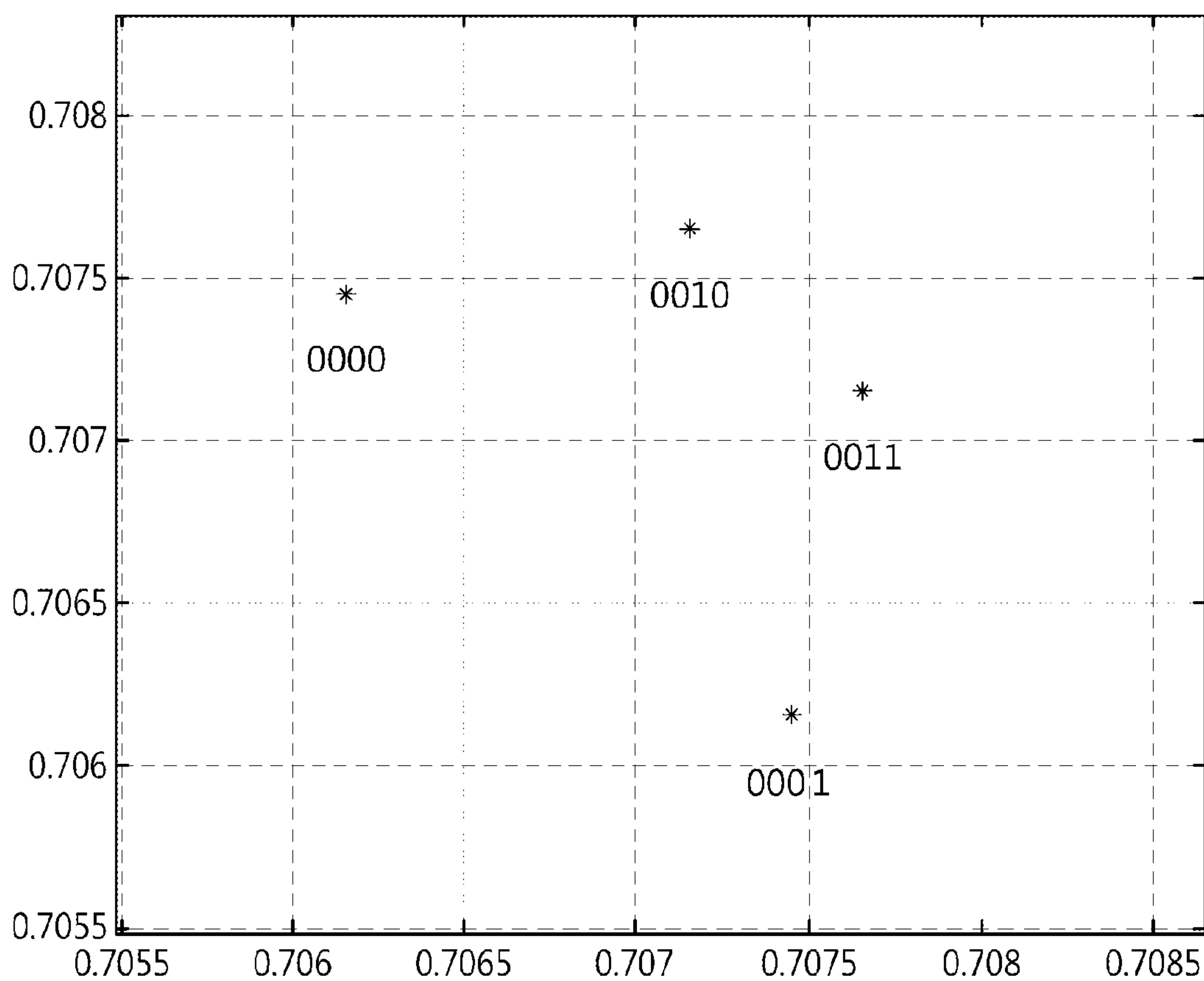
16-NUC for R=2/15 (1st Quadrature)
