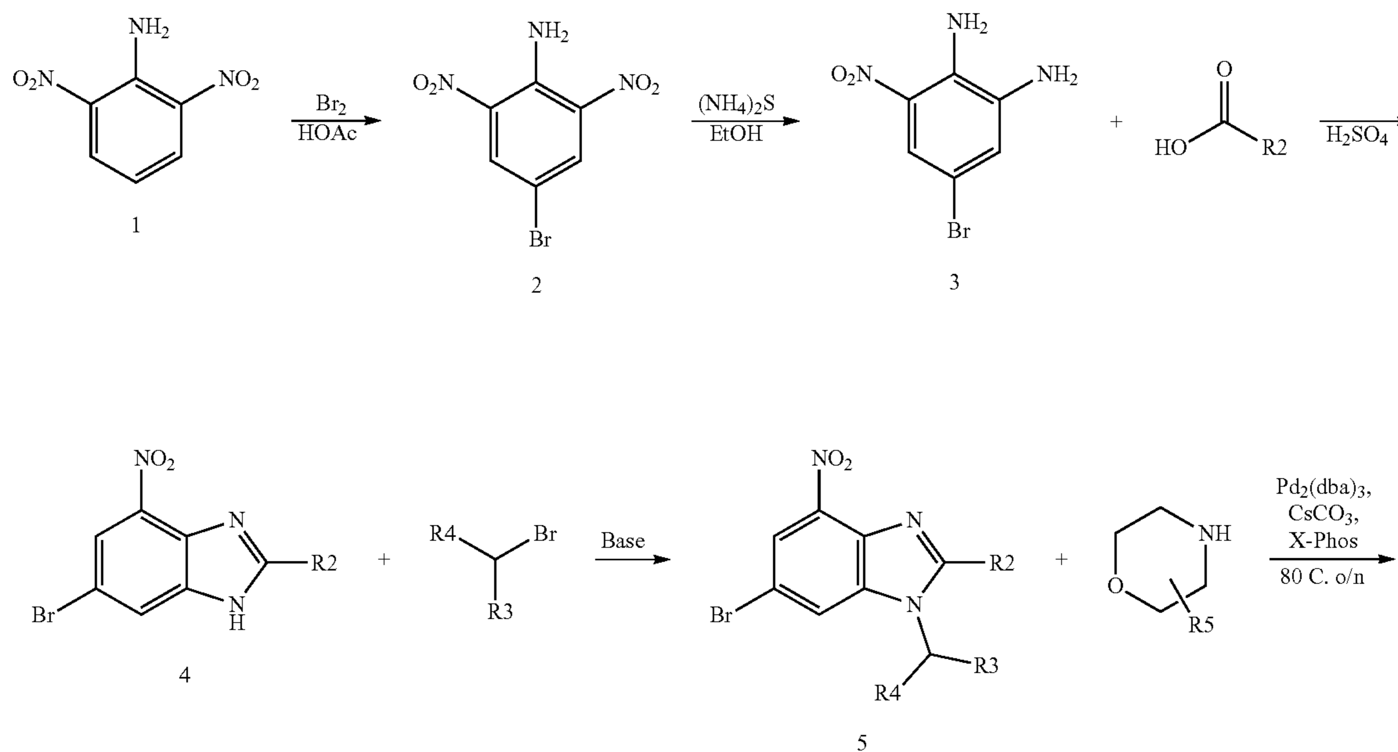
Scheme II
