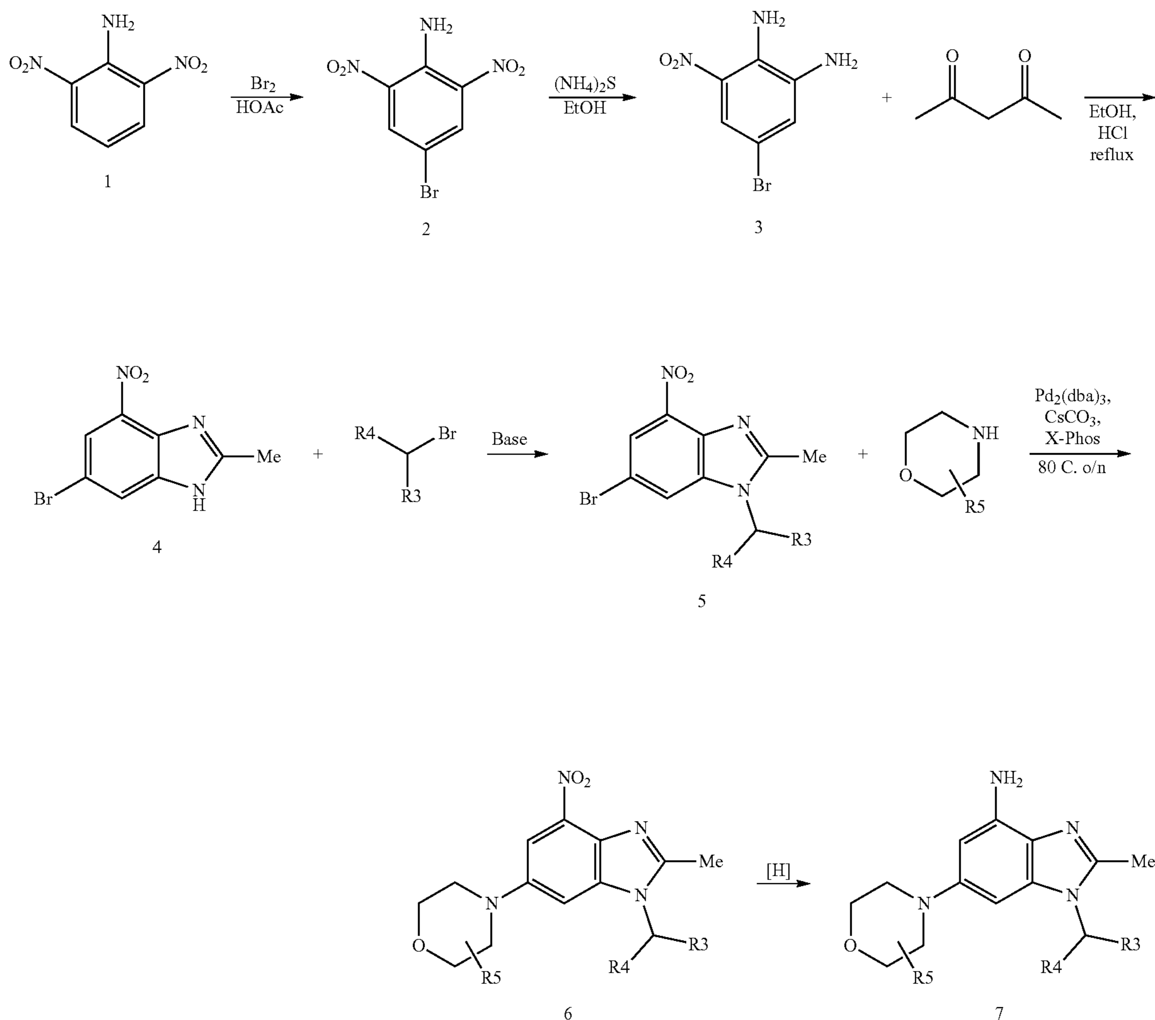
Scheme I (R2 = Me)
