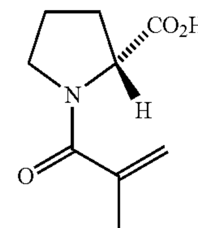
(2R)-1-Methacryloylpyrrolidin-2-carboxylic Acid
