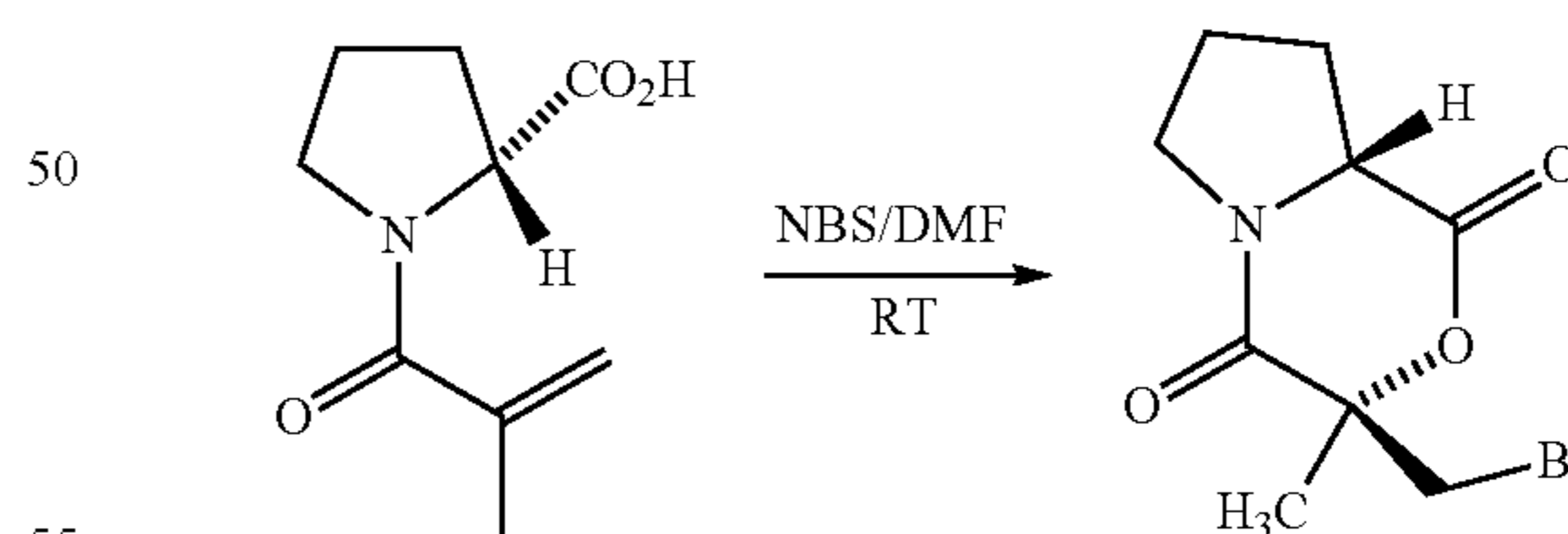
(3R,8aR)-3-Bromomethyl-3-methyl-tetrahydro-pyrrolo[2,1-c][1,4]oxazine-1,4-dione
