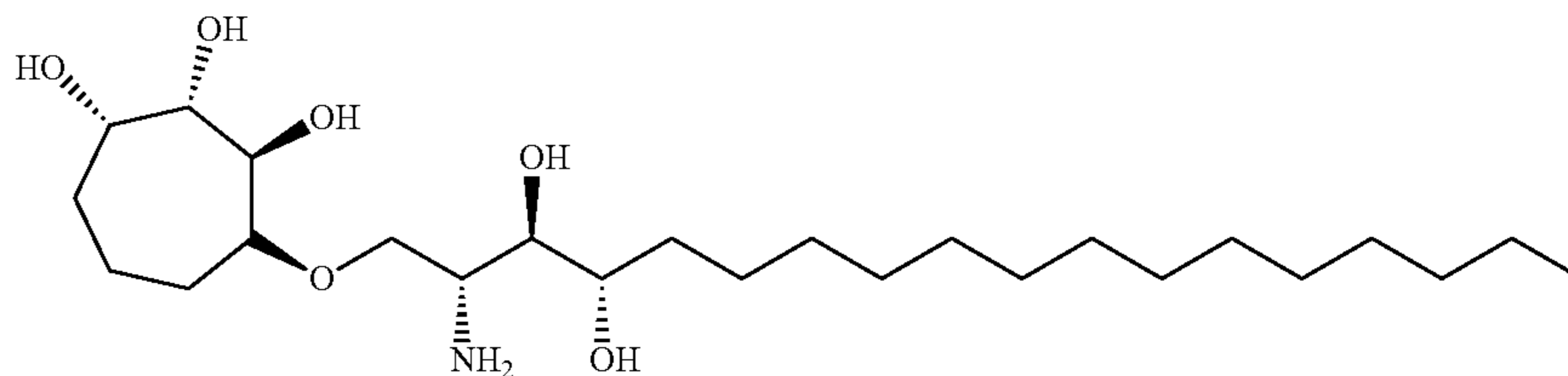
(1S,2S,3R,4R)-4-(((2R,3R,4S)-2-amino-3,4-dihydroxyoctadecyl)oxy) cycloheptane-1,2,3-triol (72)
