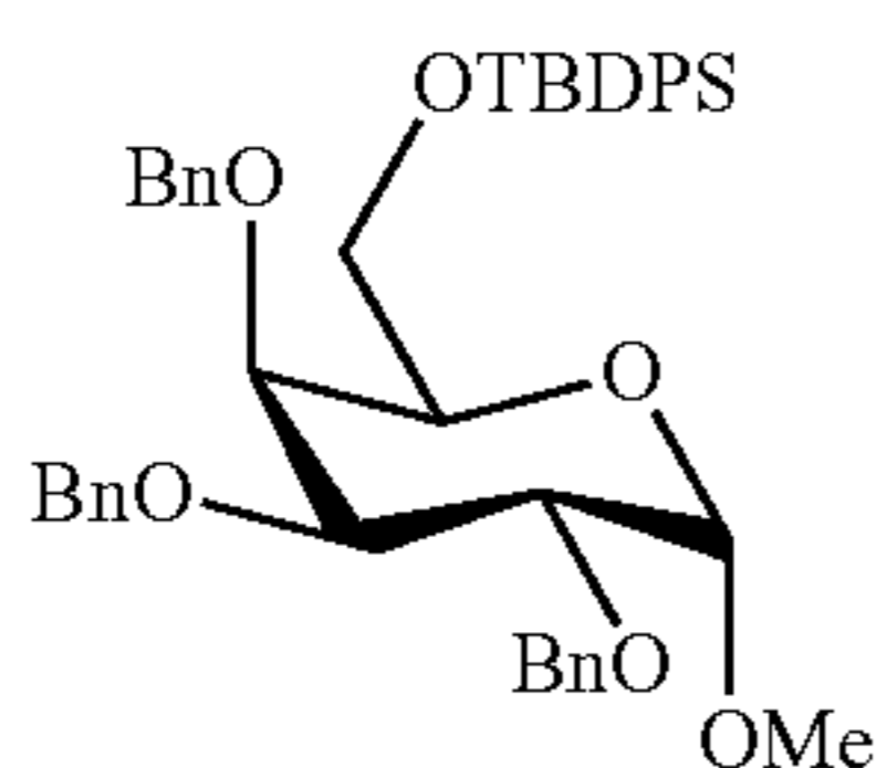
2,3,4-benzyloxy-6-((tert-butyl-diphenylsilyloxy)-methyl)- \alpha -D-galactose (51)
