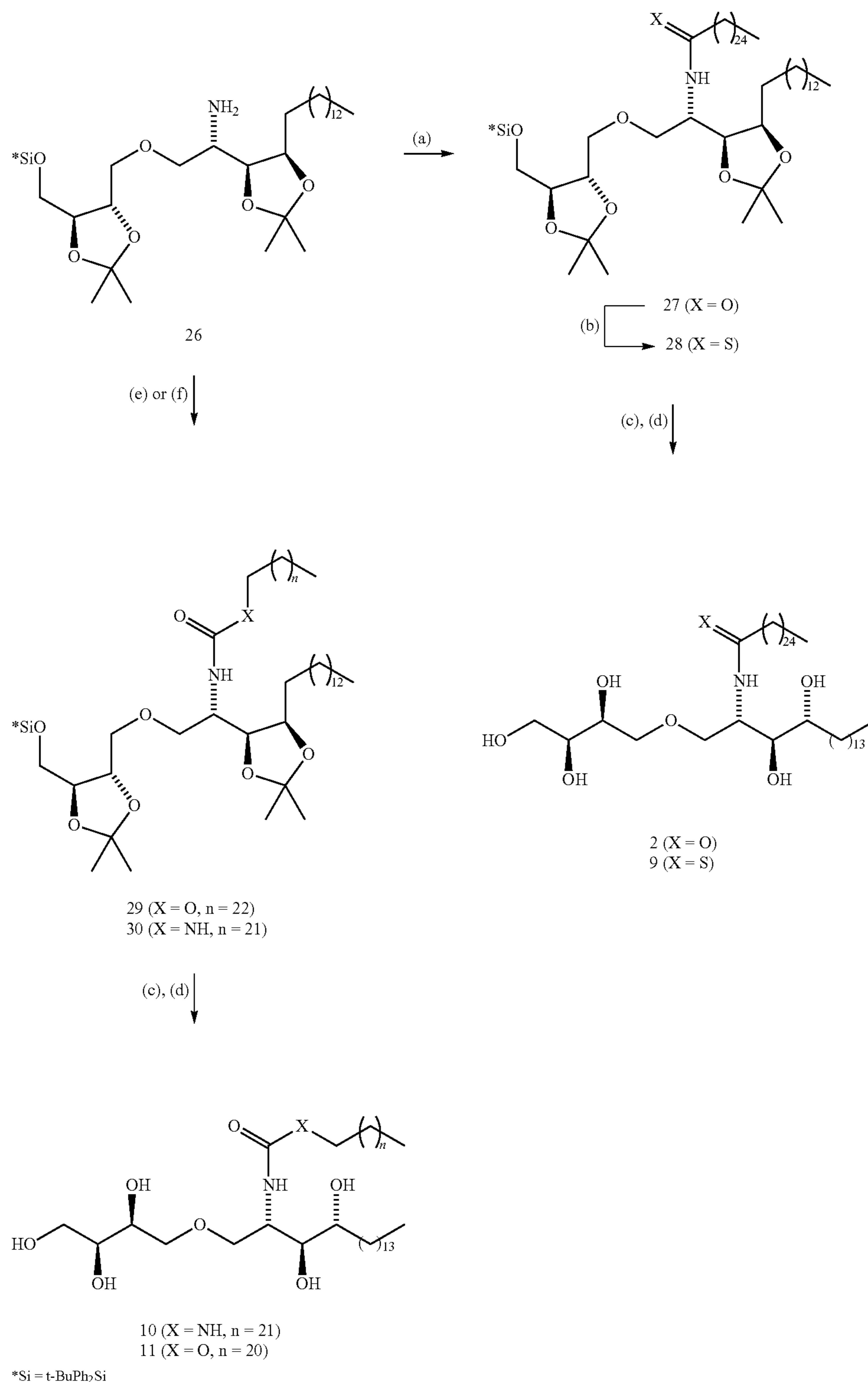
Scheme 3
