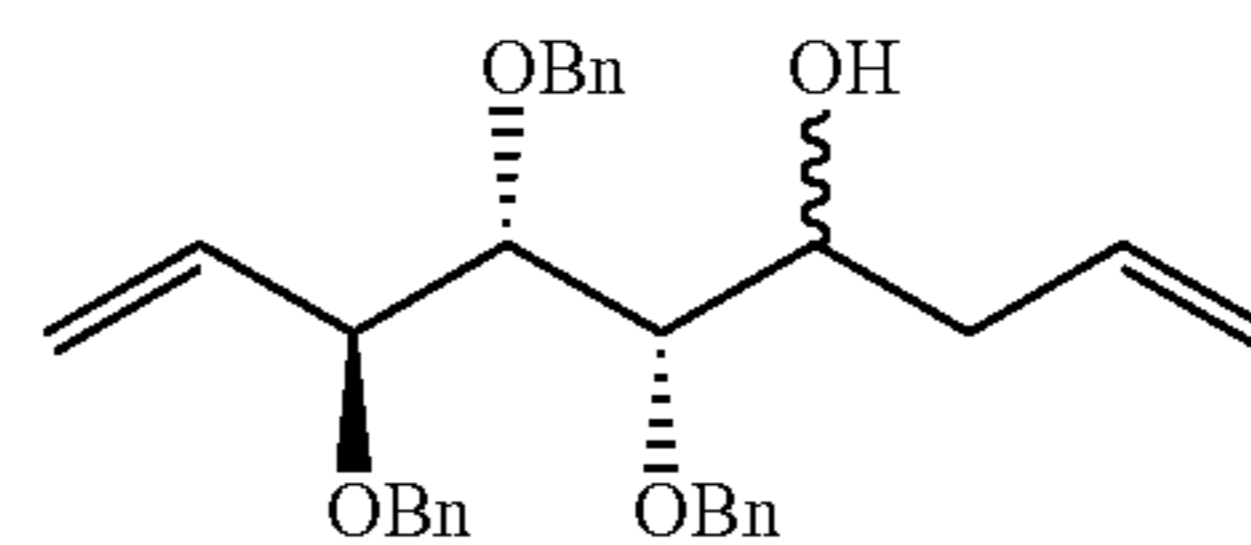
(5S,6S,7S)-5,6,7-tris(benzyloxy)nona-1,8-dien-4-ol (53)
