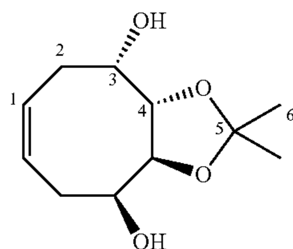
4S,4'S—O-isopropylidene-cyclooct-1-en-4,4'-diol (90)
