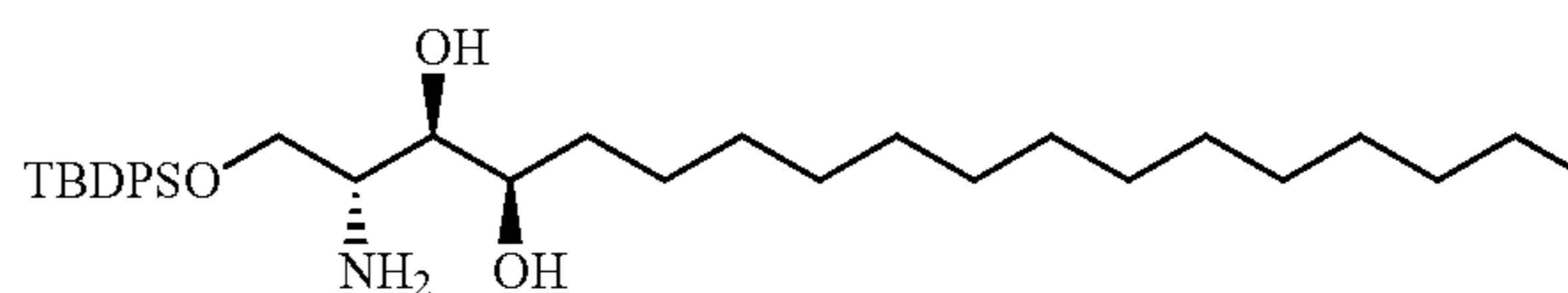
(2R,3R,4R)-2-amino-1-((tert-butyl-diphenylsilyloxy)oxy)octadecane-3,4-diol (64)
