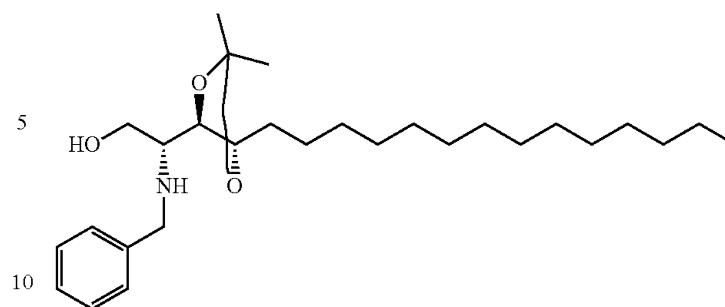
2R—N-benzyl-(3R,4R—O-isopropylidene) octadecan-1-ol (68)
