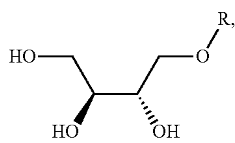
ThrCer
