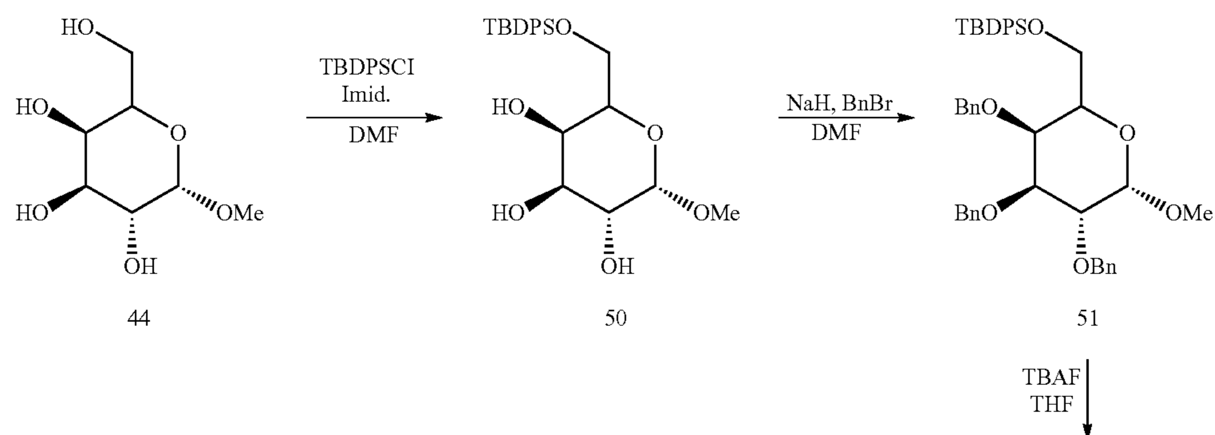
Scheme 5
