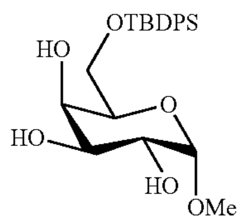
6-((tert-butyl-diphenylsilyloxy)-methyl)- \alpha -D-galactose (50)
