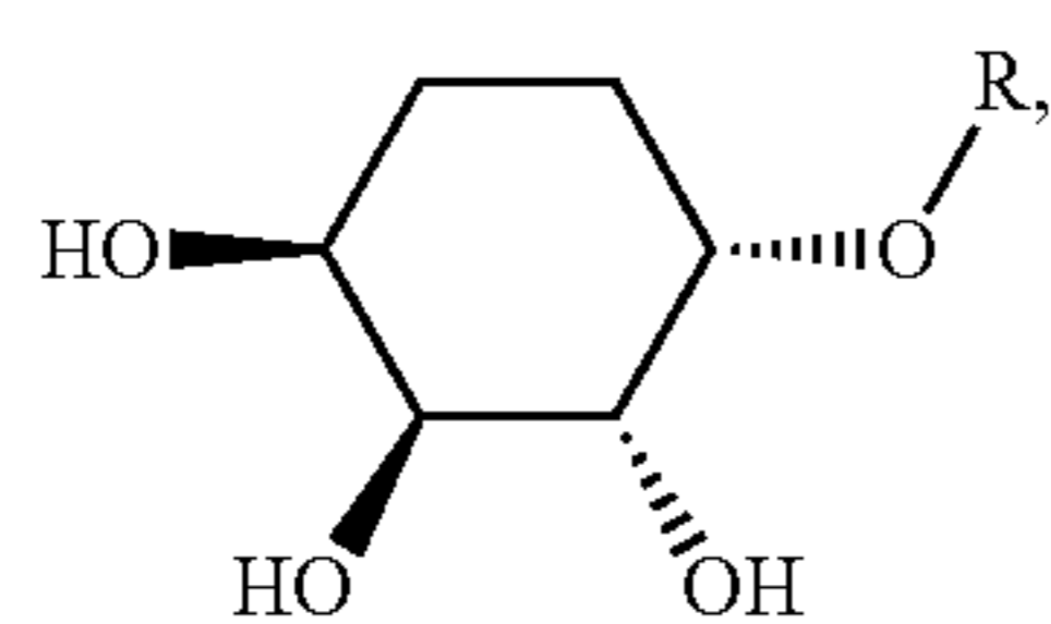
ThrCer 6
