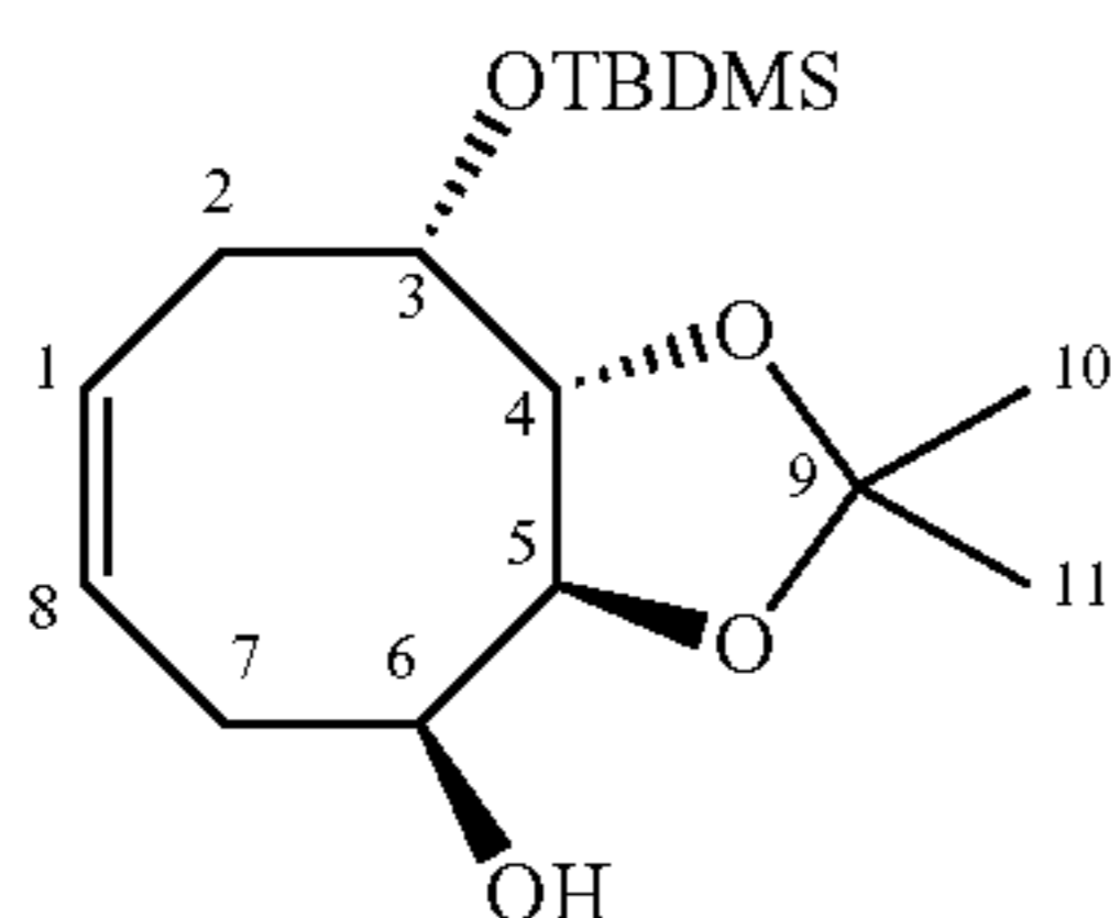
6-(tert-butyldimethylsilyloxy)-7S,8S—O-isopropylidene-cyclooct-3-en-1-ol (91)
