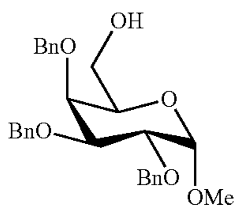
2,3,4-tribenzyloxy-methyl- \alpha -D-galactose (52)
