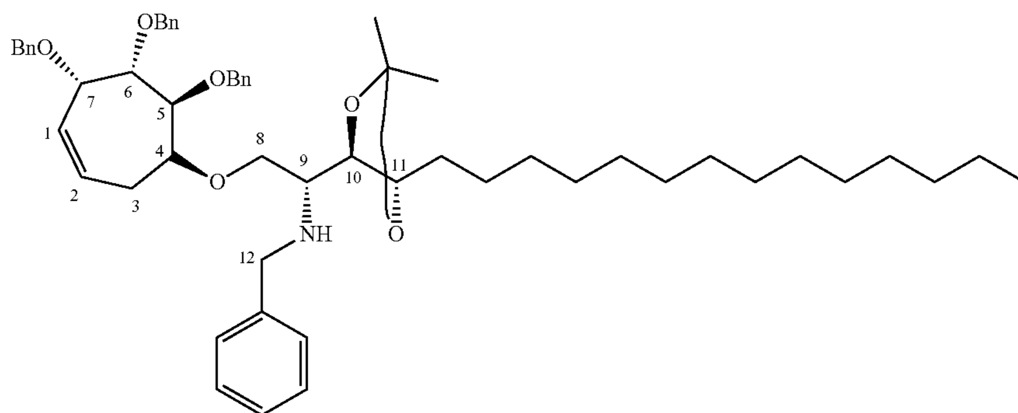
(R)—N-benzyl-1-(((4R,5S)-2,2-dimethyl-5-tetradecyl-1,3-dioxolan-4-yl)-2-(((1R,5S,6S,7S)-5,6,7-tris(benzyloxy)cyclohept-3-en-1-yl)oxy)ethanamine (71)
