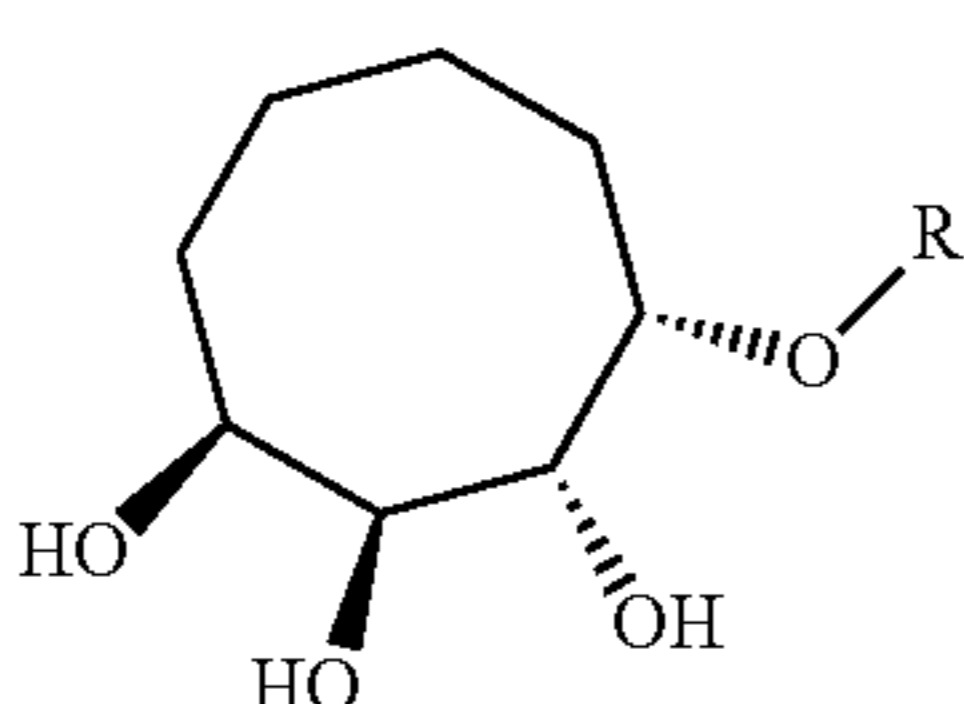
ThrCer 8
