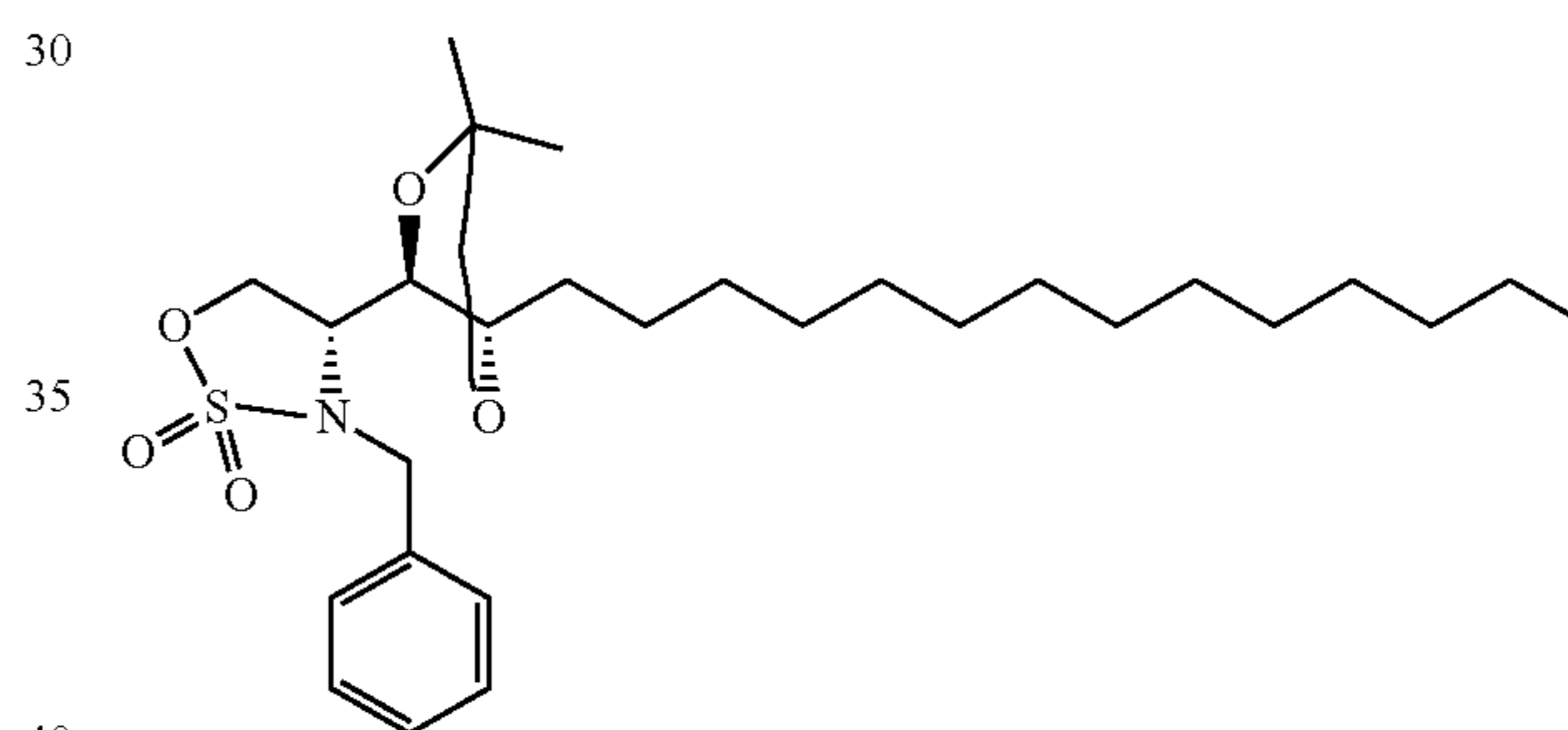
(R)-3-benzyl-4-((4R,5R)-2,2-dimethyl-5-tetradecyl-1,3-dioxolan-4-yl)-1,2,3-oxathiazolidine 2,2-dioxide (70)
