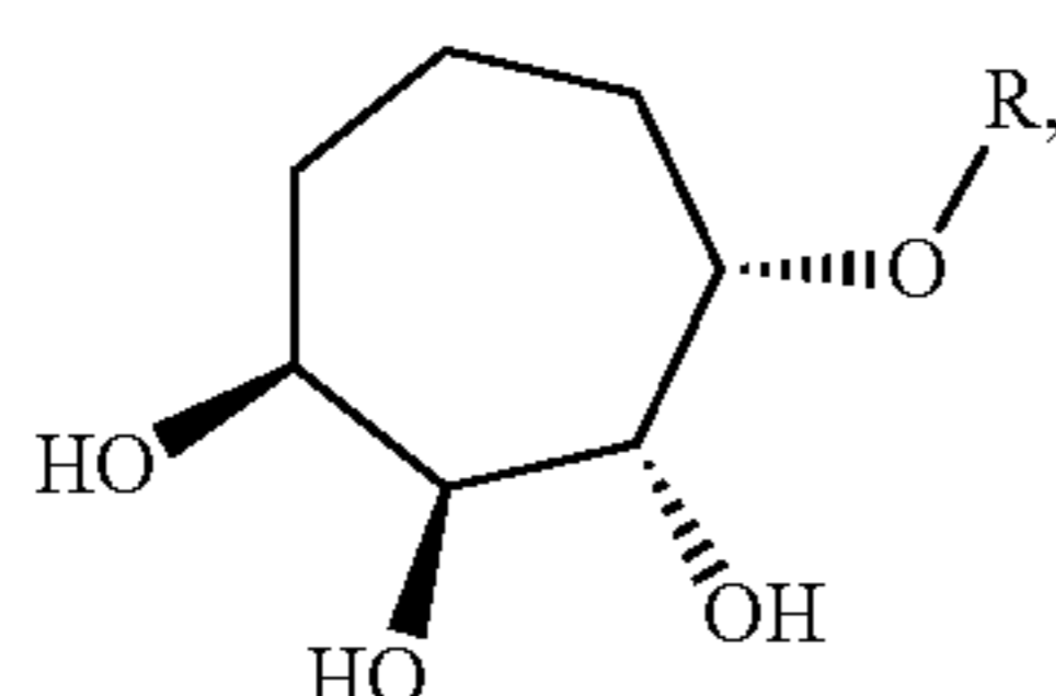
ThrCer 7
