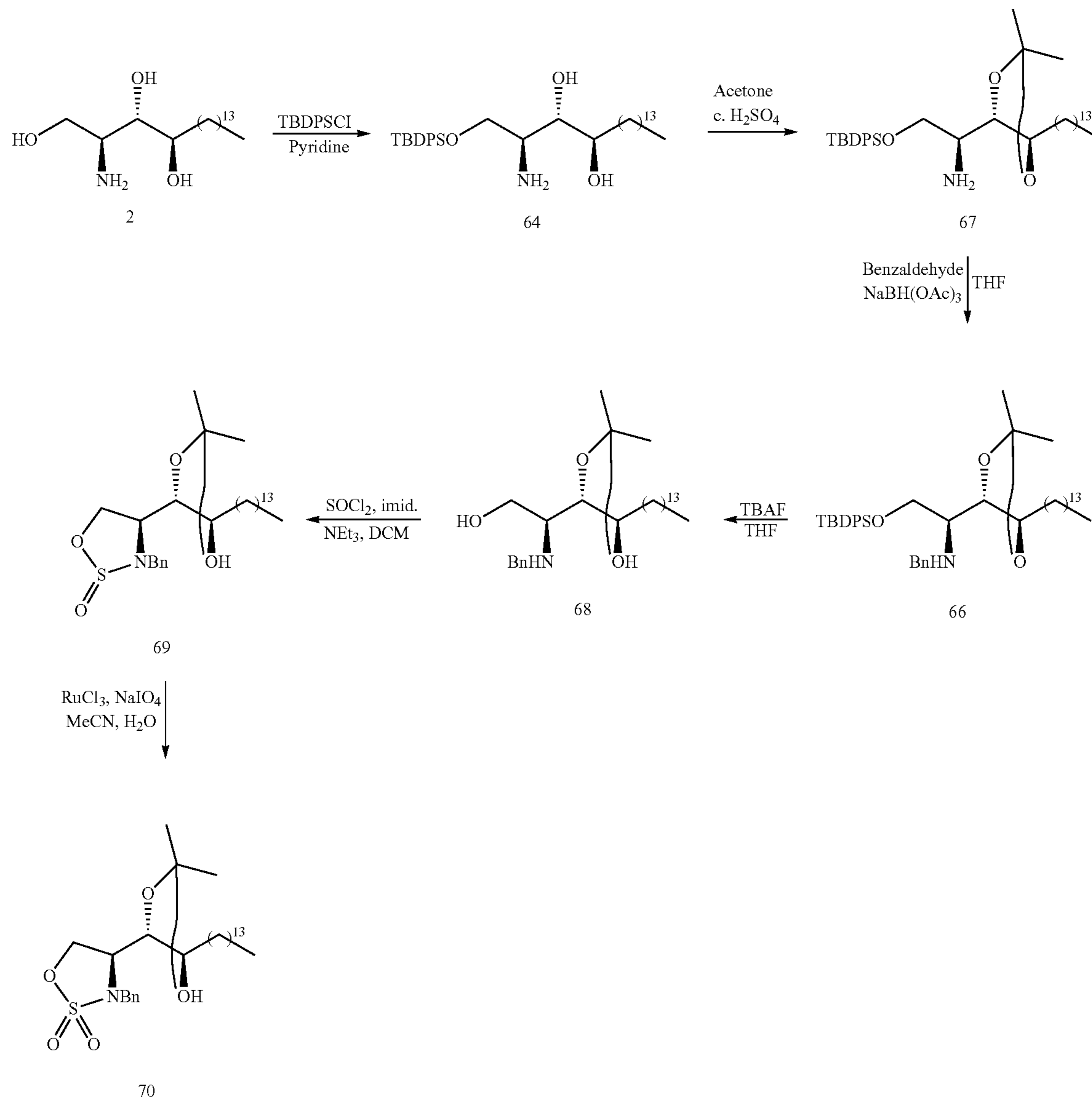
Scheme 4
