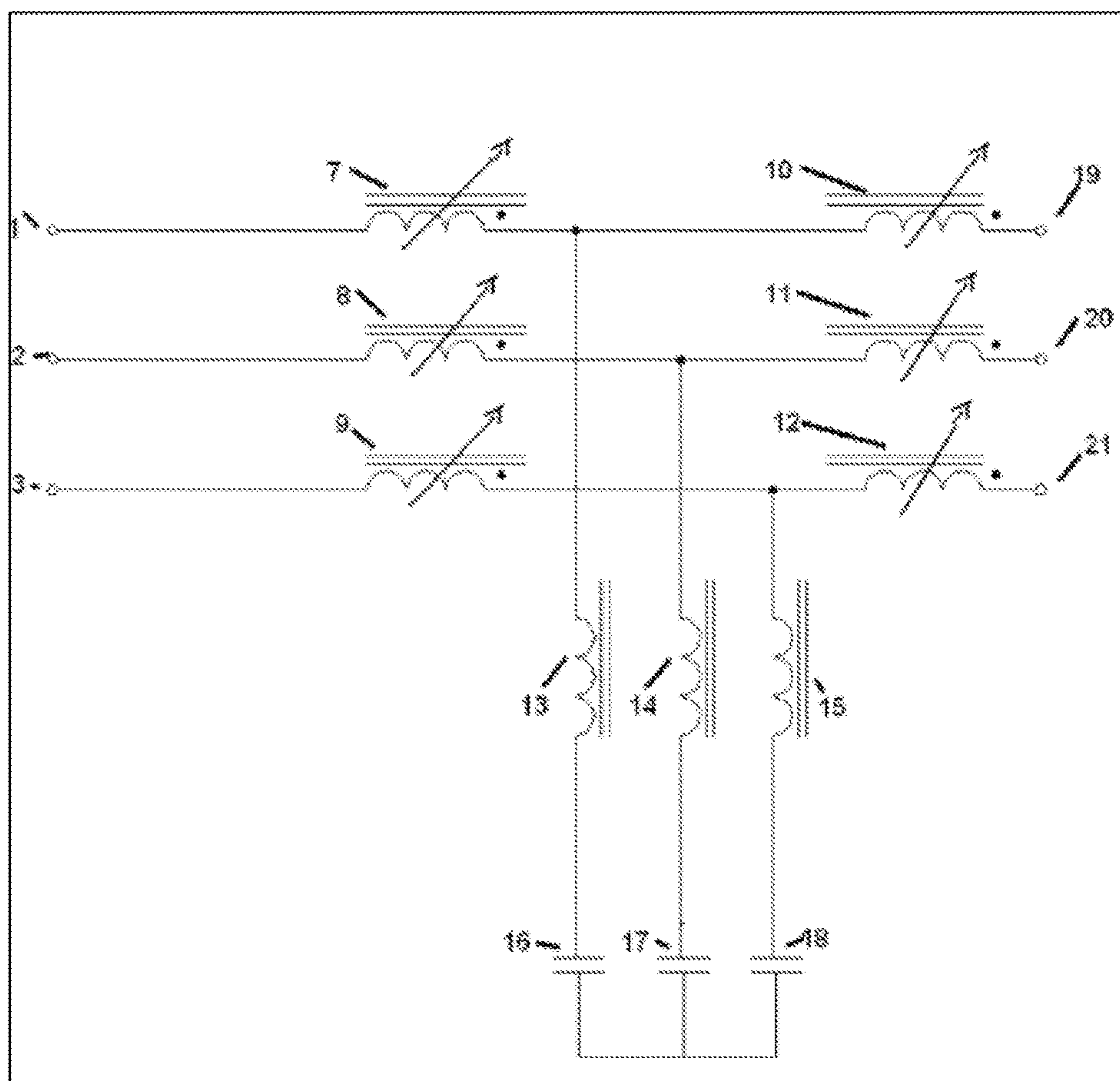
FIG. 3 (prior art)
