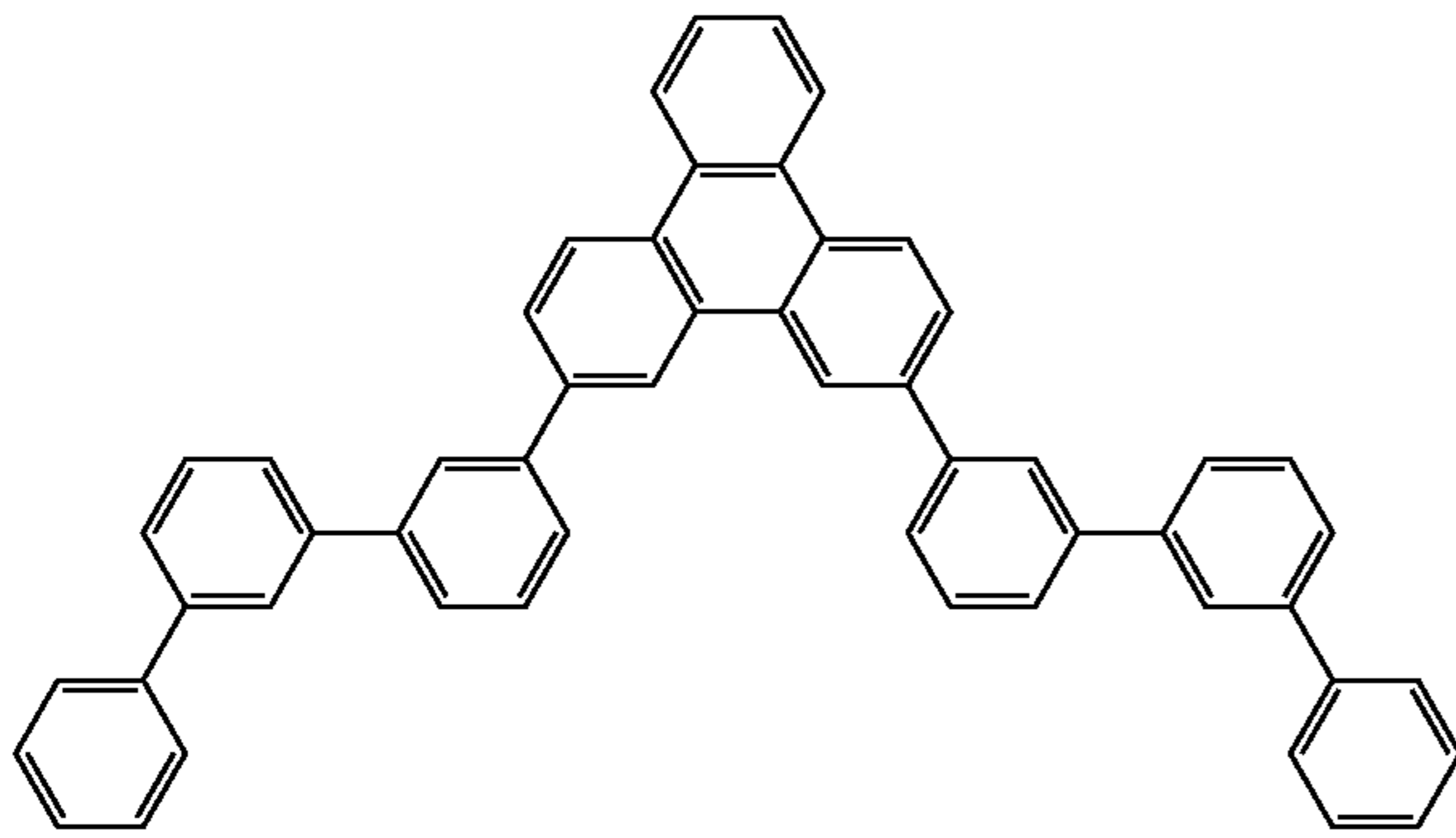
Compound 8
