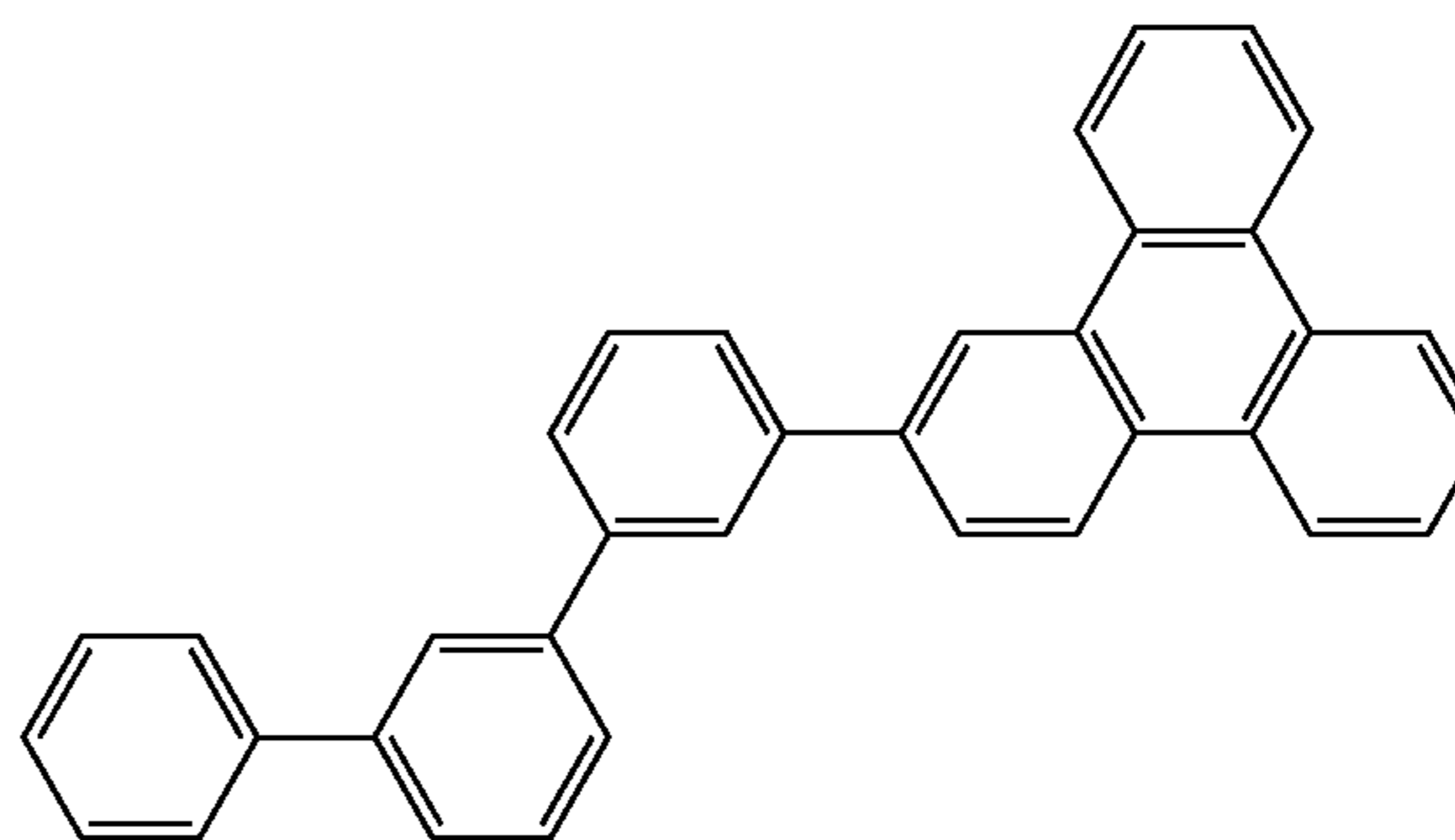
Compound 4
