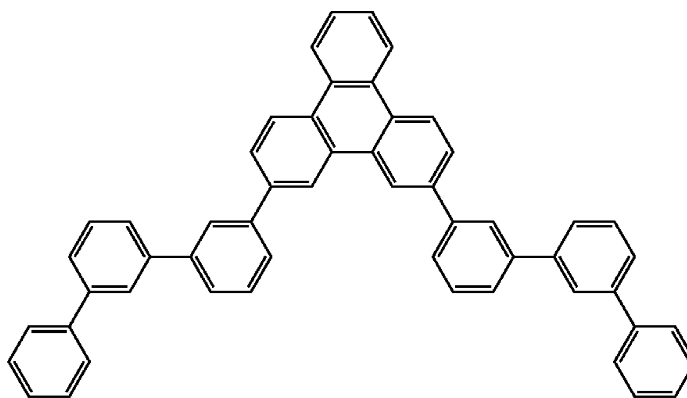
Compound 8
