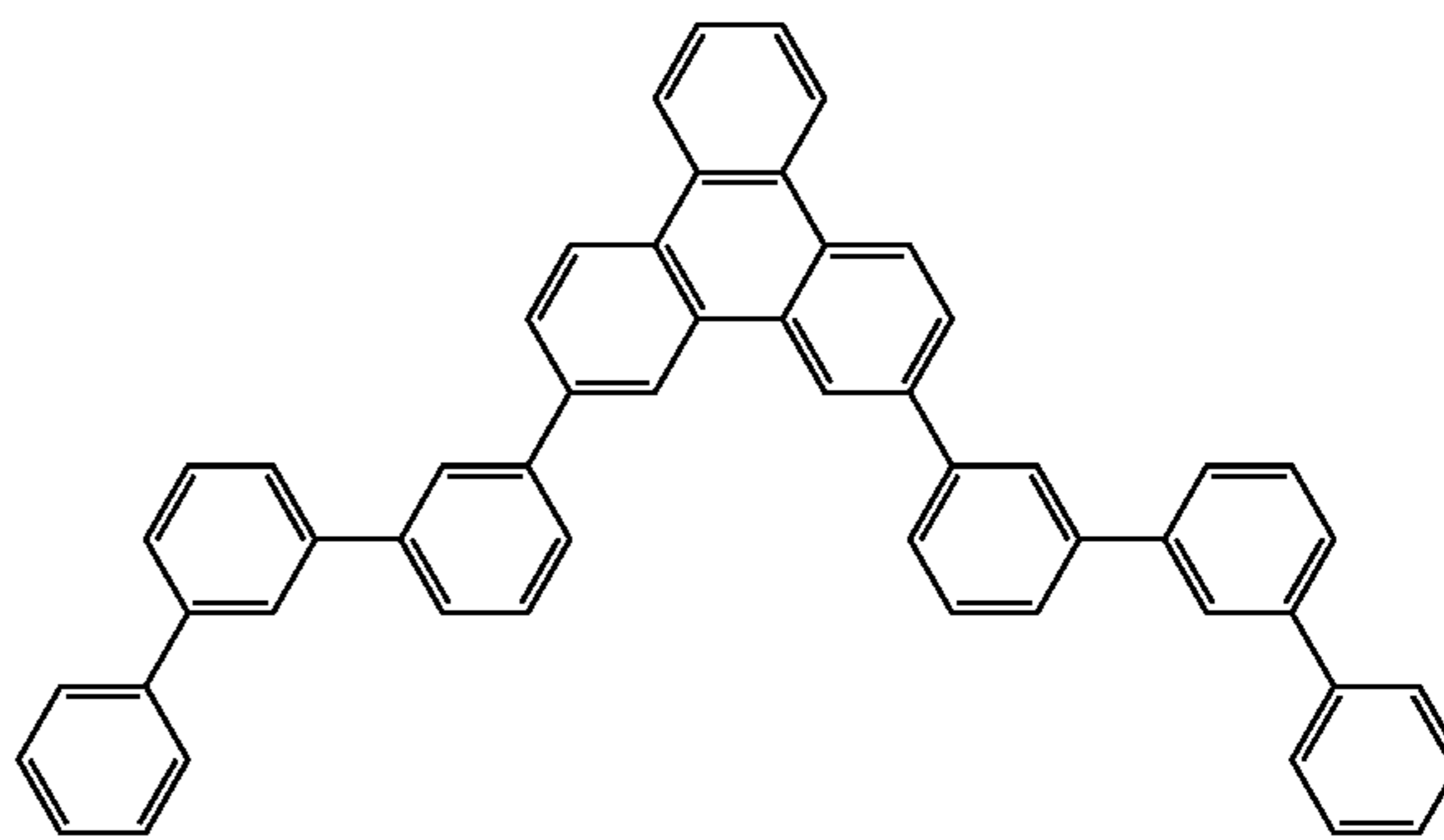
Compound 8
