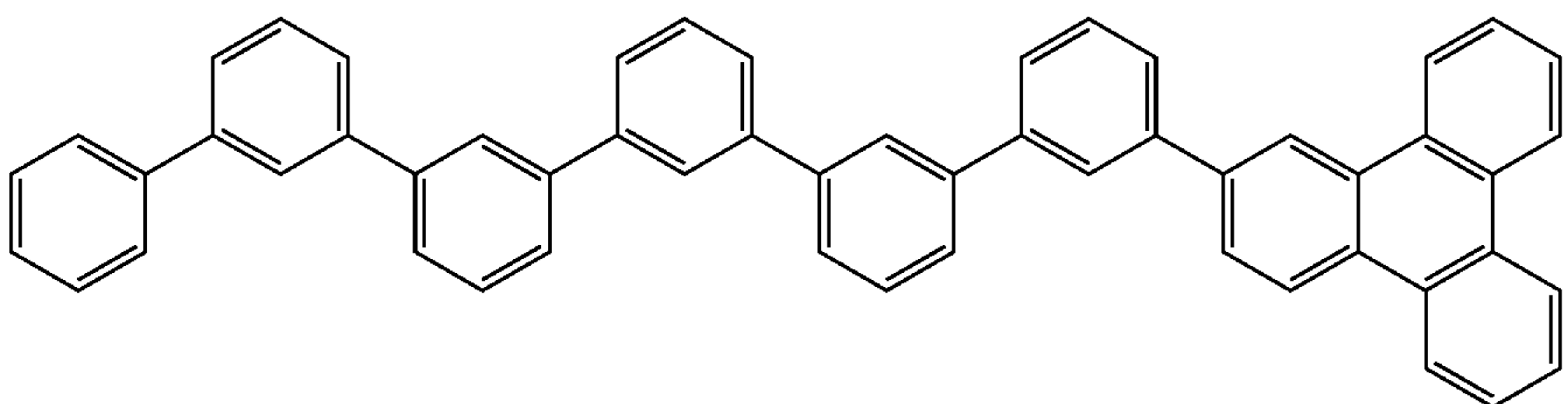
Compound 6
