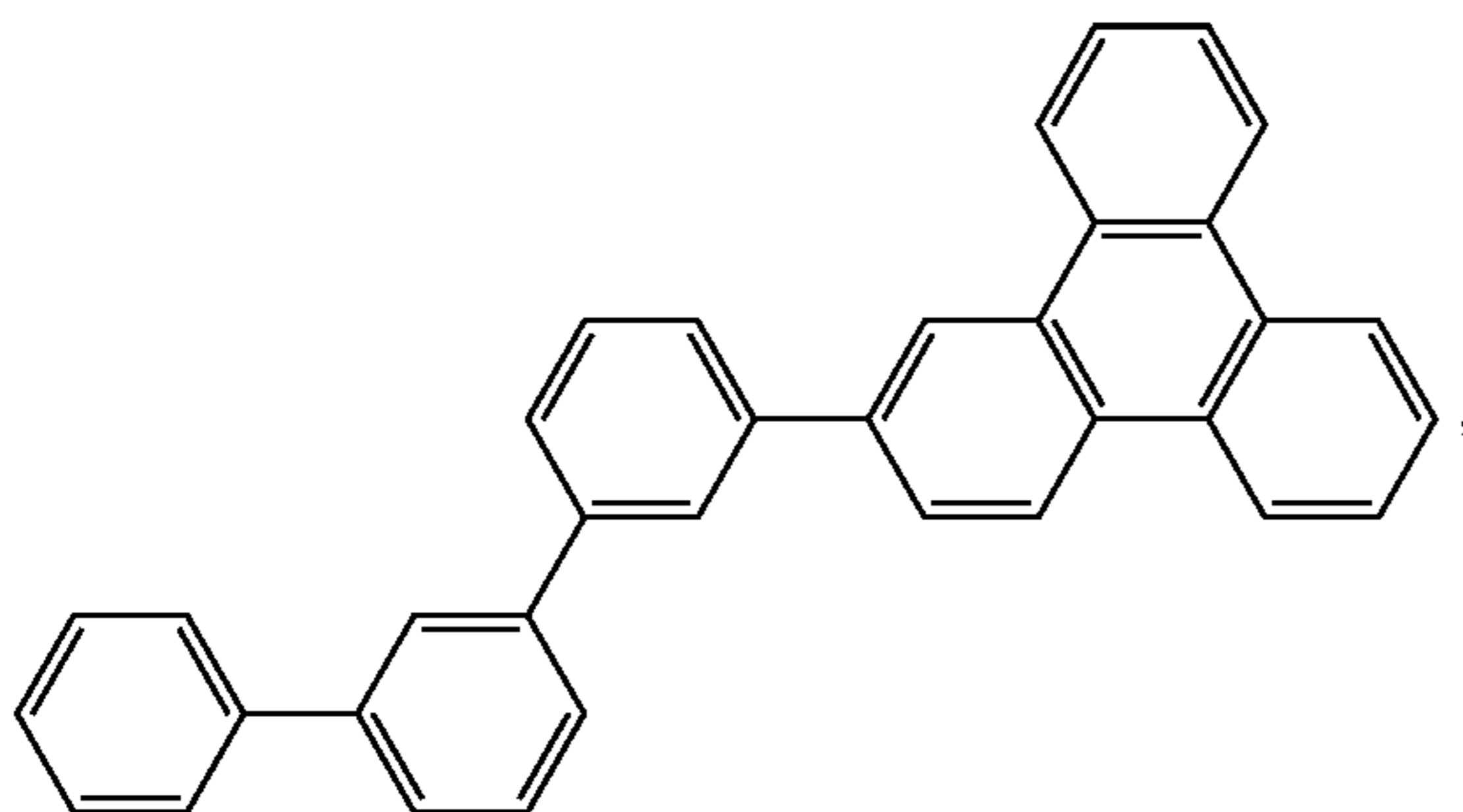
Compound 2
