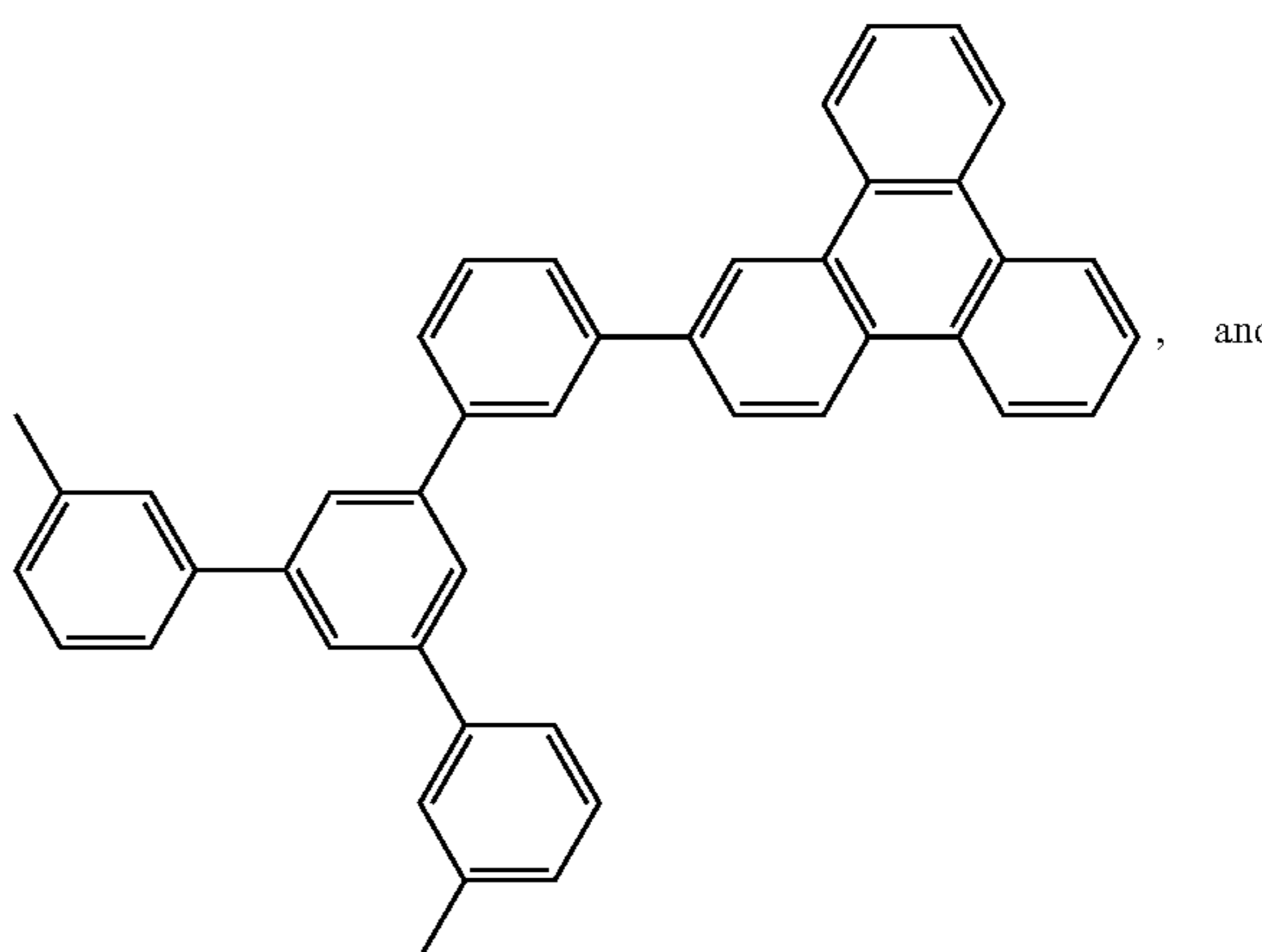
Compound 10
