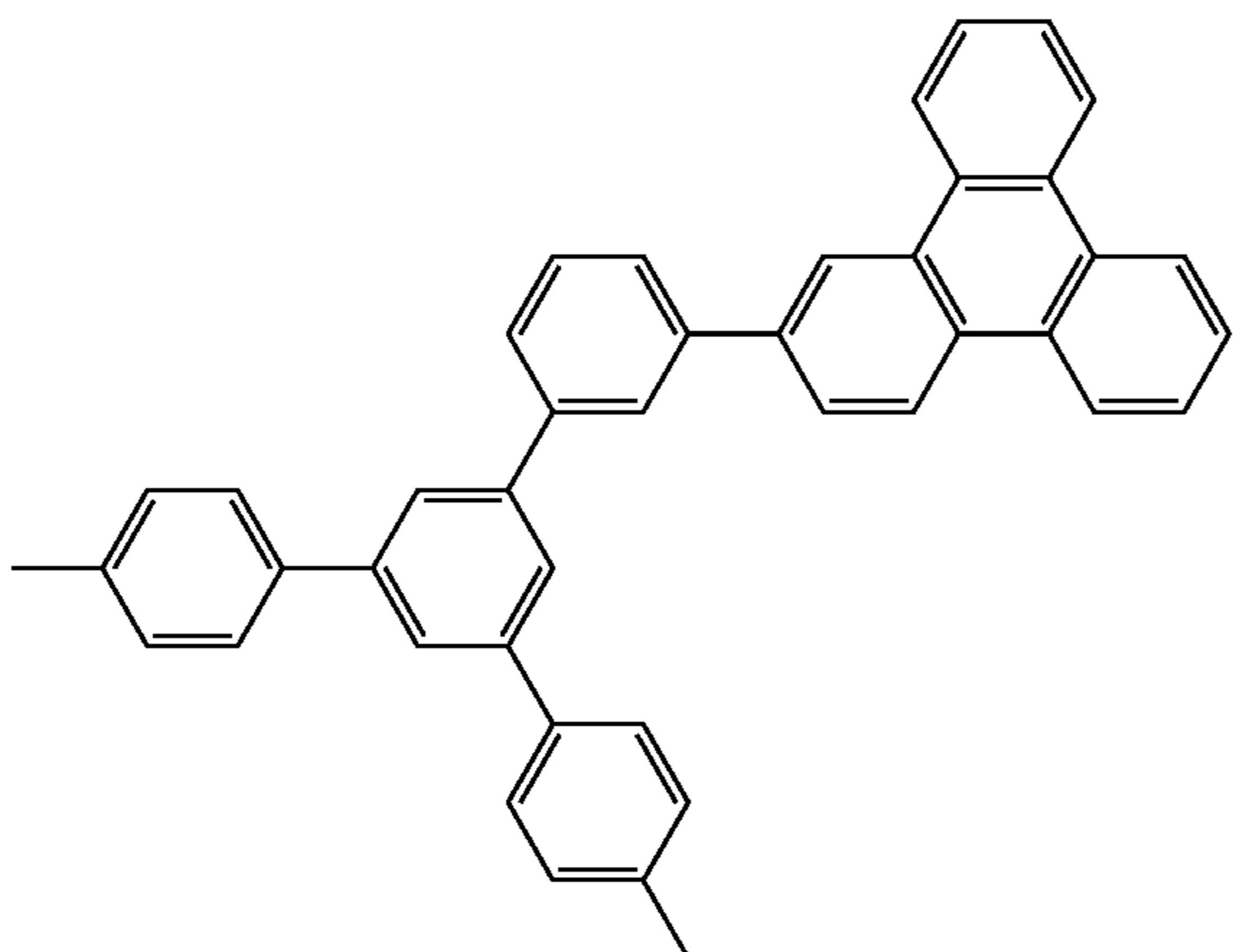
Compound 9
