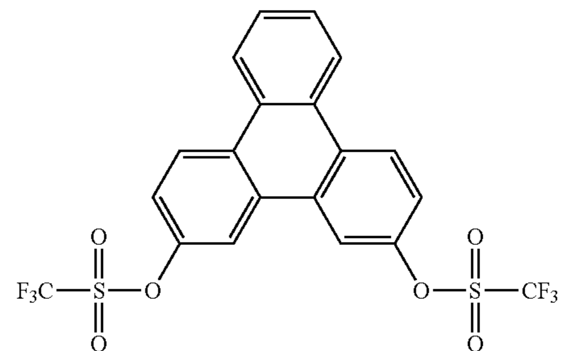
Triphenylene-2,11-dyl bis(trifluoromethanesulfonate)
