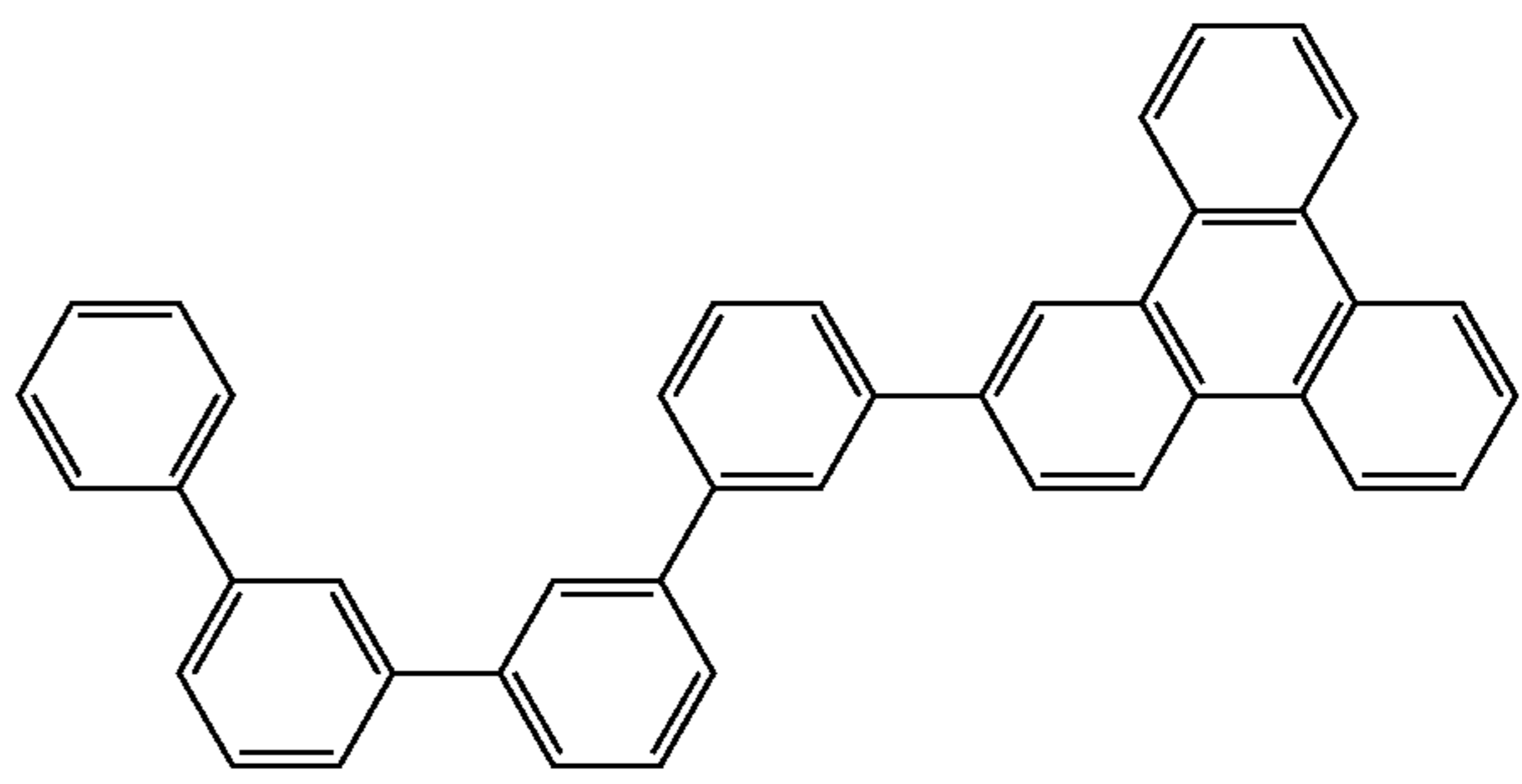
Compound 5
