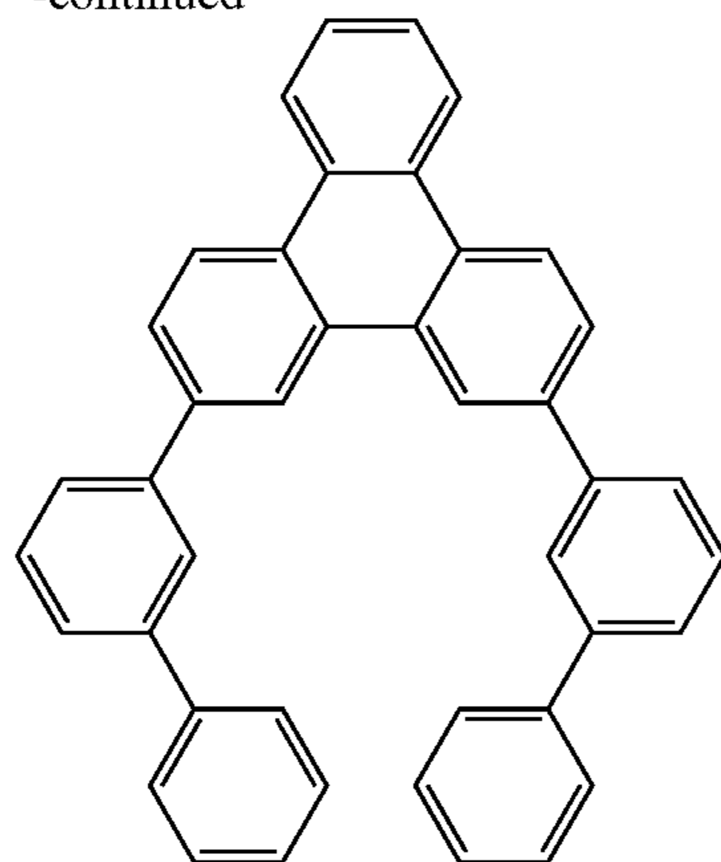
Compound 12
