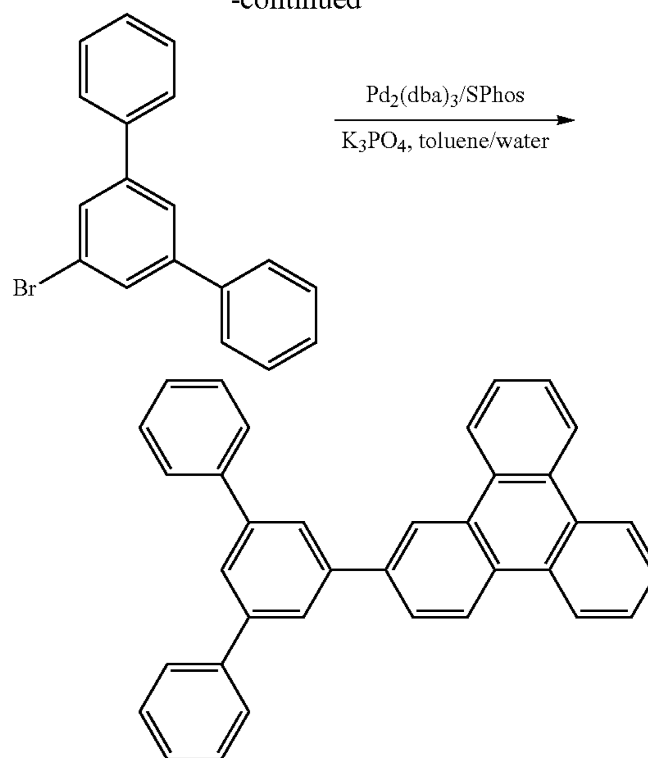
Compound 1
