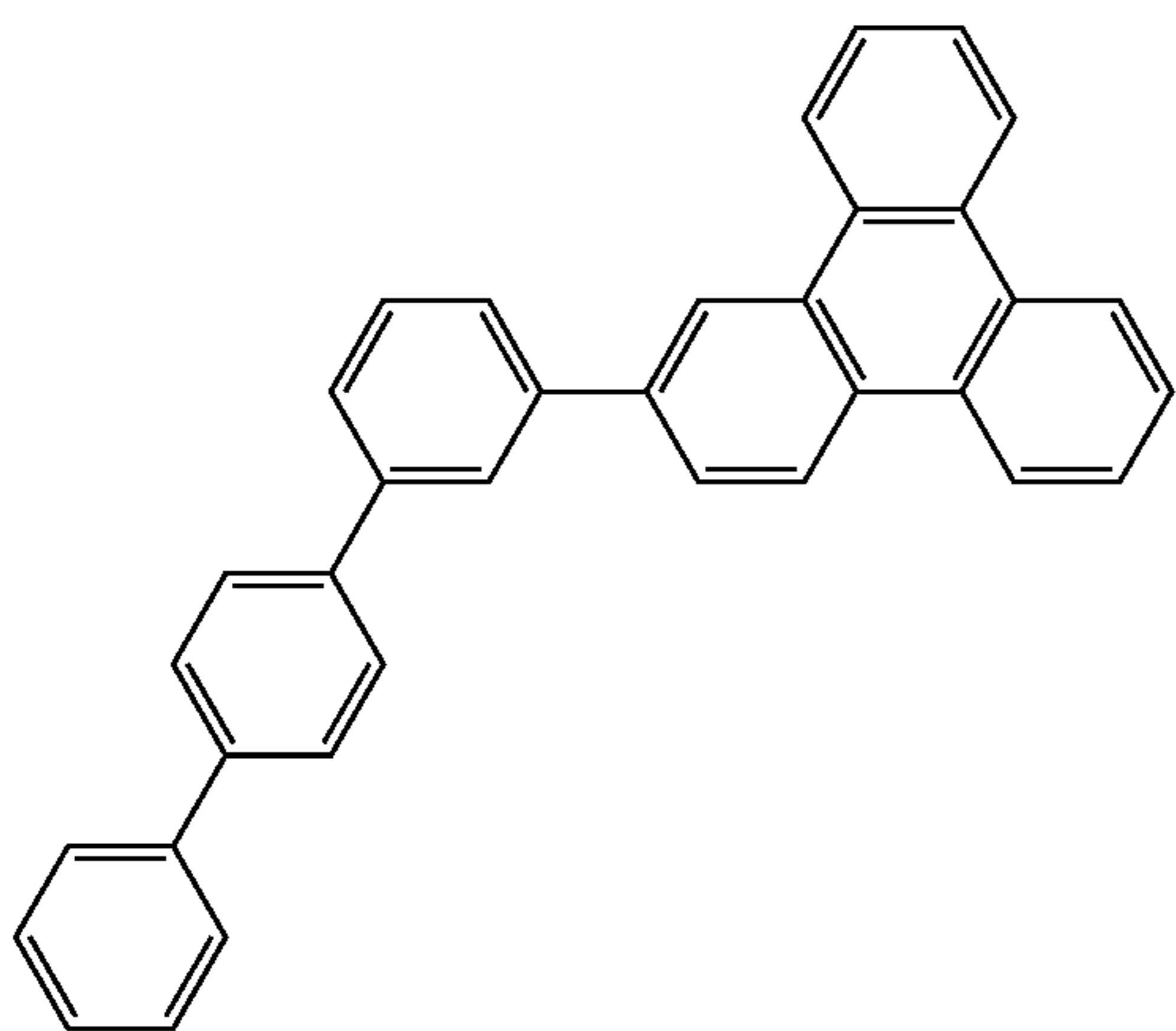
Compound 6
