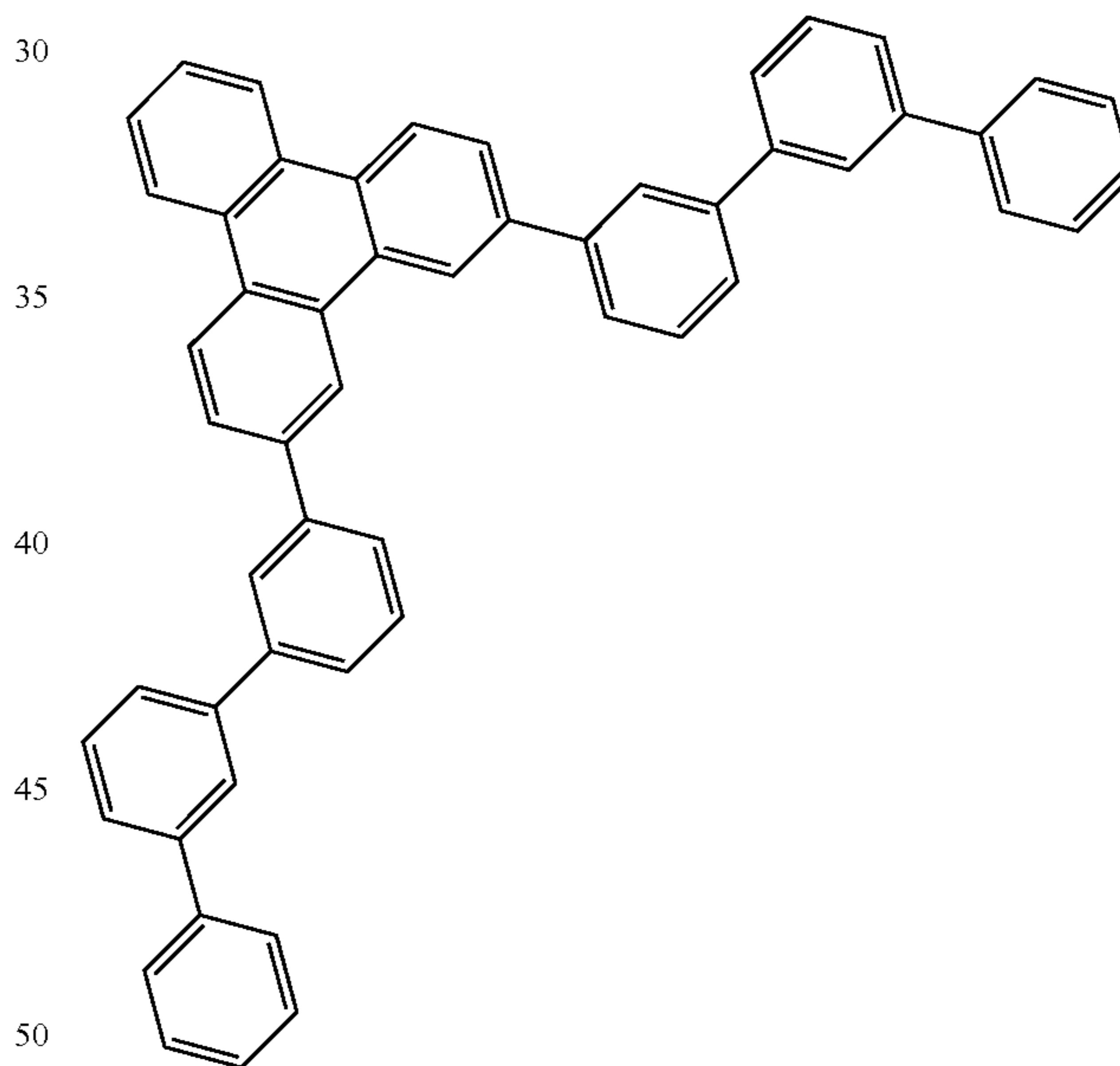
Compound 8
