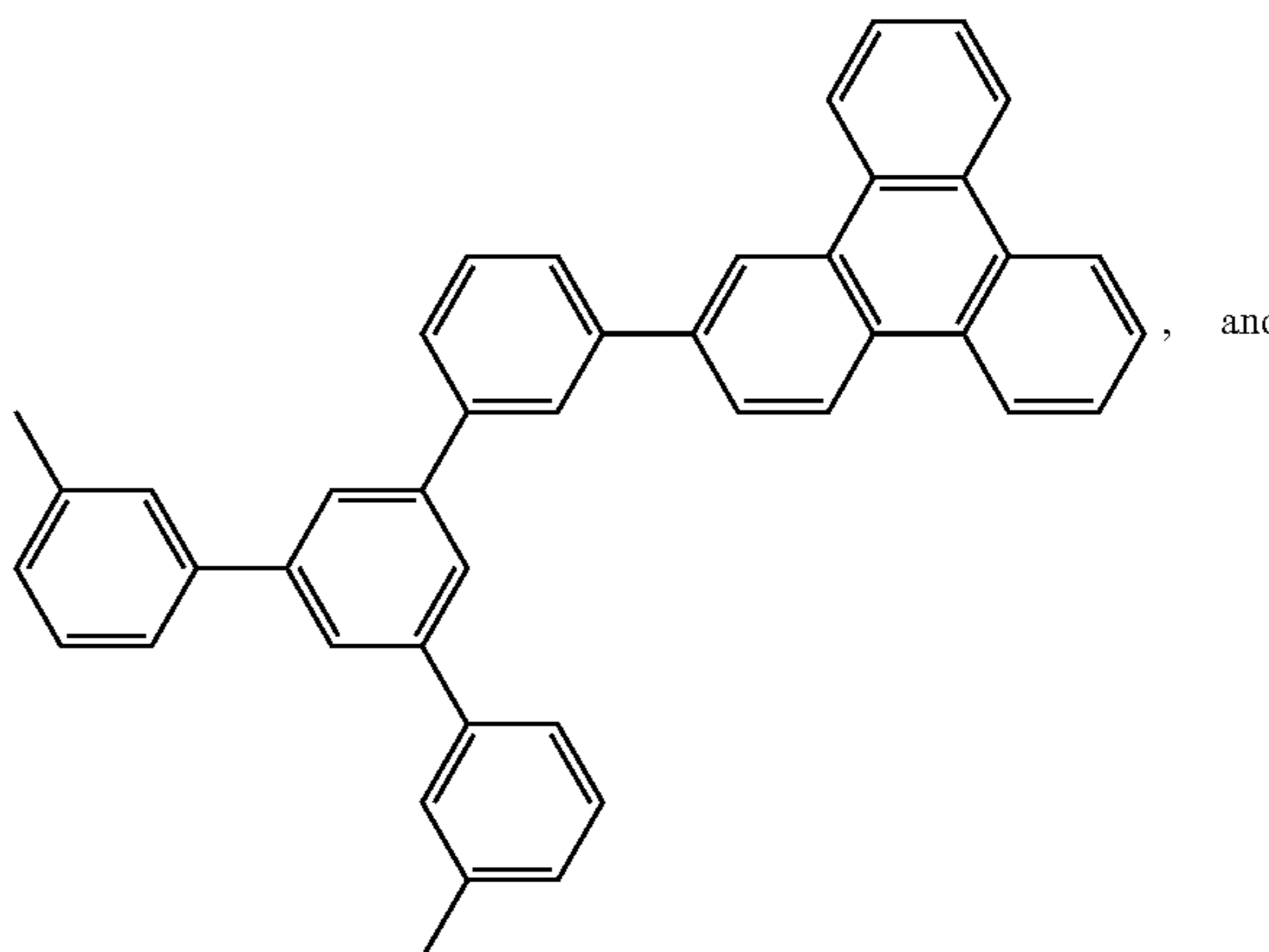
Compound 10
