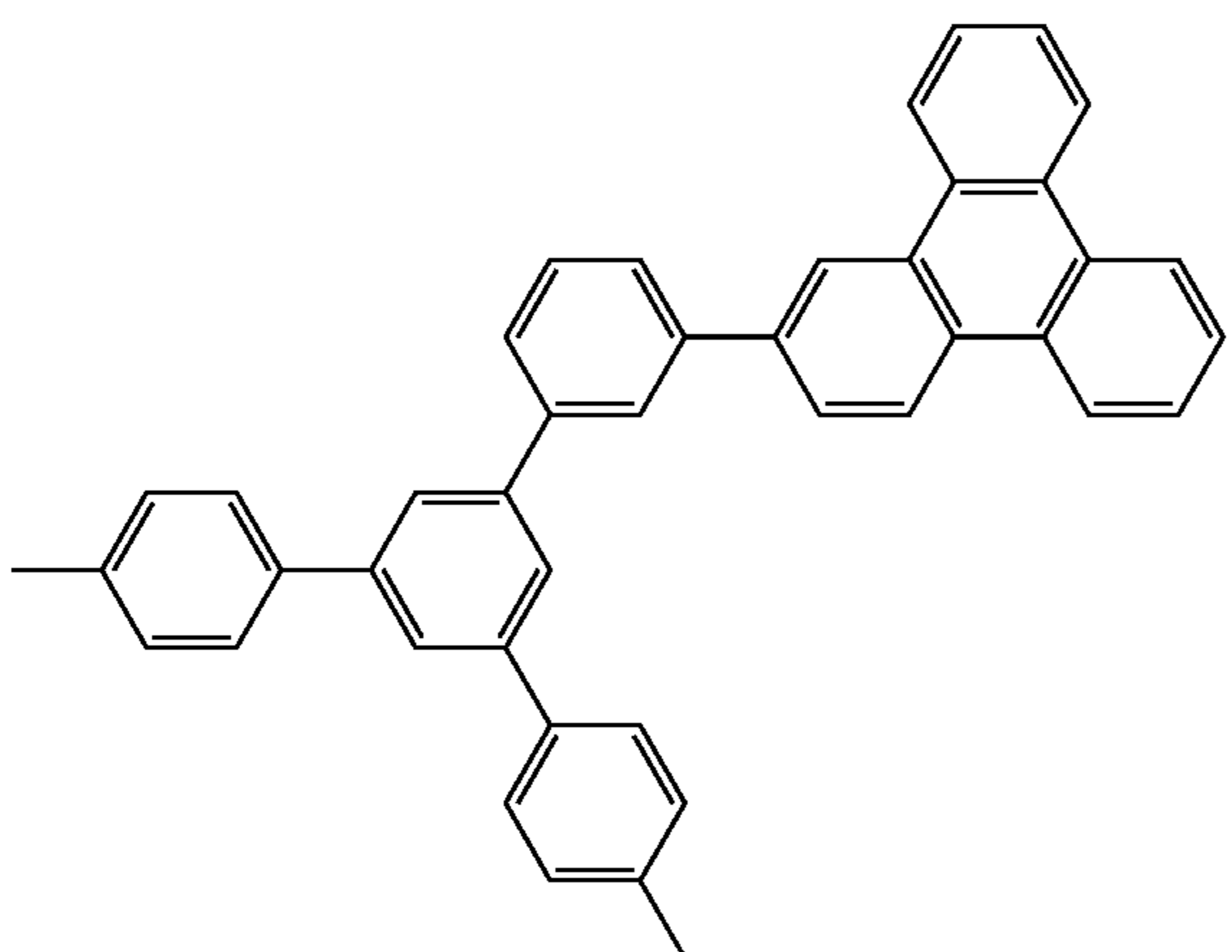
Compound 9
