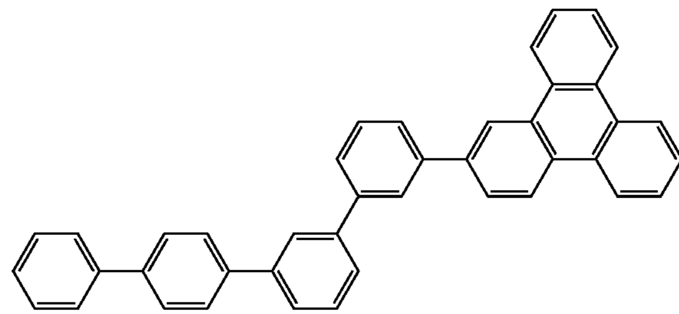
Compound 11
