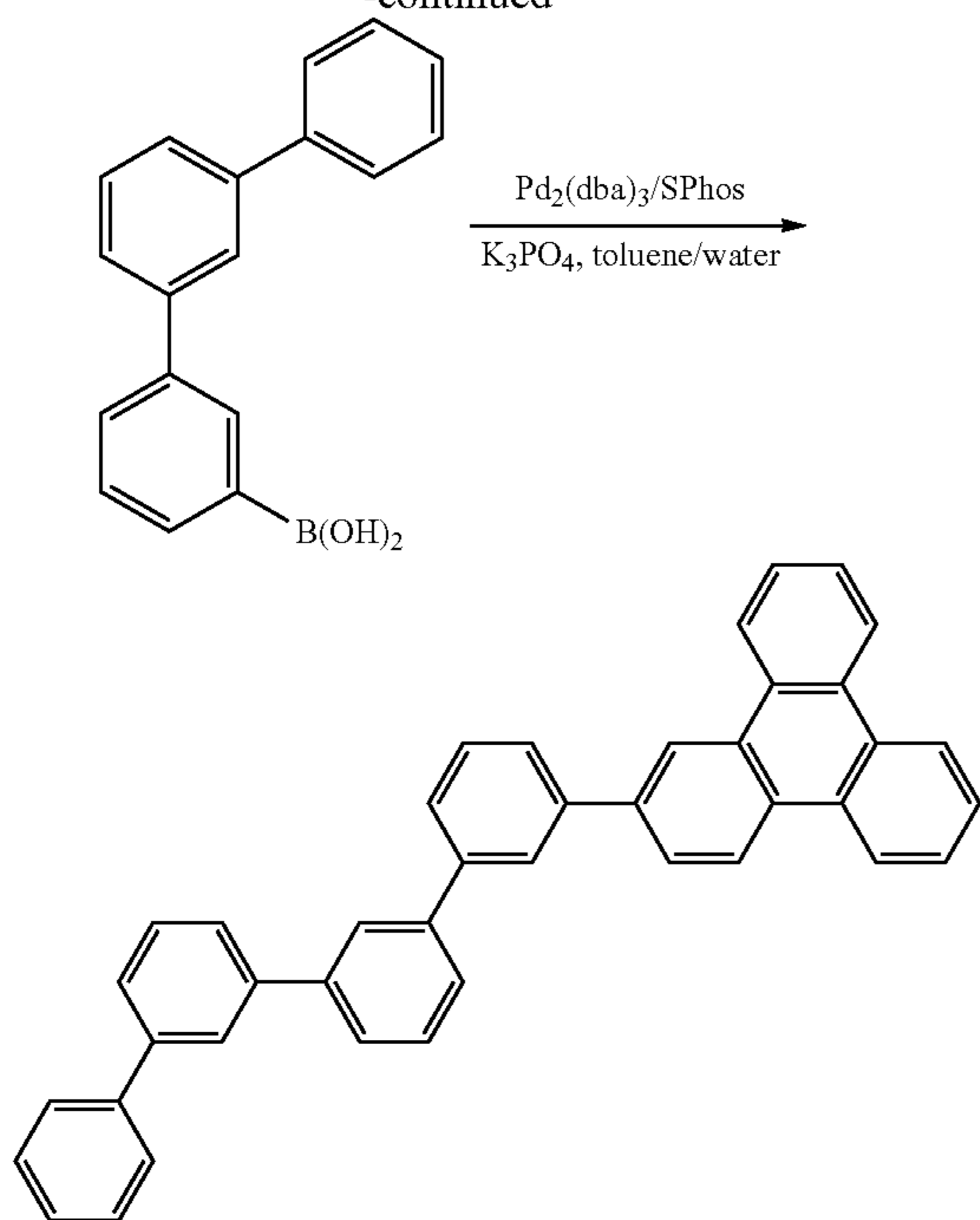
Compound 3
