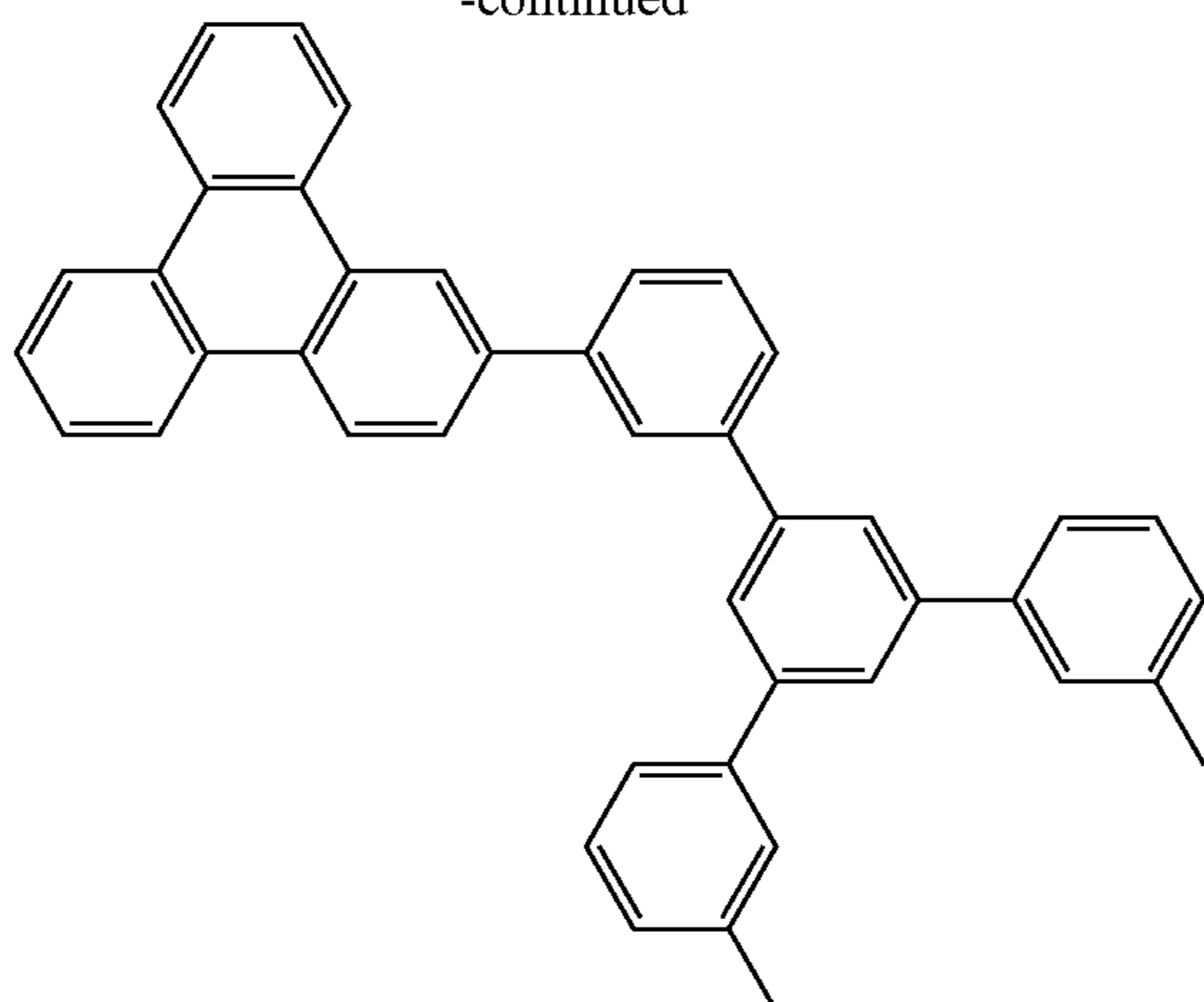
Compound 10
