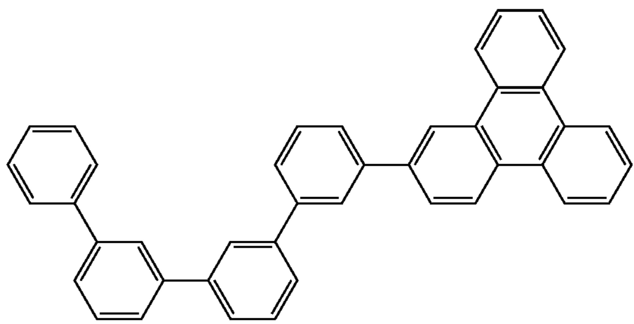
Compound 3
