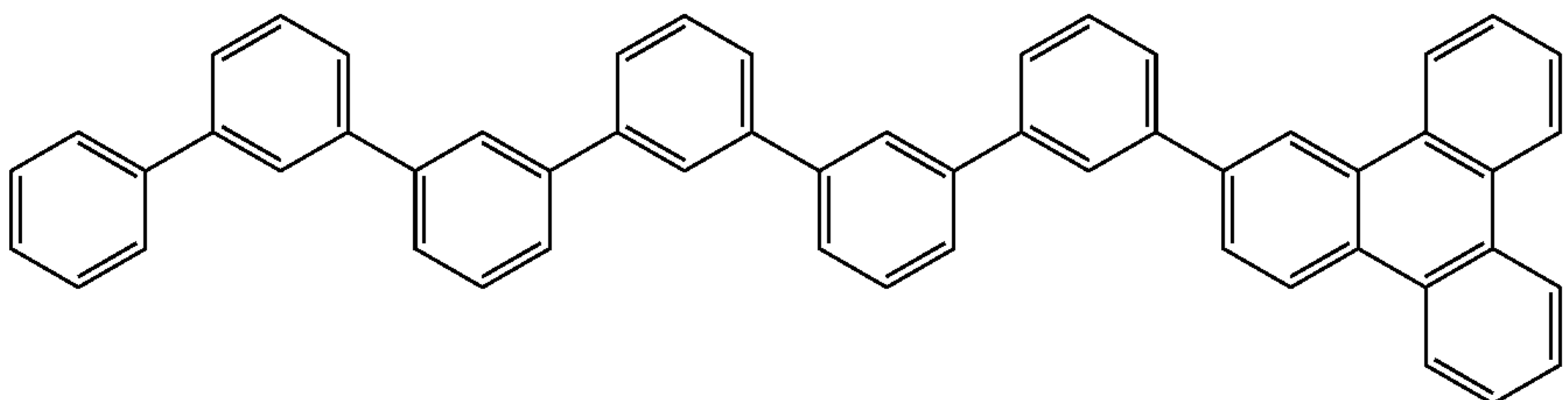
Compound 6
