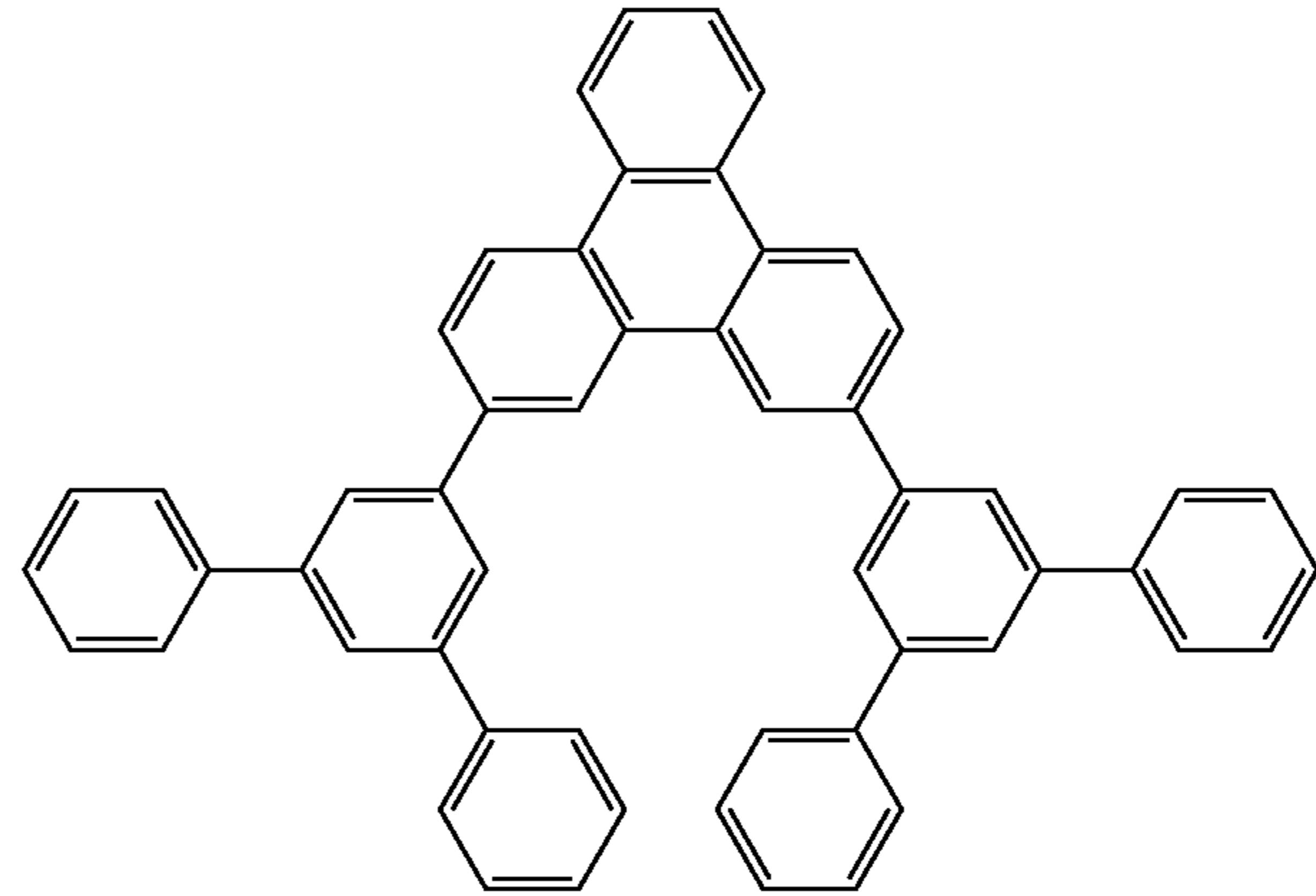
Compound 9
