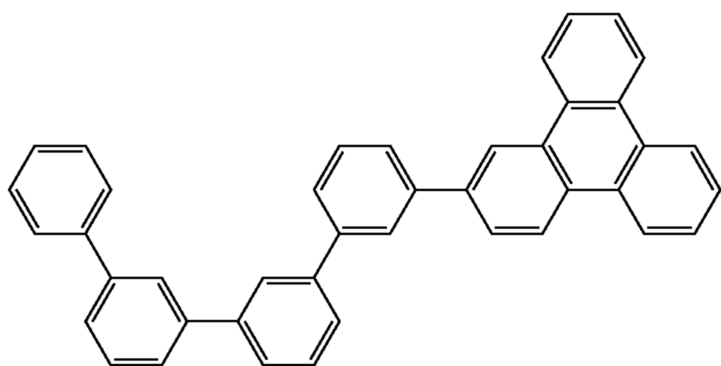
Compound 3
