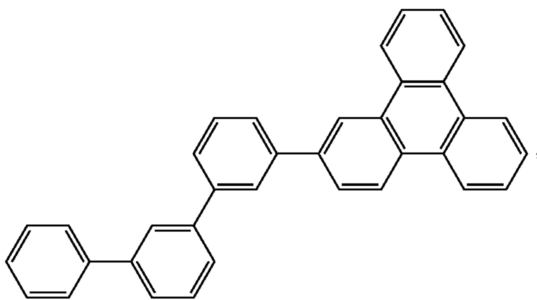
Compound 2
