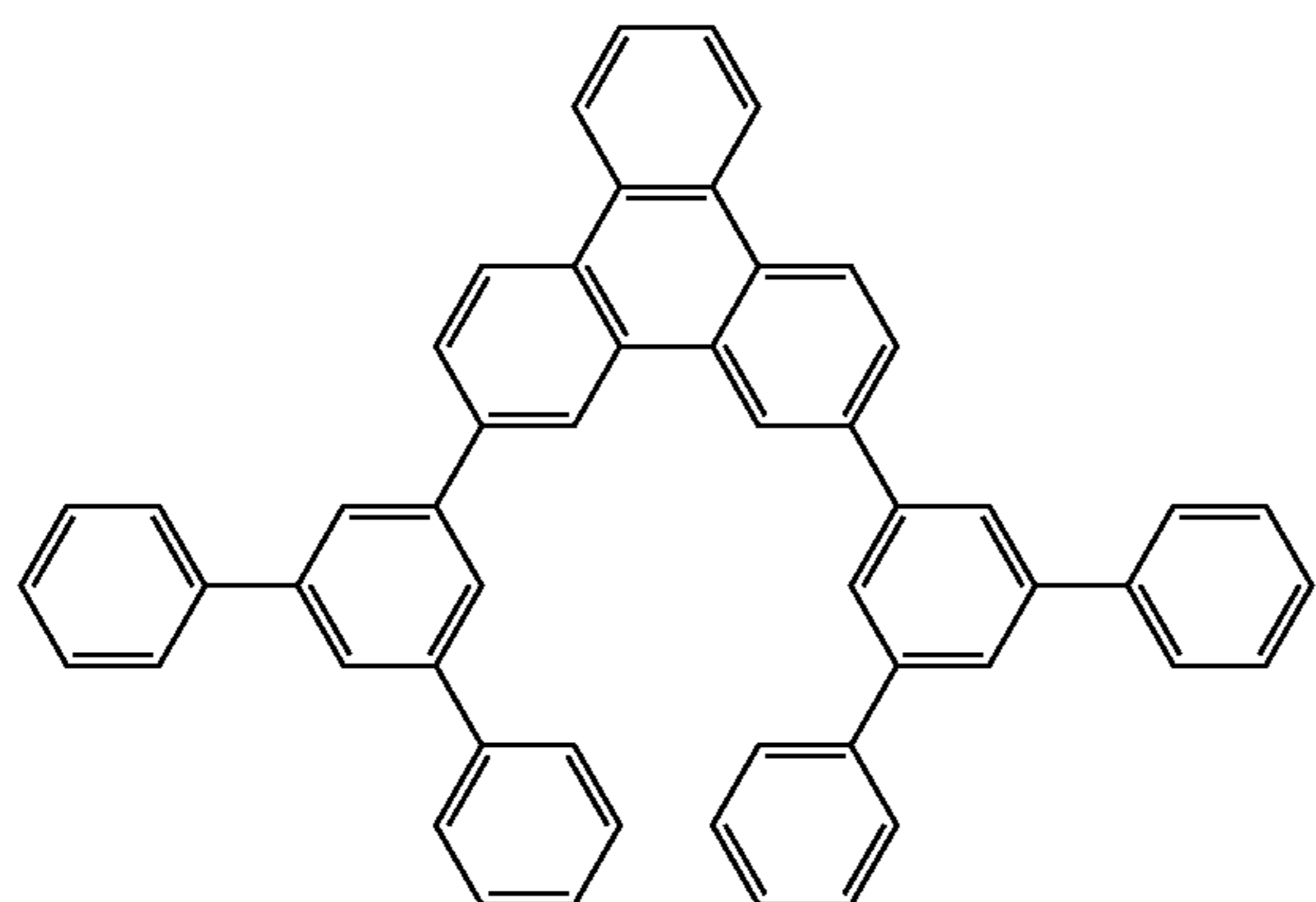
Compound 7
