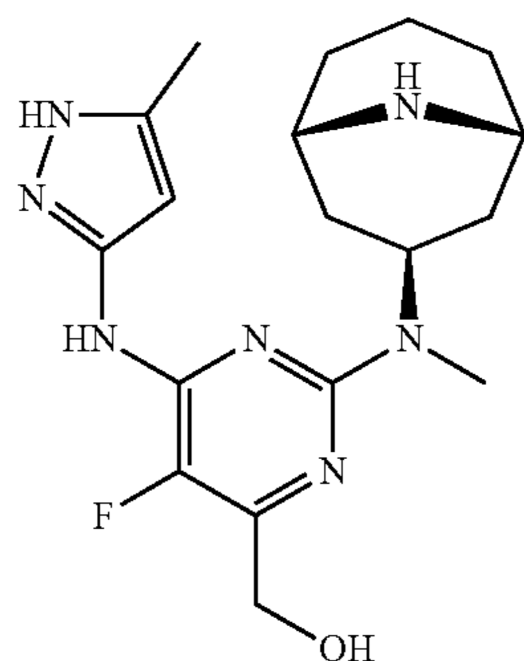
(2-(((1R,3s,5S)-9-azabicyclo[3.3.1]nonan-3-yl)(methyl)amino)-5-fluoro-6-((5-methyl-1H-pyrazol-3-yl)amino)pyrimidin-4-yl)methanol
