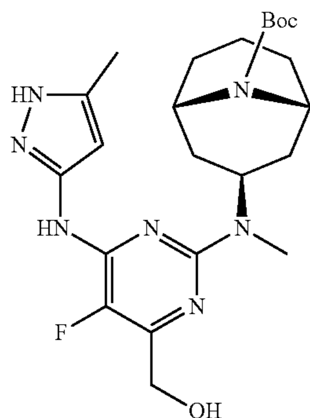
tert-butyl (1R,3s,5S)-3-((5-fluoro-4-(hydroxymethyl)-6-((5-methyl-1H-pyrazol-3-yl)amino)pyrimidin-2-yl)(methyl)amino)-9-azabicyclo[3.3.1]nonane-9-carboxylate
