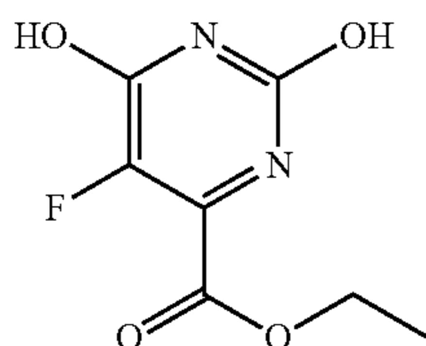
ethyl 5-fluoro-2,6-dihydroxypyrimidine-4-carboxylate
