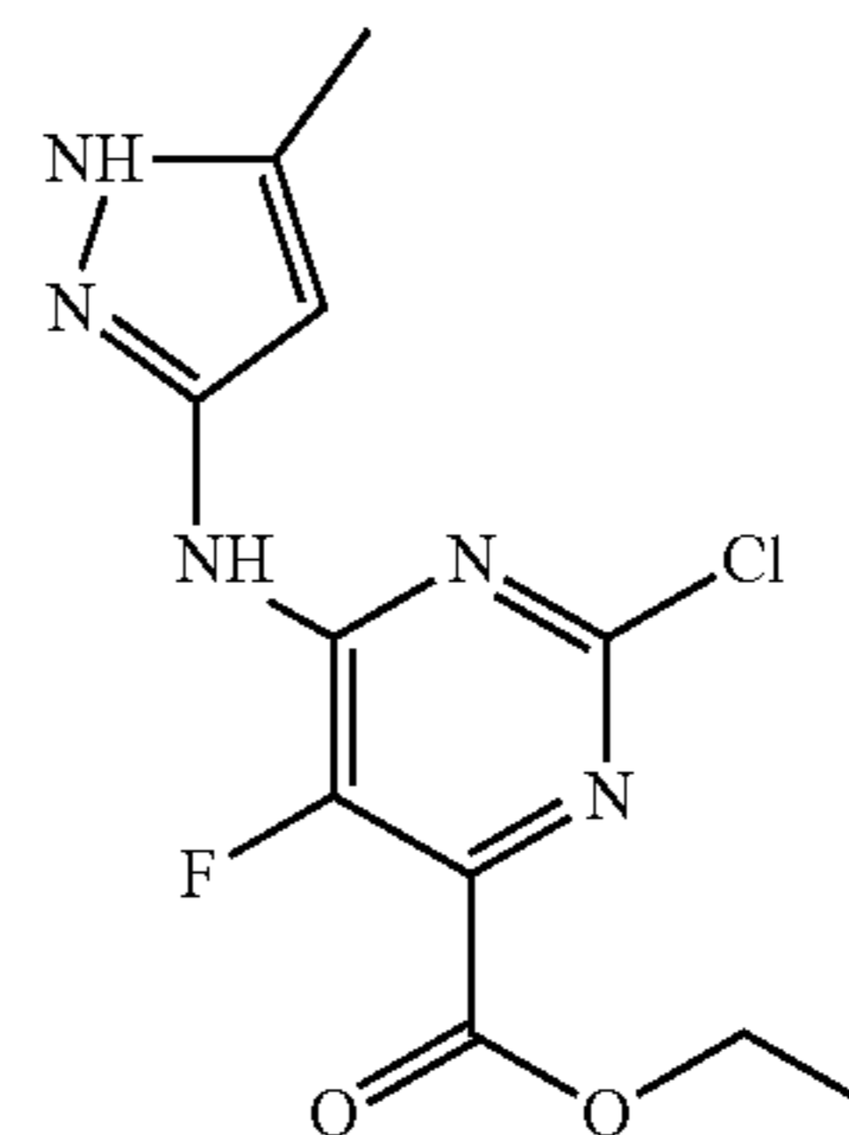
ethyl 2-chloro-5-fluoro-6-((5-methyl-1H-pyrazol-3-yl)amino)pyrimidine-4-carboxylate
