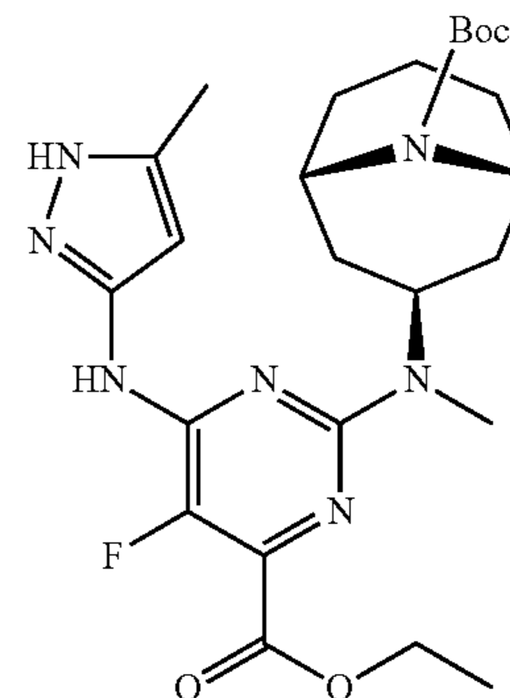
tert-butyl (1R,3s,5S)-3-((4-(ethoxycarbonyl)-5-fluoro-6-((5-methyl-1H-pyrazol-3-yl)amino)pyrimidin-2-yl)(methylamino)-9-azabicyclo[3.3.1]nonane-9-carboxylate
