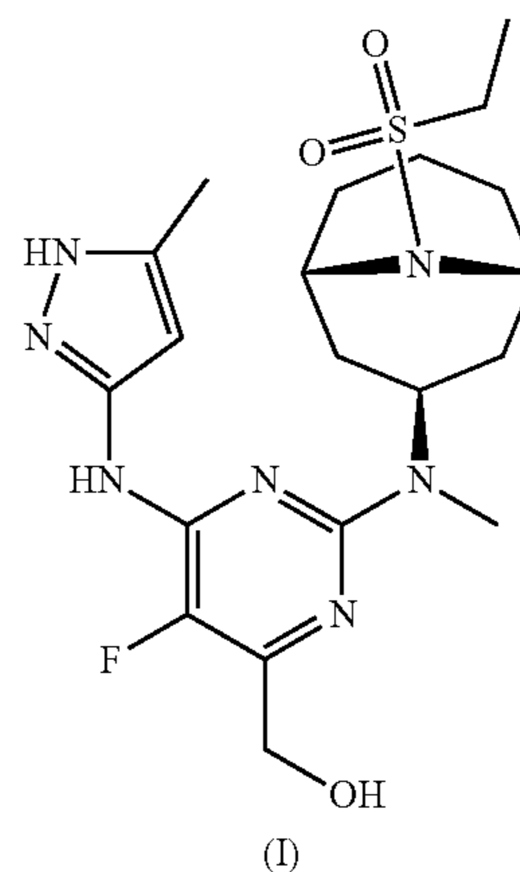
(I) 2-(((1R,3s,5S)-9-(ethylsulfonyl)-9-azabicyclo[3.3.1]nonan-3-yl)(methyl)amino)-5-fluoro-6-((5-methyl-1H-pyrazol-3-yl)amino)pyrimidin-4-yl)methanol
