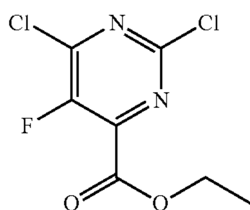
ethyl 2,6-dichloro-5-fluoropyrimidine-4-carboxylate
