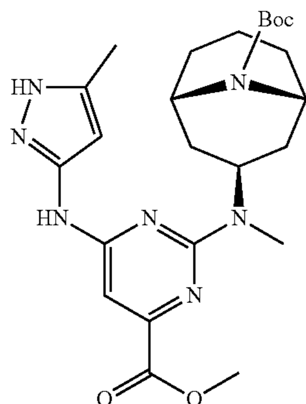
tert-butyl (1R,3s,5S)-3-((4-methoxycarbonyl-6-((5-methyl-1H-pyrazol-3-yl)amino)pyrimidin-2-yl)(methyl)amino)-9-azabicyclo[3.3.1]nonane-9-carboxylate
