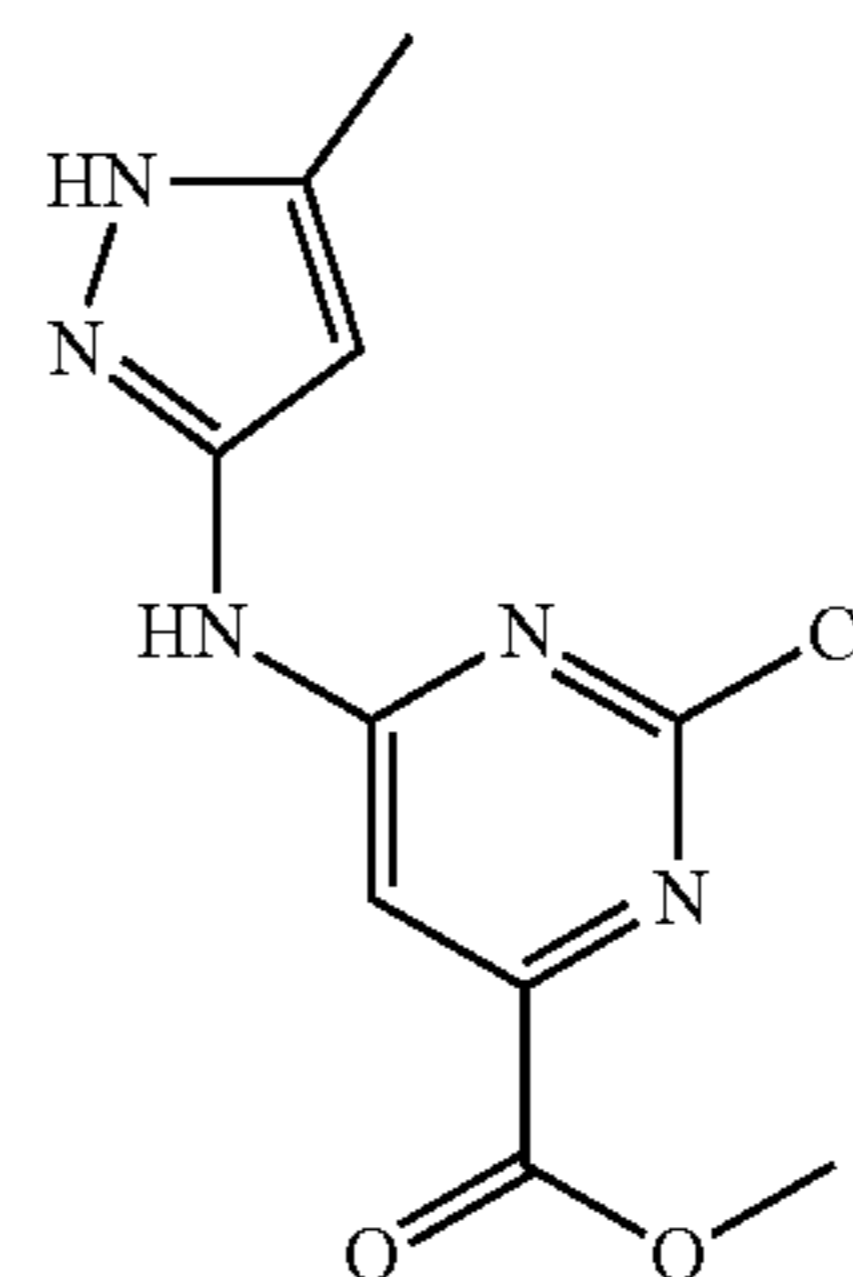
methyl 2-chloro-6-((5-methyl-1H-pyrazol-3-yl)amino)pyrimidine-4-carboxylate
