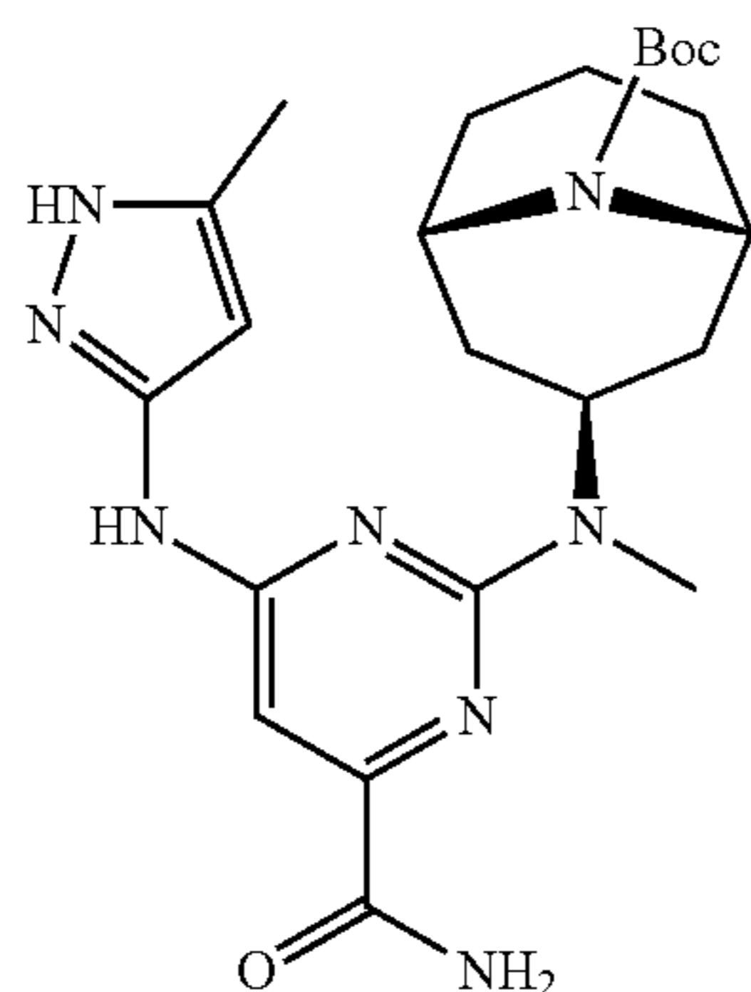
tert-butyl (1R,3s,5S)-3-((4-carbamoyl-6-((5-methyl-1H-pyrazol-3-yl)amino)pyrimidin-2-yl)(methyl)amino)-9-azabicyclo[3.3.1]nonane-9-carboxylate
