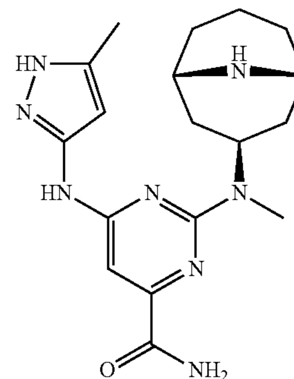
2-(((1R,3s,5S)-9-azabicyclo[3.3.1]nonan-3-yl)(methyl)amino)-6-((5-methyl-1H-pyrazol-3-yl)amino)pyrimidine-4-carboxamide
