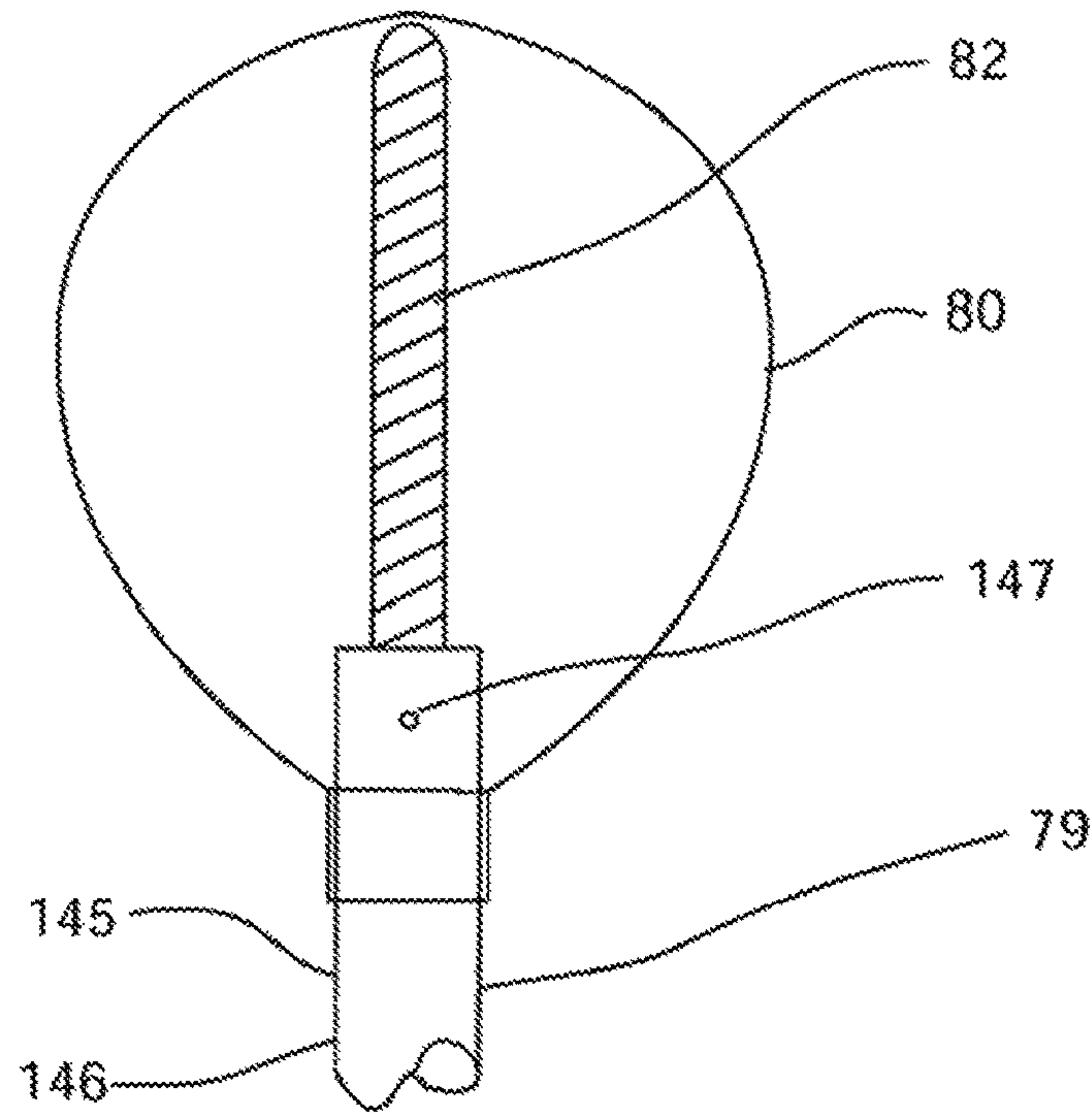
View D-D
