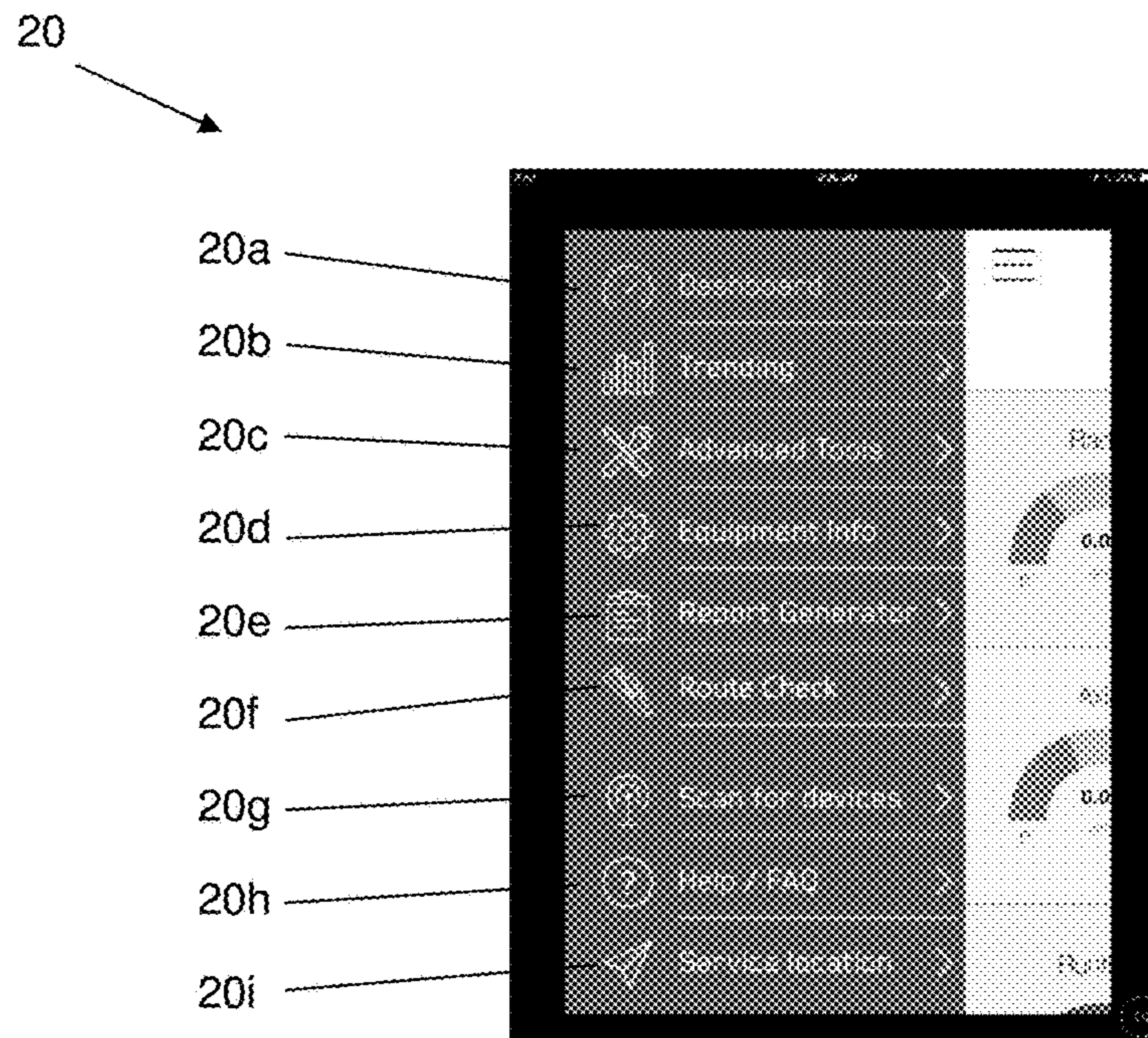
Figure 3B: Access Screen
