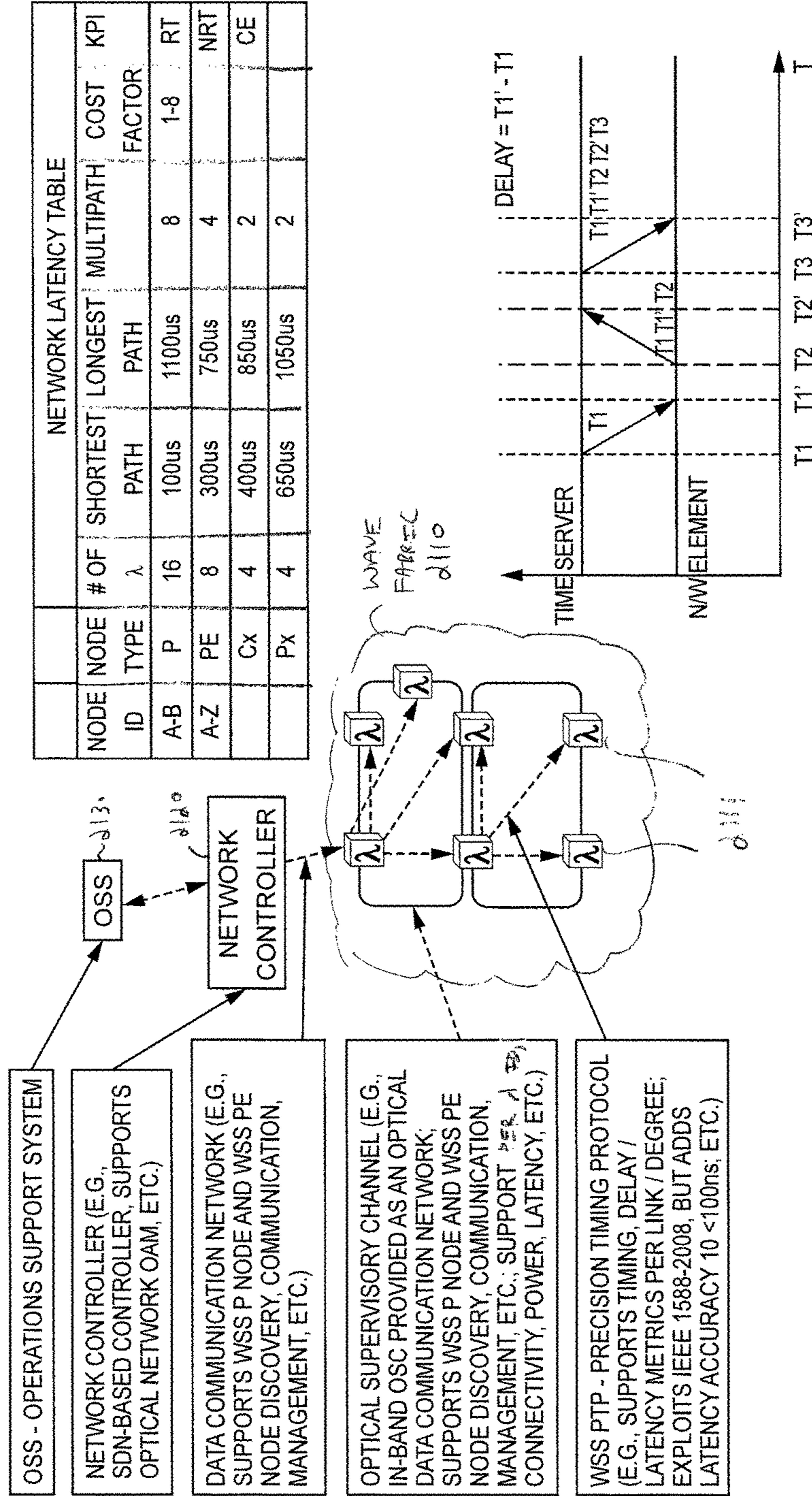
IEEE 1588 SYNCHRONIZATION MECHANISM AND DELAY CALCULATION
