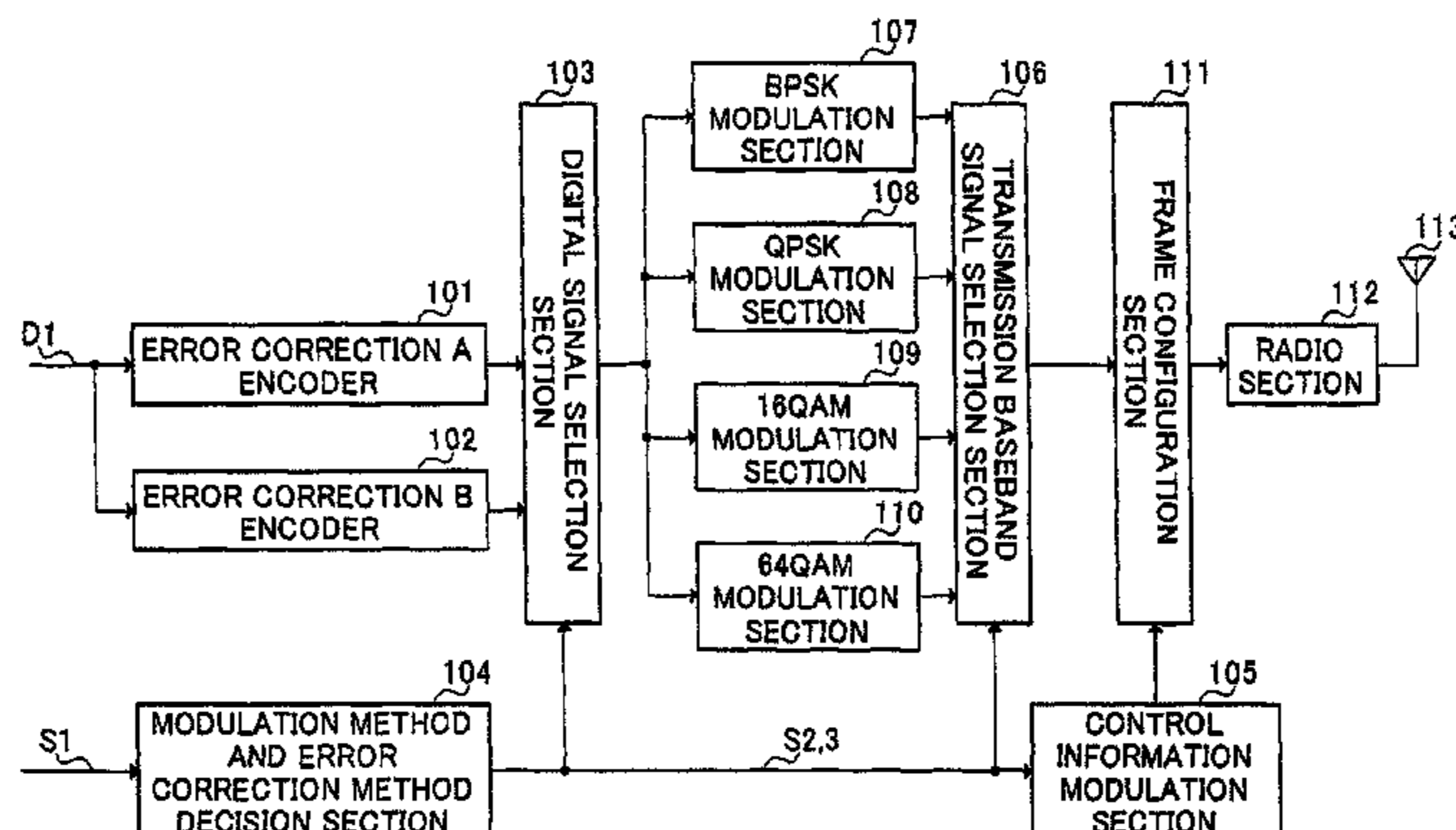
100 TRANSMITTING APPARATUS
