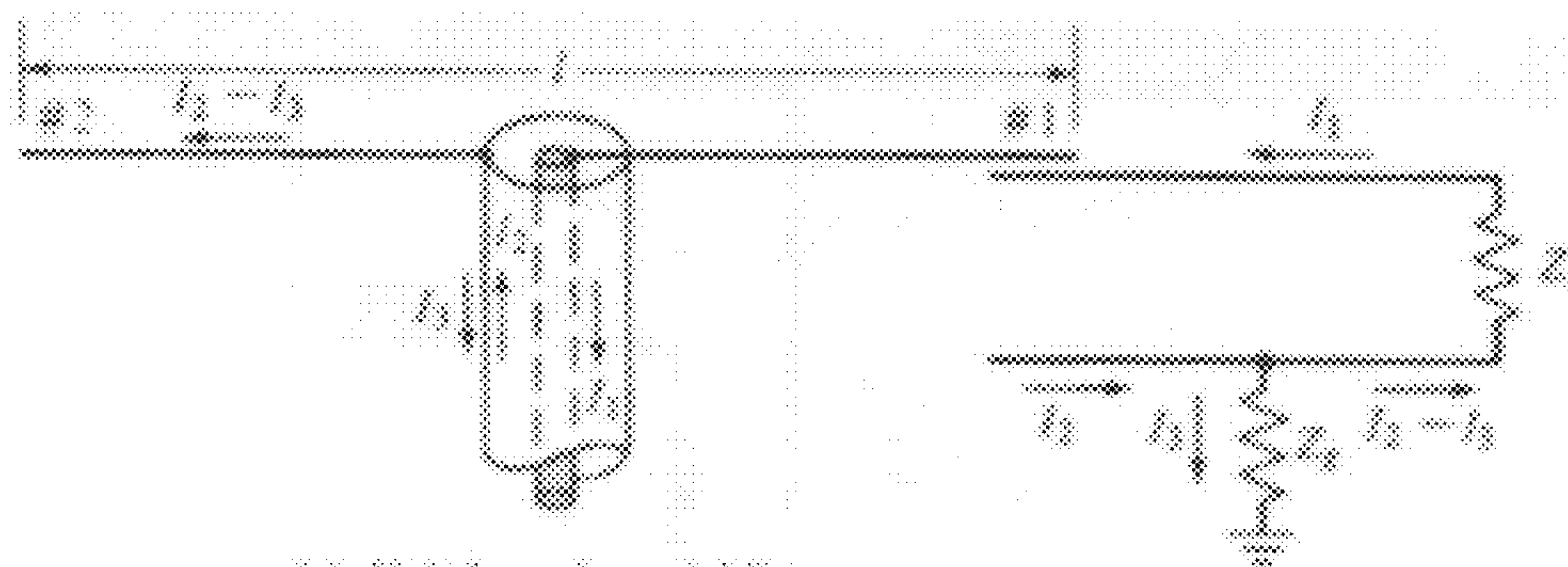
(a) Unbalanced coaxial line
