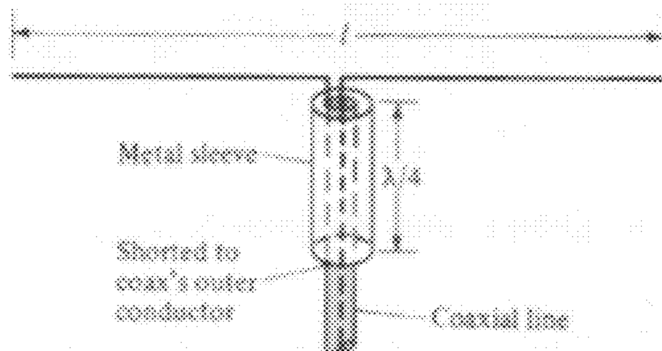
(b) Bazonka balun (1 : 1)
