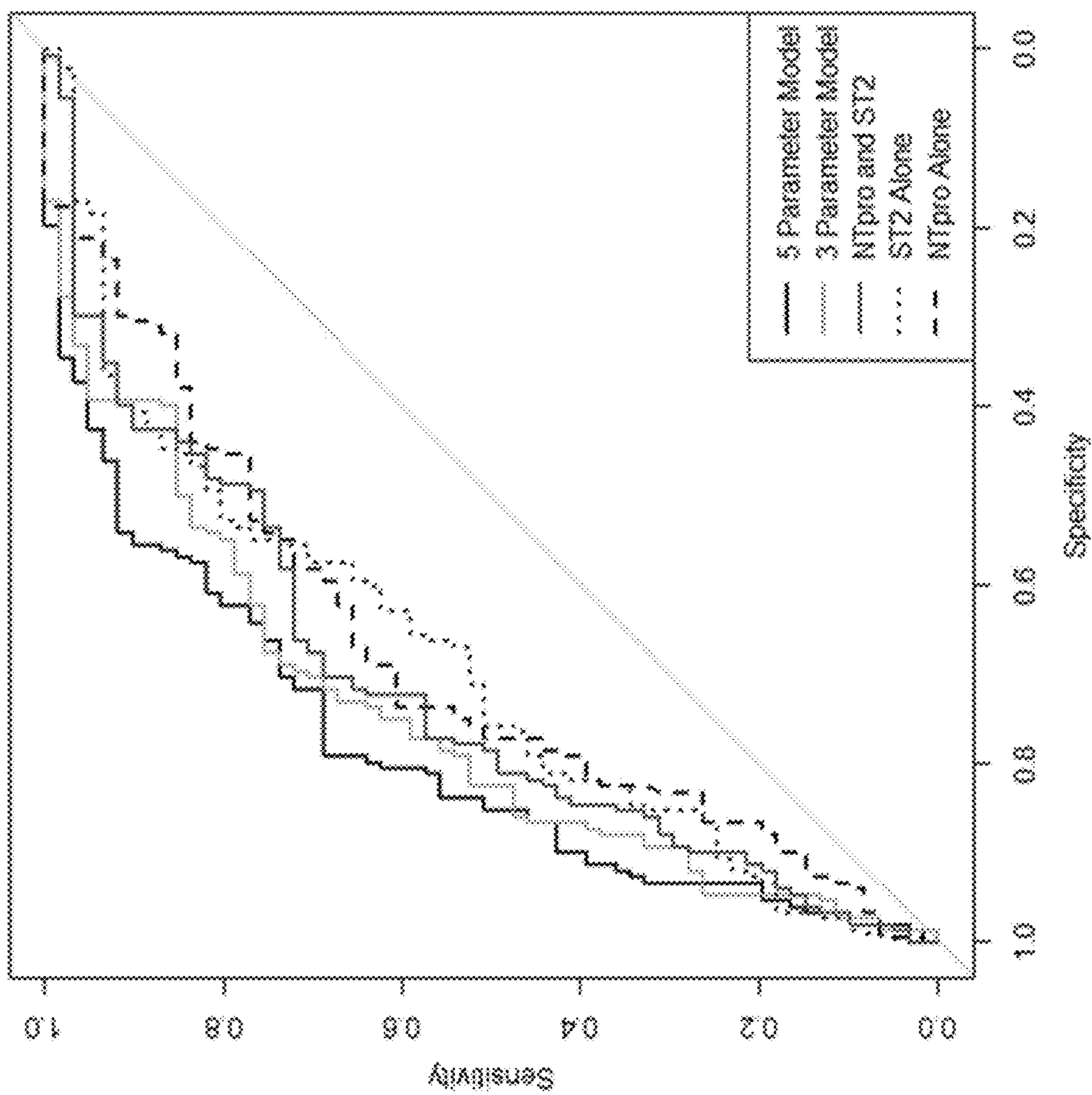
Fig. 54 ROC Curves
