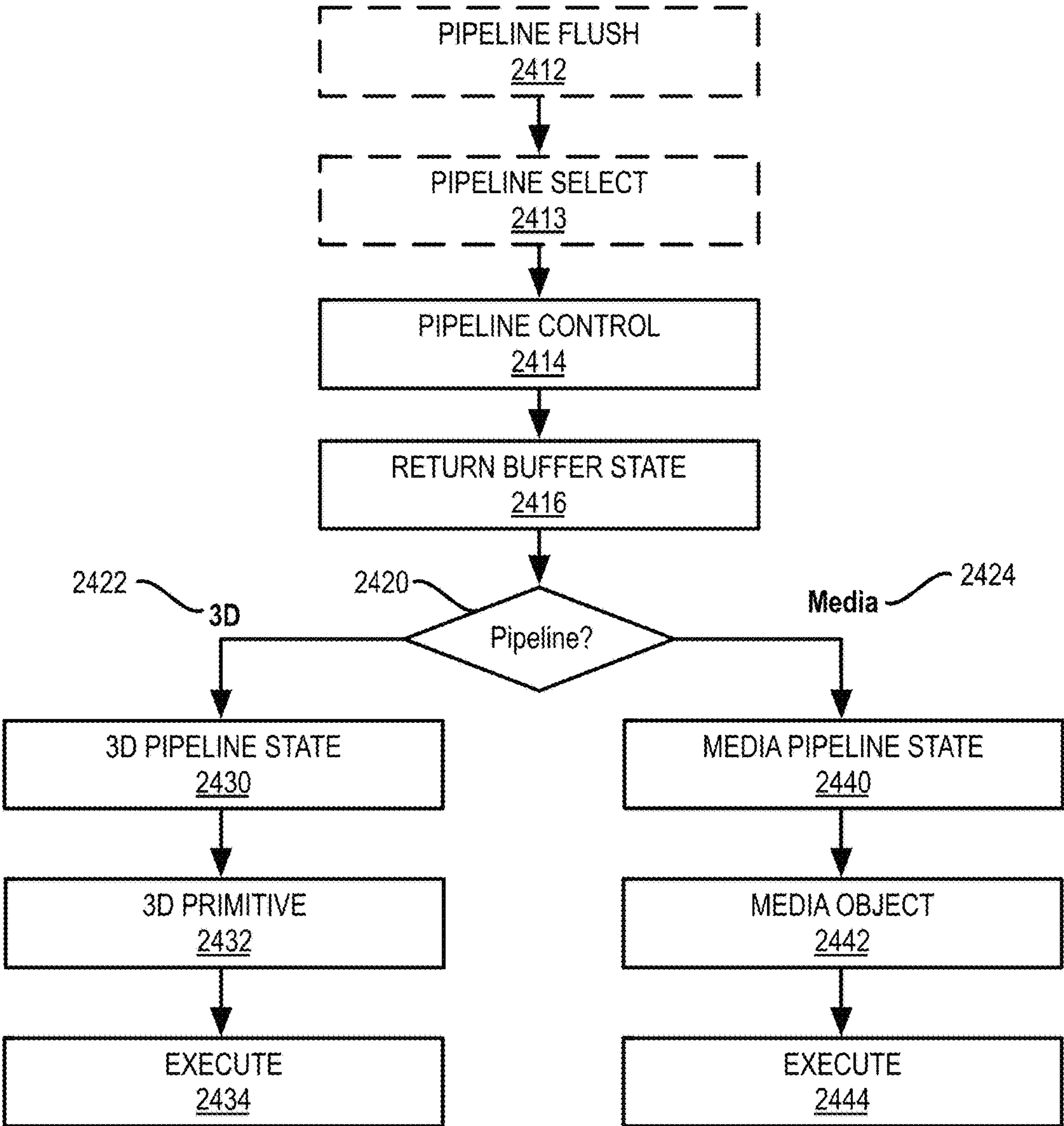
FIG. 17B GRAPHICS PROCESSOR COMMAND SEQUENCE 2410
