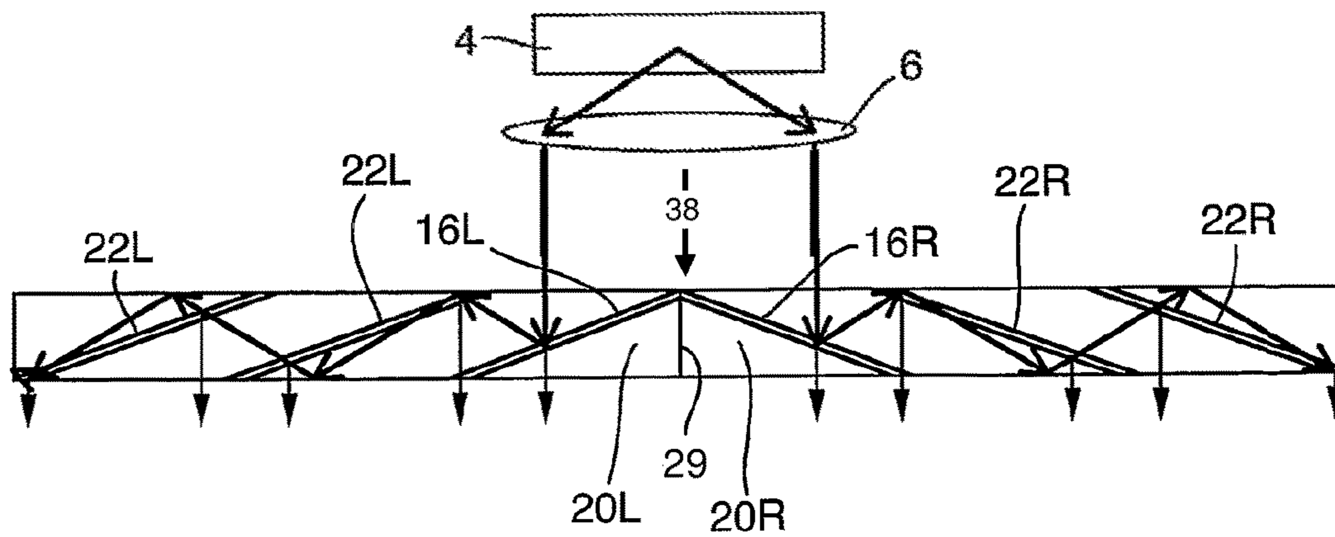
FIG. 4C PRIOR ART
