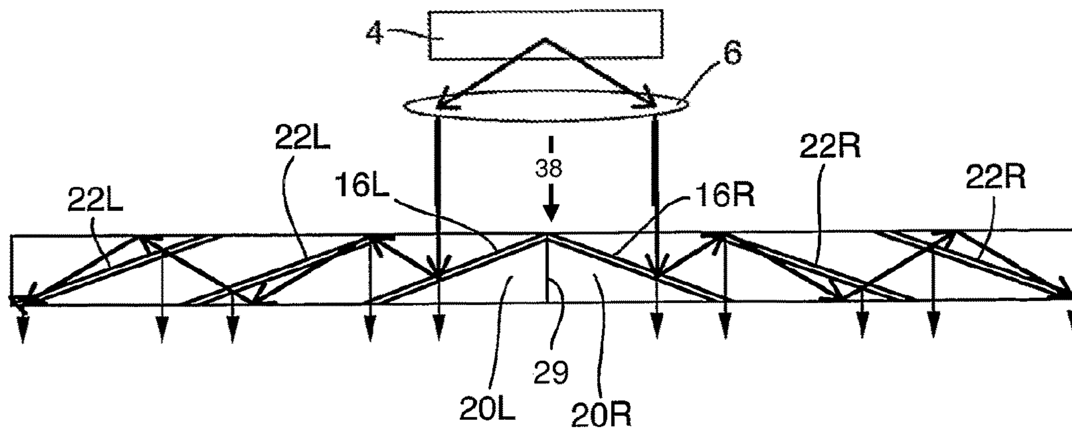
FIG. 4C PRIOR ART
