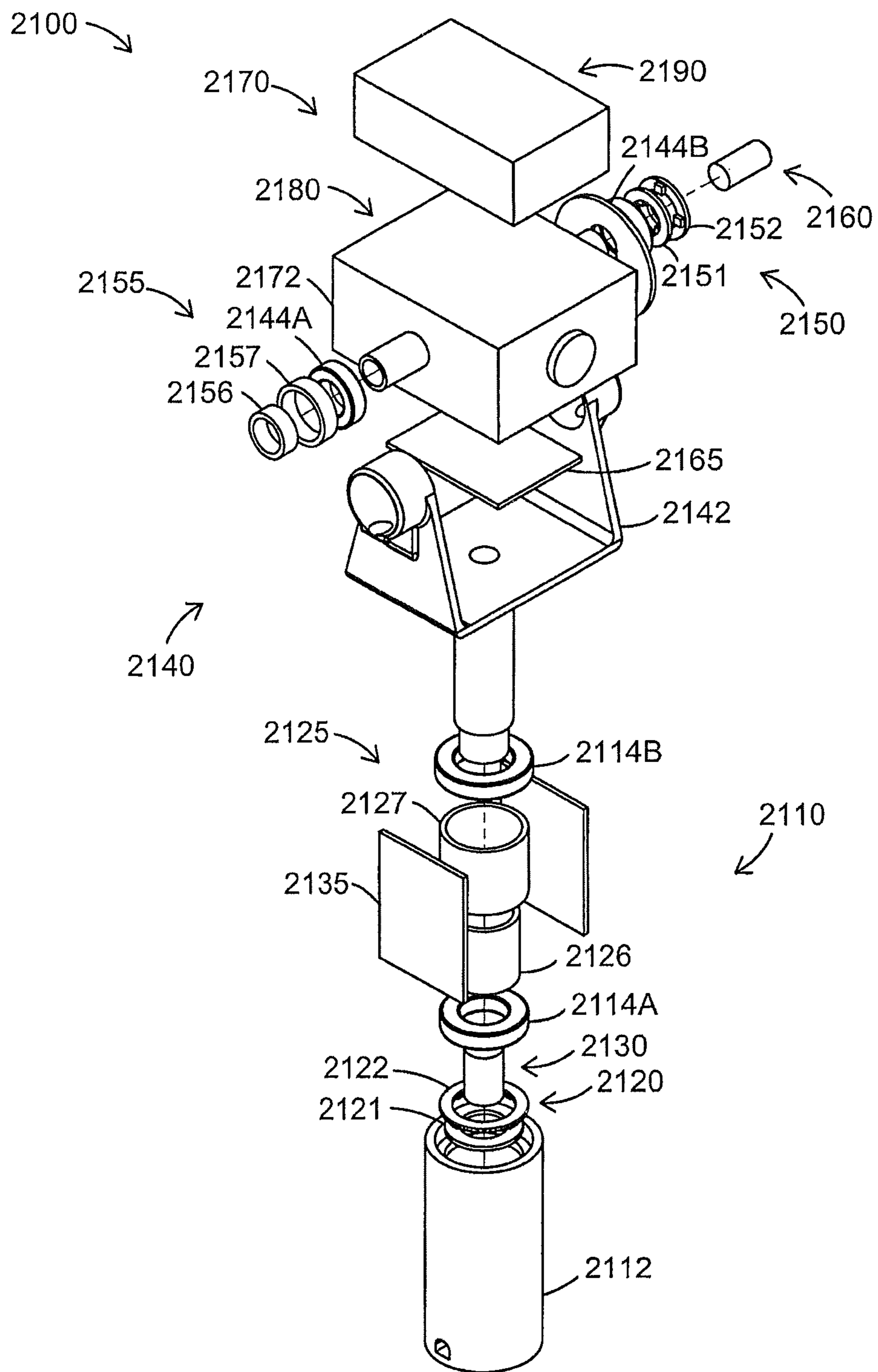
PRIOR ART FIGURE 9
